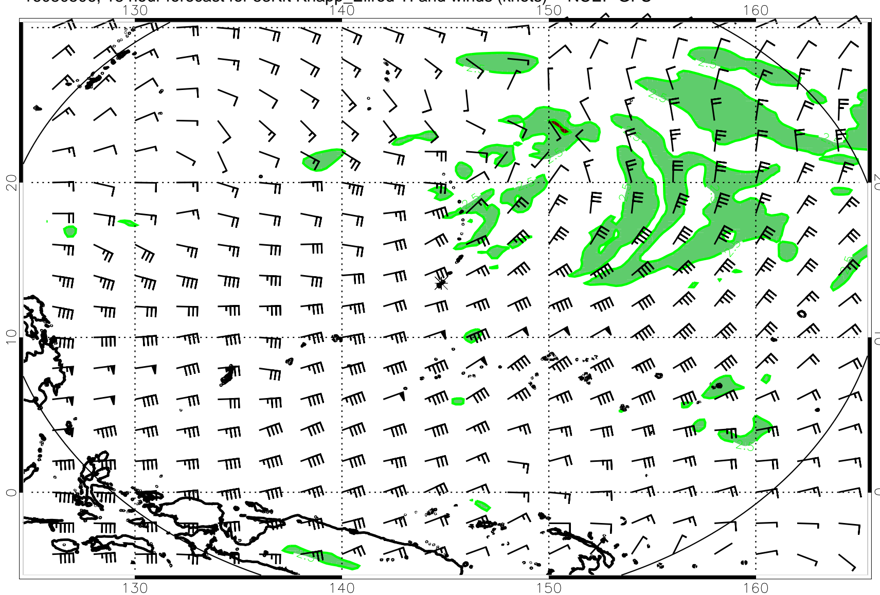
16080506, 18 hour forecast for 53Kft Knapp_Ellrod TI and winds (knots) -- NCEP GFS
