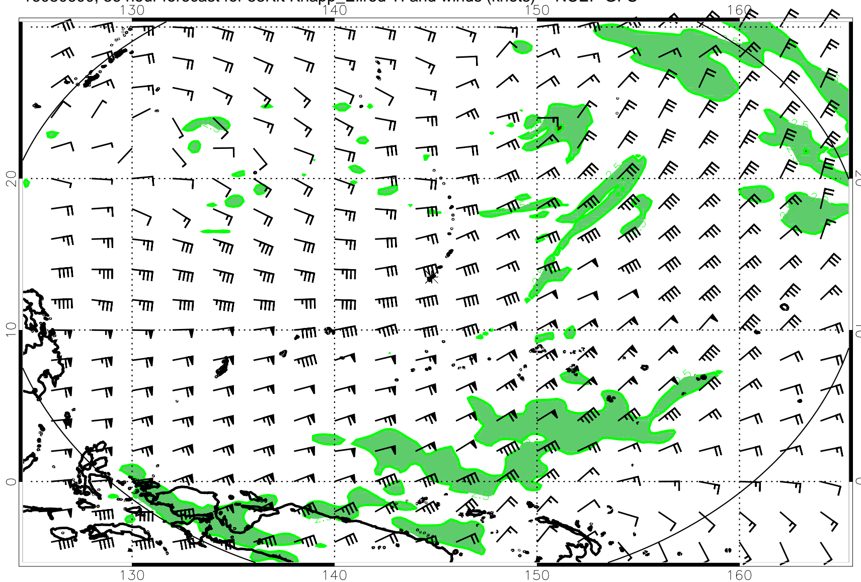
16080600, 36 hour forecast for 53Kft Knapp_Ellrod TI and winds (knots) -- NCEP GFS
