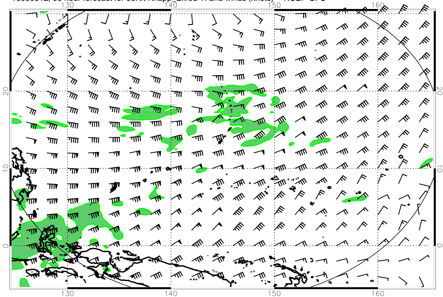
16080812, 96 hour forecast for 53Kft Knapp_Ellrod TI and winds (knots) -- NCEP GFS
