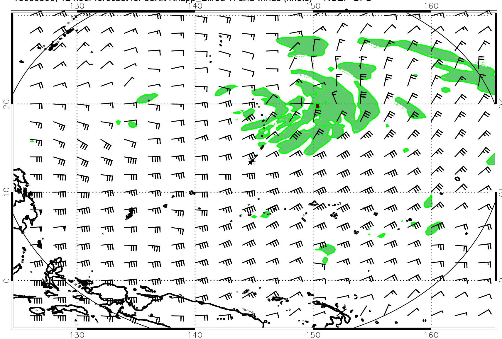
16080500, 12 hour forecast for 53Kft Knapp_Ellrod TI and winds (knots) -- NCEP GFS
