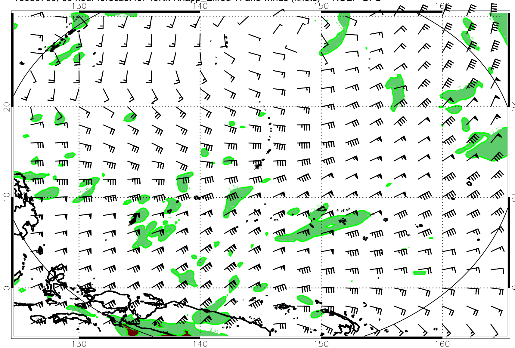
16080700, 60 hour forecast for 49Kft Knapp_Ellrod TI and winds (knots) -- NCEP GFS
