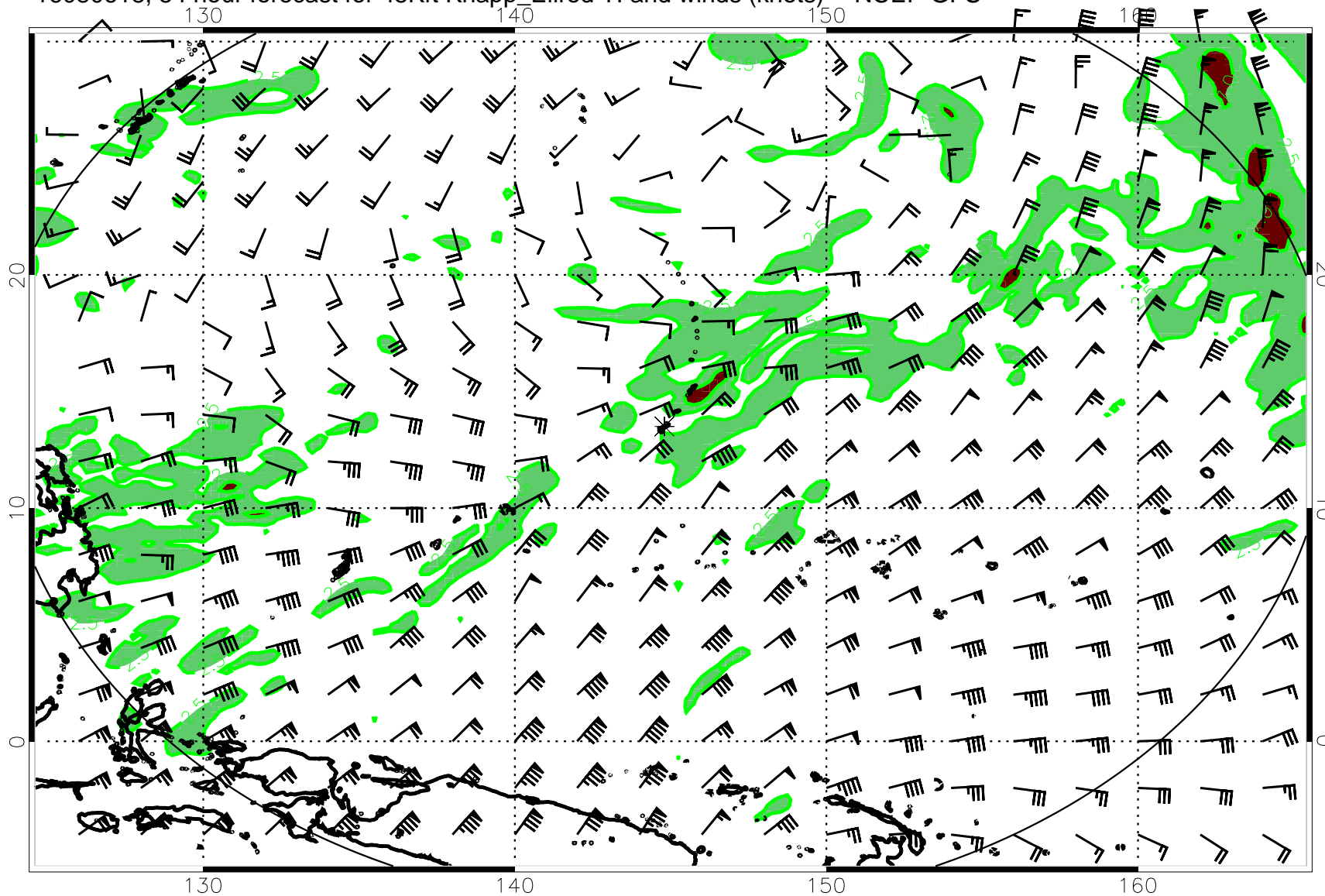
16080618, 54 hour forecast for 45Kft Knapp_Ellrod TI and winds (knots) -- NCEP GFS
