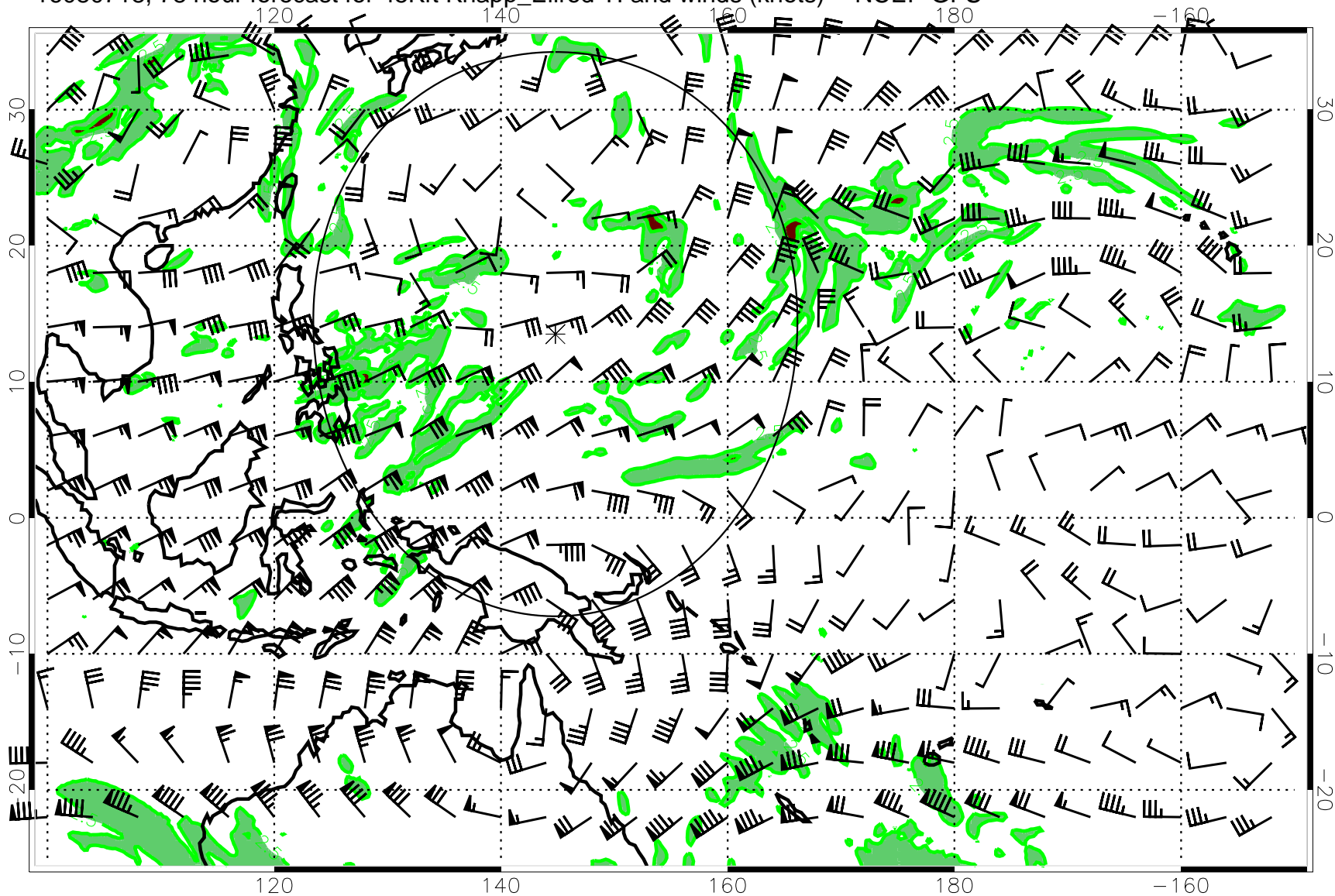
16080718, 78 hour forecast for 45Kft Knapp_Ellrod TI and winds (knots) -- NCEP GFS
