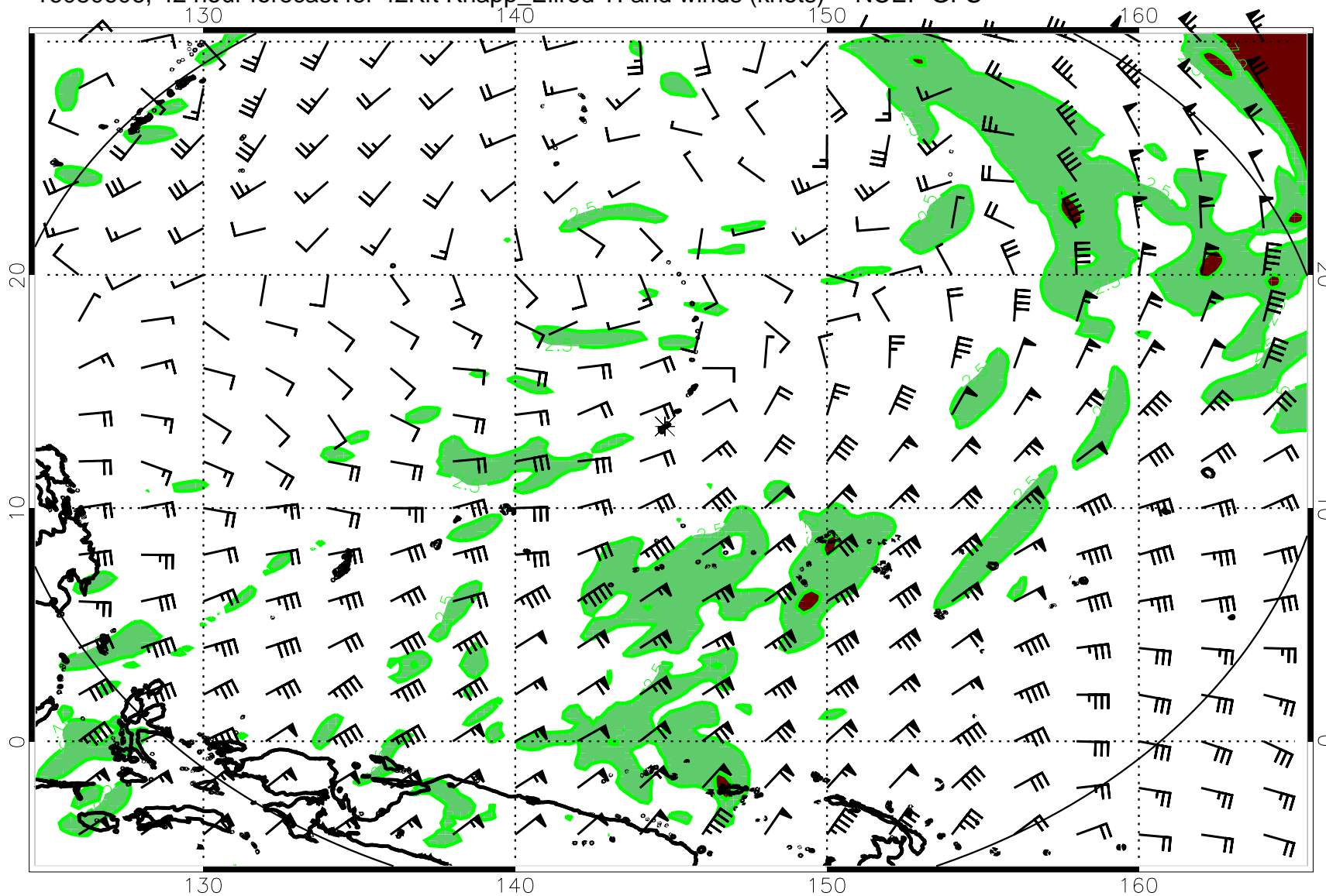
16080606, 42 hour forecast for 42Kft Knapp_Ellrod TI and winds (knots) -- NCEP GFS
