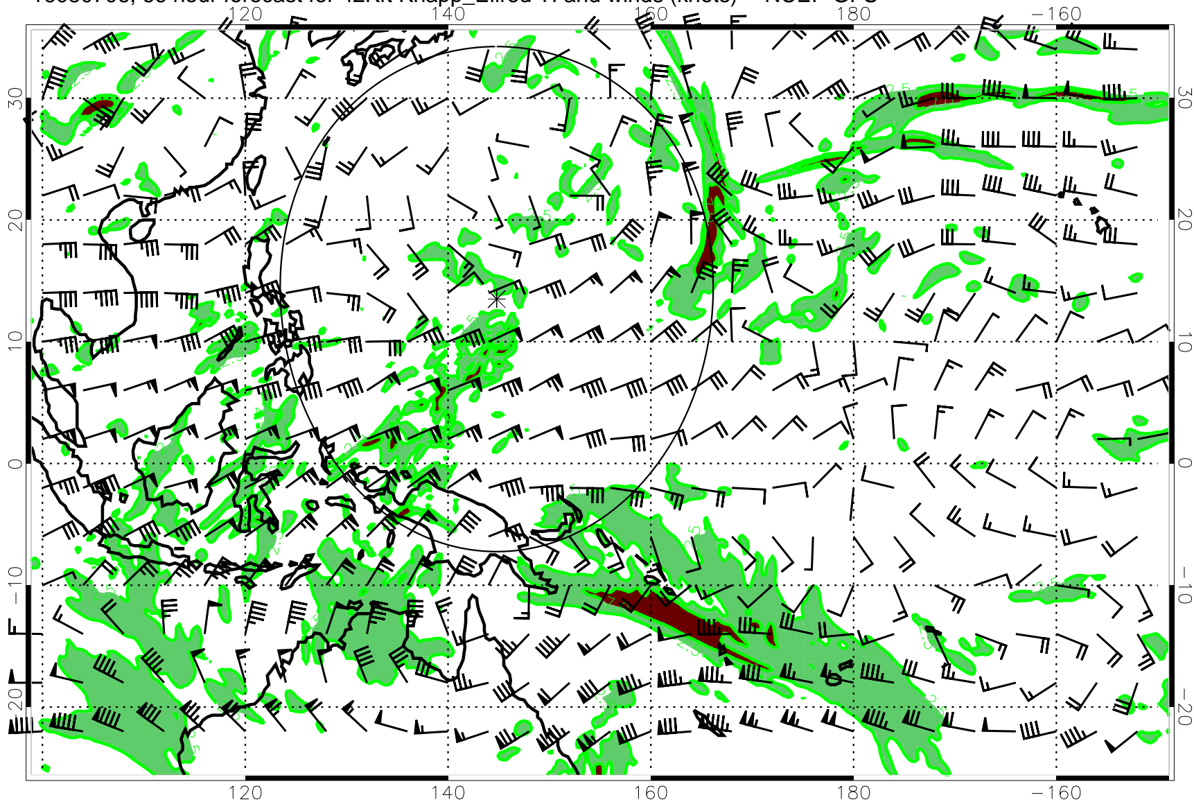
16080706, 66 hour forecast for 42Kft Knapp_Ellrod TI and winds (knots) -- NCEP GFS
