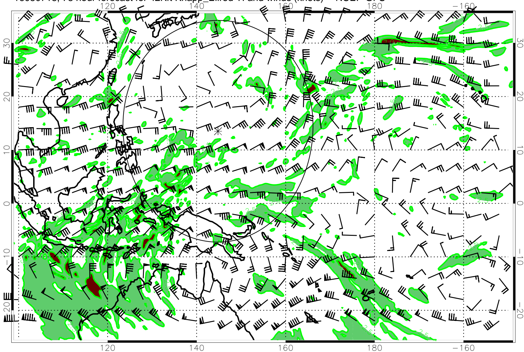
16080718, 78 hour forecast for 42Kft Knapp_Ellrod TI and winds (knots) -- NCEP GFS
