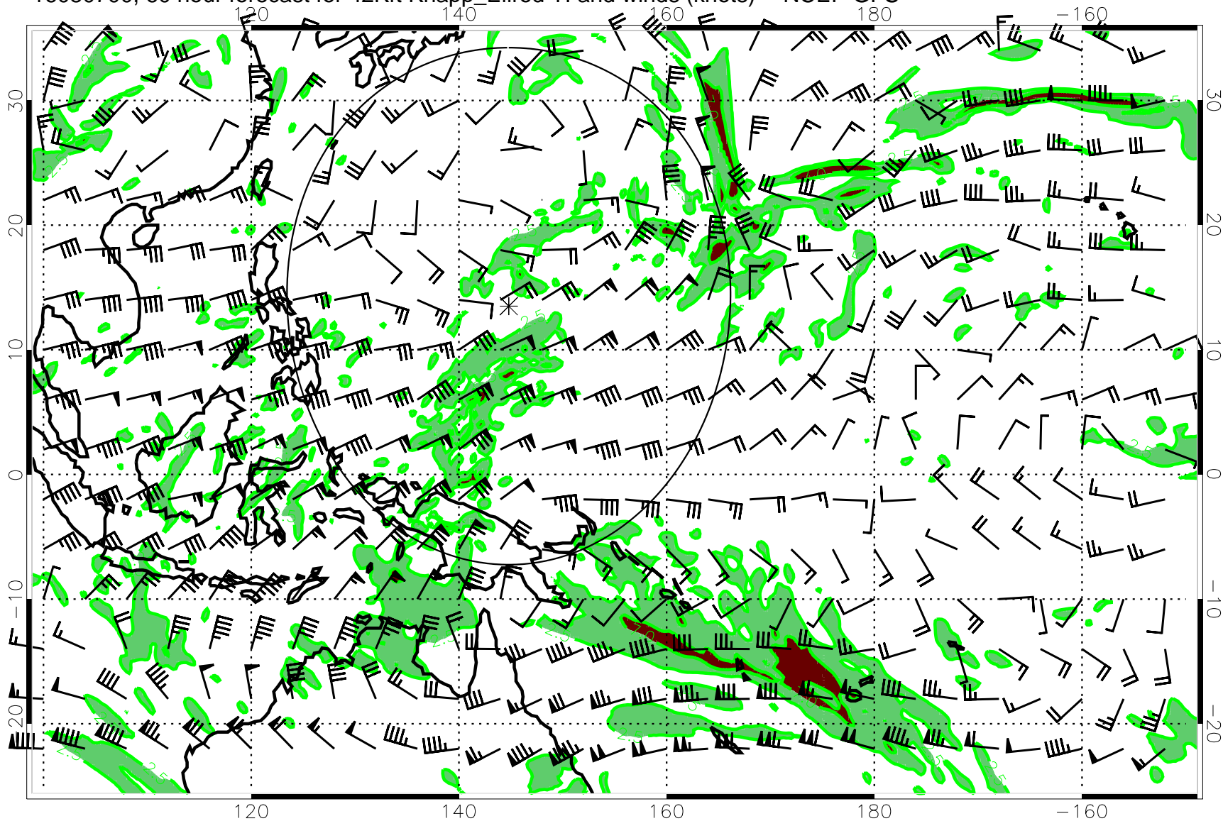
16080700, 60 hour forecast for 42Kft Knapp_Ellrod TI and winds (knots) -- NCEP GFS
