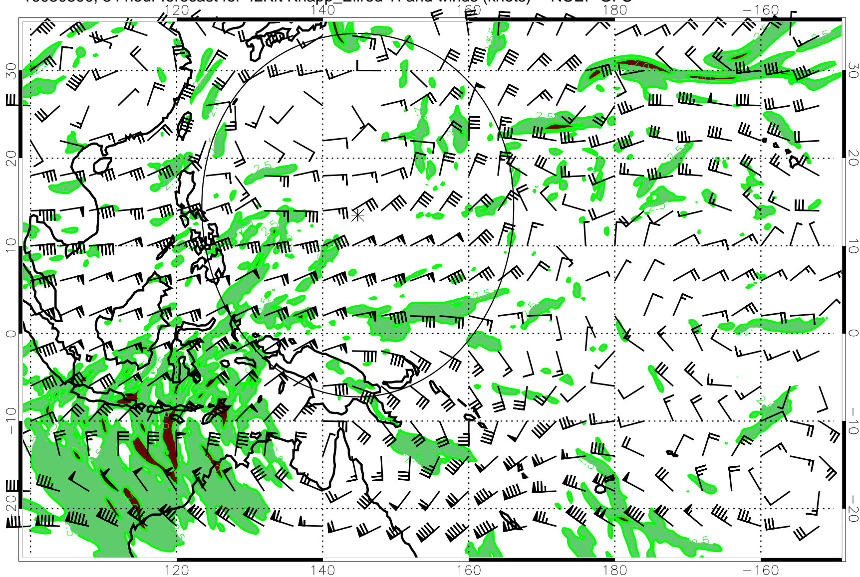
16080800, 84 hour forecast for 42Kft Knapp_Ellrod TI and winds (knots) -- NCEP GFS
