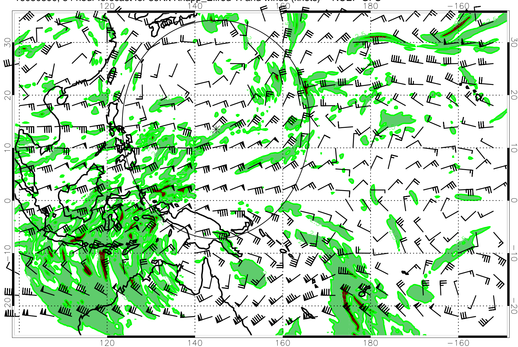
16080800, 84 hour forecast for 39Kft Knapp_Ellrod TI and winds (knots) -- NCEP GFS
