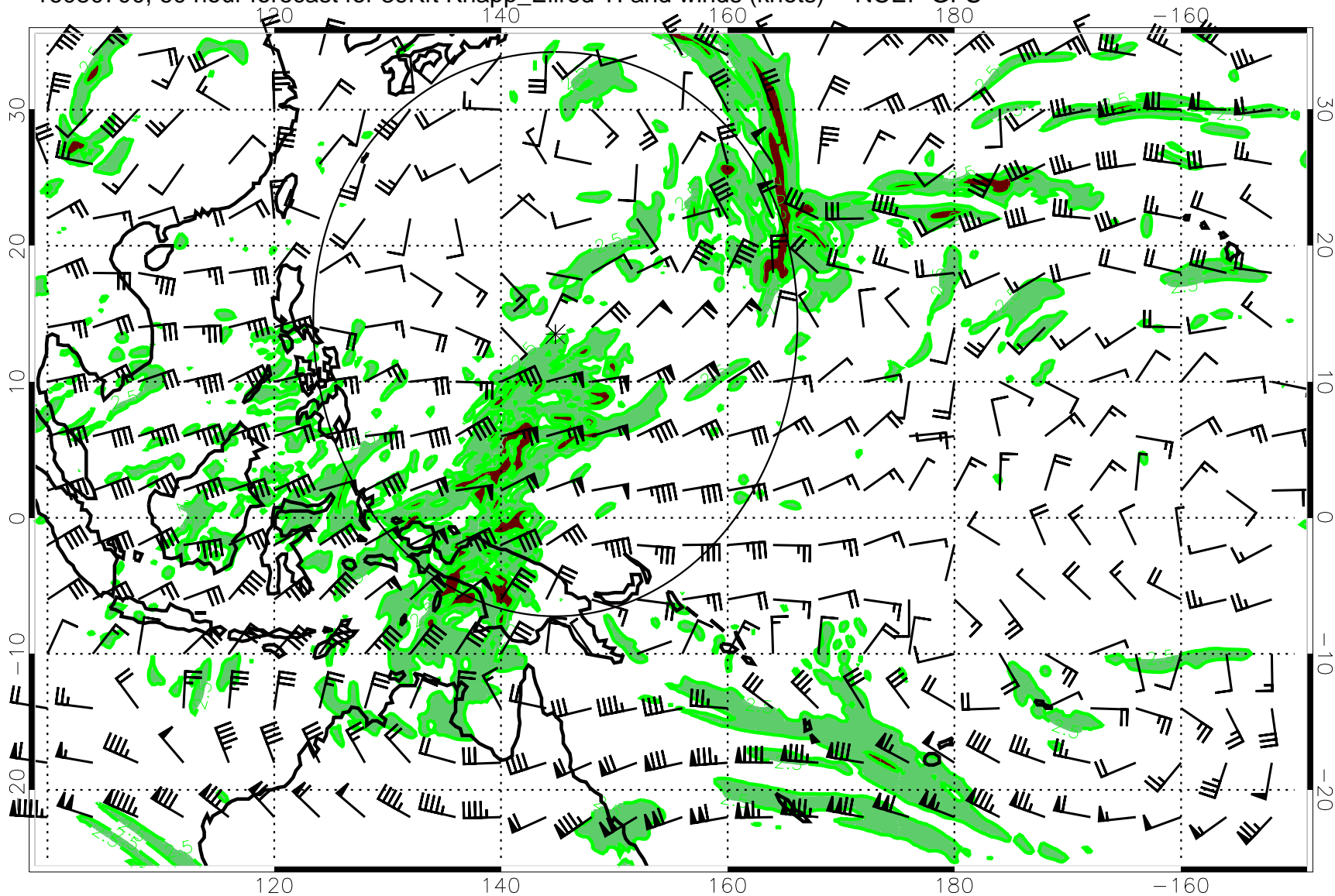
16080700, 60 hour forecast for 39Kft Knapp_Ellrod TI and winds (knots) -- NCEP GFS
