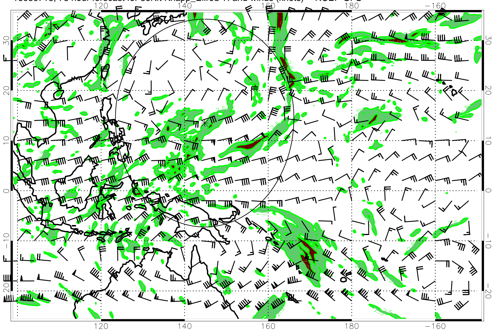
16080718, 78 hour forecast for 36Kft Knapp_Ellrod TI and winds (knots) -- NCEP GFS
