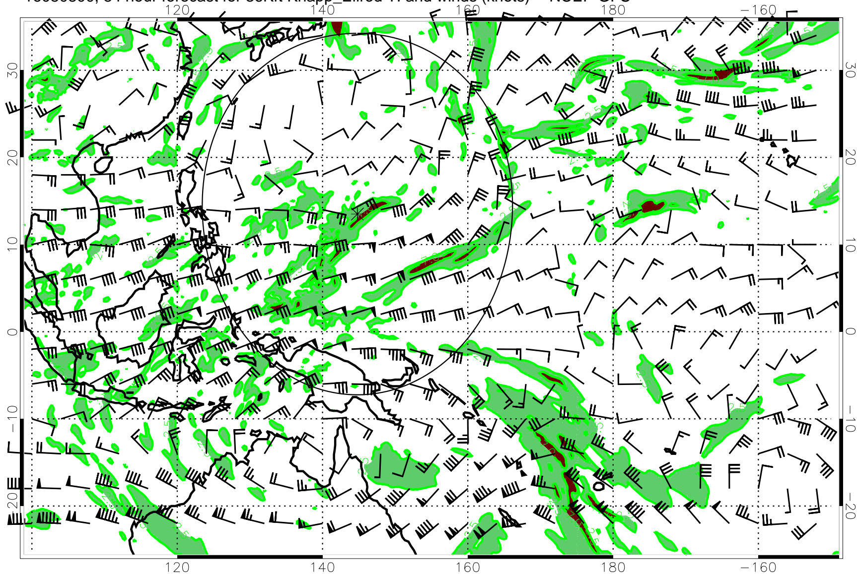
16080800, 84 hour forecast for 36Kft Knapp_Ellrod TI and winds (knots) -- NCEP GFS
