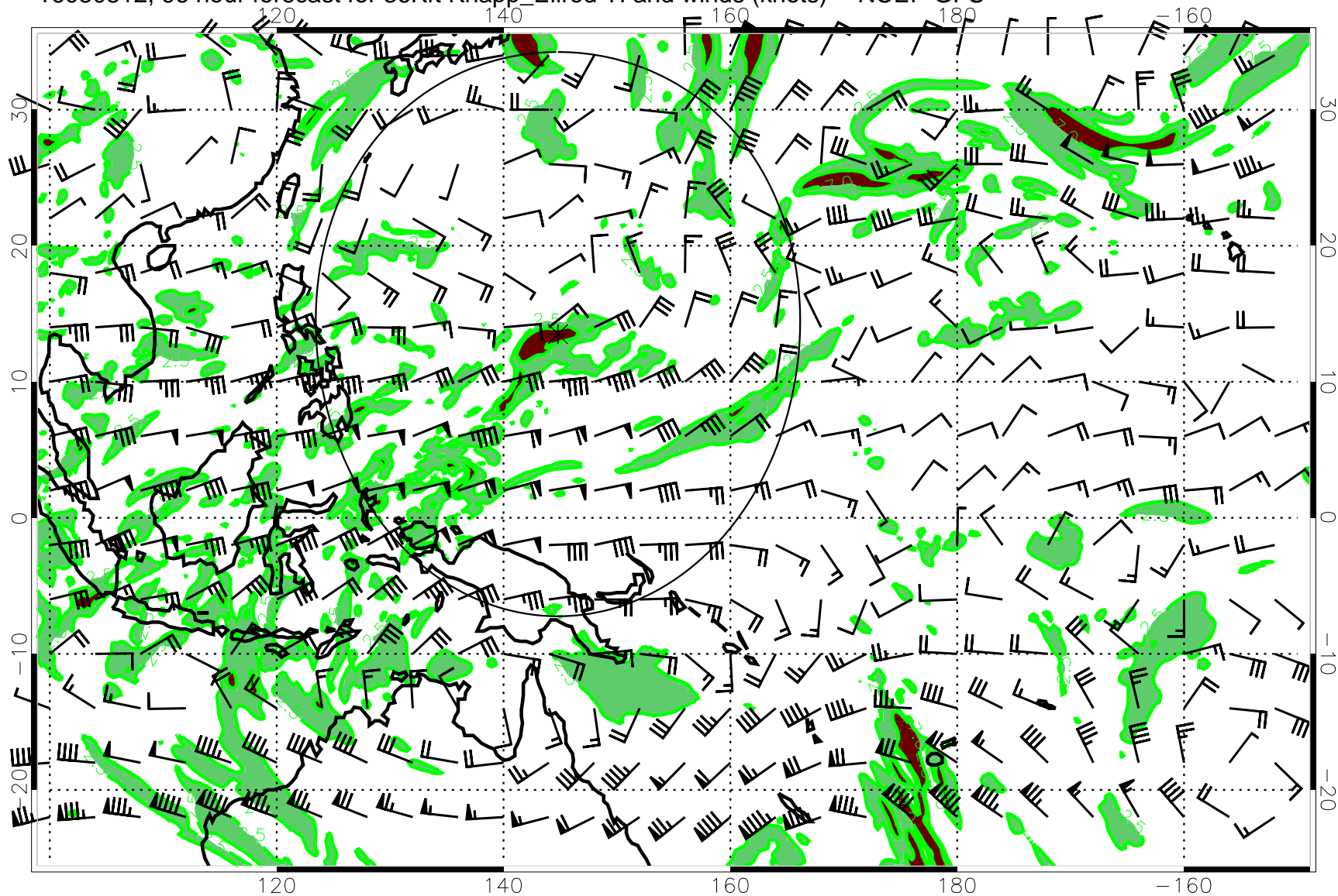
16080812, 96 hour forecast for 36Kft Knapp_Ellrod TI and winds (knots) -- NCEP GFS
