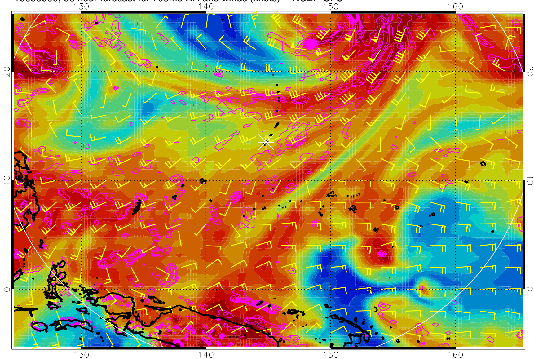
16080600, 36 hour forecast for 700mb RH and winds (knots) -- NCEP GFS
