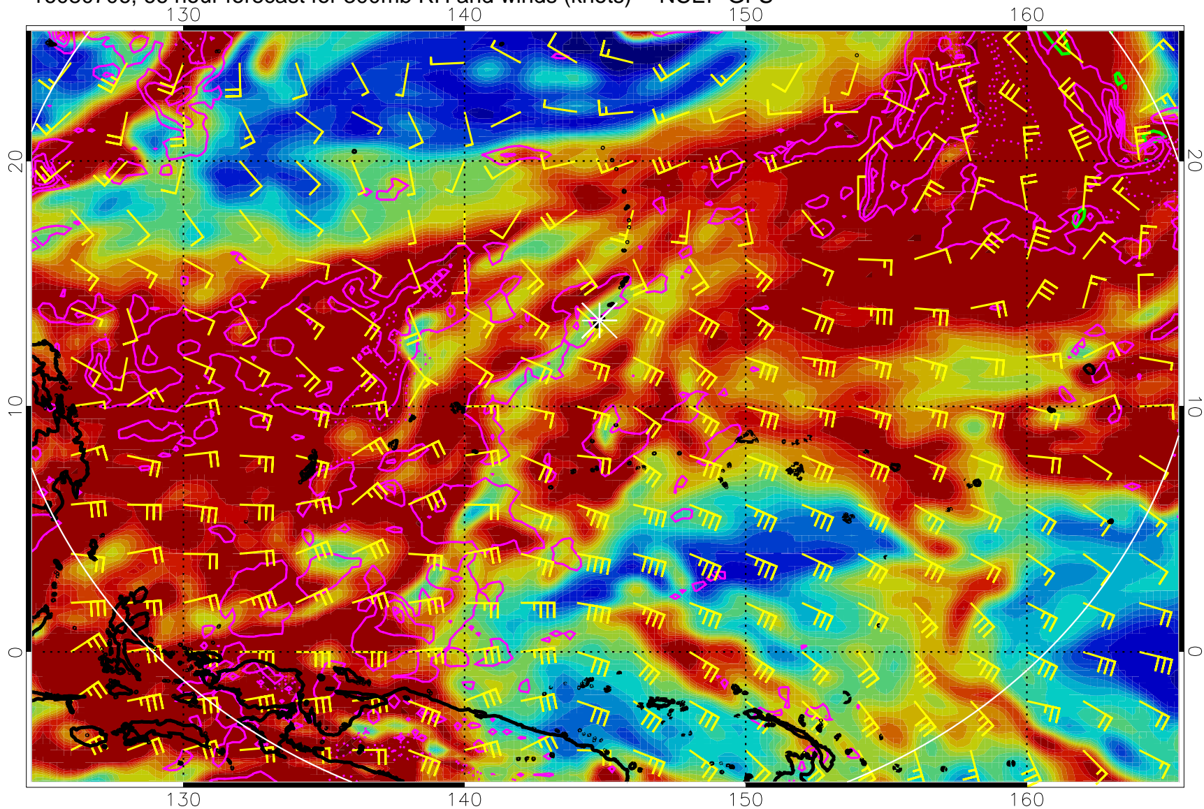
16080706, 66 hour forecast for 300mb RH and winds (knots) -- NCEP GFS
