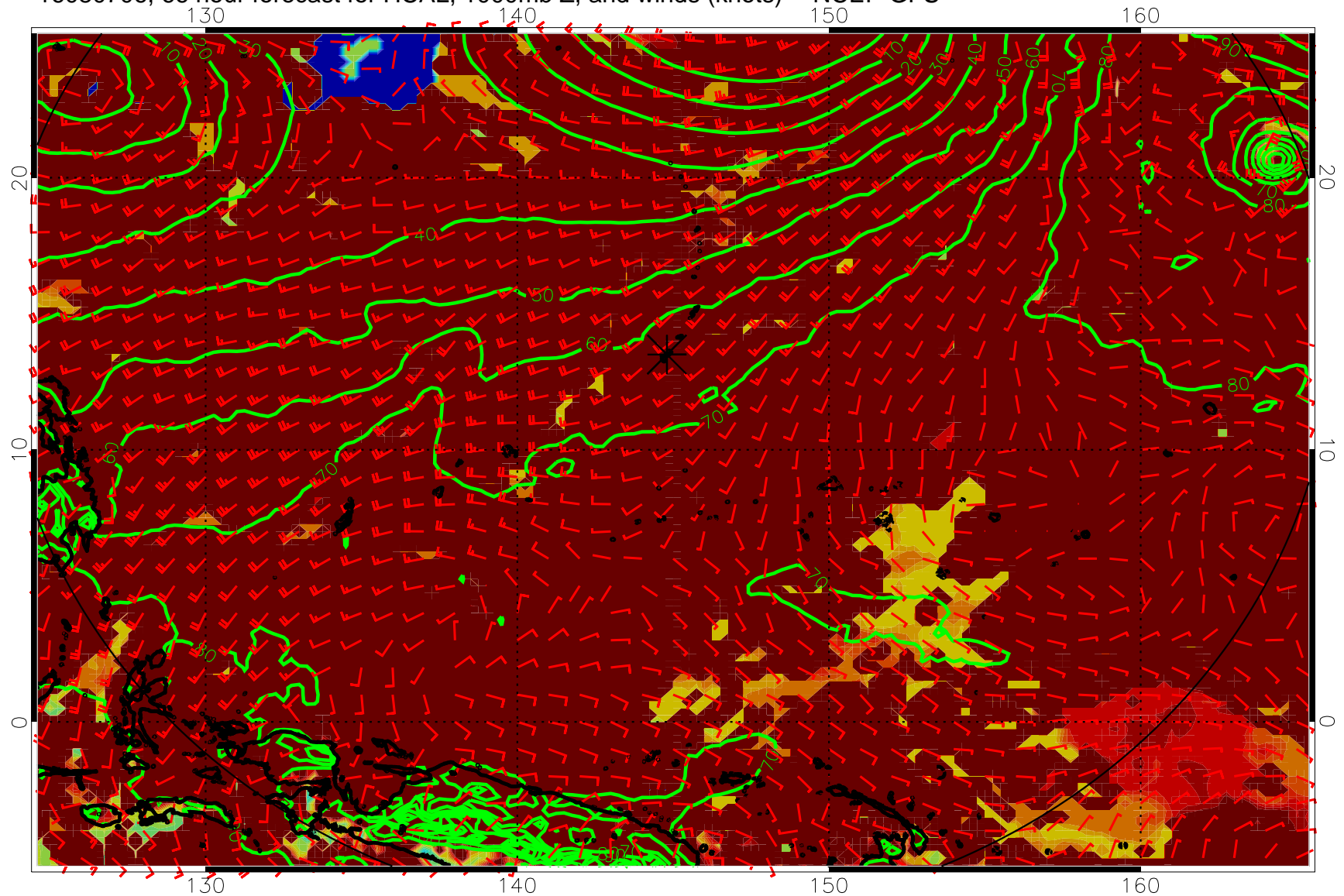
16080706, 66 hour forecast for HCAL, 1000mb Z, and winds (knots) -- NCEP GFS
