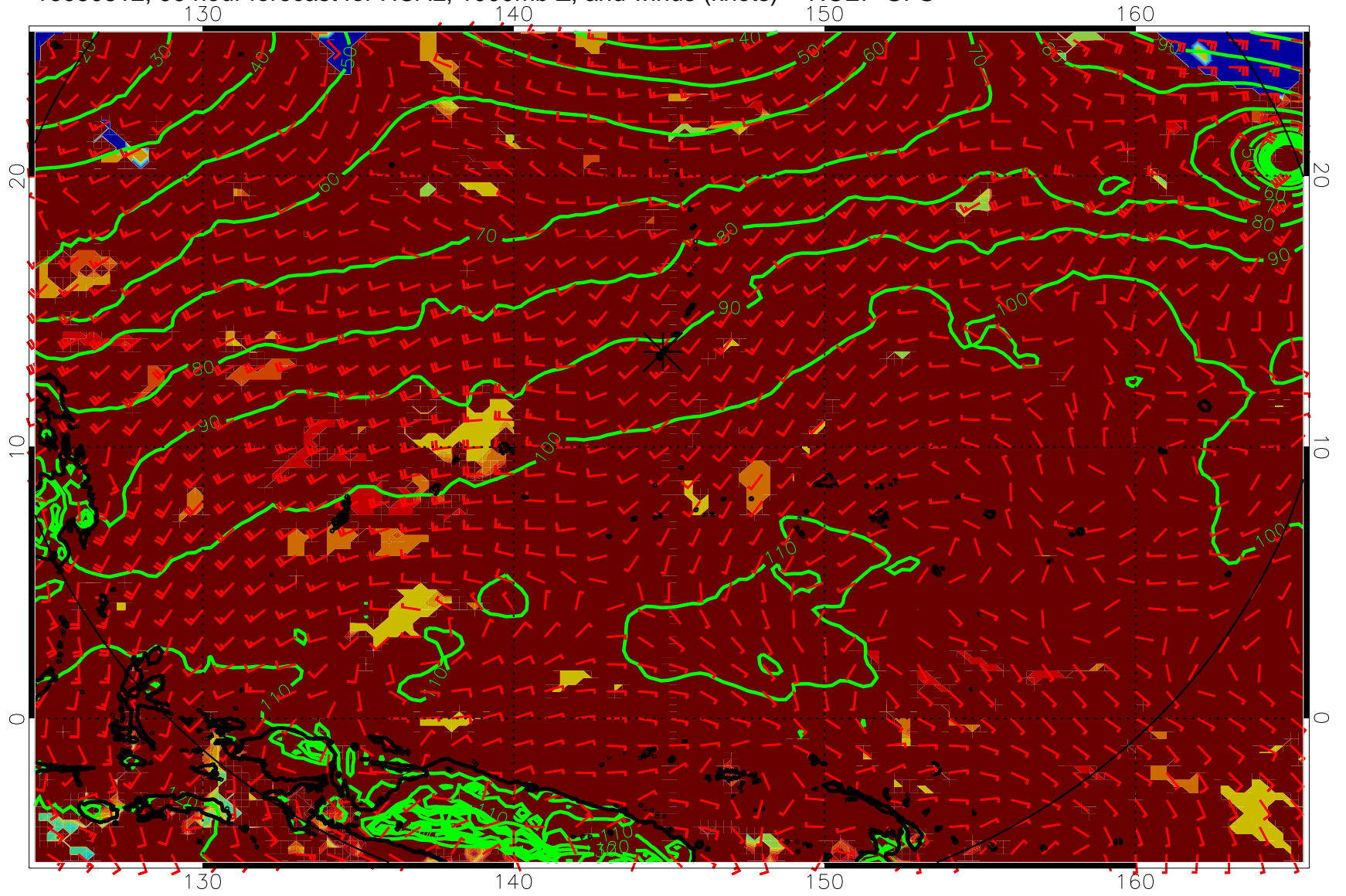
16080812, 96 hour forecast for HCAL, 1000mb Z, and winds (knots) -- NCEP GFS
