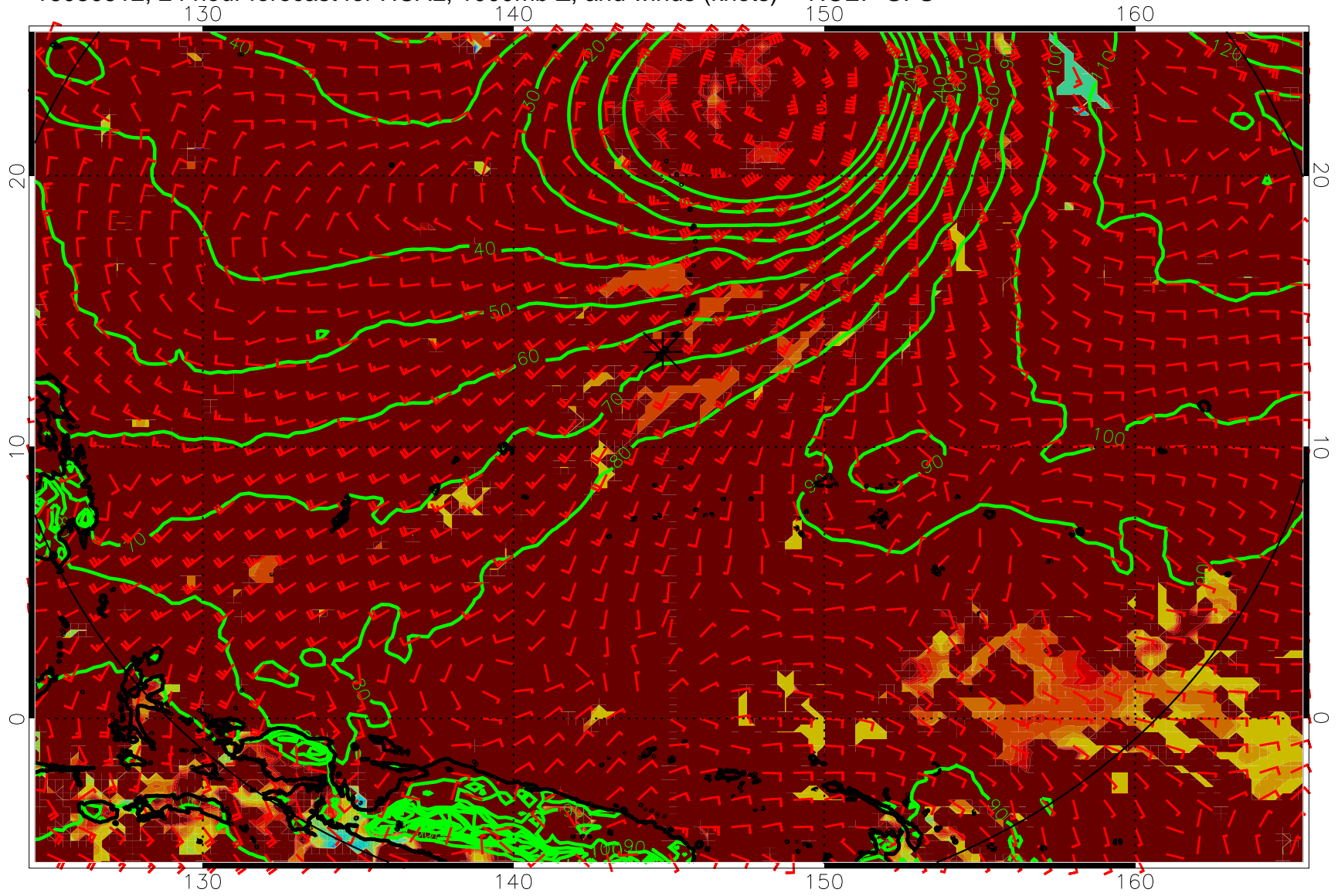
16080512, 24 hour forecast for HCAL, 1000mb Z, and winds (knots) -- NCEP GFS
