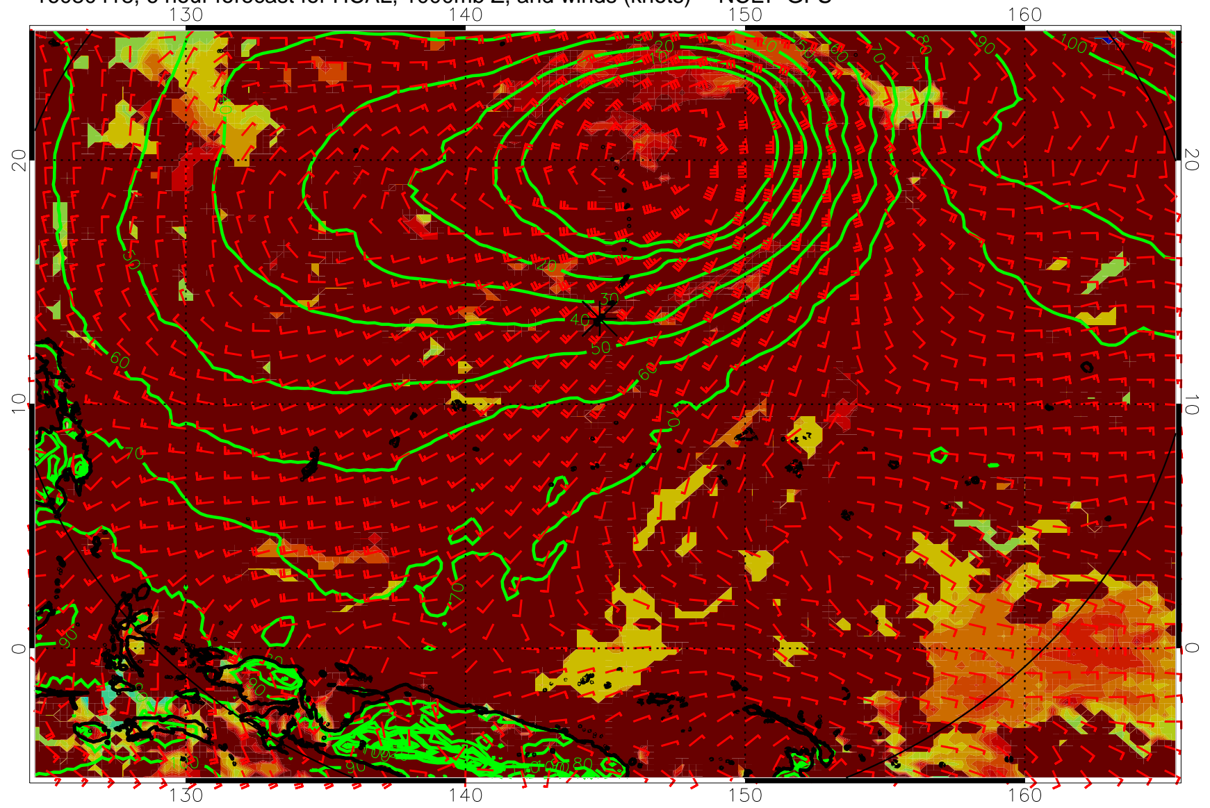
16080418, 6 hour forecast for HCAL, 1000mb Z, and winds (knots) -- NCEP GFS
