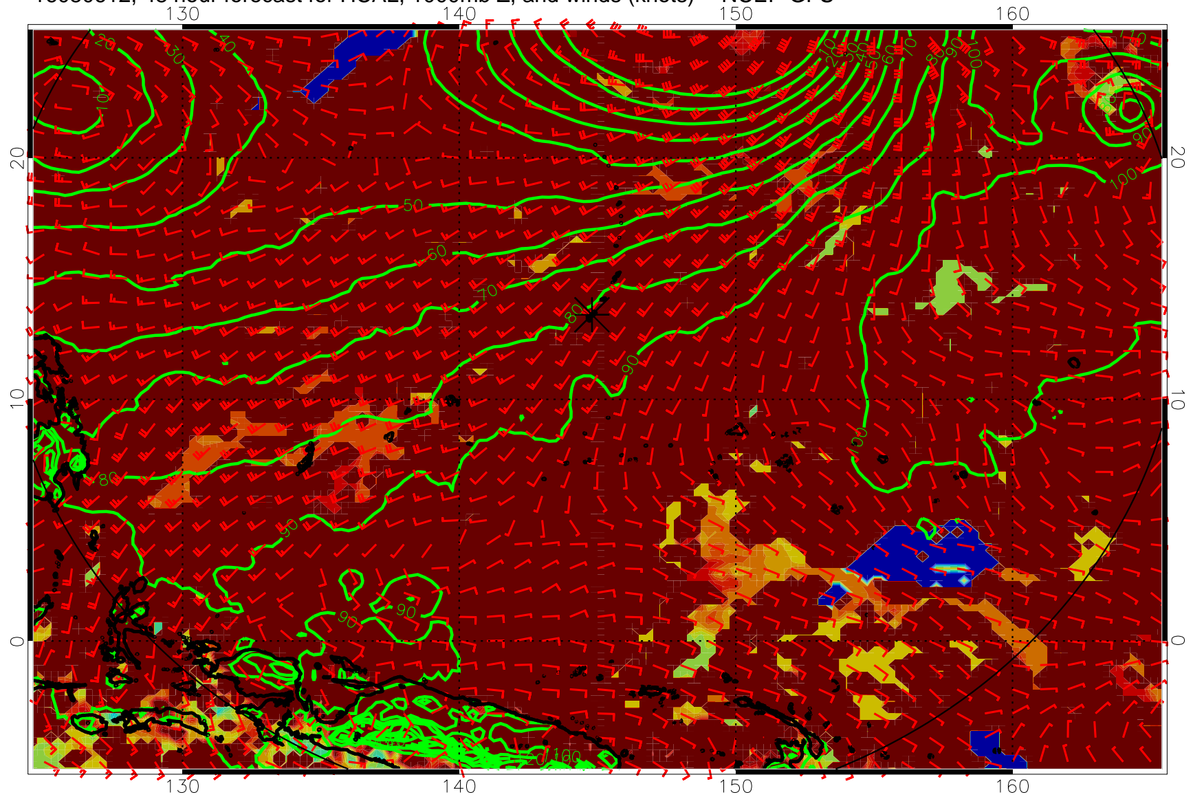
16080612, 48 hour forecast for HCAL, 1000mb Z, and winds (knots) -- NCEP GFS
