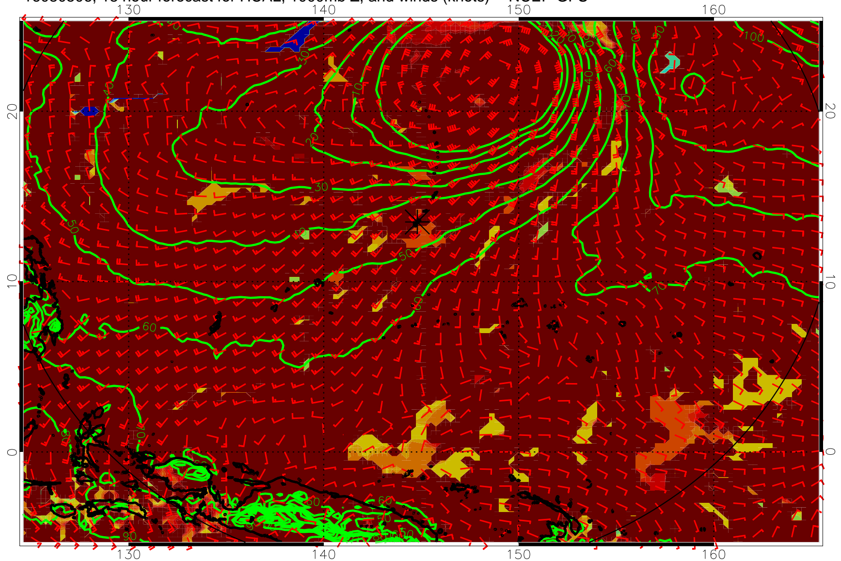
16080506, 18 hour forecast for HCAL, 1000mb Z, and winds (knots) -- NCEP GFS
