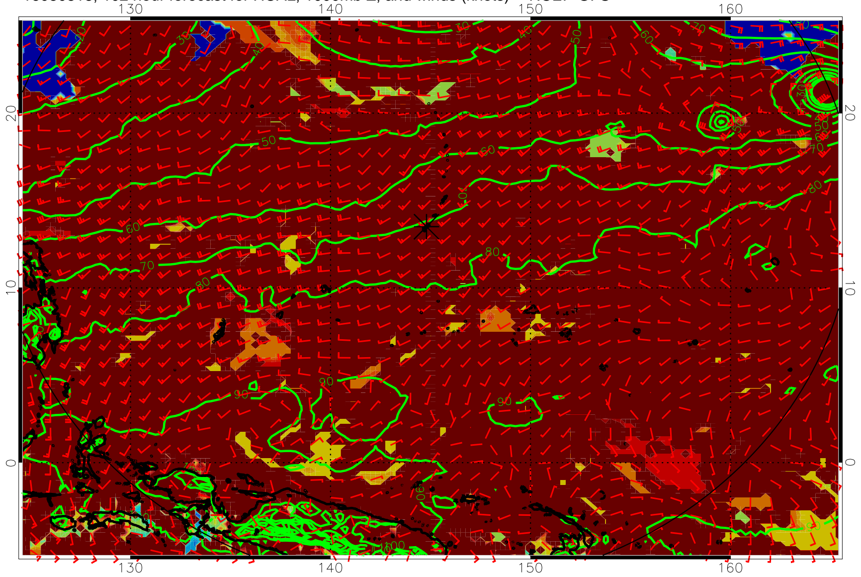
16080818, 102 hour forecast for HCAL, 1000mb Z, and winds (knots) -- NCEP GFS
