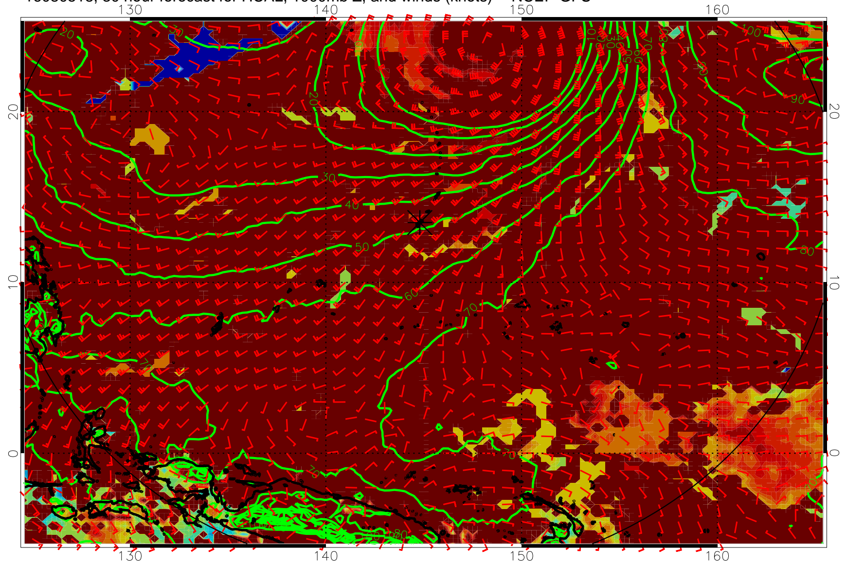
16080518, 30 hour forecast for HCAL, 1000mb Z, and winds (knots) -- NCEP GFS
