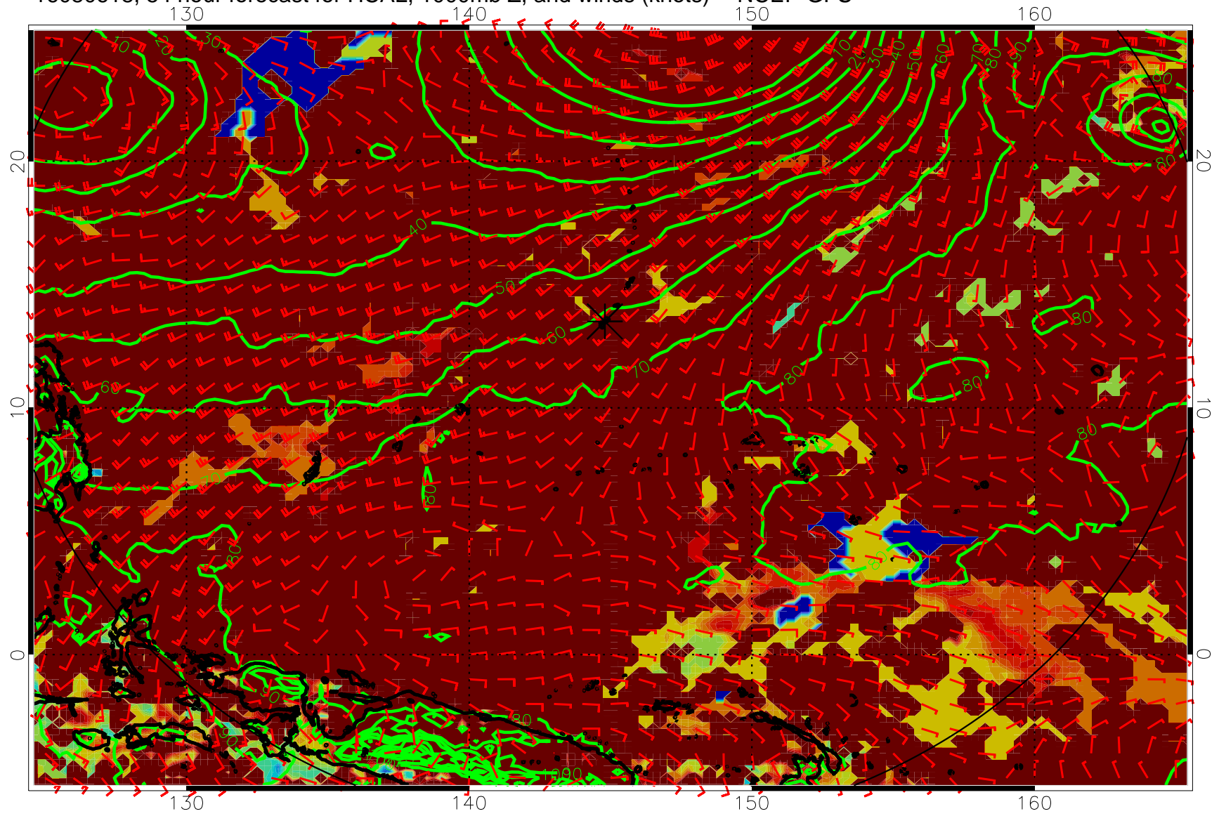
16080618, 54 hour forecast for HCAL, 1000mb Z, and winds (knots) -- NCEP GFS
