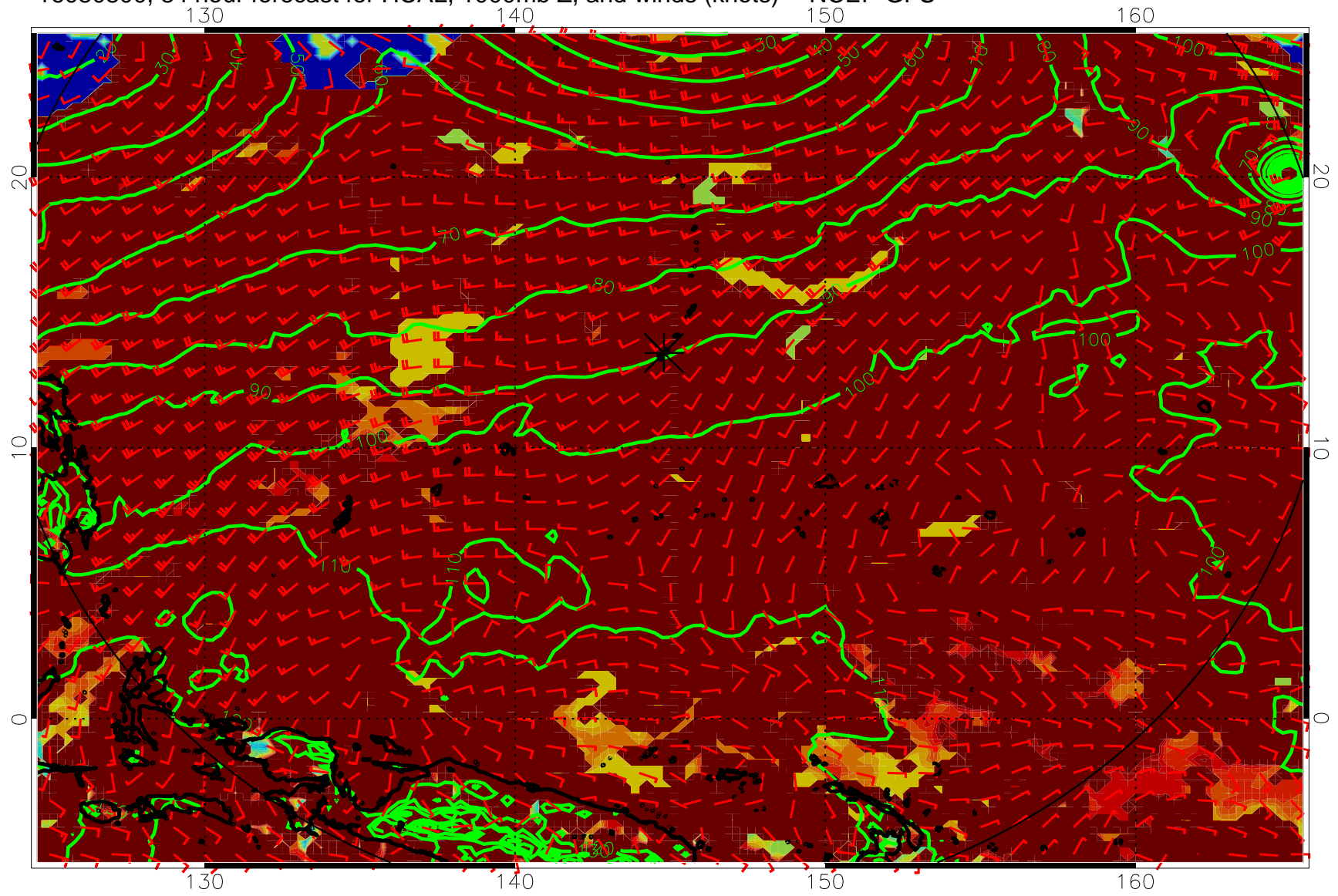
16080800, 84 hour forecast for HCAL, 1000mb Z, and winds (knots) -- NCEP GFS
