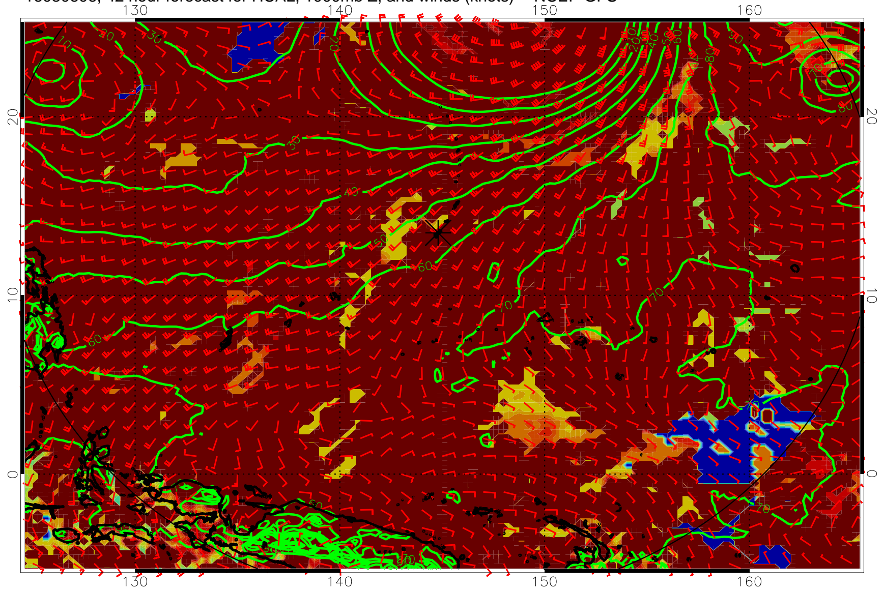
16080606, 42 hour forecast for HCAL, 1000mb Z, and winds (knots) -- NCEP GFS
