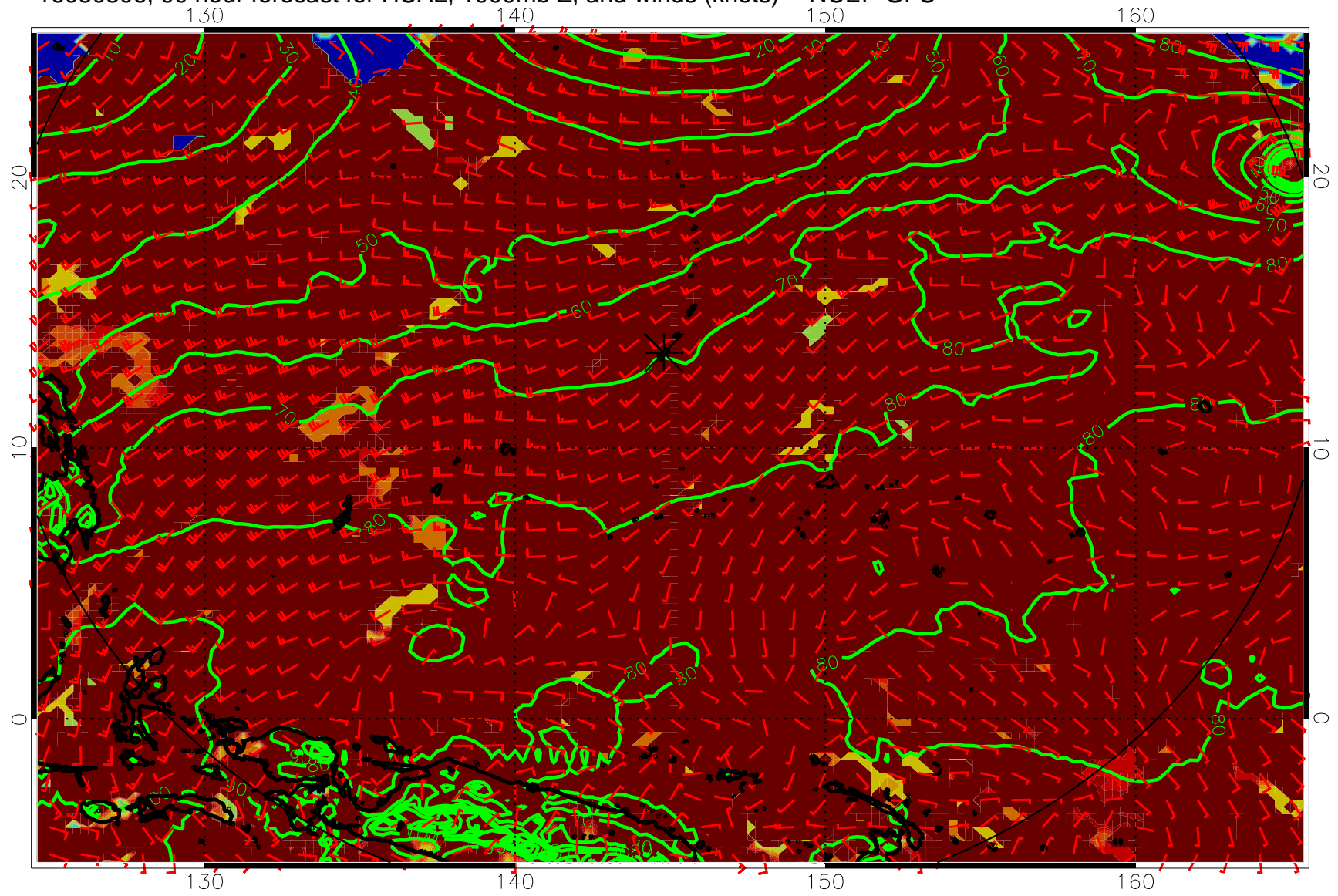
16080806, 90 hour forecast for HCAL, 1000mb Z, and winds (knots) -- NCEP GFS
