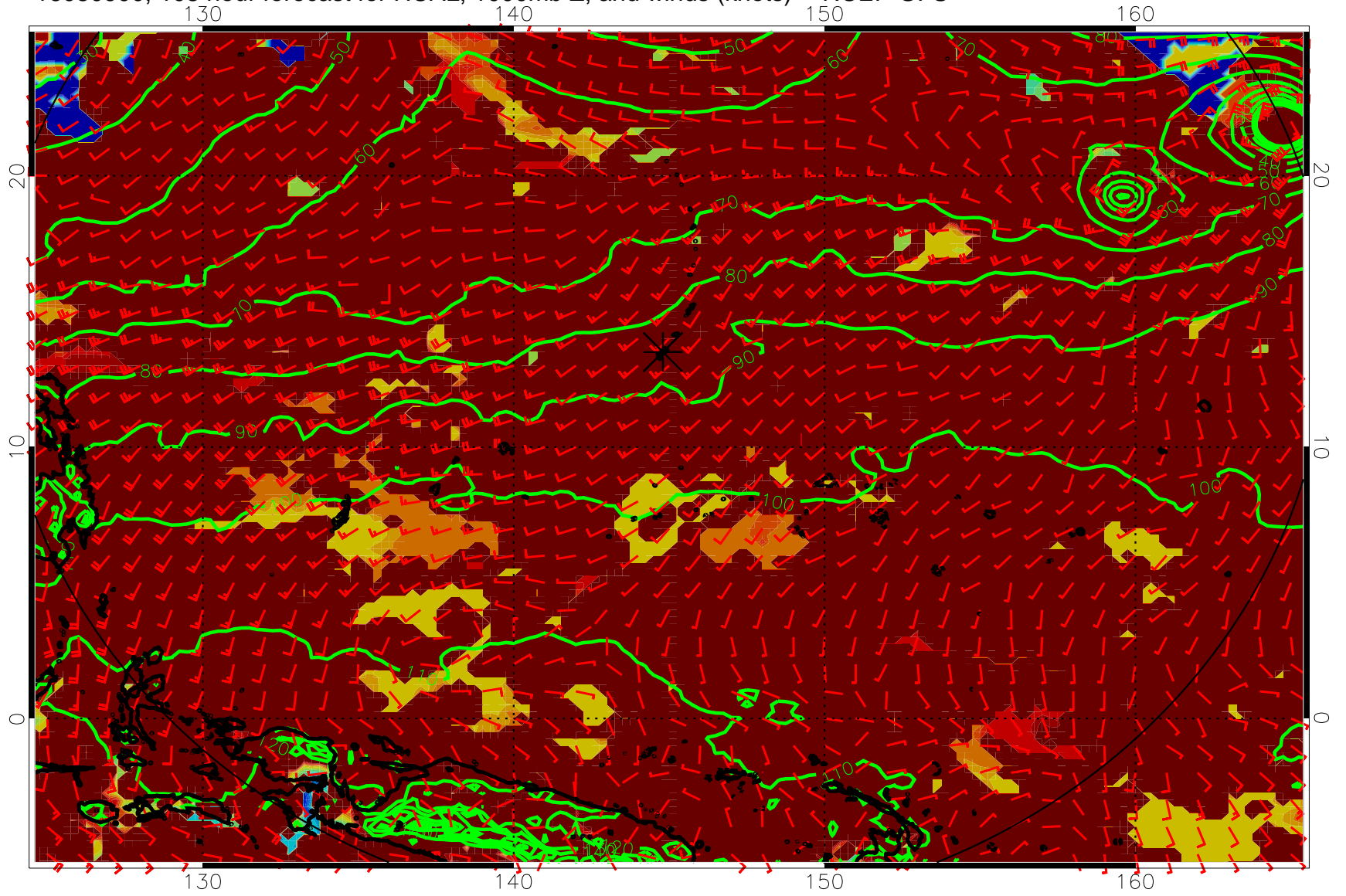
16080900, 108 hour forecast for HCAL, 1000mb Z, and winds (knots) -- NCEP GFS
