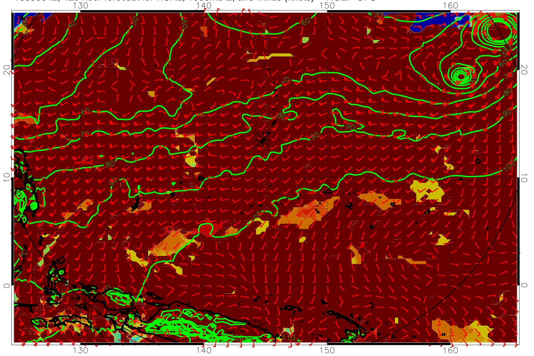
16080912, 120 hour forecast for HCAL, 1000mb Z, and winds (knots) -- NCEP GFS
