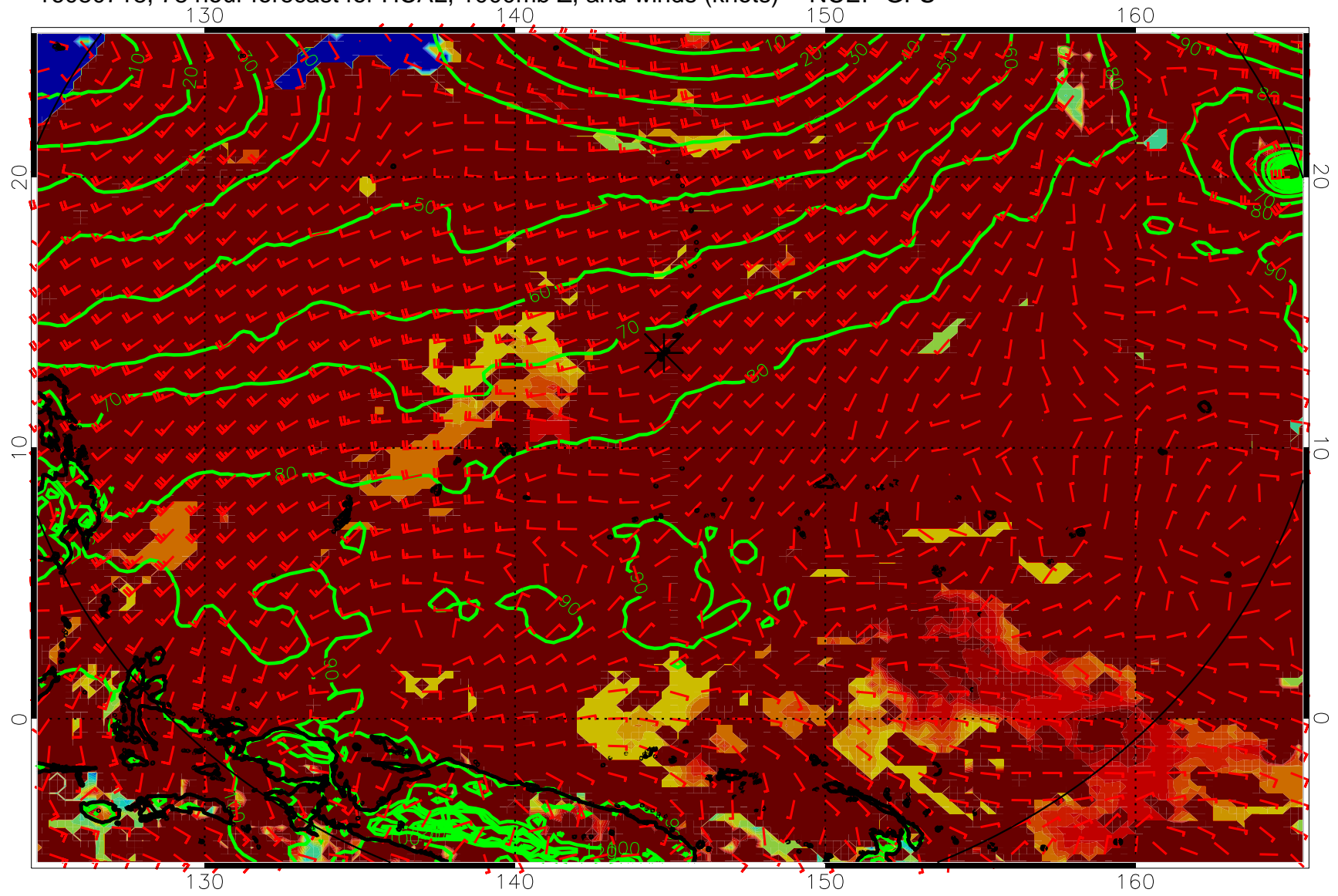
16080718, 78 hour forecast for HCAL, 1000mb Z, and winds (knots) -- NCEP GFS
