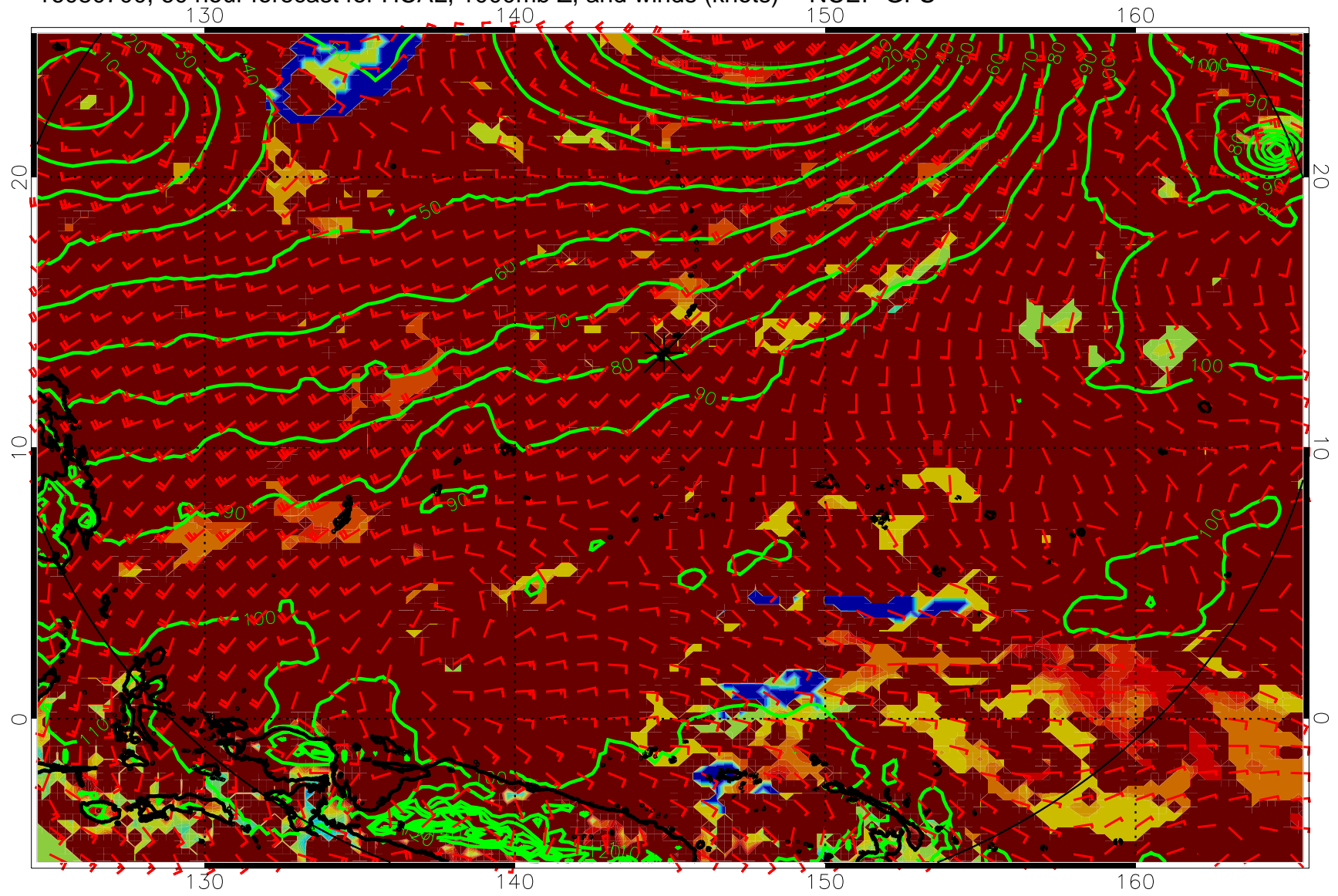
16080700, 60 hour forecast for HCAL, 1000mb Z, and winds (knots) -- NCEP GFS
