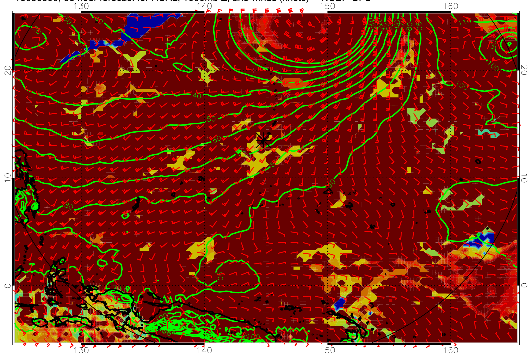
16080600, 36 hour forecast for HCAL, 1000mb Z, and winds (knots) -- NCEP GFS
