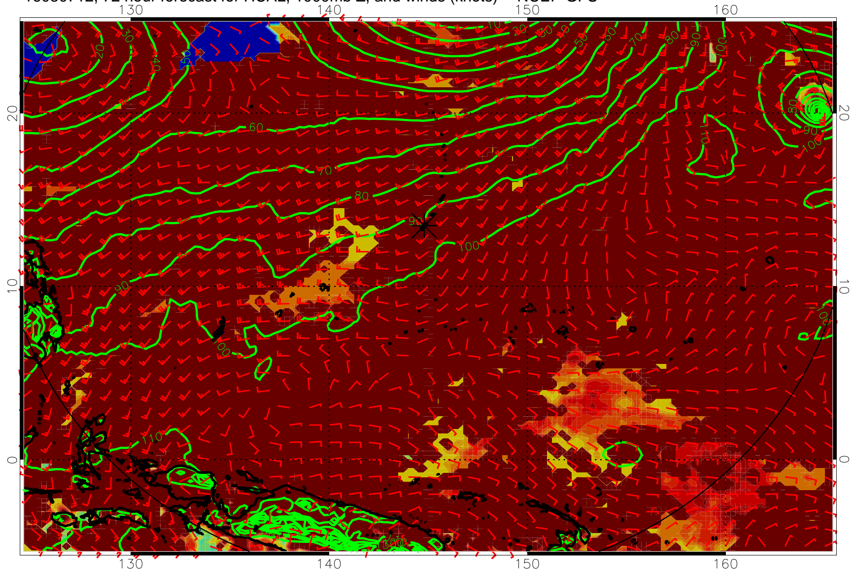
16080712, 72 hour forecast for HCAL, 1000mb Z, and winds (knots) -- NCEP GFS
