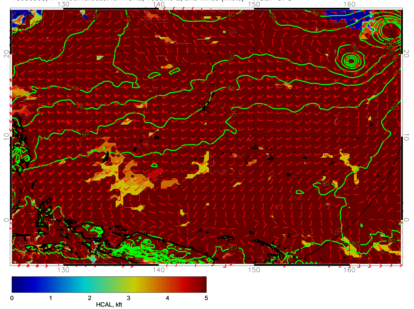
16080906, 114 hour forecast for HCAL, 1000mb Z, and winds (knots) -- NCEP GFS
