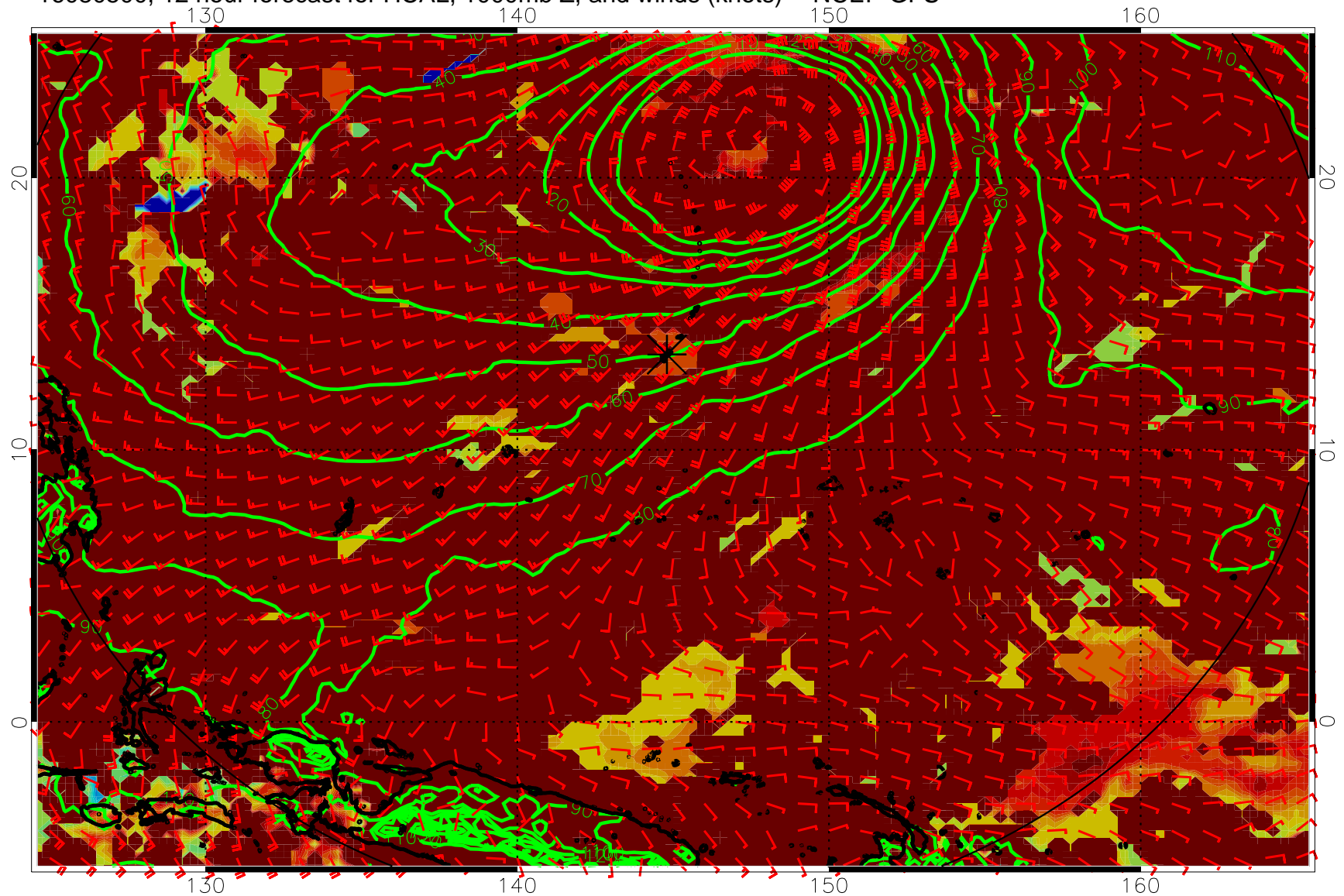
16080500, 12 hour forecast for HCAL, 1000mb Z, and winds (knots) -- NCEP GFS
