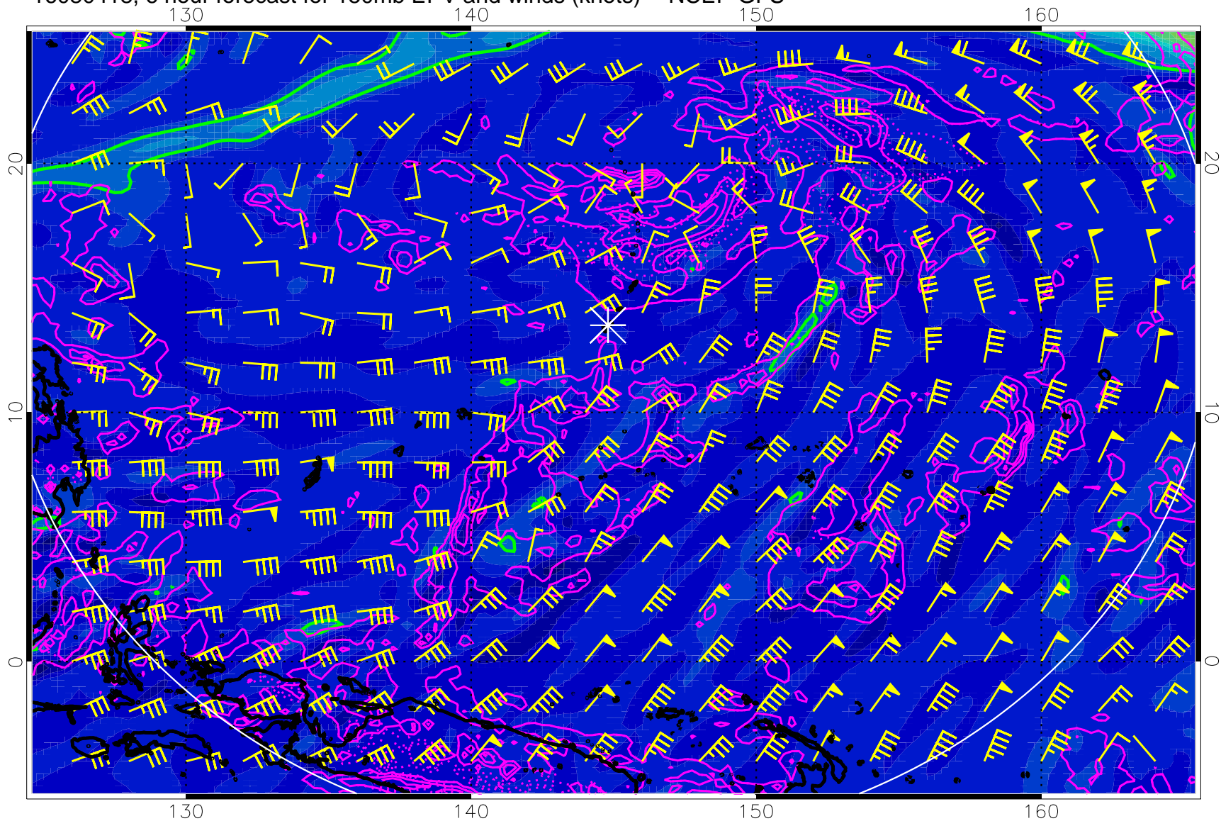
16080418, 6 hour forecast for 150mb EPV and winds (knots) -- NCEP GFS
