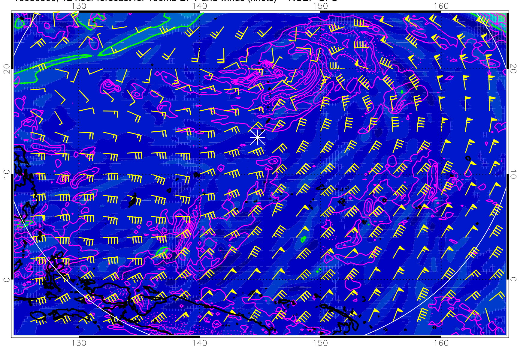
16080500, 12 hour forecast for 150mb EPV and winds (knots) -- NCEP GFS
