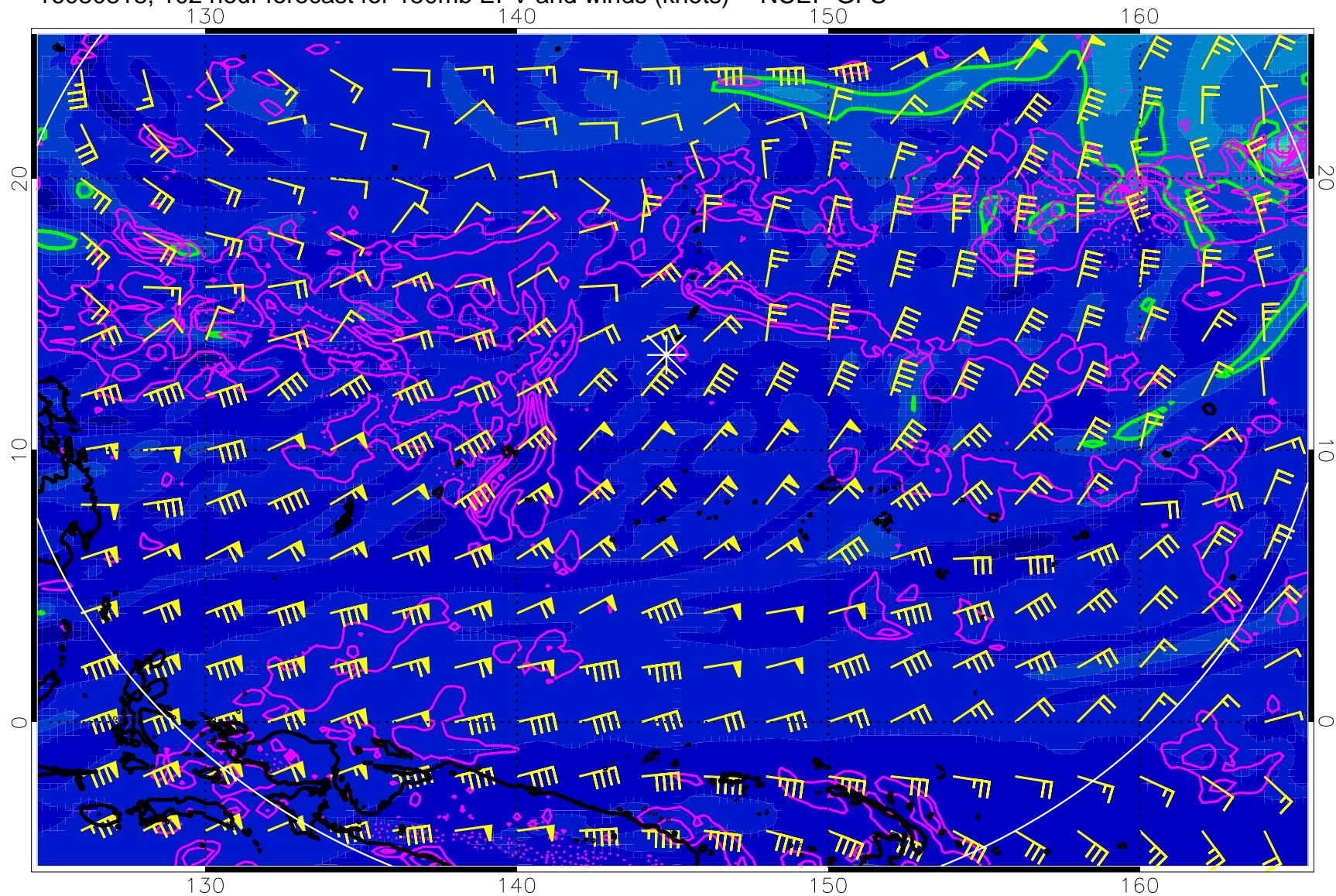
16080818, 102 hour forecast for 150mb EPV and winds (knots) -- NCEP GFS
