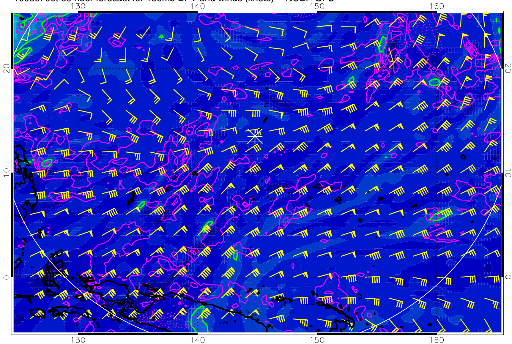
16080700, 60 hour forecast for 150mb EPV and winds (knots) -- NCEP GFS
