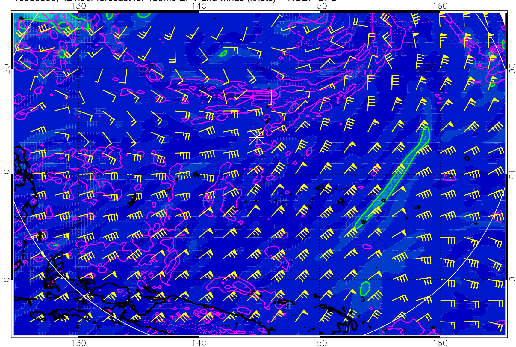
16080606, 42 hour forecast for 150mb EPV and winds (knots) -- NCEP GFS
