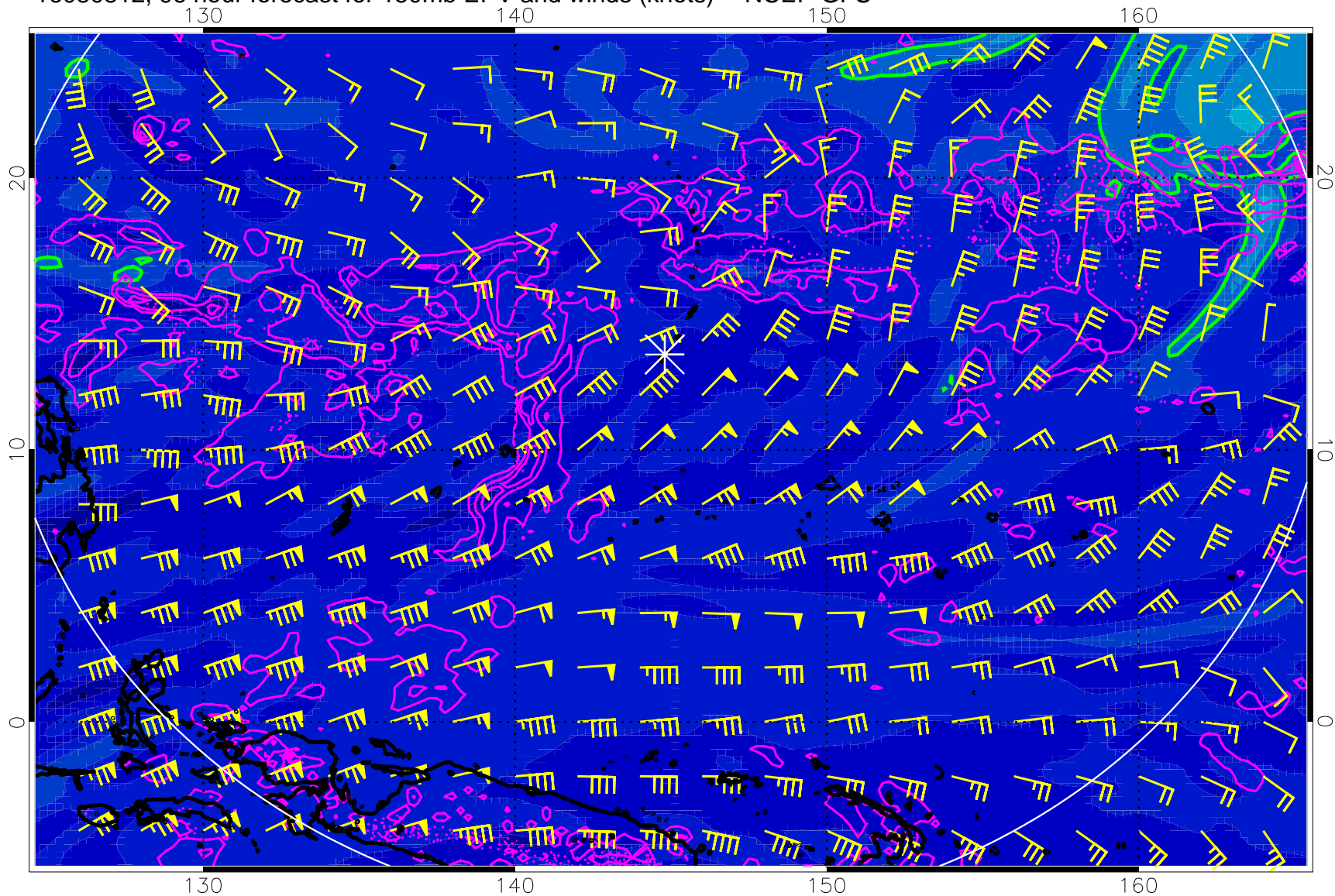
16080812, 96 hour forecast for 150mb EPV and winds (knots) -- NCEP GFS
