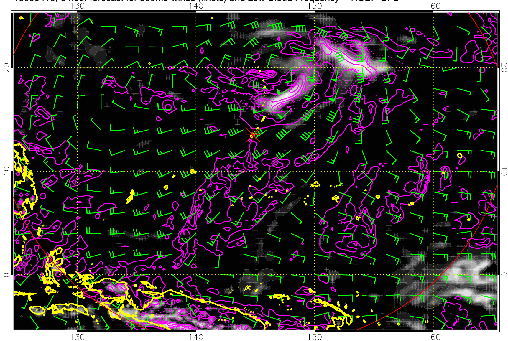
16080418, 6 hour forecast for 850mb winds (knots) and Low Cloud Frequency -- NCEP GFS
