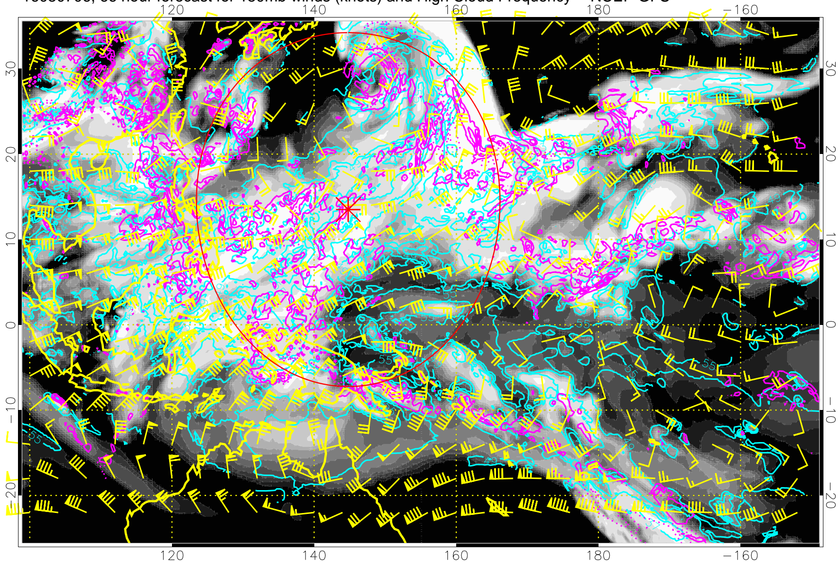
16080706, 66 hour forecast for 150mb winds (knots) and High Cloud Frequency -- NCEP GFS
