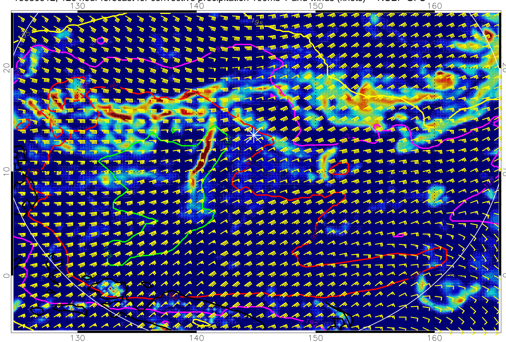
16080912, 120 hour forecast for convective precipitation 100mb T and winds (knots) -- NCEP GFS
