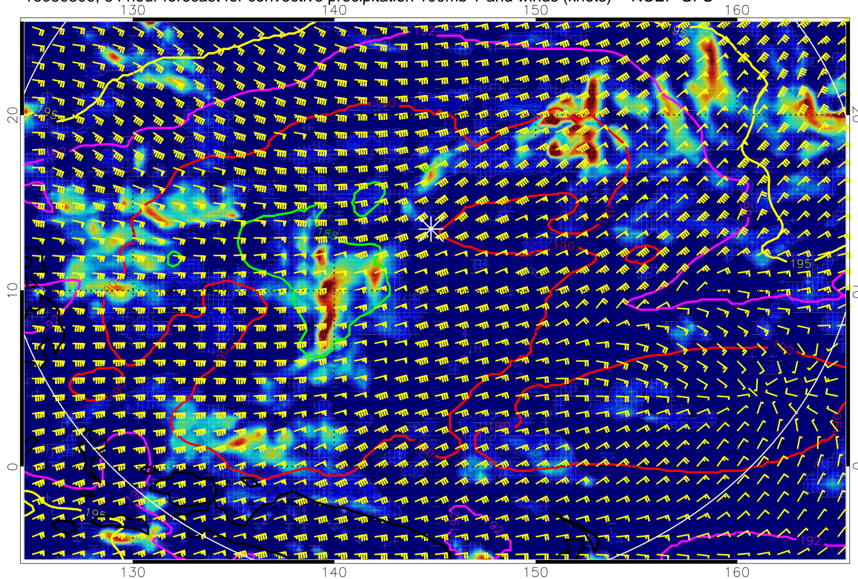
16080800, 84 hour forecast for convective precipitation 100mb T and winds (knots) -- NCEP GFS
