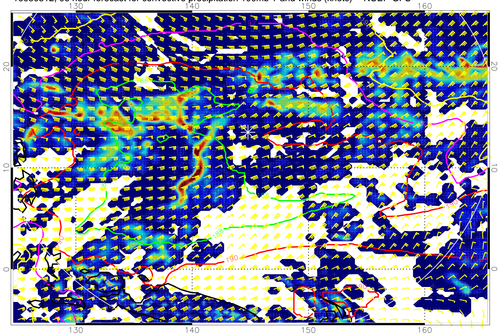
16080812, 96 hour forecast for convective precipitation 100mb T and winds (knots) -- NCEP GFS
