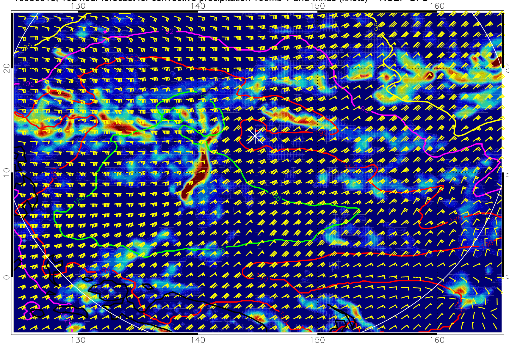
16080818, 102 hour forecast for convective precipitation 100mb T and winds (knots) -- NCEP GFS
