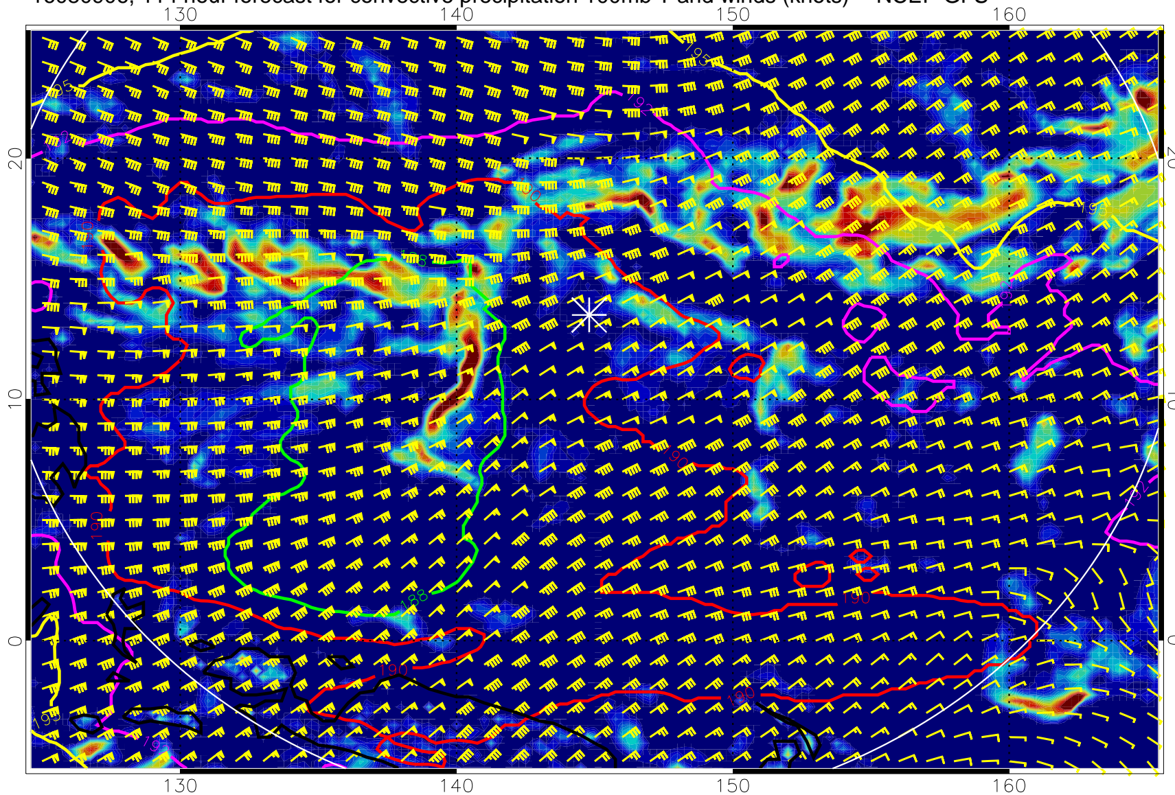
16080906, 114 hour forecast for convective precipitation 100mb T and winds (knots) -- NCEP GFS
