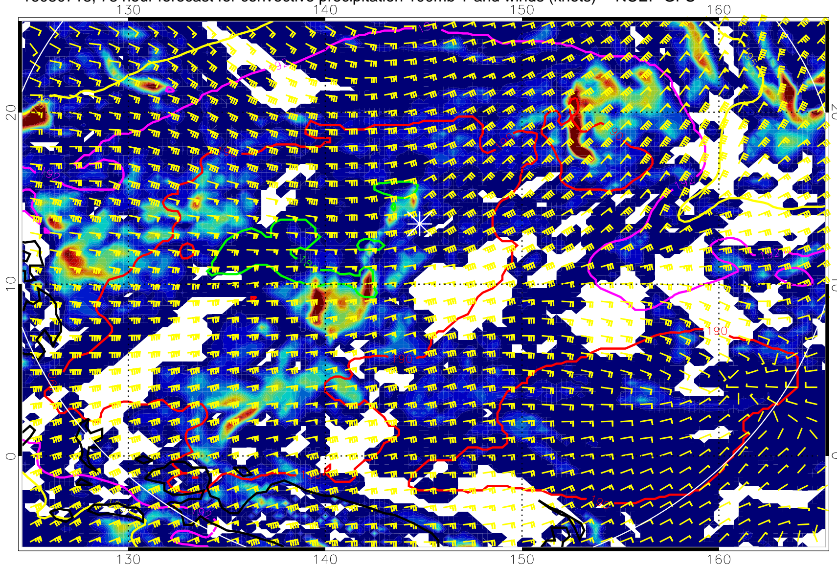
16080718, 78 hour forecast for convective precipitation 100mb T and winds (knots) -- NCEP GFS
