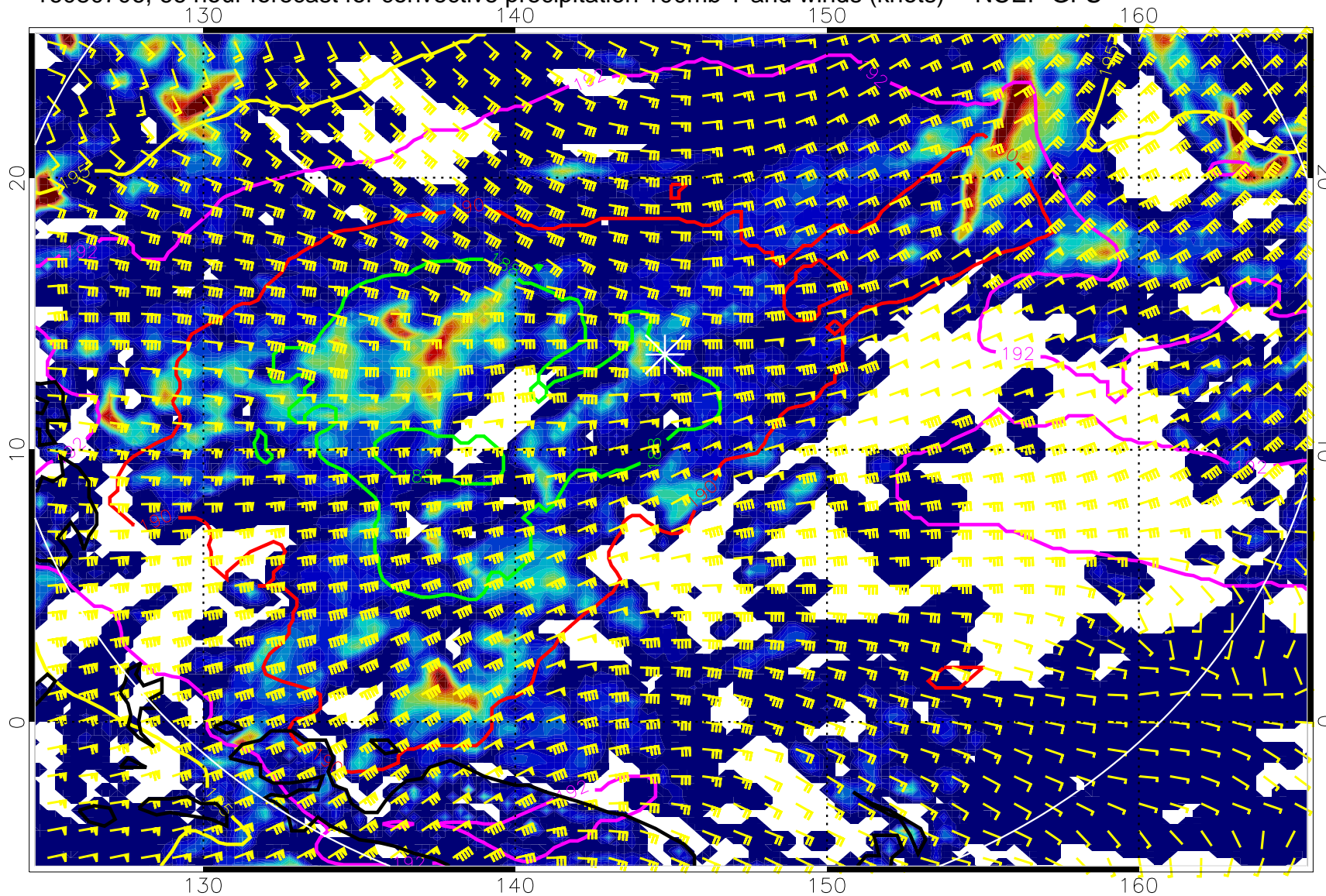
16080706, 66 hour forecast for convective precipitation 100mb T and winds (knots) -- NCEP GFS
