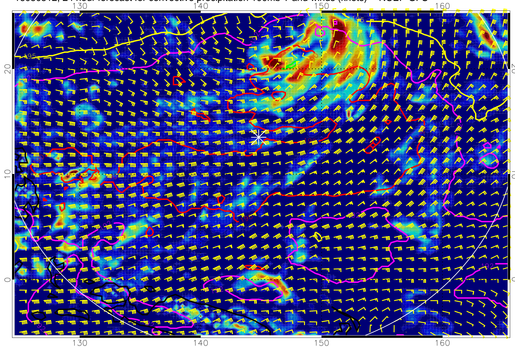
16080512, 24 hour forecast for convective precipitation 100mb T and winds (knots) -- NCEP GFS
