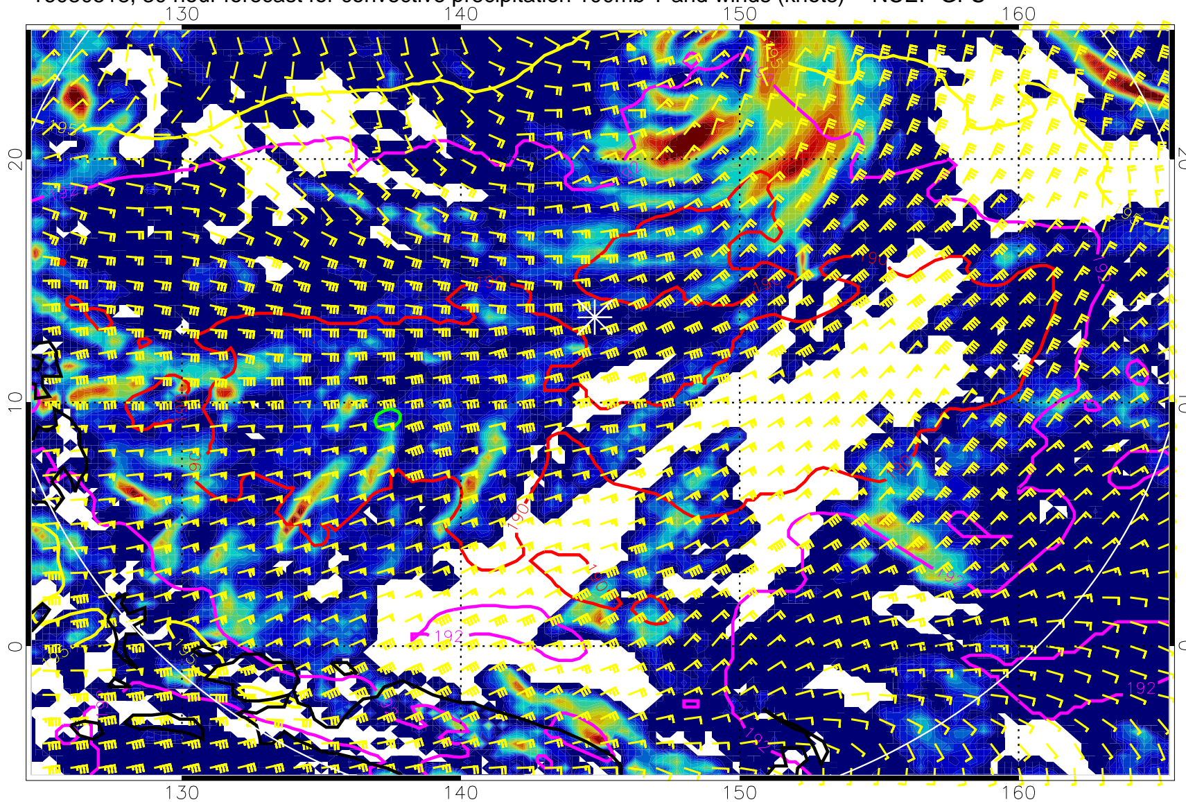
16080518, 30 hour forecast for convective precipitation 100mb T and winds (knots) -- NCEP GFS
