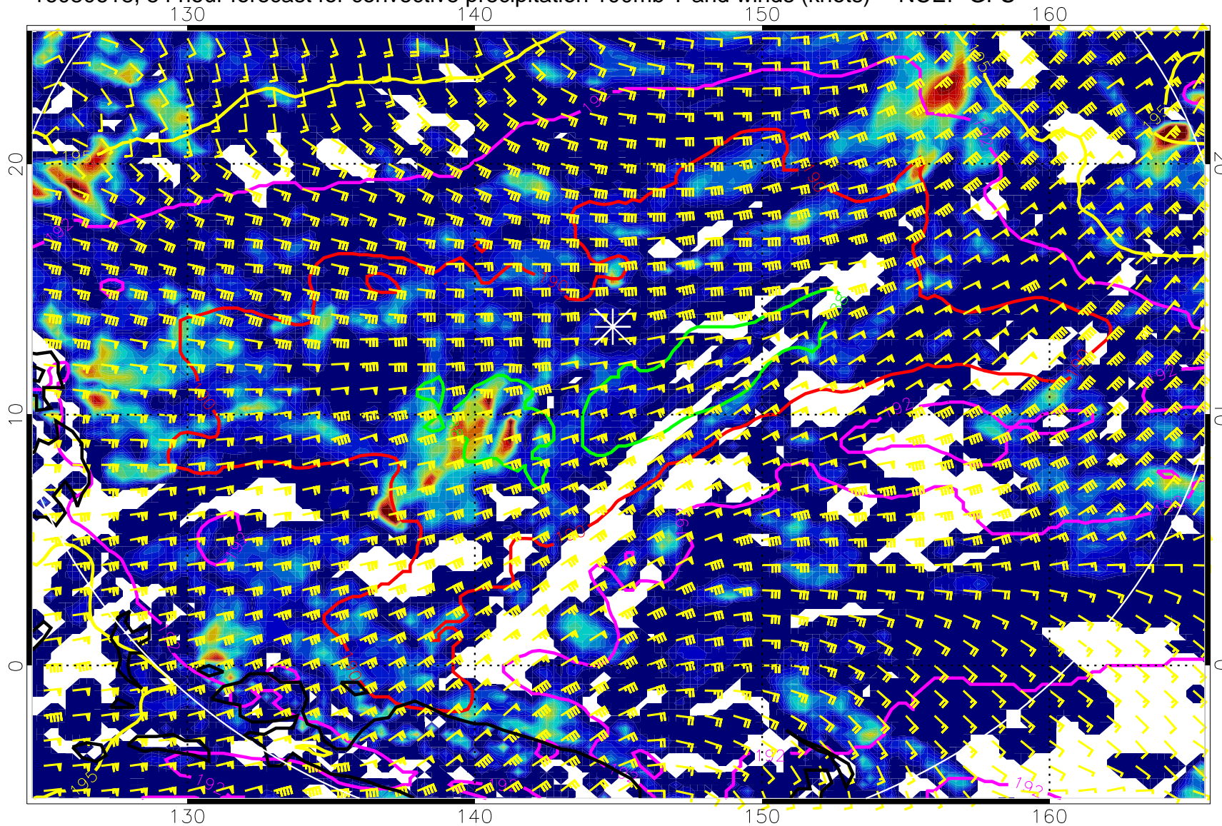
16080618, 54 hour forecast for convective precipitation 100mb T and winds (knots) -- NCEP GFS
