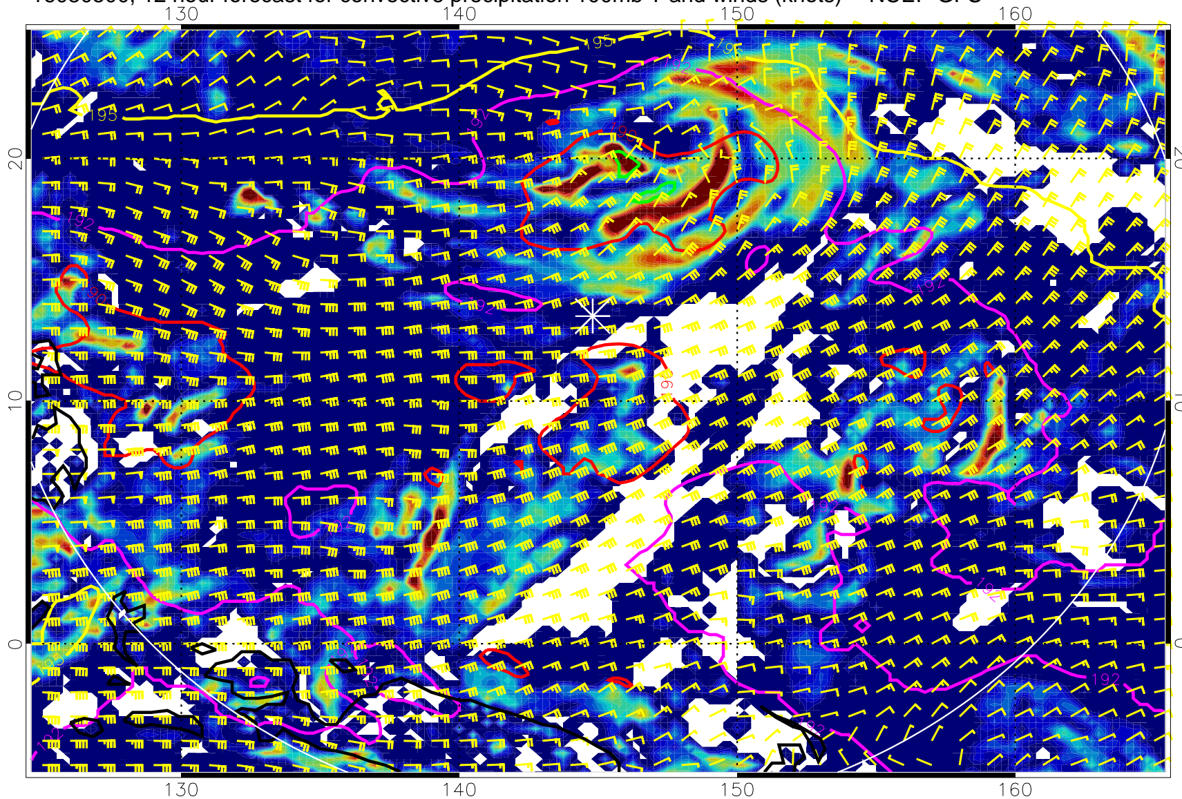
16080500, 12 hour forecast for convective precipitation 100mb T and winds (knots) -- NCEP GFS
