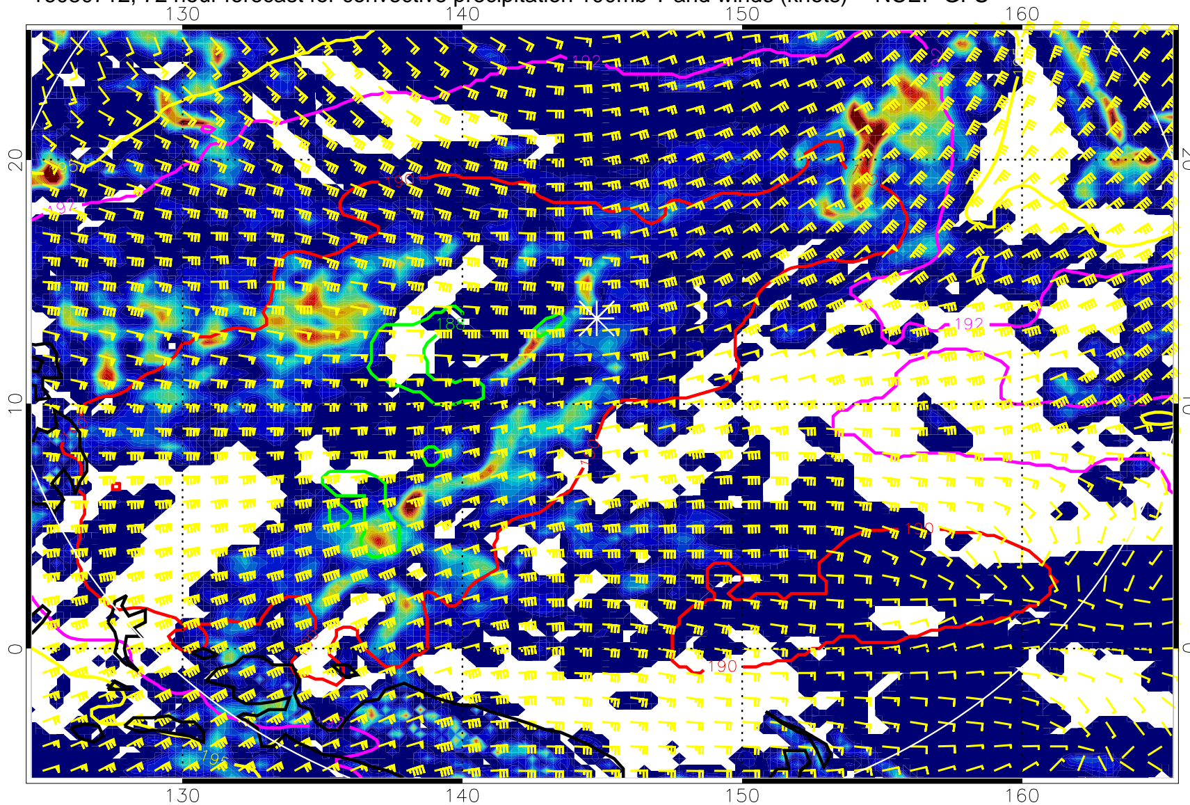
16080712, 72 hour forecast for convective precipitation 100mb T and winds (knots) -- NCEP GFS
