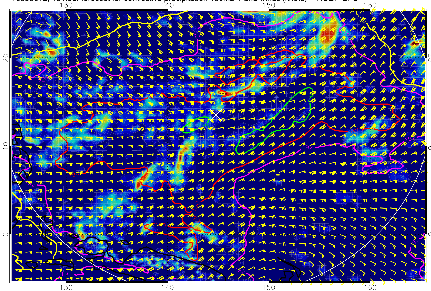
16080612, 48 hour forecast for convective precipitation 100mb T and winds (knots) -- NCEP GFS
