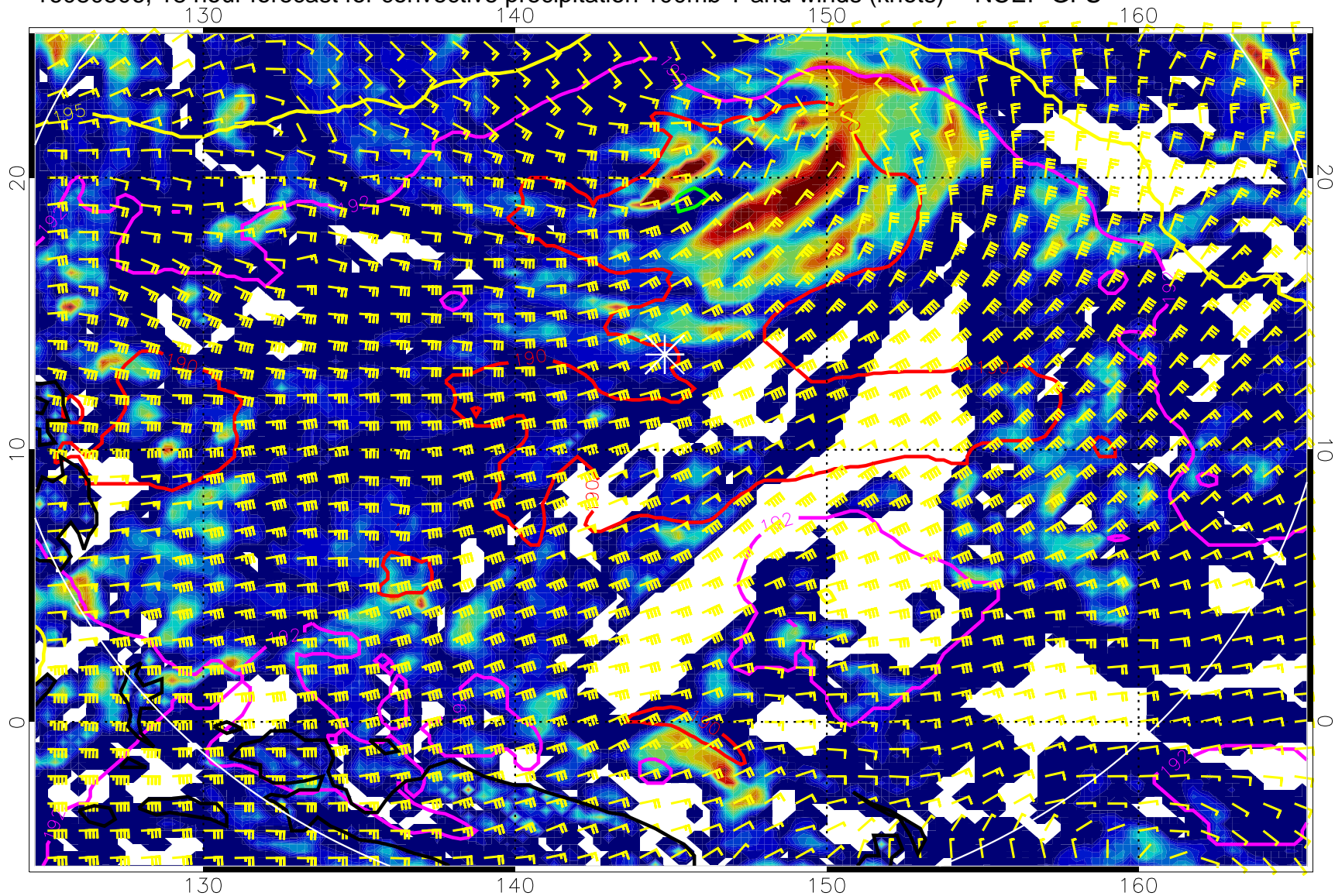
16080506, 18 hour forecast for convective precipitation 100mb T and winds (knots) -- NCEP GFS
