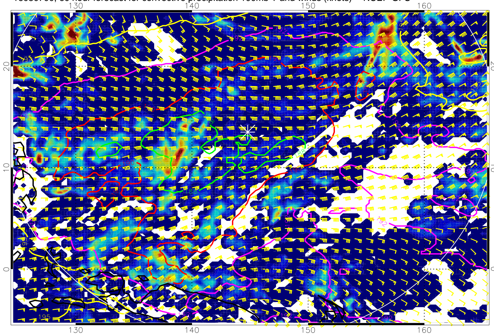
16080700, 60 hour forecast for convective precipitation 100mb T and winds (knots) -- NCEP GFS
