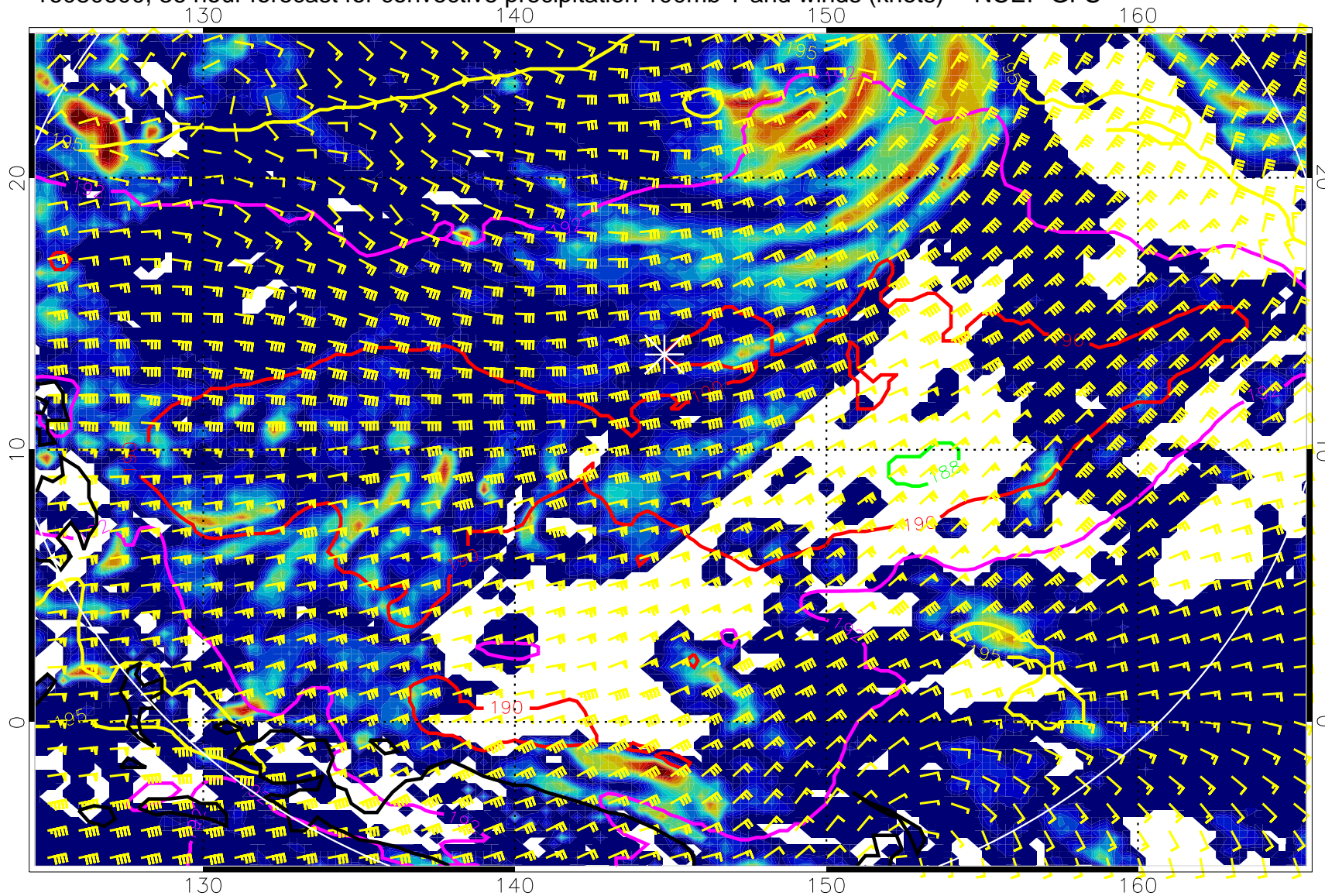
16080600, 36 hour forecast for convective precipitation 100mb T and winds (knots) -- NCEP GFS
