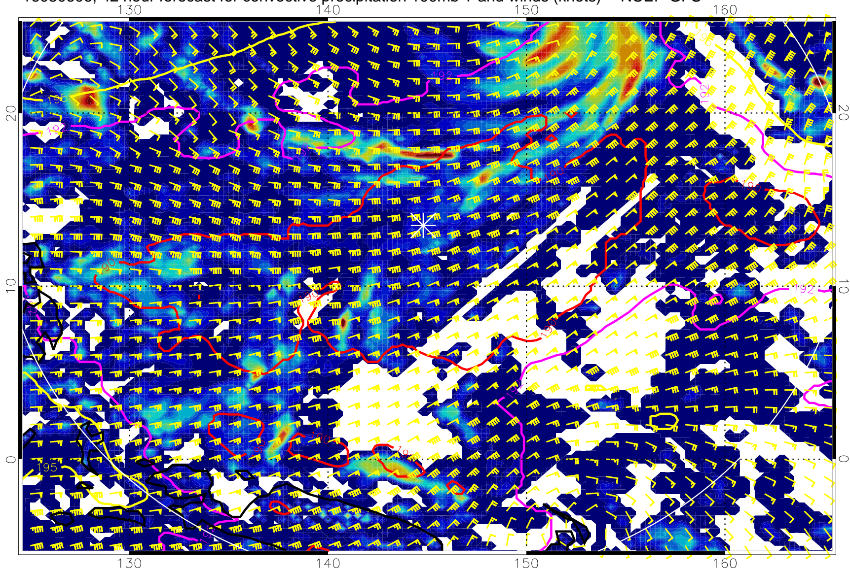
16080606, 42 hour forecast for convective precipitation 100mb T and winds (knots) -- NCEP GFS
