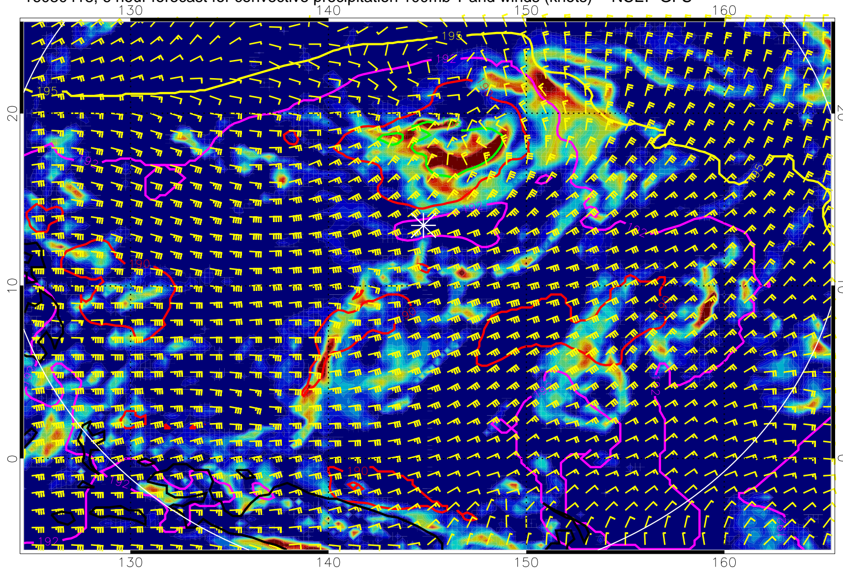
16080418, 6 hour forecast for convective precipitation 100mb T and winds (knots) -- NCEP GFS
