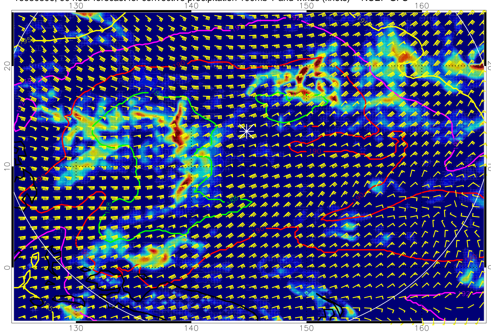
16080806, 90 hour forecast for convective precipitation 100mb T and winds (knots) -- NCEP GFS
