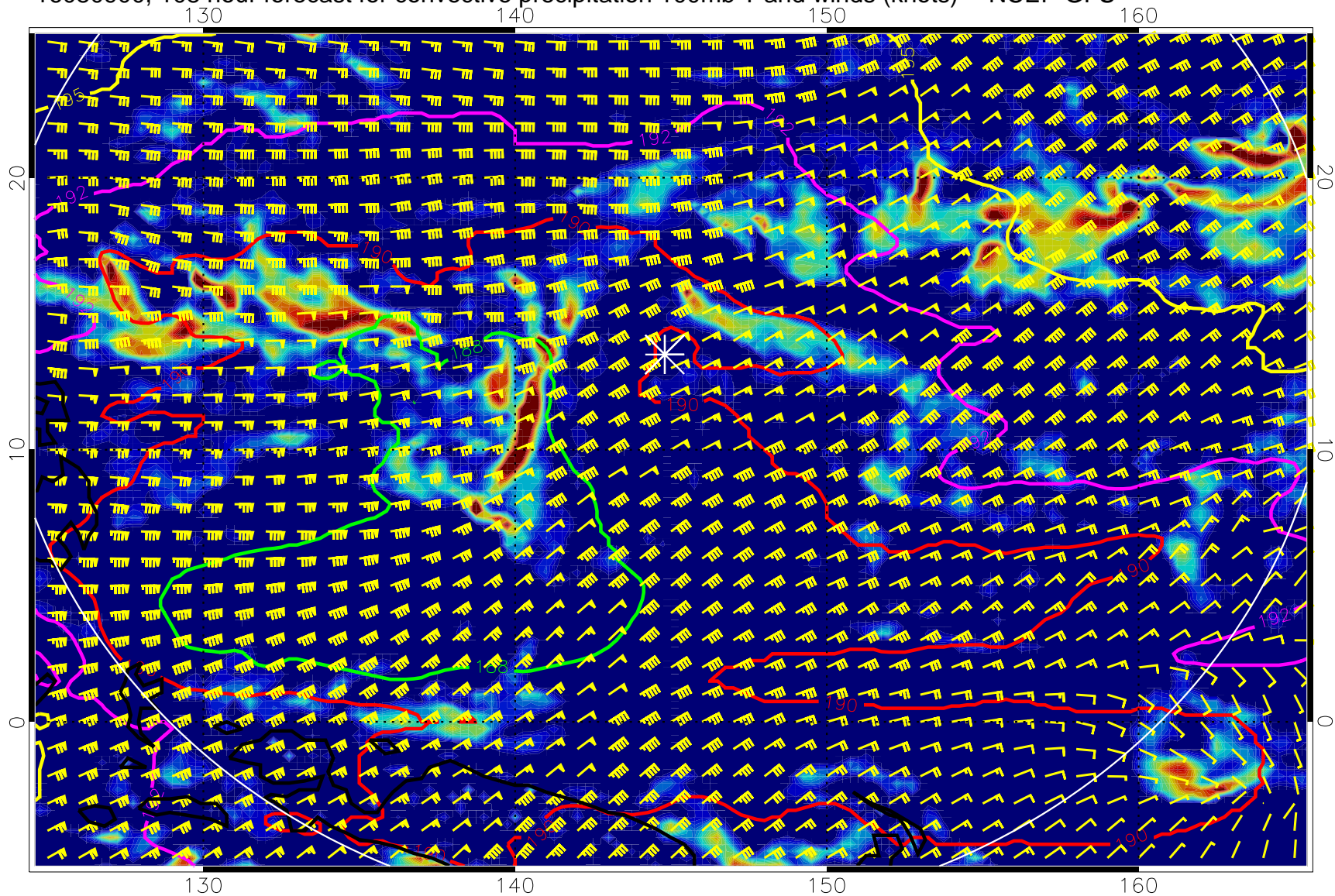
16080900, 108 hour forecast for convective precipitation 100mb T and winds (knots) -- NCEP GFS
