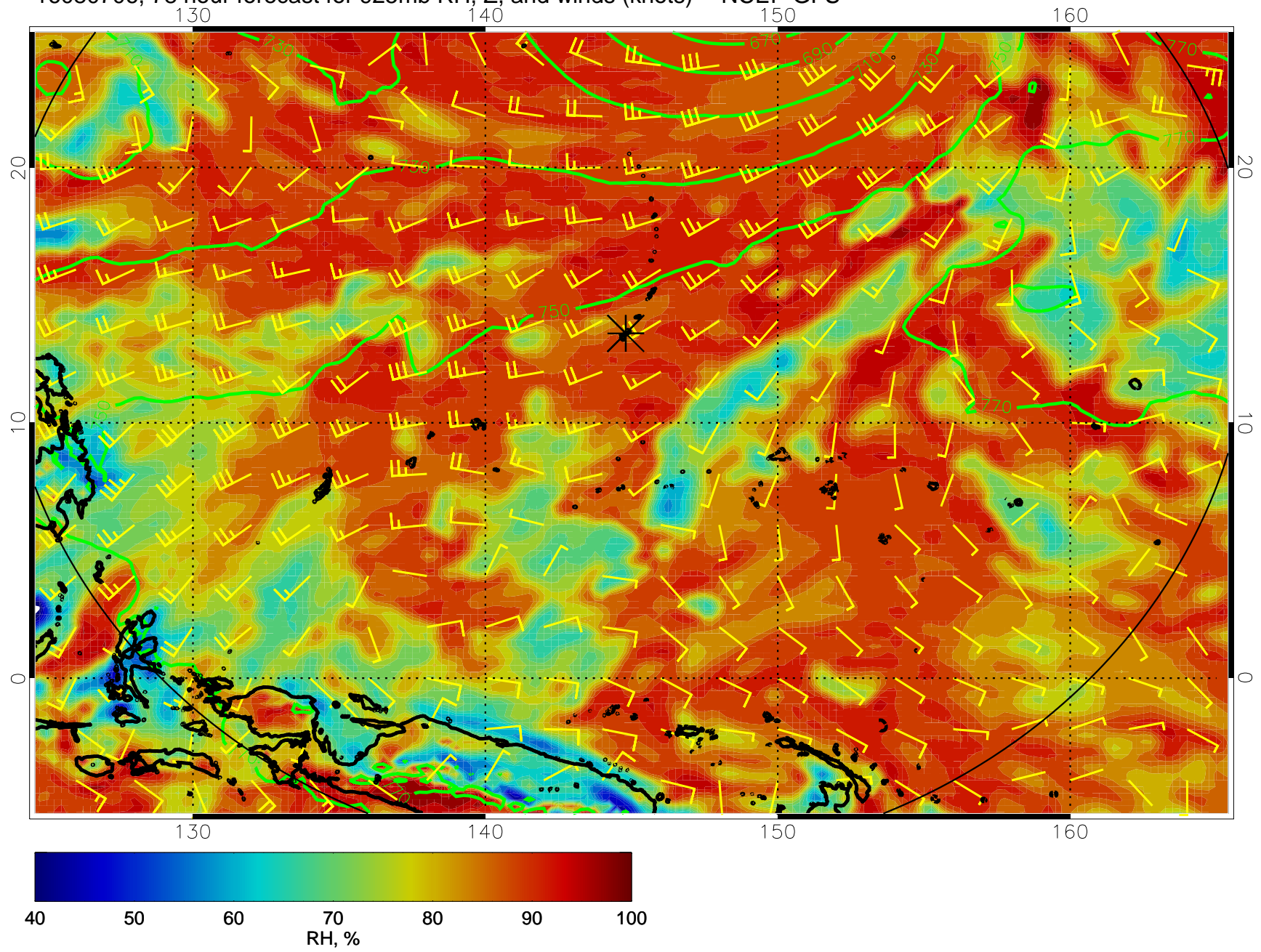
16080706, 78 hour forecast for 925mb RH, Z, and winds (knots) -- NCEP GFS
