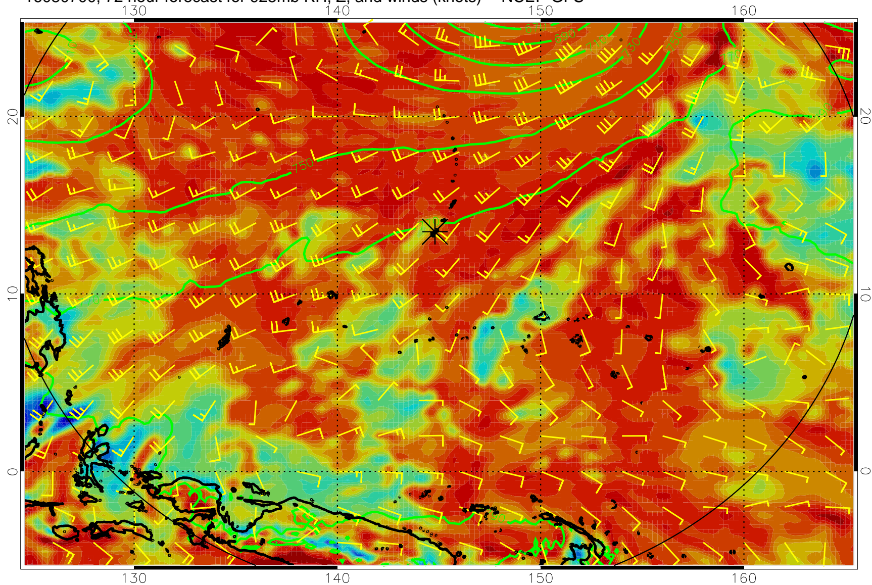
16080700, 72 hour forecast for 925mb RH, Z, and winds (knots) -- NCEP GFS
