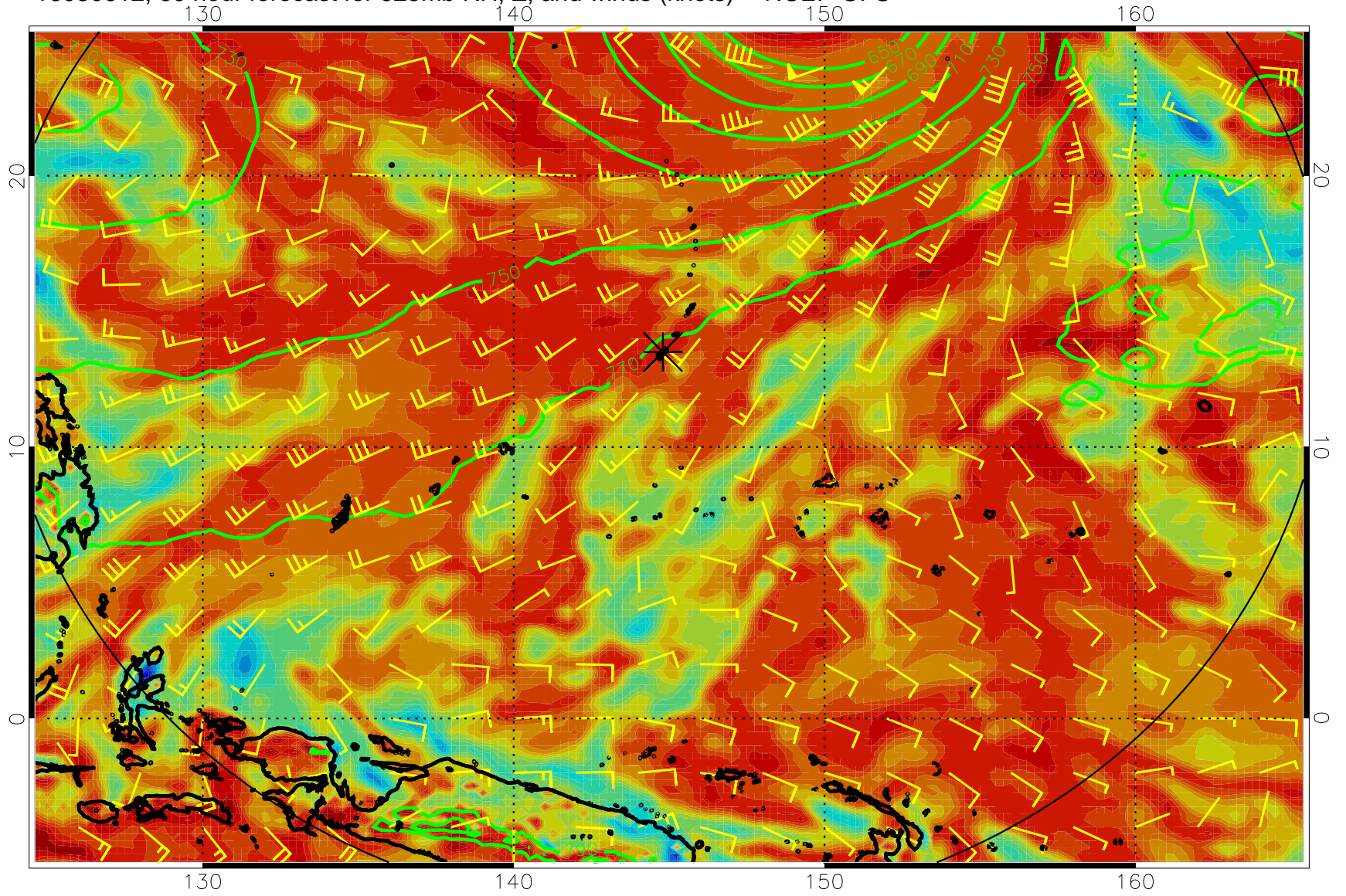
16080612, 60 hour forecast for 925mb RH, Z, and winds (knots) -- NCEP GFS
