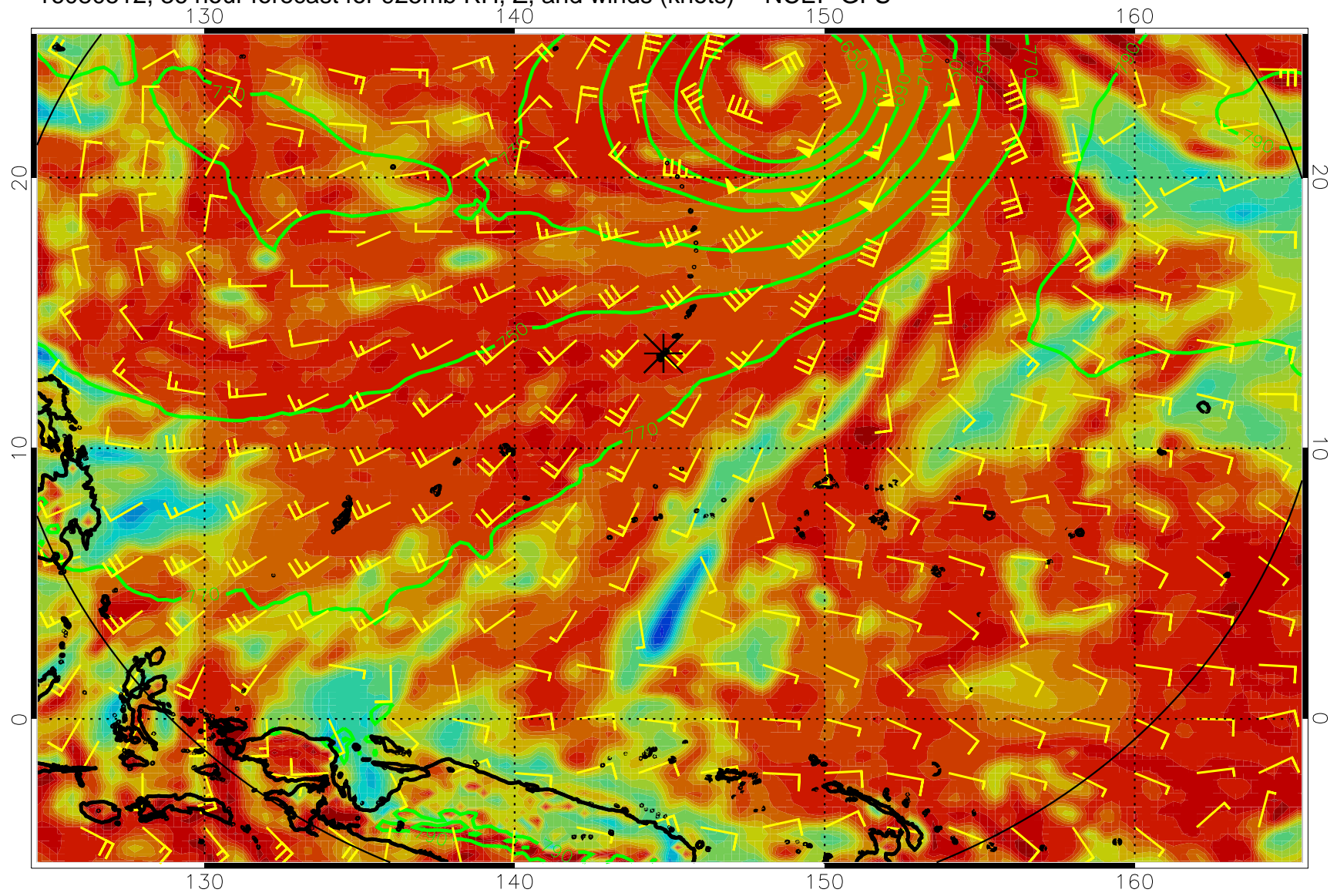
16080512, 36 hour forecast for 925mb RH, Z, and winds (knots) -- NCEP GFS
