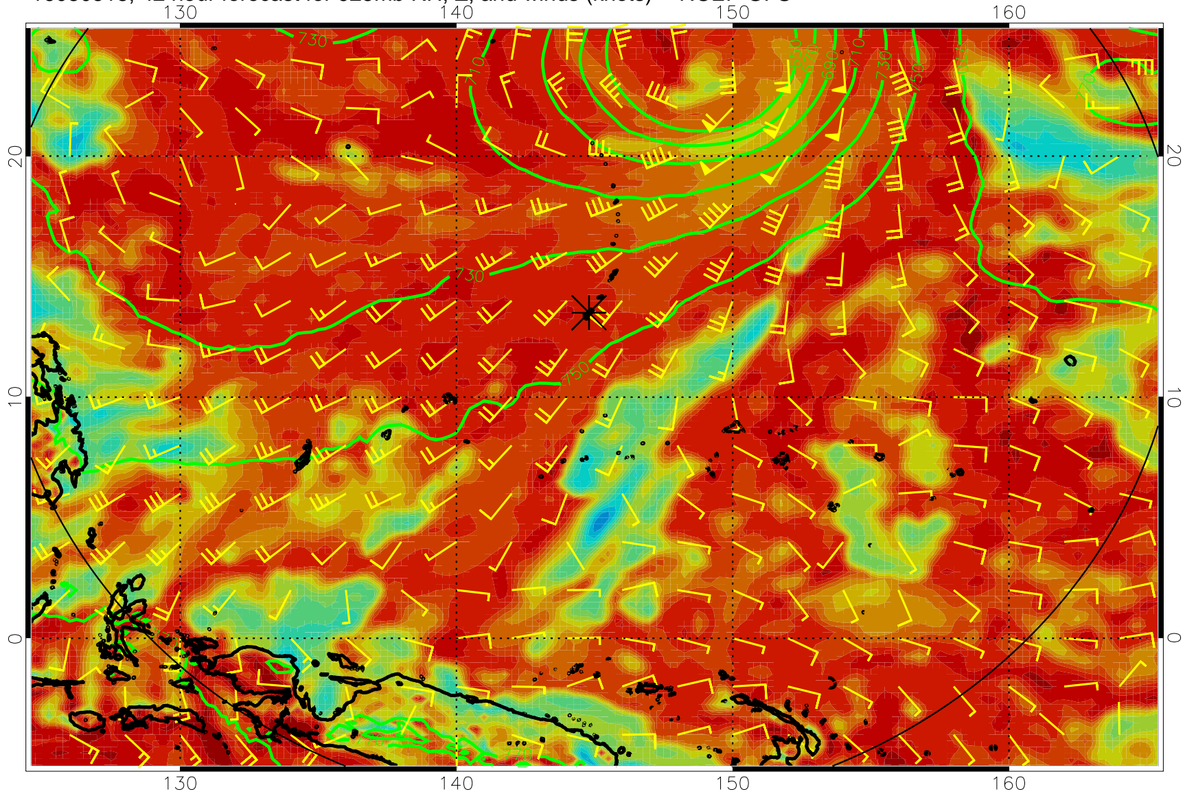
16080518, 42 hour forecast for 925mb RH, Z, and winds (knots) -- NCEP GFS
