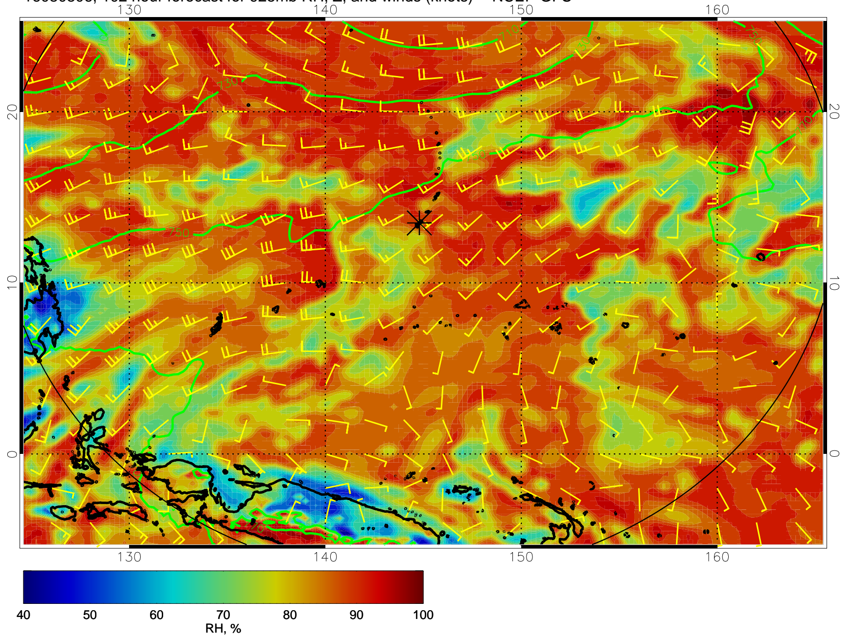
16080806, 102 hour forecast for 925mb RH, Z, and winds (knots) -- NCEP GFS
