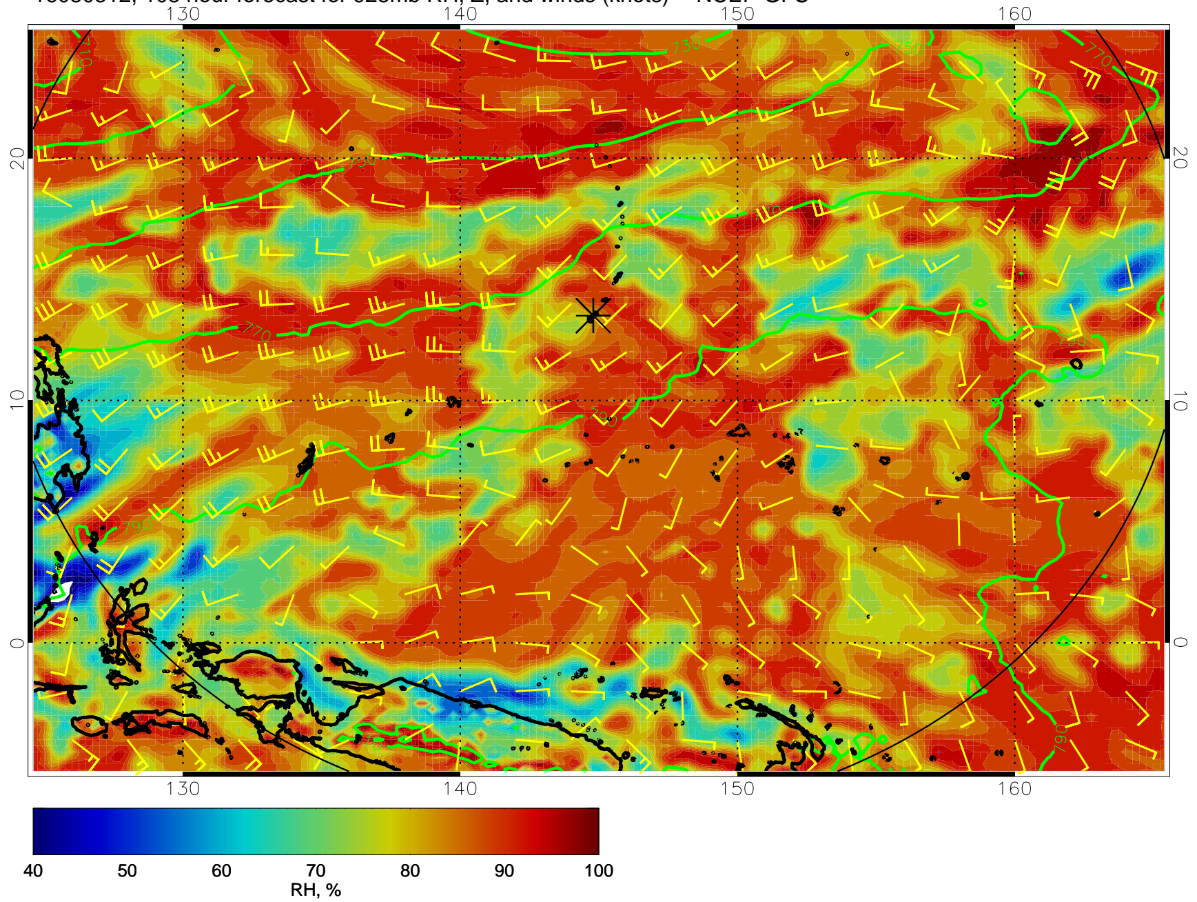
16080812, 108 hour forecast for 925mb RH, Z, and winds (knots) -- NCEP GFS
