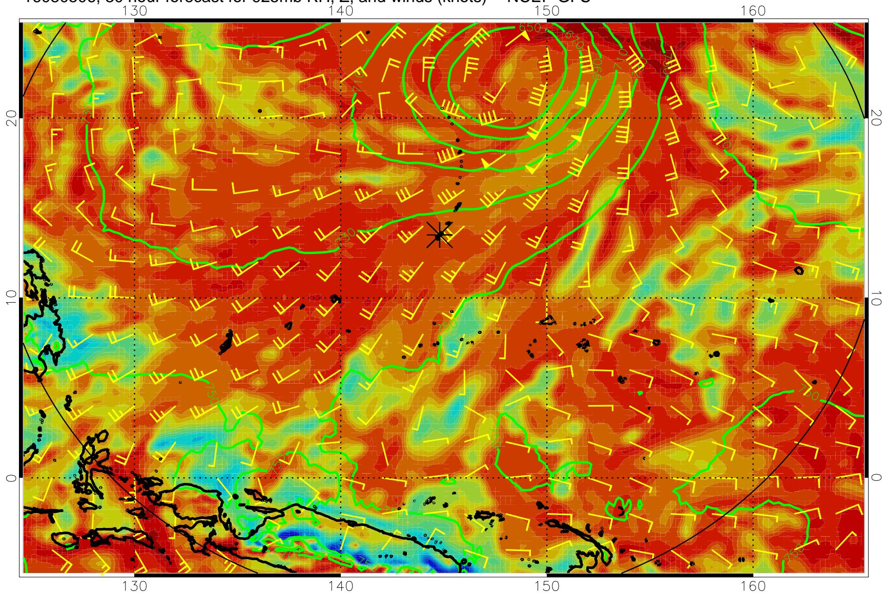
16080506, 30 hour forecast for 925mb RH, Z, and winds (knots) -- NCEP GFS
