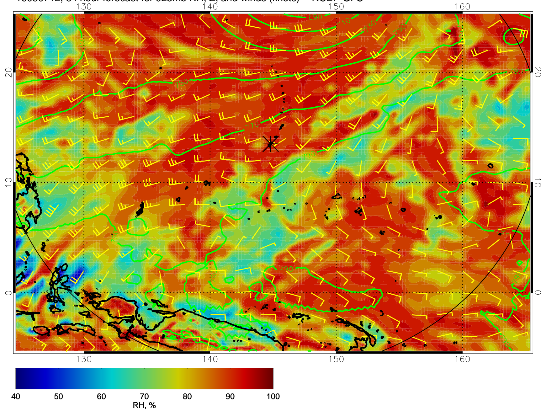
16080712, 84 hour forecast for 925mb RH, Z, and winds (knots) -- NCEP GFS
