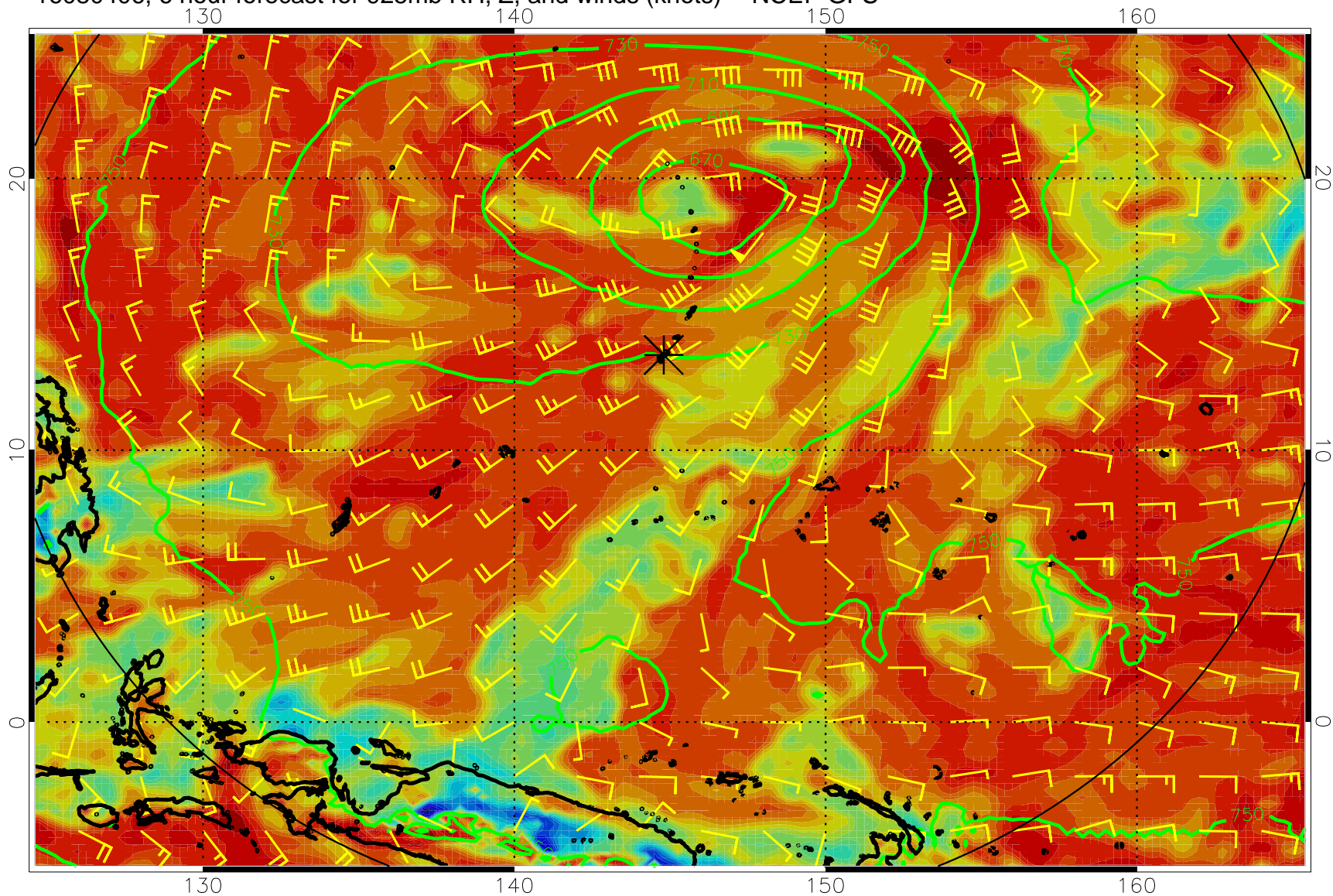
16080406, 6 hour forecast for 925mb RH, Z, and winds (knots) -- NCEP GFS
