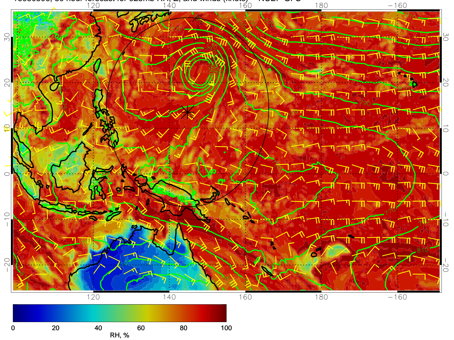
16080506, 30 hour forecast for 925mb RH, Z, and winds (knots) -- NCEP GFS
