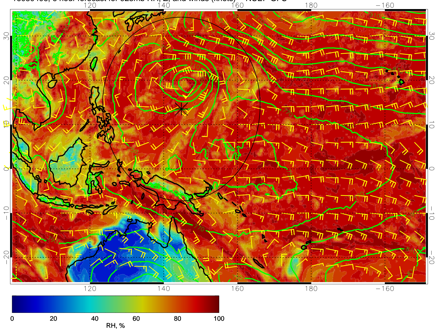
16080406, 6 hour forecast for 925mb RH, Z, and winds (knots) -- NCEP GFS
