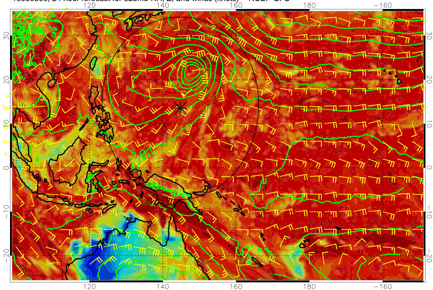
16080500, 24 hour forecast for 925mb RH, Z, and winds (knots) -- NCEP GFS
