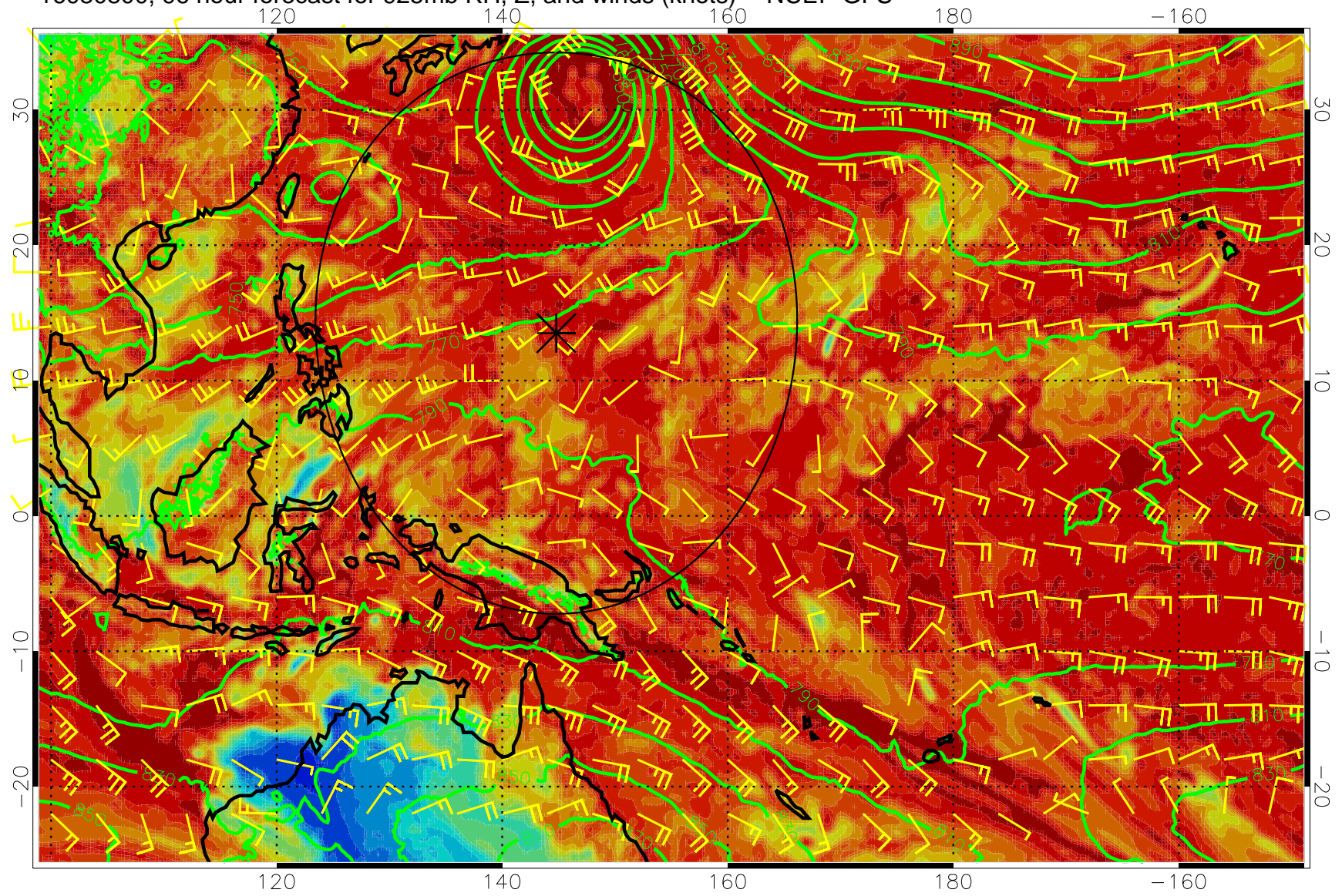
16080800, 96 hour forecast for 925mb RH, Z, and winds (knots) -- NCEP GFS
