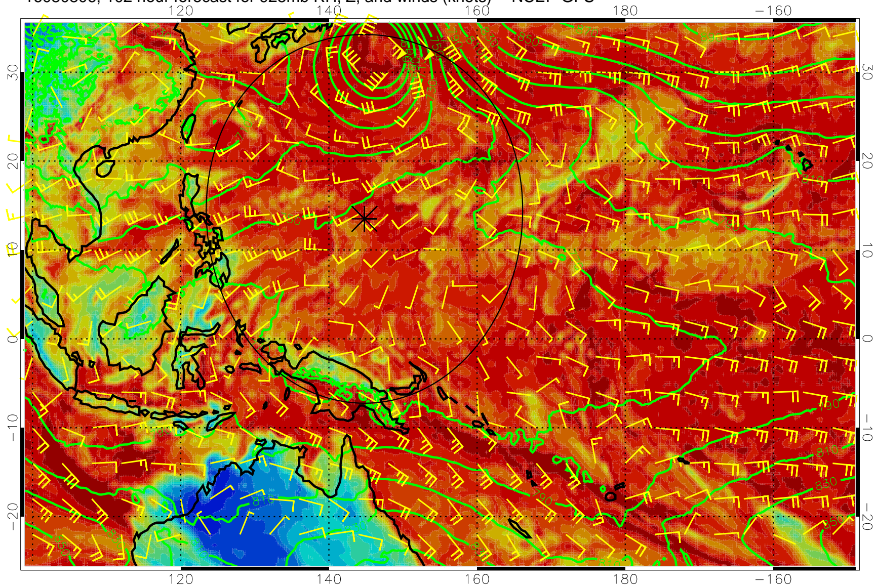
16080806, 102 hour forecast for 925mb RH, Z, and winds (knots) -- NCEP GFS
