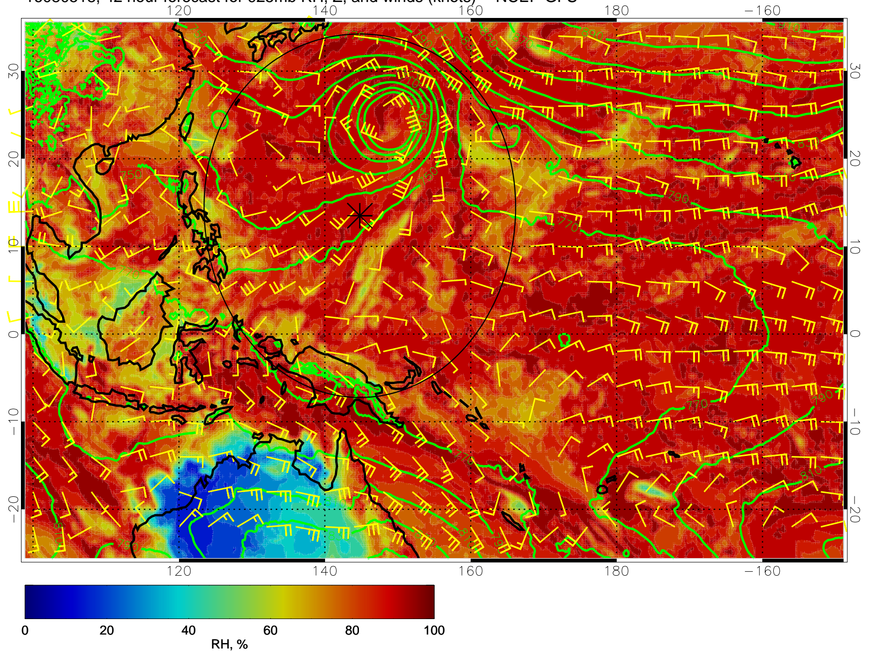
16080518, 42 hour forecast for 925mb RH, Z, and winds (knots) -- NCEP GFS
