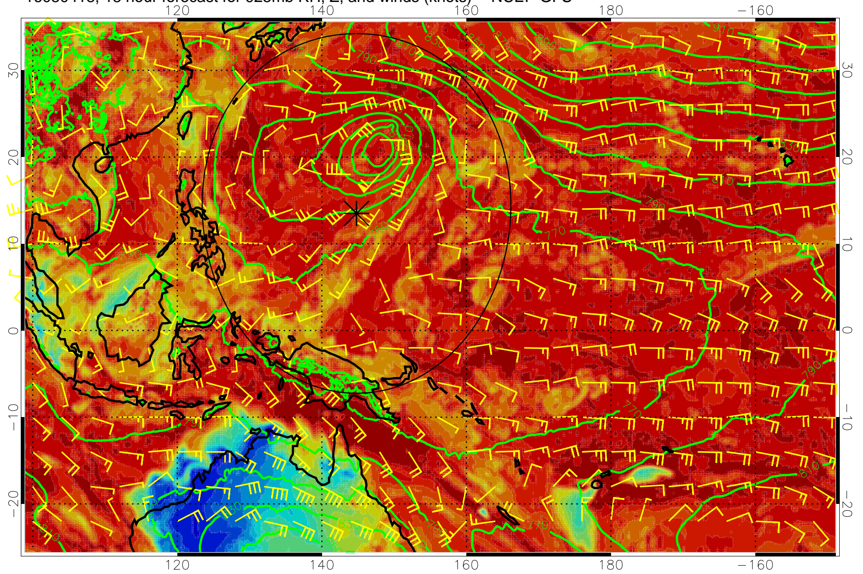
16080418, 18 hour forecast for 925mb RH, Z, and winds (knots) -- NCEP GFS
