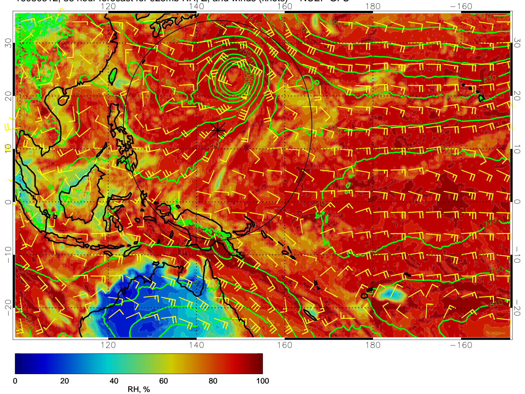
16080512, 36 hour forecast for 925mb RH, Z, and winds (knots) -- NCEP GFS
