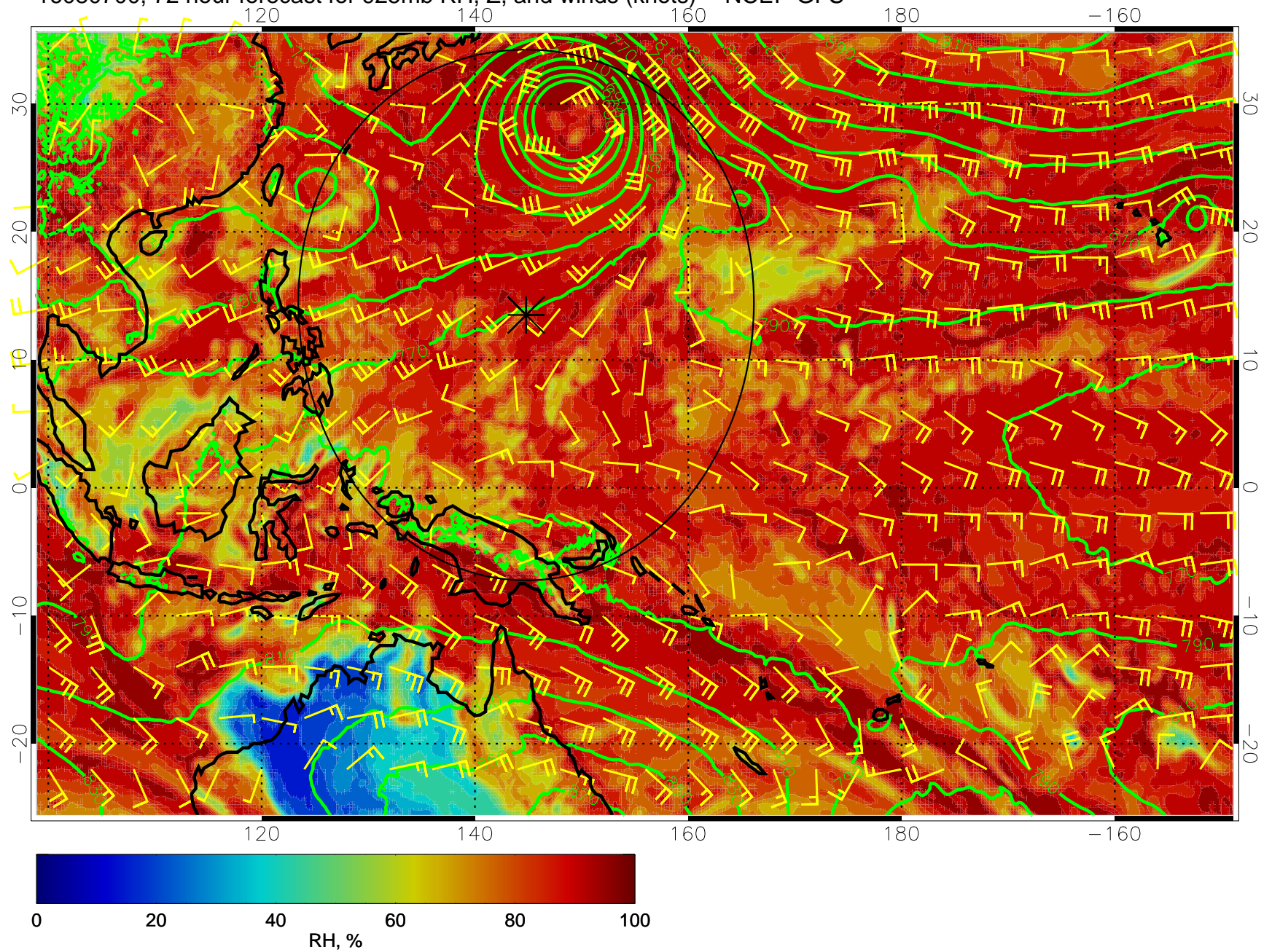
16080700, 72 hour forecast for 925mb RH, Z, and winds (knots) -- NCEP GFS
