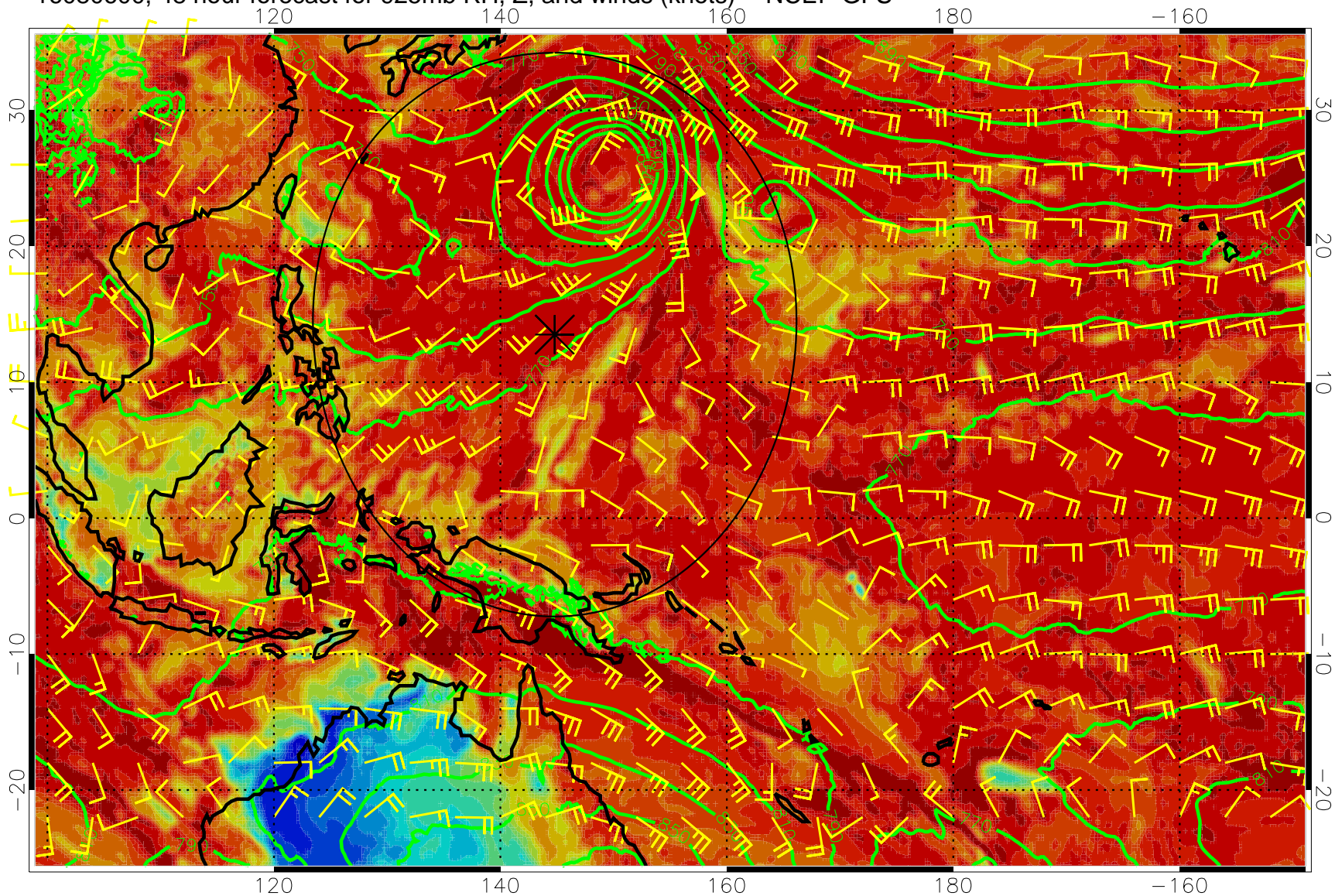
16080600, 48 hour forecast for 925mb RH, Z, and winds (knots) -- NCEP GFS
