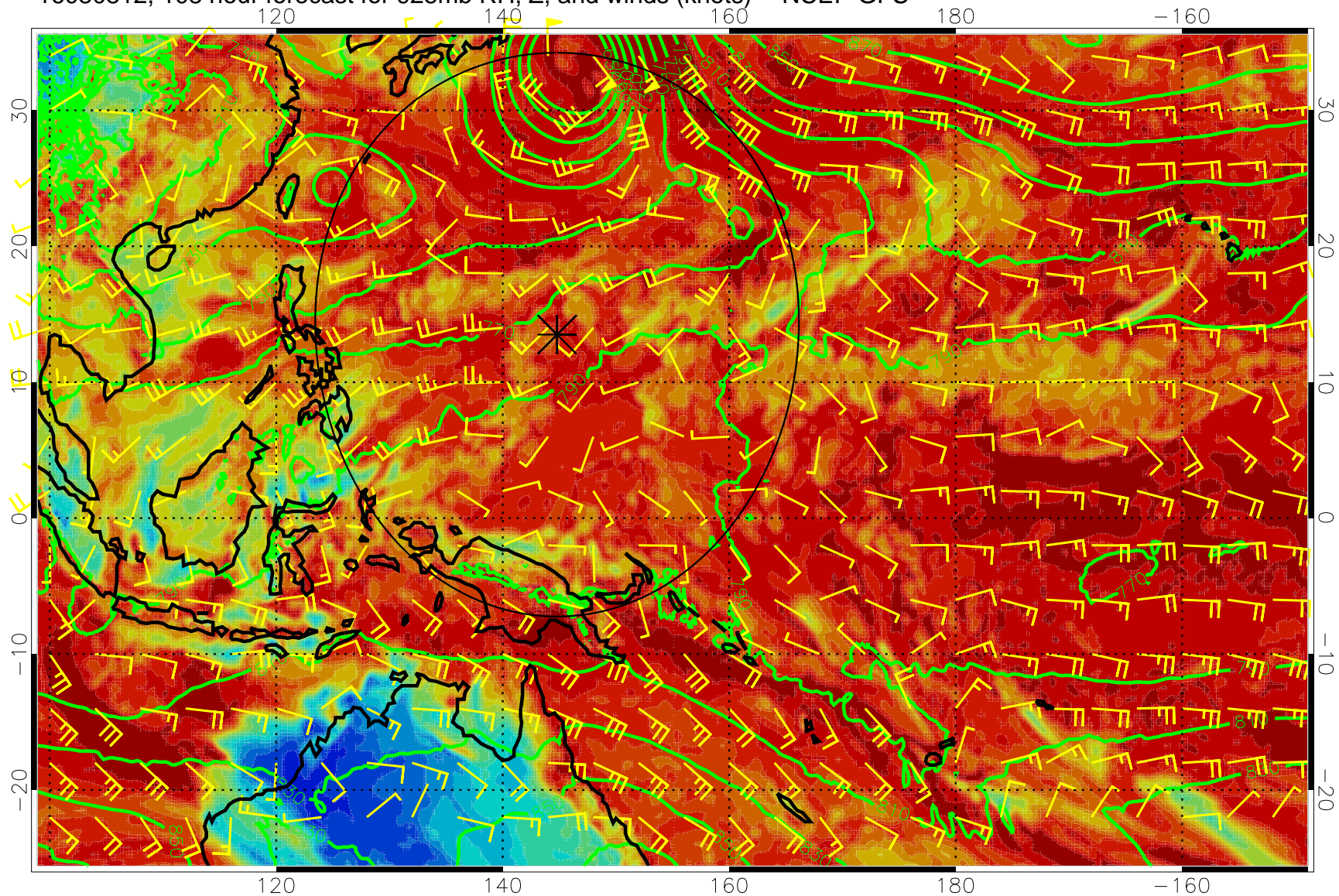
16080812, 108 hour forecast for 925mb RH, Z, and winds (knots) -- NCEP GFS
