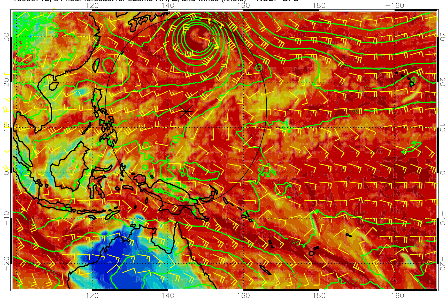
16080712, 84 hour forecast for 925mb RH, Z, and winds (knots) -- NCEP GFS
