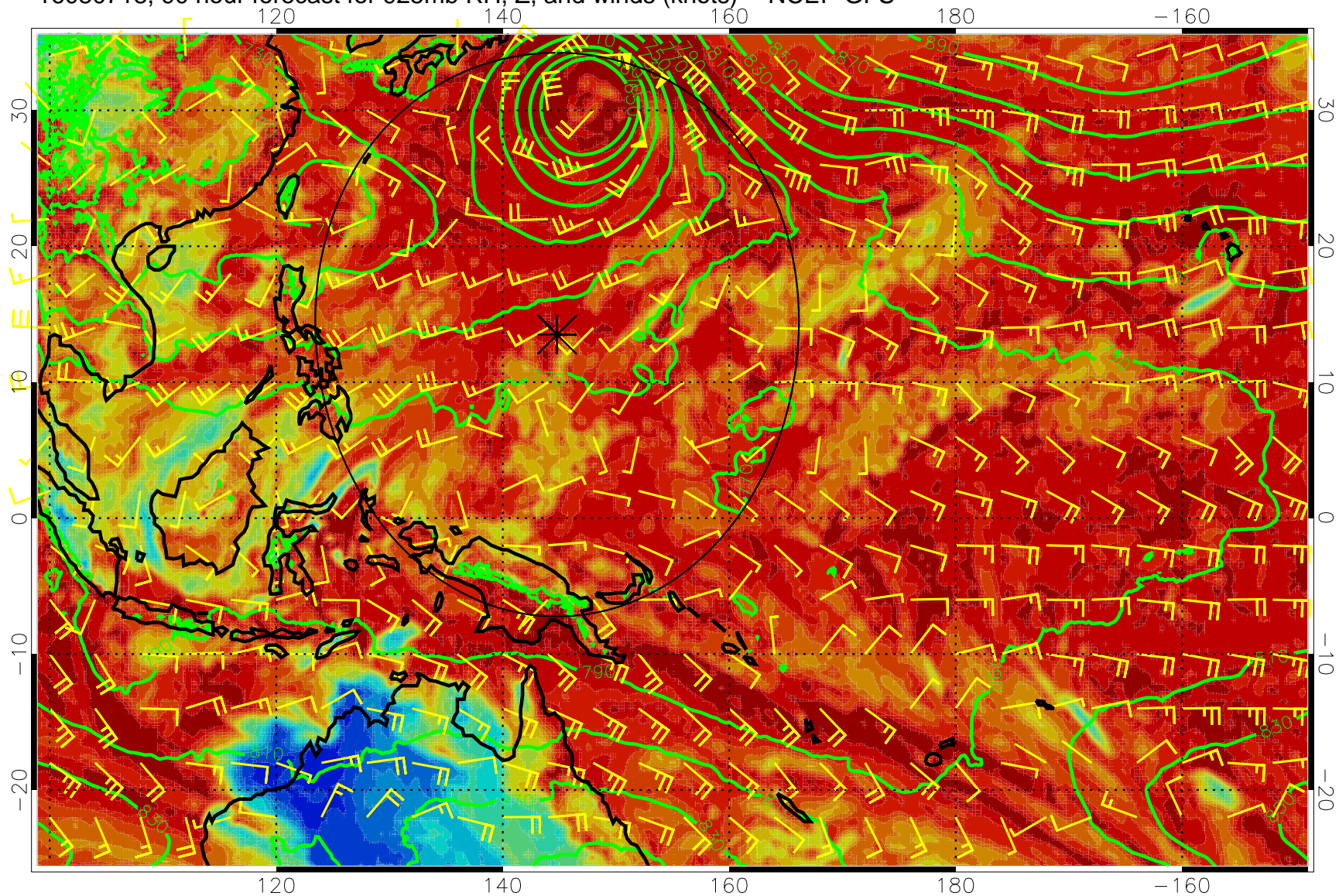
16080718, 90 hour forecast for 925mb RH, Z, and winds (knots) -- NCEP GFS
