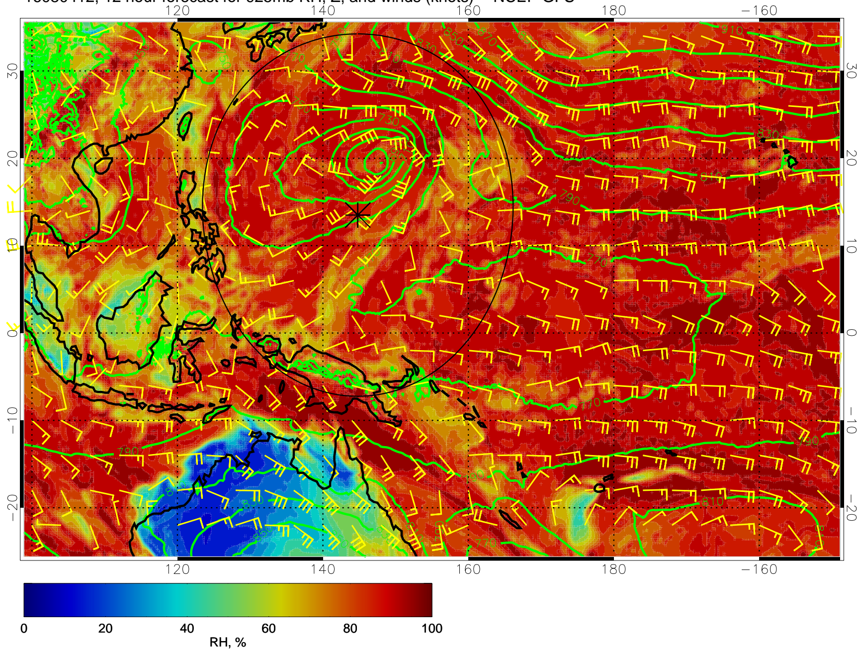
16080412, 12 hour forecast for 925mb RH, Z, and winds (knots) -- NCEP GFS
