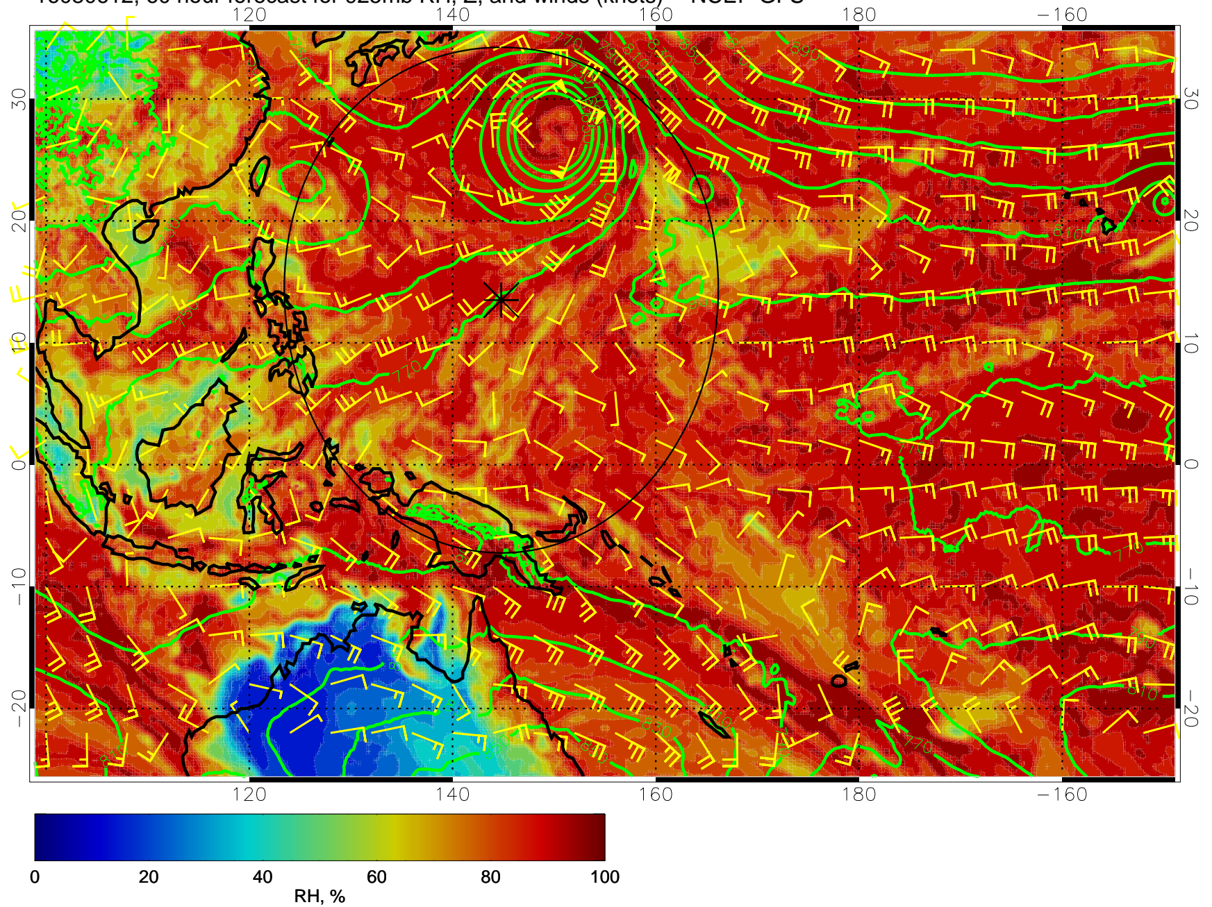
16080612, 60 hour forecast for 925mb RH, Z, and winds (knots) -- NCEP GFS
