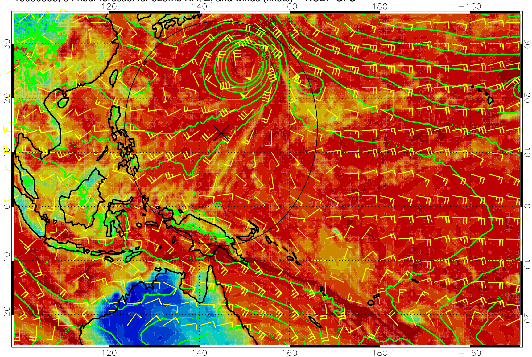
16080606, 54 hour forecast for 925mb RH, Z, and winds (knots) -- NCEP GFS
