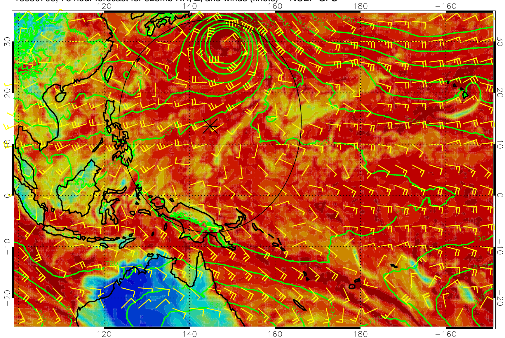
16080706, 78 hour forecast for 925mb RH, Z, and winds (knots) -- NCEP GFS
