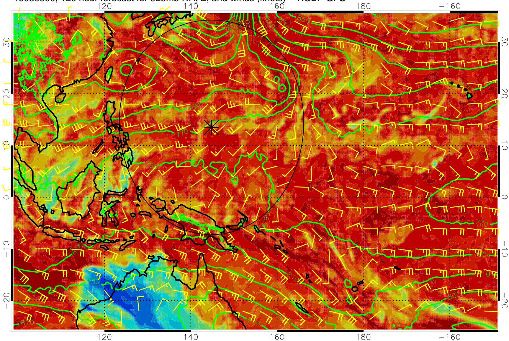
16080900, 120 hour forecast for 925mb RH, Z, and winds (knots) -- NCEP GFS
