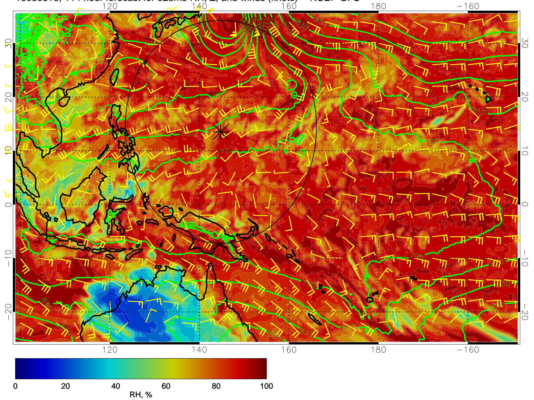
16080818, 114 hour forecast for 925mb RH, Z, and winds (knots) -- NCEP GFS
