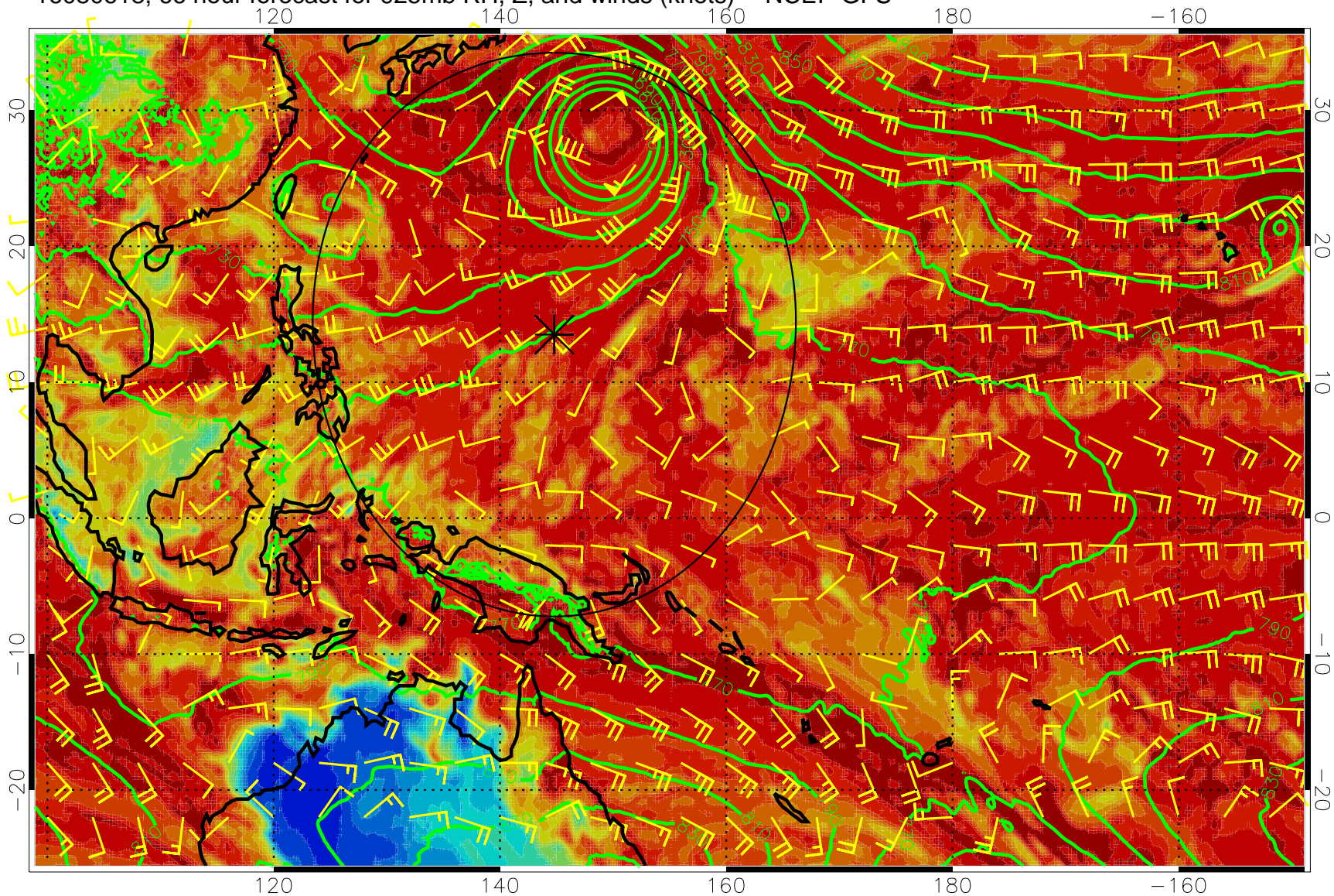
16080618, 66 hour forecast for 925mb RH, Z, and winds (knots) -- NCEP GFS
