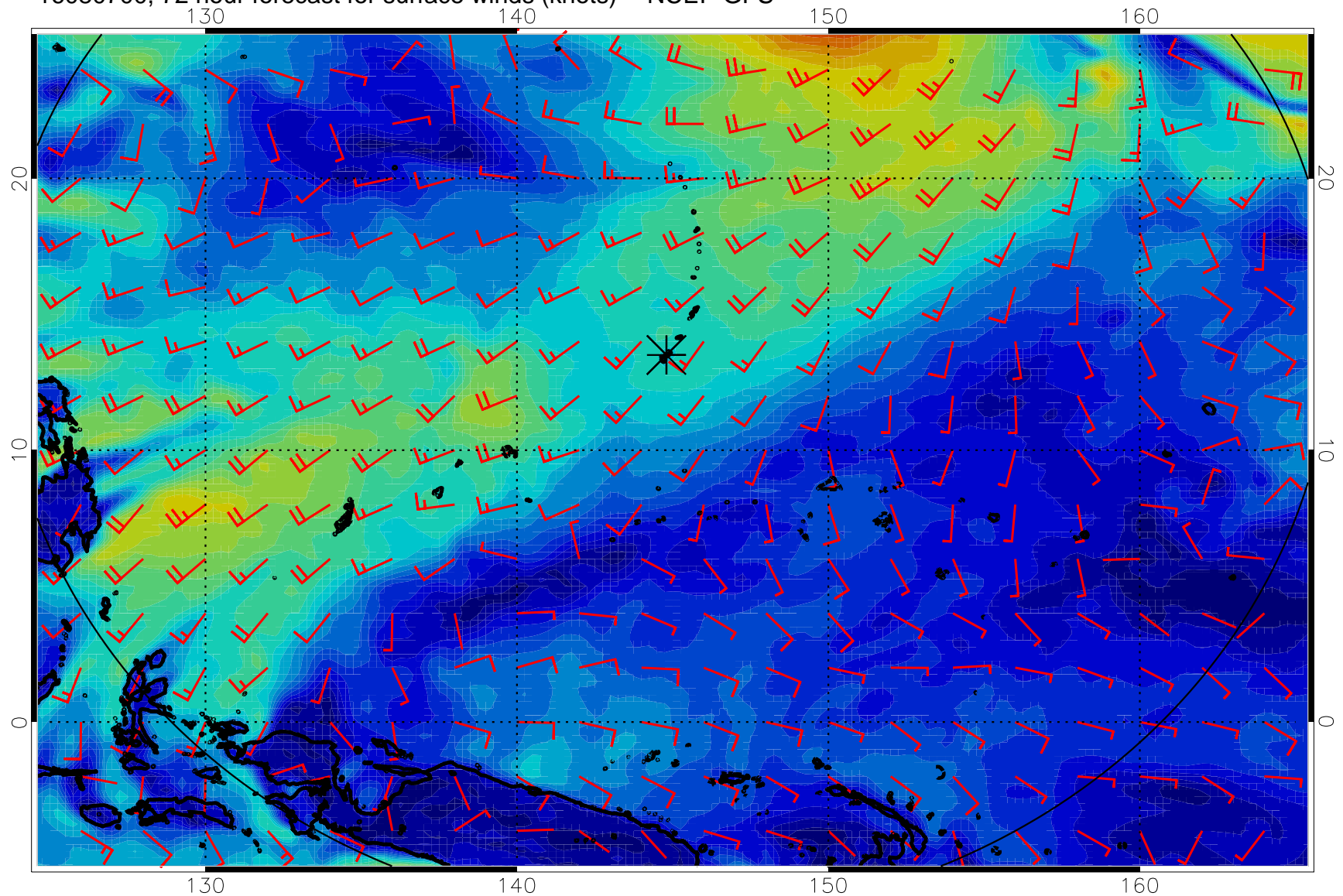
16080700, 72 hour forecast for surface winds (knots) -- NCEP GFS
