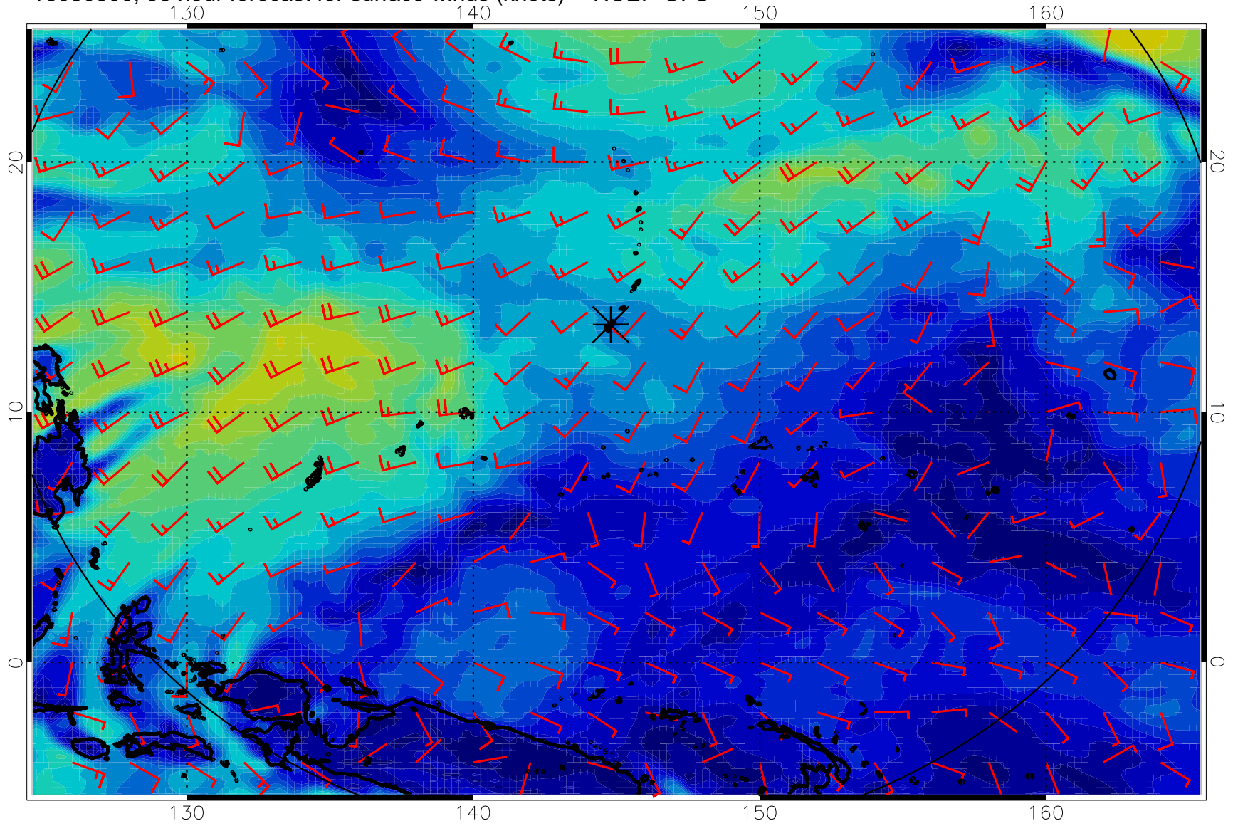
16080800, 96 hour forecast for surface winds (knots) -- NCEP GFS
