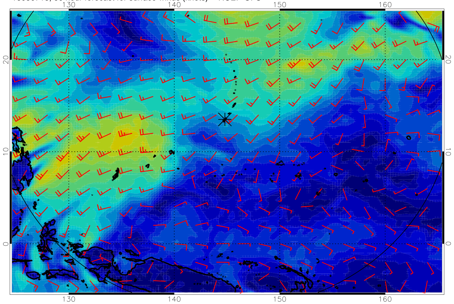
16080718, 90 hour forecast for surface winds (knots) -- NCEP GFS
