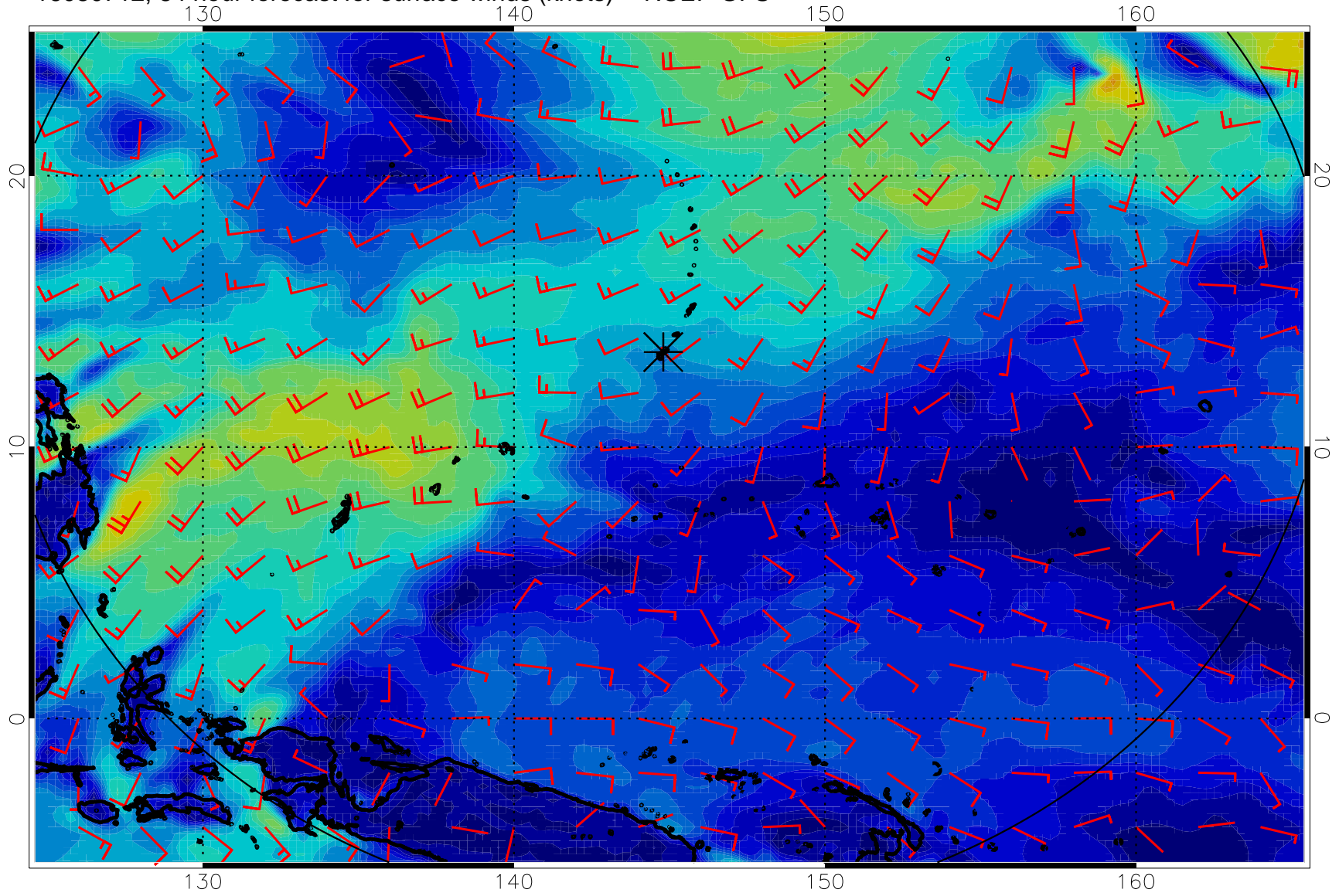
16080712, 84 hour forecast for surface winds (knots) -- NCEP GFS
