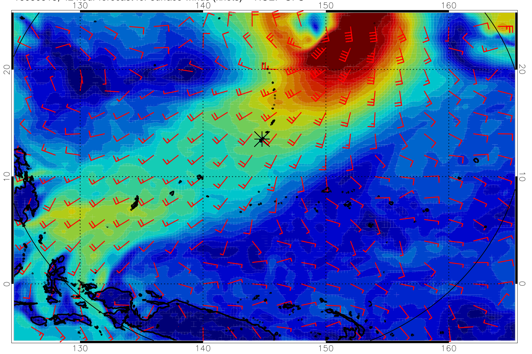
16080518, 42 hour forecast for surface winds (knots) -- NCEP GFS
