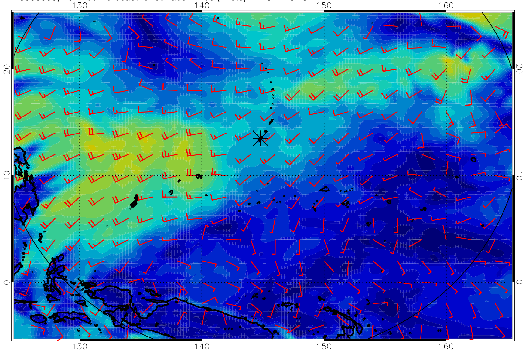
16080806, 102 hour forecast for surface winds (knots) -- NCEP GFS
