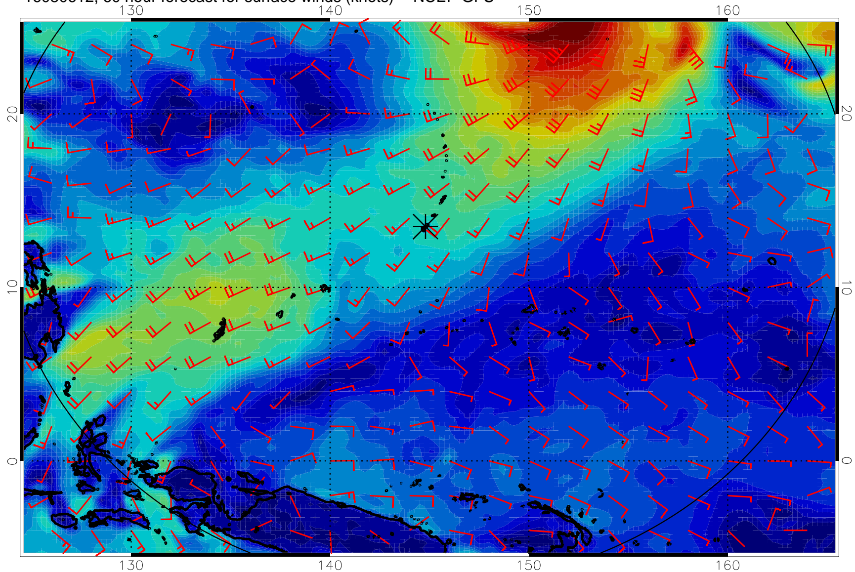
16080612, 60 hour forecast for surface winds (knots) -- NCEP GFS
