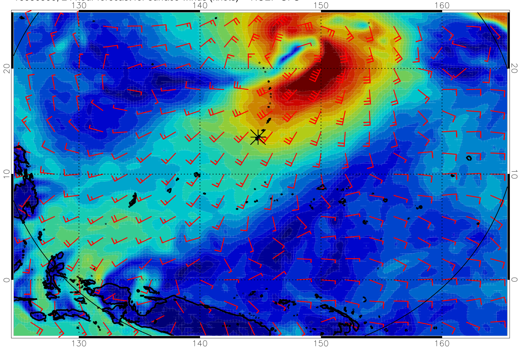
16080500, 24 hour forecast for surface winds (knots) -- NCEP GFS
