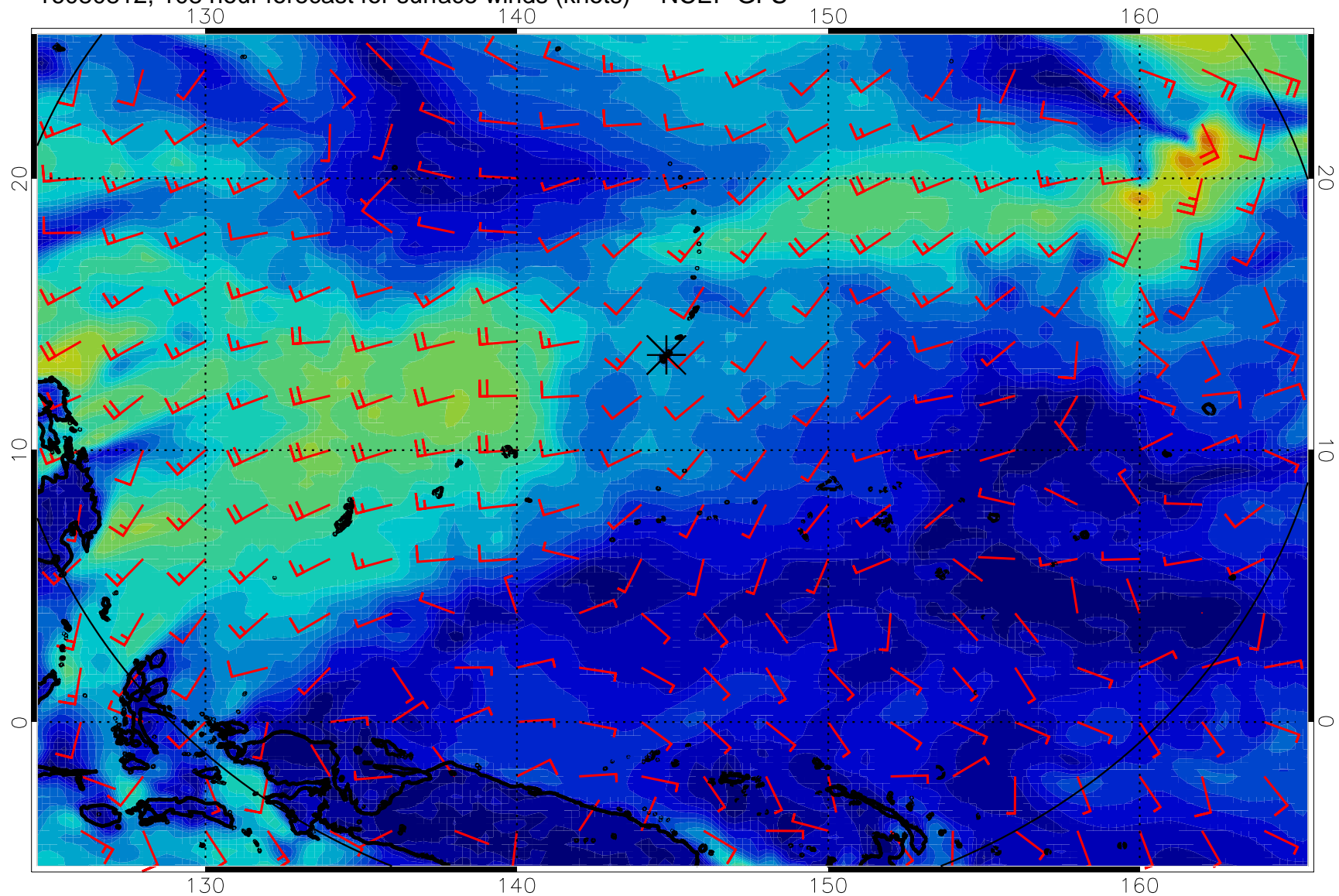
16080812, 108 hour forecast for surface winds (knots) -- NCEP GFS
