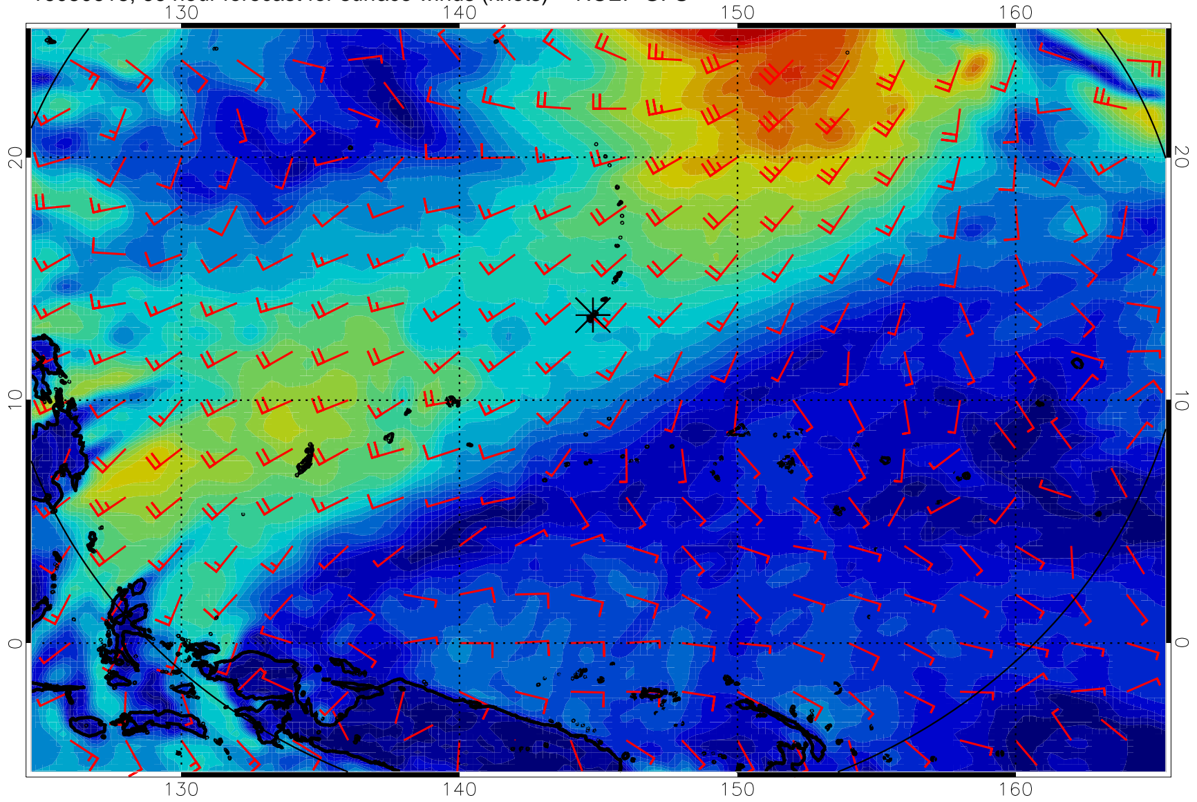
16080618, 66 hour forecast for surface winds (knots) -- NCEP GFS
