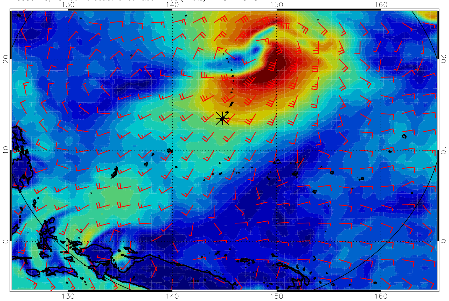
16080418, 18 hour forecast for surface winds (knots) -- NCEP GFS
