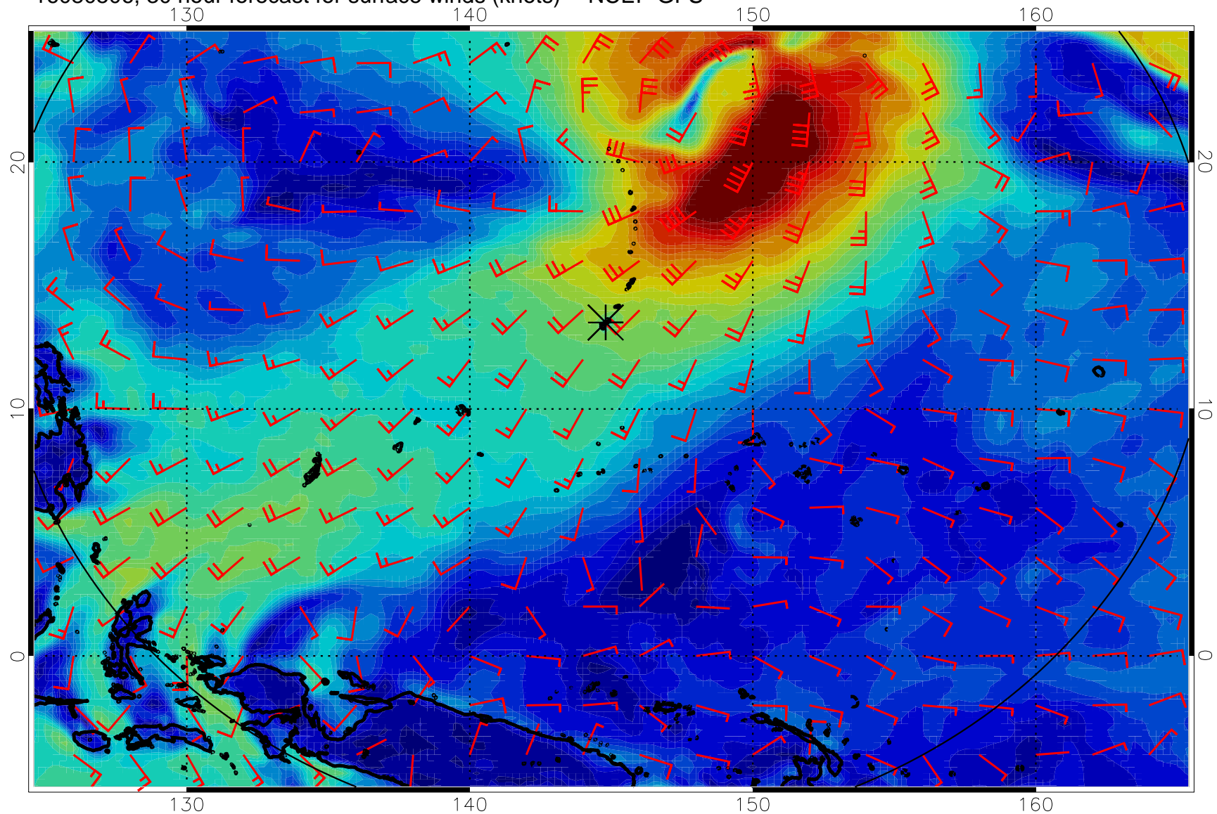
16080506, 30 hour forecast for surface winds (knots) -- NCEP GFS
