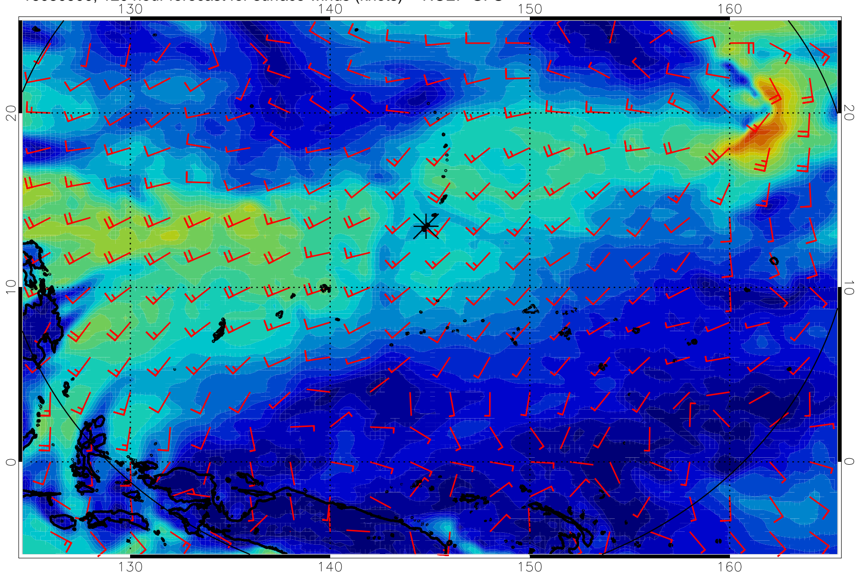
16080900, 120 hour forecast for surface winds (knots) -- NCEP GFS
