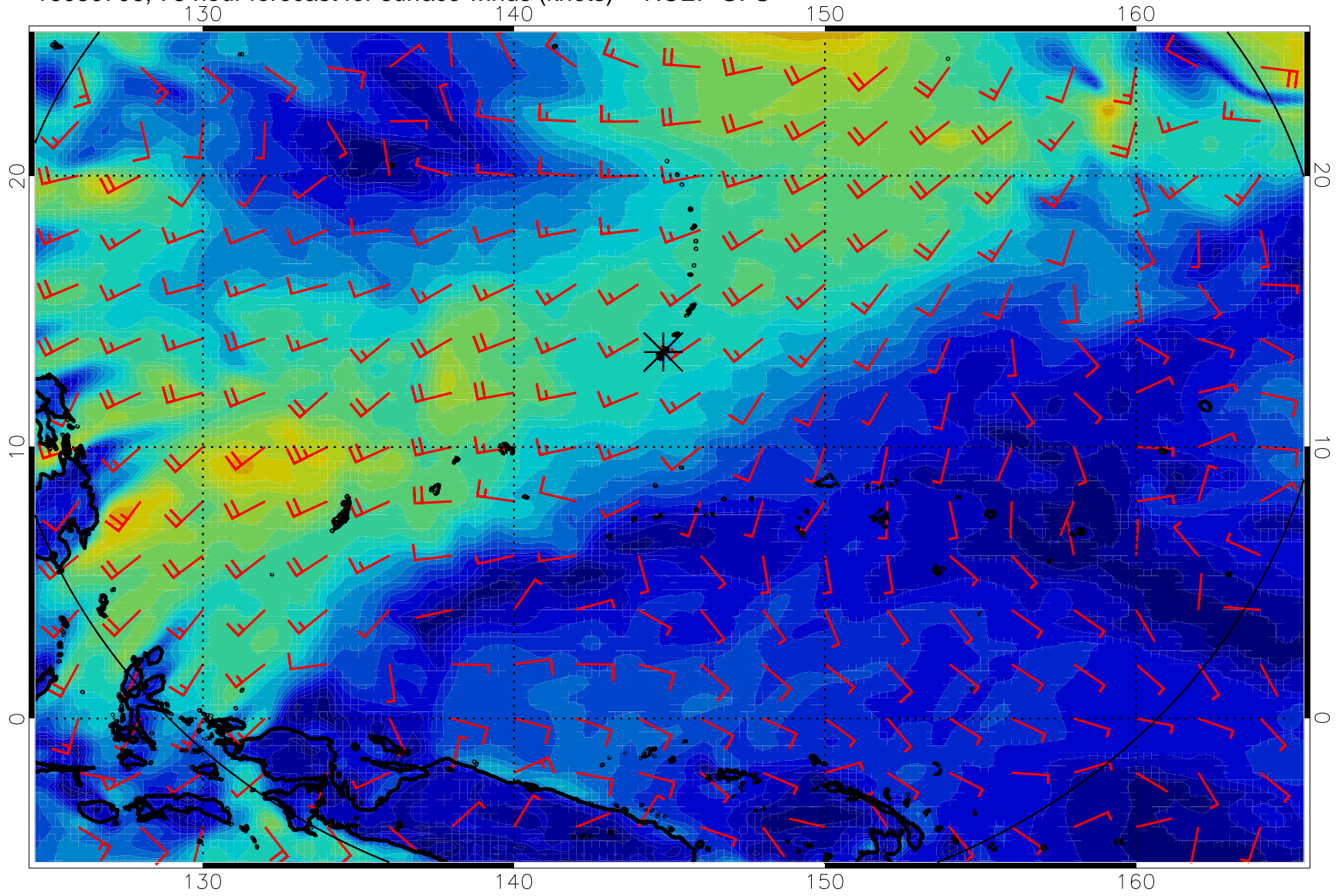
16080706, 78 hour forecast for surface winds (knots) -- NCEP GFS
