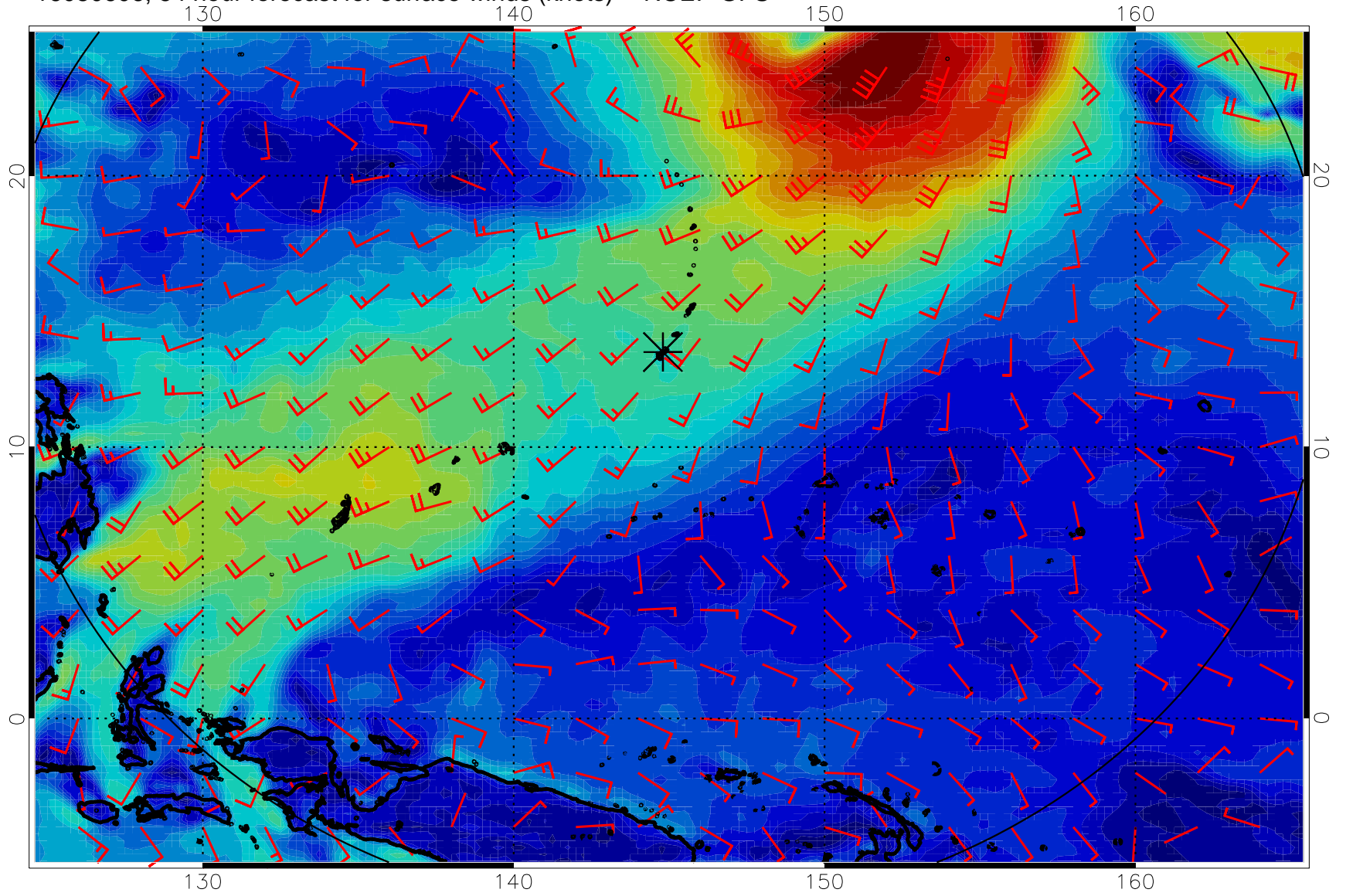
16080606, 54 hour forecast for surface winds (knots) -- NCEP GFS
