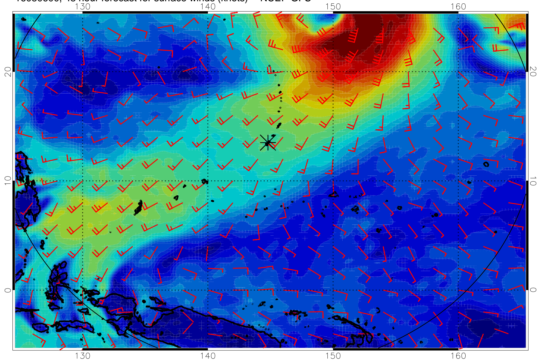
16080600, 48 hour forecast for surface winds (knots) -- NCEP GFS
