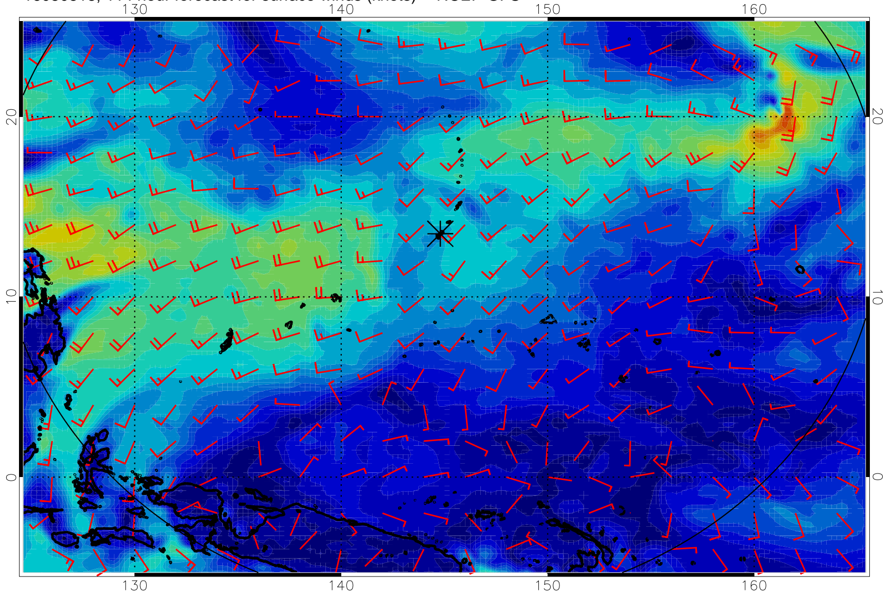
16080818, 114 hour forecast for surface winds (knots) -- NCEP GFS
