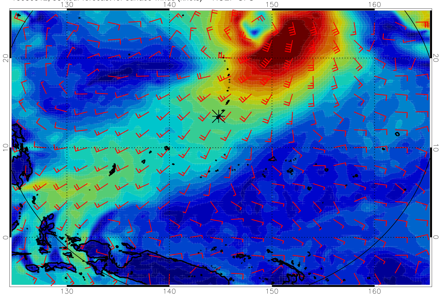
16080512, 36 hour forecast for surface winds (knots) -- NCEP GFS
