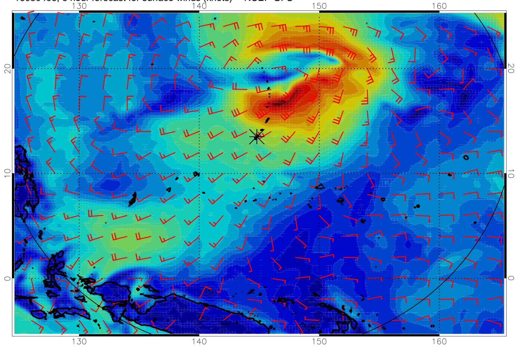
16080406, 6 hour forecast for surface winds (knots) -- NCEP GFS
