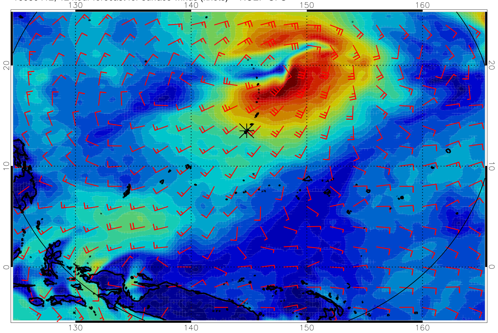
16080412, 12 hour forecast for surface winds (knots) -- NCEP GFS
