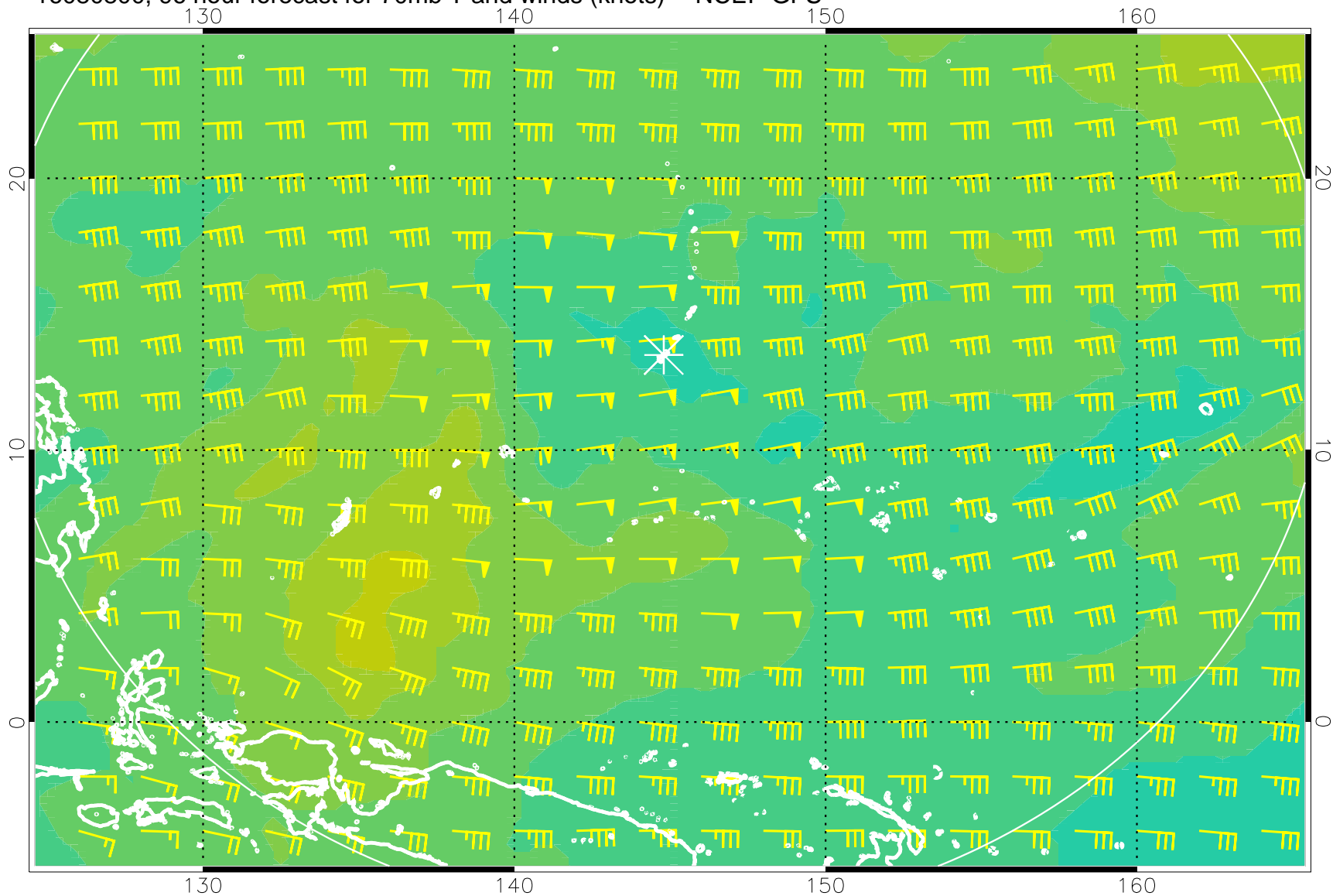
16080800, 96 hour forecast for 70mb T and winds (knots) -- NCEP GFS
