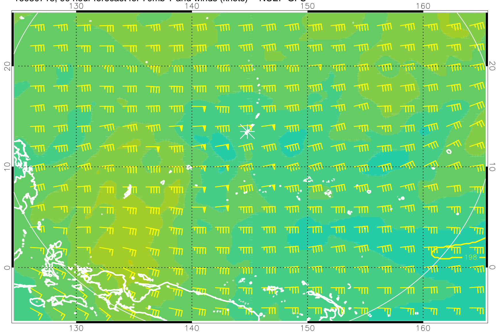
16080718, 90 hour forecast for 70mb T and winds (knots) -- NCEP GFS
