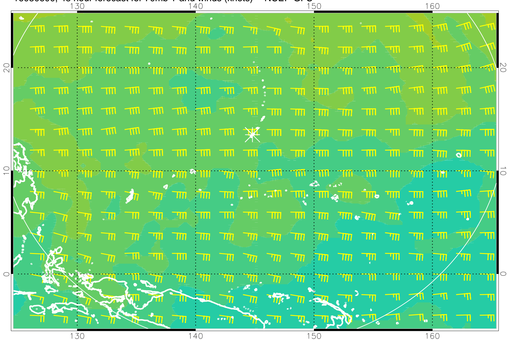
16080600, 48 hour forecast for 70mb T and winds (knots) -- NCEP GFS
