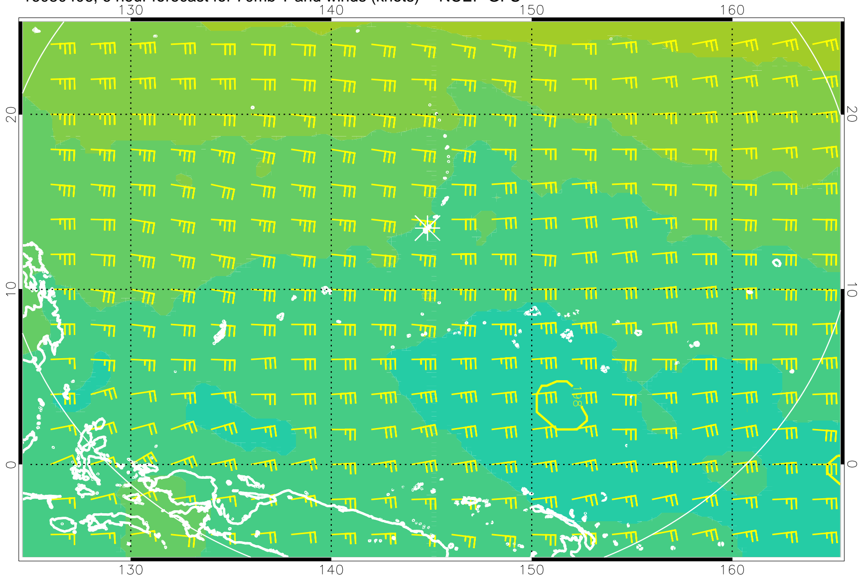
16080406, 6 hour forecast for 70mb T and winds (knots) -- NCEP GFS
