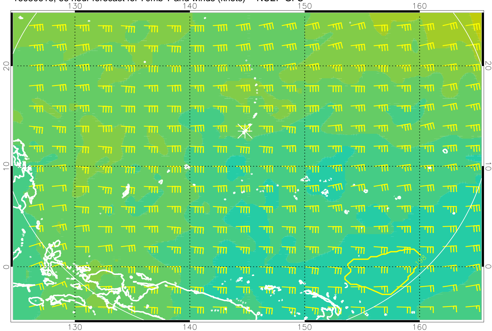
16080618, 66 hour forecast for 70mb T and winds (knots) -- NCEP GFS
