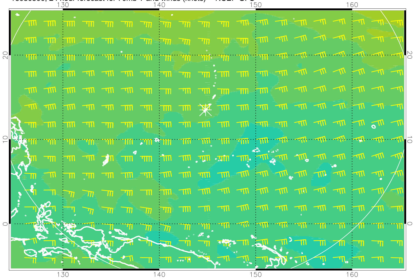
16080500, 24 hour forecast for 70mb T and winds (knots) -- NCEP GFS
