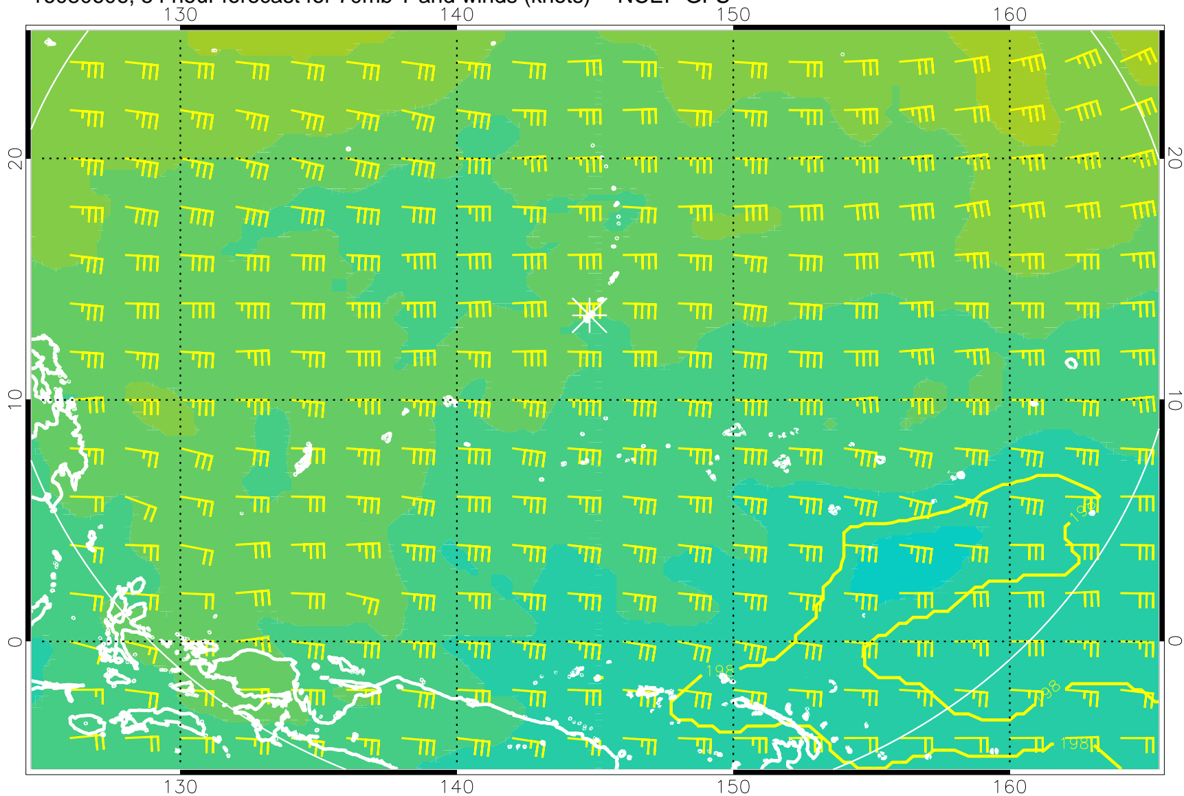
16080606, 54 hour forecast for 70mb T and winds (knots) -- NCEP GFS
