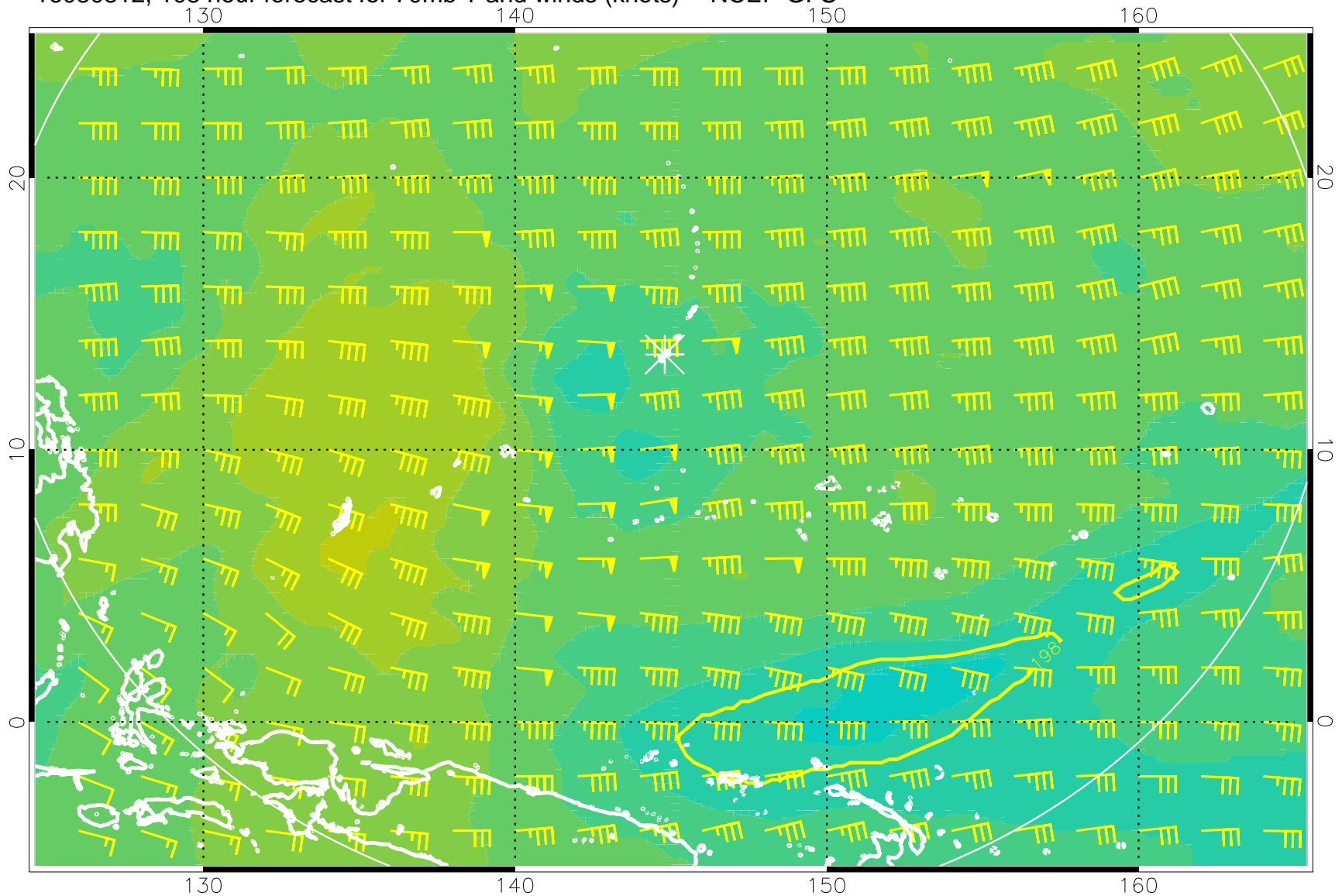
16080812, 108 hour forecast for 70mb T and winds (knots) -- NCEP GFS
