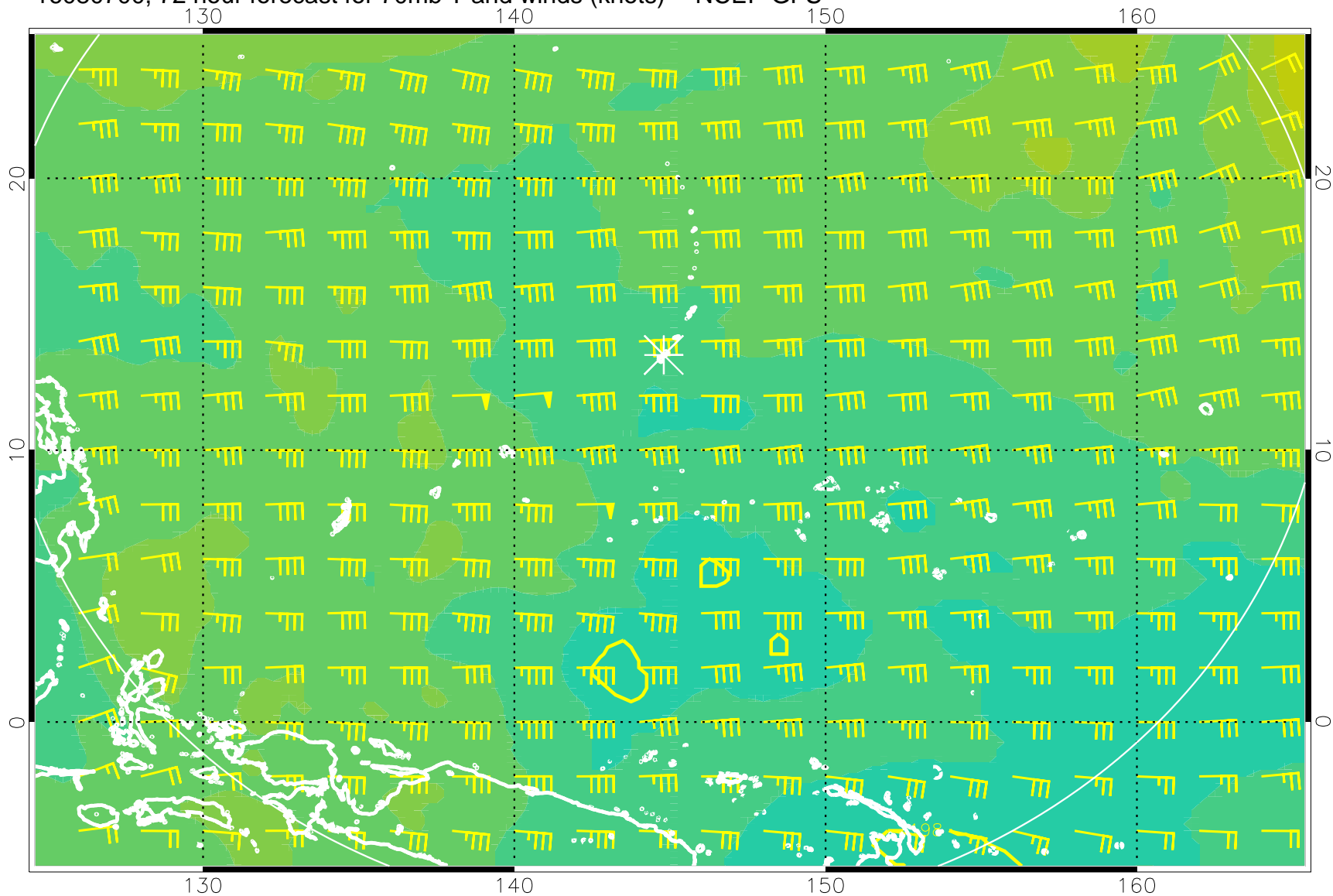
16080700, 72 hour forecast for 70mb T and winds (knots) -- NCEP GFS
