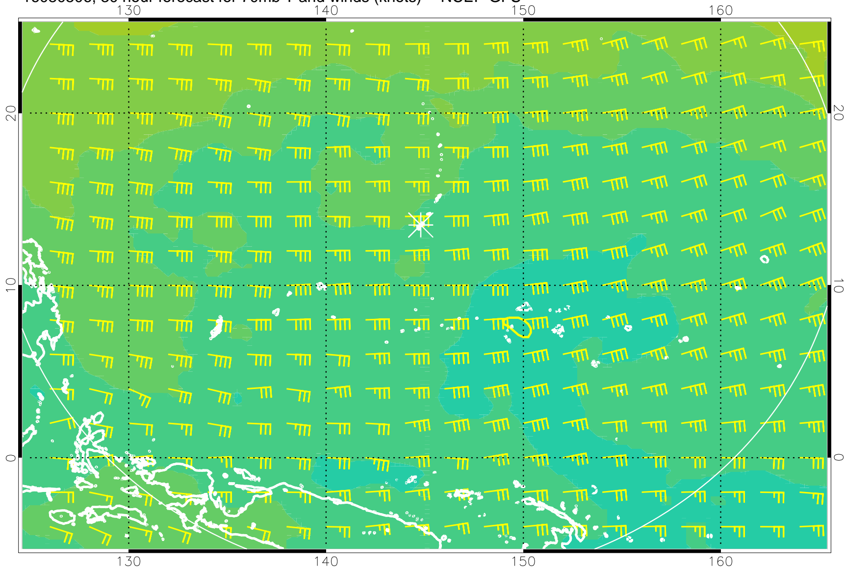
16080506, 30 hour forecast for 70mb T and winds (knots) -- NCEP GFS
