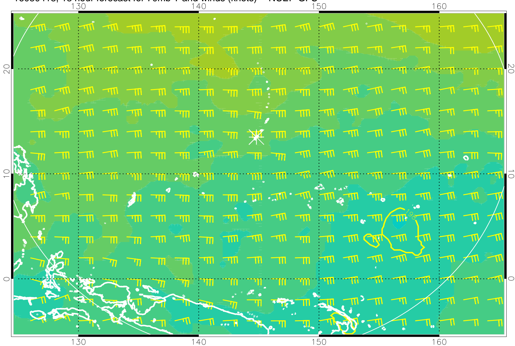
16080418, 18 hour forecast for 70mb T and winds (knots) -- NCEP GFS
