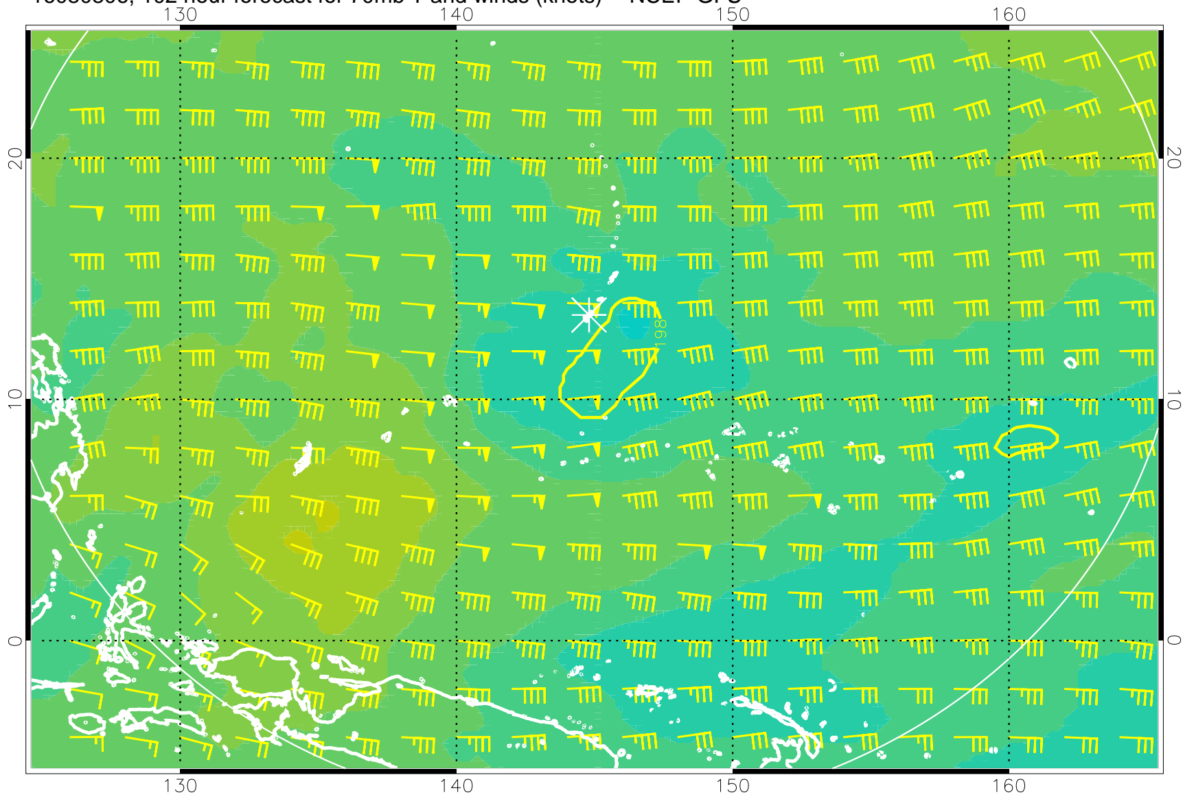
16080806, 102 hour forecast for 70mb T and winds (knots) -- NCEP GFS
