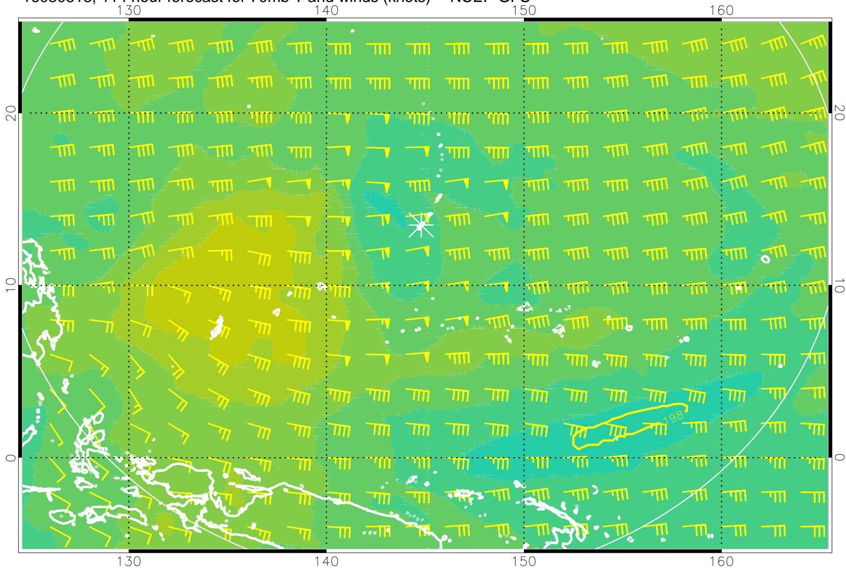
16080818, 114 hour forecast for 70mb T and winds (knots) -- NCEP GFS
