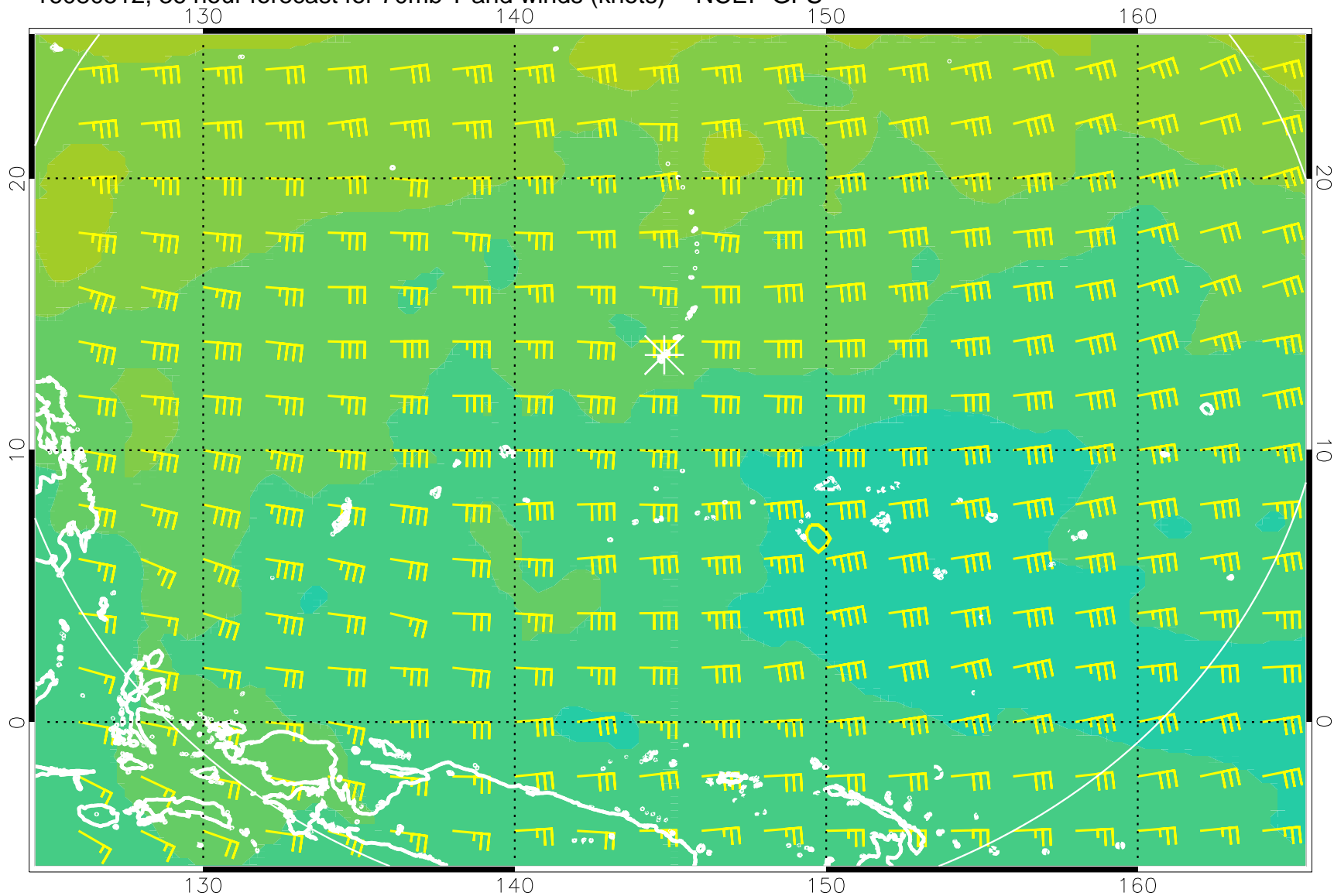
16080512, 36 hour forecast for 70mb T and winds (knots) -- NCEP GFS
