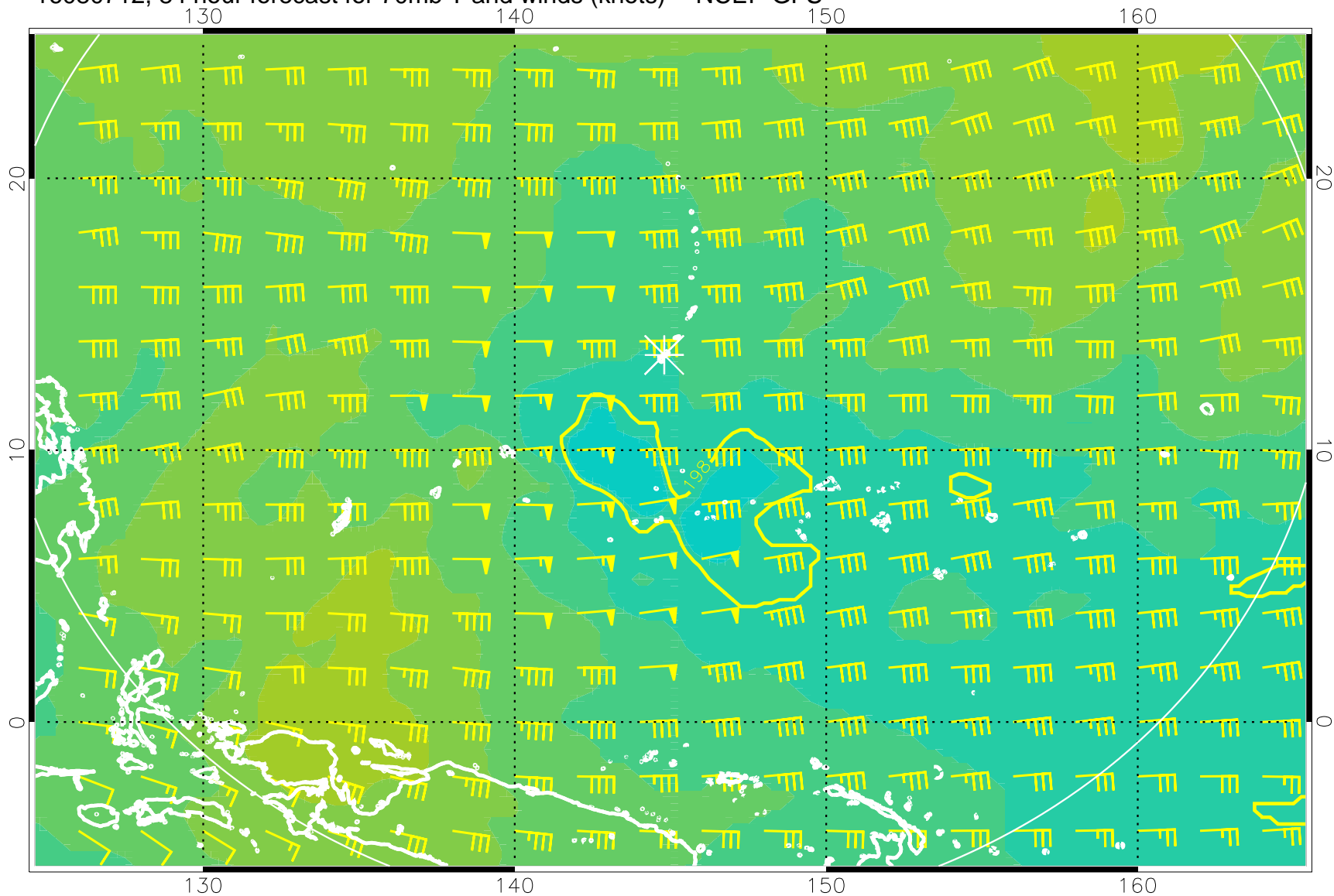
16080712, 84 hour forecast for 70mb T and winds (knots) -- NCEP GFS
