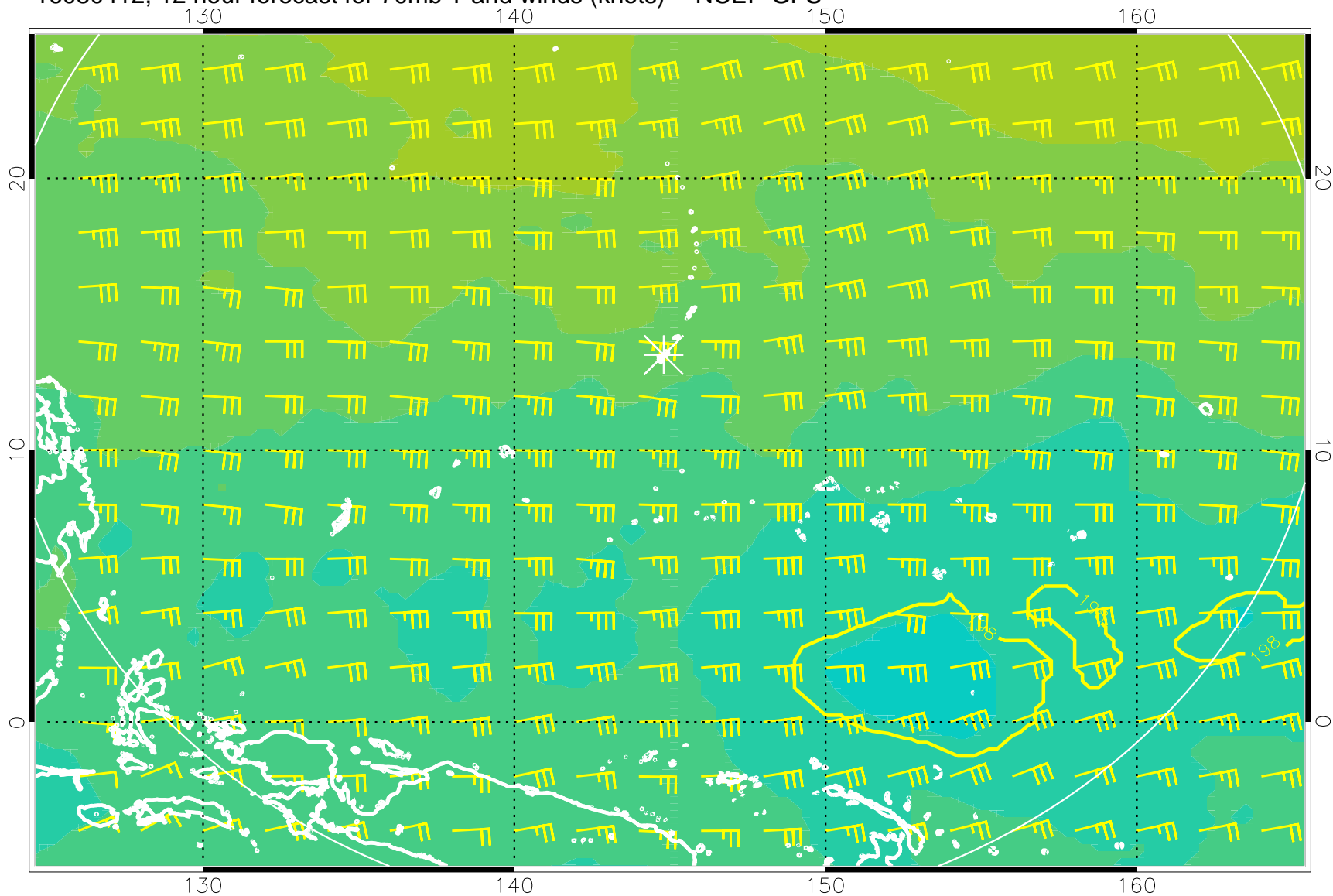
16080412, 12 hour forecast for 70mb T and winds (knots) -- NCEP GFS
