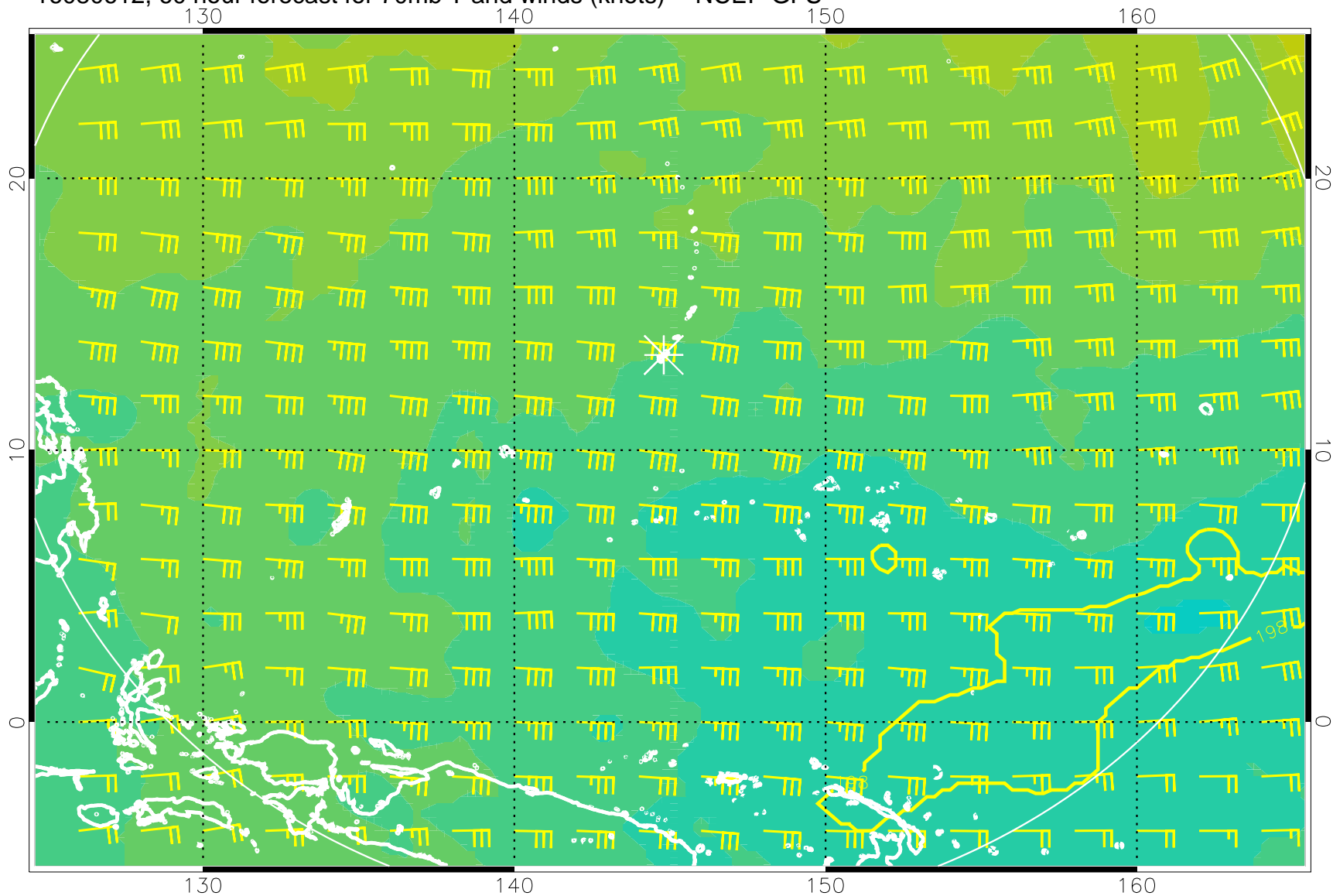
16080612, 60 hour forecast for 70mb T and winds (knots) -- NCEP GFS
