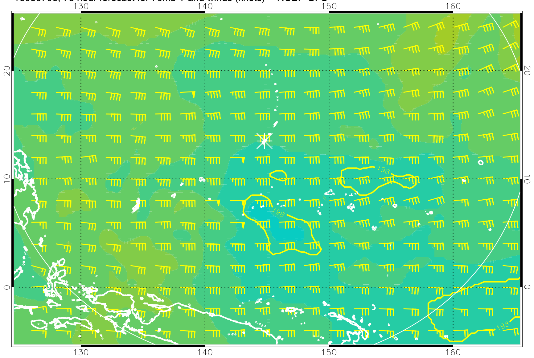
16080706, 78 hour forecast for 70mb T and winds (knots) -- NCEP GFS
