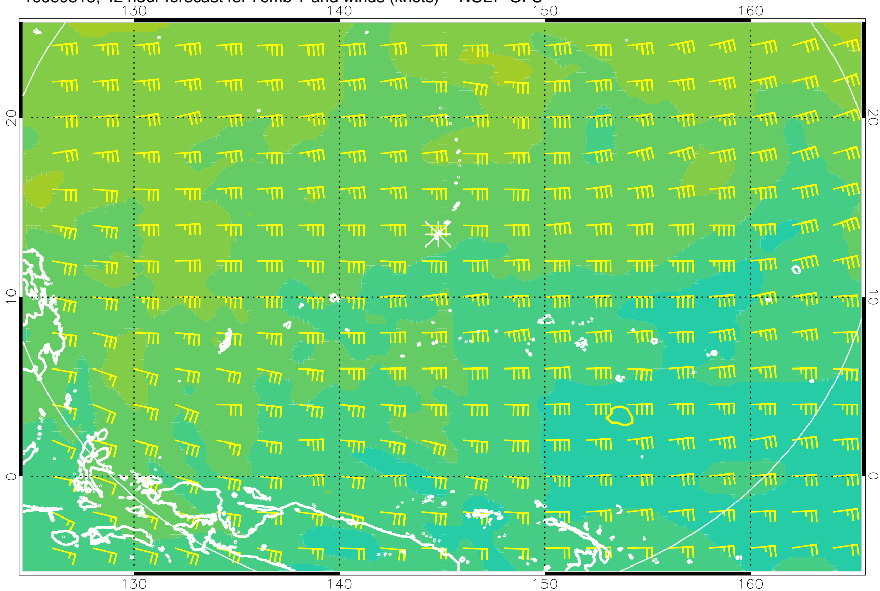
16080518, 42 hour forecast for 70mb T and winds (knots) -- NCEP GFS
