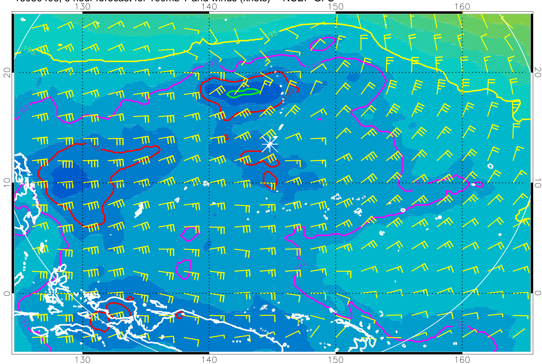
16080406, 6 hour forecast for 100mb T and winds (knots) -- NCEP GFS
