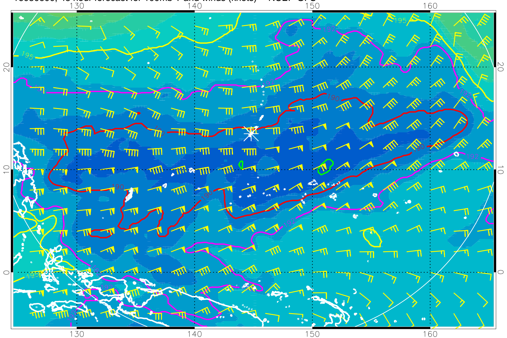
16080600, 48 hour forecast for 100mb T and winds (knots) -- NCEP GFS
