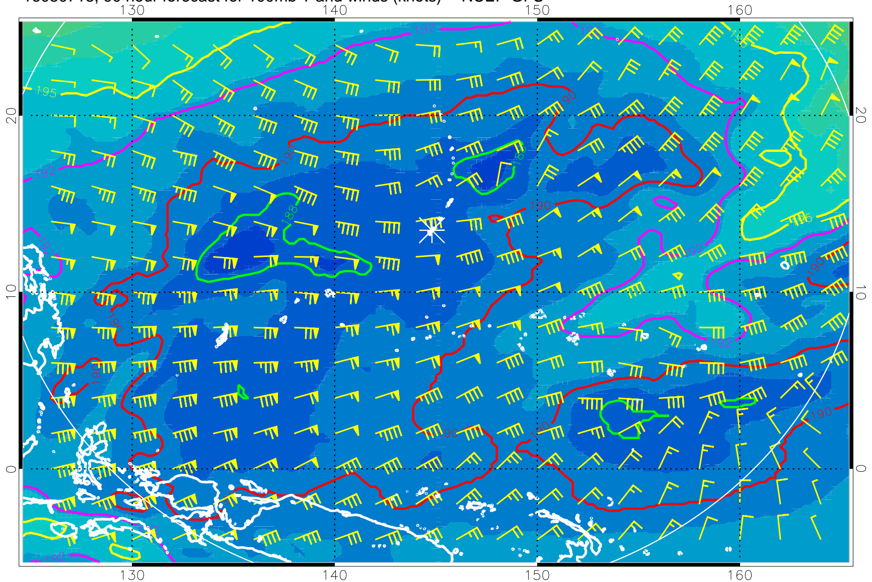
16080718, 90 hour forecast for 100mb T and winds (knots) -- NCEP GFS
