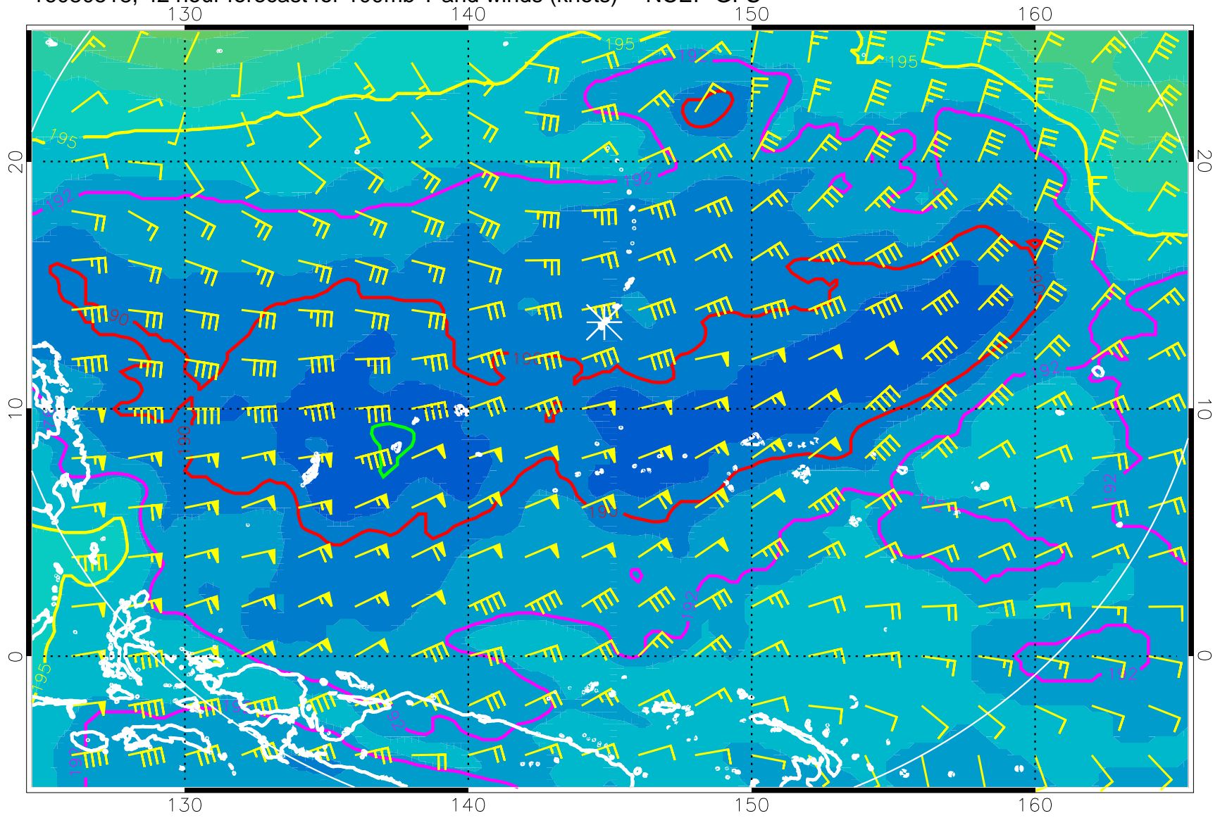
16080518, 42 hour forecast for 100mb T and winds (knots) -- NCEP GFS
