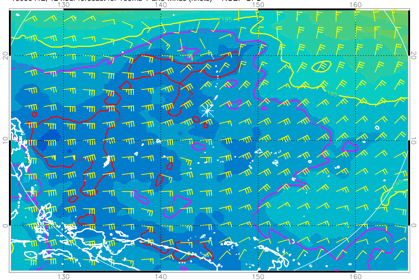
16080412, 12 hour forecast for 100mb T and winds (knots) -- NCEP GFS
