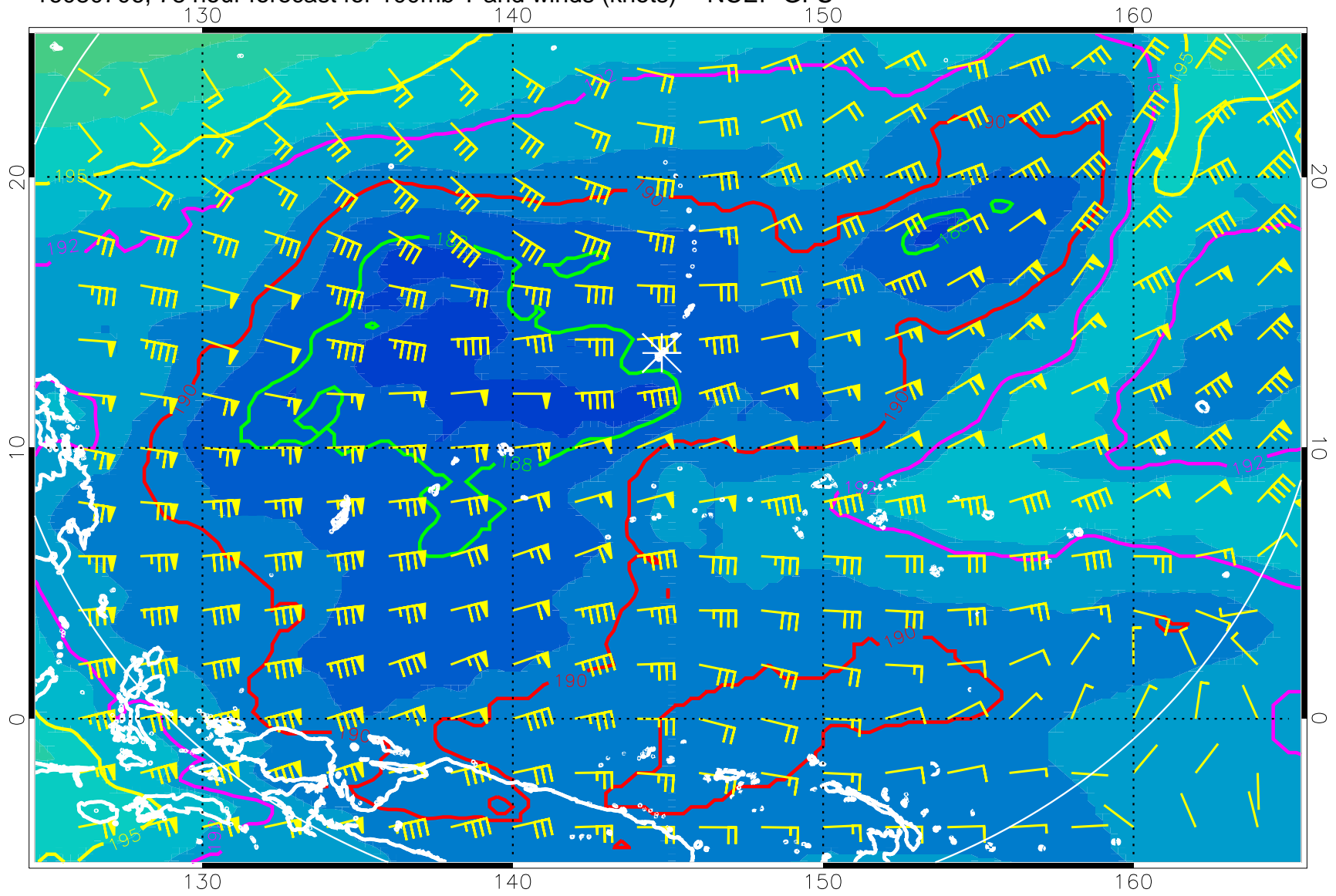
16080706, 78 hour forecast for 100mb T and winds (knots) -- NCEP GFS
