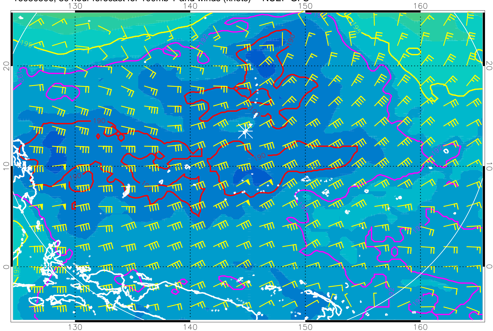
16080506, 30 hour forecast for 100mb T and winds (knots) -- NCEP GFS
