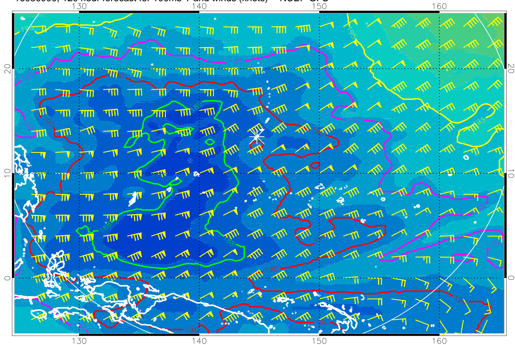
16080900, 120 hour forecast for 100mb T and winds (knots) -- NCEP GFS
