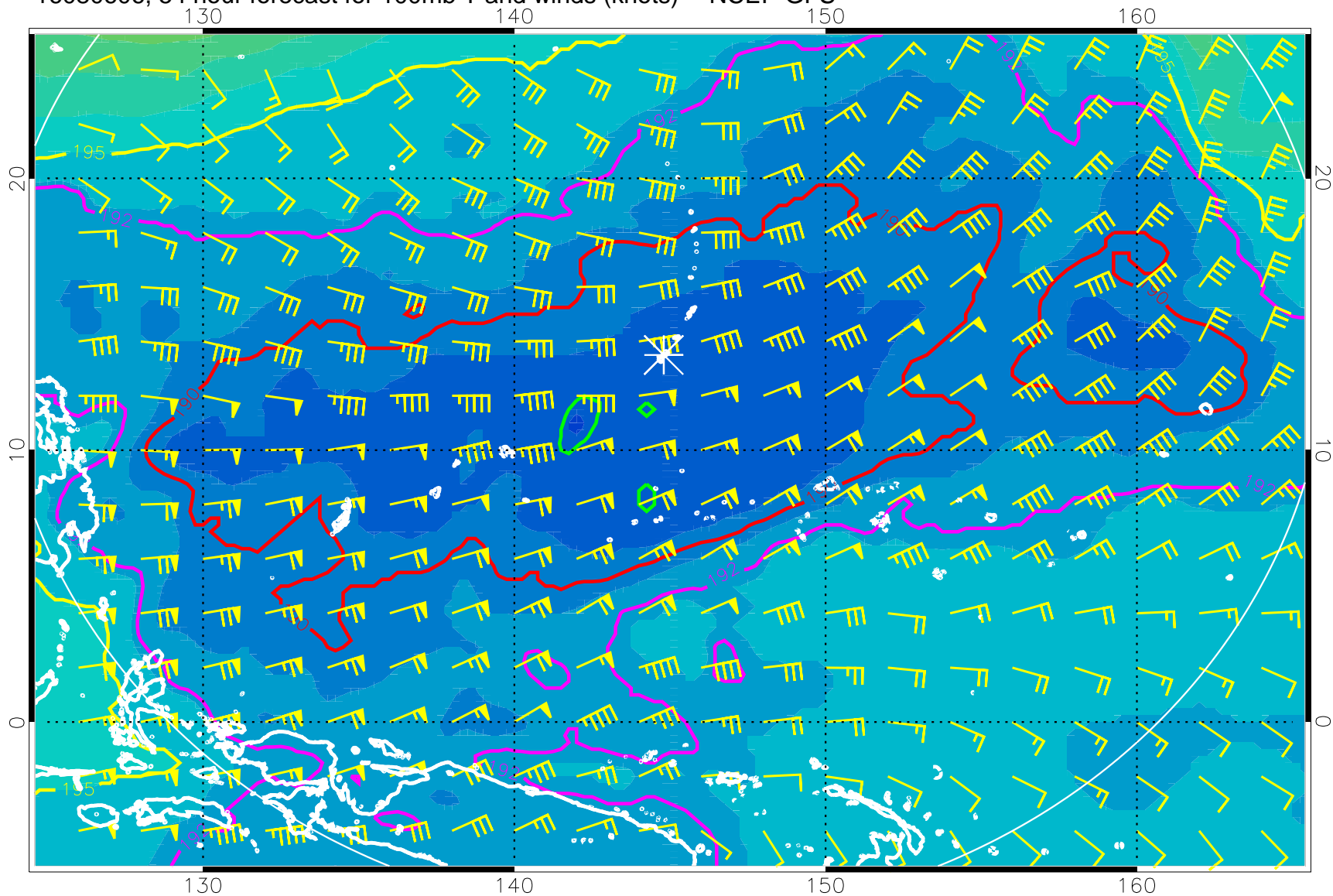
16080606, 54 hour forecast for 100mb T and winds (knots) -- NCEP GFS
