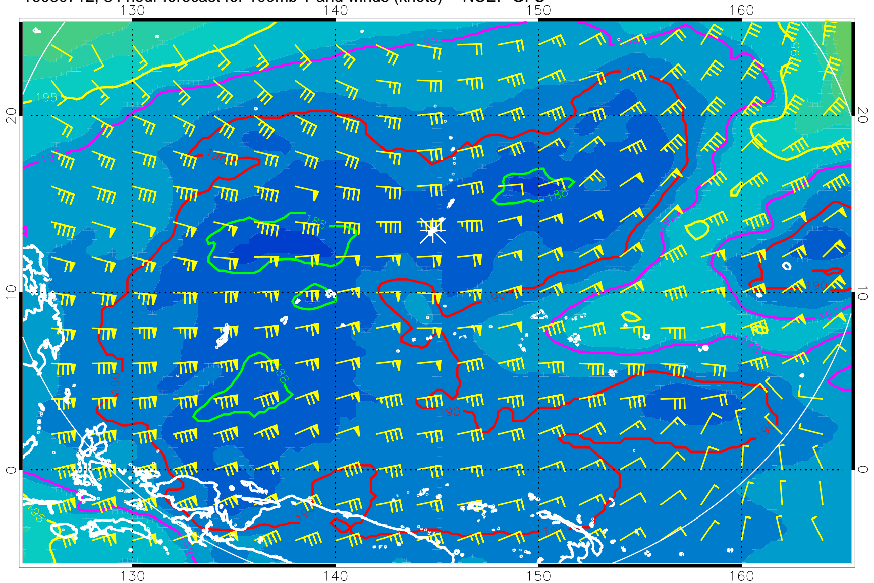
16080712, 84 hour forecast for 100mb T and winds (knots) -- NCEP GFS
