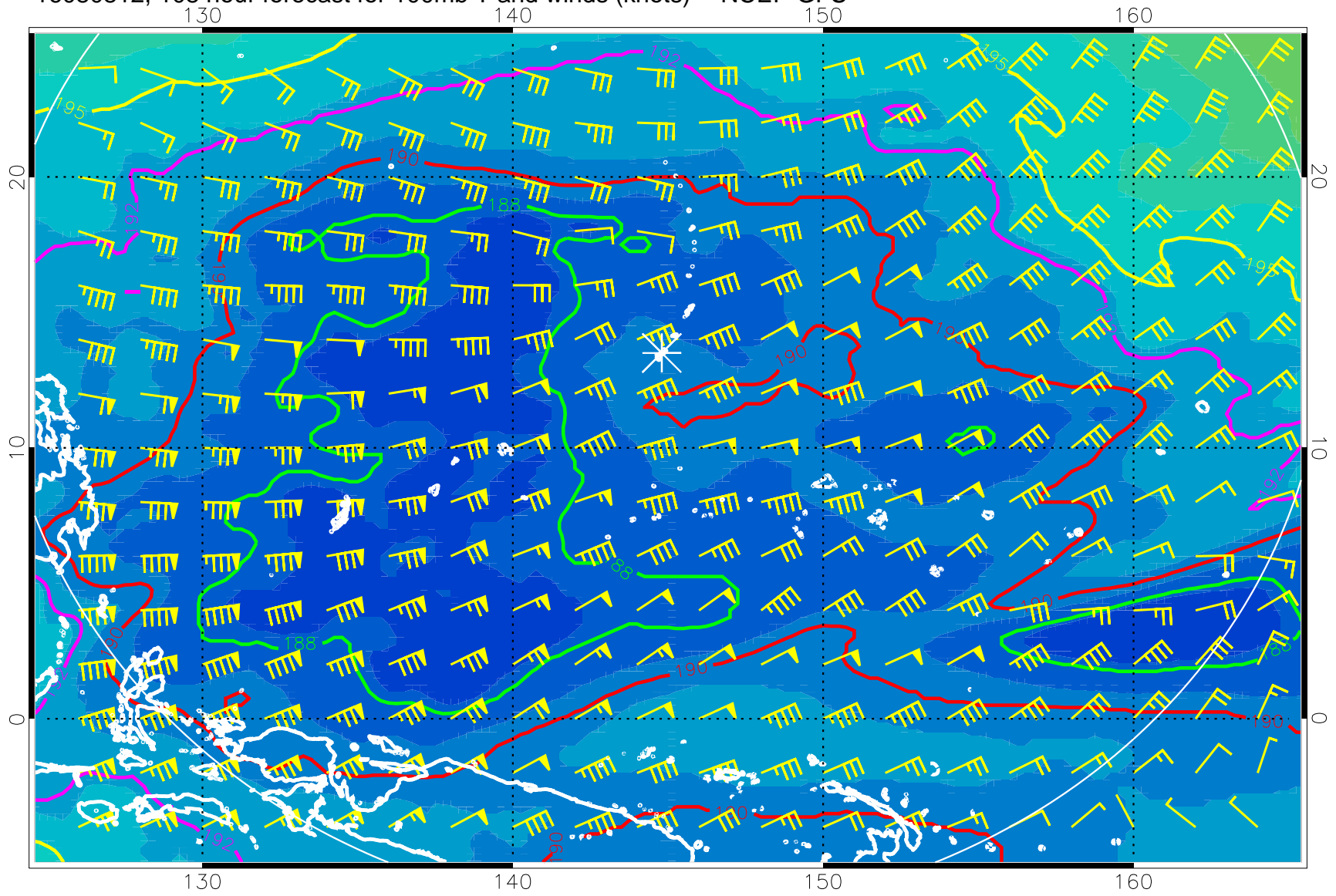
16080812, 108 hour forecast for 100mb T and winds (knots) -- NCEP GFS
