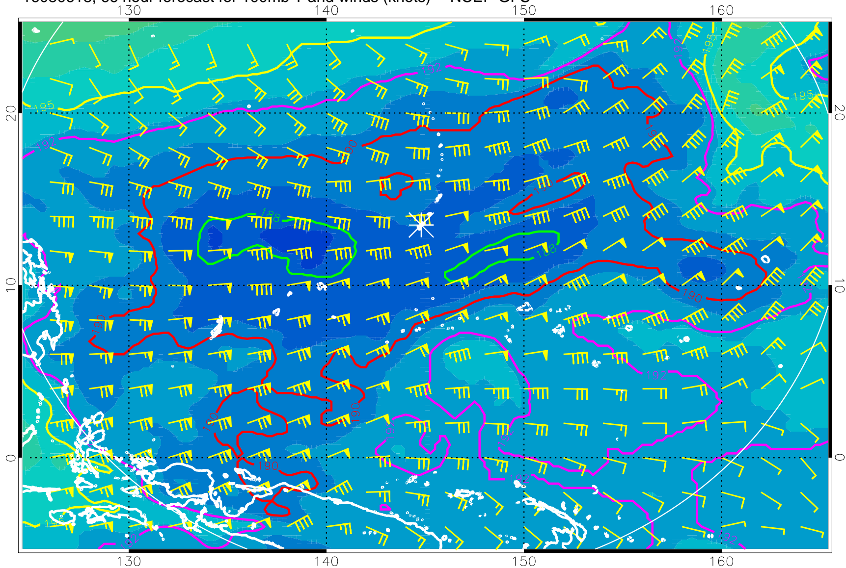
16080618, 66 hour forecast for 100mb T and winds (knots) -- NCEP GFS
