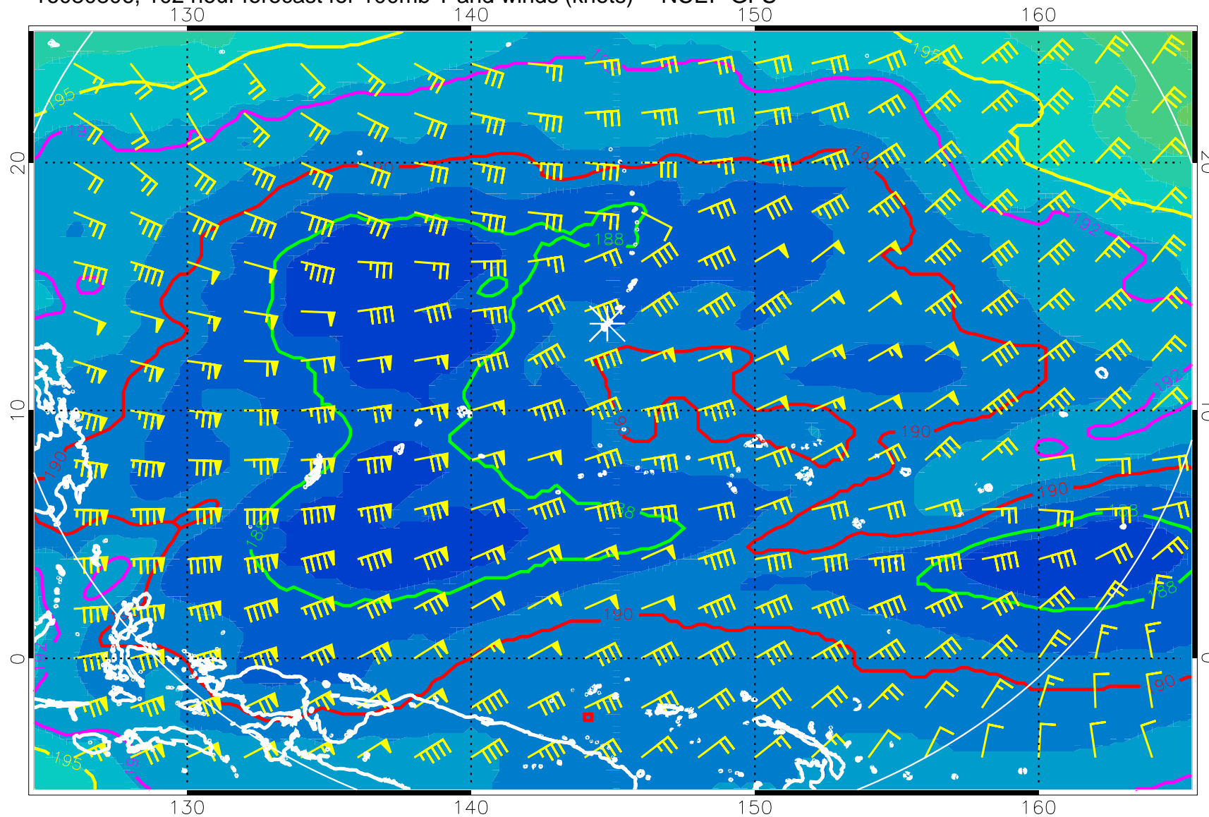
16080806, 102 hour forecast for 100mb T and winds (knots) -- NCEP GFS
