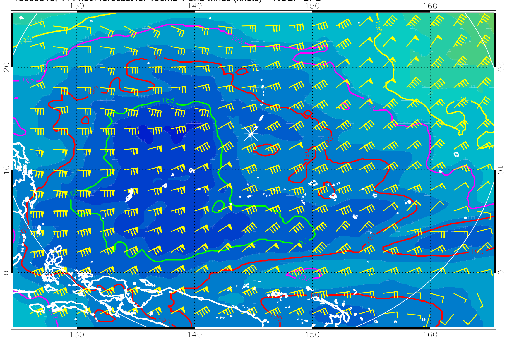
16080818, 114 hour forecast for 100mb T and winds (knots) -- NCEP GFS
