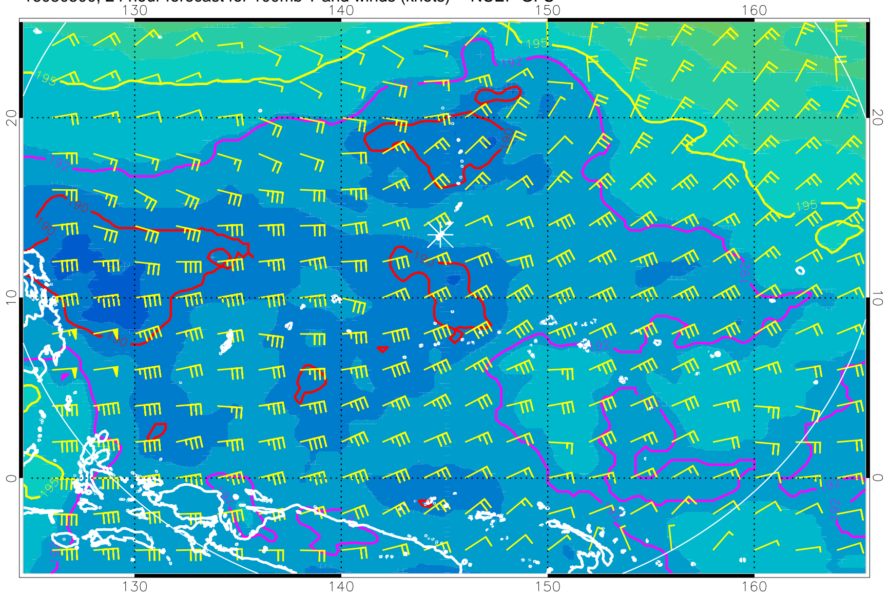
16080500, 24 hour forecast for 100mb T and winds (knots) -- NCEP GFS
