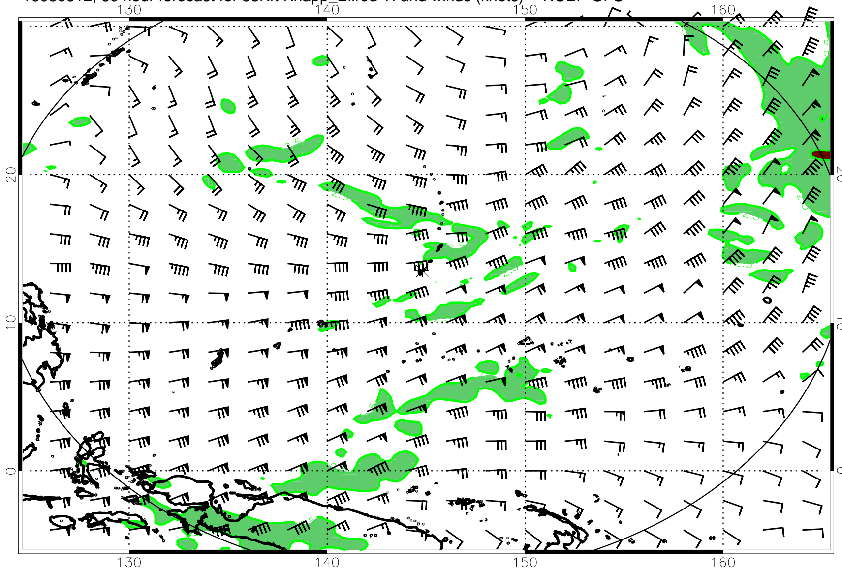
16080612, 60 hour forecast for 53Kft Knapp_Ellrod TI and winds (knots) -- NCEP GFS
