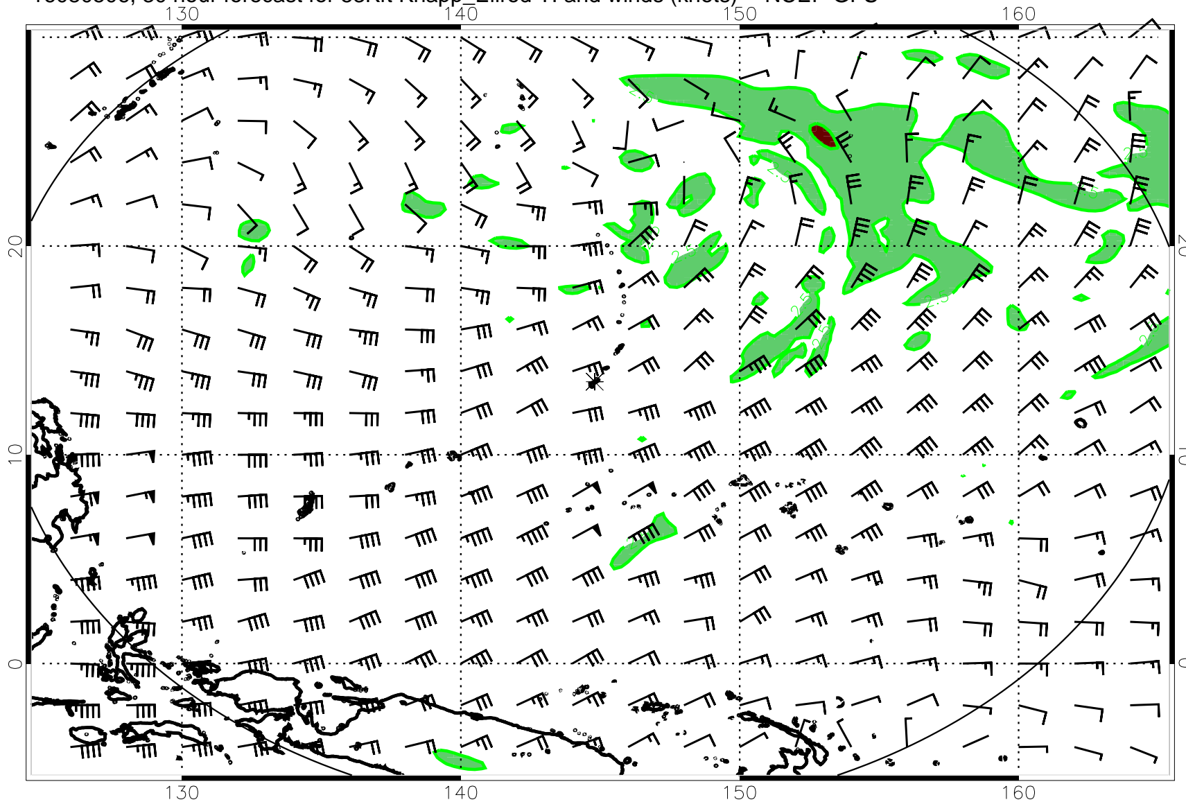
16080506, 30 hour forecast for 53Kft Knapp_Ellrod TI and winds (knots) -- NCEP GFS
