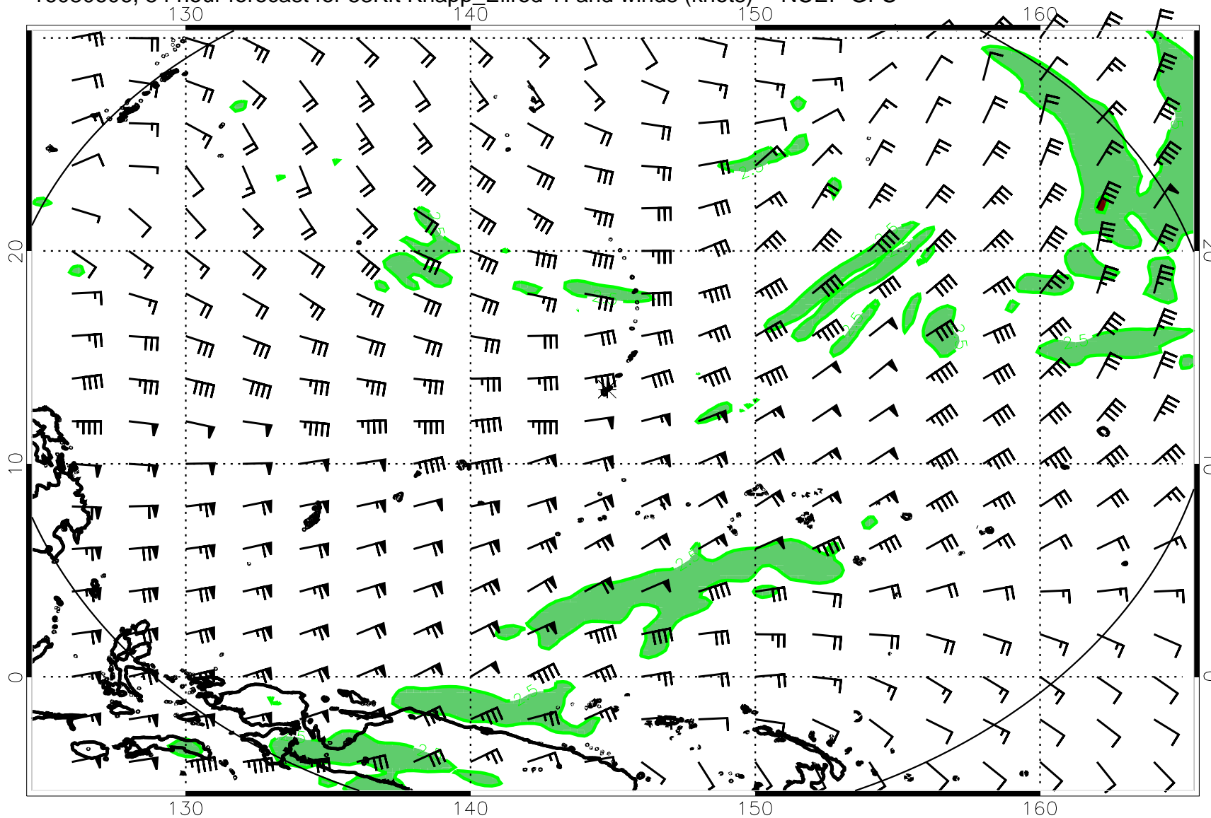
16080606, 54 hour forecast for 53Kft Knapp_Ellrod TI and winds (knots) -- NCEP GFS
