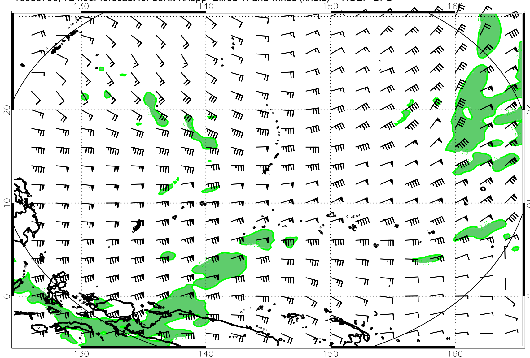
16080700, 72 hour forecast for 53Kft Knapp_Ellrod TI and winds (knots) -- NCEP GFS
