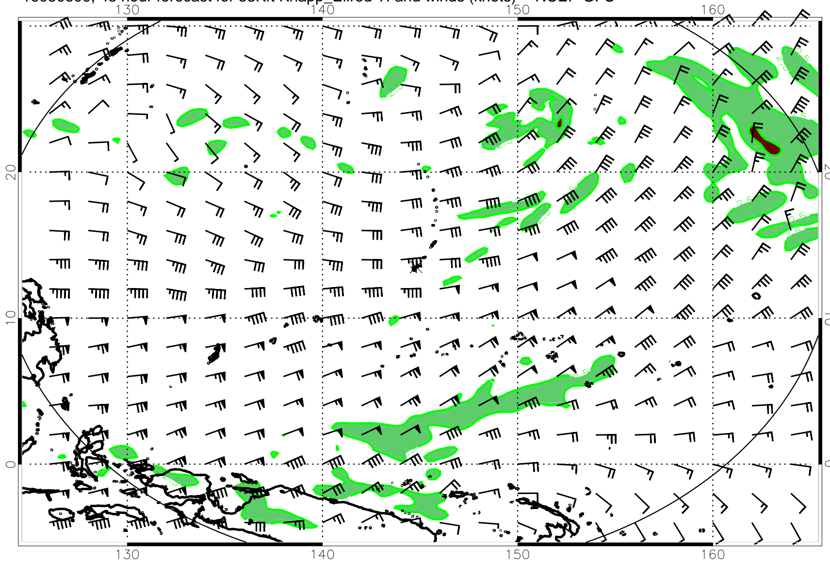
16080600, 48 hour forecast for 53Kft Knapp_Ellrod TI and winds (knots) -- NCEP GFS
