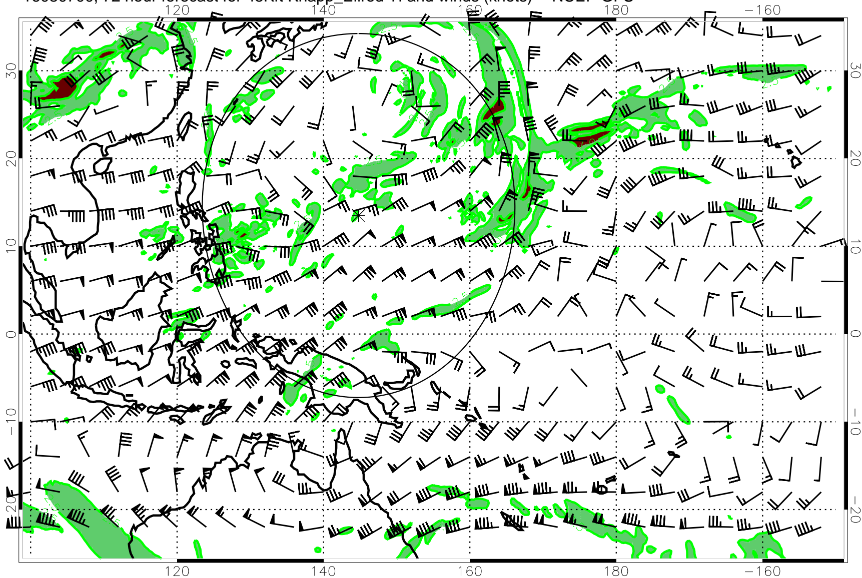
16080700, 72 hour forecast for 45Kft Knapp_Ellrod TI and winds (knots) -- NCEP GFS
