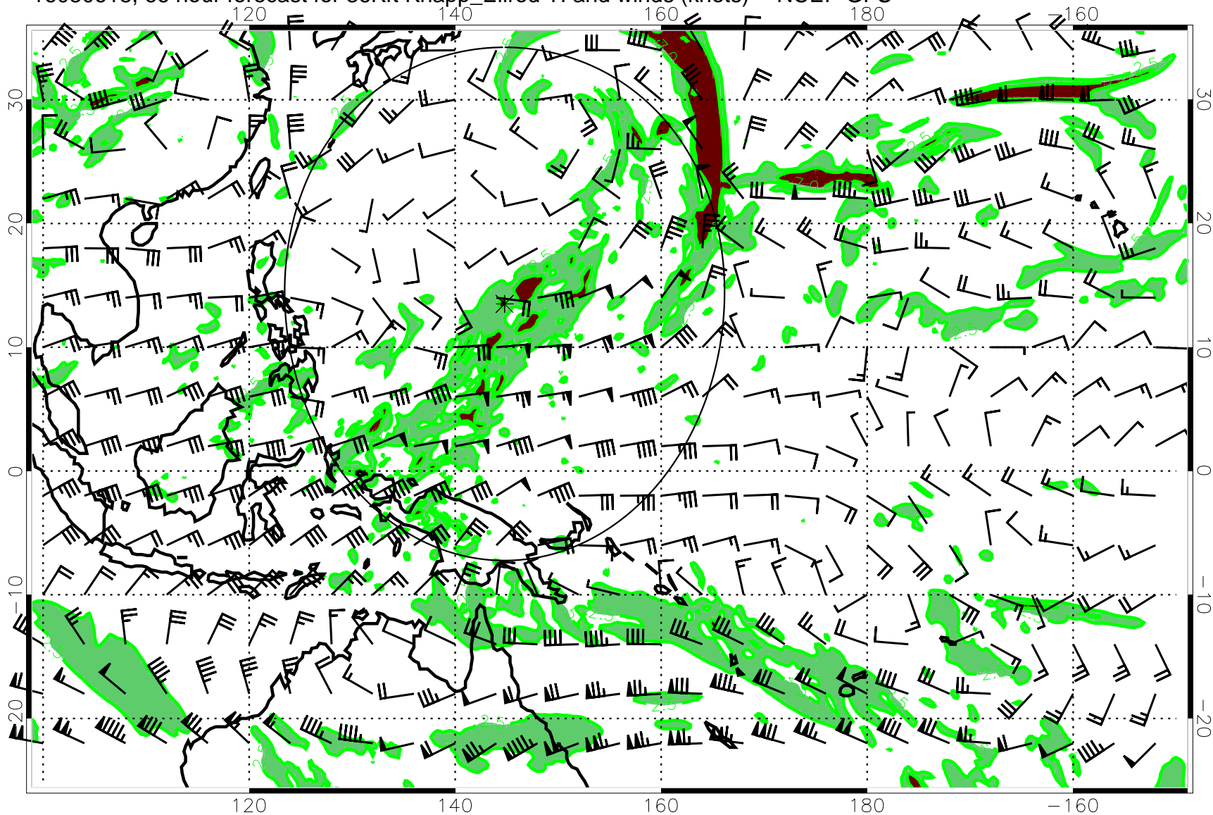
16080618, 66 hour forecast for 36Kft Knapp_Ellrod TI and winds (knots) -- NCEP GFS
