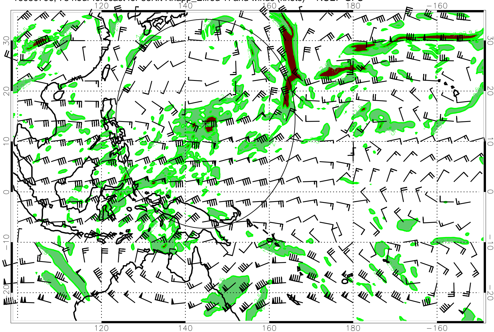
16080706, 78 hour forecast for 36Kft Knapp_Ellrod TI and winds (knots) -- NCEP GFS
