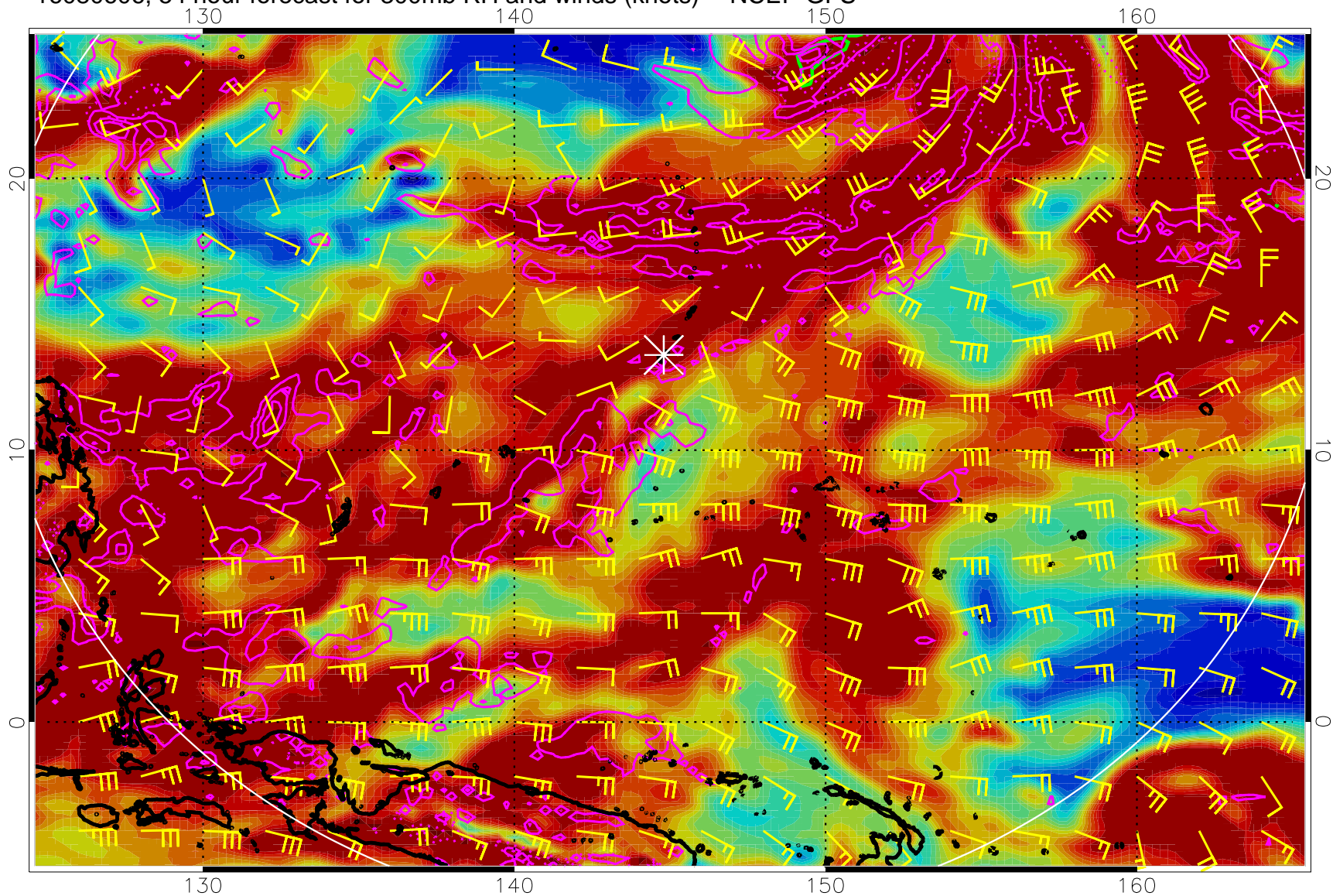
16080606, 54 hour forecast for 300mb RH and winds (knots) -- NCEP GFS
