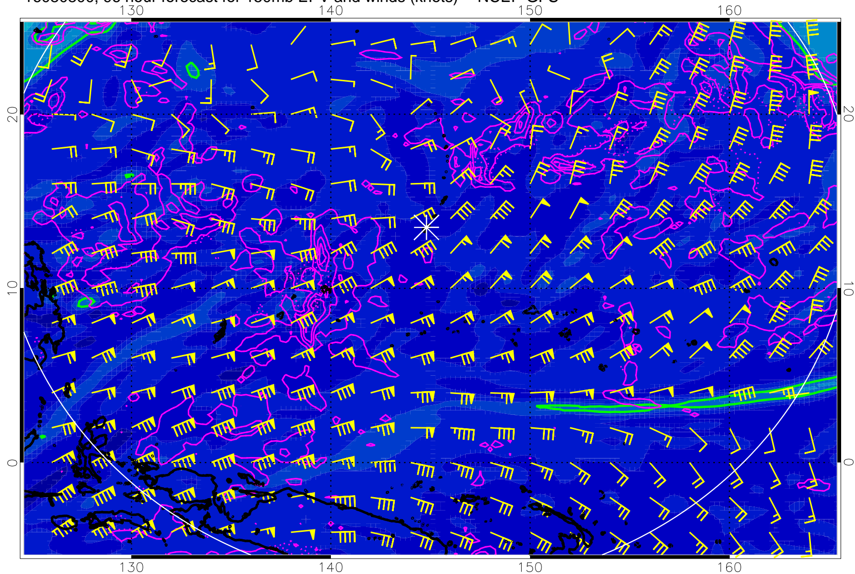
16080800, 96 hour forecast for 150mb EPV and winds (knots) -- NCEP GFS
