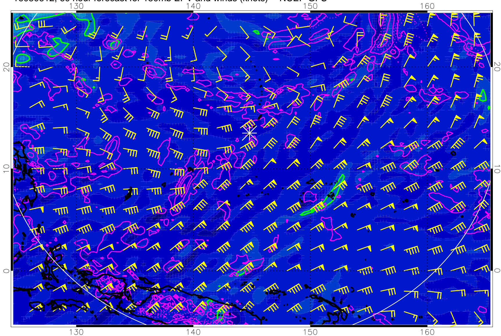
16080612, 60 hour forecast for 150mb EPV and winds (knots) -- NCEP GFS
