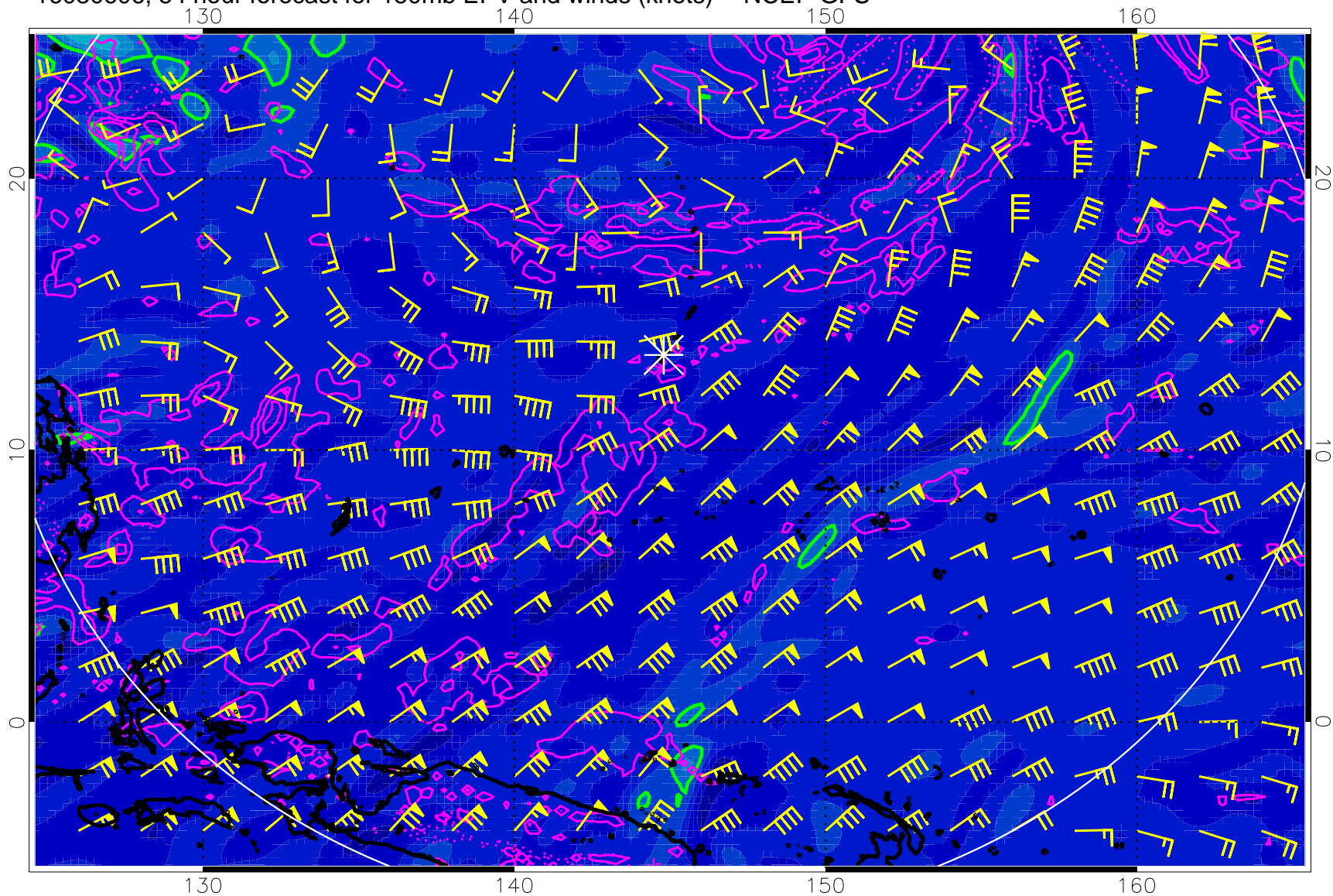
16080606, 54 hour forecast for 150mb EPV and winds (knots) -- NCEP GFS
