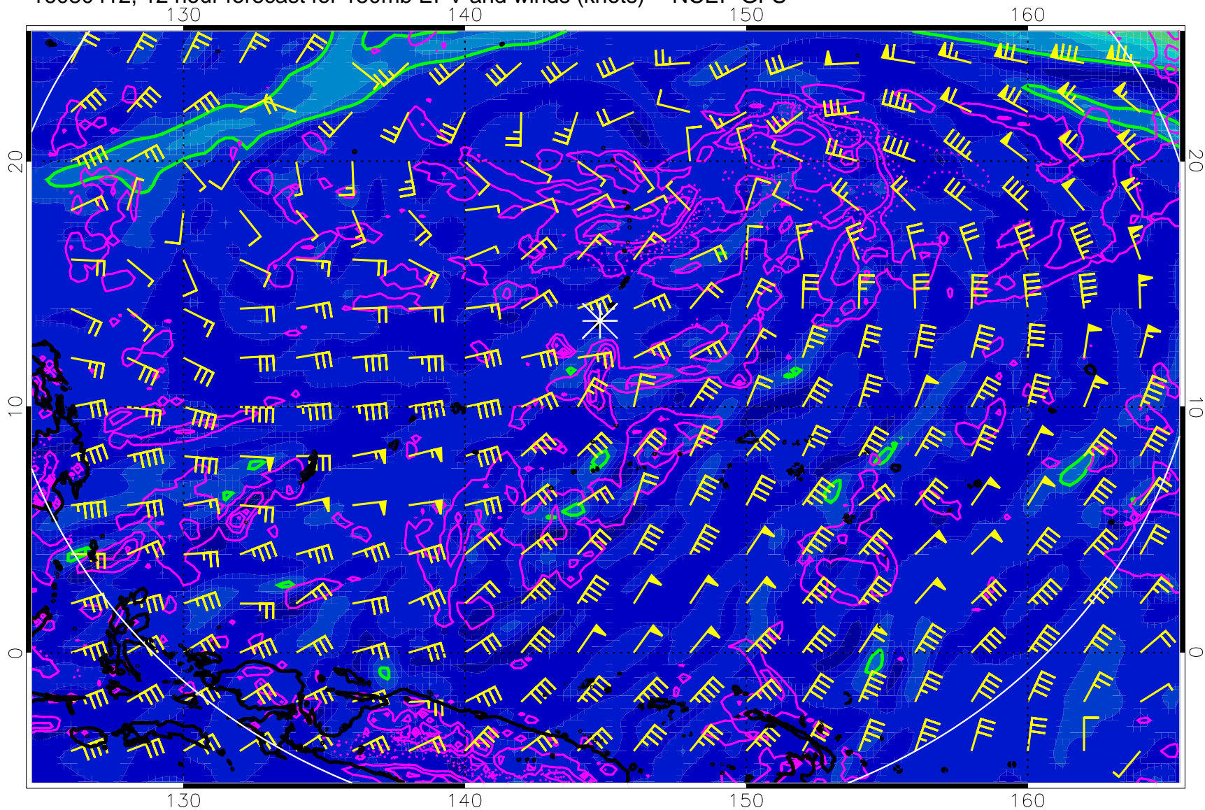
16080412, 12 hour forecast for 150mb EPV and winds (knots) -- NCEP GFS
