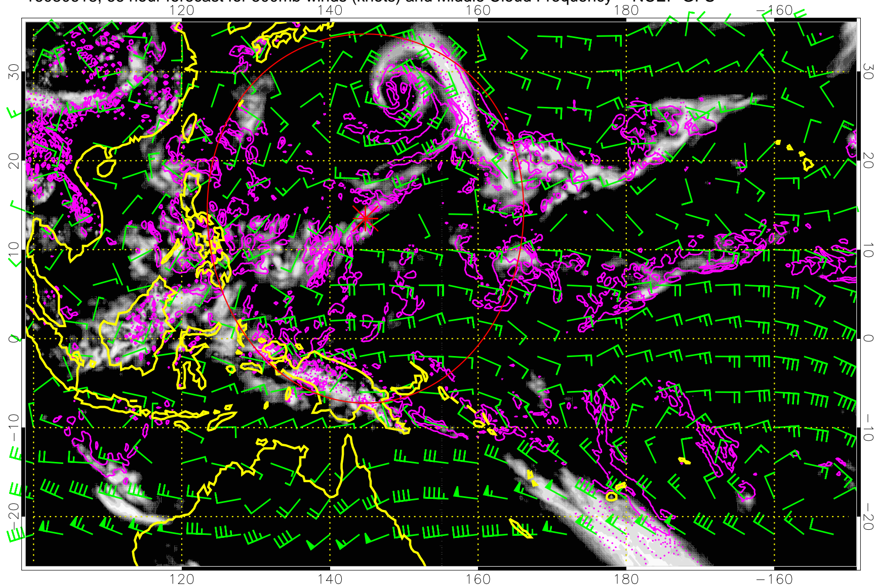
16080618, 66 hour forecast for 500mb winds (knots) and Middle Cloud Frequency -- NCEP GFS
