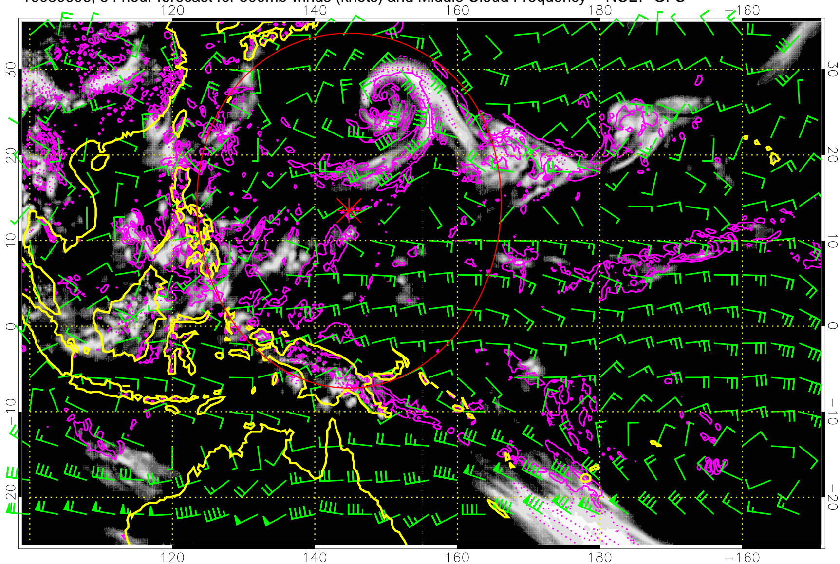
16080606, 54 hour forecast for 500mb winds (knots) and Middle Cloud Frequency -- NCEP GFS
