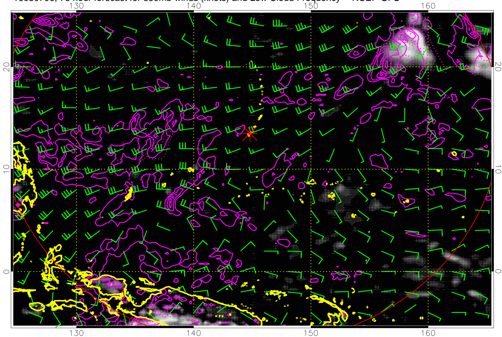
16080706, 78 hour forecast for 850mb winds (knots) and Low Cloud Frequency -- NCEP GFS
