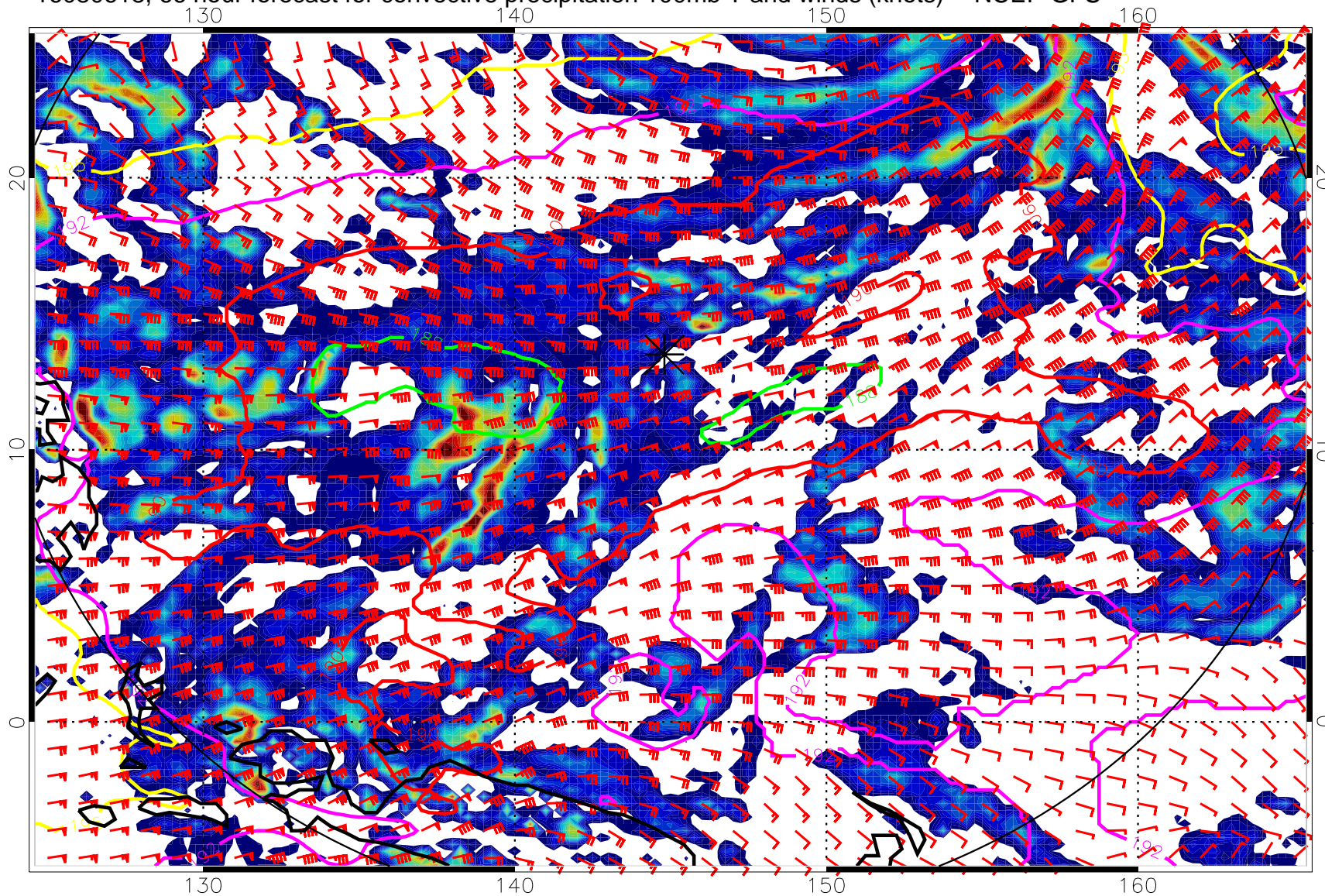
16080618, 66 hour forecast for convective precipitation 100mb T and winds (knots) -- NCEP GFS
