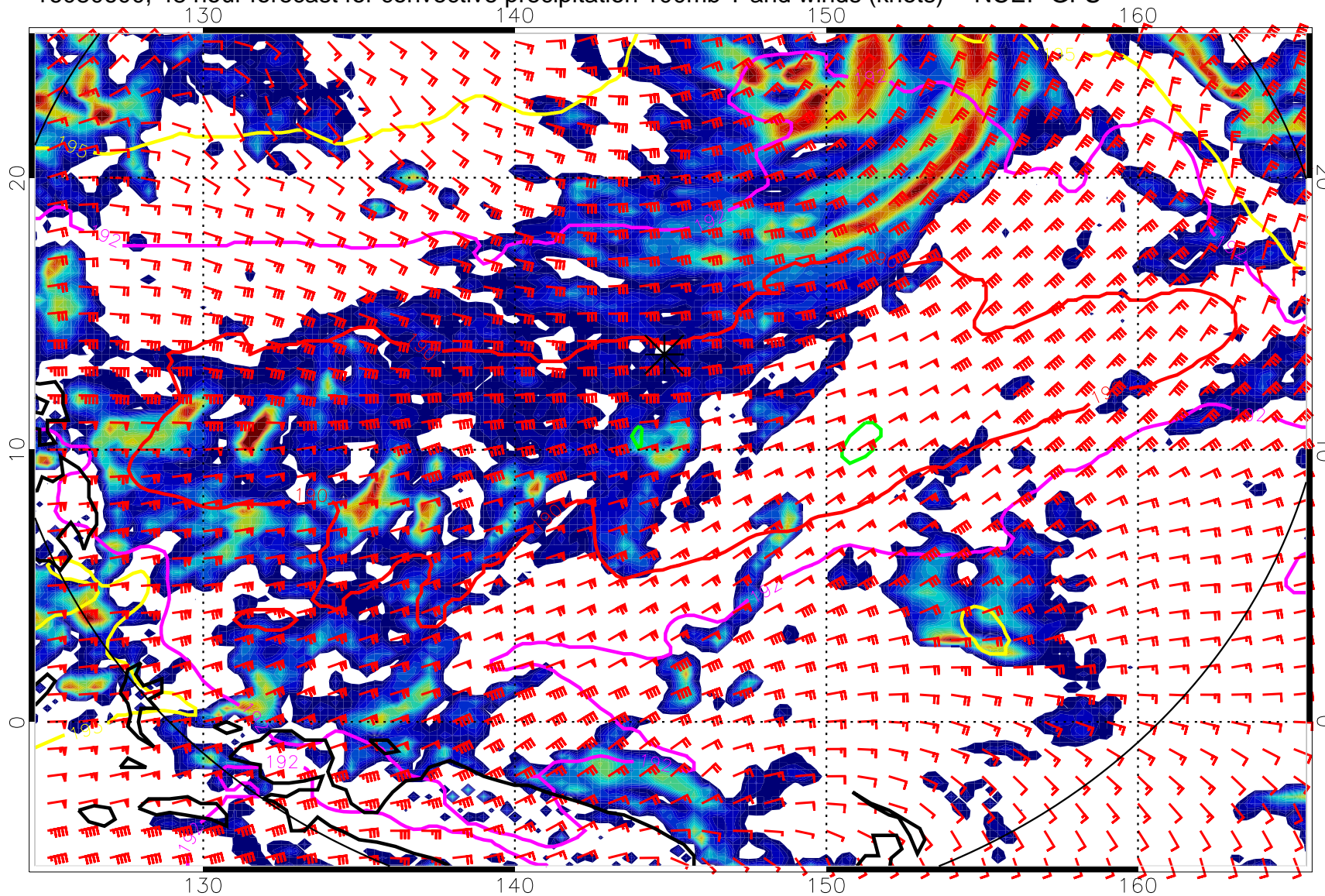
16080600, 48 hour forecast for convective precipitation 100mb T and winds (knots) -- NCEP GFS
