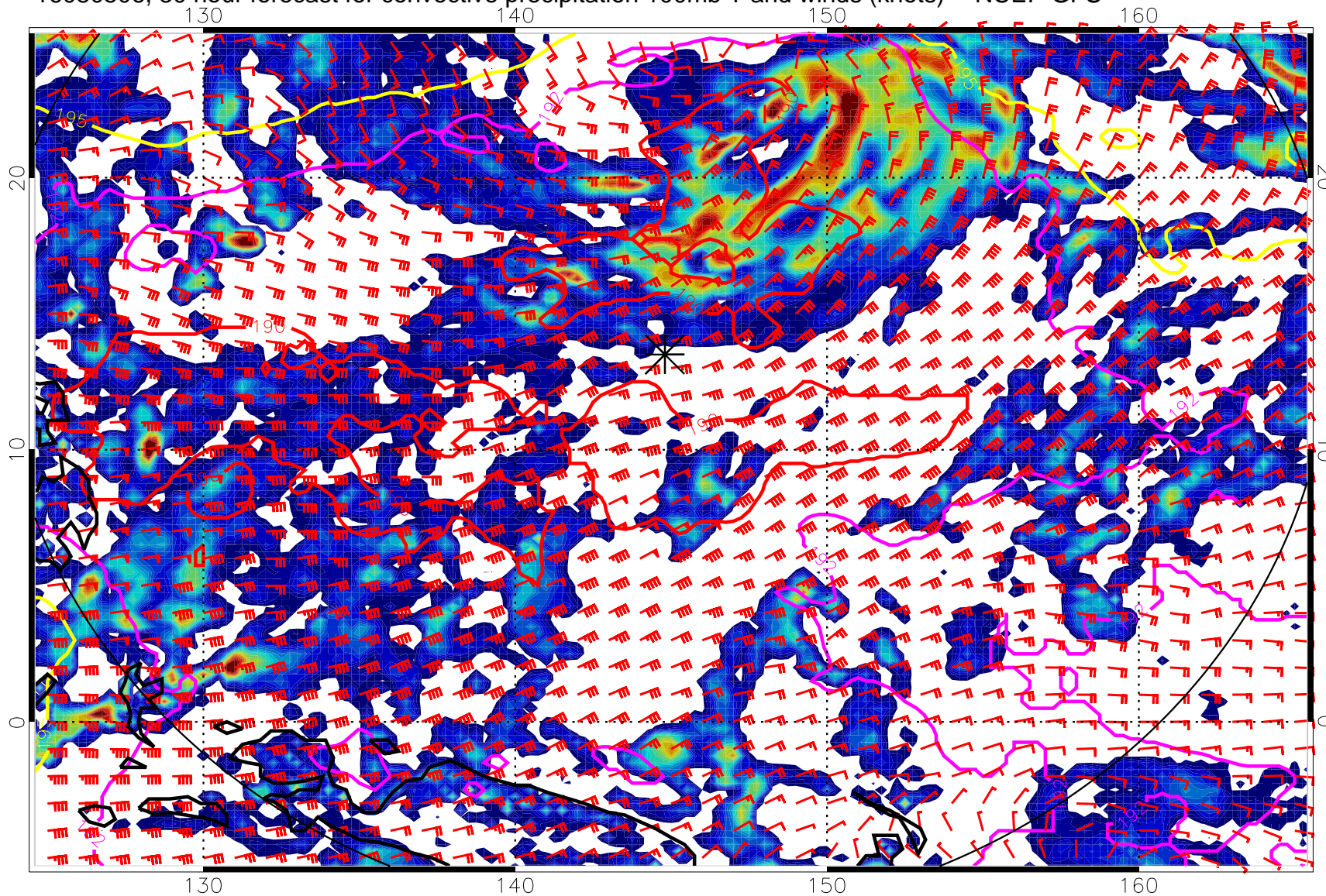
16080506, 30 hour forecast for convective precipitation 100mb T and winds (knots) -- NCEP GFS
