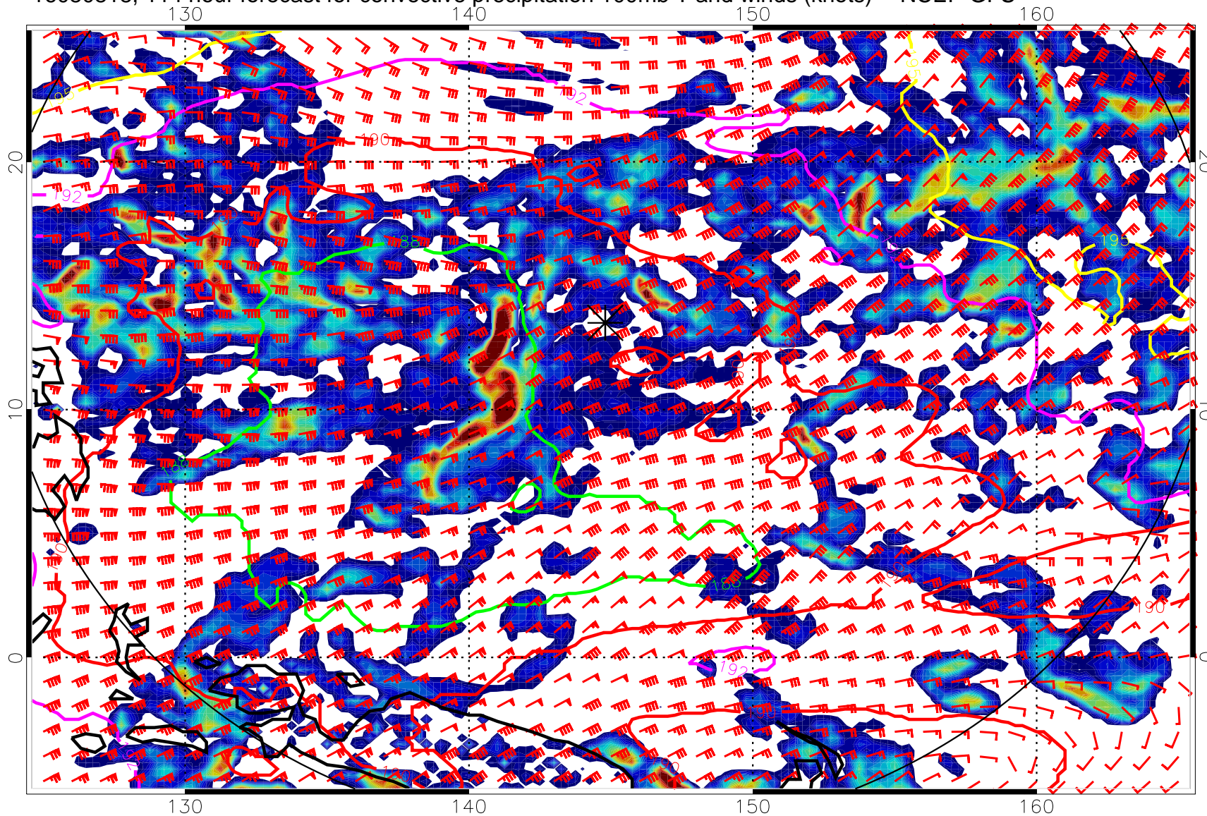
16080818, 114 hour forecast for convective precipitation 100mb T and winds (knots) -- NCEP GFS
