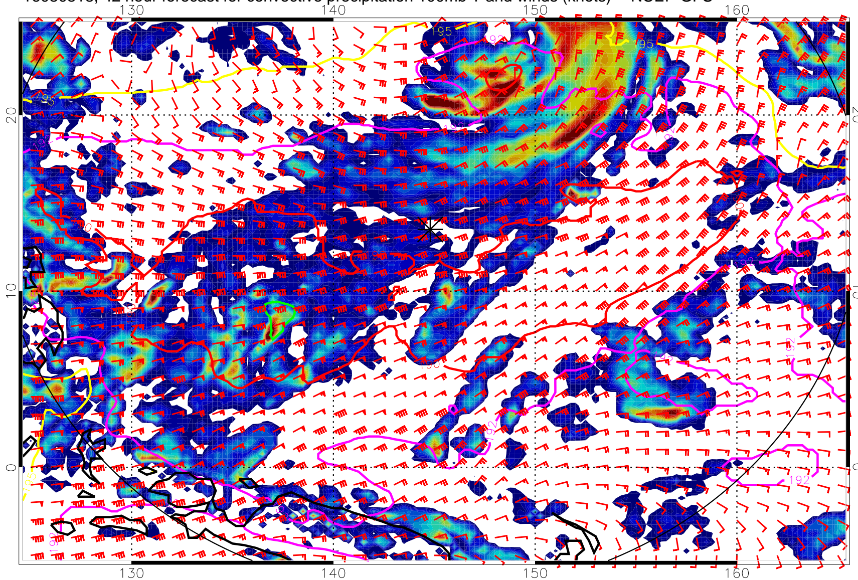
16080518, 42 hour forecast for convective precipitation 100mb T and winds (knots) -- NCEP GFS
