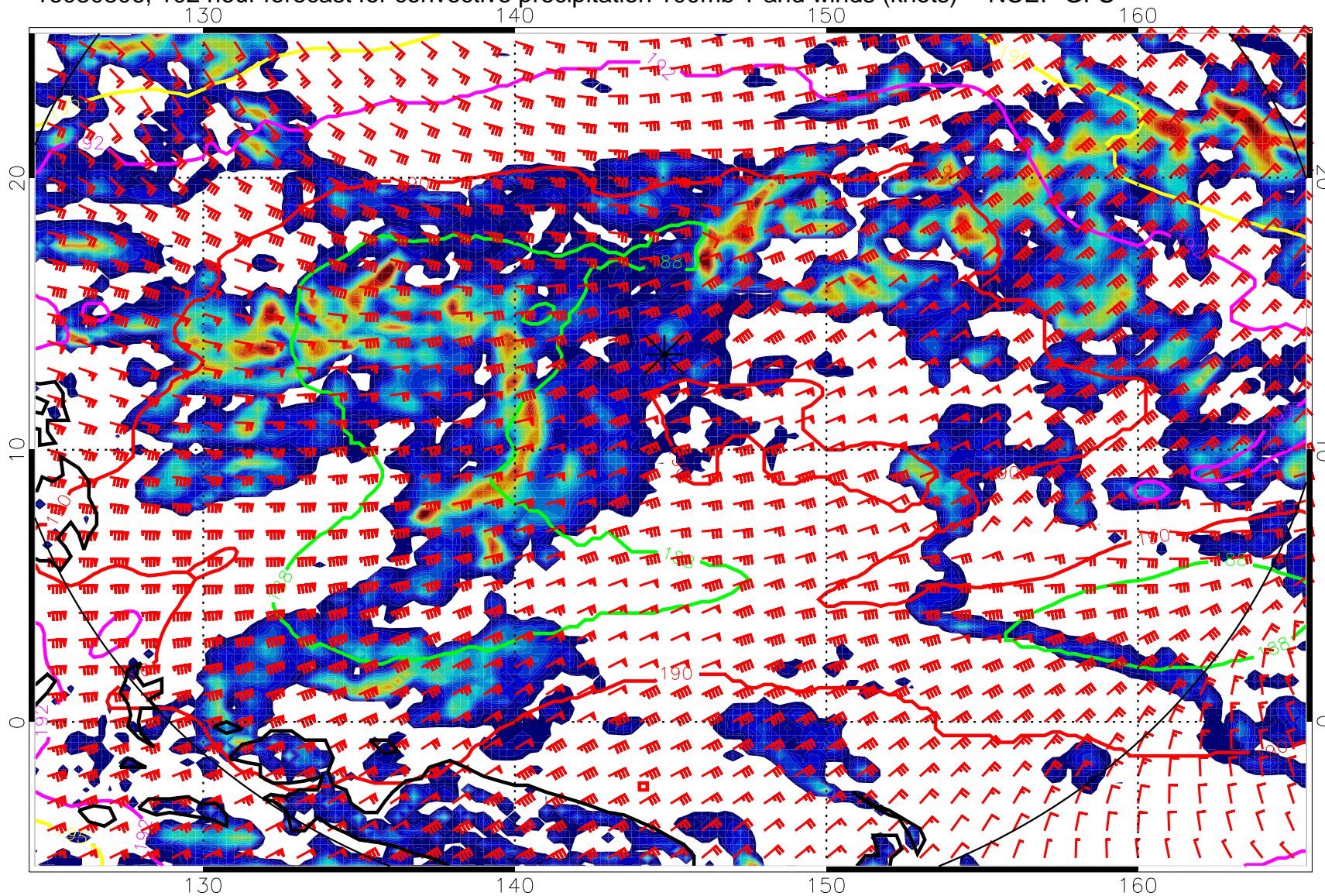
16080806, 102 hour forecast for convective precipitation 100mb T and winds (knots) -- NCEP GFS
