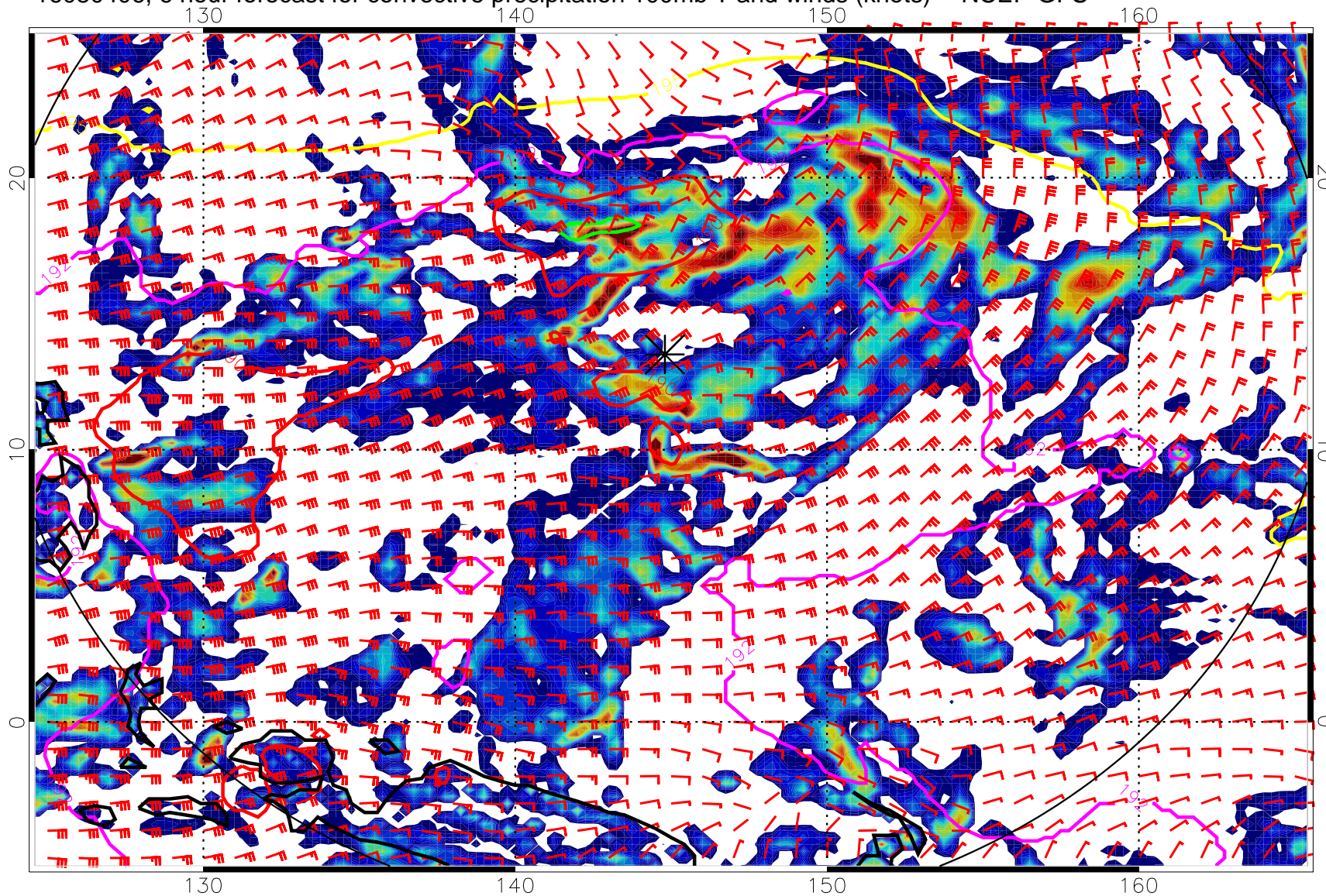
16080406, 6 hour forecast for convective precipitation 100mb T and winds (knots) -- NCEP GFS
