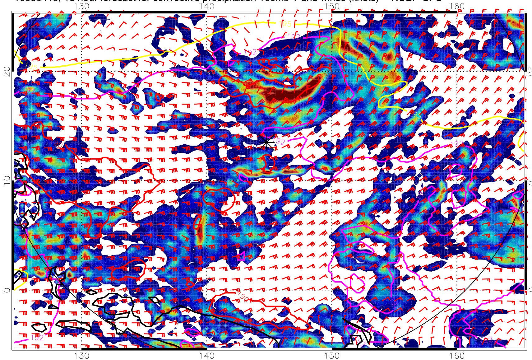
16080418, 18 hour forecast for convective precipitation 100mb T and winds (knots) -- NCEP GFS
