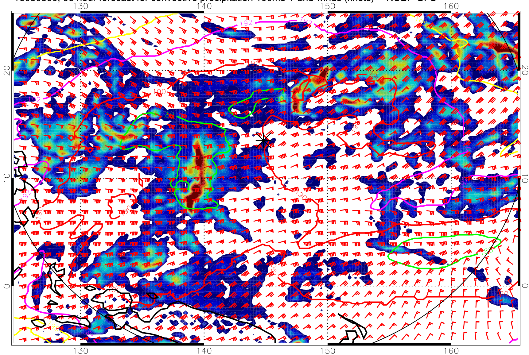
16080800, 96 hour forecast for convective precipitation 100mb T and winds (knots) -- NCEP GFS
