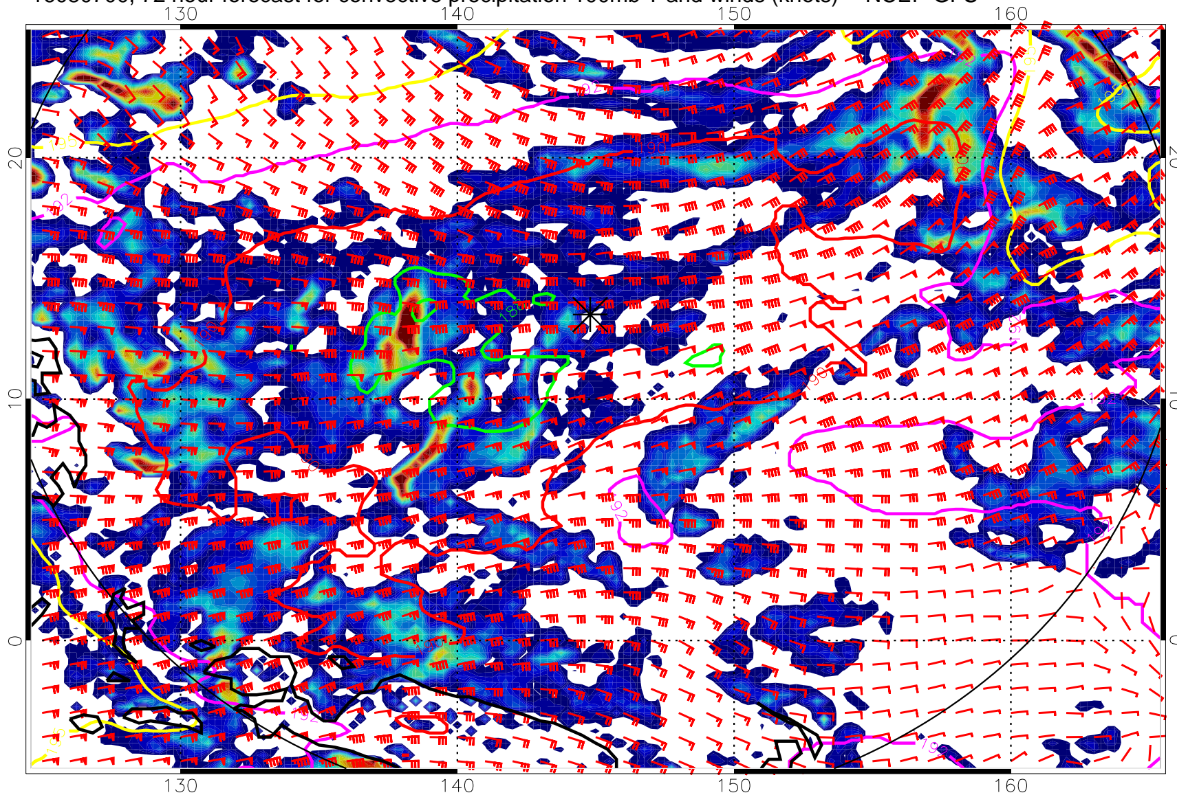
16080700, 72 hour forecast for convective precipitation 100mb T and winds (knots) -- NCEP GFS
