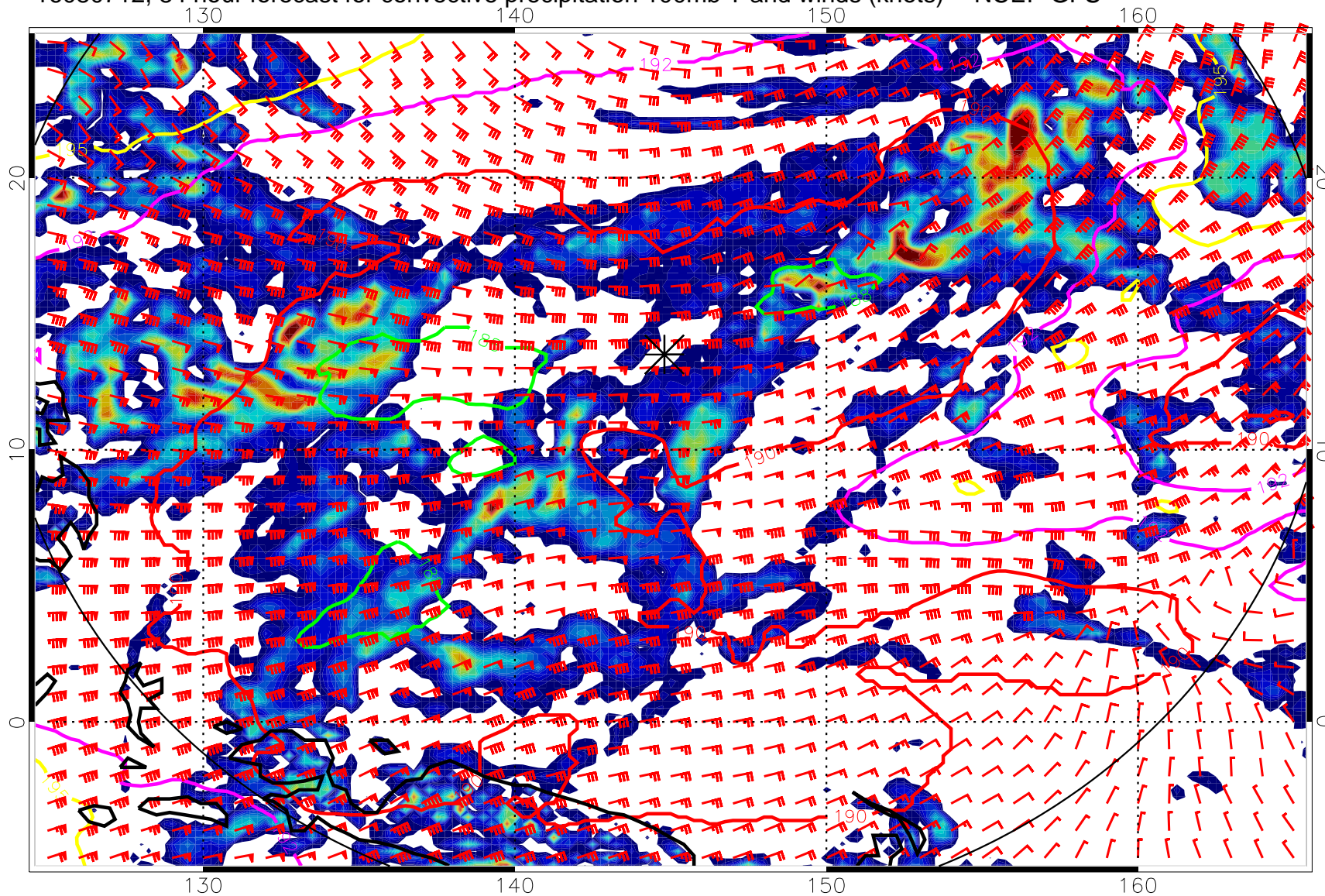
16080712, 84 hour forecast for convective precipitation 100mb T and winds (knots) -- NCEP GFS
