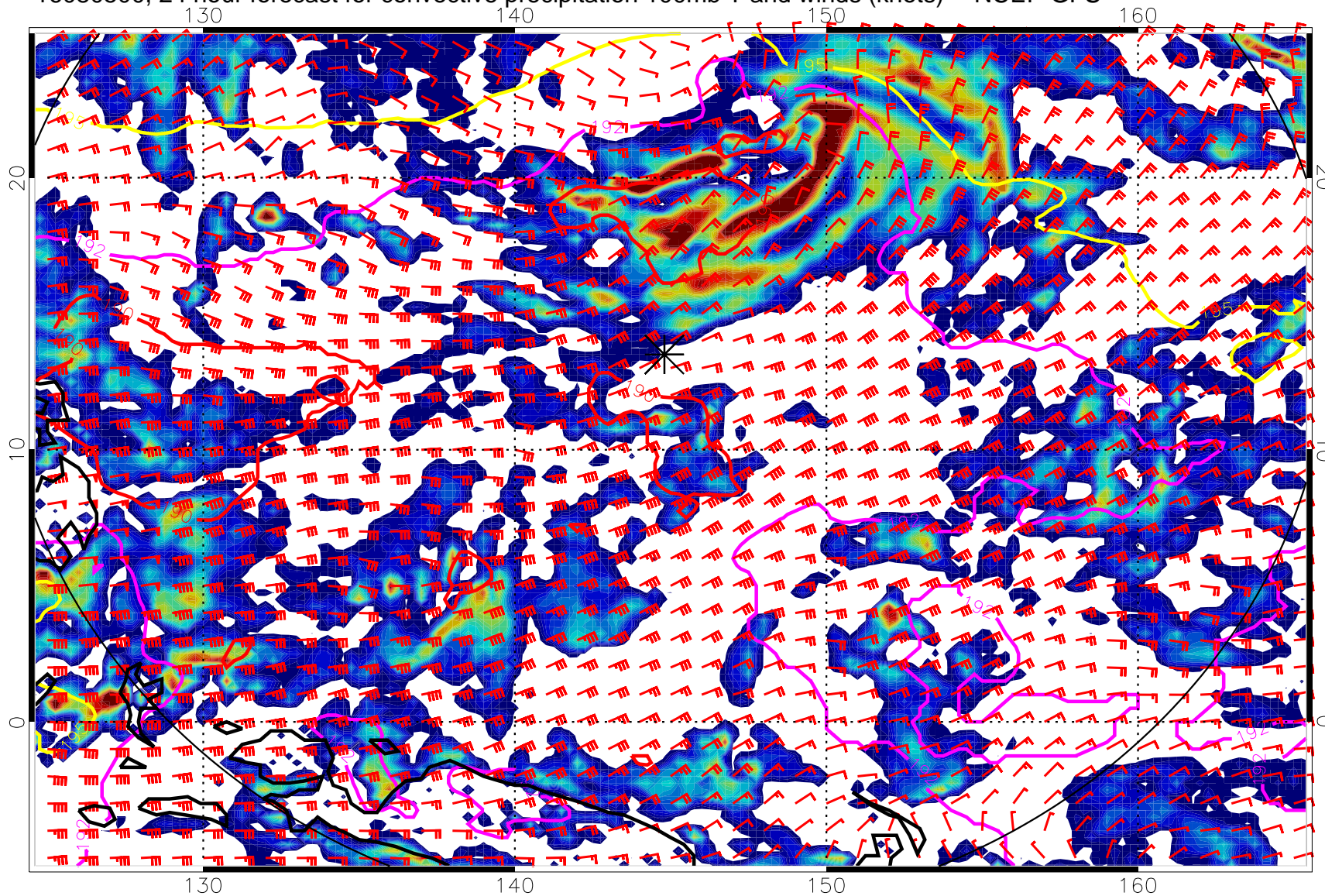
16080500, 24 hour forecast for convective precipitation 100mb T and winds (knots) -- NCEP GFS
