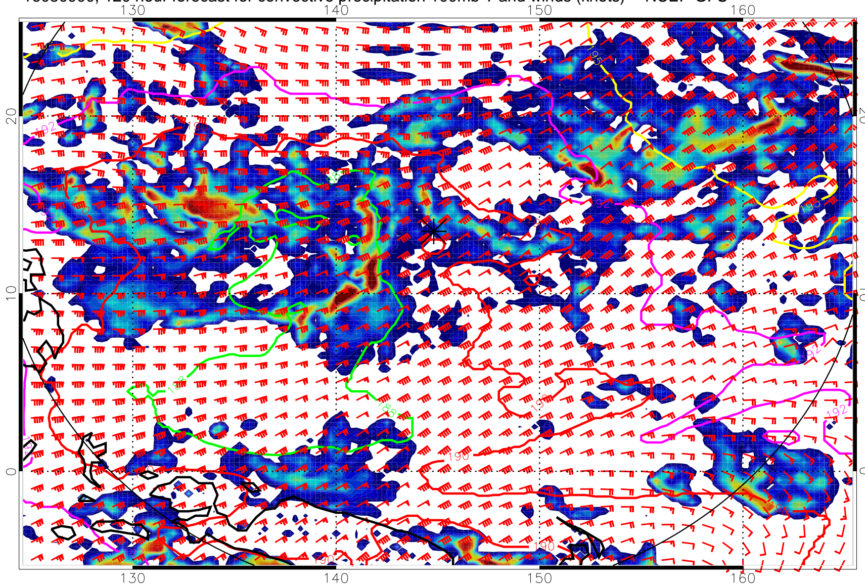
16080900, 120 hour forecast for convective precipitation 100mb T and winds (knots) -- NCEP GFS
