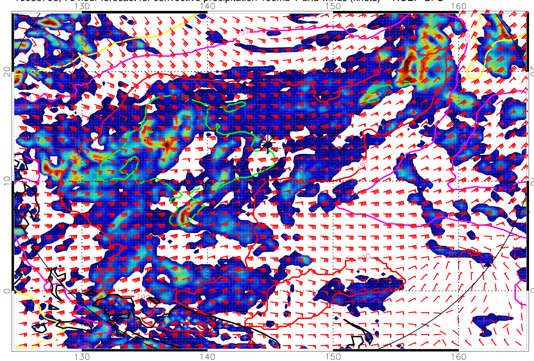
16080706, 78 hour forecast for convective precipitation 100mb T and winds (knots) -- NCEP GFS
