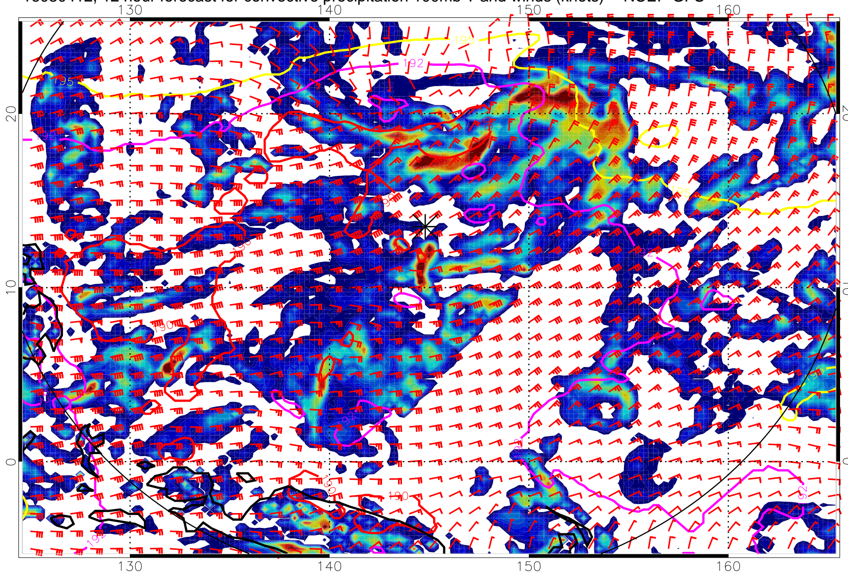
16080412, 12 hour forecast for convective precipitation 100mb T and winds (knots) -- NCEP GFS
