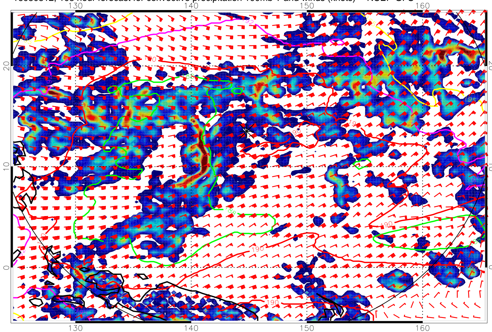
16080812, 108 hour forecast for convective precipitation 100mb T and winds (knots) -- NCEP GFS
