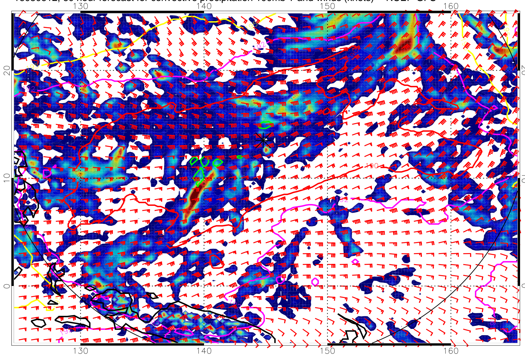
16080612, 60 hour forecast for convective precipitation 100mb T and winds (knots) -- NCEP GFS
