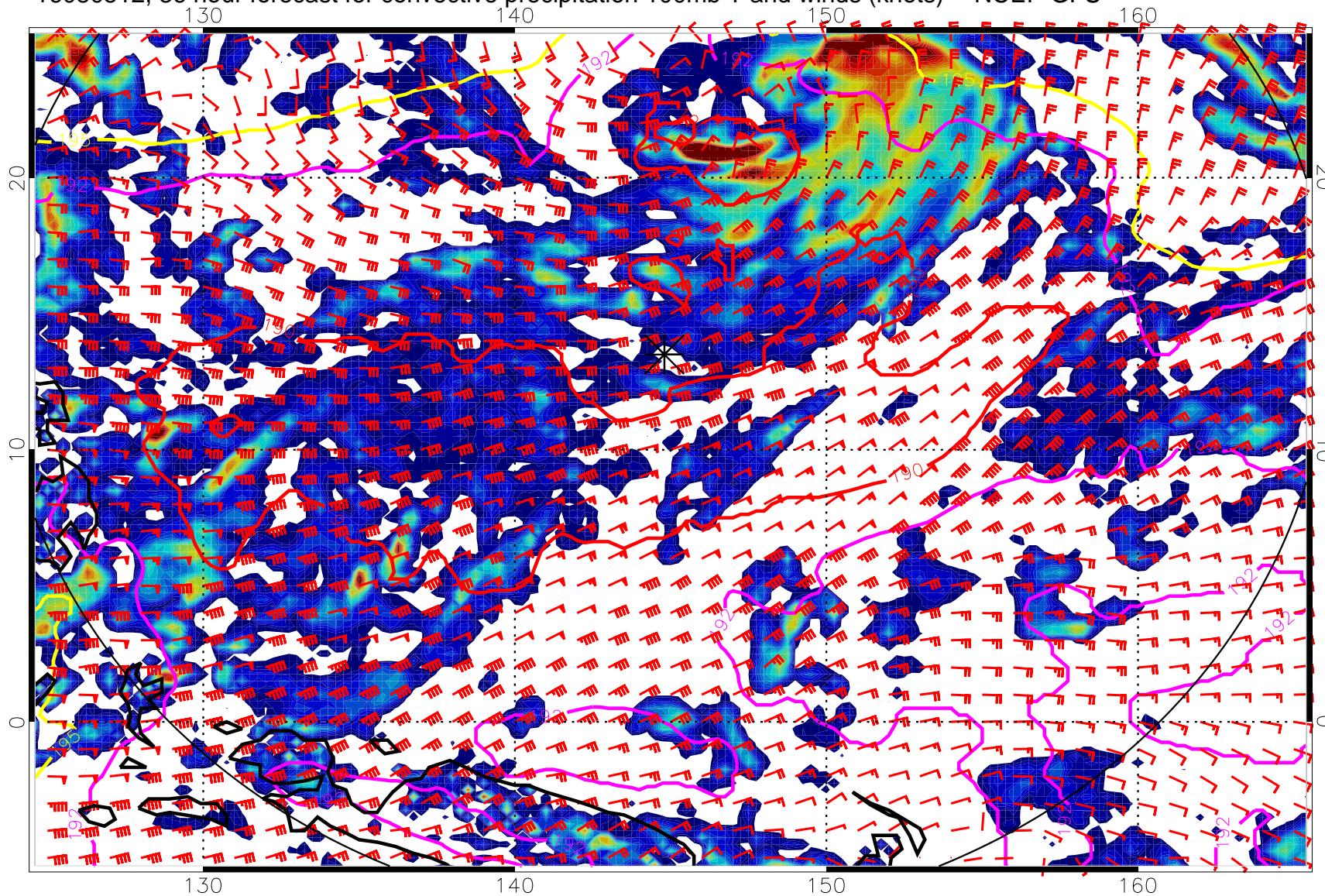
16080512, 36 hour forecast for convective precipitation 100mb T and winds (knots) -- NCEP GFS
