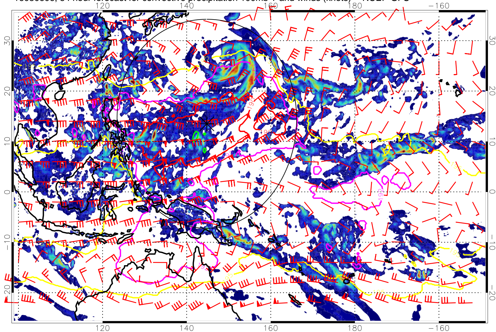
16080606, 54 hour forecast for convective precipitation 100mb T and winds (knots) -- NCEP GFS
