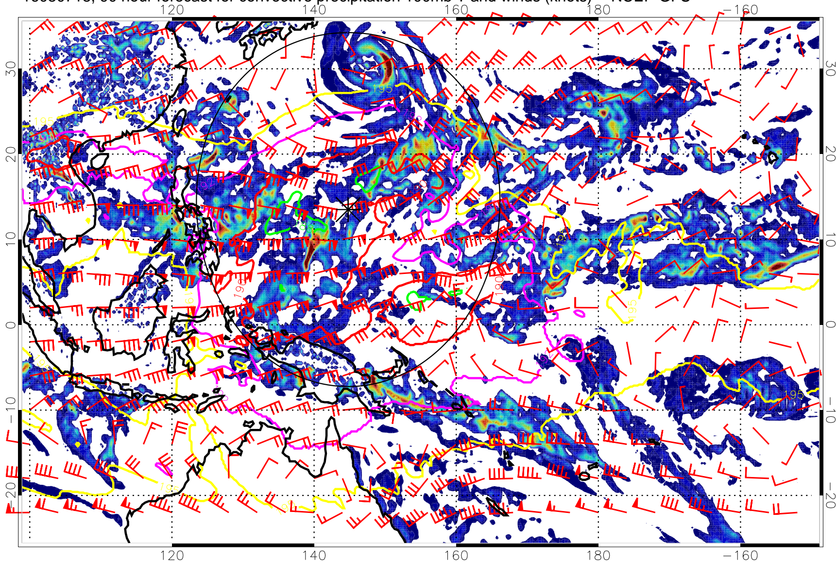
16080718, 90 hour forecast for convective precipitation 100mb T and winds (knots) -- NCEP GFS
