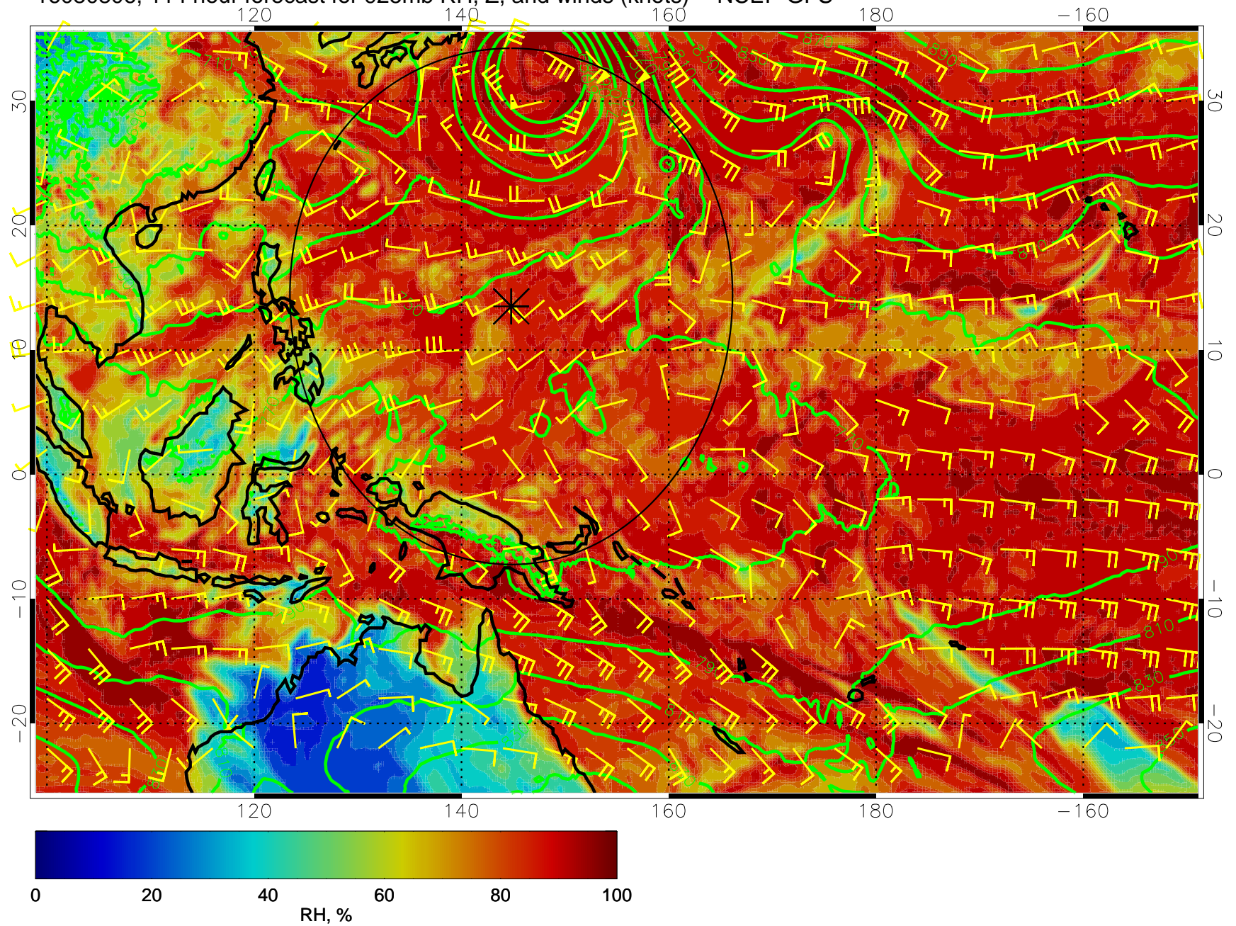
16080806, 114 hour forecast for 925mb RH, Z, and winds (knots) -- NCEP GFS
