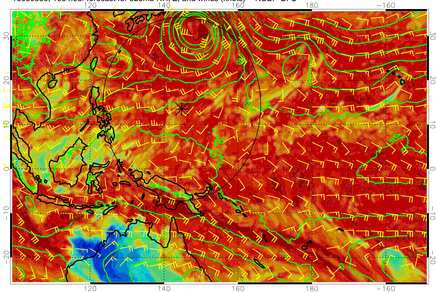
16080800, 108 hour forecast for 925mb RH, Z, and winds (knots) -- NCEP GFS
