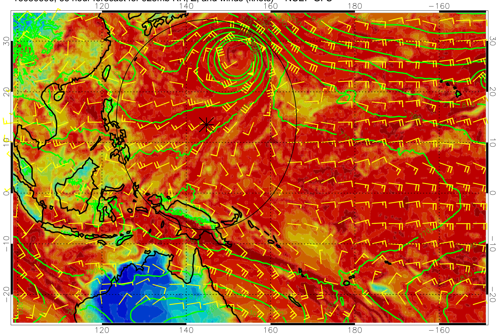
16080606, 66 hour forecast for 925mb RH, Z, and winds (knots) -- NCEP GFS
