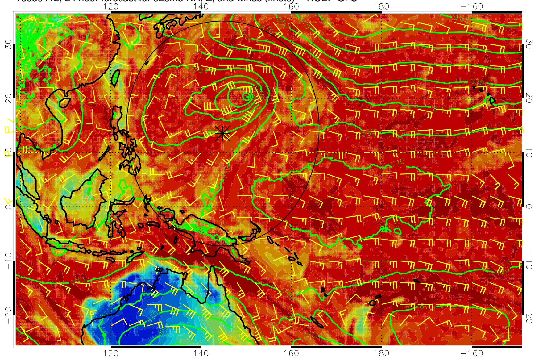
16080412, 24 hour forecast for 925mb RH, Z, and winds (knots) -- NCEP GFS
