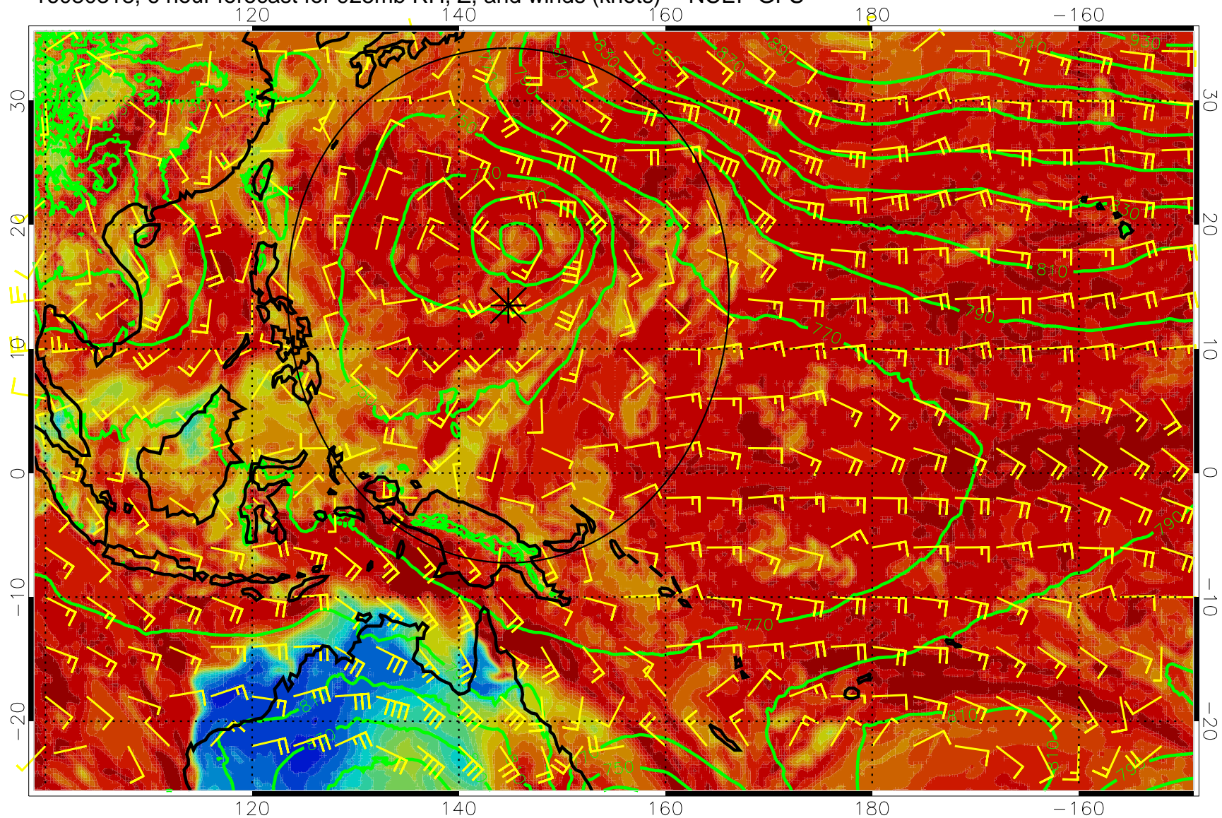
16080318, 6 hour forecast for 925mb RH, Z, and winds (knots) -- NCEP GFS
