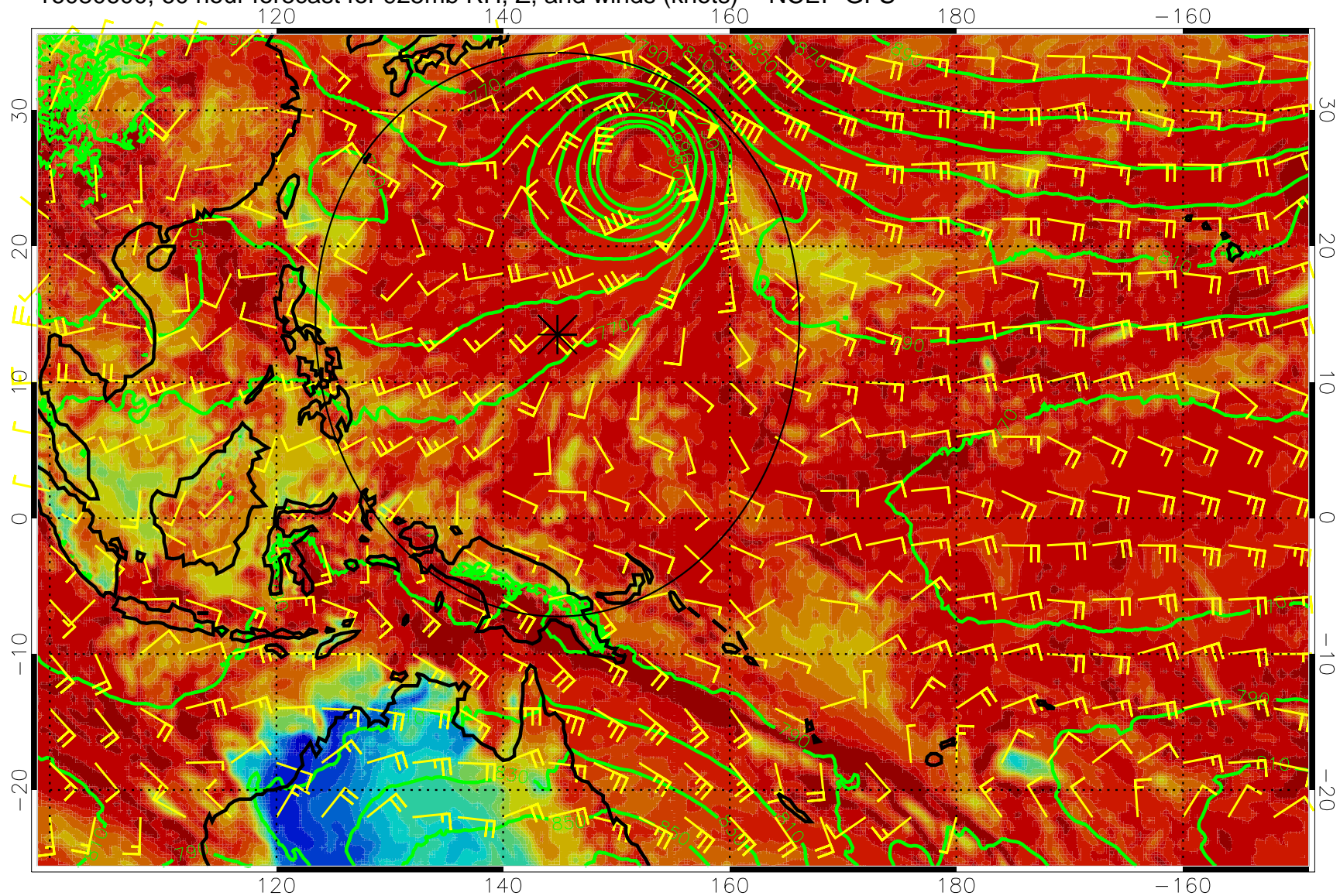
16080600, 60 hour forecast for 925mb RH, Z, and winds (knots) -- NCEP GFS
