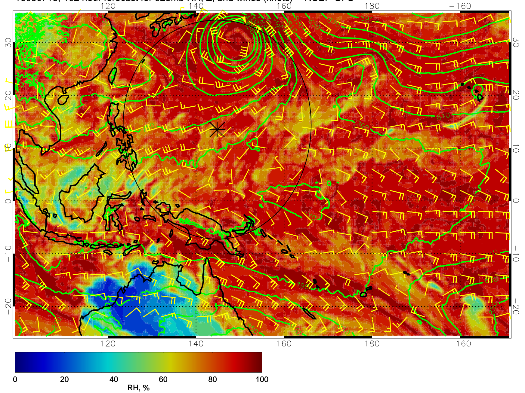
16080718, 102 hour forecast for 925mb RH, Z, and winds (knots) -- NCEP GFS
