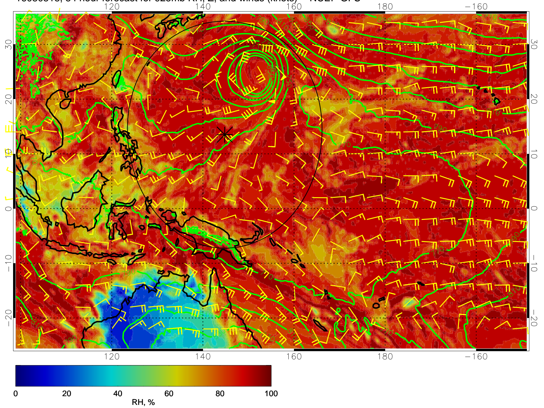
16080518, 54 hour forecast for 925mb RH, Z, and winds (knots) -- NCEP GFS
