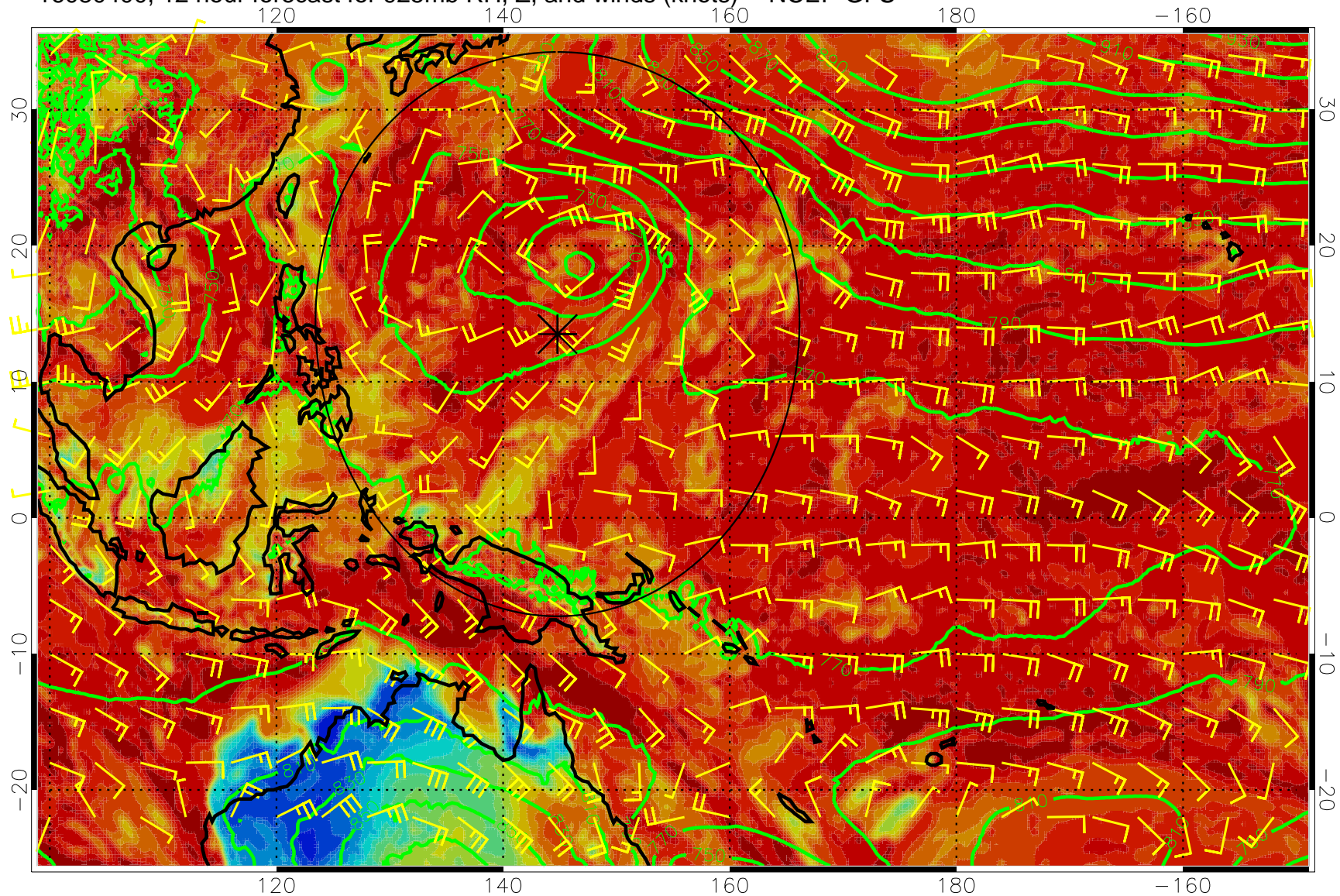
16080400, 12 hour forecast for 925mb RH, Z, and winds (knots) -- NCEP GFS
