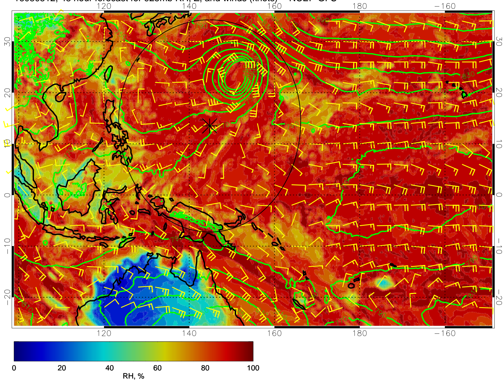
16080512, 48 hour forecast for 925mb RH, Z, and winds (knots) -- NCEP GFS
