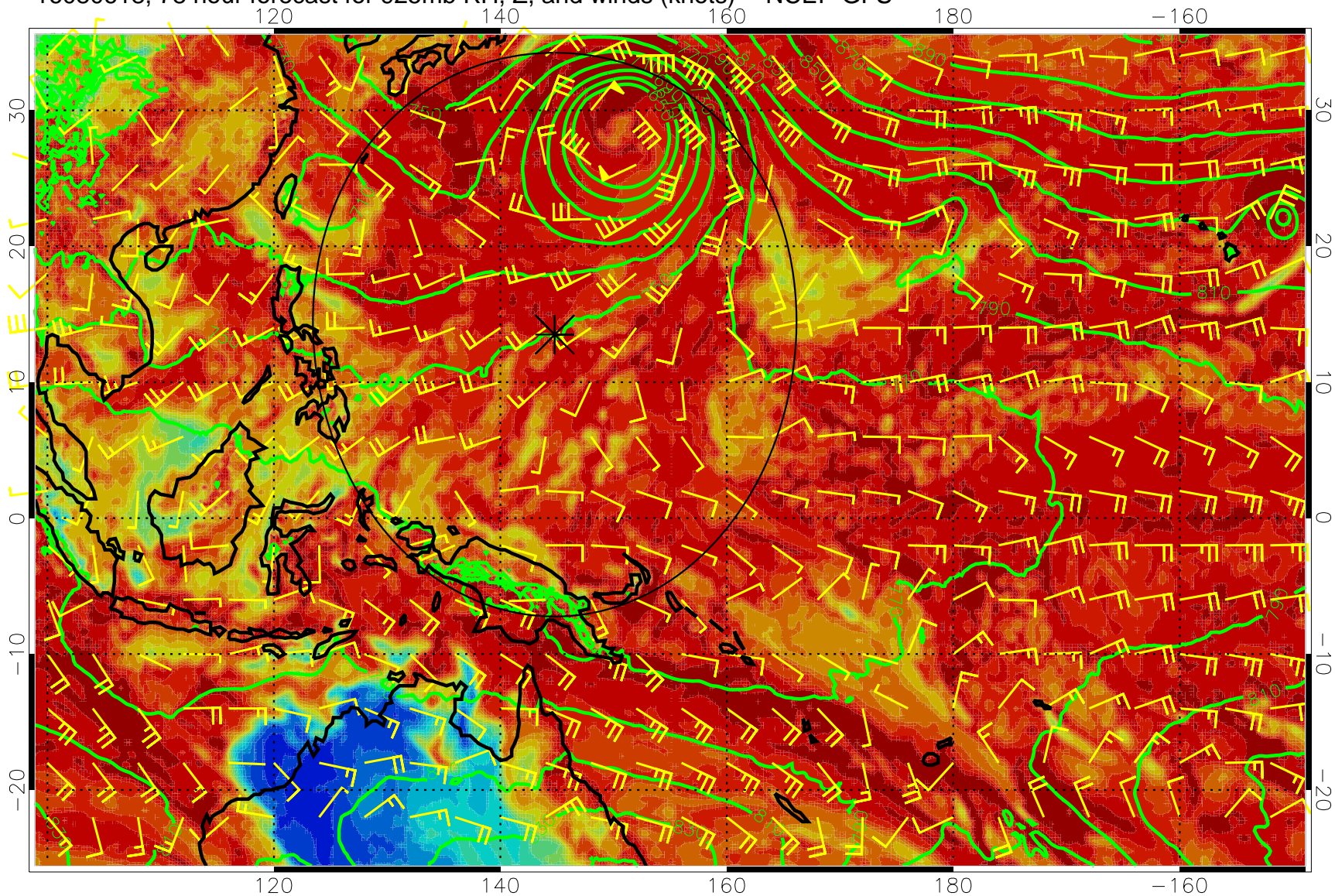
16080618, 78 hour forecast for 925mb RH, Z, and winds (knots) -- NCEP GFS
