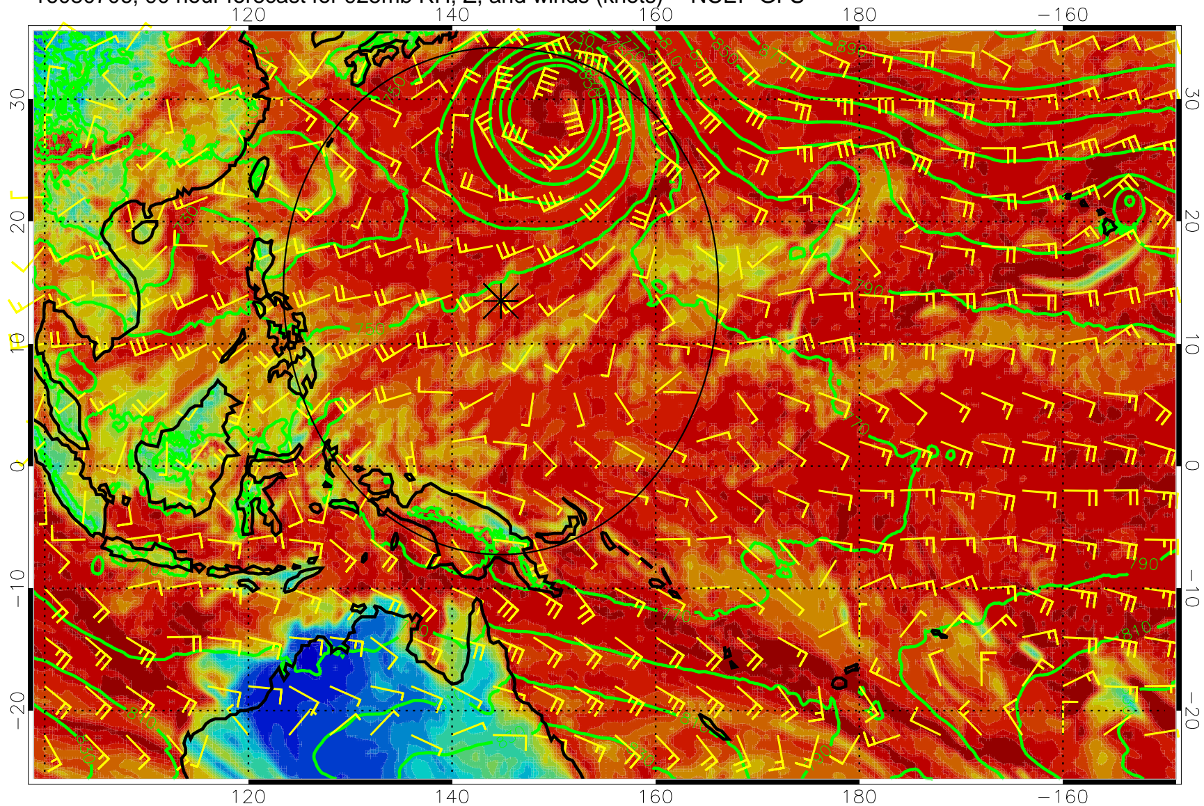
16080706, 90 hour forecast for 925mb RH, Z, and winds (knots) -- NCEP GFS
