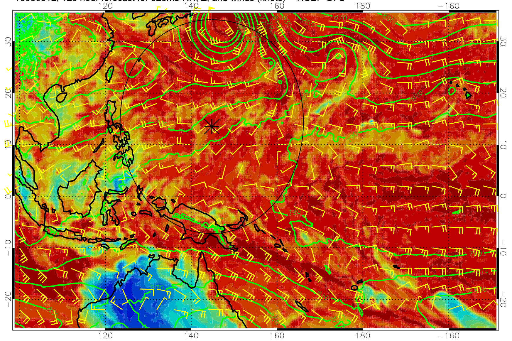
16080812, 120 hour forecast for 925mb RH, Z, and winds (knots) -- NCEP GFS
