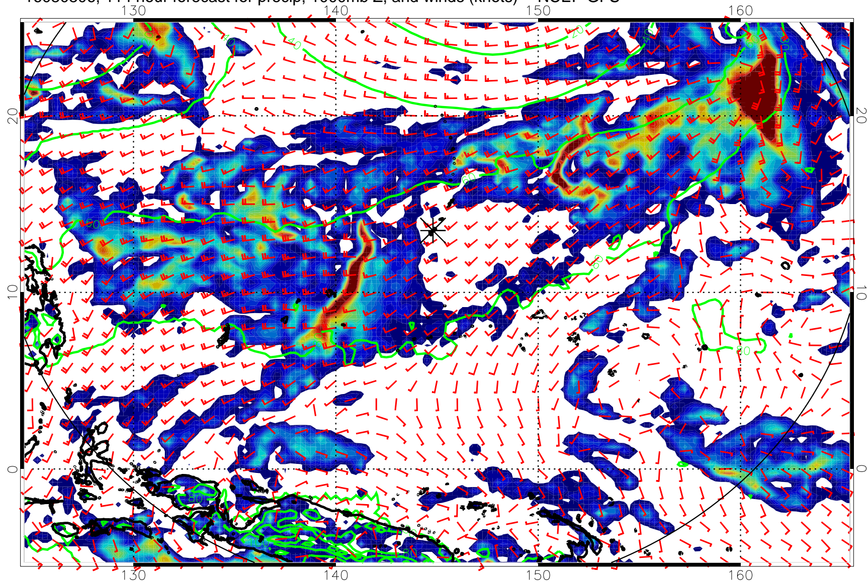
16080806, 114 hour forecast for precip, 1000mb Z, and winds (knots) -- NCEP GFS
