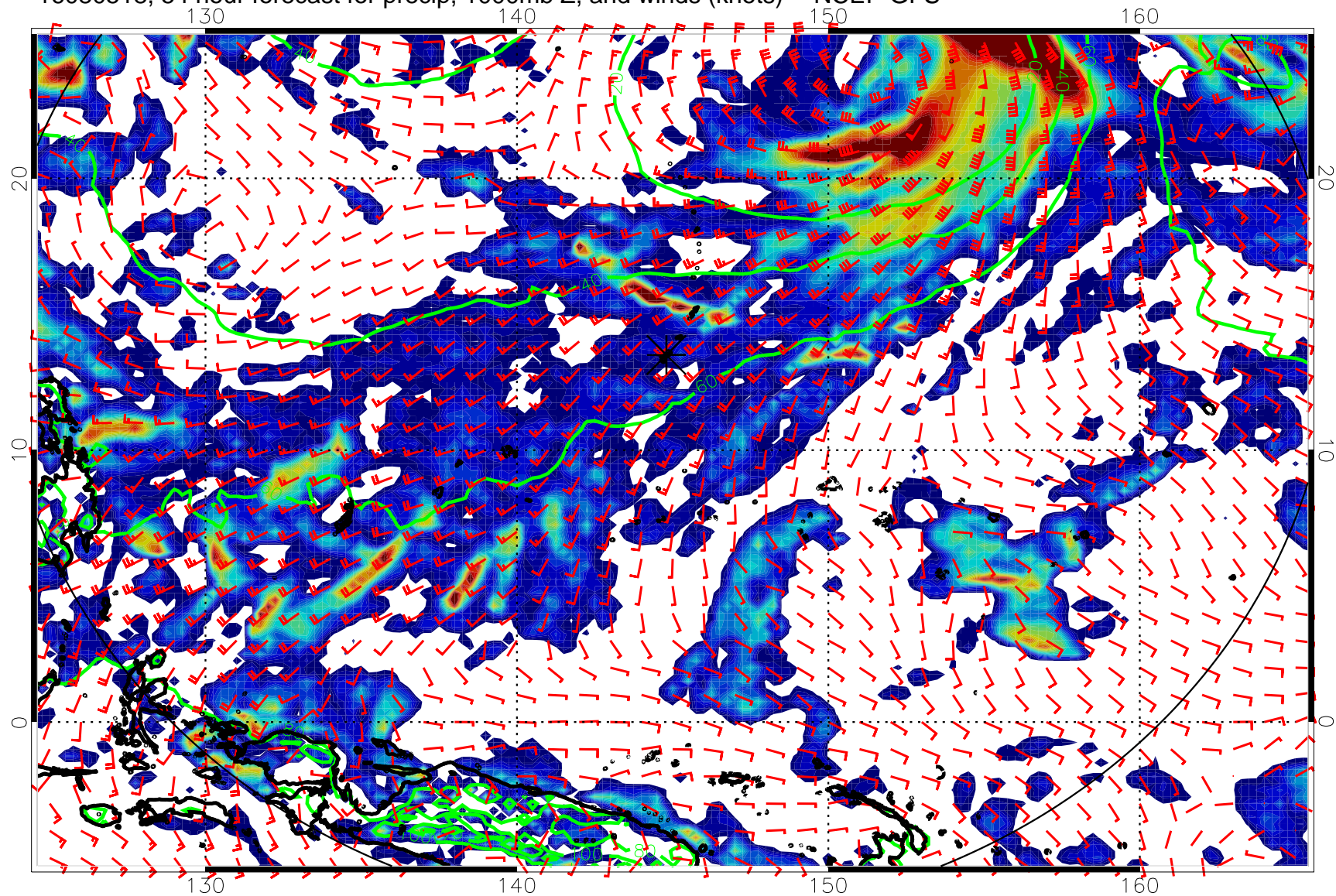
16080518, 54 hour forecast for precip, 1000mb Z, and winds (knots) -- NCEP GFS
