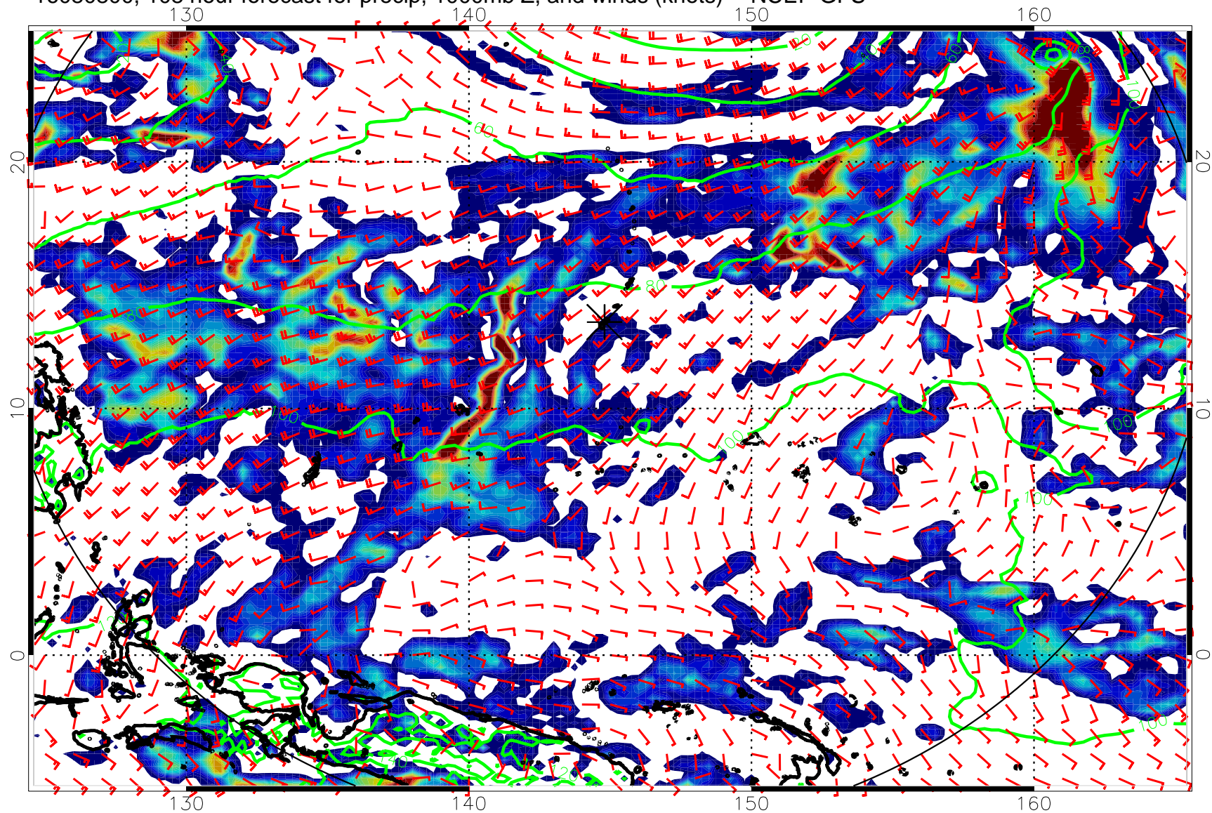
16080800, 108 hour forecast for precip, 1000mb Z, and winds (knots) -- NCEP GFS
