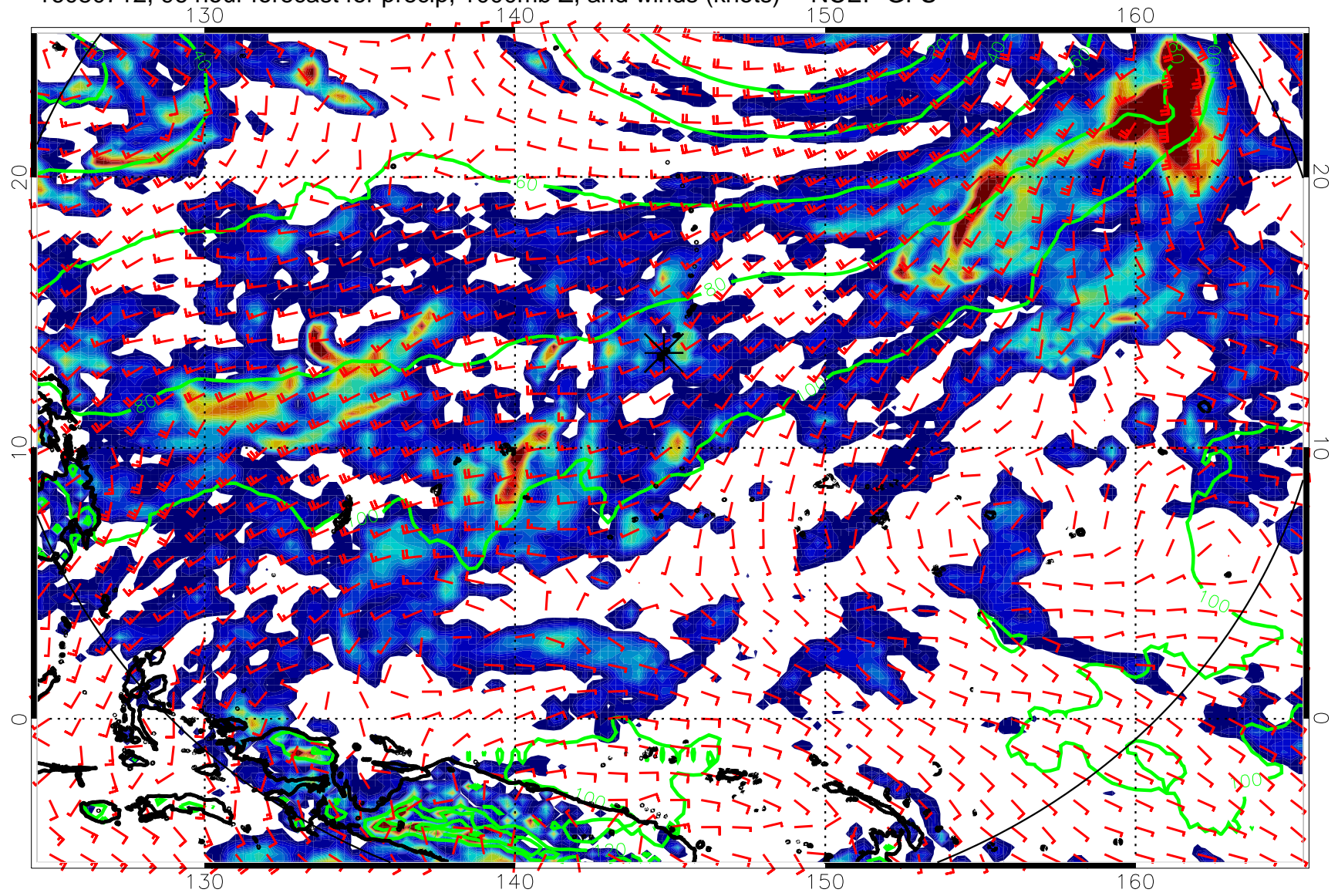
16080712, 96 hour forecast for precip, 1000mb Z, and winds (knots) -- NCEP GFS
