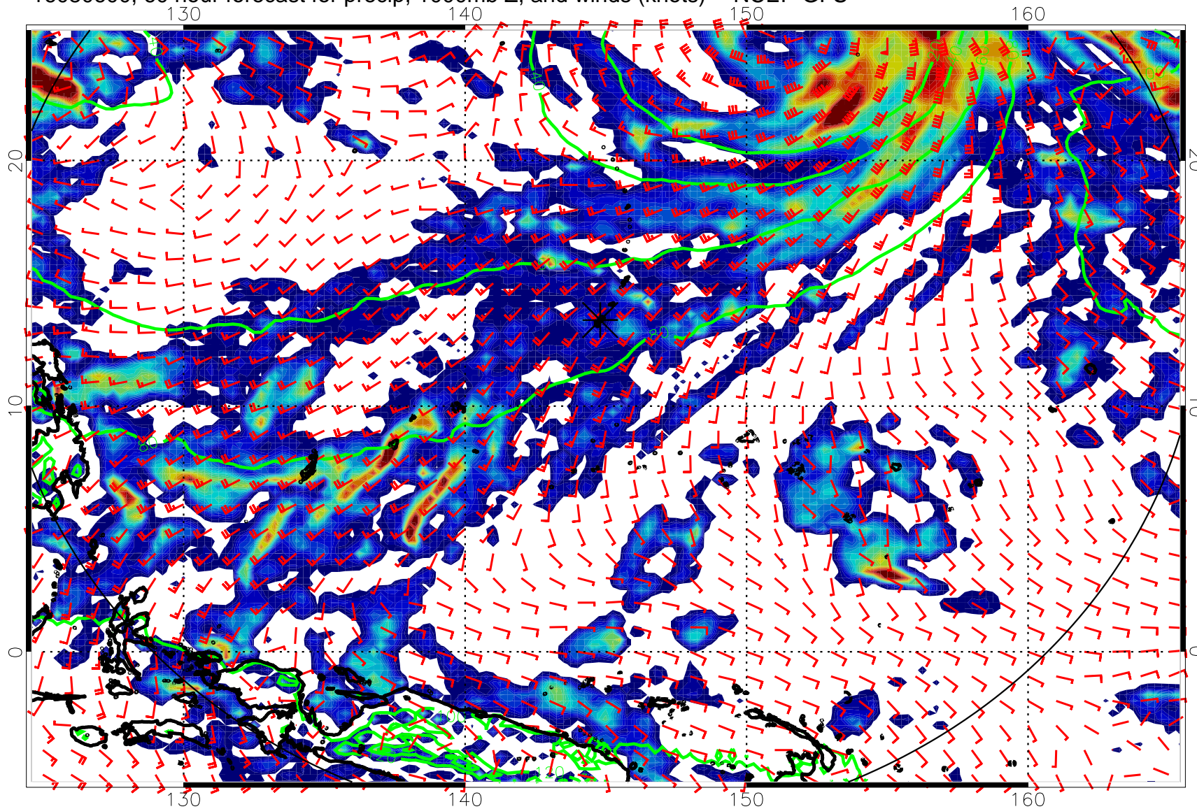
16080600, 60 hour forecast for precip, 1000mb Z, and winds (knots) -- NCEP GFS
