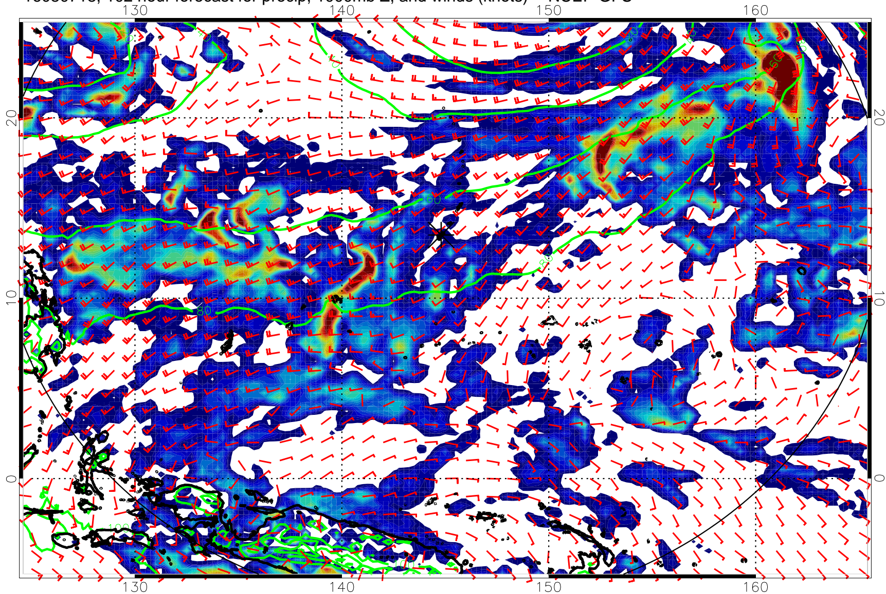
16080718, 102 hour forecast for precip, 1000mb Z, and winds (knots) -- NCEP GFS
