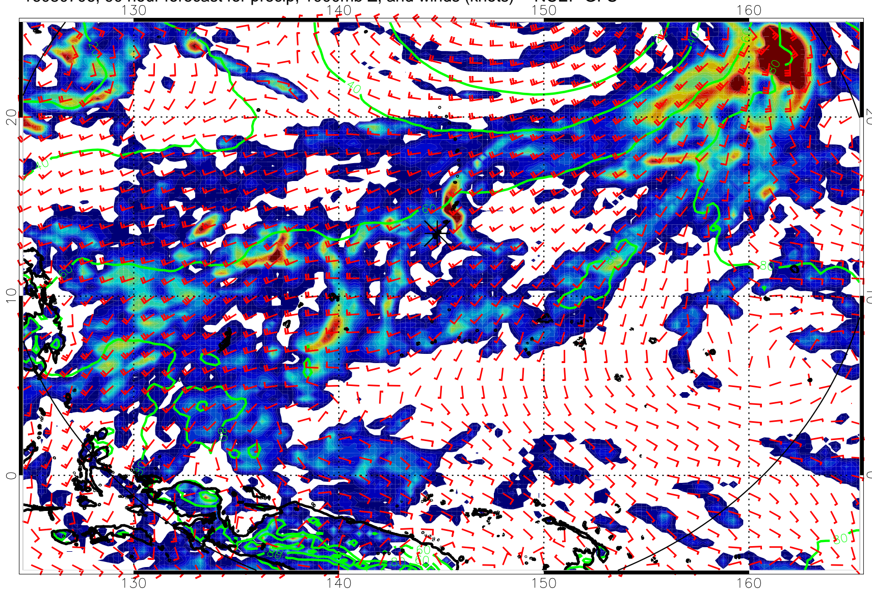
16080706, 90 hour forecast for precip, 1000mb Z, and winds (knots) -- NCEP GFS
