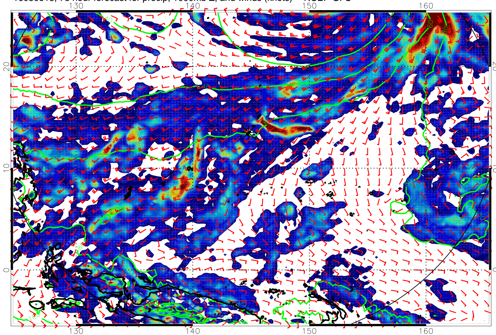
16080618, 78 hour forecast for precip, 1000mb Z, and winds (knots) -- NCEP GFS
