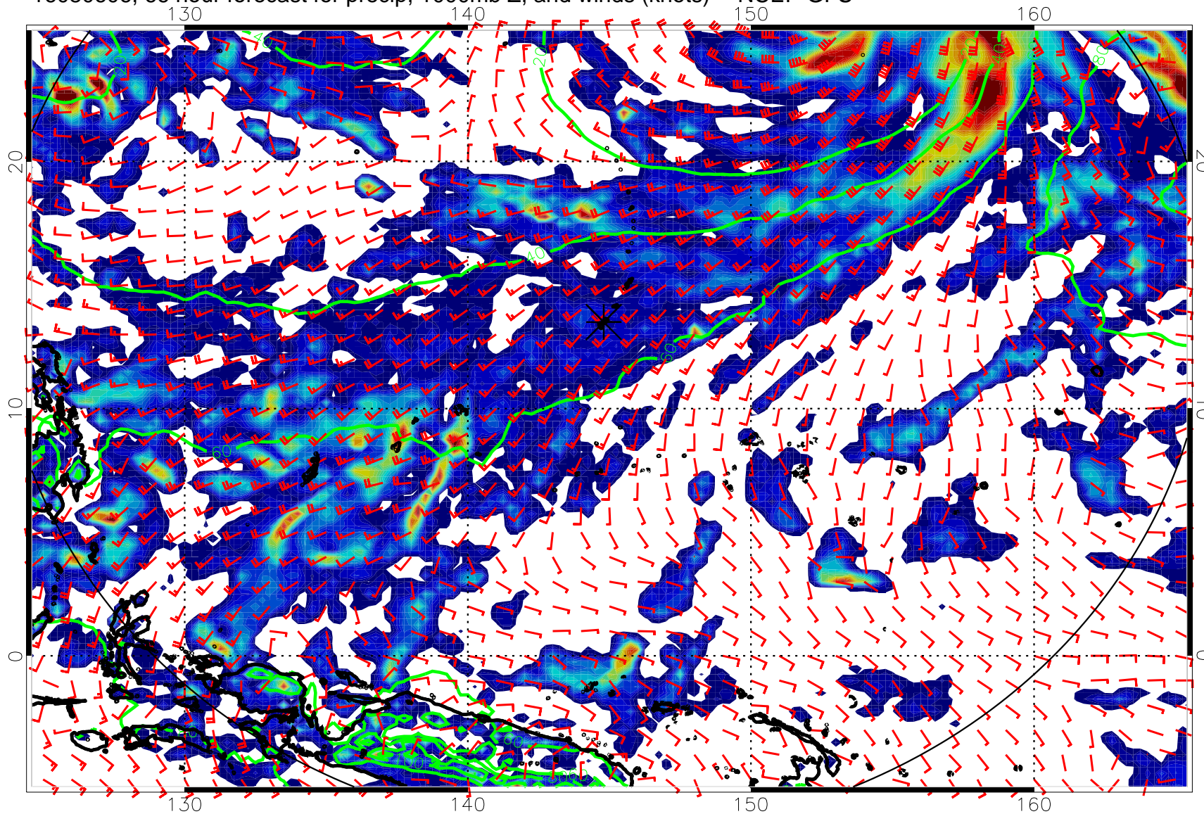
16080606, 66 hour forecast for precip, 1000mb Z, and winds (knots) -- NCEP GFS
