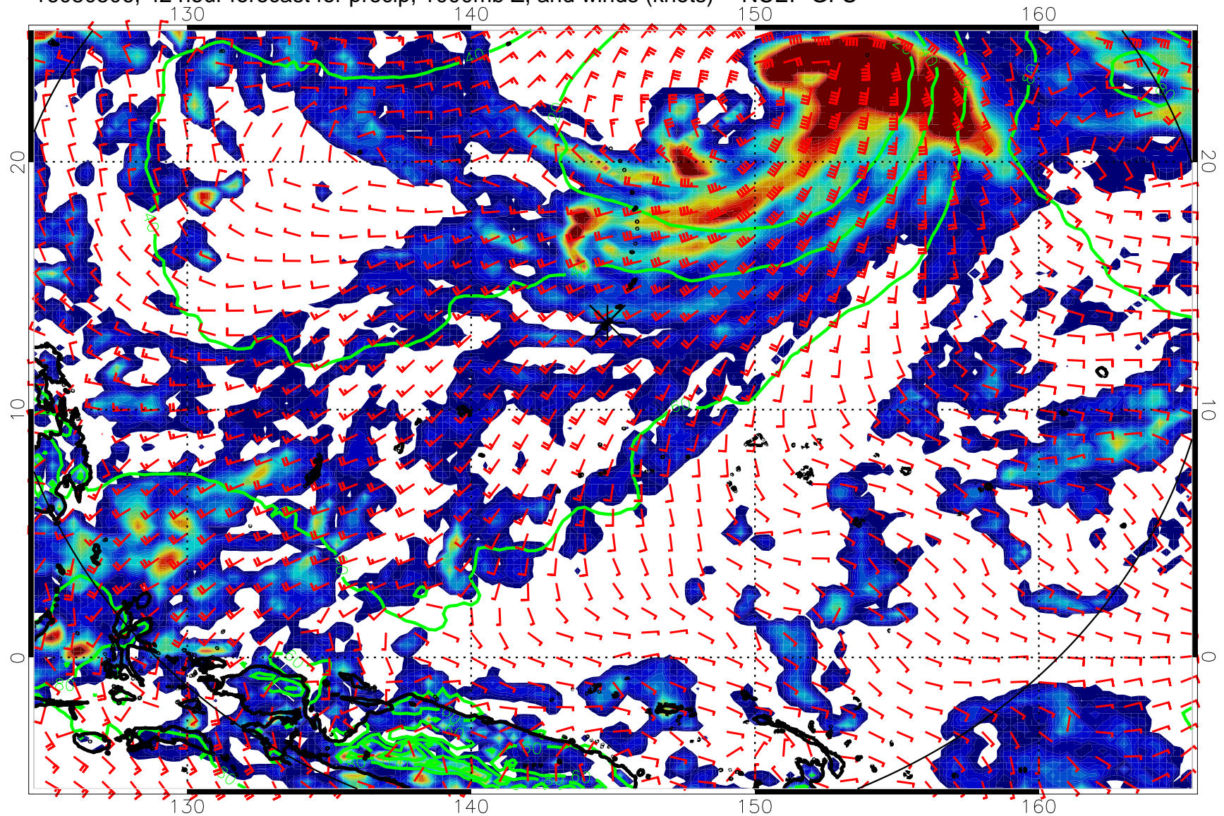
16080506, 42 hour forecast for precip, 1000mb Z, and winds (knots) -- NCEP GFS
