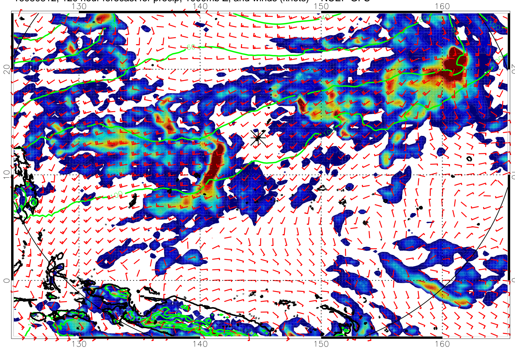
16080812, 120 hour forecast for precip, 1000mb Z, and winds (knots) -- NCEP GFS
