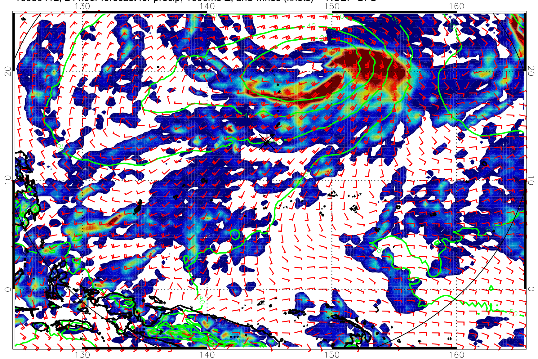
16080412, 24 hour forecast for precip, 1000mb Z, and winds (knots) -- NCEP GFS
