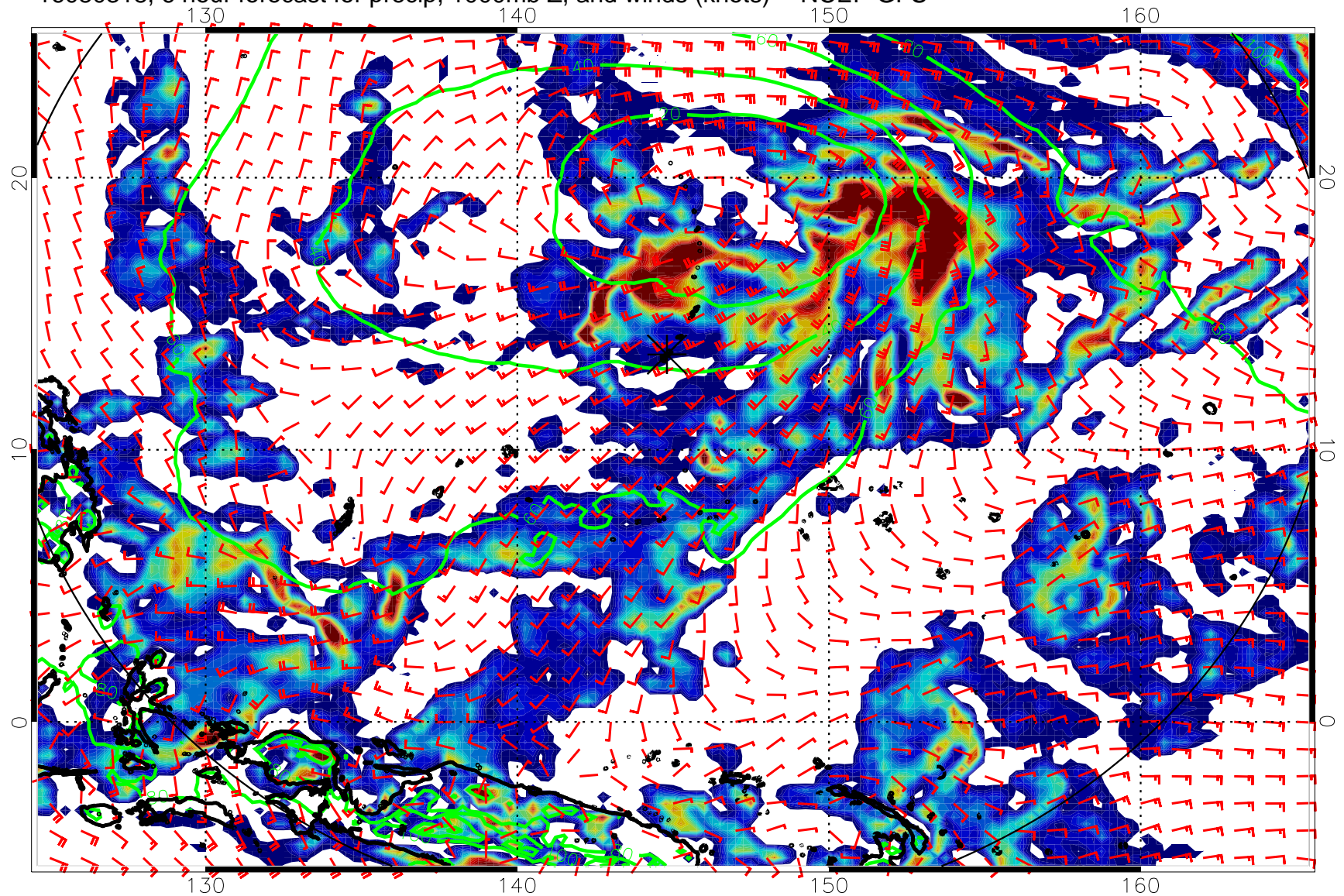
16080318, 6 hour forecast for precip, 1000mb Z, and winds (knots) -- NCEP GFS
