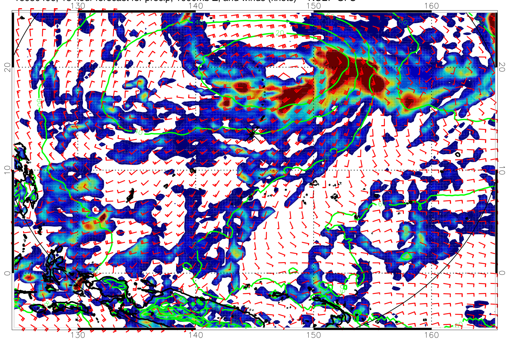
16080406, 18 hour forecast for precip, 1000mb Z, and winds (knots) -- NCEP GFS
