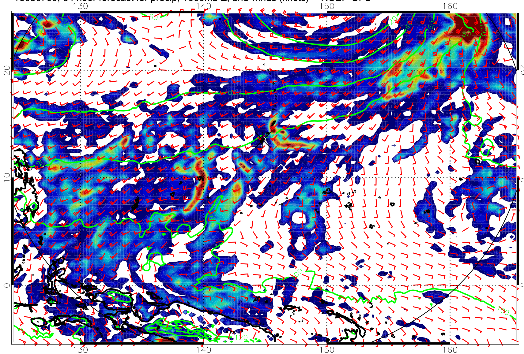
16080700, 84 hour forecast for precip, 1000mb Z, and winds (knots) -- NCEP GFS
