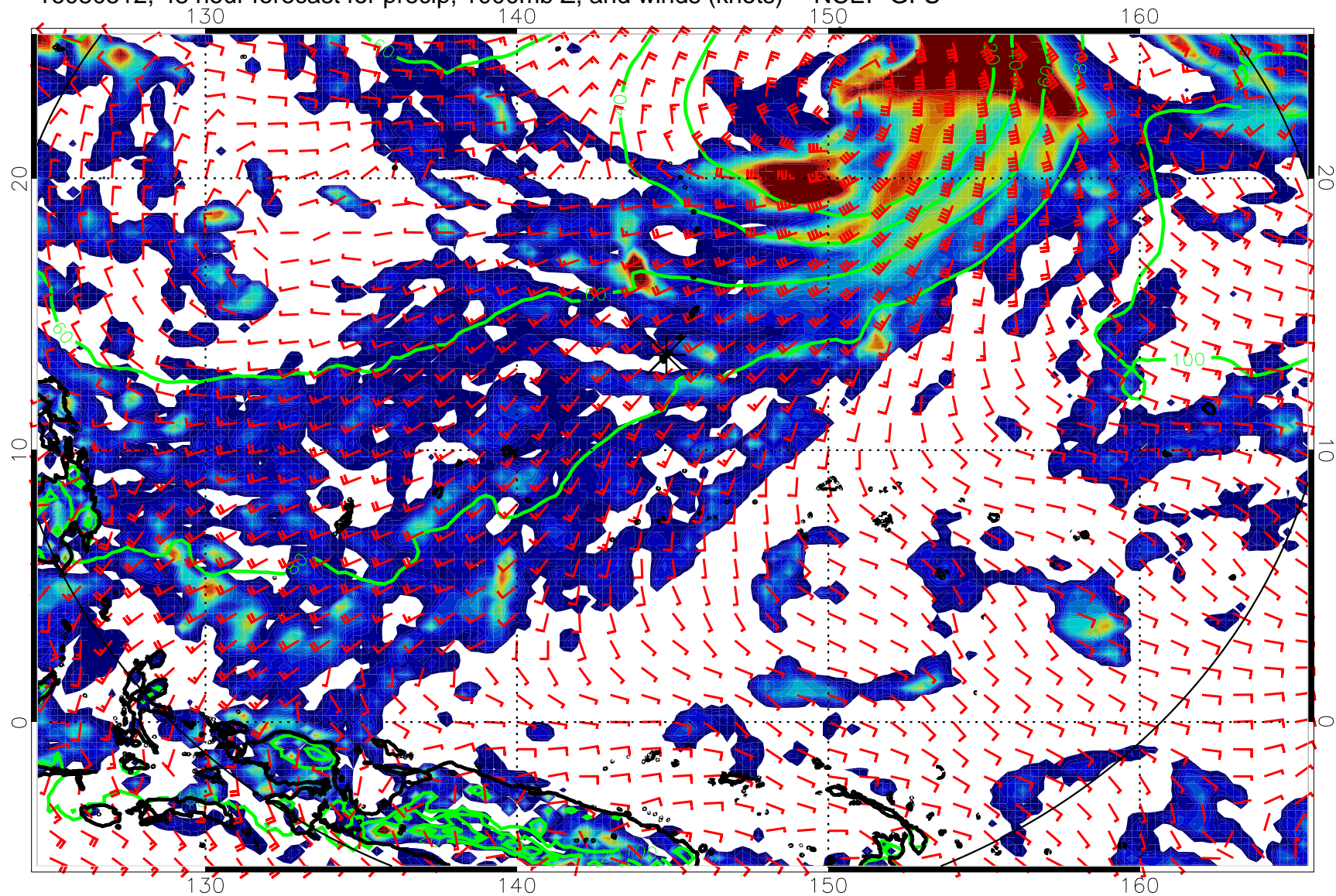
16080512, 48 hour forecast for precip, 1000mb Z, and winds (knots) -- NCEP GFS
