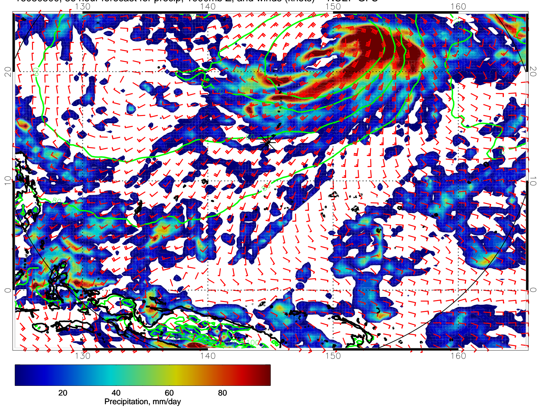
16080500, 36 hour forecast for precip, 1000mb Z, and winds (knots) -- NCEP GFS
