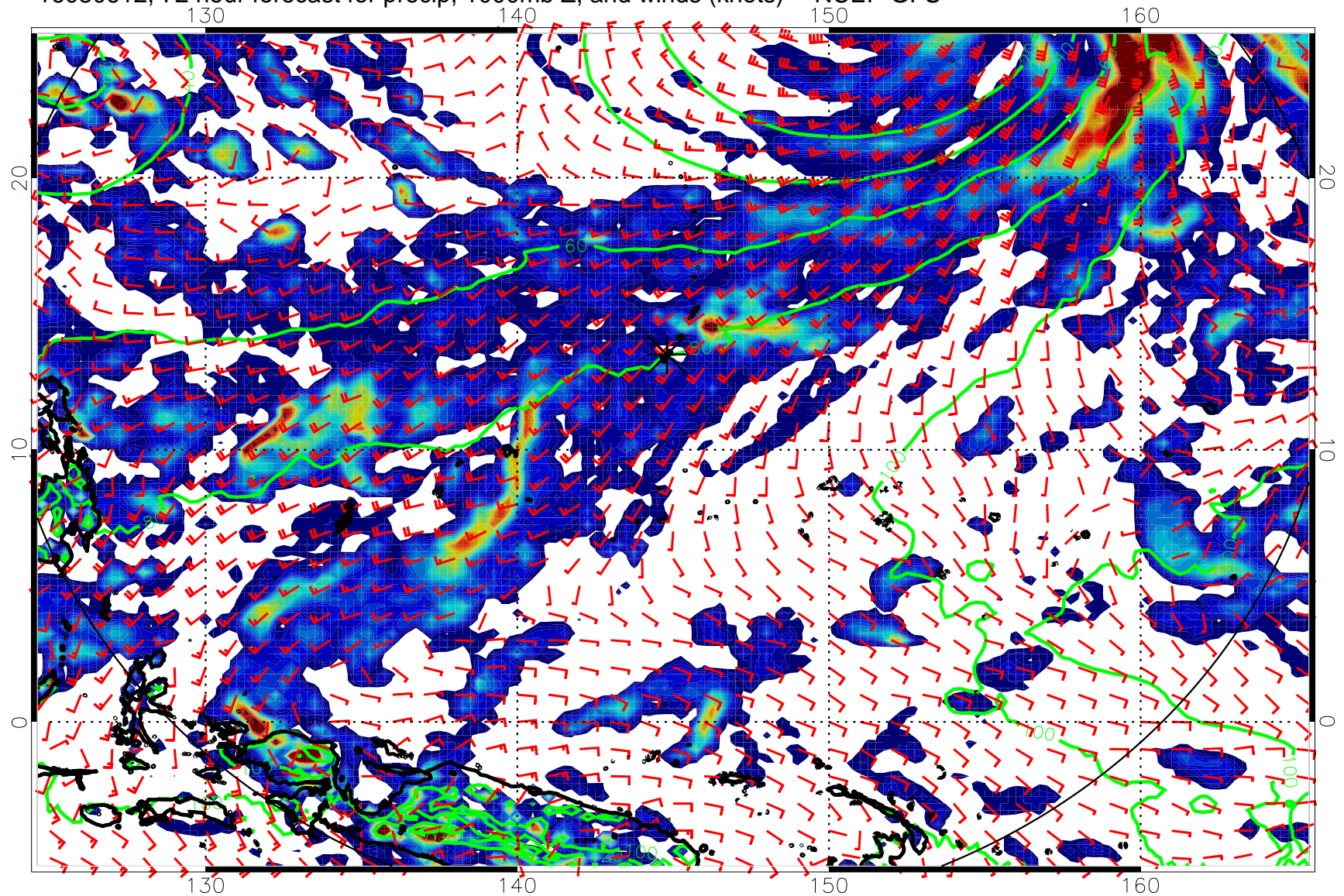
16080612, 72 hour forecast for precip, 1000mb Z, and winds (knots) -- NCEP GFS
