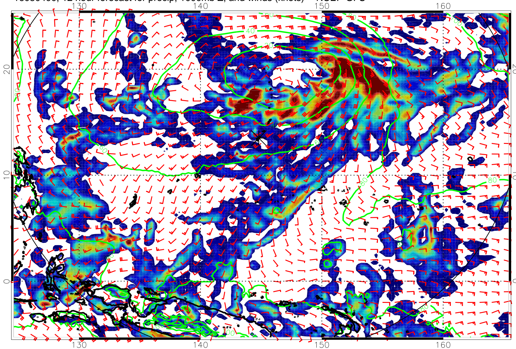
16080400, 12 hour forecast for precip, 1000mb Z, and winds (knots) -- NCEP GFS
