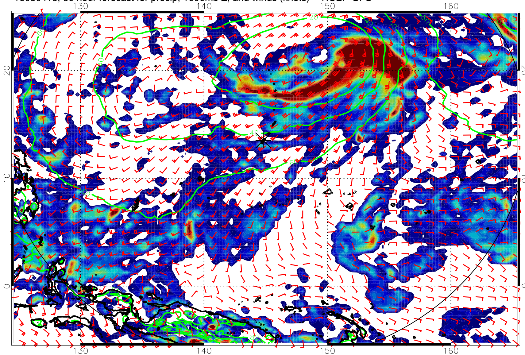
16080418, 30 hour forecast for precip, 1000mb Z, and winds (knots) -- NCEP GFS
