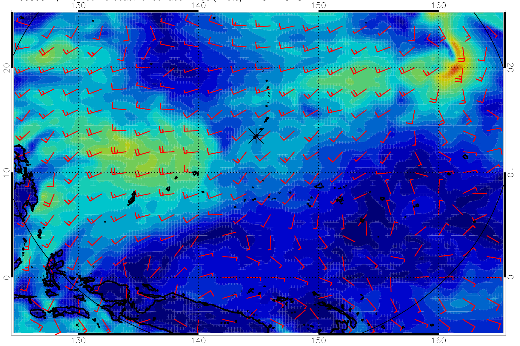
16080812, 120 hour forecast for surface winds (knots) -- NCEP GFS
