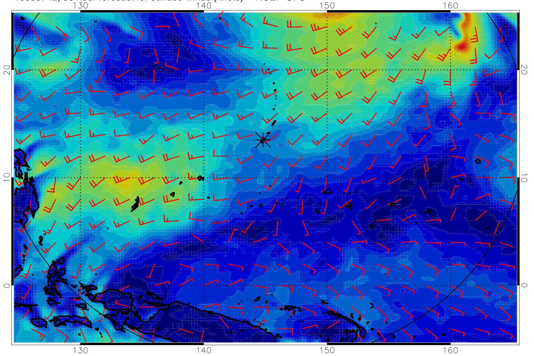
16080712, 96 hour forecast for surface winds (knots) -- NCEP GFS
