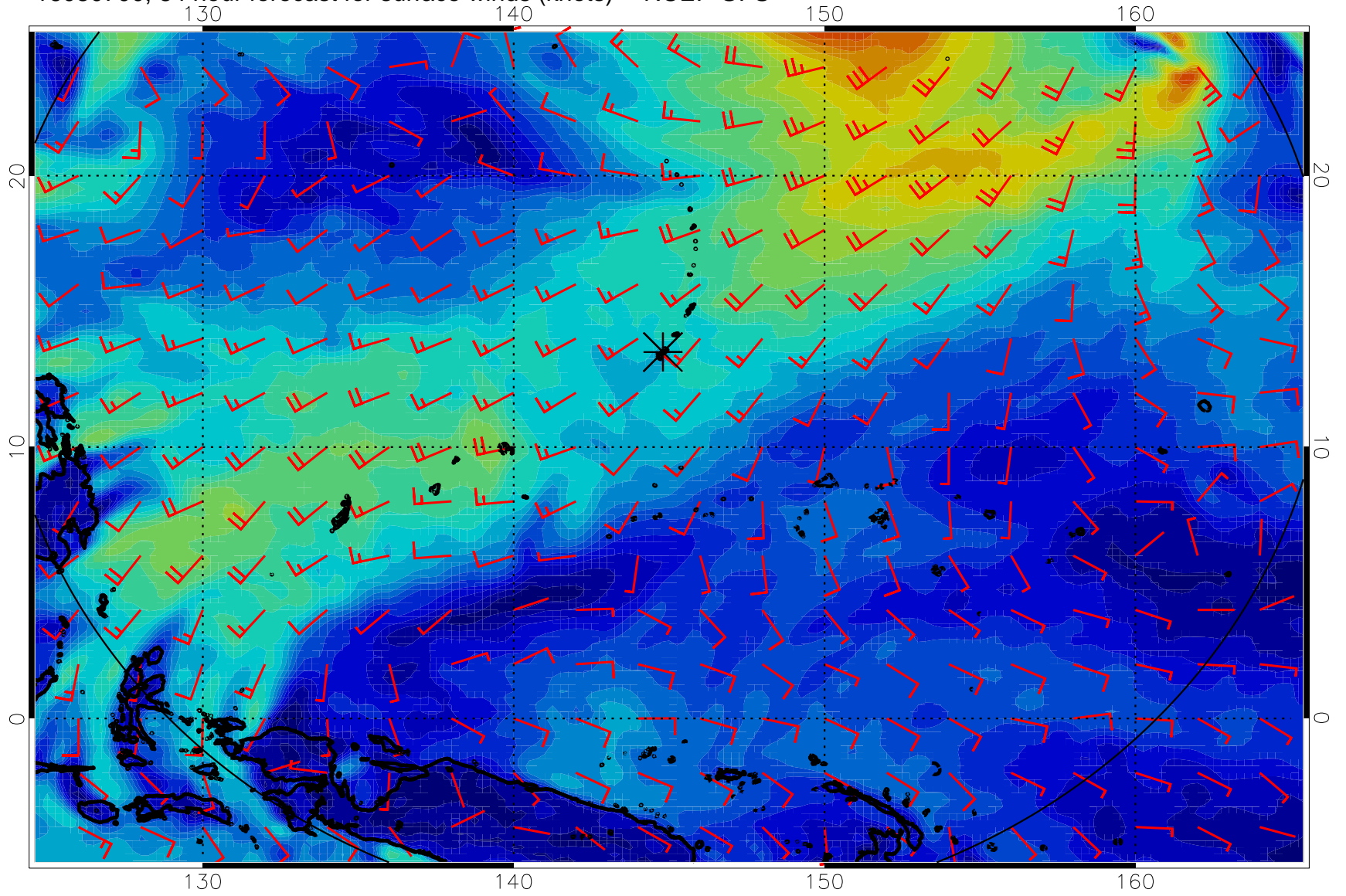
16080700, 84 hour forecast for surface winds (knots) -- NCEP GFS
