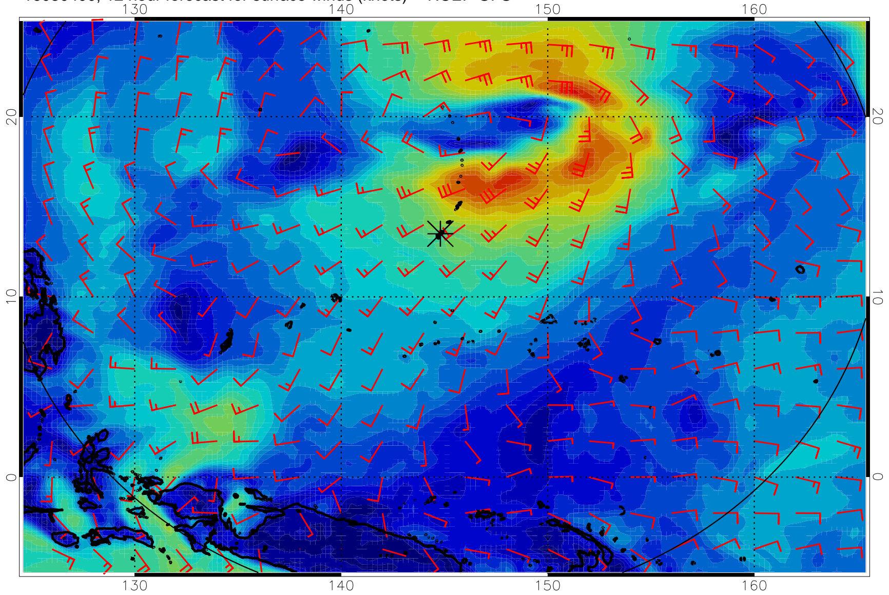
16080400, 12 hour forecast for surface winds (knots) -- NCEP GFS
