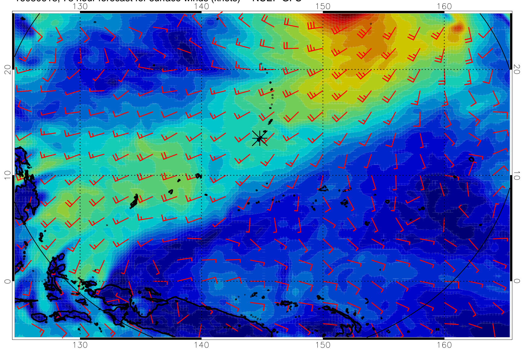
16080618, 78 hour forecast for surface winds (knots) -- NCEP GFS
