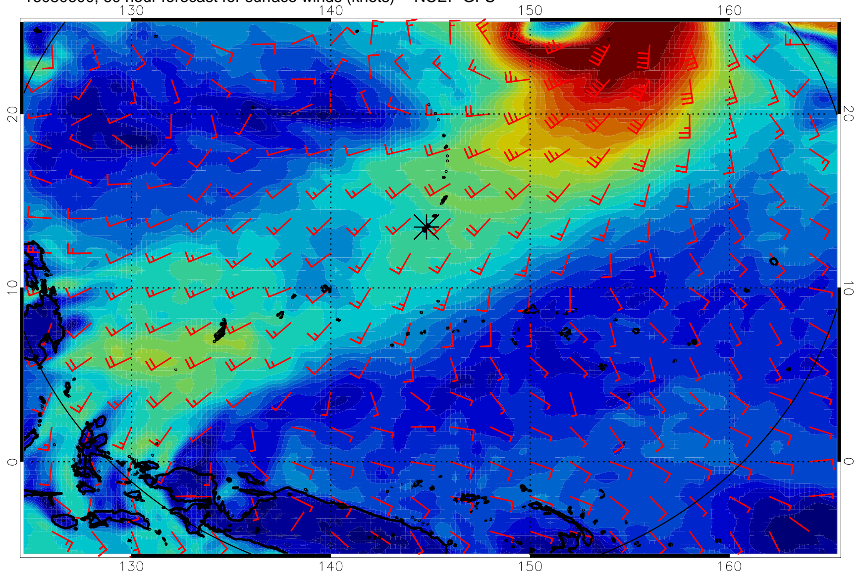
16080600, 60 hour forecast for surface winds (knots) -- NCEP GFS
