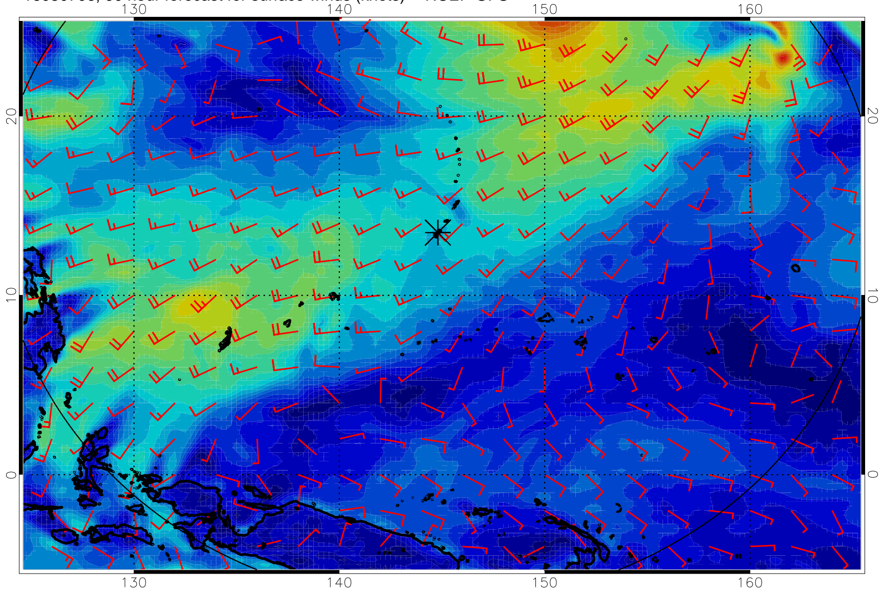
16080706, 90 hour forecast for surface winds (knots) -- NCEP GFS
