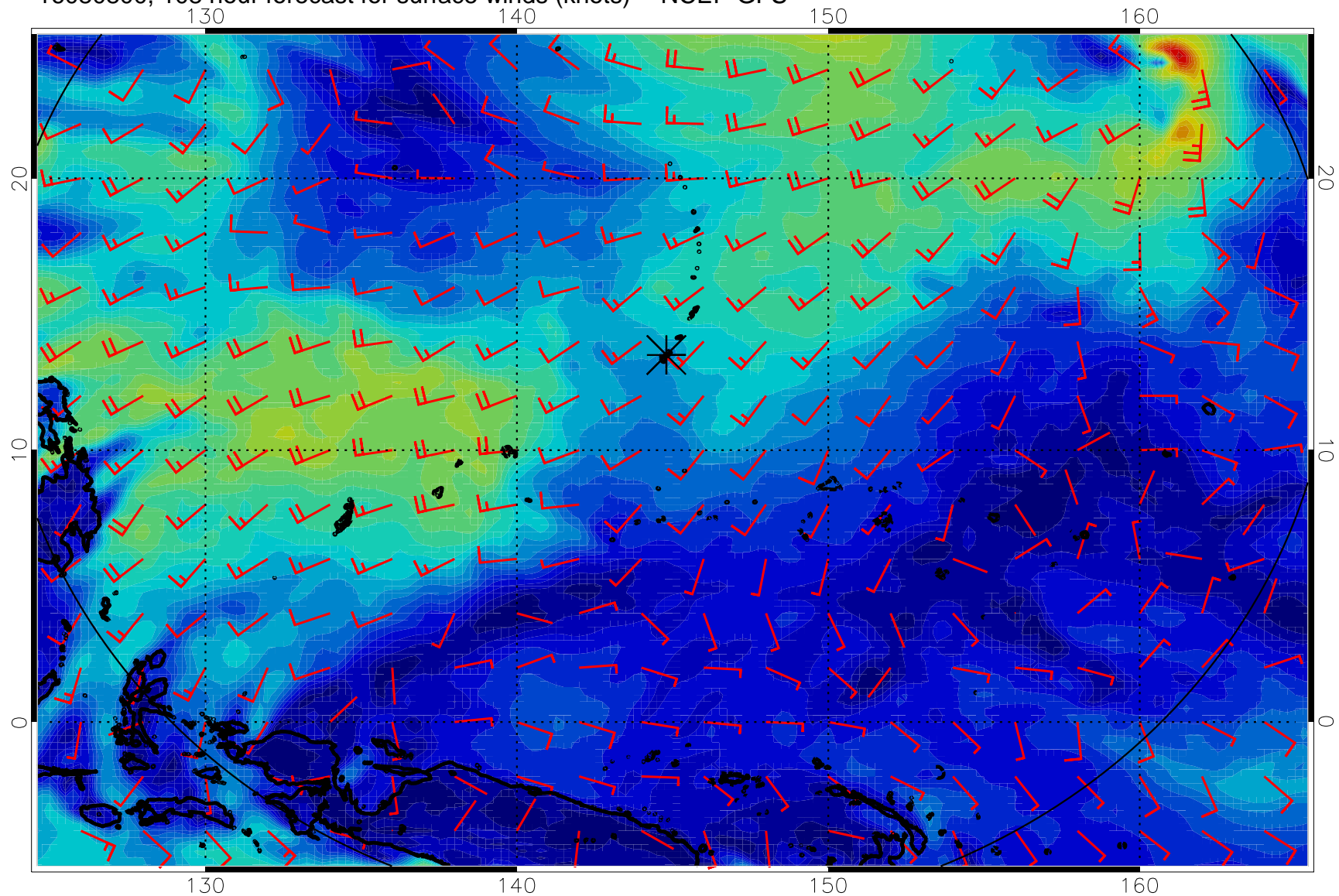
16080800, 108 hour forecast for surface winds (knots) -- NCEP GFS
