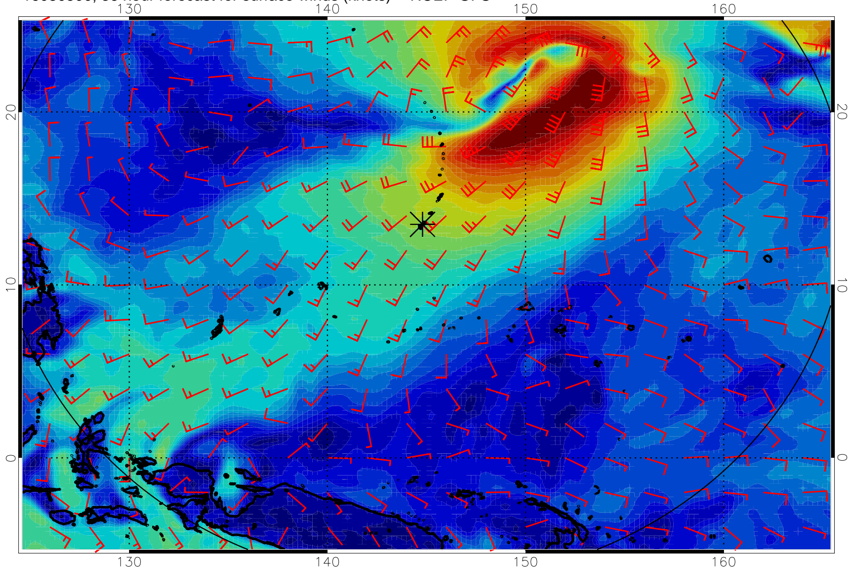
16080500, 36 hour forecast for surface winds (knots) -- NCEP GFS
