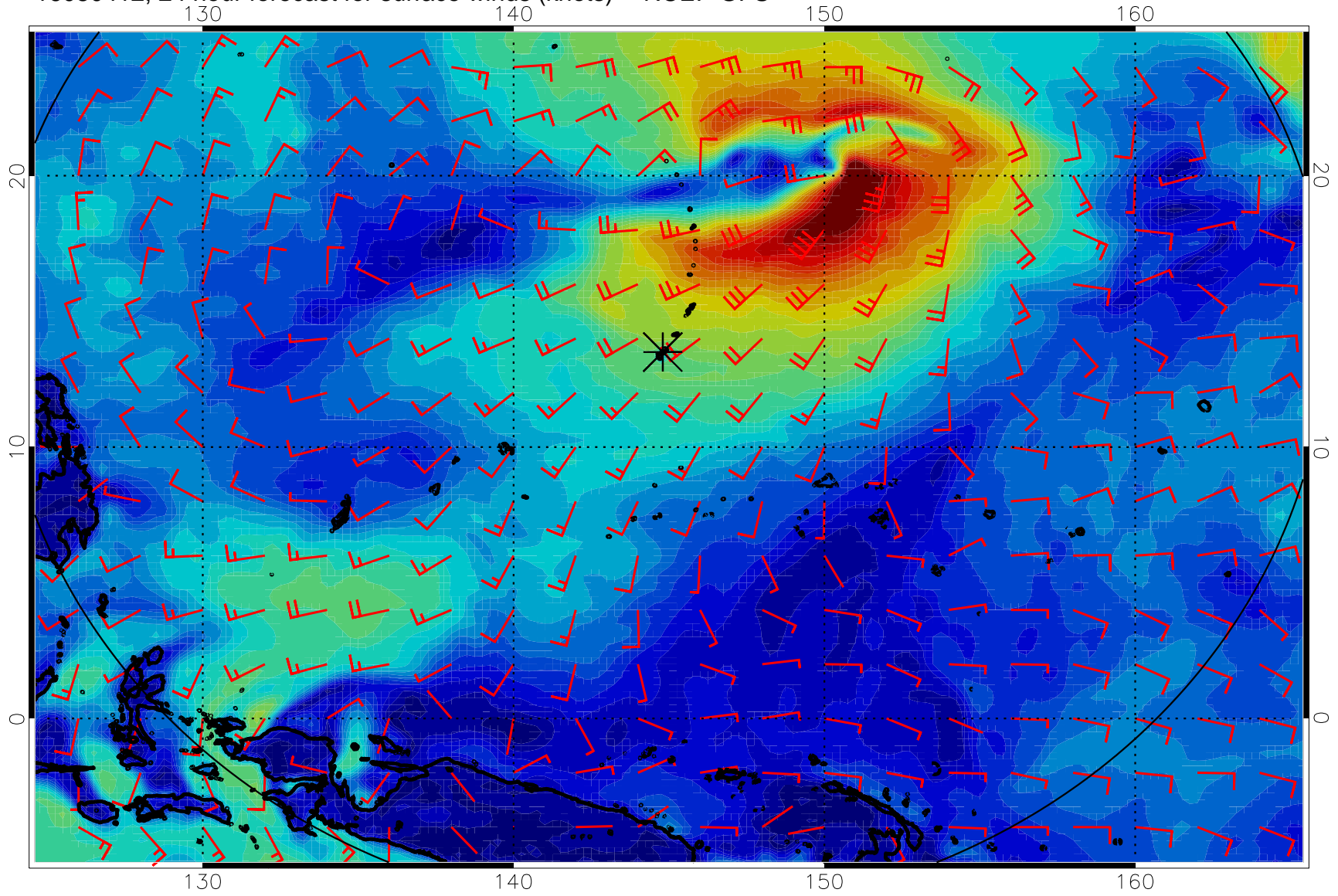
16080412, 24 hour forecast for surface winds (knots) -- NCEP GFS
