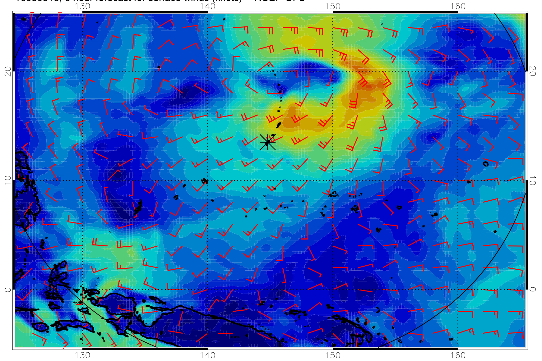
16080318, 6 hour forecast for surface winds (knots) -- NCEP GFS
