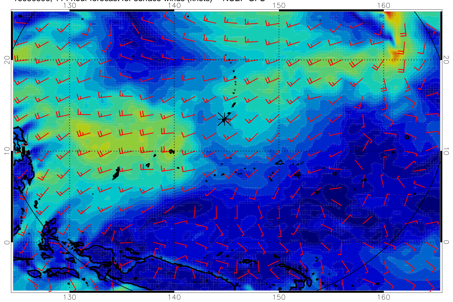
16080806, 114 hour forecast for surface winds (knots) -- NCEP GFS
