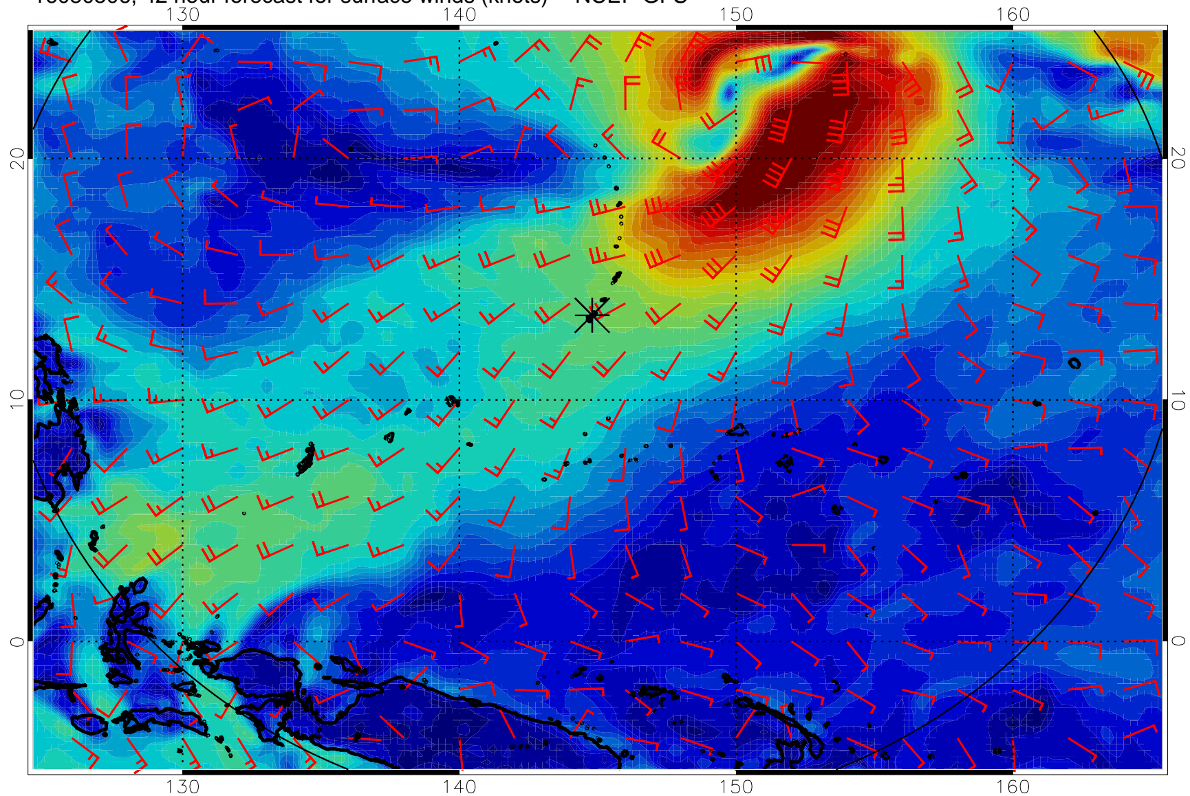
16080506, 42 hour forecast for surface winds (knots) -- NCEP GFS
