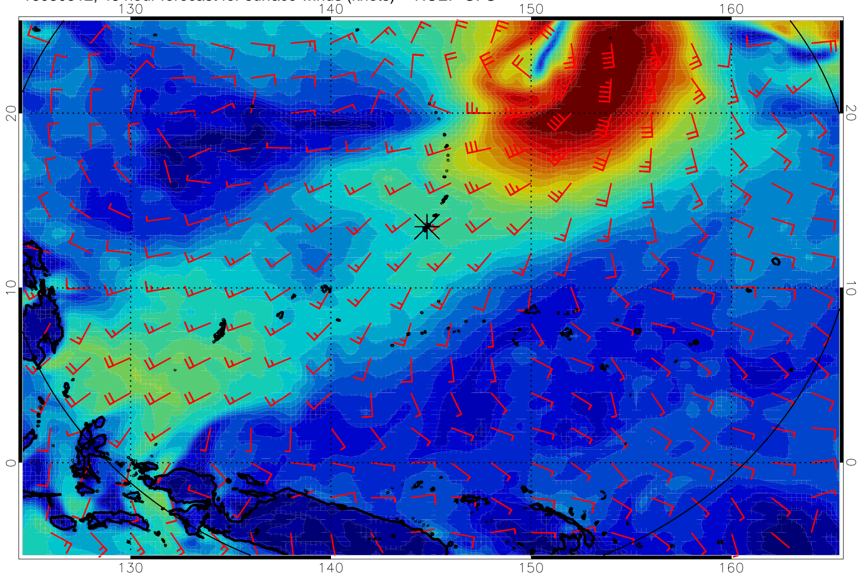
16080512, 48 hour forecast for surface winds (knots) -- NCEP GFS
