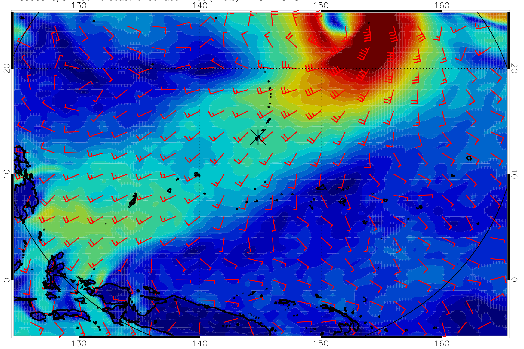
16080518, 54 hour forecast for surface winds (knots) -- NCEP GFS
