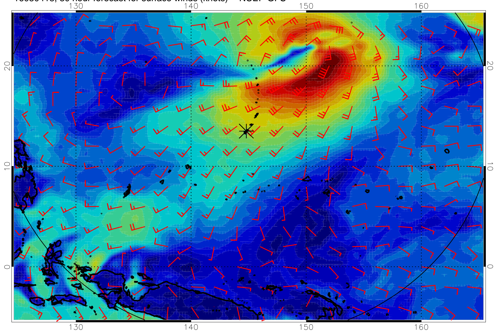
16080418, 30 hour forecast for surface winds (knots) -- NCEP GFS
