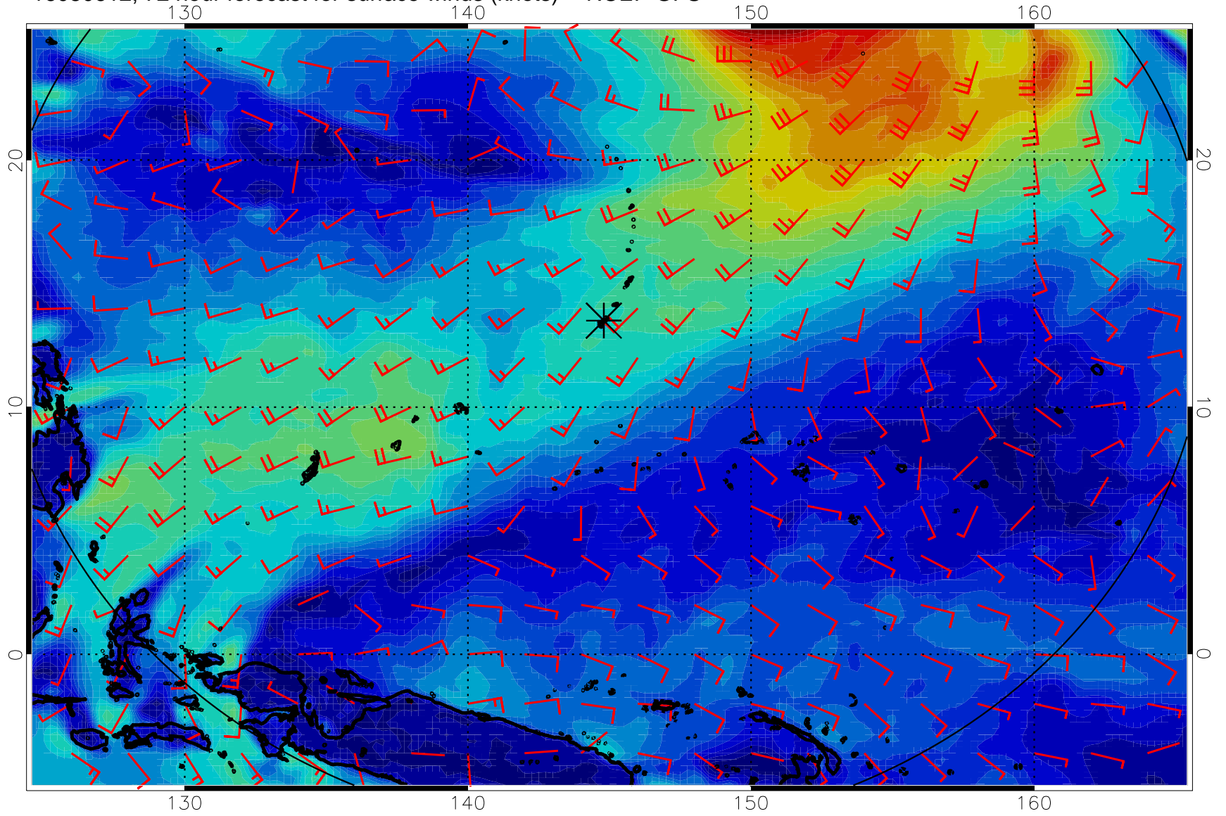
16080612, 72 hour forecast for surface winds (knots) -- NCEP GFS
