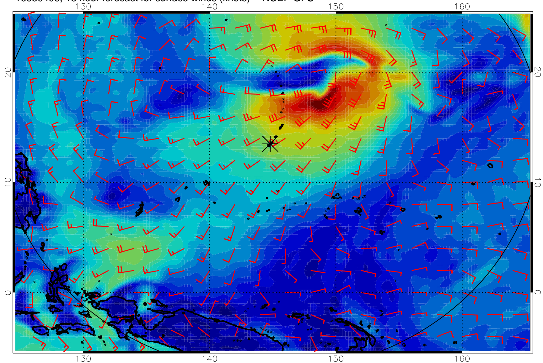
16080406, 18 hour forecast for surface winds (knots) -- NCEP GFS
