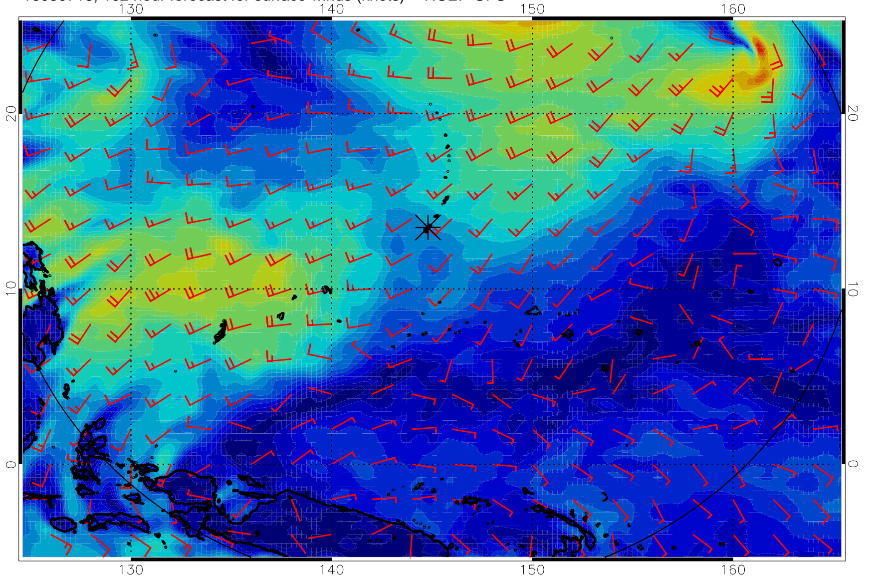
16080718, 102 hour forecast for surface winds (knots) -- NCEP GFS
