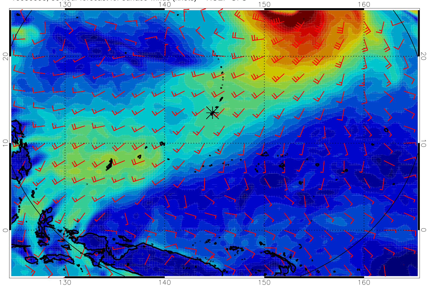
16080606, 66 hour forecast for surface winds (knots) -- NCEP GFS
