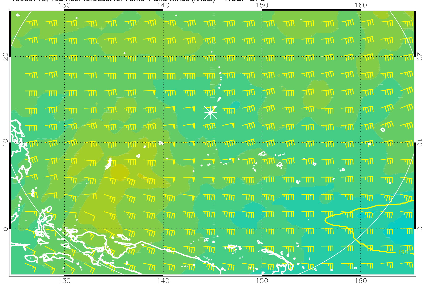
16080718, 102 hour forecast for 70mb T and winds (knots) -- NCEP GFS
