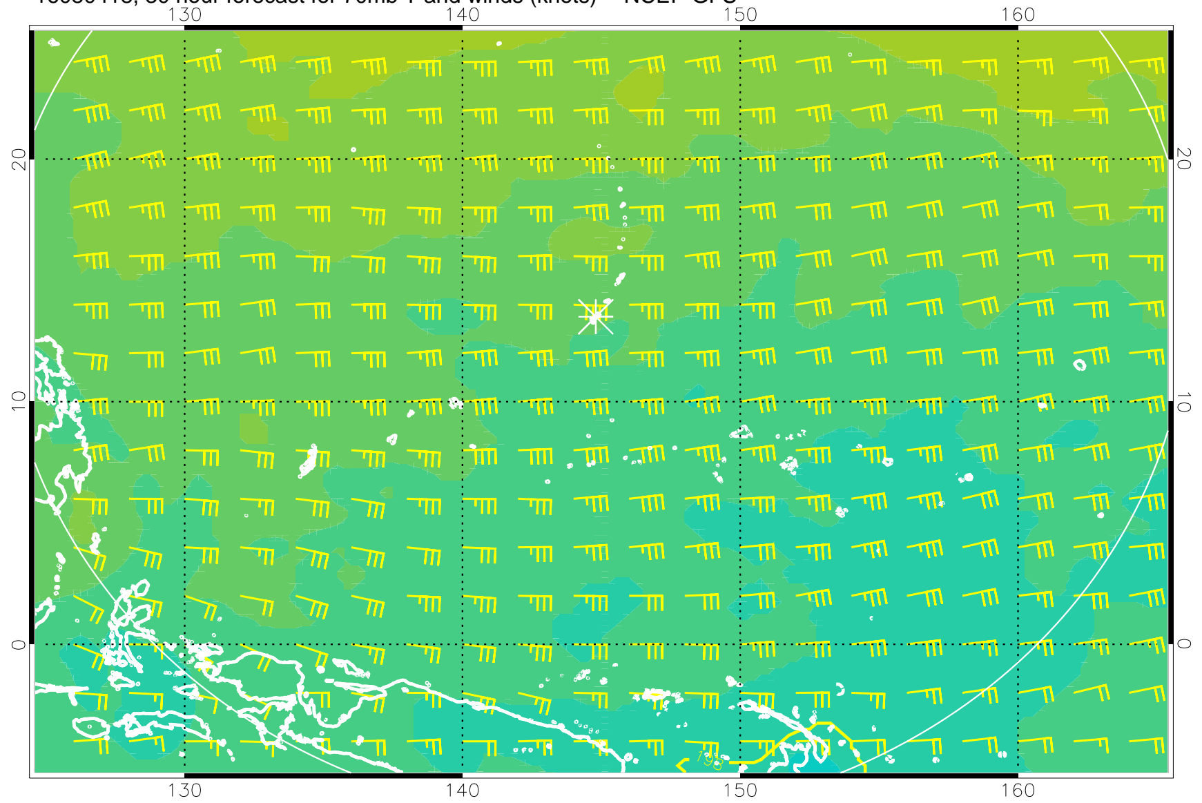
16080418, 30 hour forecast for 70mb T and winds (knots) -- NCEP GFS
