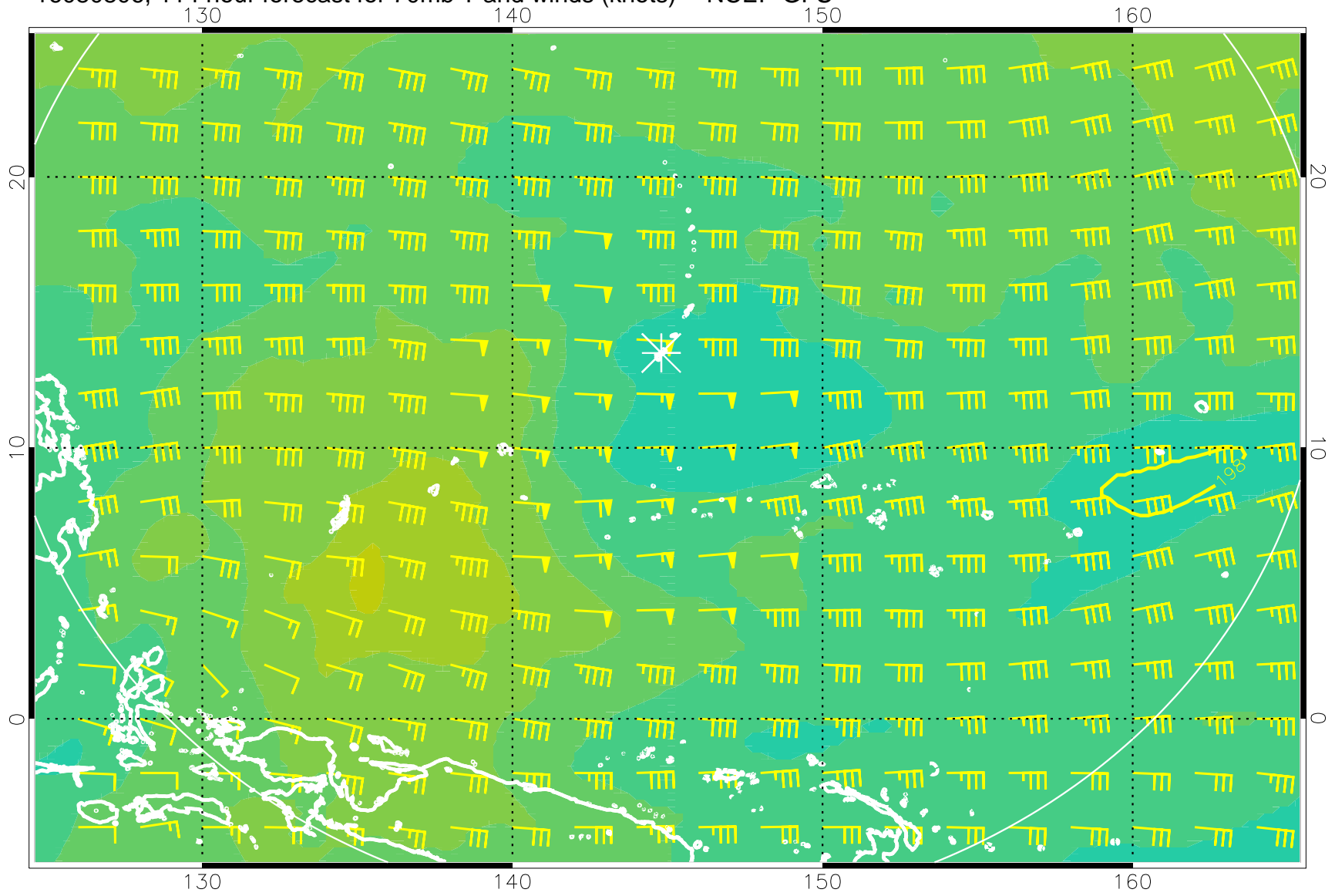
16080806, 114 hour forecast for 70mb T and winds (knots) -- NCEP GFS
