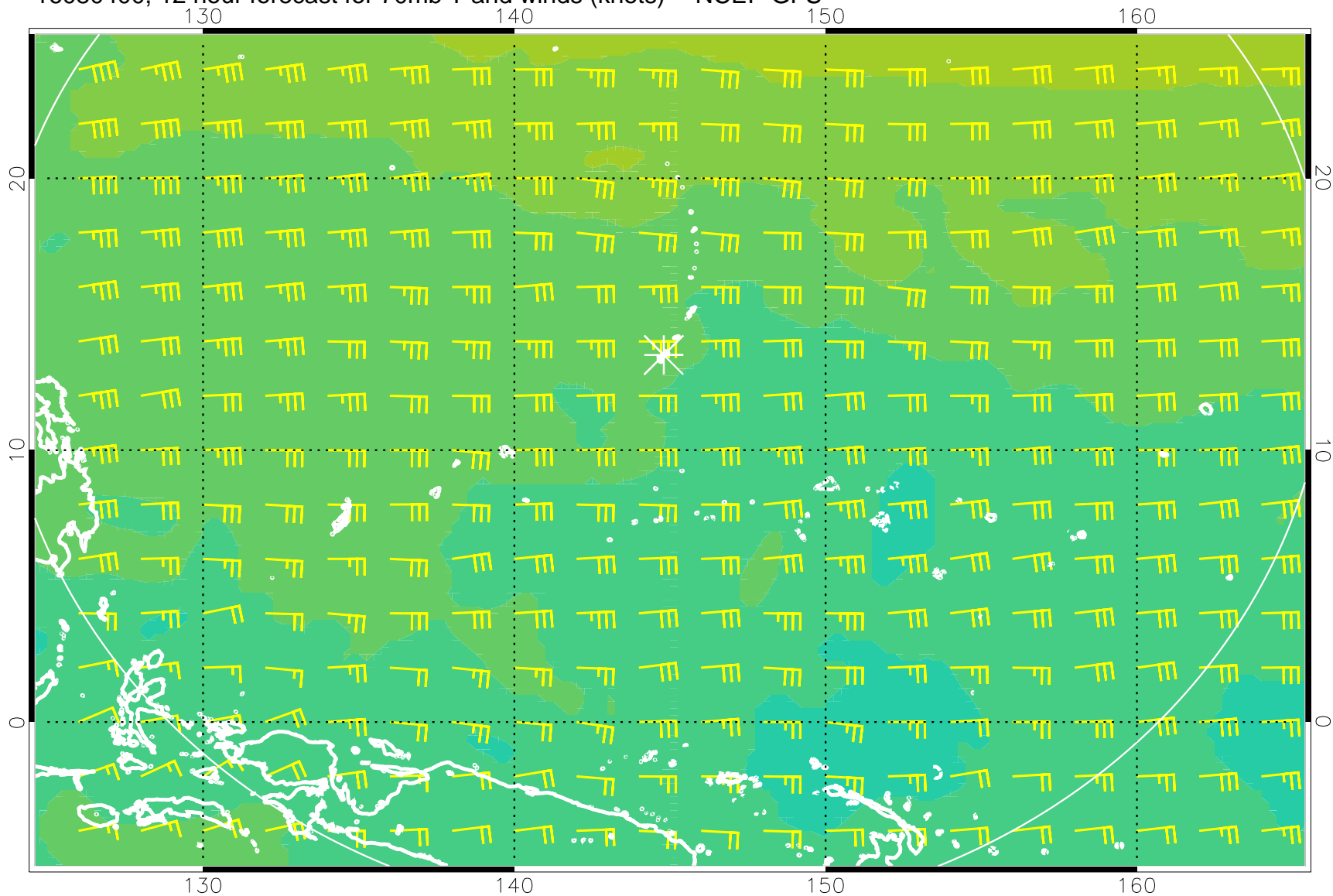
16080400, 12 hour forecast for 70mb T and winds (knots) -- NCEP GFS
