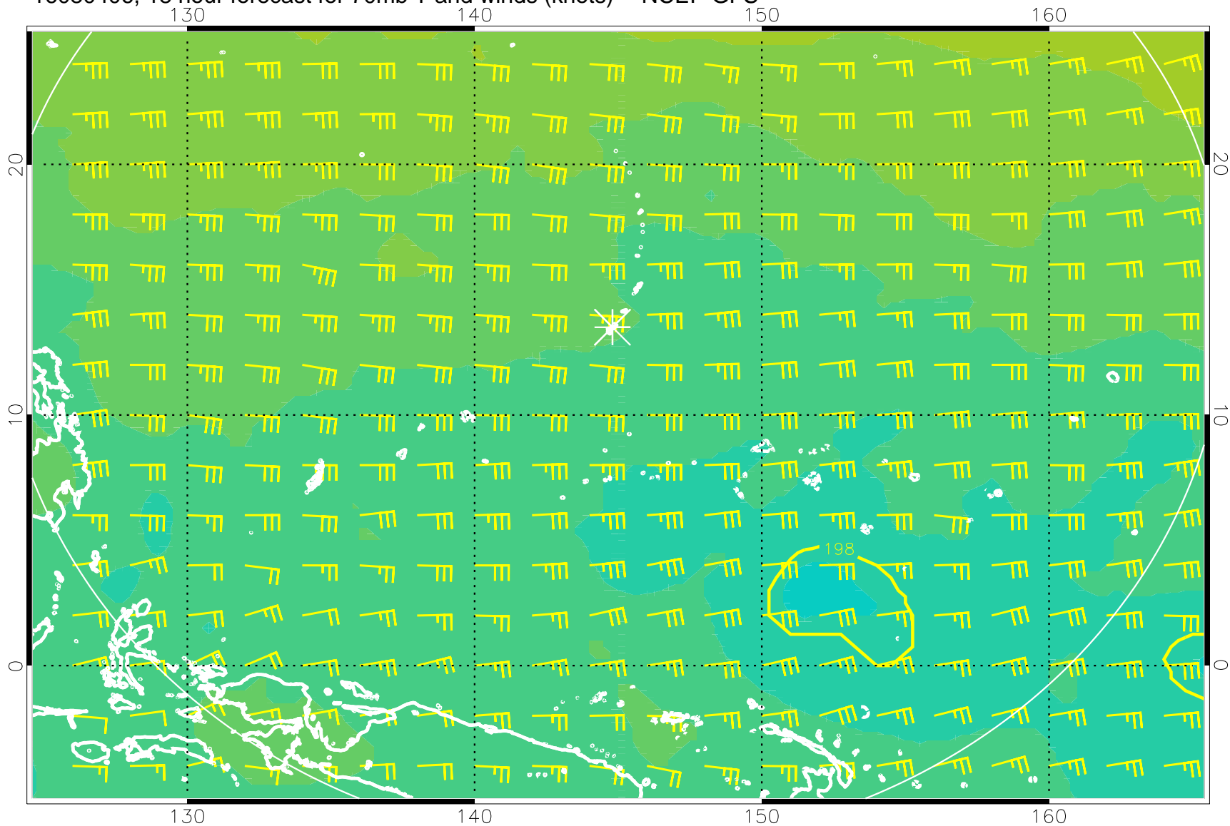
16080406, 18 hour forecast for 70mb T and winds (knots) -- NCEP GFS
