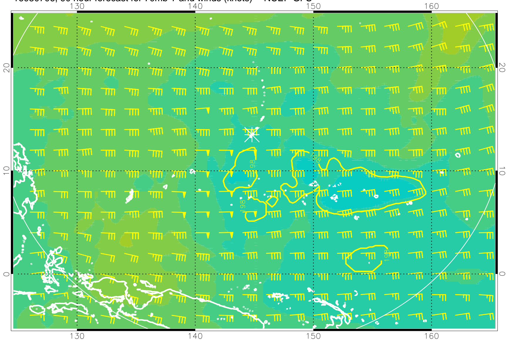
16080706, 90 hour forecast for 70mb T and winds (knots) -- NCEP GFS
