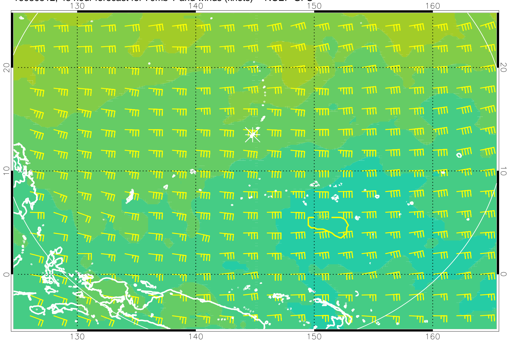
16080512, 48 hour forecast for 70mb T and winds (knots) -- NCEP GFS
