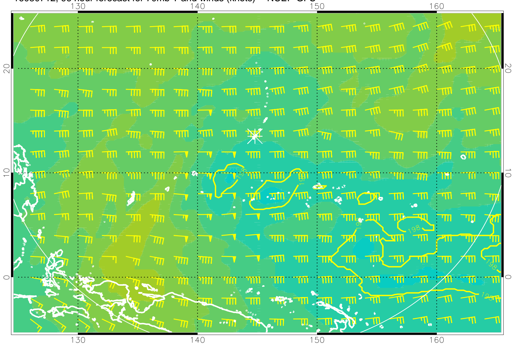
16080712, 96 hour forecast for 70mb T and winds (knots) -- NCEP GFS
