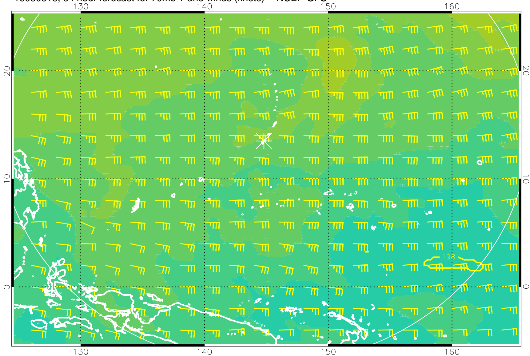
16080518, 54 hour forecast for 70mb T and winds (knots) -- NCEP GFS
