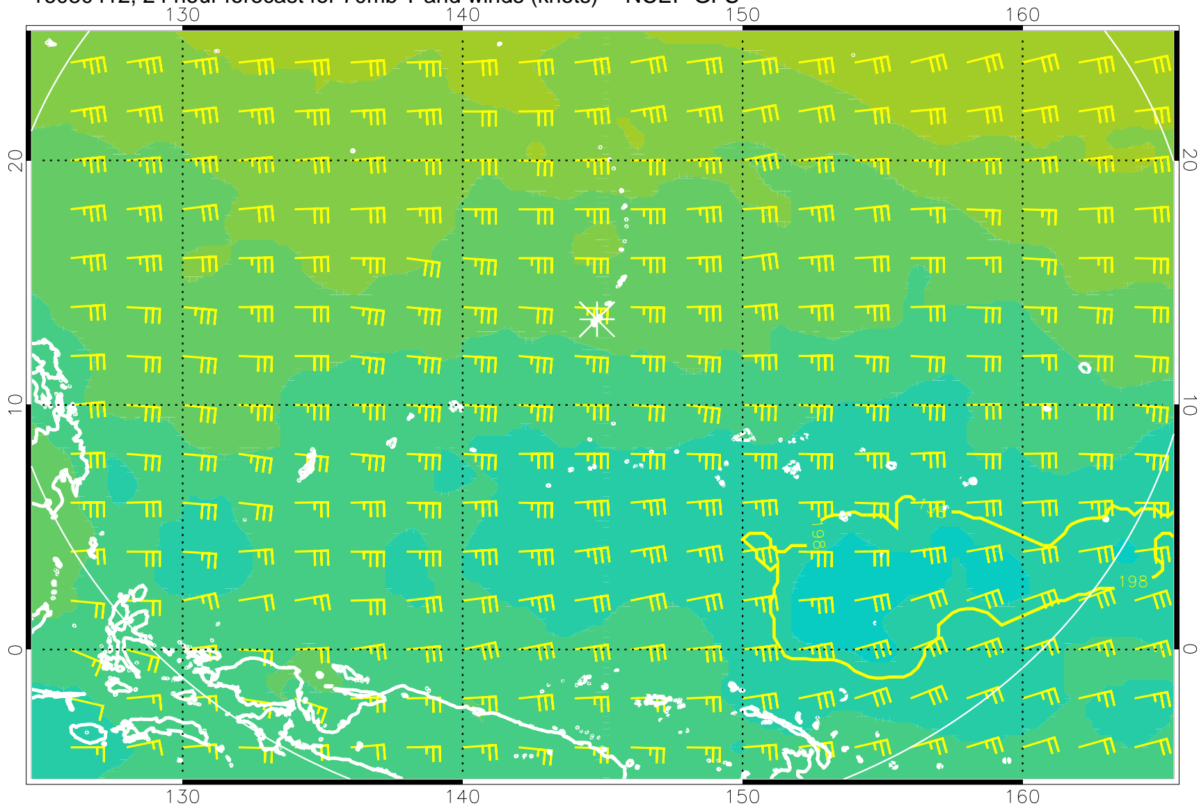
16080412, 24 hour forecast for 70mb T and winds (knots) -- NCEP GFS
