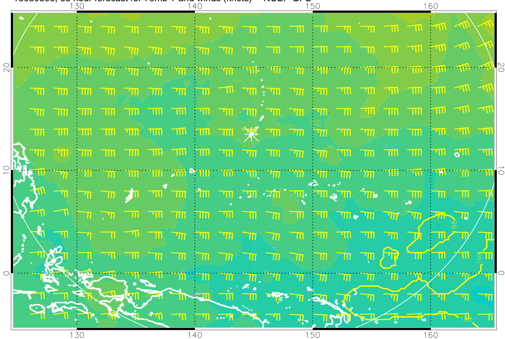
16080606, 66 hour forecast for 70mb T and winds (knots) -- NCEP GFS
