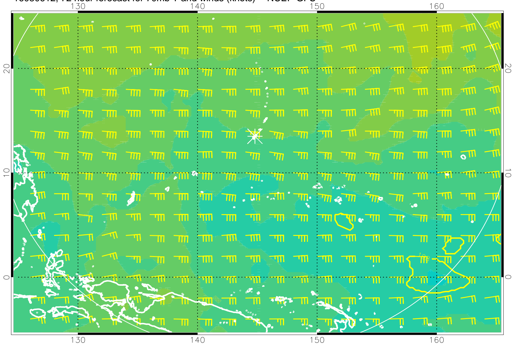
16080612, 72 hour forecast for 70mb T and winds (knots) -- NCEP GFS
