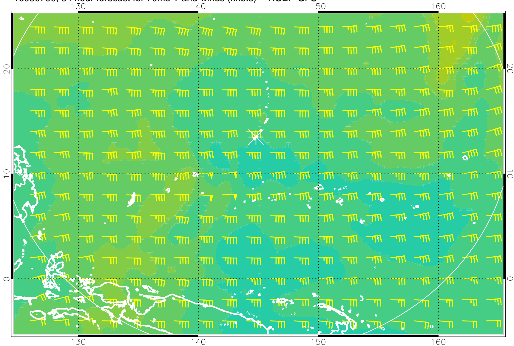
16080700, 84 hour forecast for 70mb T and winds (knots) -- NCEP GFS
