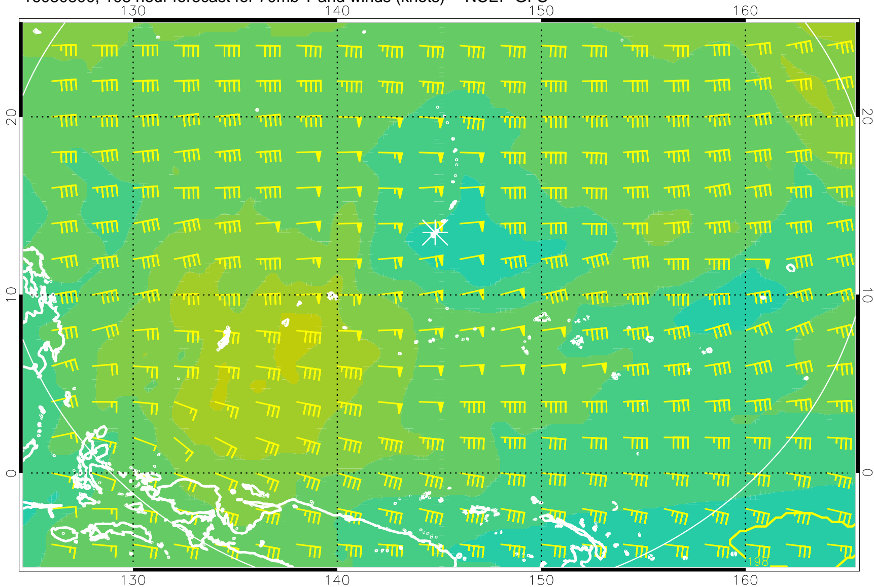
16080800, 108 hour forecast for 70mb T and winds (knots) -- NCEP GFS
