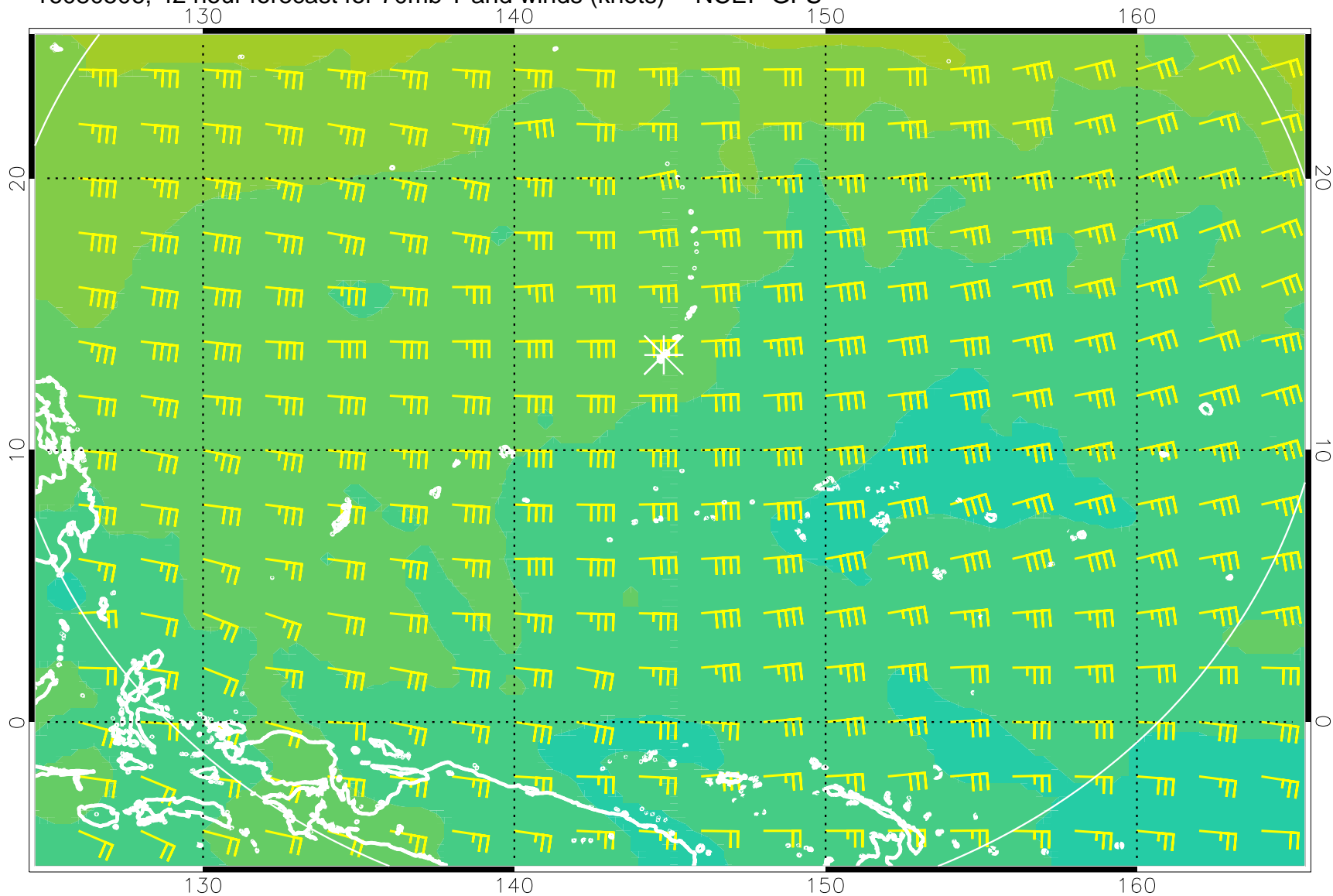
16080506, 42 hour forecast for 70mb T and winds (knots) -- NCEP GFS
