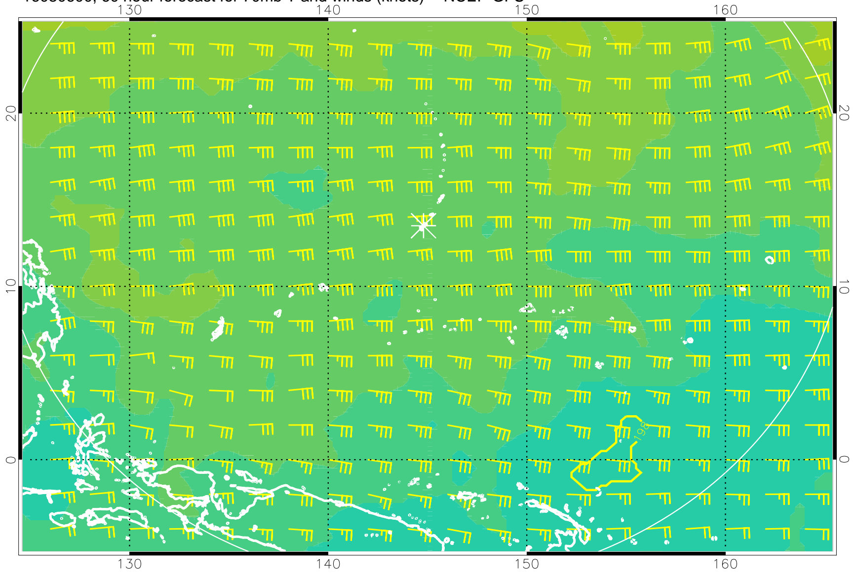
16080600, 60 hour forecast for 70mb T and winds (knots) -- NCEP GFS
