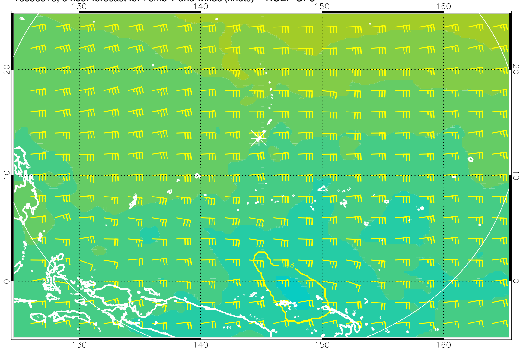
16080318, 6 hour forecast for 70mb T and winds (knots) -- NCEP GFS
