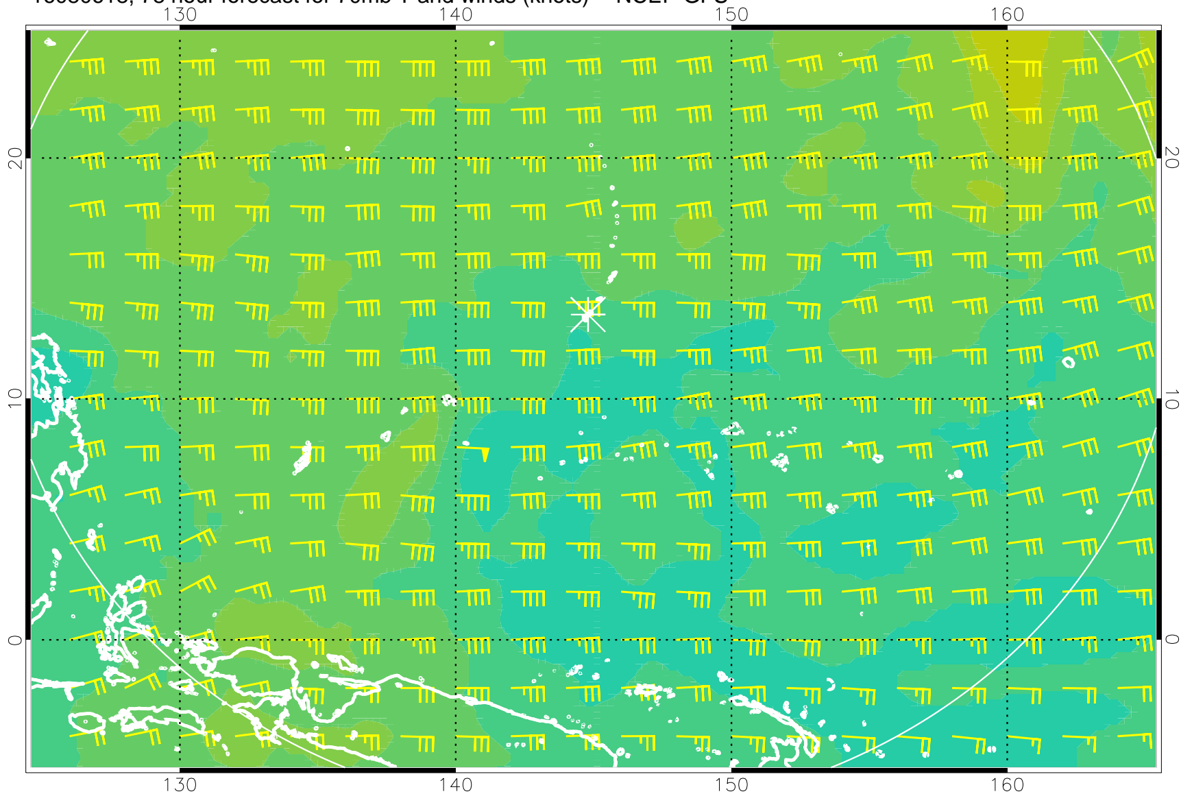
16080618, 78 hour forecast for 70mb T and winds (knots) -- NCEP GFS
