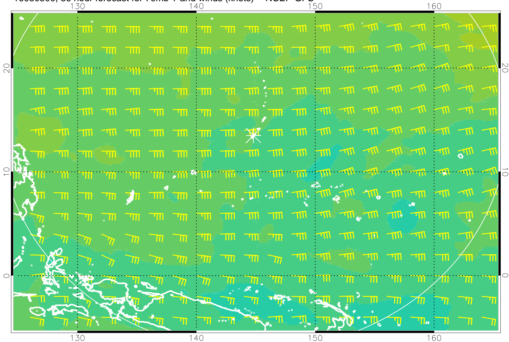
16080500, 36 hour forecast for 70mb T and winds (knots) -- NCEP GFS
