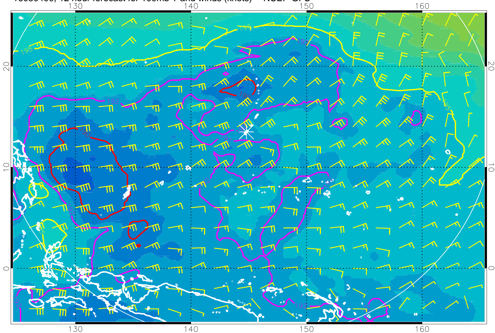
16080400, 12 hour forecast for 100mb T and winds (knots) -- NCEP GFS
