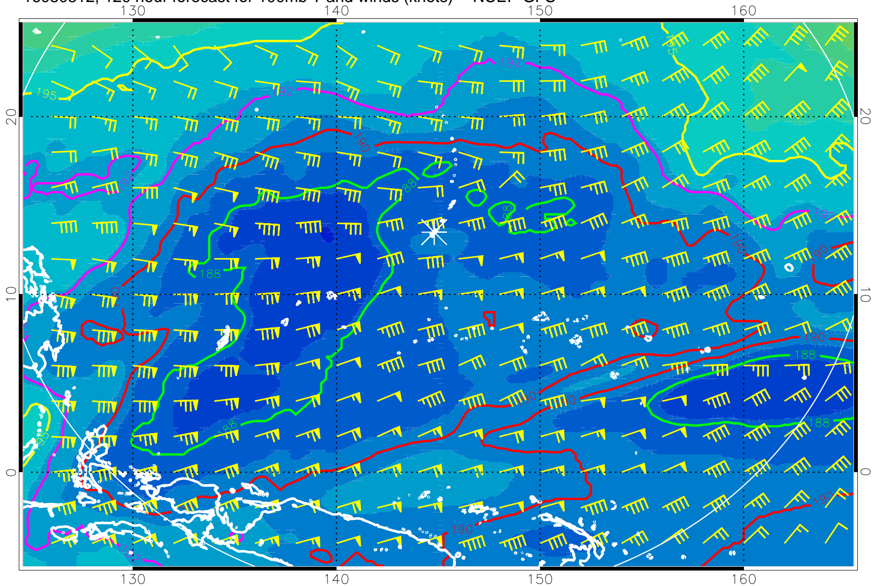
16080812, 120 hour forecast for 100mb T and winds (knots) -- NCEP GFS
