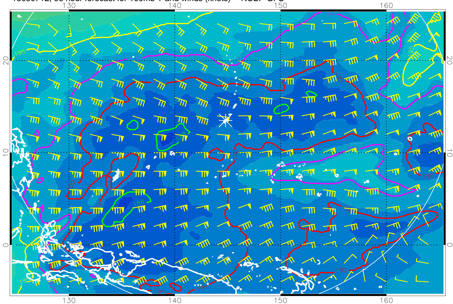
16080712, 96 hour forecast for 100mb T and winds (knots) -- NCEP GFS
