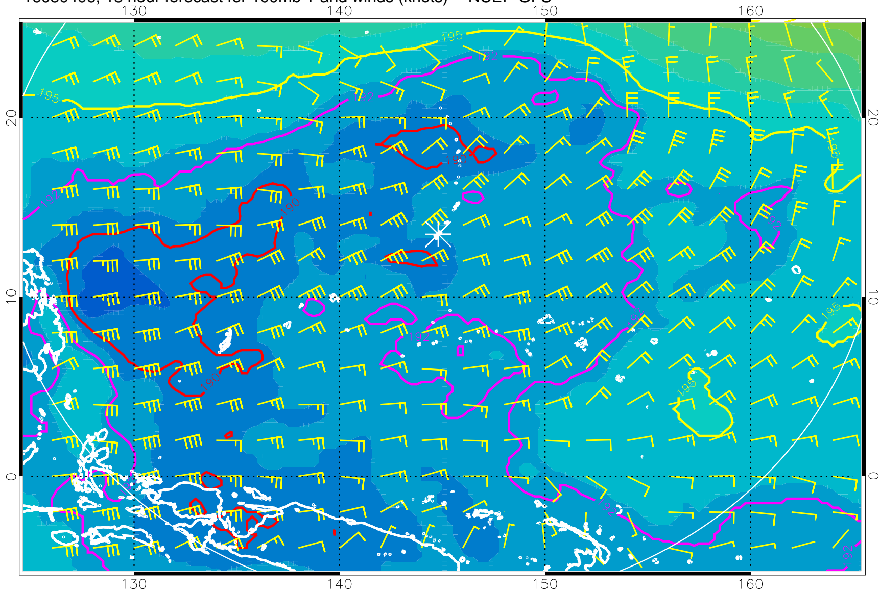
16080406, 18 hour forecast for 100mb T and winds (knots) -- NCEP GFS
