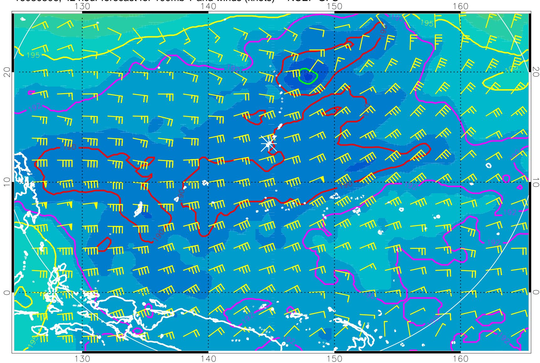
16080506, 42 hour forecast for 100mb T and winds (knots) -- NCEP GFS
