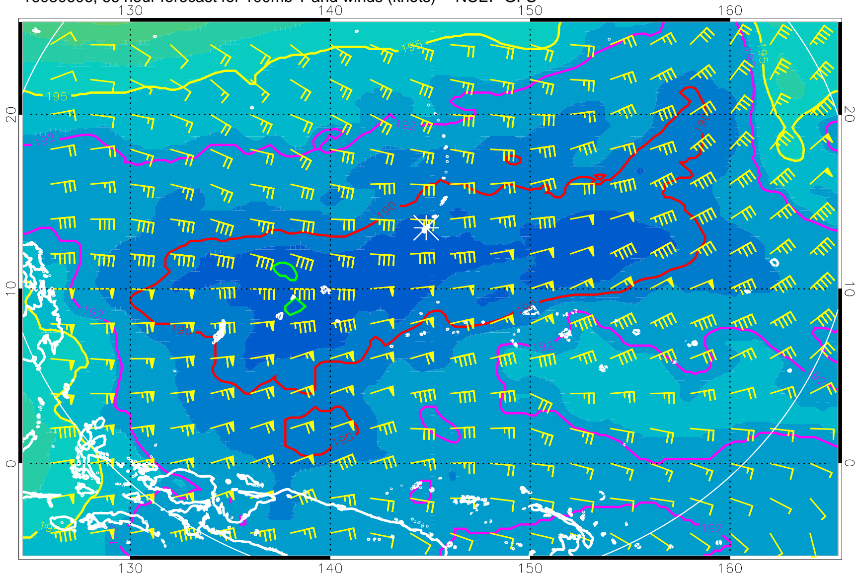
16080606, 66 hour forecast for 100mb T and winds (knots) -- NCEP GFS
