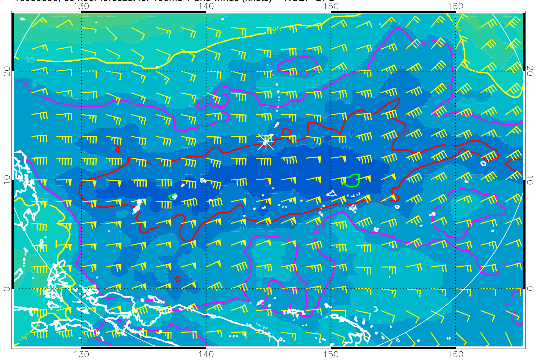
16080600, 60 hour forecast for 100mb T and winds (knots) -- NCEP GFS
