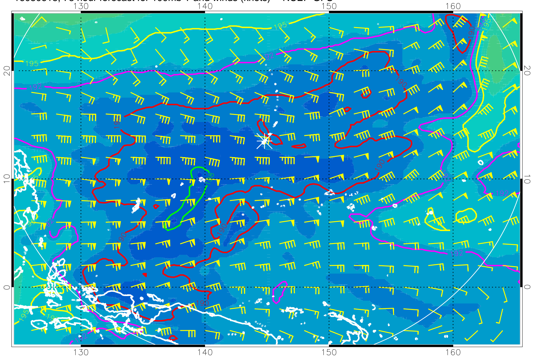
16080618, 78 hour forecast for 100mb T and winds (knots) -- NCEP GFS
