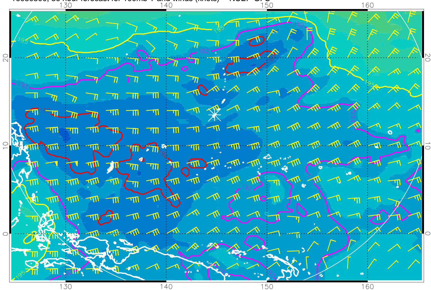
16080500, 36 hour forecast for 100mb T and winds (knots) -- NCEP GFS
