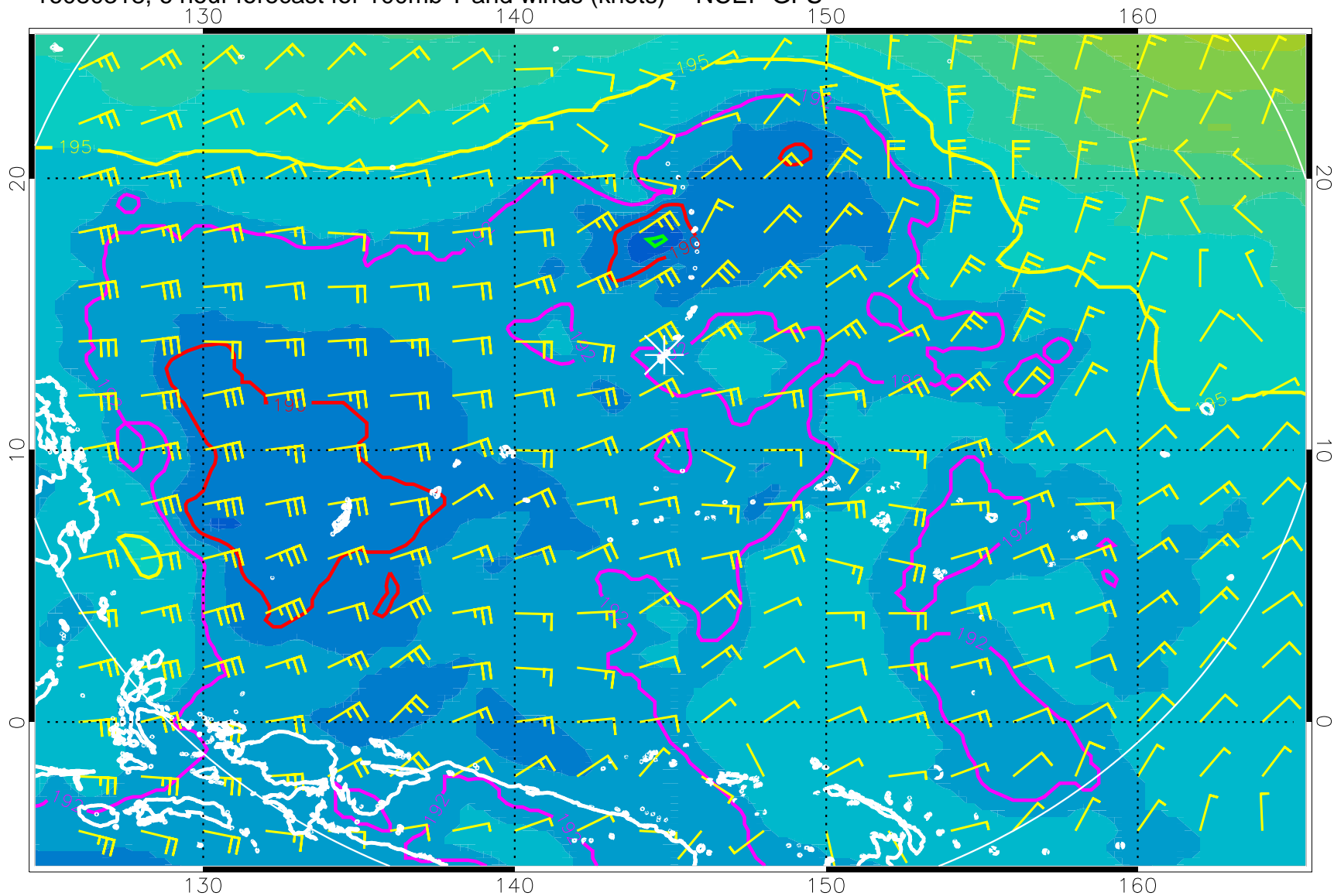
16080318, 6 hour forecast for 100mb T and winds (knots) -- NCEP GFS
