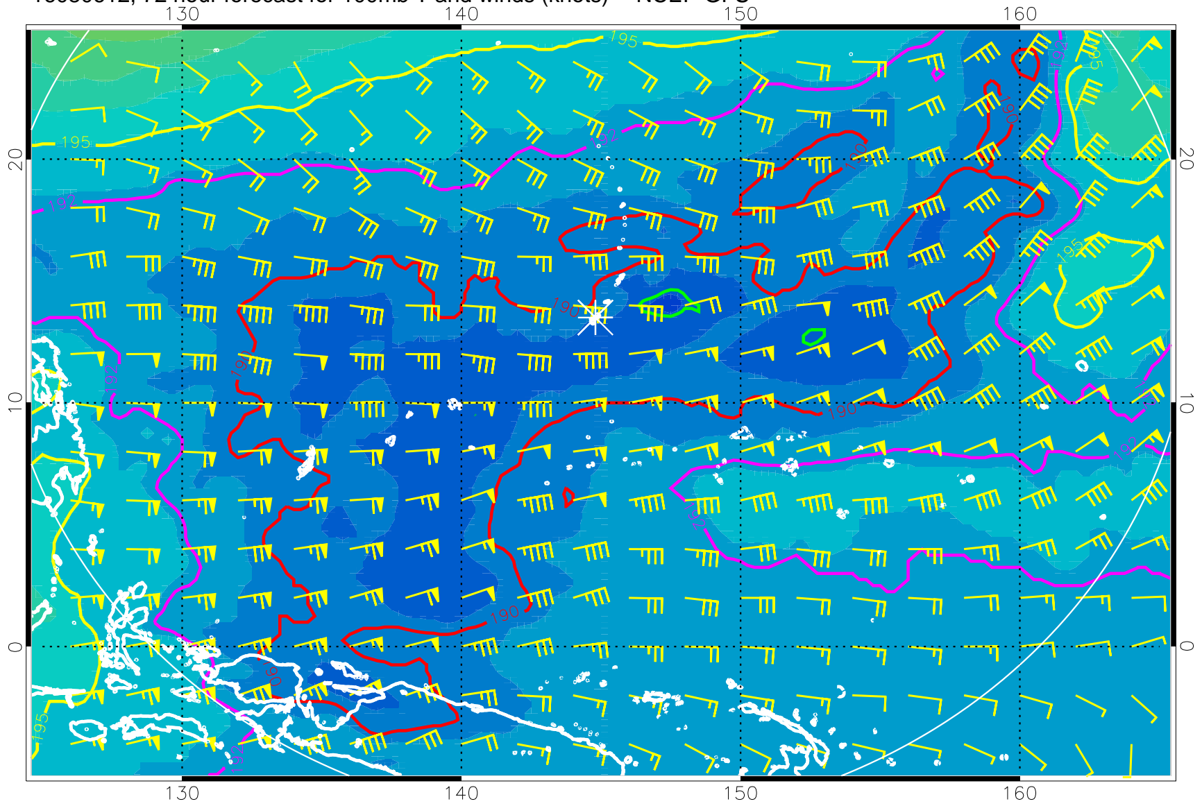
16080612, 72 hour forecast for 100mb T and winds (knots) -- NCEP GFS
