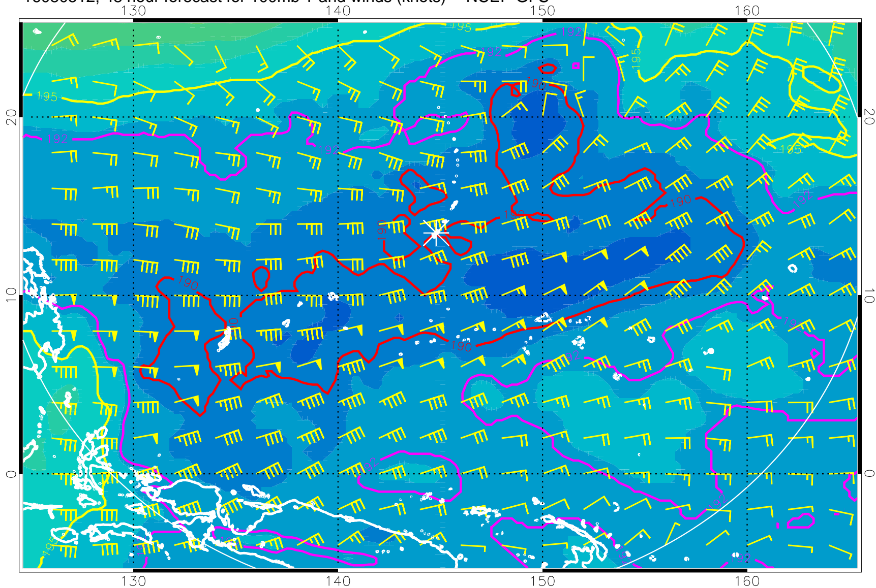
16080512, 48 hour forecast for 100mb T and winds (knots) -- NCEP GFS
