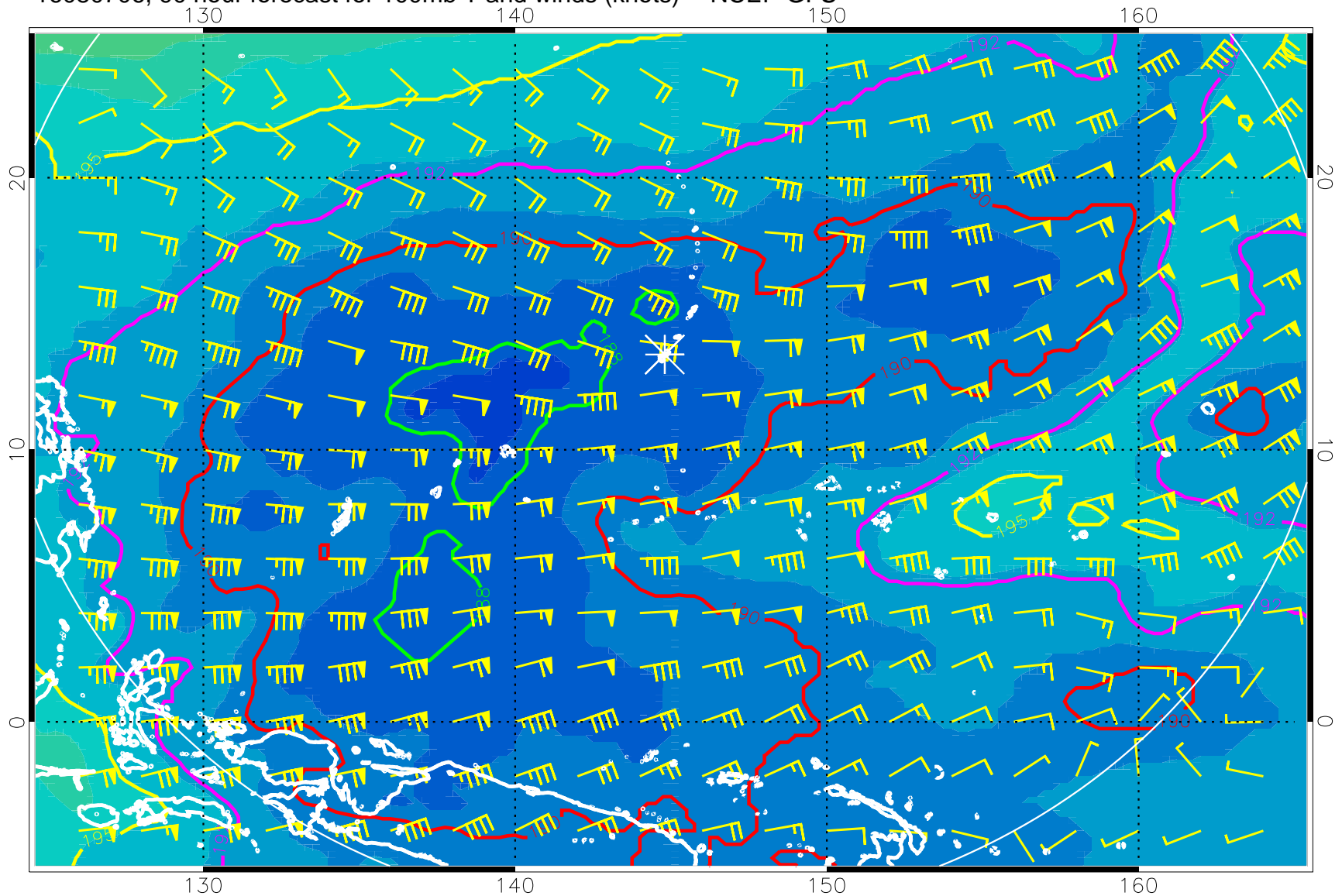
16080706, 90 hour forecast for 100mb T and winds (knots) -- NCEP GFS
