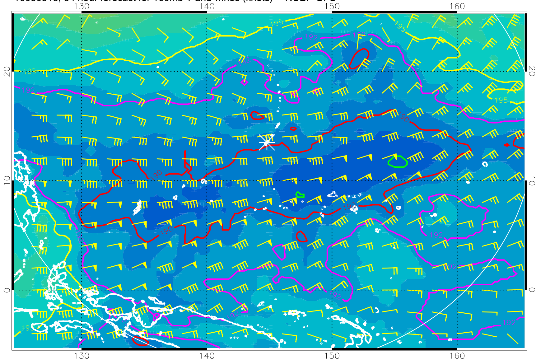
16080518, 54 hour forecast for 100mb T and winds (knots) -- NCEP GFS
