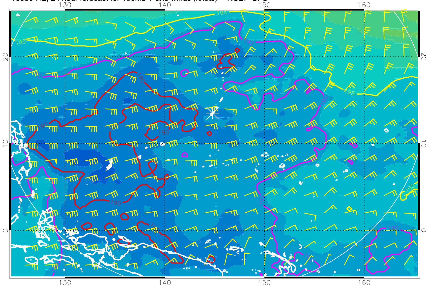
16080412, 24 hour forecast for 100mb T and winds (knots) -- NCEP GFS
