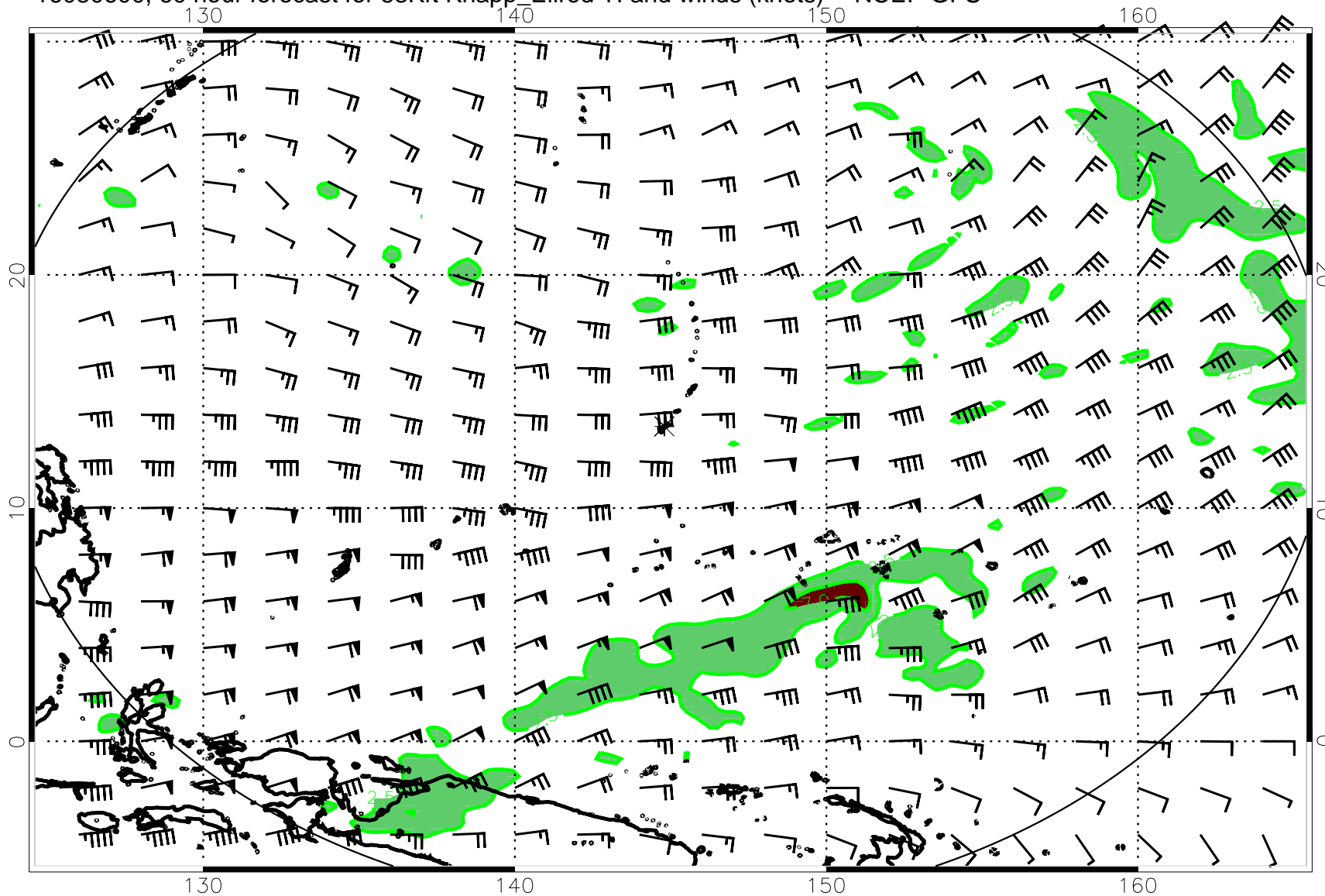
16080600, 60 hour forecast for 53Kft Knapp_Ellrod TI and winds (knots) -- NCEP GFS
