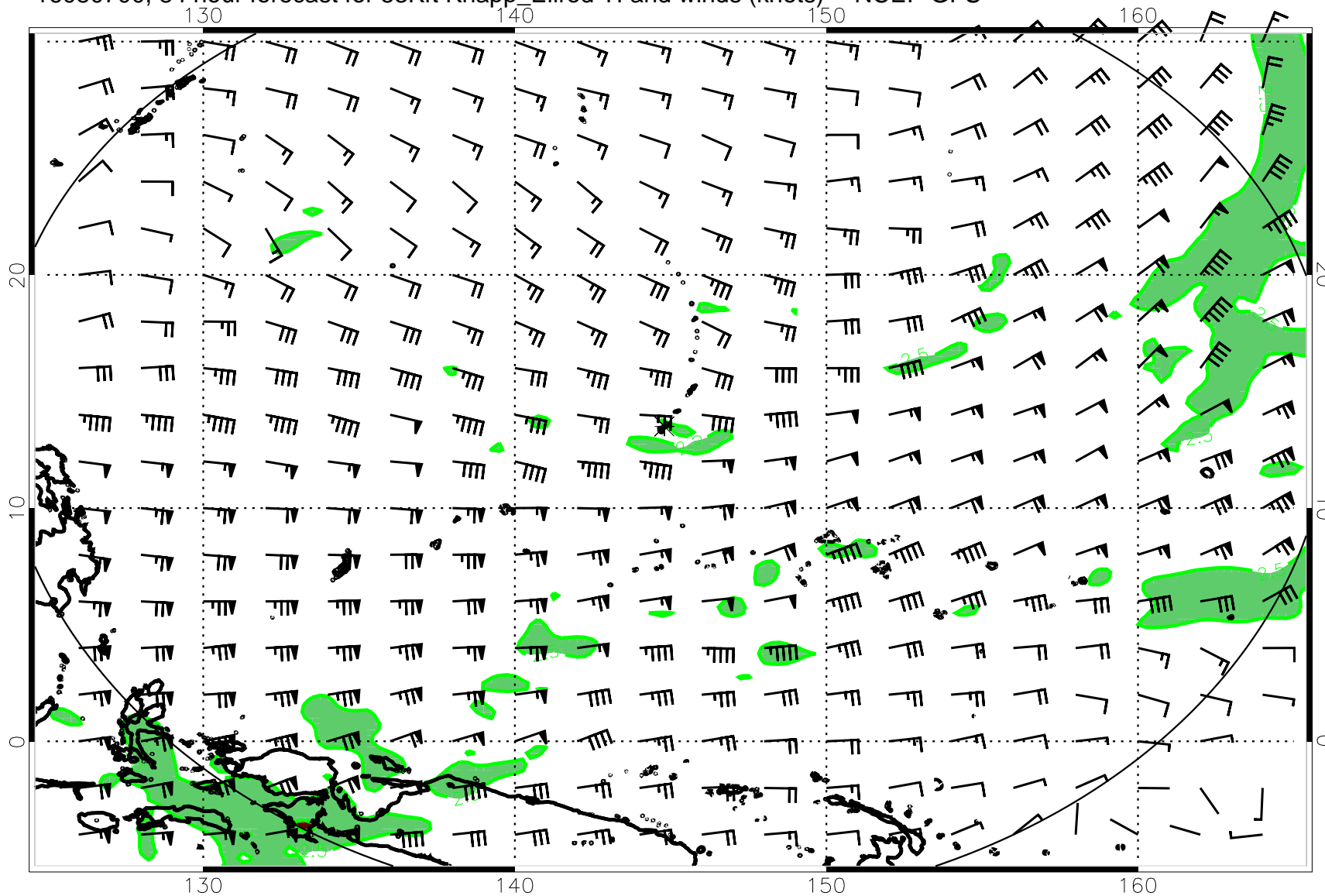
16080700, 84 hour forecast for 53Kft Knapp_Ellrod TI and winds (knots) -- NCEP GFS
