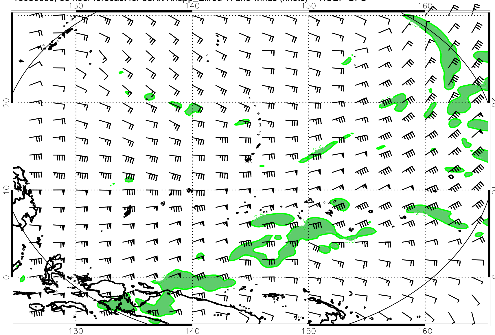
16080606, 66 hour forecast for 53Kft Knapp_Ellrod TI and winds (knots) -- NCEP GFS
