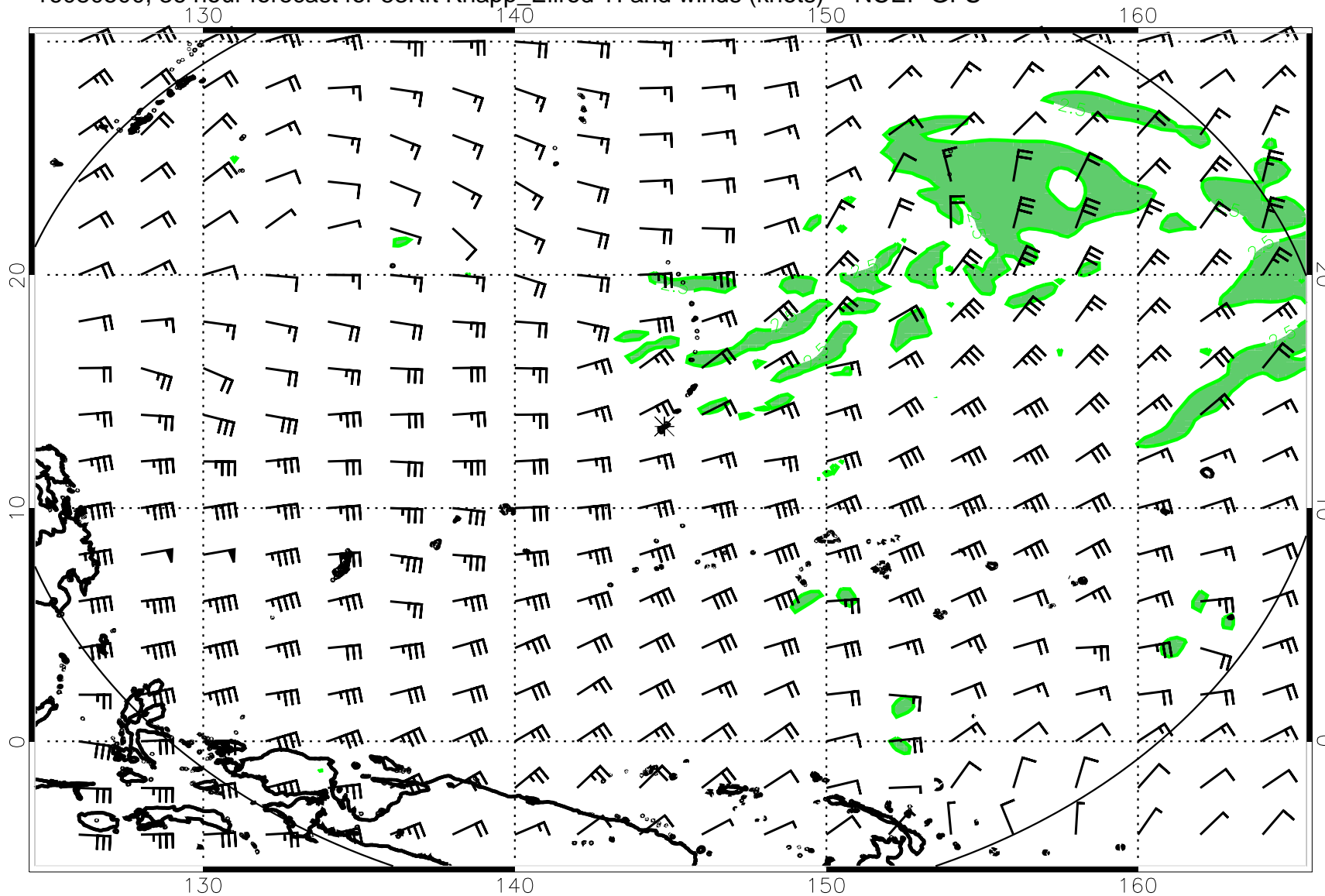
16080500, 36 hour forecast for 53Kft Knapp_Ellrod TI and winds (knots) -- NCEP GFS
