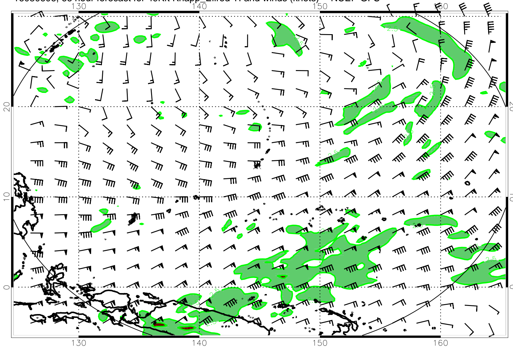
16080606, 66 hour forecast for 49Kft Knapp_Ellrod TI and winds (knots) -- NCEP GFS
