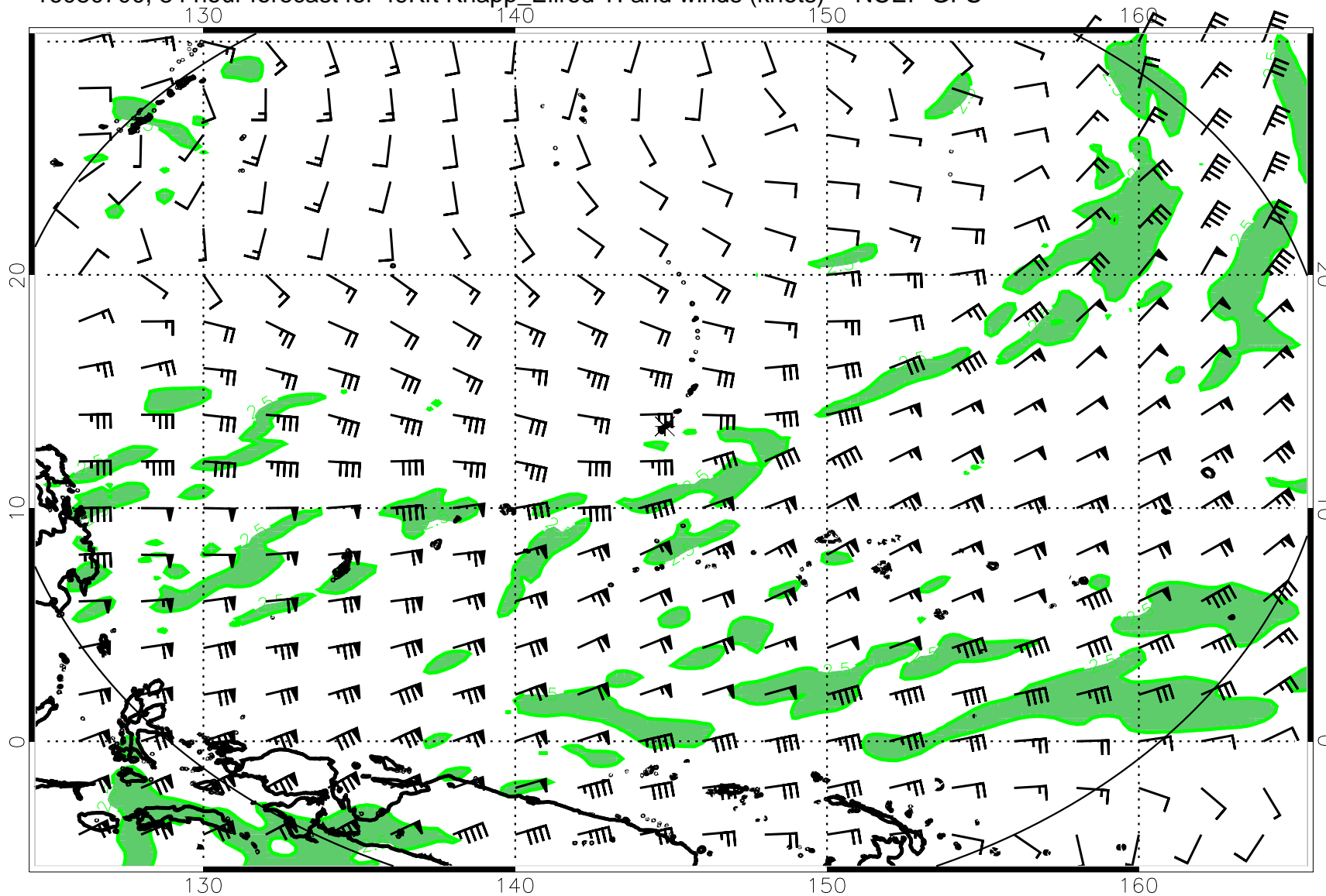
16080700, 84 hour forecast for 49Kft Knapp_Ellrod TI and winds (knots) -- NCEP GFS
