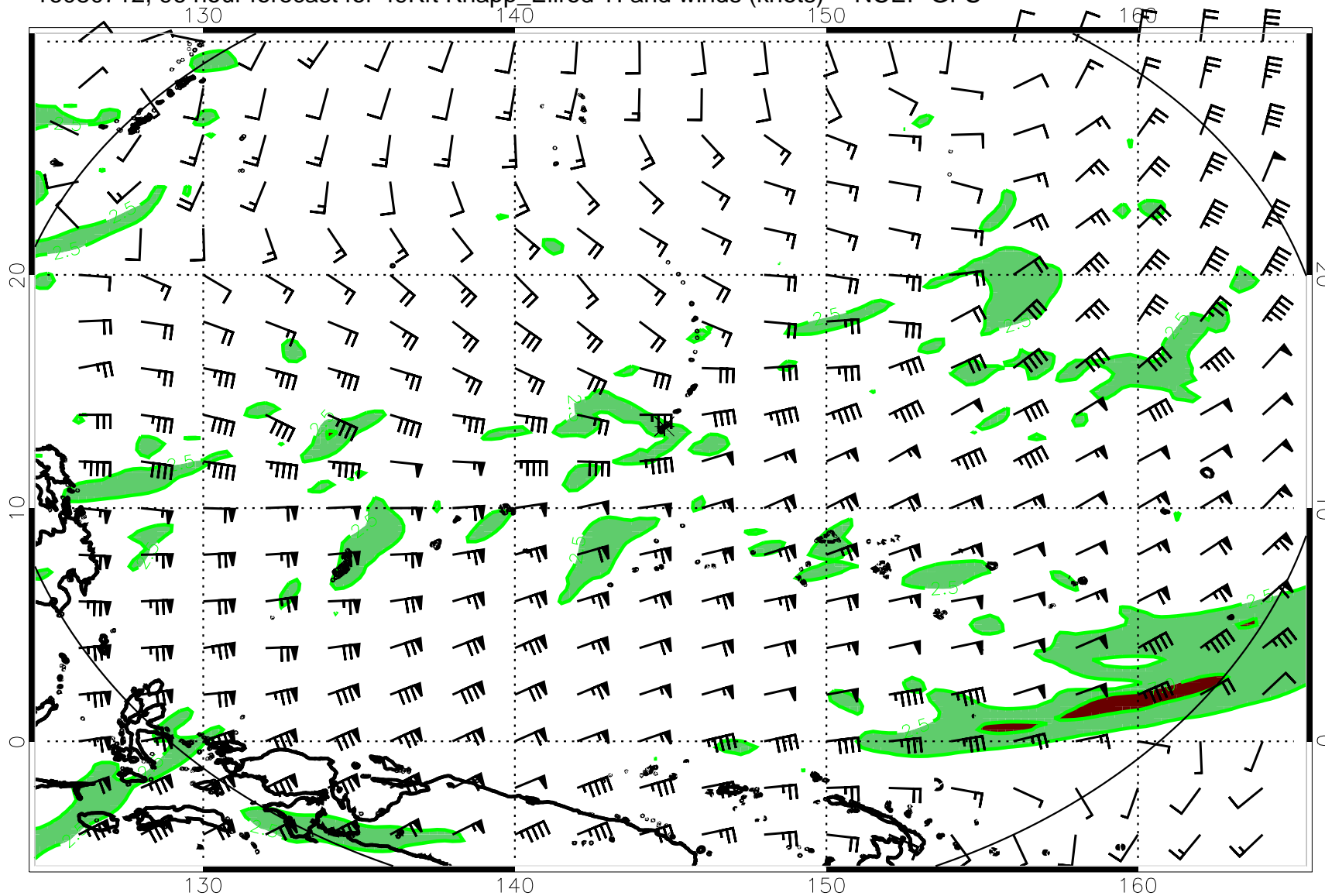
16080712, 96 hour forecast for 49Kft Knapp_Ellrod TI and winds (knots) -- NCEP GFS
