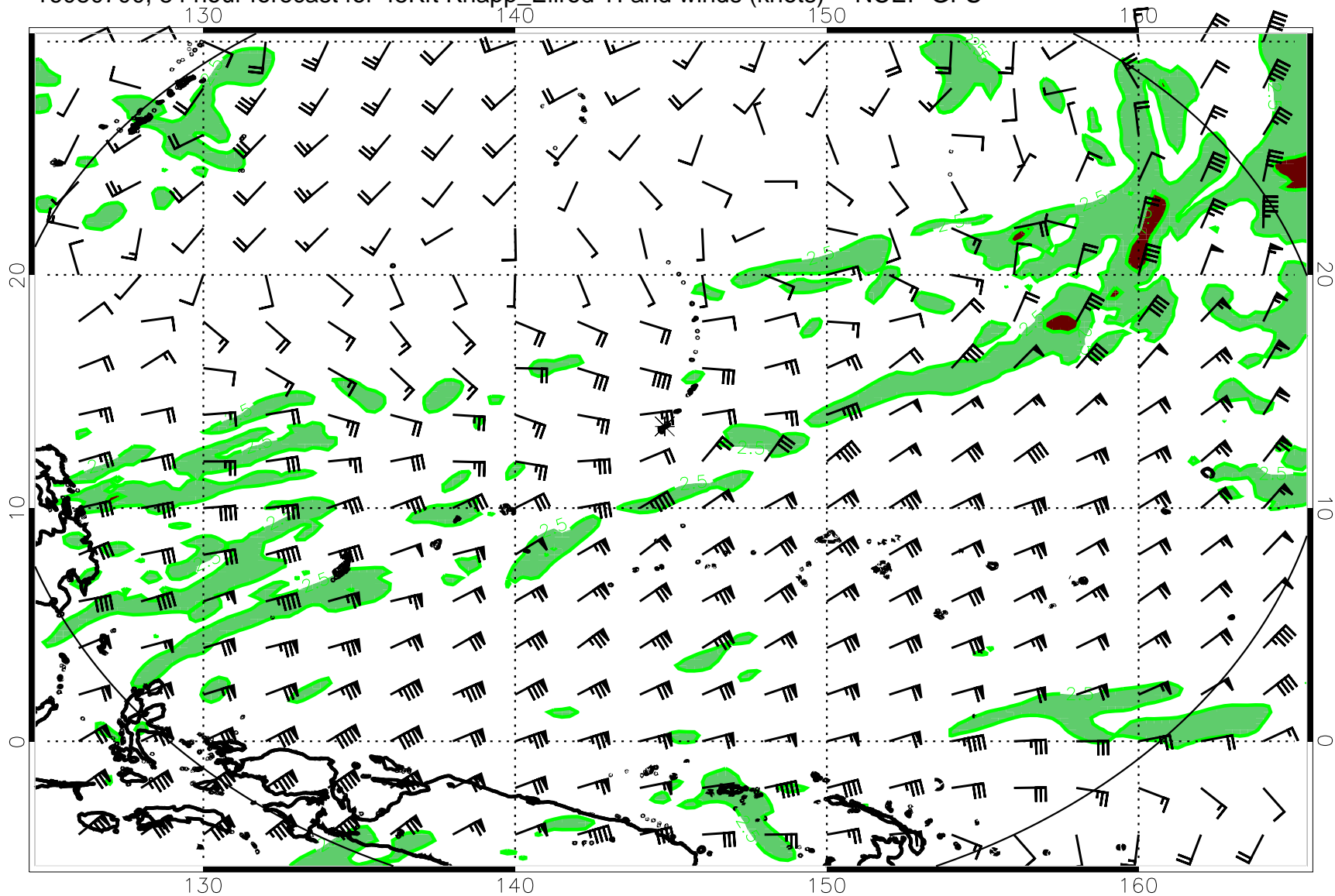
16080700, 84 hour forecast for 45Kft Knapp_Ellrod TI and winds (knots) -- NCEP GFS
