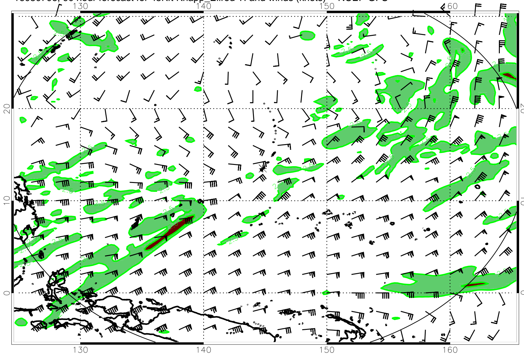
16080706, 90 hour forecast for 45Kft Knapp_Ellrod TI and winds (knots) -- NCEP GFS
