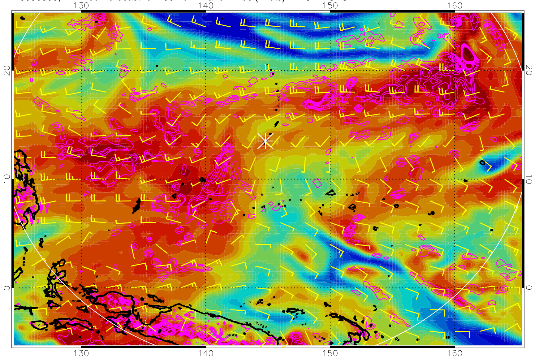
16080806, 114 hour forecast for 700mb RH and winds (knots) -- NCEP GFS
