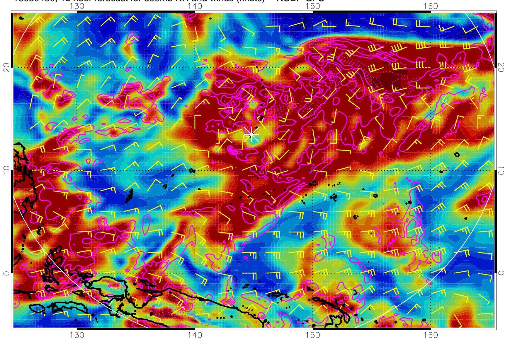
16080400, 12 hour forecast for 300mb RH and winds (knots) -- NCEP GFS
