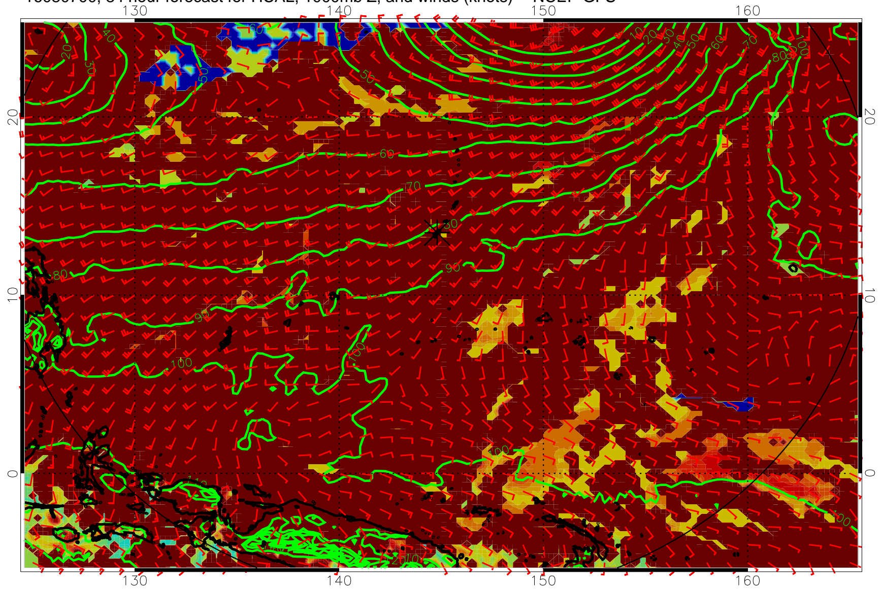
16080700, 84 hour forecast for HCAL, 1000mb Z, and winds (knots) -- NCEP GFS
