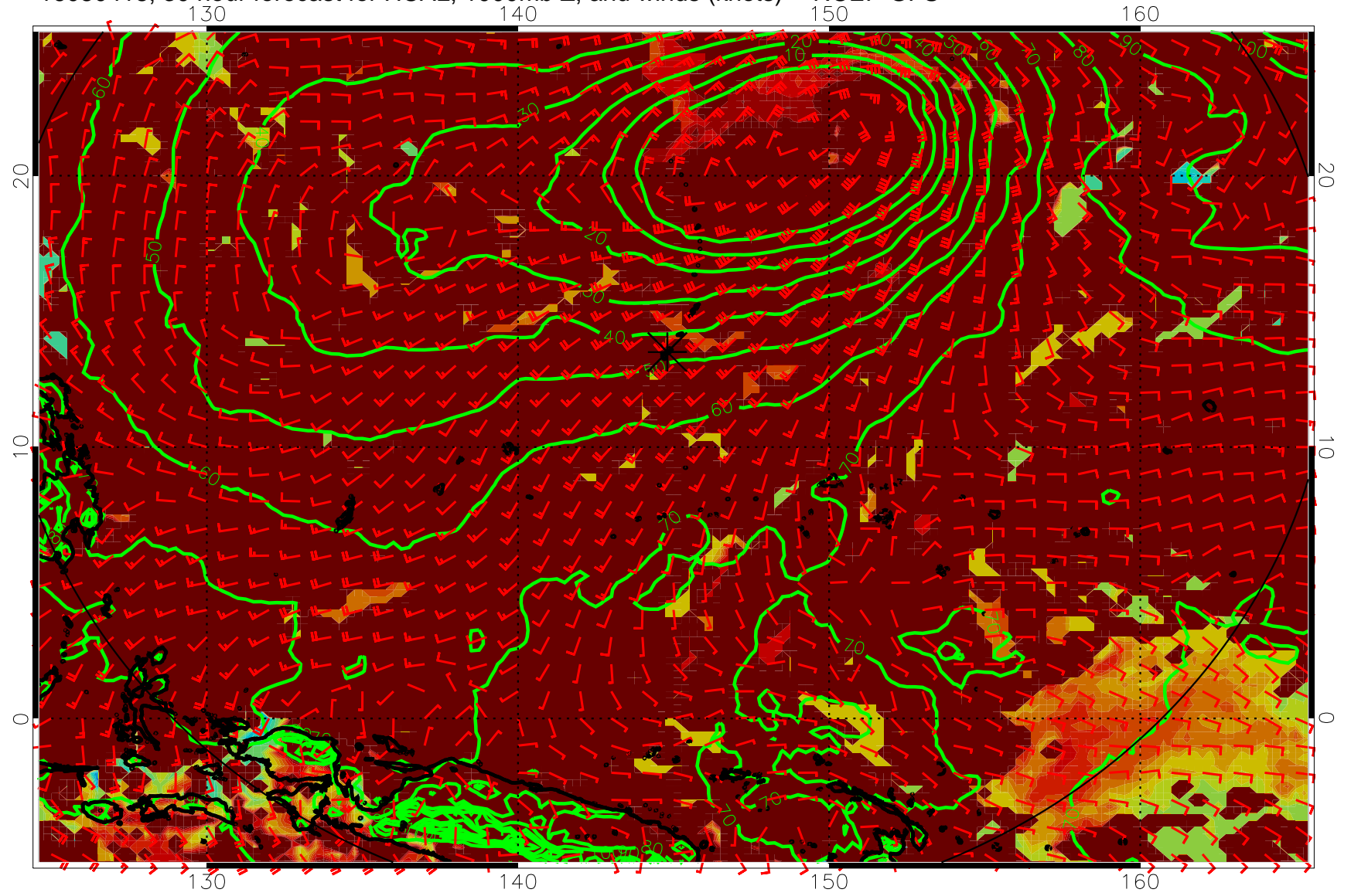
16080418, 30 hour forecast for HCAL, 1000mb Z, and winds (knots) -- NCEP GFS
