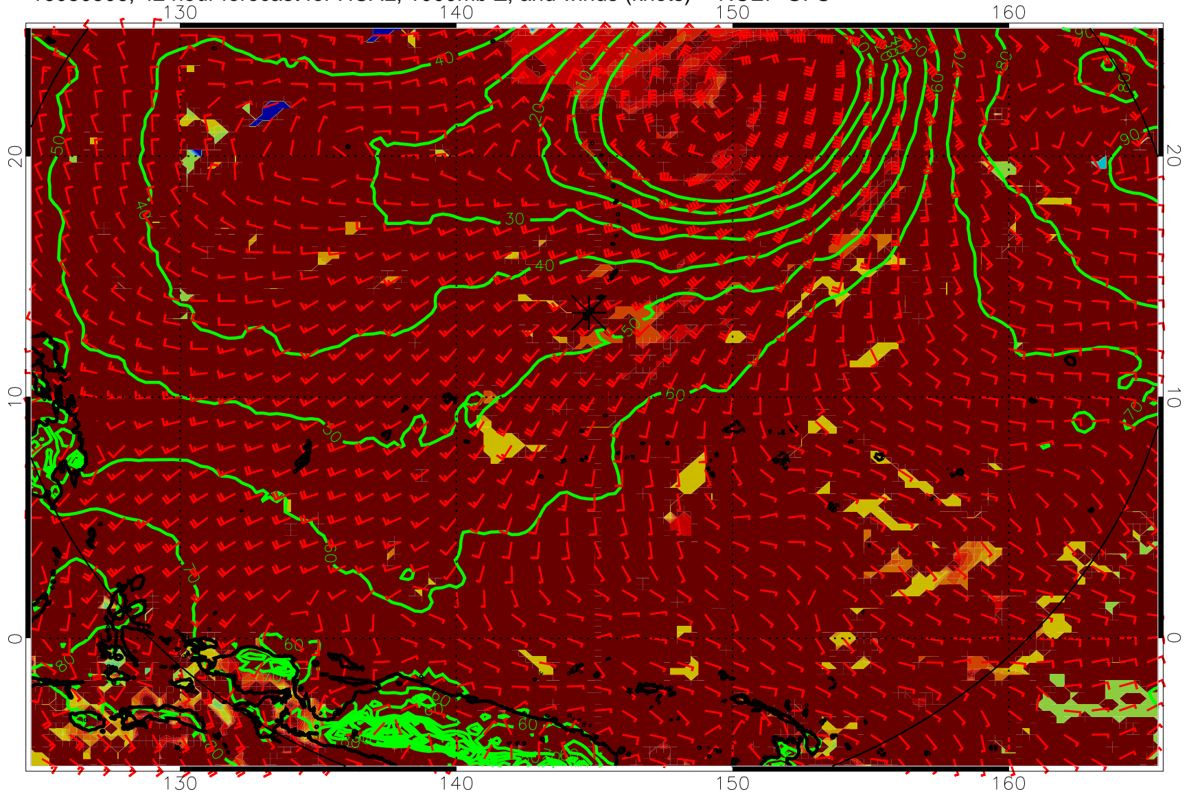
16080506, 42 hour forecast for HCAL, 1000mb Z, and winds (knots) -- NCEP GFS
