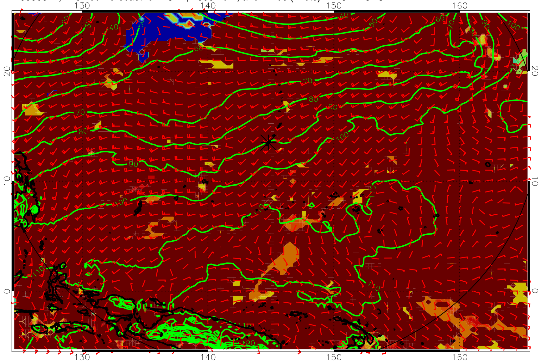
16080812, 120 hour forecast for HCAL, 1000mb Z, and winds (knots) -- NCEP GFS
