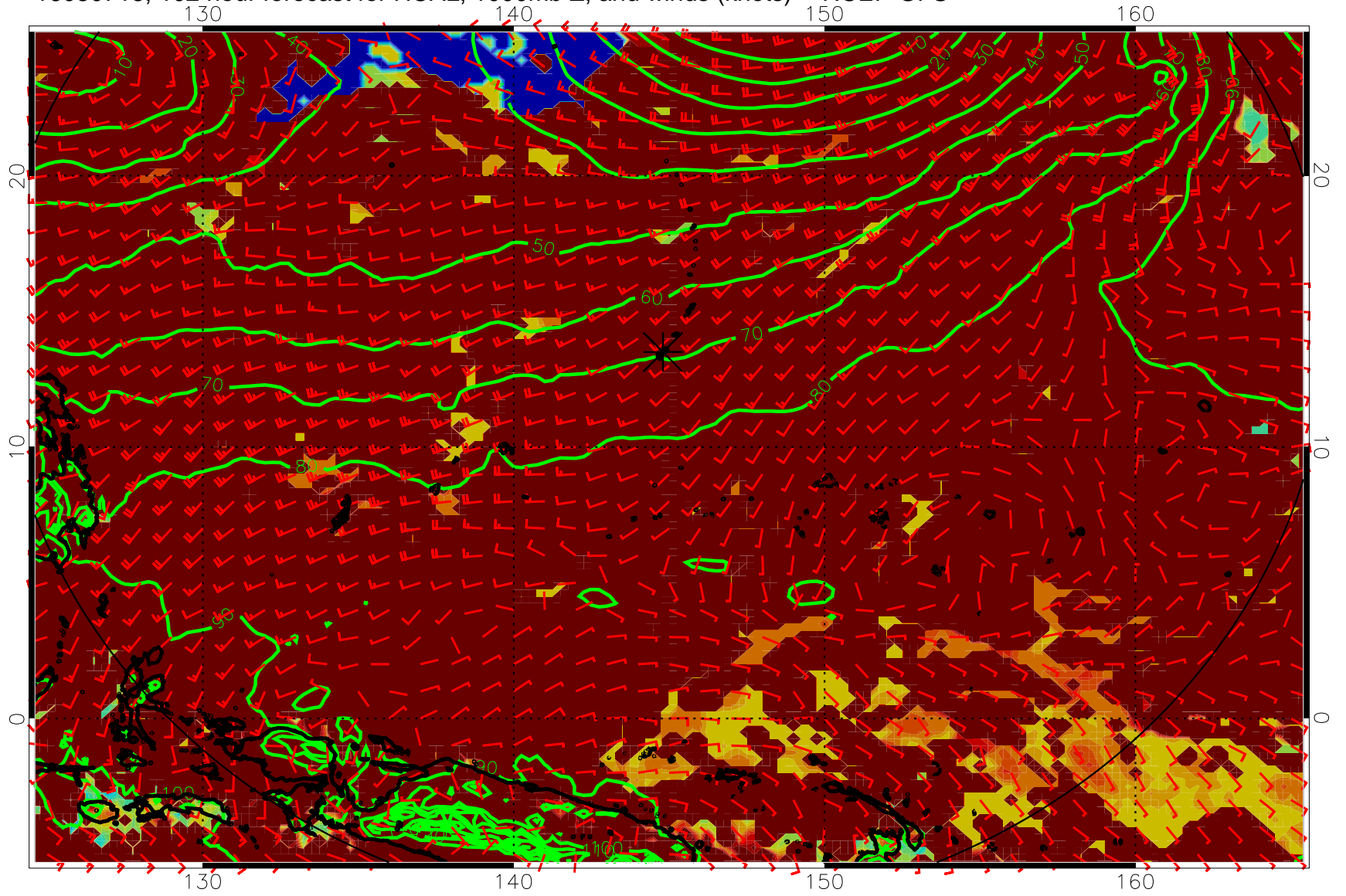
16080718, 102 hour forecast for HCAL, 1000mb Z, and winds (knots) -- NCEP GFS
