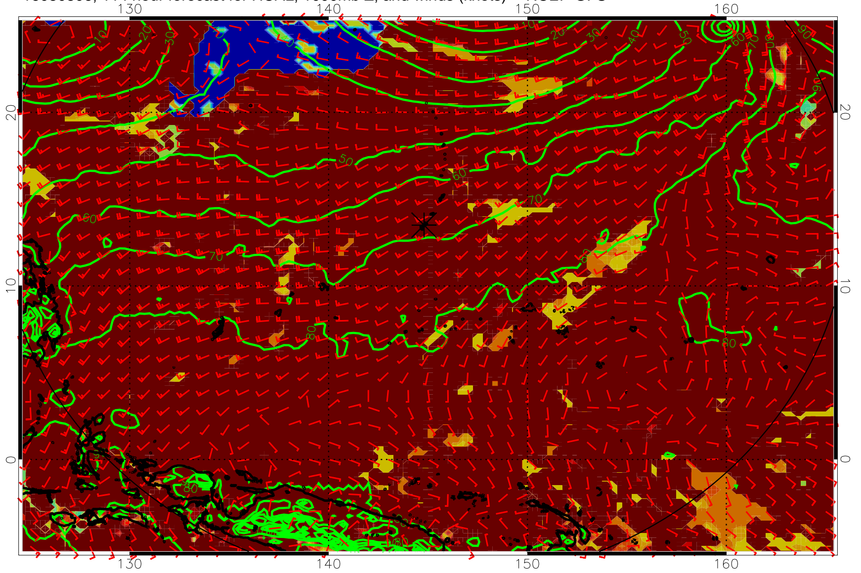
16080806, 114 hour forecast for HCAL, 1000mb Z, and winds (knots) -- NCEP GFS
