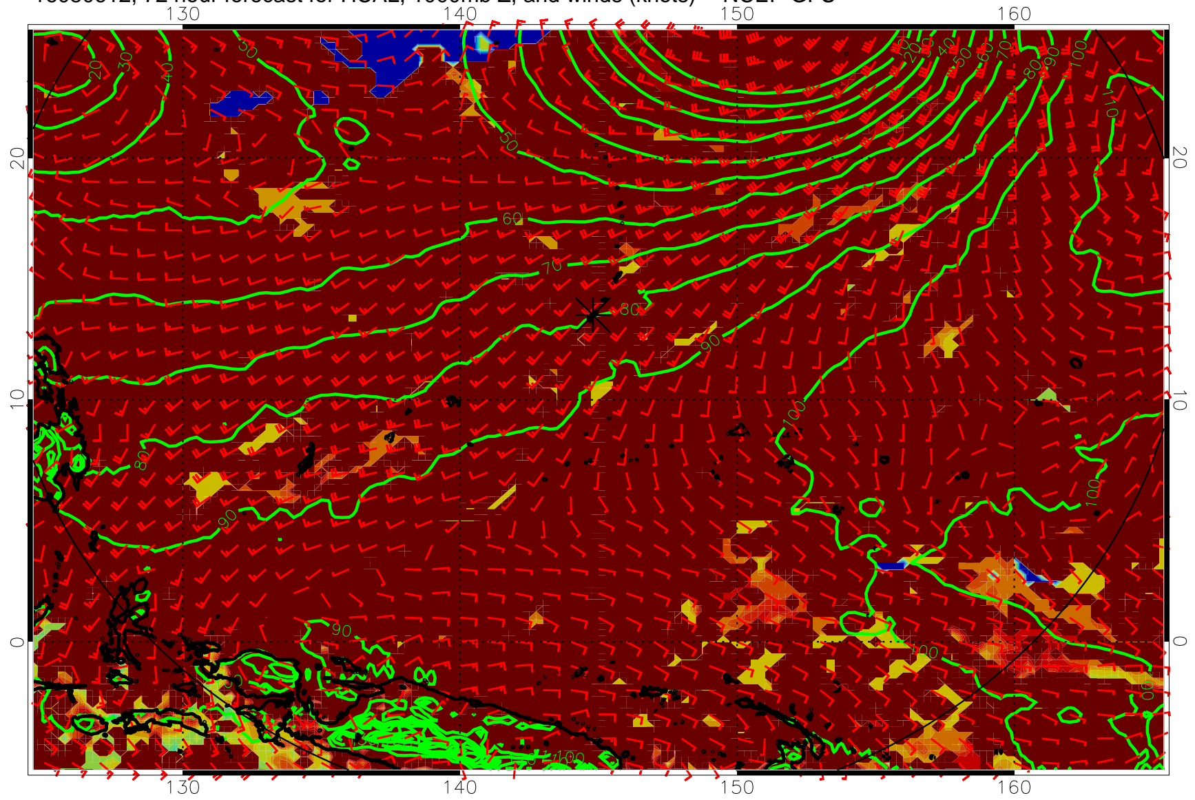
16080612, 72 hour forecast for HCAL, 1000mb Z, and winds (knots) -- NCEP GFS
