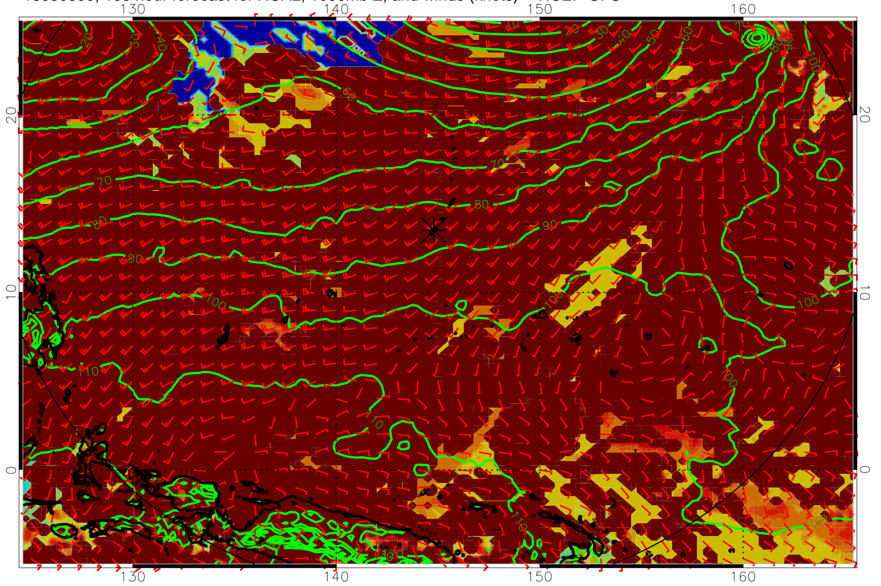
16080800, 108 hour forecast for HCAL, 1000mb Z, and winds (knots) -- NCEP GFS
