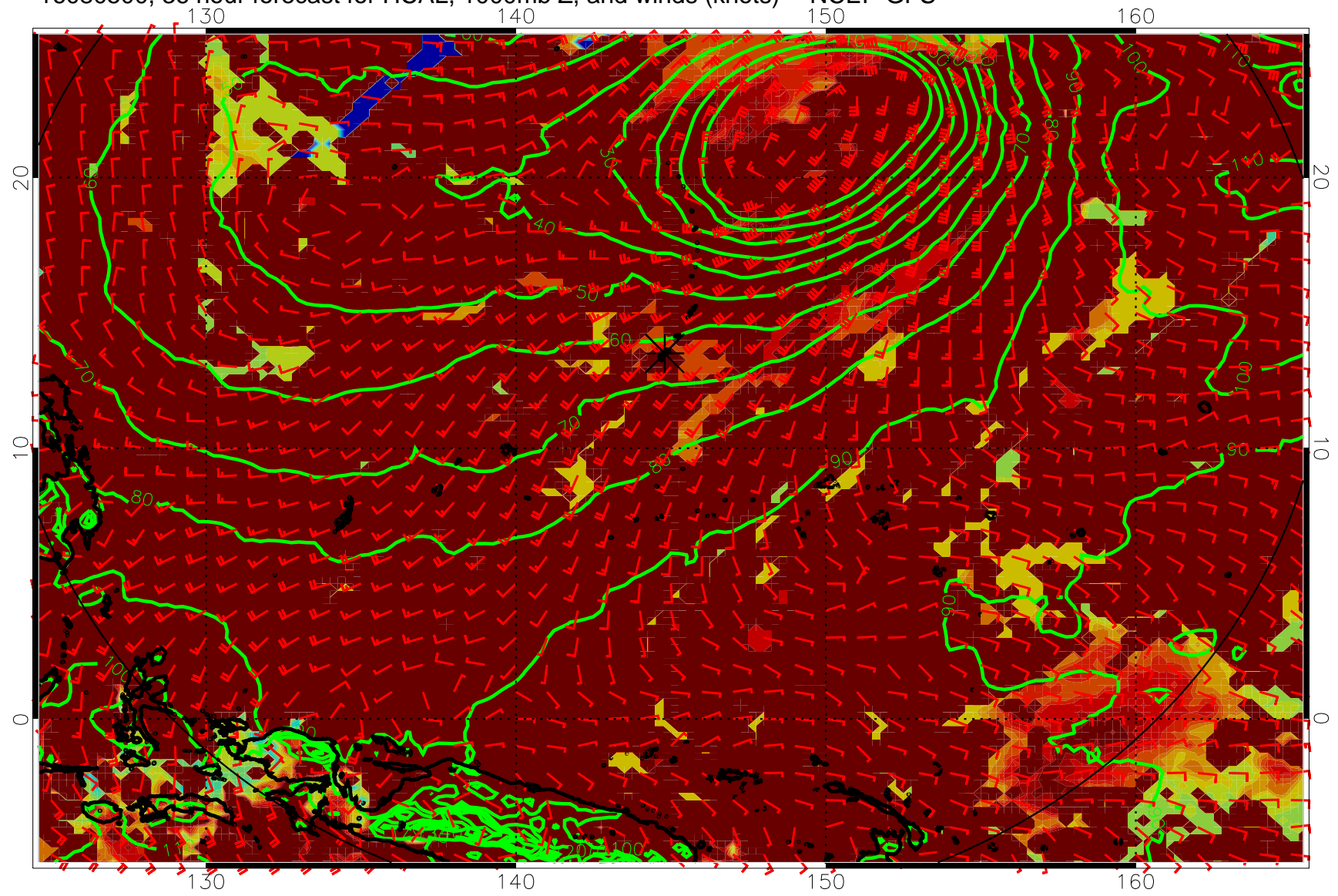
16080500, 36 hour forecast for HCAL, 1000mb Z, and winds (knots) -- NCEP GFS
