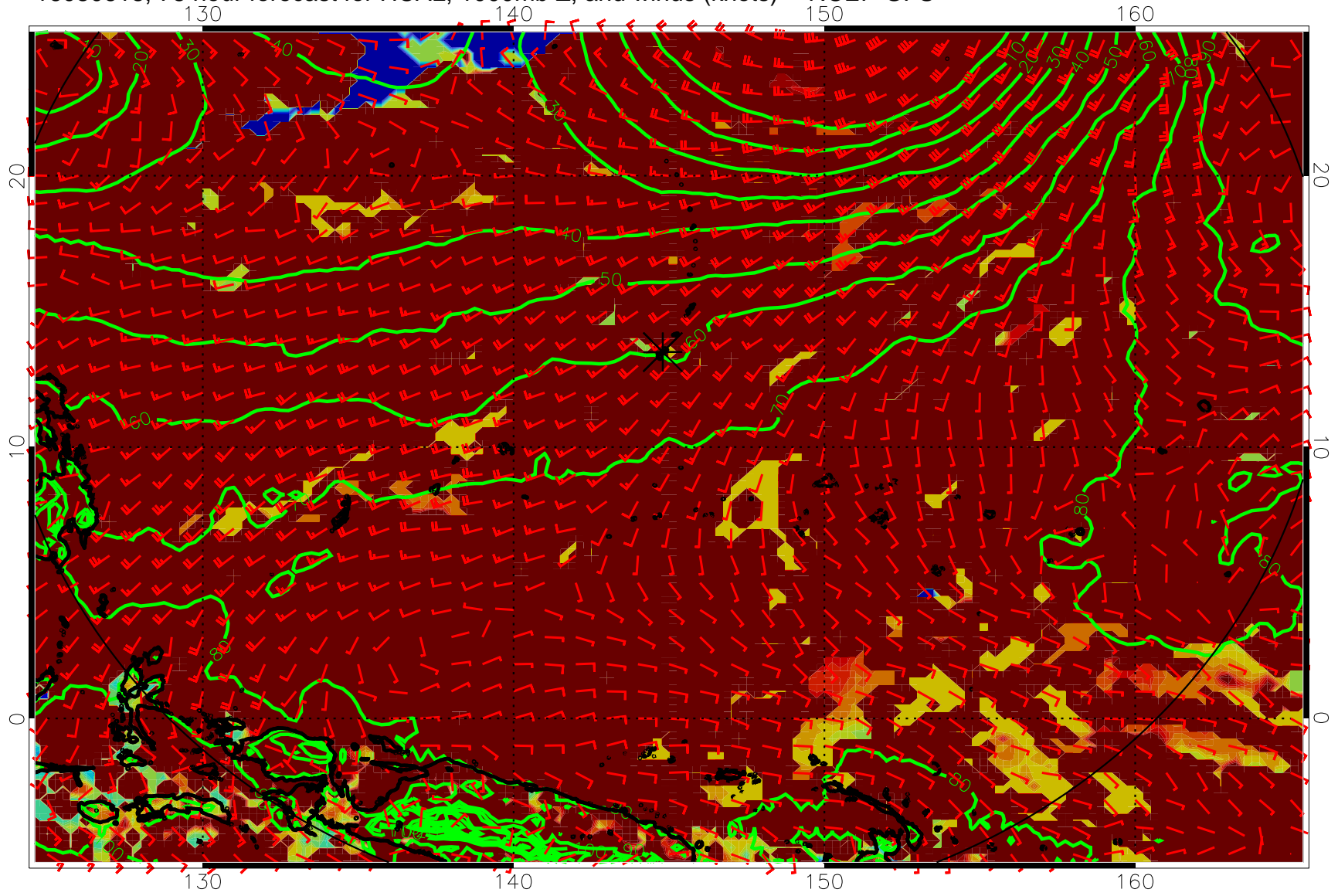
16080618, 78 hour forecast for HCAL, 1000mb Z, and winds (knots) -- NCEP GFS
