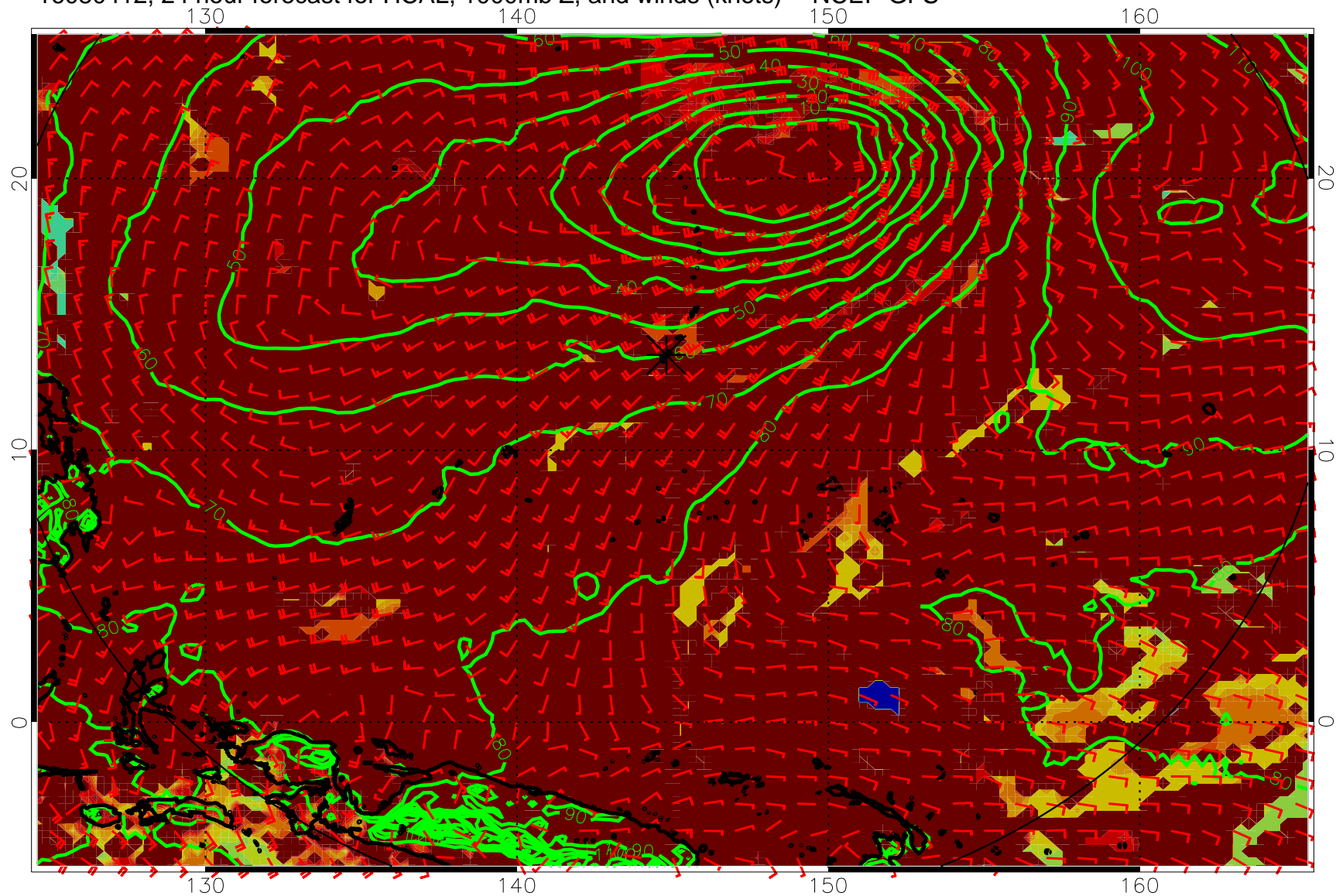
16080412, 24 hour forecast for HCAL, 1000mb Z, and winds (knots) -- NCEP GFS
