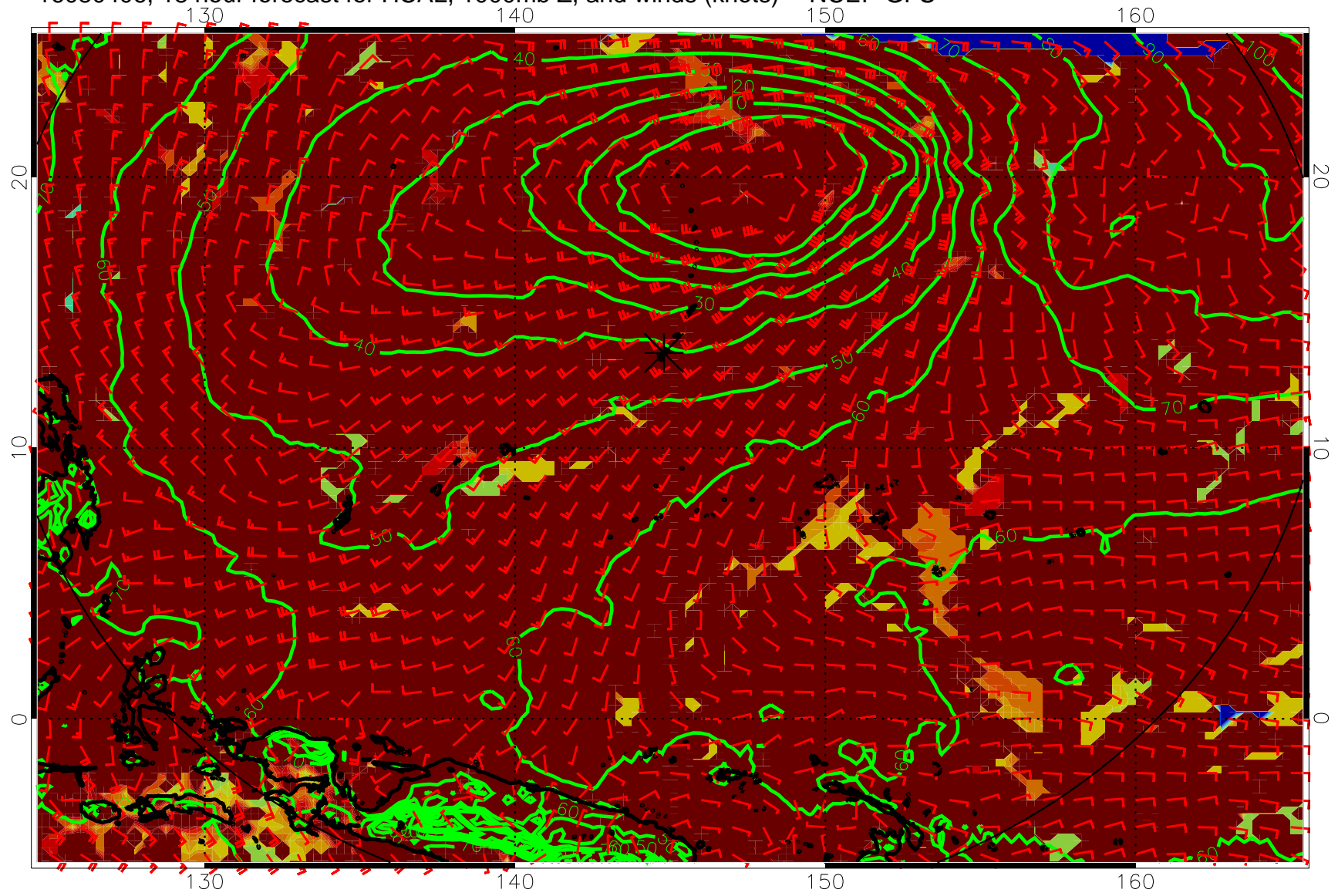
16080406, 18 hour forecast for HCAL, 1000mb Z, and winds (knots) -- NCEP GFS
