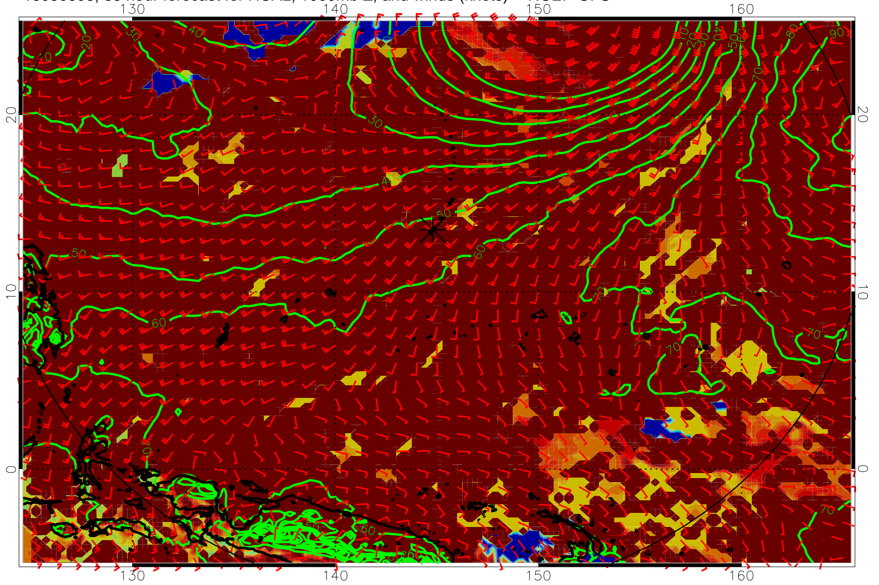
16080606, 66 hour forecast for HCAL, 1000mb Z, and winds (knots) -- NCEP GFS
