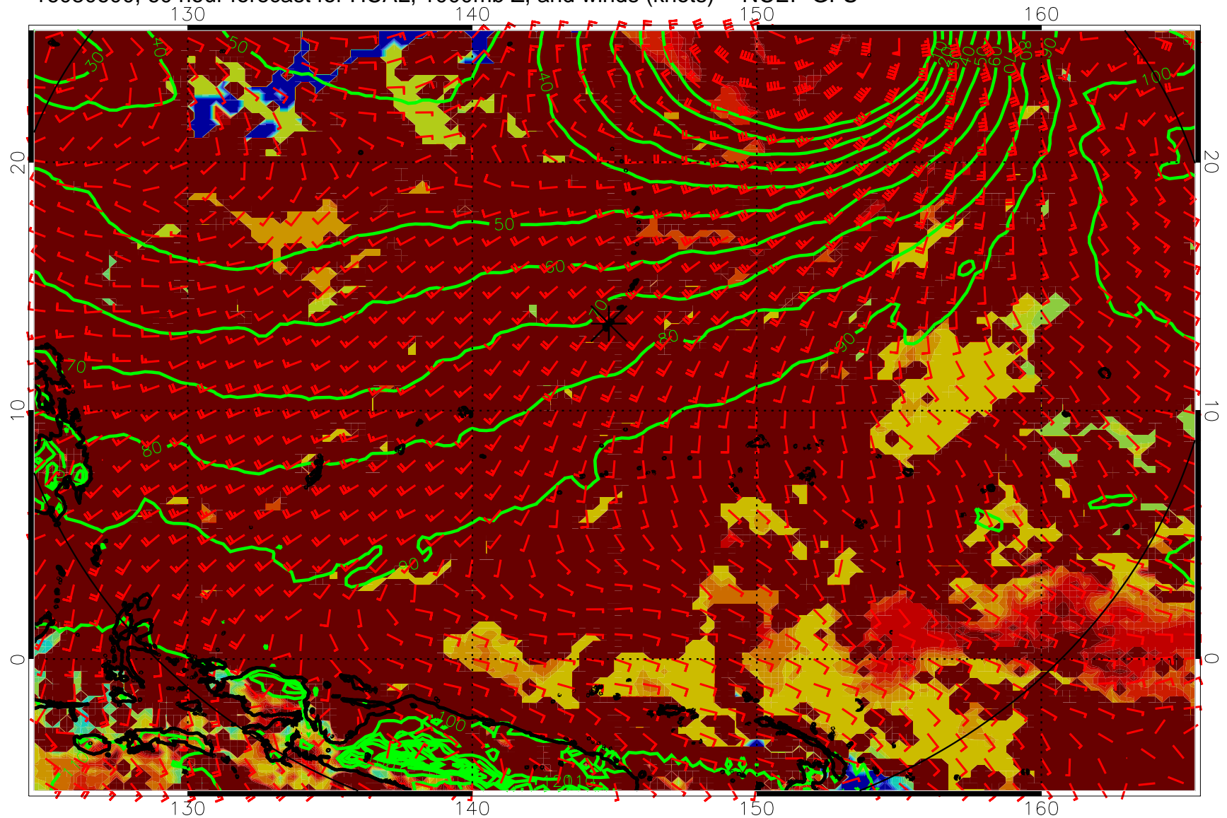
16080600, 60 hour forecast for HCAL, 1000mb Z, and winds (knots) -- NCEP GFS
