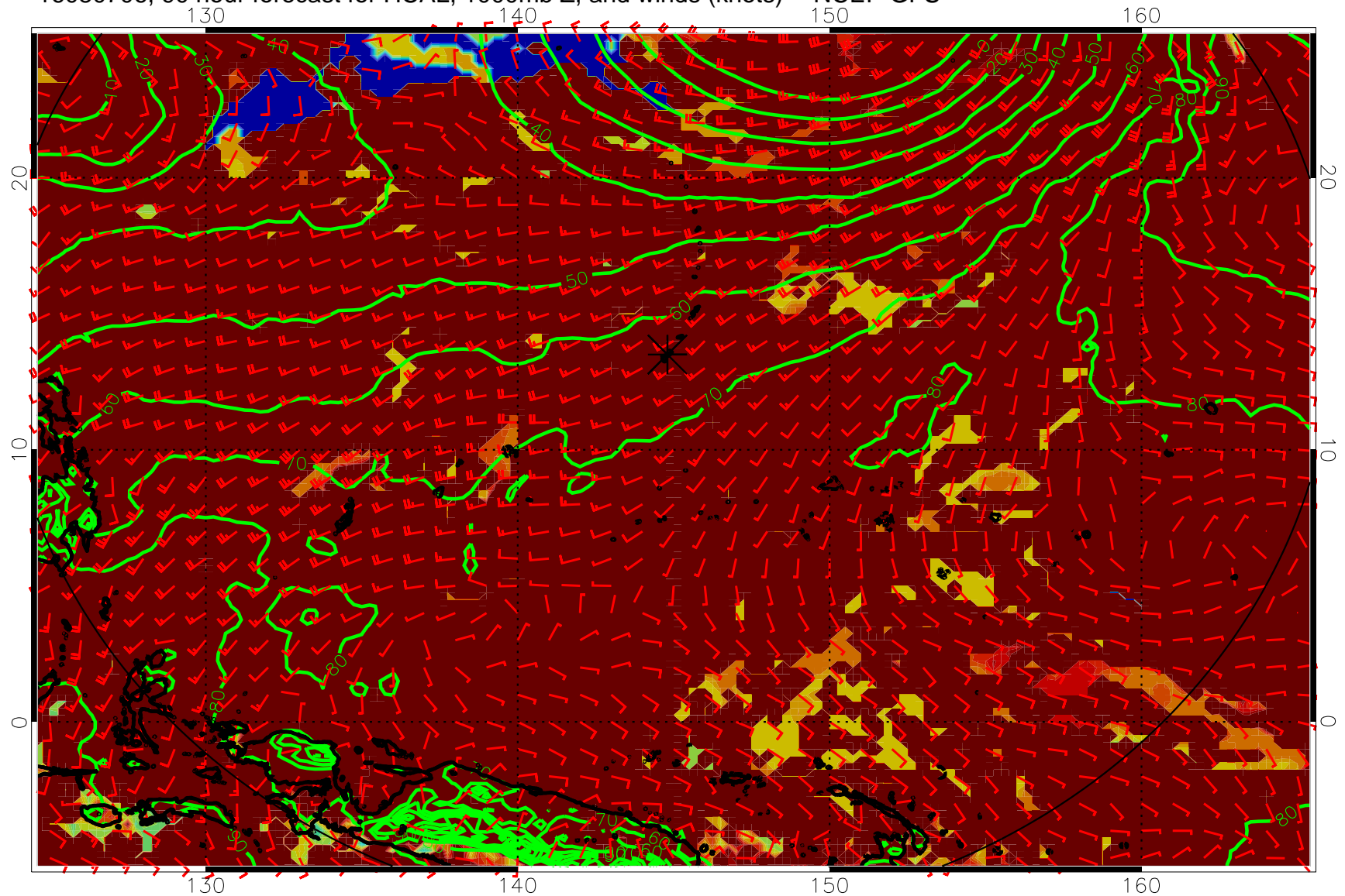
16080706, 90 hour forecast for HCAL, 1000mb Z, and winds (knots) -- NCEP GFS
