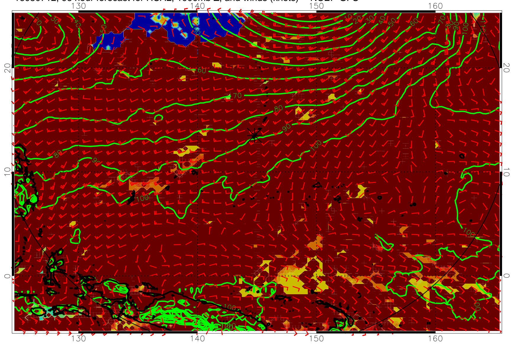
16080712, 96 hour forecast for HCAL, 1000mb Z, and winds (knots) -- NCEP GFS
