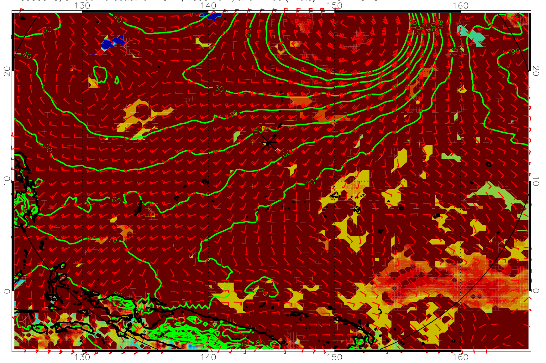
16080518, 54 hour forecast for HCAL, 1000mb Z, and winds (knots) -- NCEP GFS
