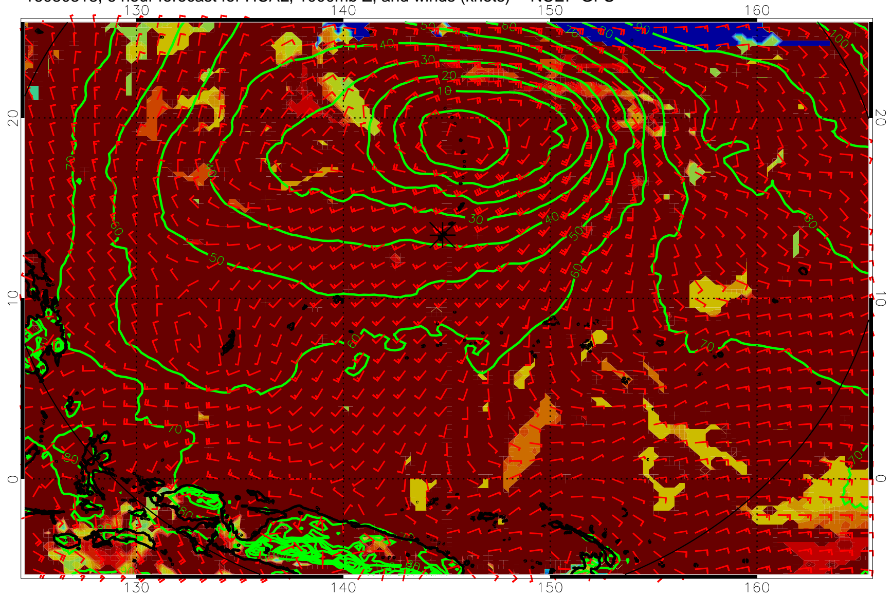
16080318, 6 hour forecast for HCAL, 1000mb Z, and winds (knots) -- NCEP GFS
