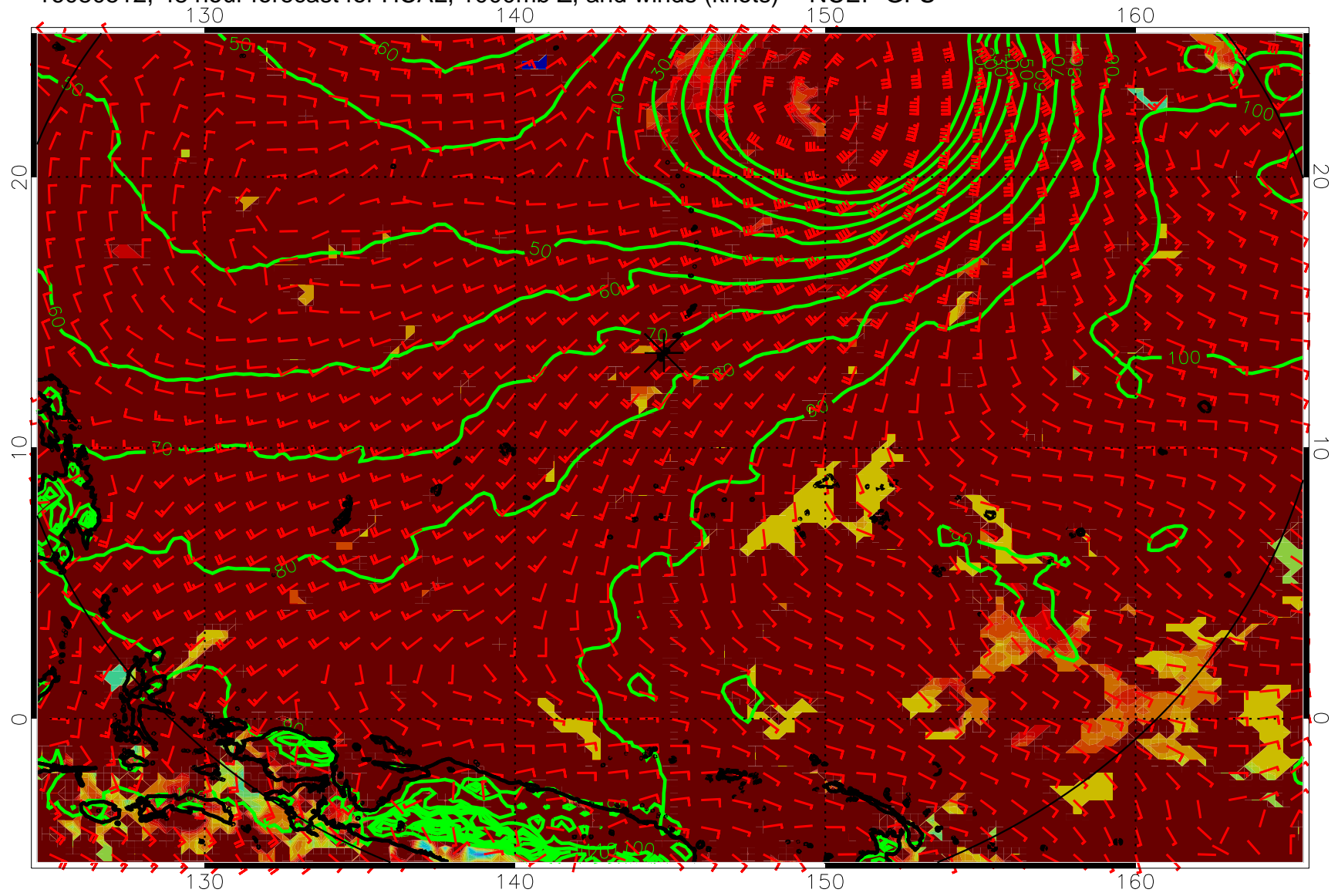
16080512, 48 hour forecast for HCAL, 1000mb Z, and winds (knots) -- NCEP GFS
