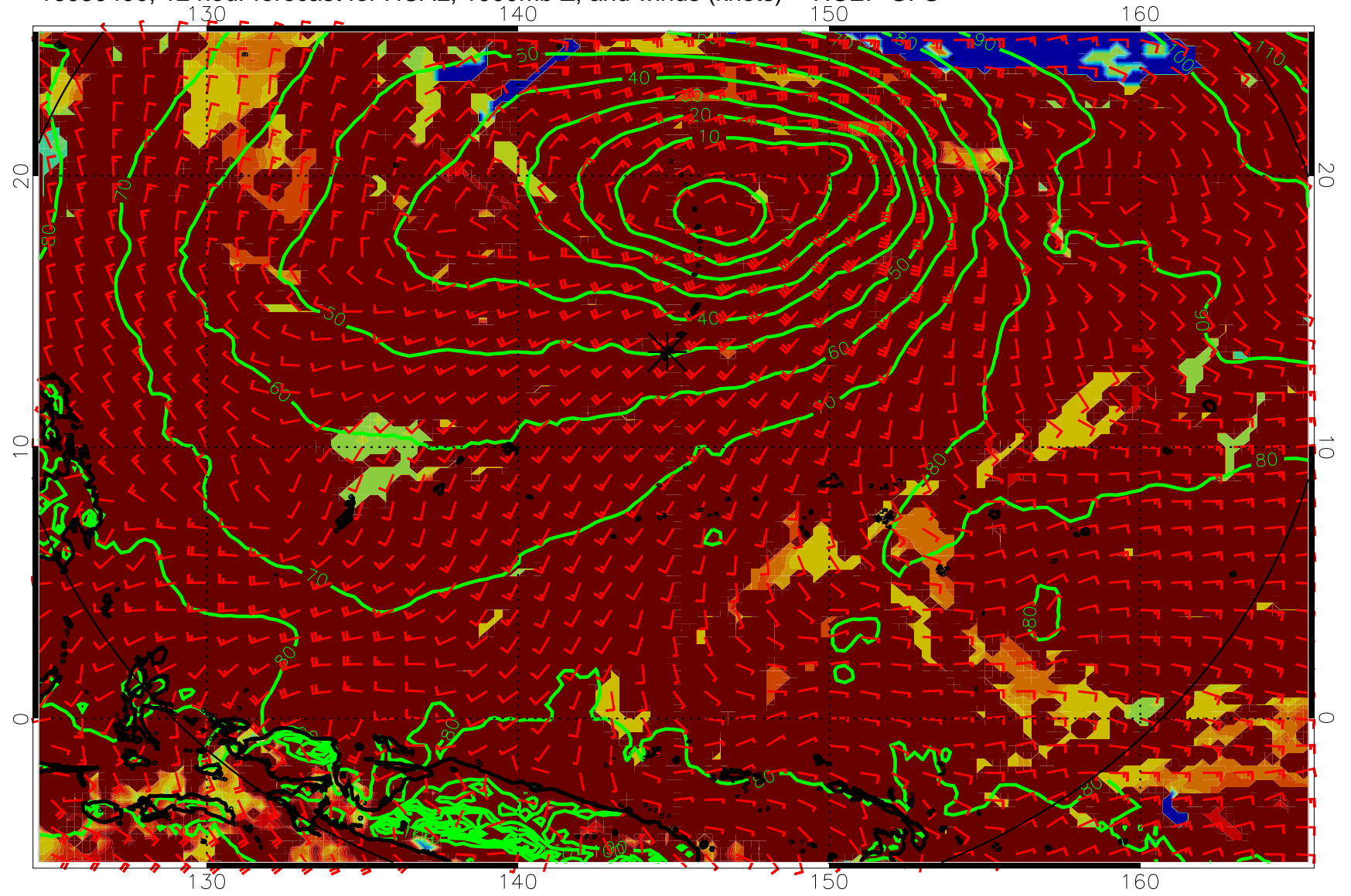
16080400, 12 hour forecast for HCAL, 1000mb Z, and winds (knots) -- NCEP GFS
