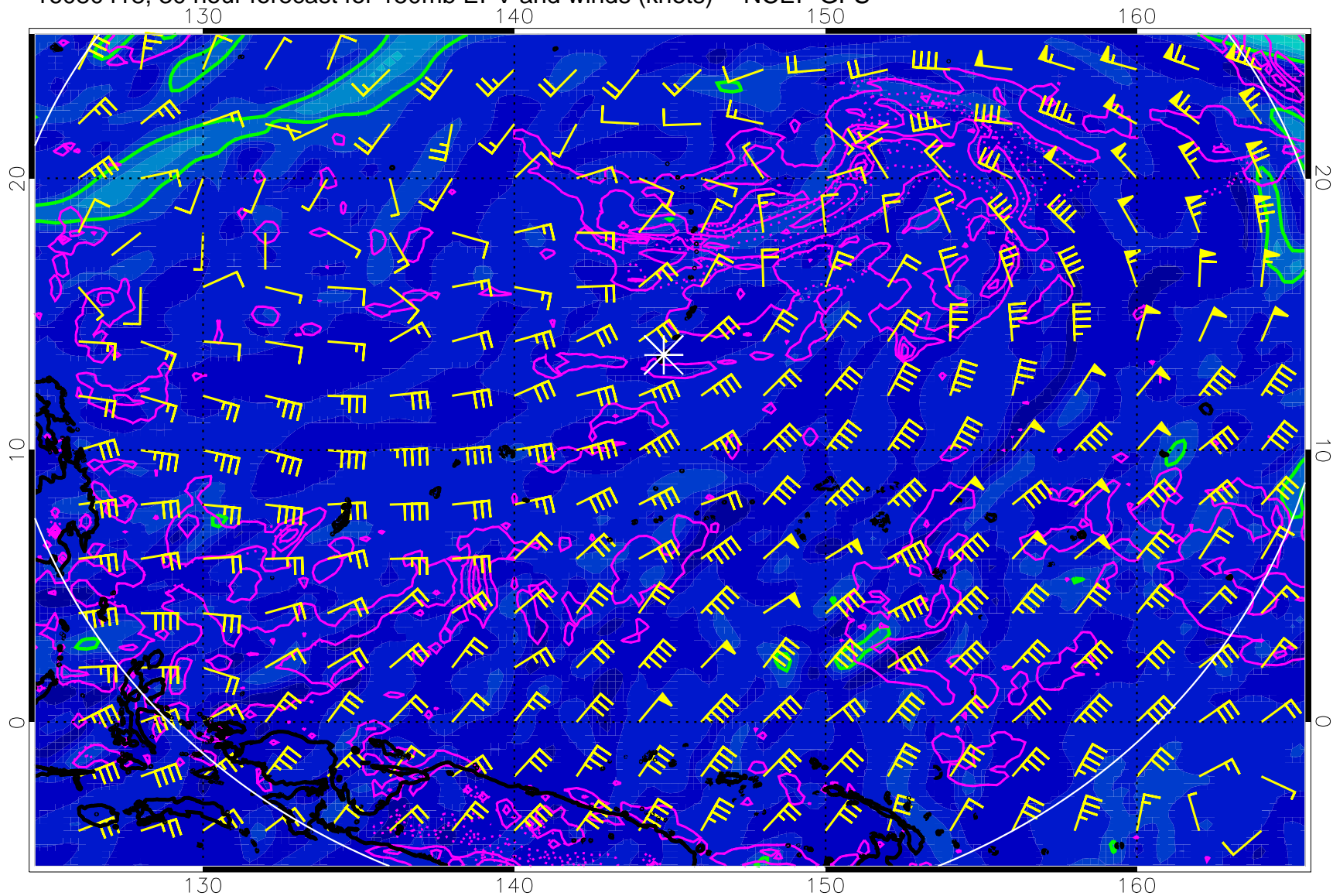
16080418, 30 hour forecast for 150mb EPV and winds (knots) -- NCEP GFS
