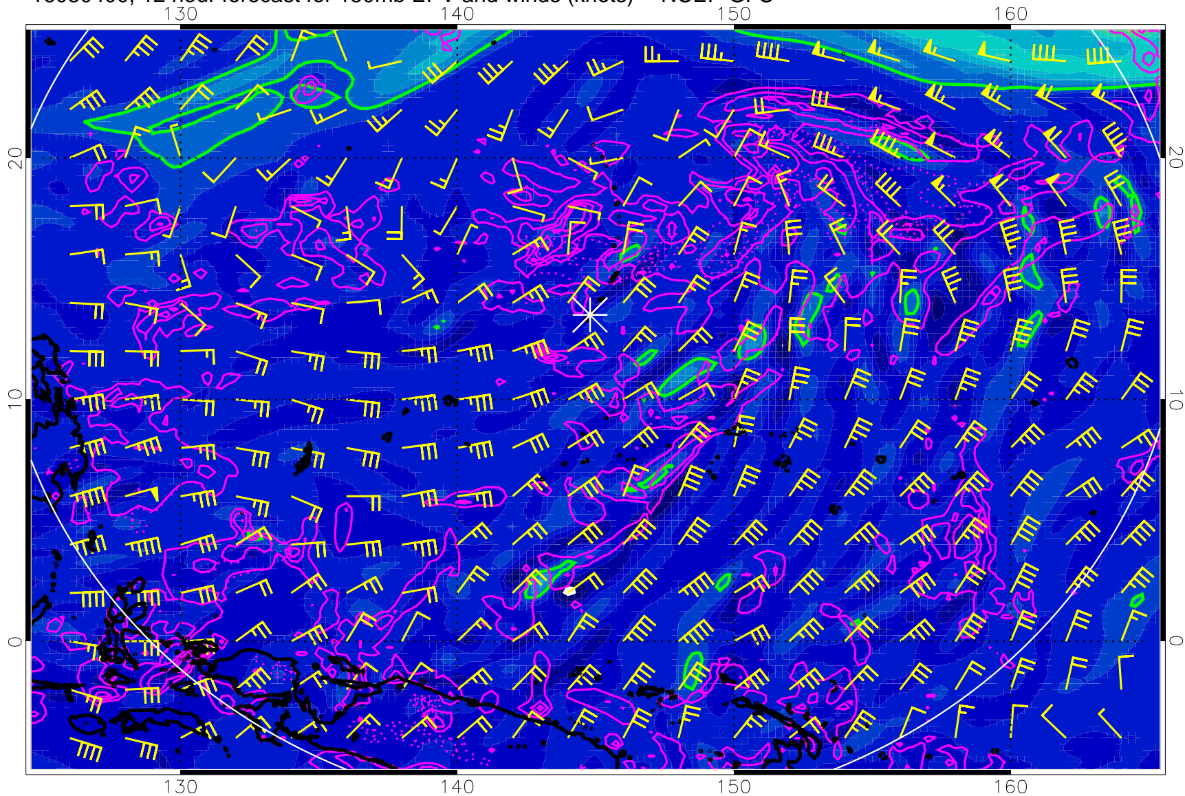
16080400, 12 hour forecast for 150mb EPV and winds (knots) -- NCEP GFS
