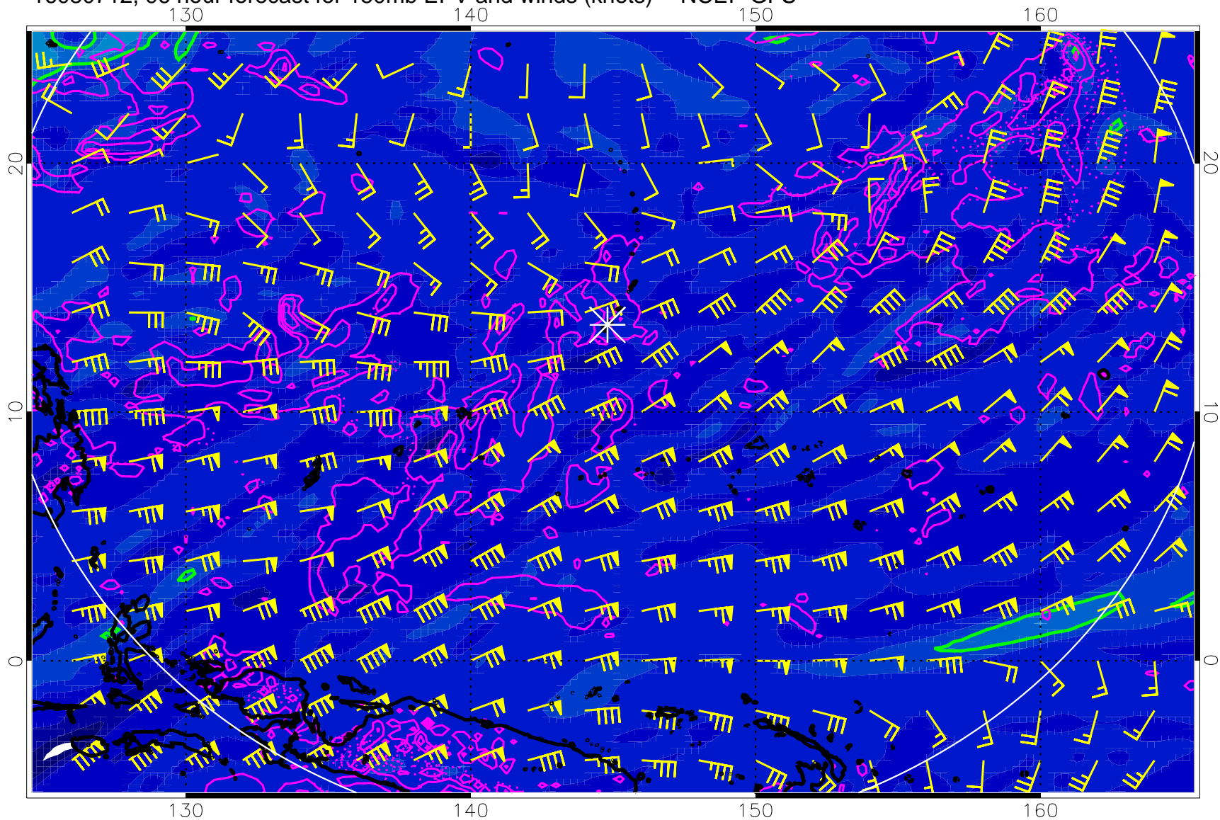
16080712, 96 hour forecast for 150mb EPV and winds (knots) -- NCEP GFS
