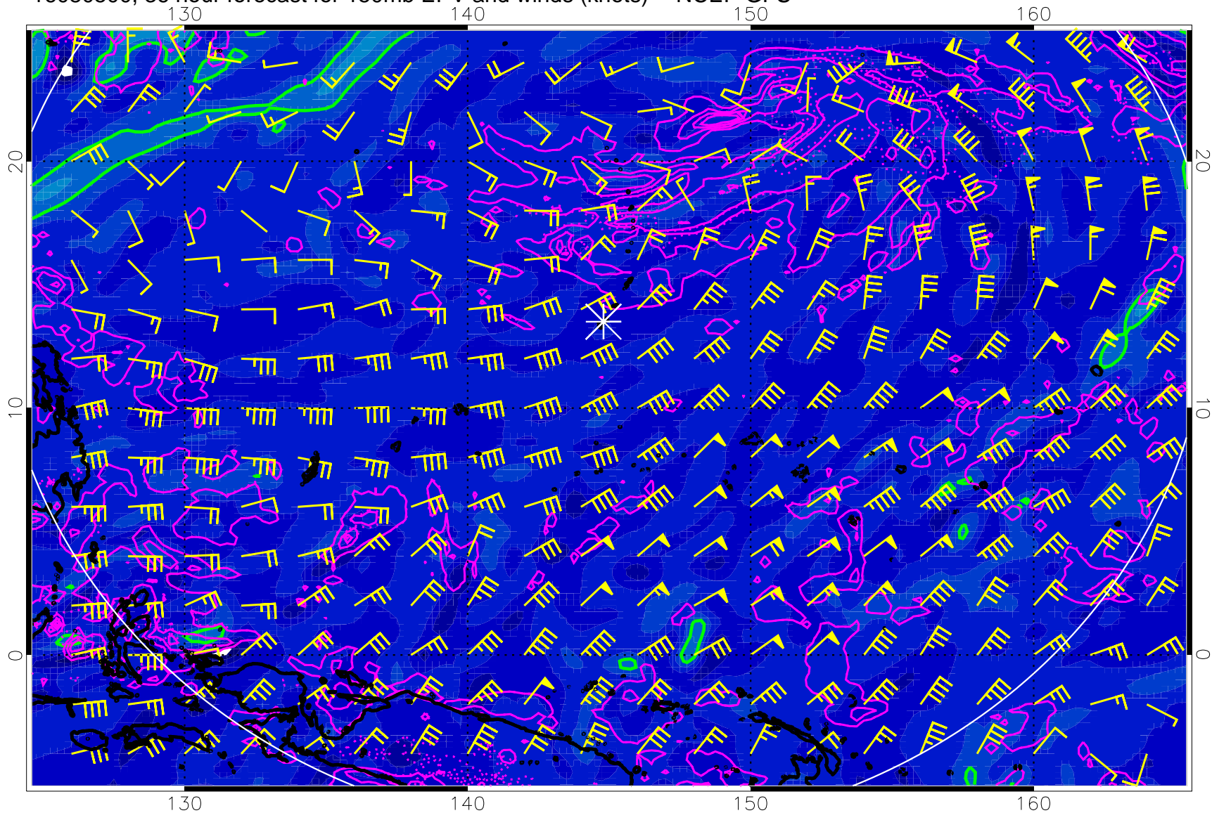
16080500, 36 hour forecast for 150mb EPV and winds (knots) -- NCEP GFS
