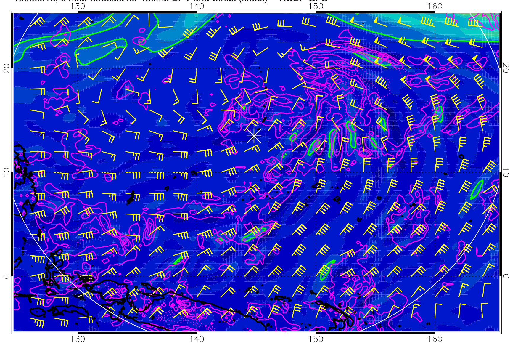
16080318, 6 hour forecast for 150mb EPV and winds (knots) -- NCEP GFS
