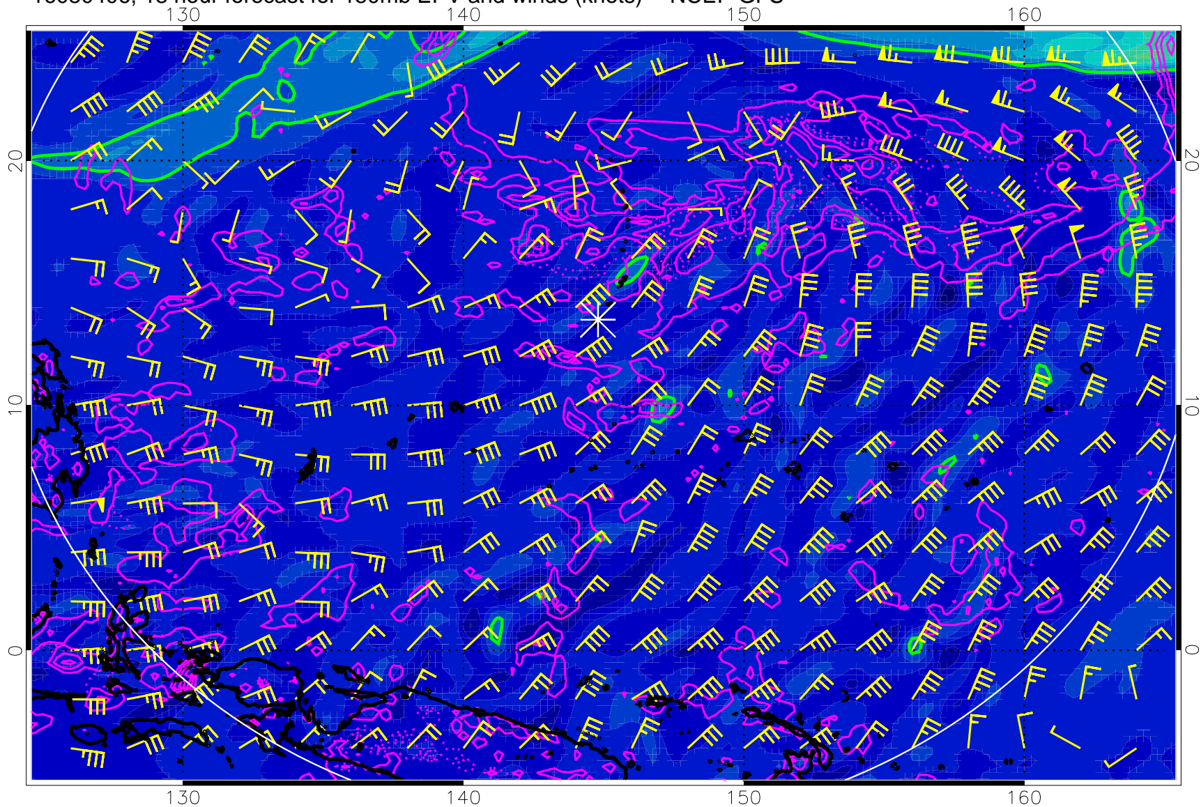
16080406, 18 hour forecast for 150mb EPV and winds (knots) -- NCEP GFS
