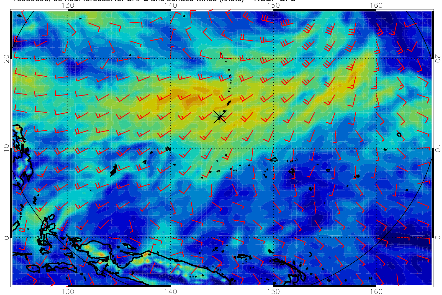
16080606, 66 hour forecast for CAPE and surface winds (knots) -- NCEP GFS
