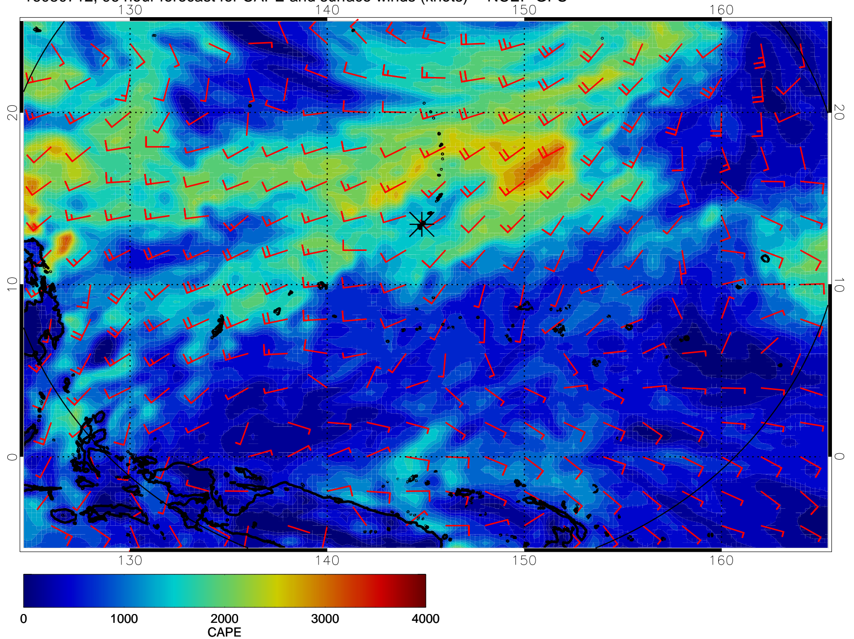
16080712, 96 hour forecast for CAPE and surface winds (knots) -- NCEP GFS
