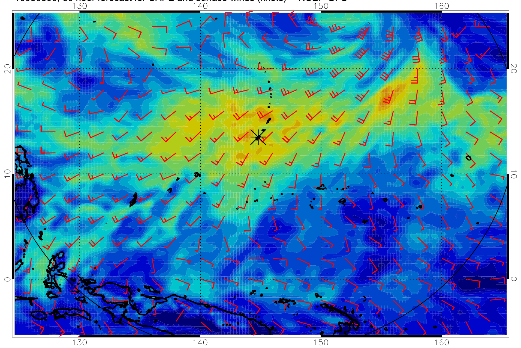
16080600, 60 hour forecast for CAPE and surface winds (knots) -- NCEP GFS
