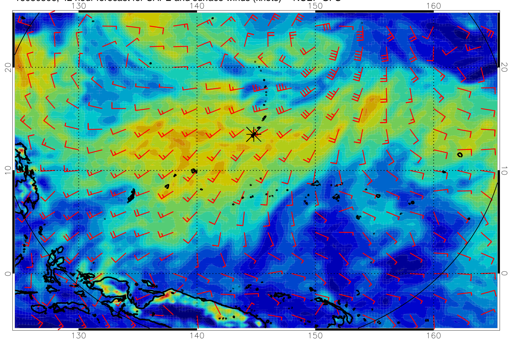
16080506, 42 hour forecast for CAPE and surface winds (knots) -- NCEP GFS
