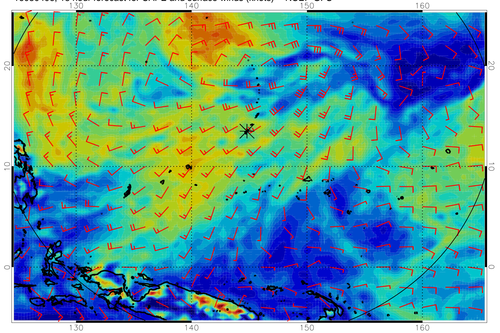
16080406, 18 hour forecast for CAPE and surface winds (knots) -- NCEP GFS
