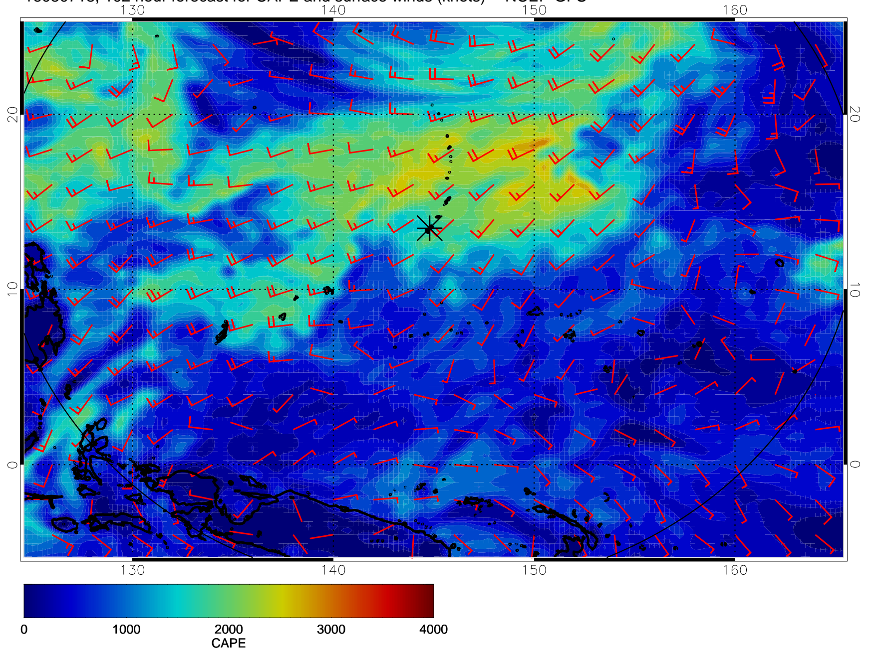
16080718, 102 hour forecast for CAPE and surface winds (knots) -- NCEP GFS
