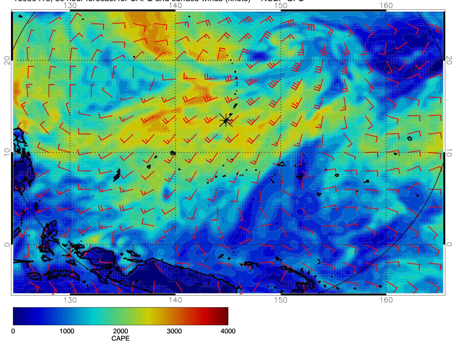
16080418, 30 hour forecast for CAPE and surface winds (knots) -- NCEP GFS
