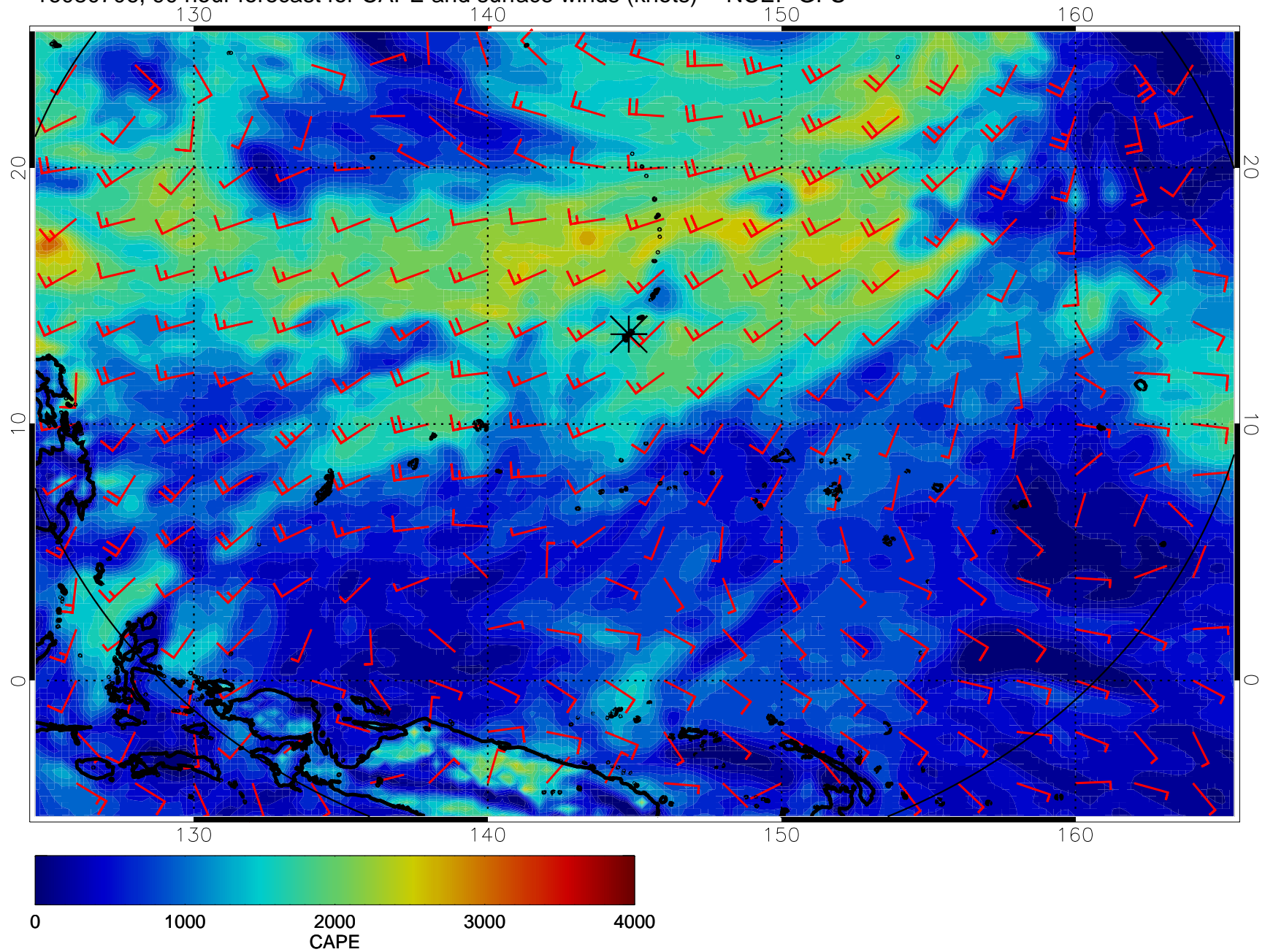
16080706, 90 hour forecast for CAPE and surface winds (knots) -- NCEP GFS
