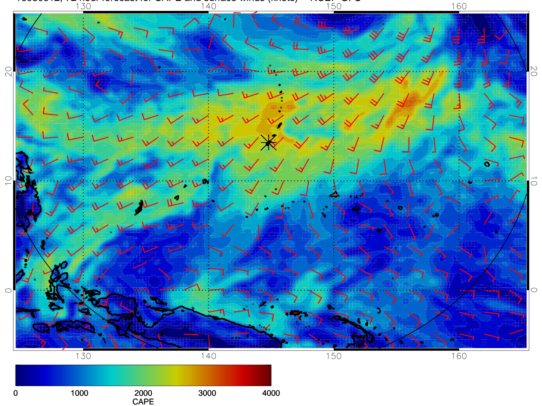
16080612, 72 hour forecast for CAPE and surface winds (knots) -- NCEP GFS
