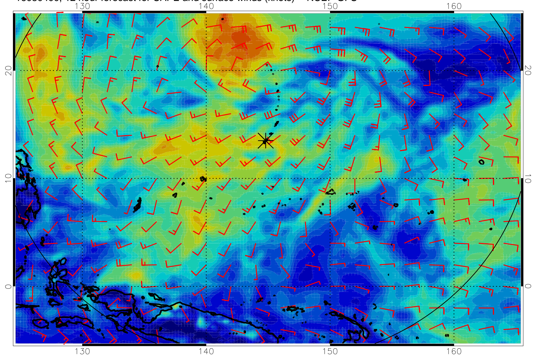
16080400, 12 hour forecast for CAPE and surface winds (knots) -- NCEP GFS
