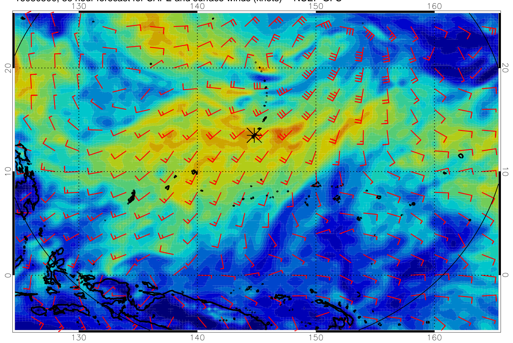
16080500, 36 hour forecast for CAPE and surface winds (knots) -- NCEP GFS
