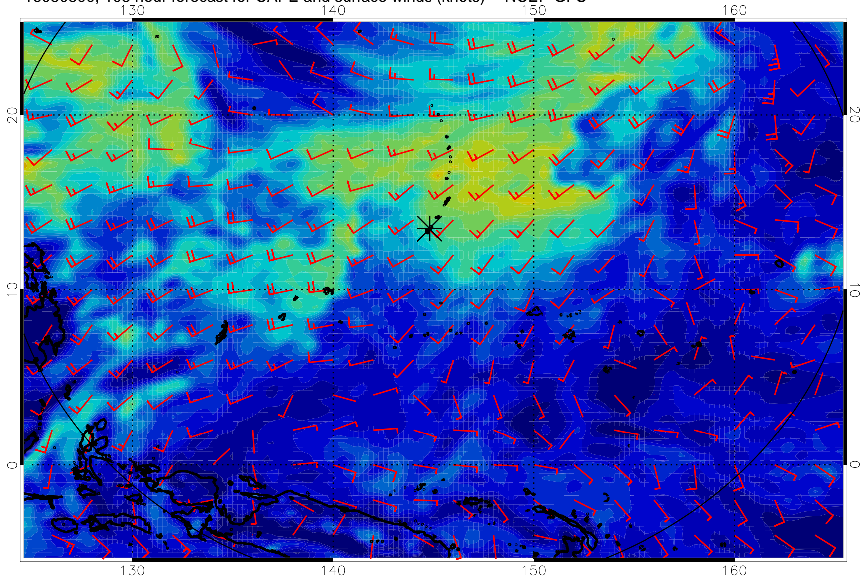
16080800, 108 hour forecast for CAPE and surface winds (knots) -- NCEP GFS
