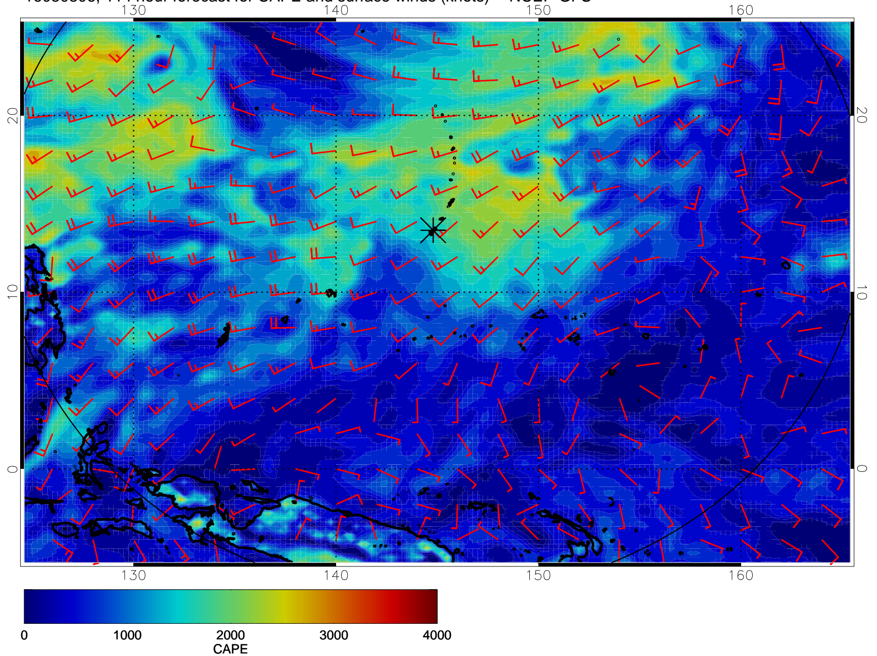
16080806, 114 hour forecast for CAPE and surface winds (knots) -- NCEP GFS
