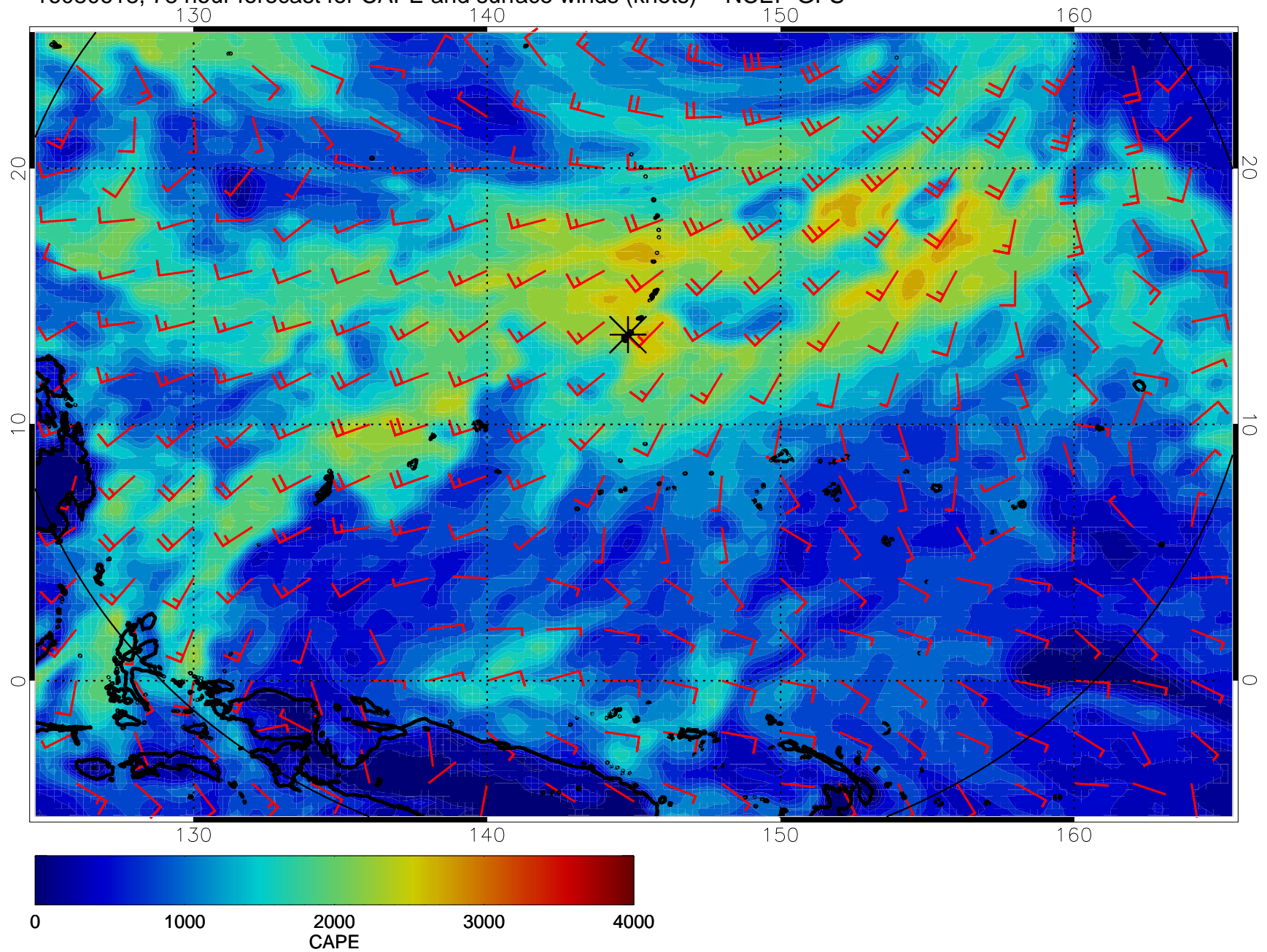
16080618, 78 hour forecast for CAPE and surface winds (knots) -- NCEP GFS
