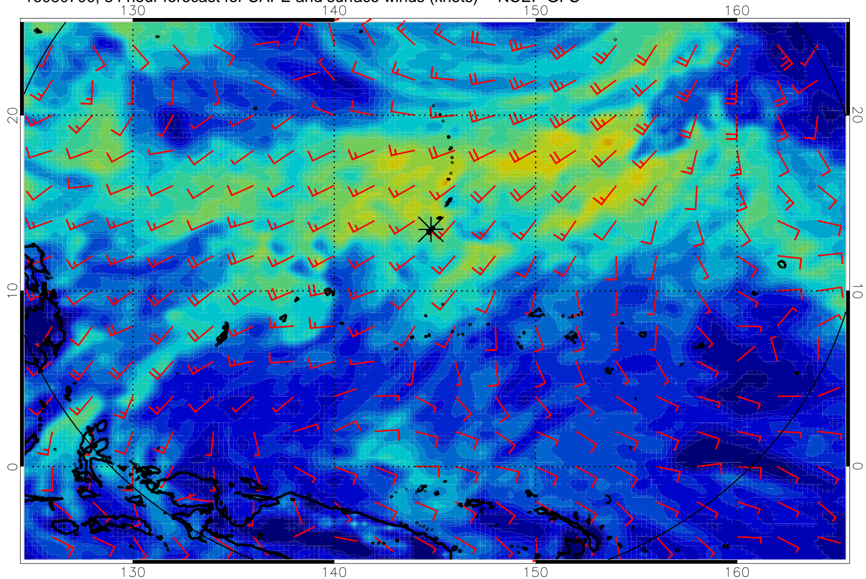
16080700, 84 hour forecast for CAPE and surface winds (knots) -- NCEP GFS
