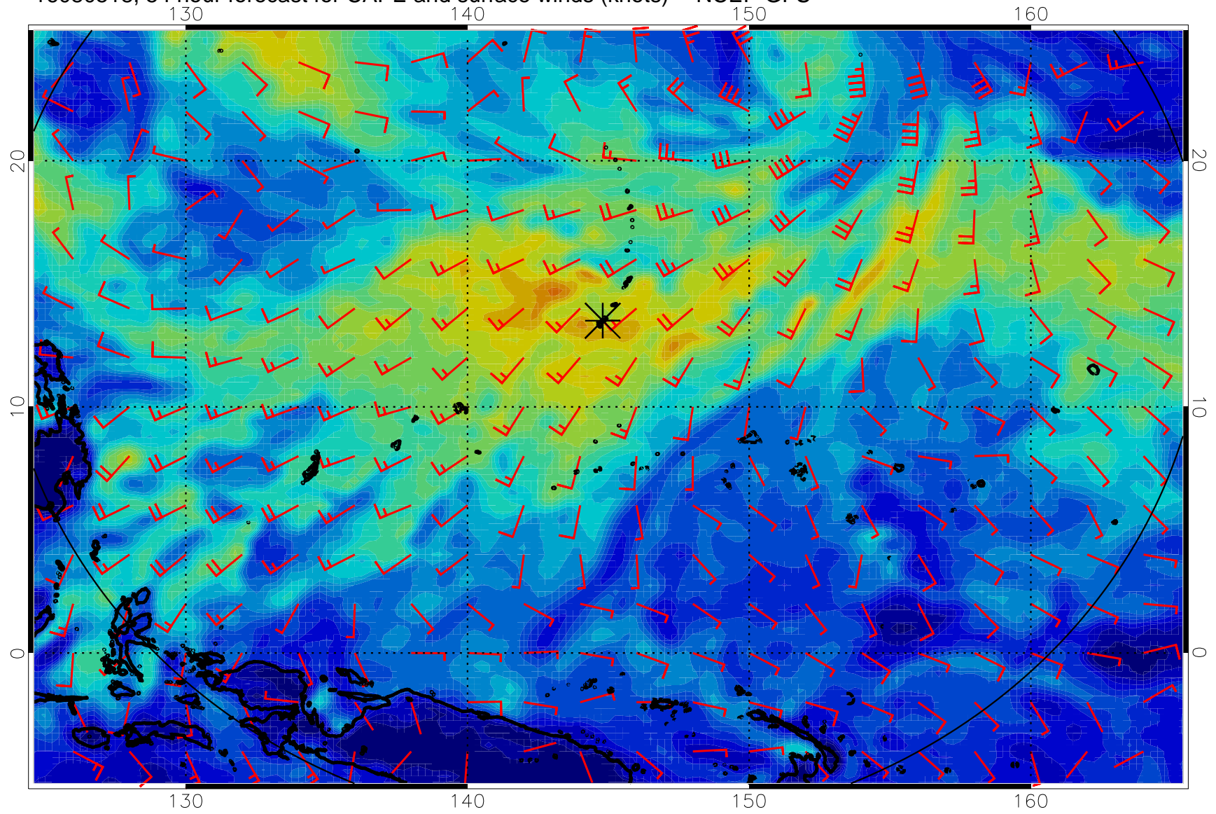
16080518, 54 hour forecast for CAPE and surface winds (knots) -- NCEP GFS
