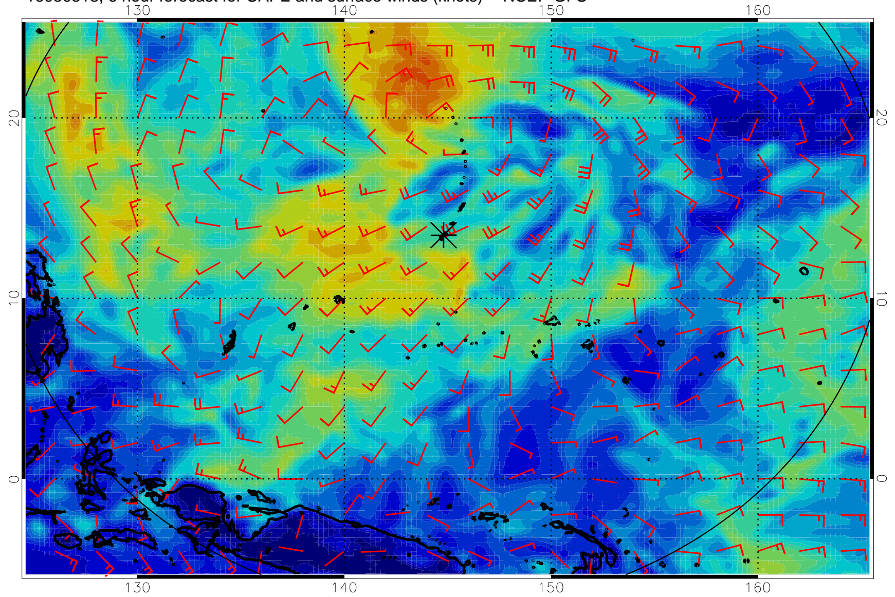
16080318, 6 hour forecast for CAPE and surface winds (knots) -- NCEP GFS
