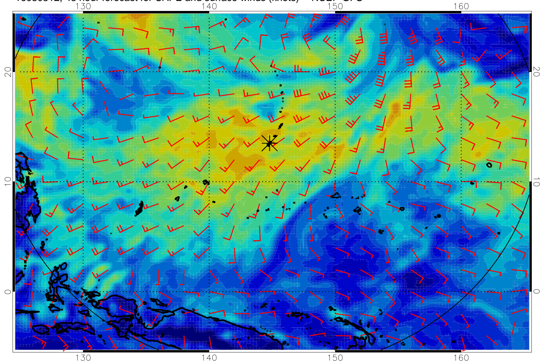
16080512, 48 hour forecast for CAPE and surface winds (knots) -- NCEP GFS
