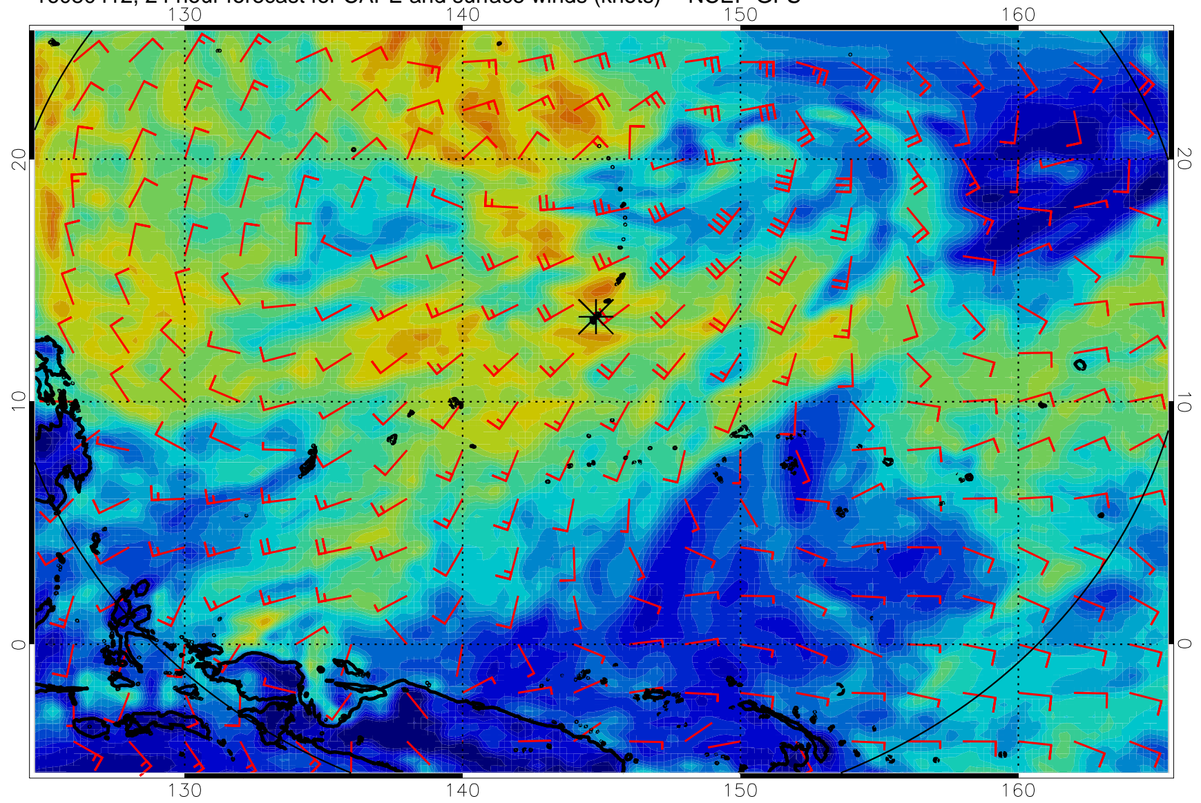
16080412, 24 hour forecast for CAPE and surface winds (knots) -- NCEP GFS
