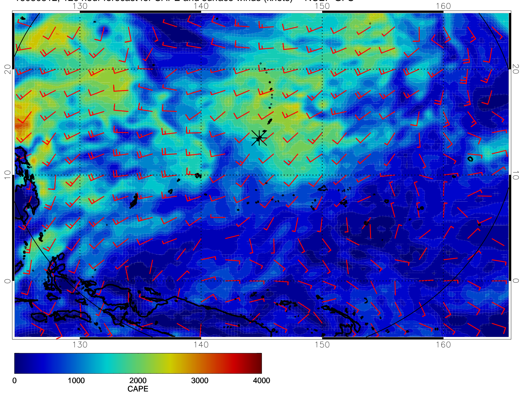
16080812, 120 hour forecast for CAPE and surface winds (knots) -- NCEP GFS
