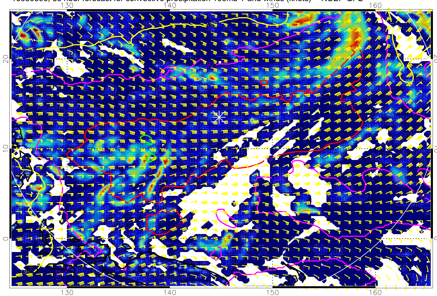
16080606, 66 hour forecast for convective precipitation 100mb T and winds (knots) -- NCEP GFS
