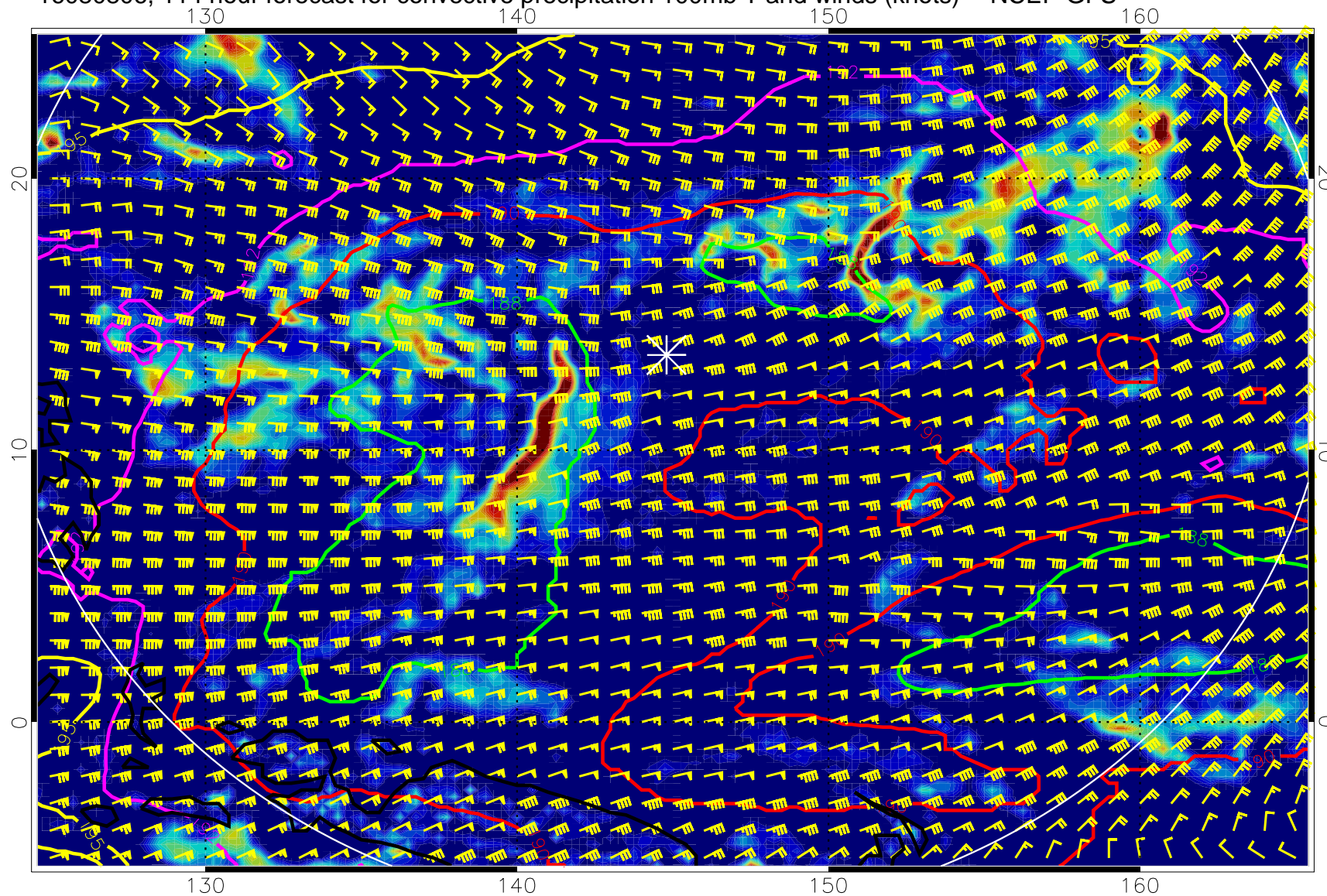
16080806, 114 hour forecast for convective precipitation 100mb T and winds (knots) -- NCEP GFS
