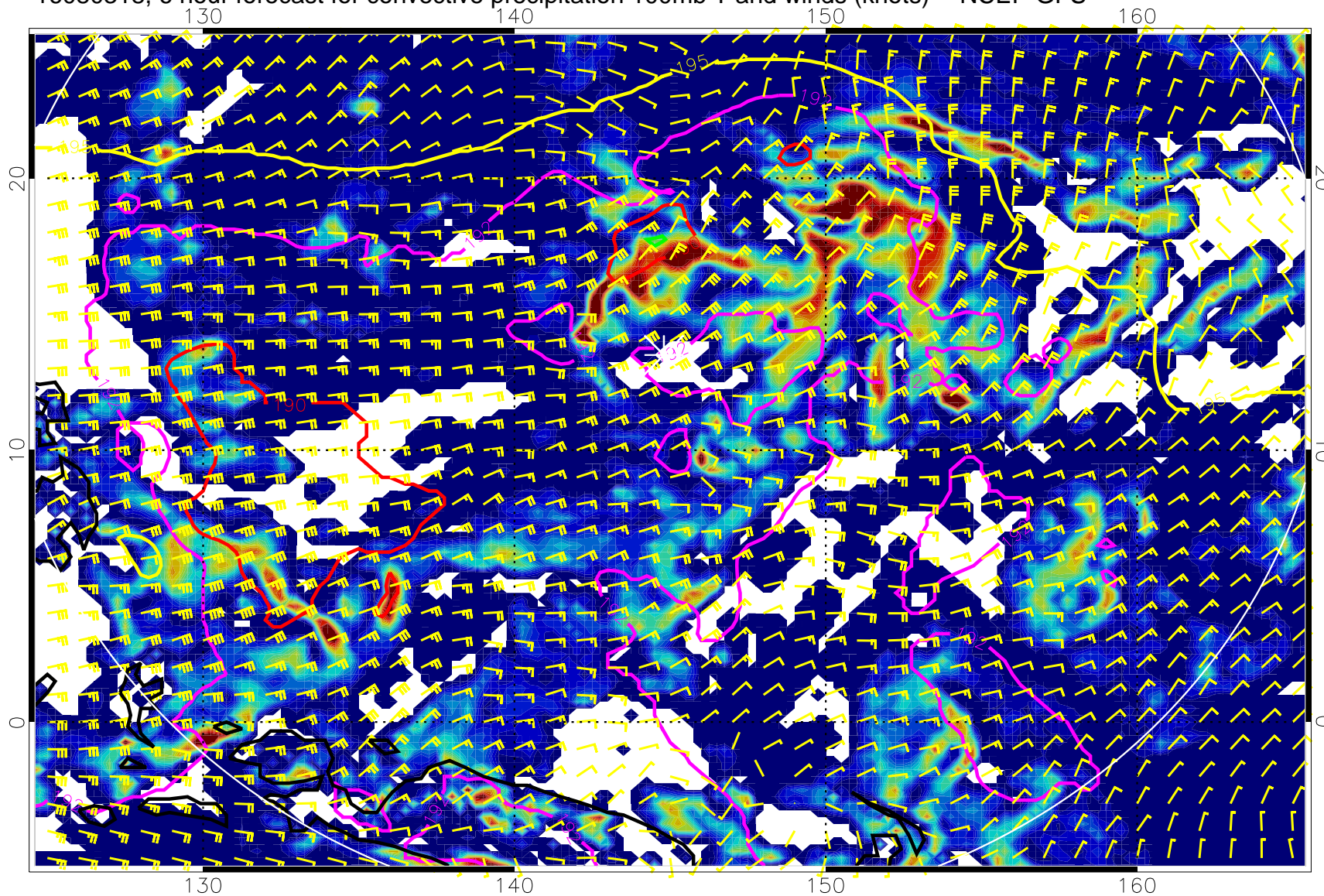
16080318, 6 hour forecast for convective precipitation 100mb T and winds (knots) -- NCEP GFS
