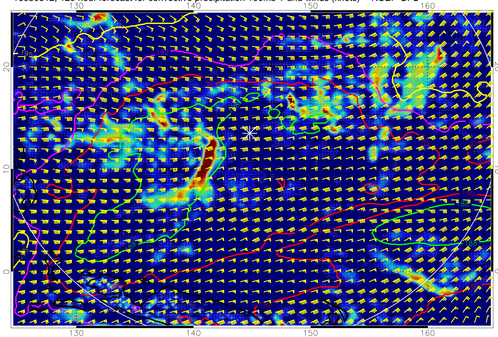
16080812, 120 hour forecast for convective precipitation 100mb T and winds (knots) -- NCEP GFS
