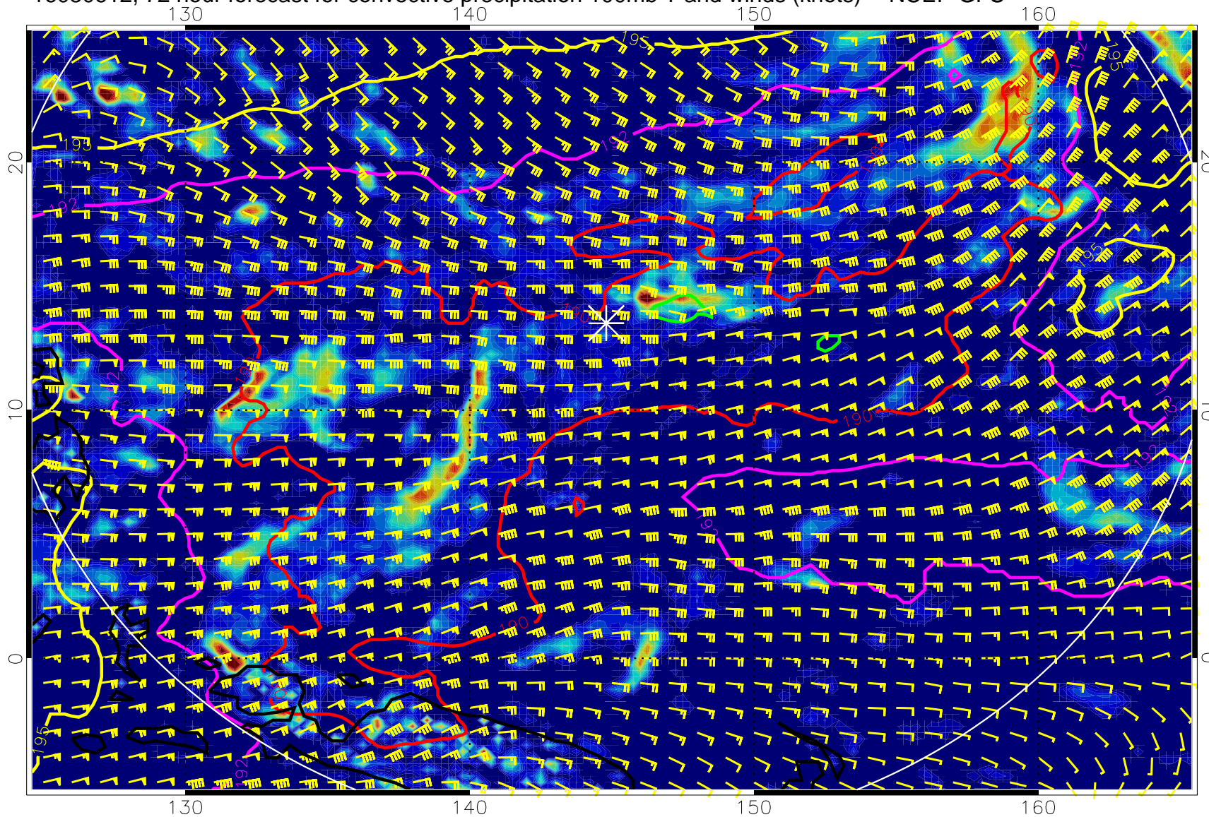
16080612, 72 hour forecast for convective precipitation 100mb T and winds (knots) -- NCEP GFS
