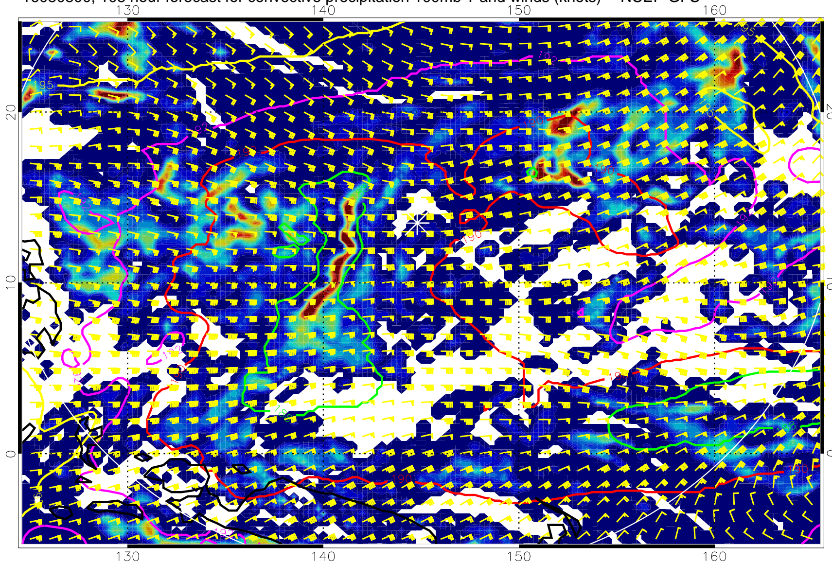
16080800, 108 hour forecast for convective precipitation 100mb T and winds (knots) -- NCEP GFS
