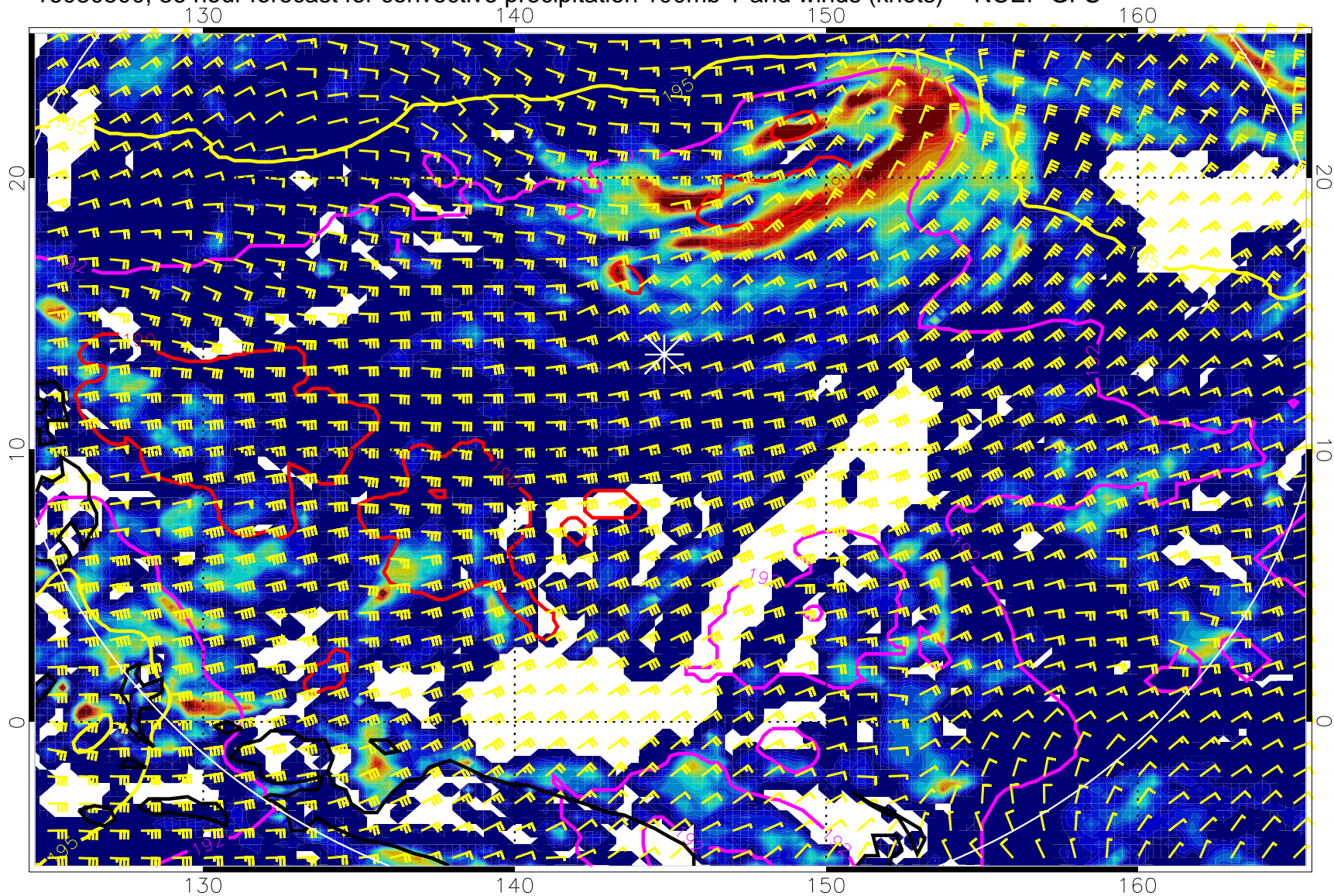
16080500, 36 hour forecast for convective precipitation 100mb T and winds (knots) -- NCEP GFS
