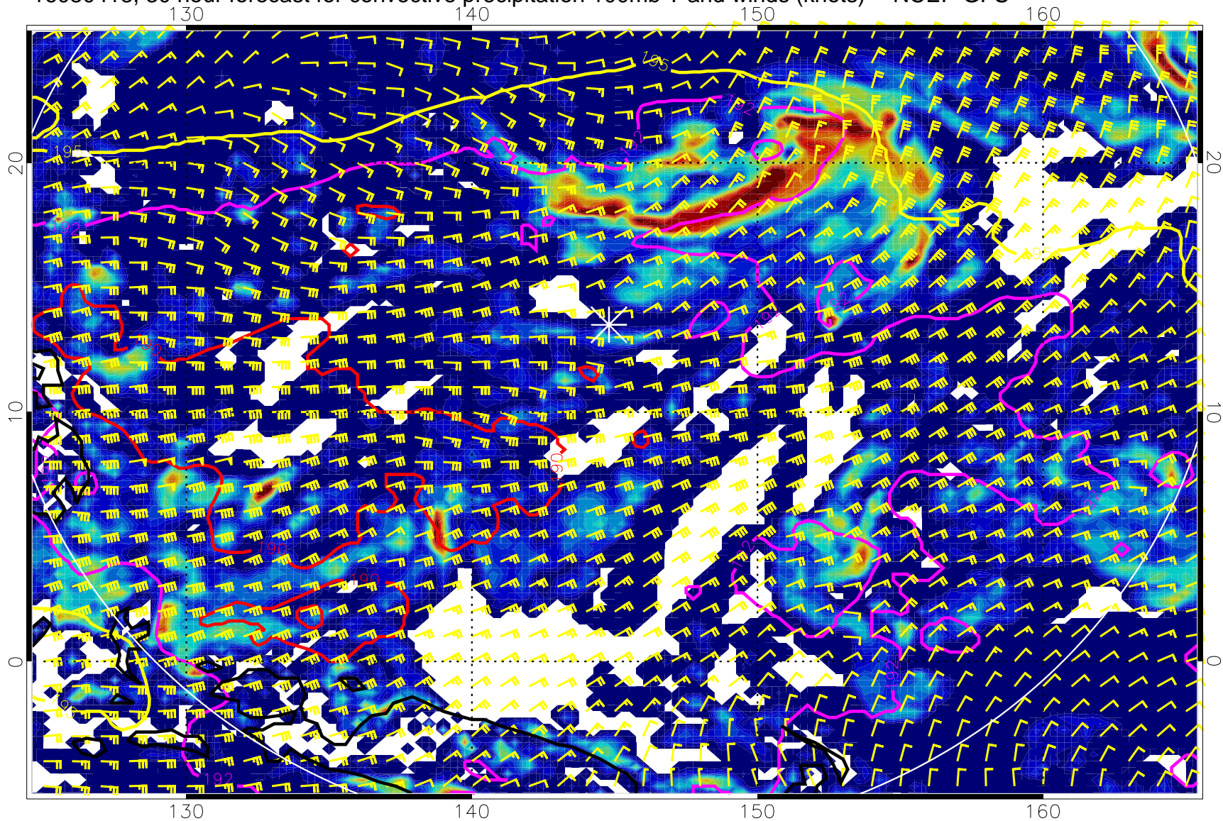
16080418, 30 hour forecast for convective precipitation 100mb T and winds (knots) -- NCEP GFS
