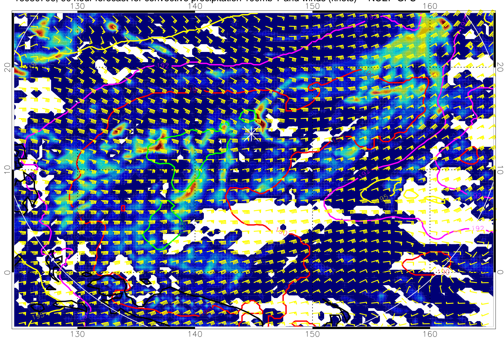
16080706, 90 hour forecast for convective precipitation 100mb T and winds (knots) -- NCEP GFS
