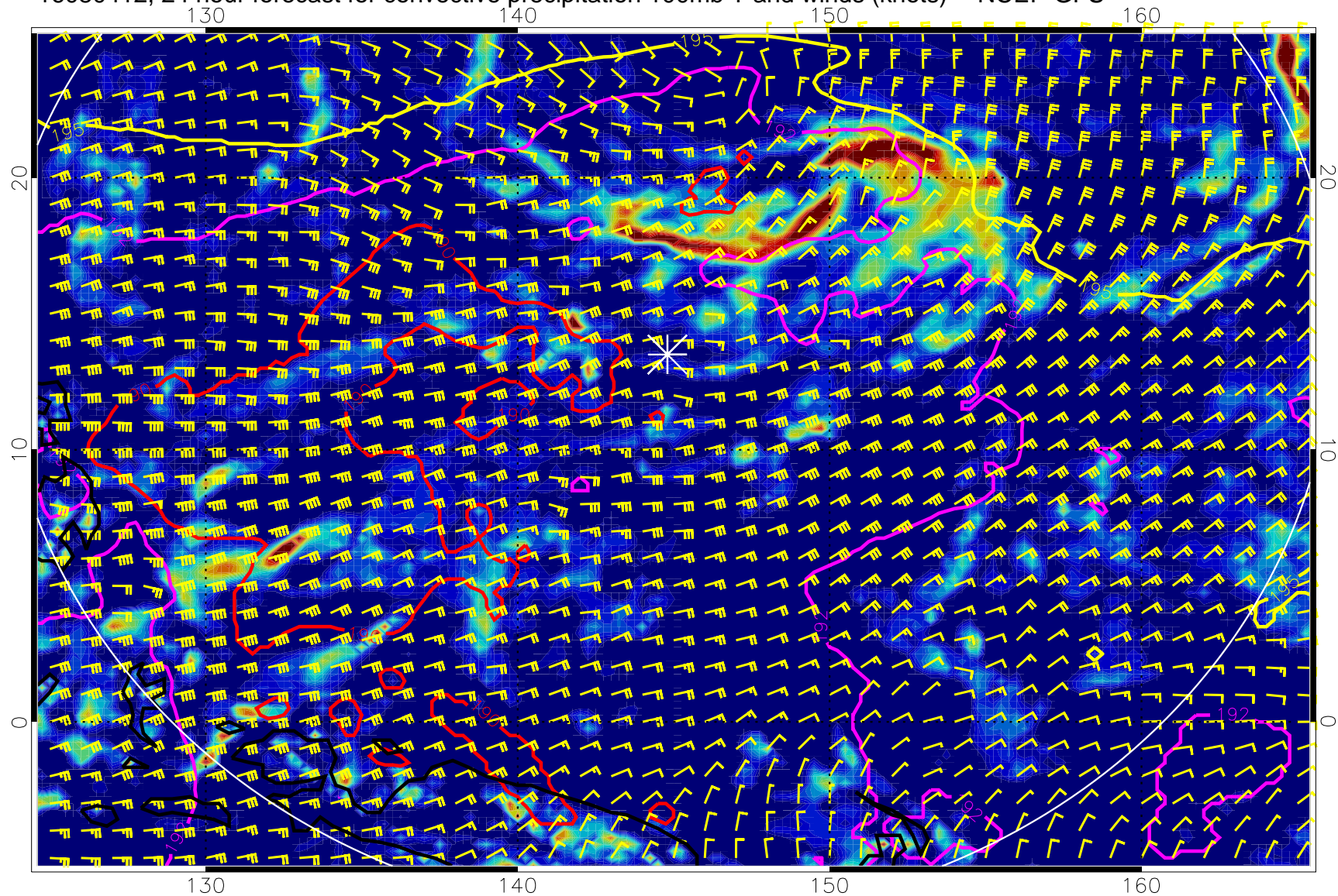
16080412, 24 hour forecast for convective precipitation 100mb T and winds (knots) -- NCEP GFS
