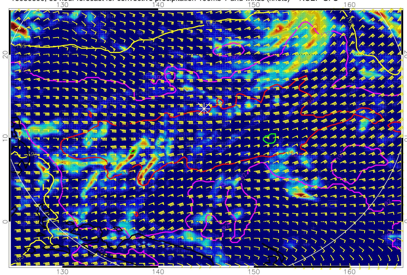
16080600, 60 hour forecast for convective precipitation 100mb T and winds (knots) -- NCEP GFS
