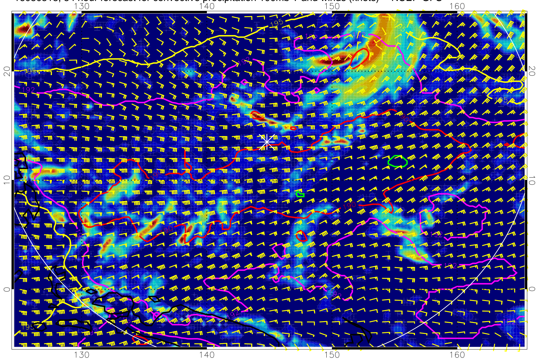
16080518, 54 hour forecast for convective precipitation 100mb T and winds (knots) -- NCEP GFS
