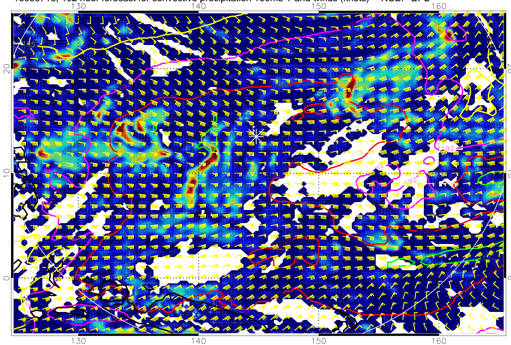
16080718, 102 hour forecast for convective precipitation 100mb T and winds (knots) -- NCEP GFS
