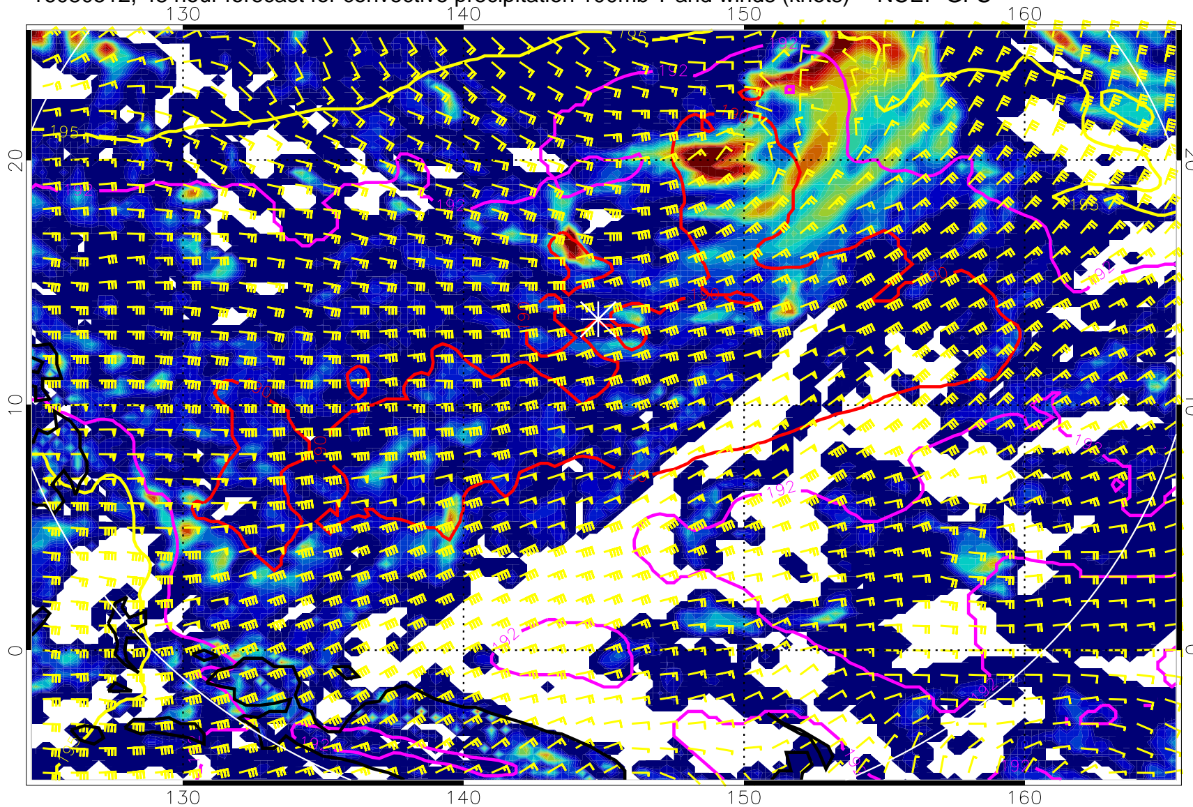
16080512, 48 hour forecast for convective precipitation 100mb T and winds (knots) -- NCEP GFS
