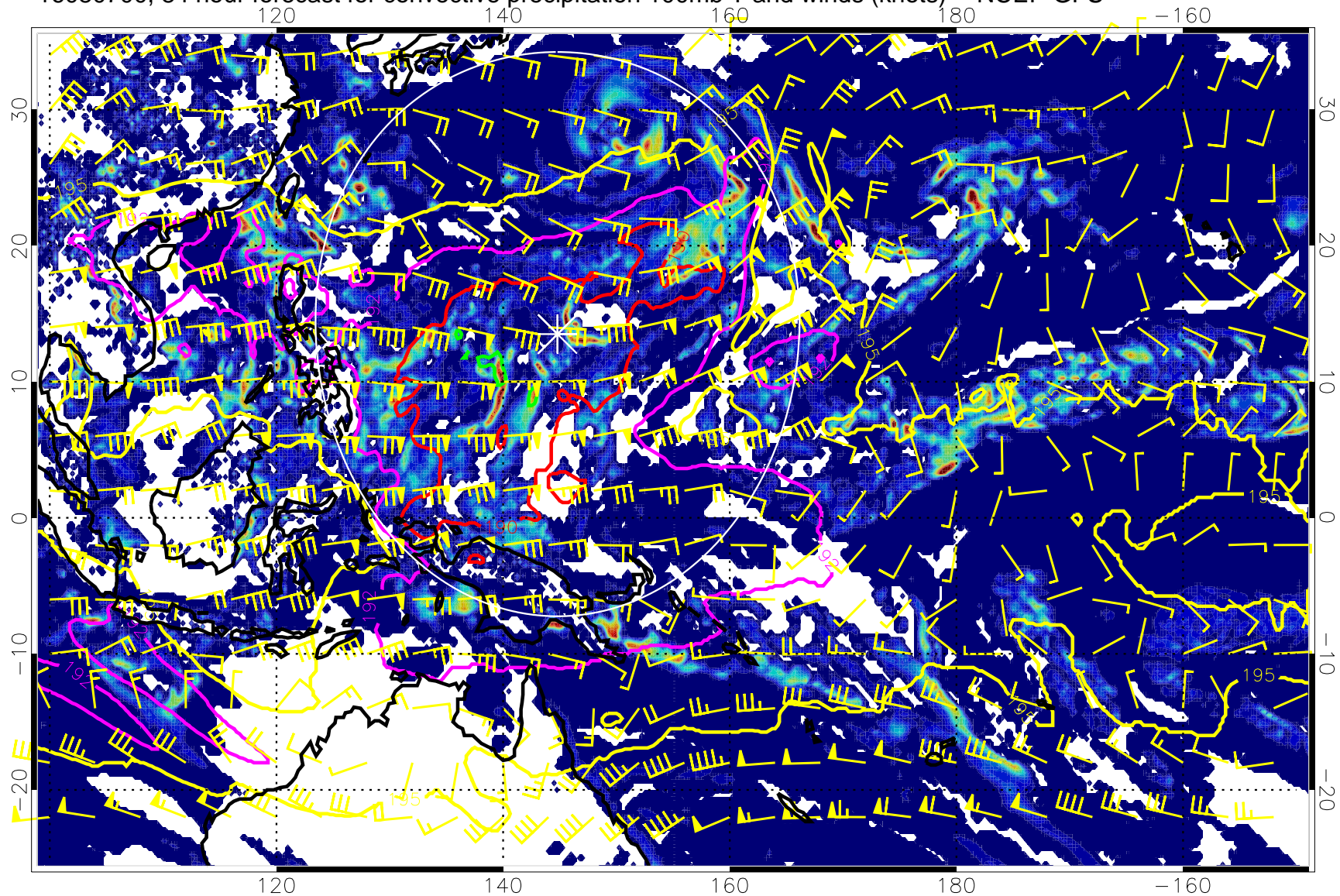
16080700, 84 hour forecast for convective precipitation 100mb T and winds (knots) -- NCEP GFS
