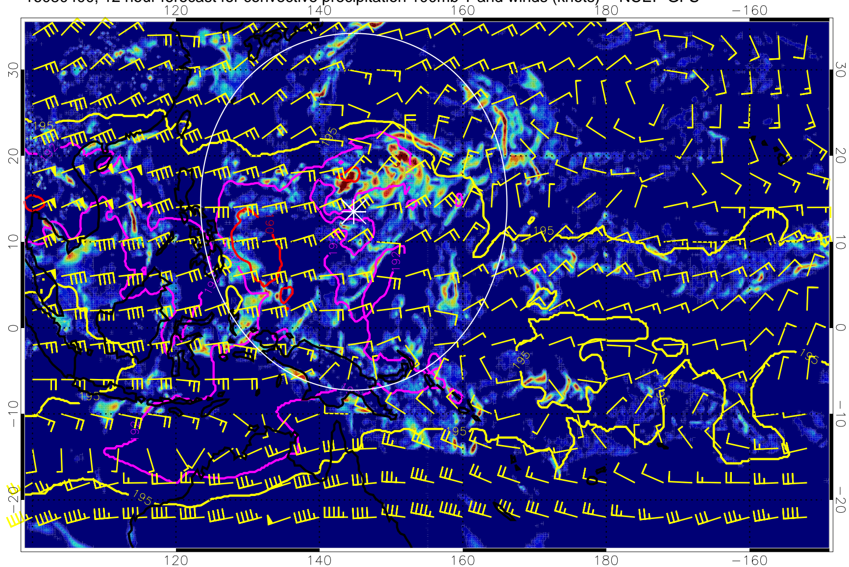
16080400, 12 hour forecast for convective precipitation 100mb T and winds (knots) -- NCEP GFS
