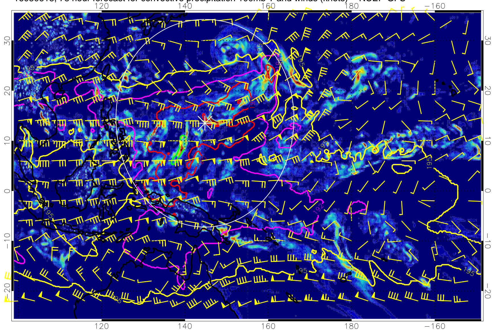
16080618, 78 hour forecast for convective precipitation 100mb T and winds (knots) -- NCEP GFS
