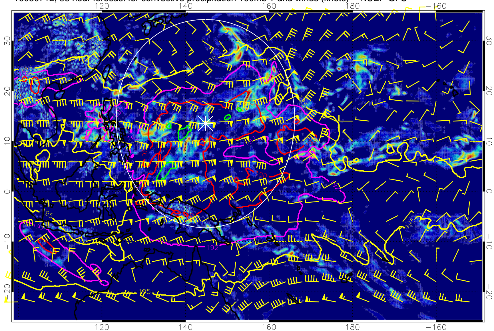
16080712, 96 hour forecast for convective precipitation 100mb T and winds (knots) -- NCEP GFS
