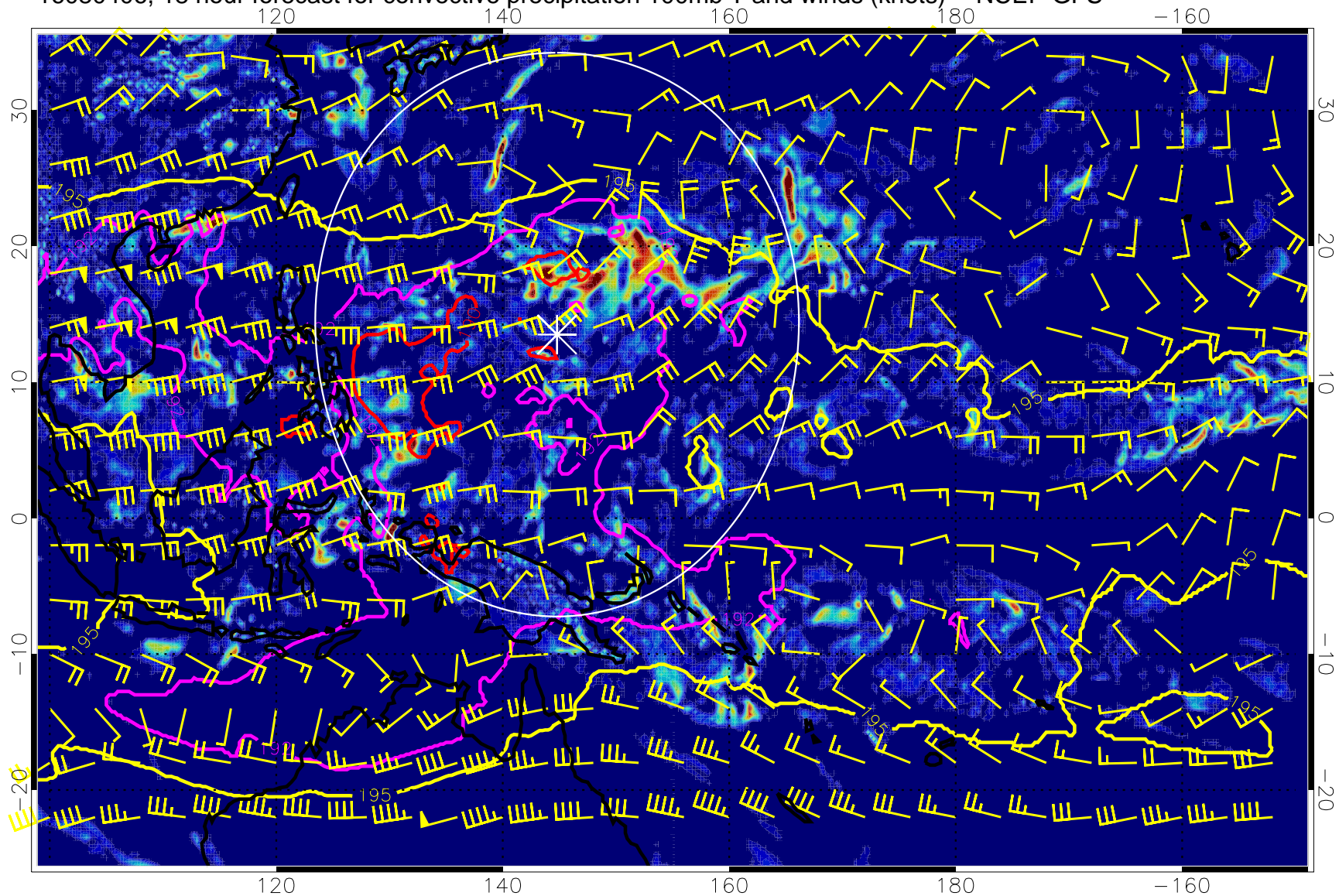
16080406, 18 hour forecast for convective precipitation 100mb T and winds (knots) -- NCEP GFS
