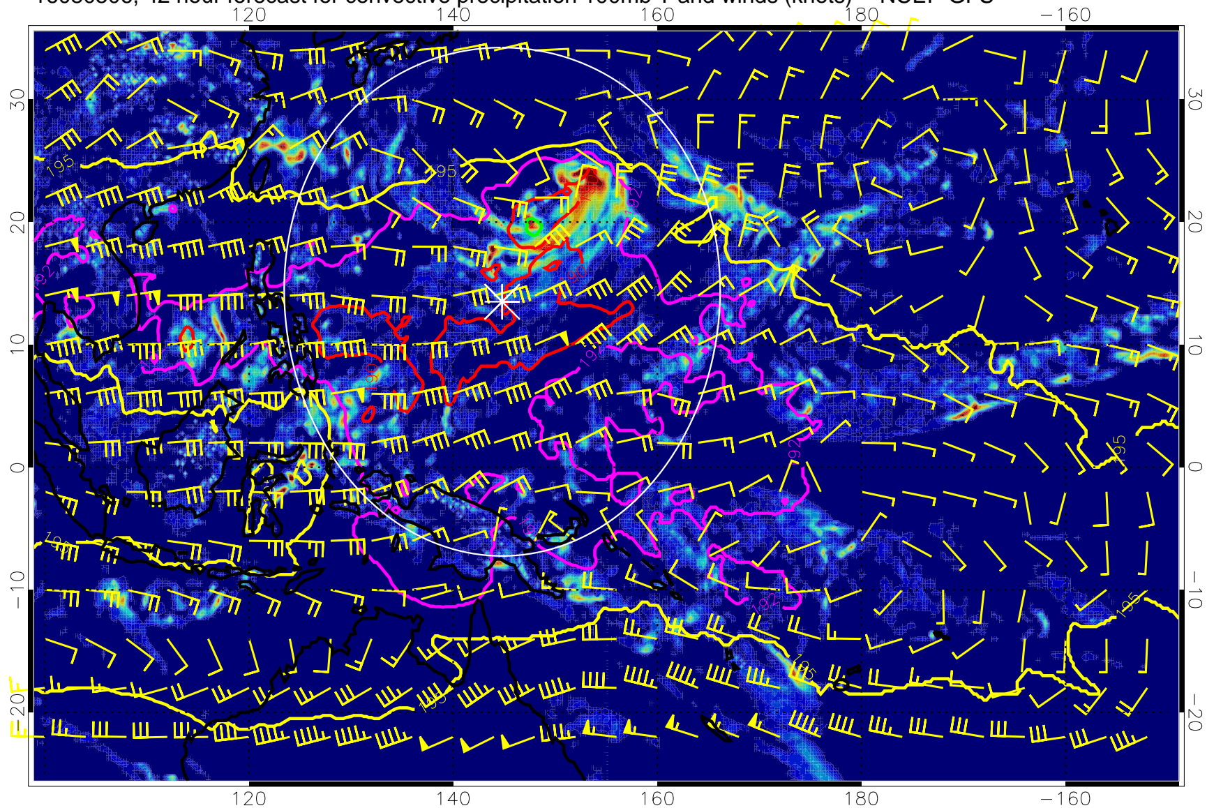
16080506, 42 hour forecast for convective precipitation 100mb T and winds (knots) -- NCEP GFS
