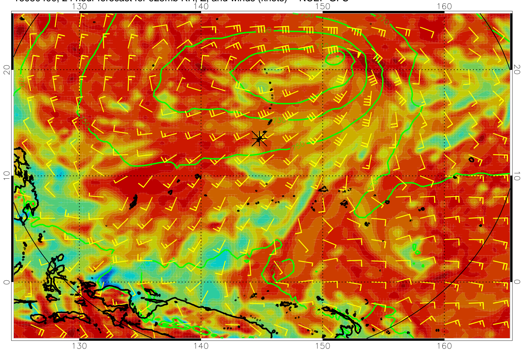
16080400, 24 hour forecast for 925mb RH, Z, and winds (knots) -- NCEP GFS
