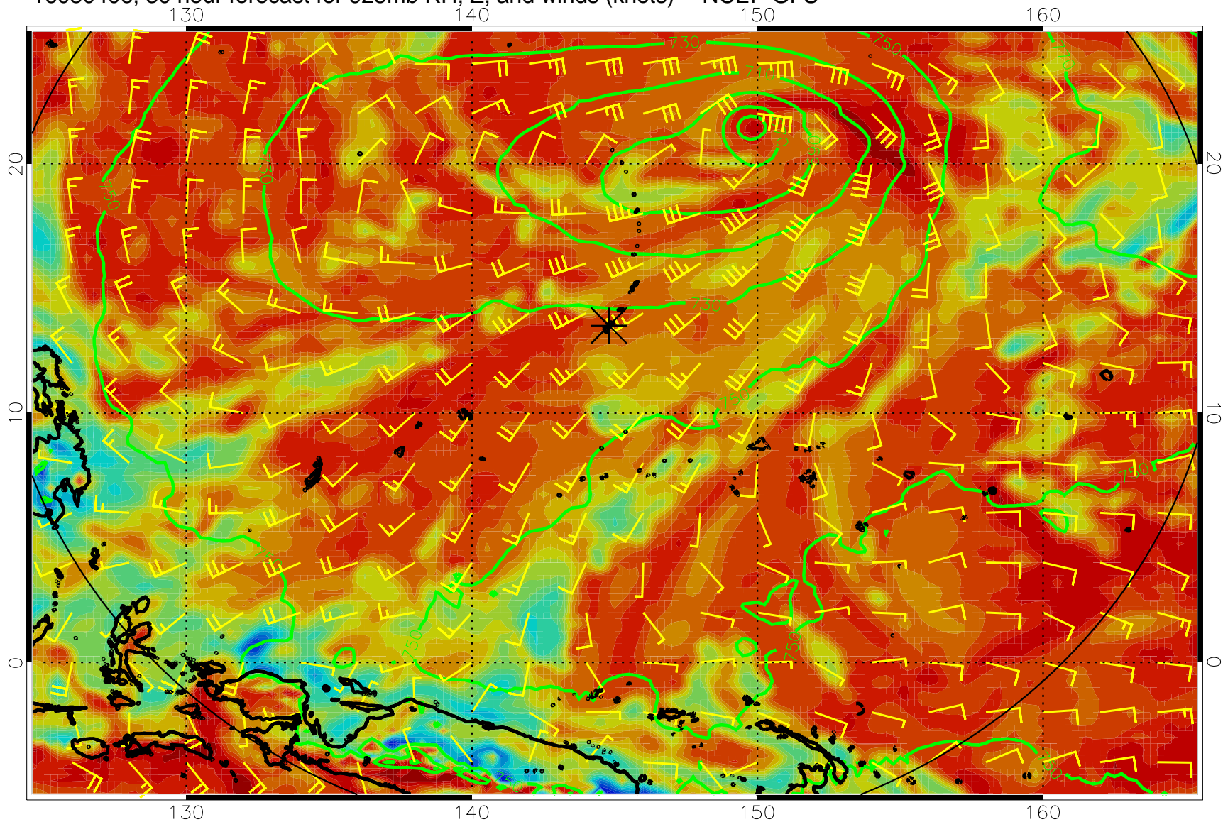
16080406, 30 hour forecast for 925mb RH, Z, and winds (knots) -- NCEP GFS
