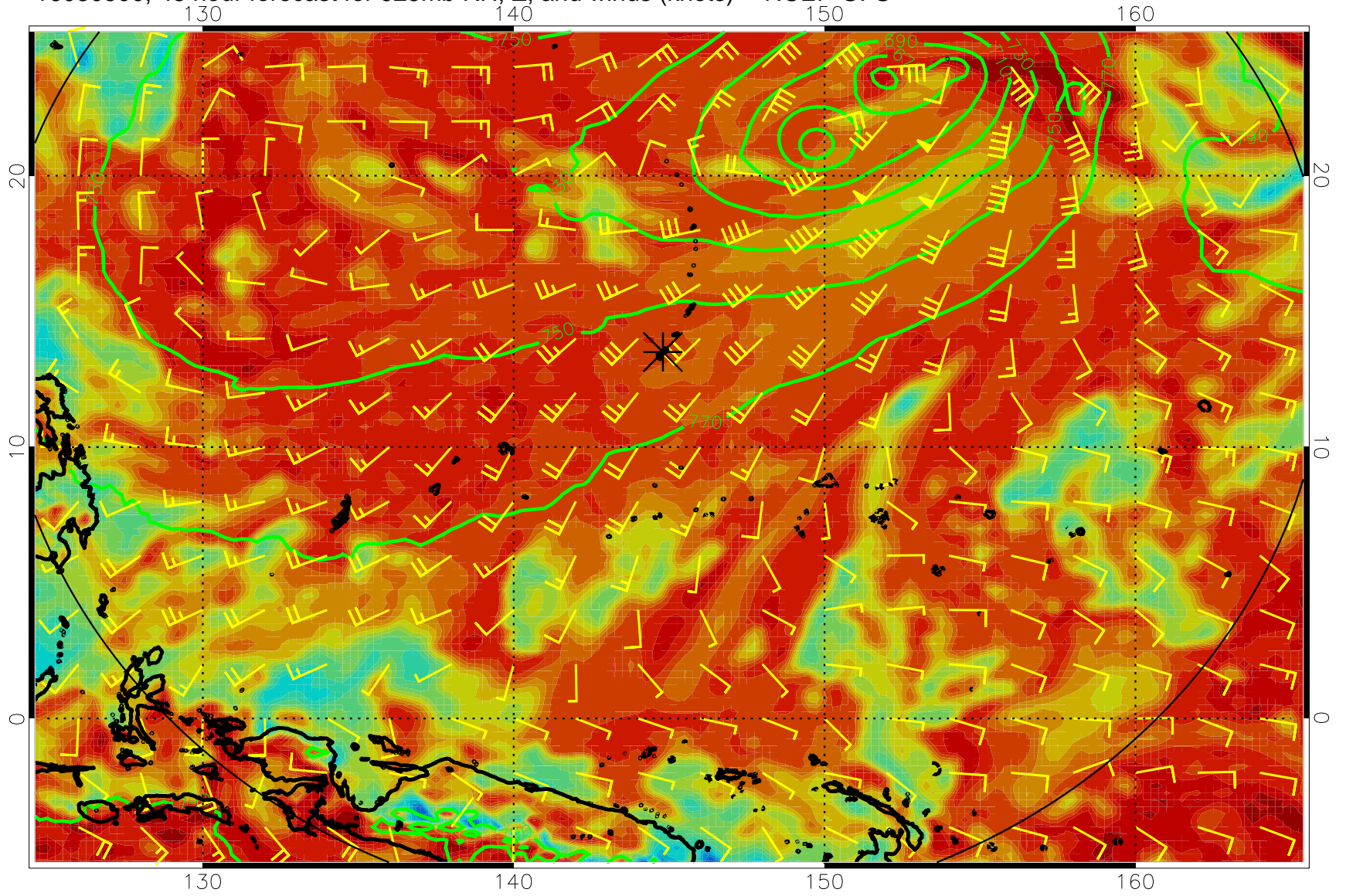
16080500, 48 hour forecast for 925mb RH, Z, and winds (knots) -- NCEP GFS
