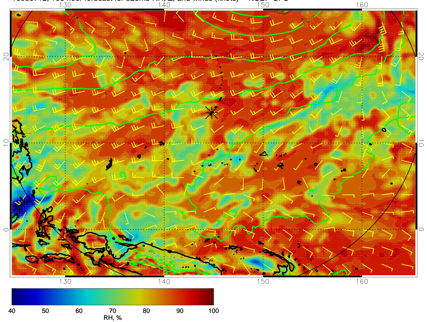
16080712, 108 hour forecast for 925mb RH, Z, and winds (knots) -- NCEP GFS
