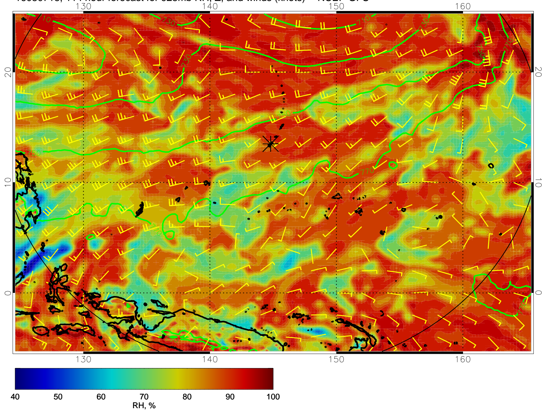
16080718, 114 hour forecast for 925mb RH, Z, and winds (knots) -- NCEP GFS
