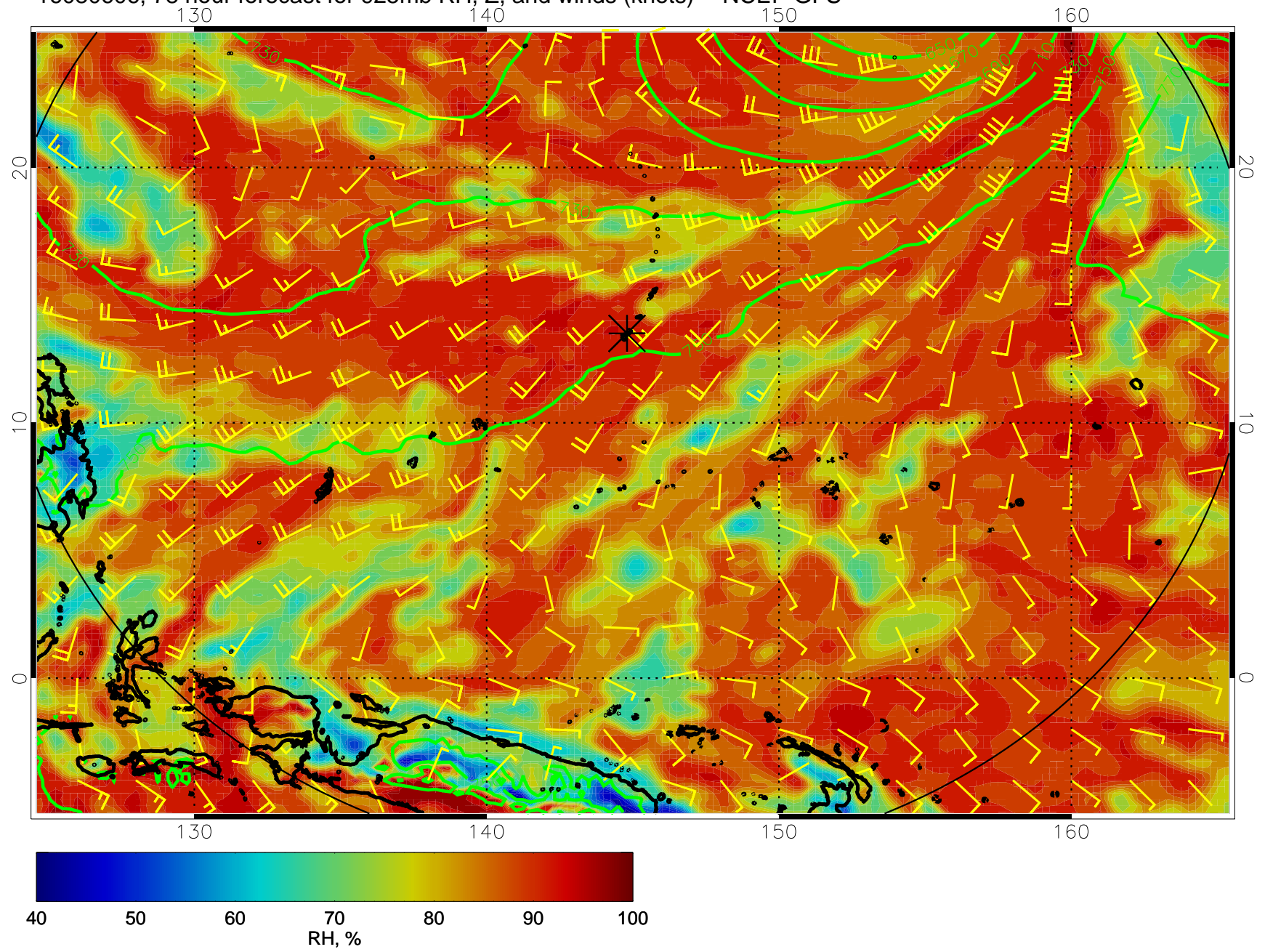
16080606, 78 hour forecast for 925mb RH, Z, and winds (knots) -- NCEP GFS
