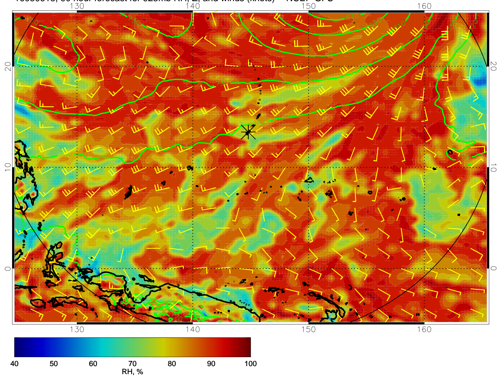
16080618, 90 hour forecast for 925mb RH, Z, and winds (knots) -- NCEP GFS
