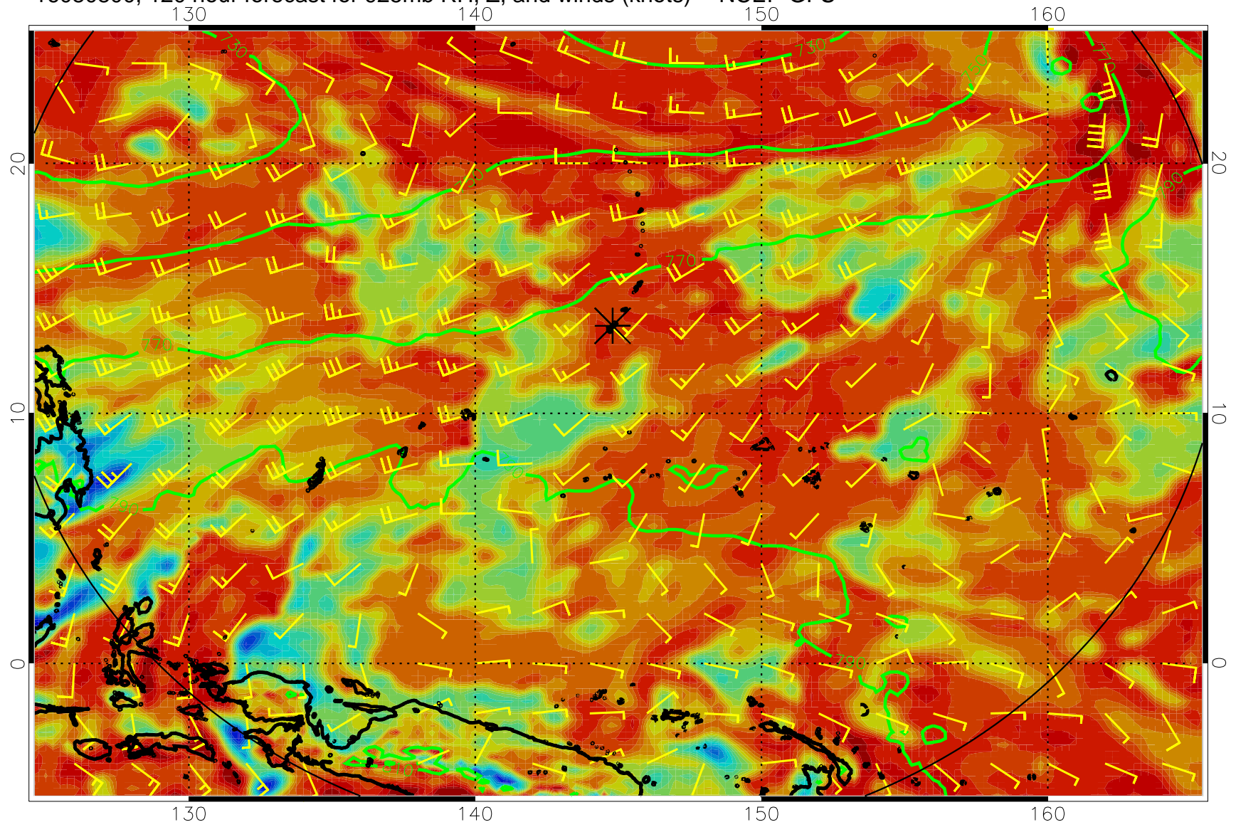
16080800, 120 hour forecast for 925mb RH, Z, and winds (knots) -- NCEP GFS
