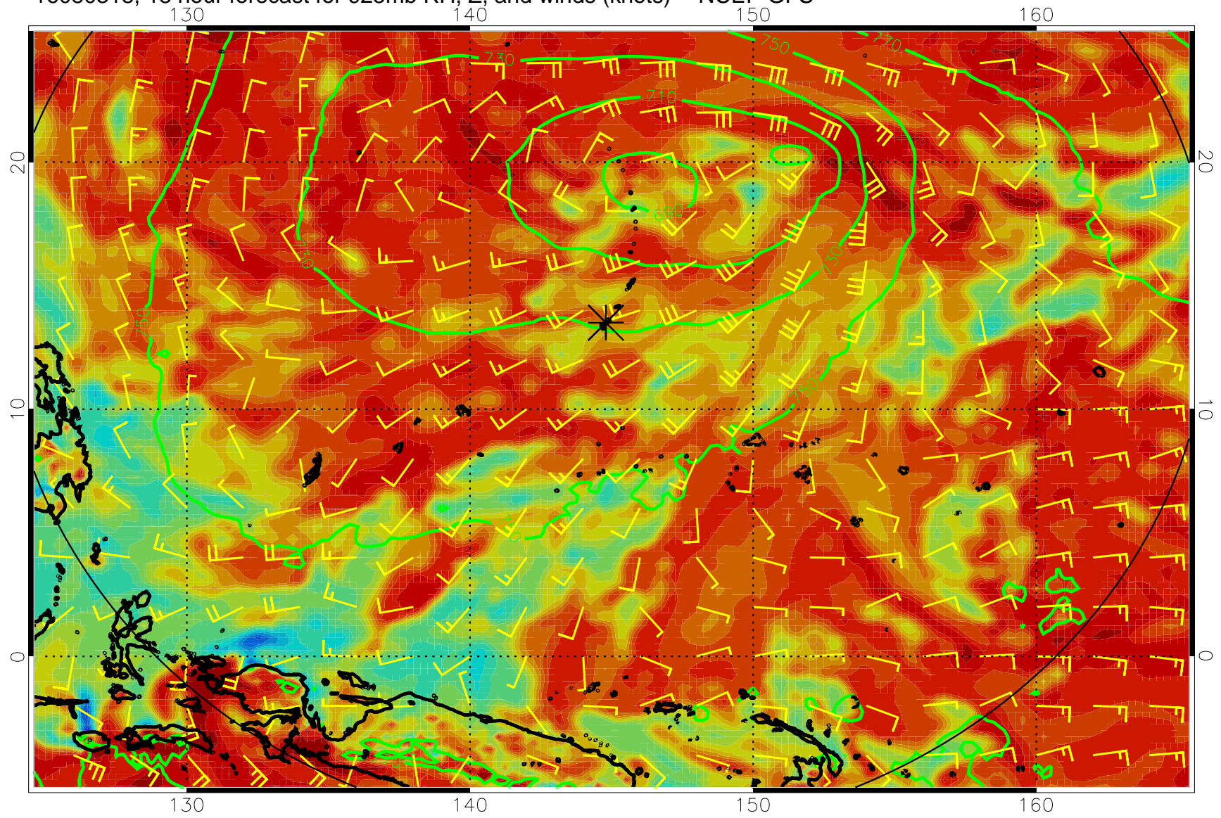
16080318, 18 hour forecast for 925mb RH, Z, and winds (knots) -- NCEP GFS
