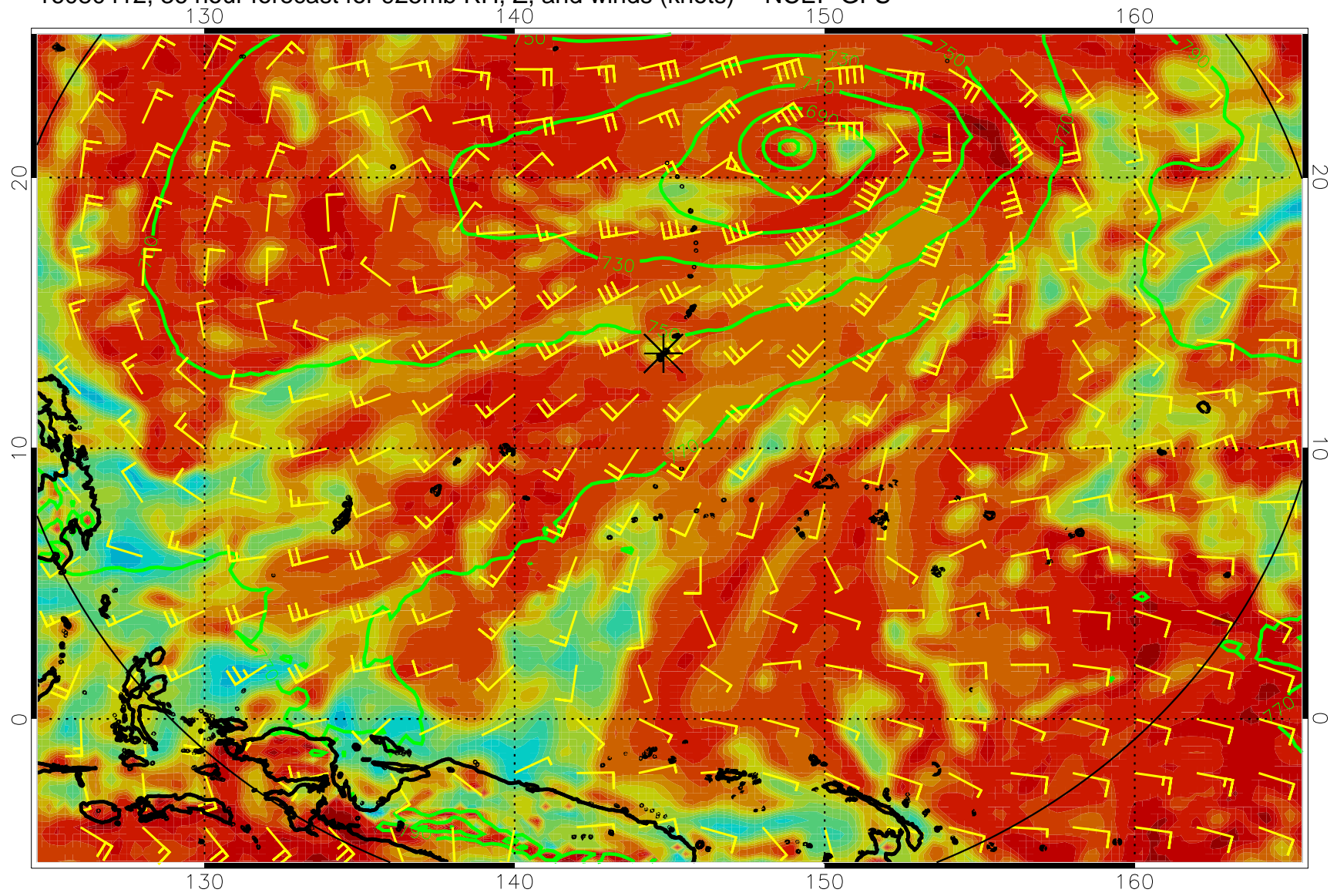
16080412, 36 hour forecast for 925mb RH, Z, and winds (knots) -- NCEP GFS
