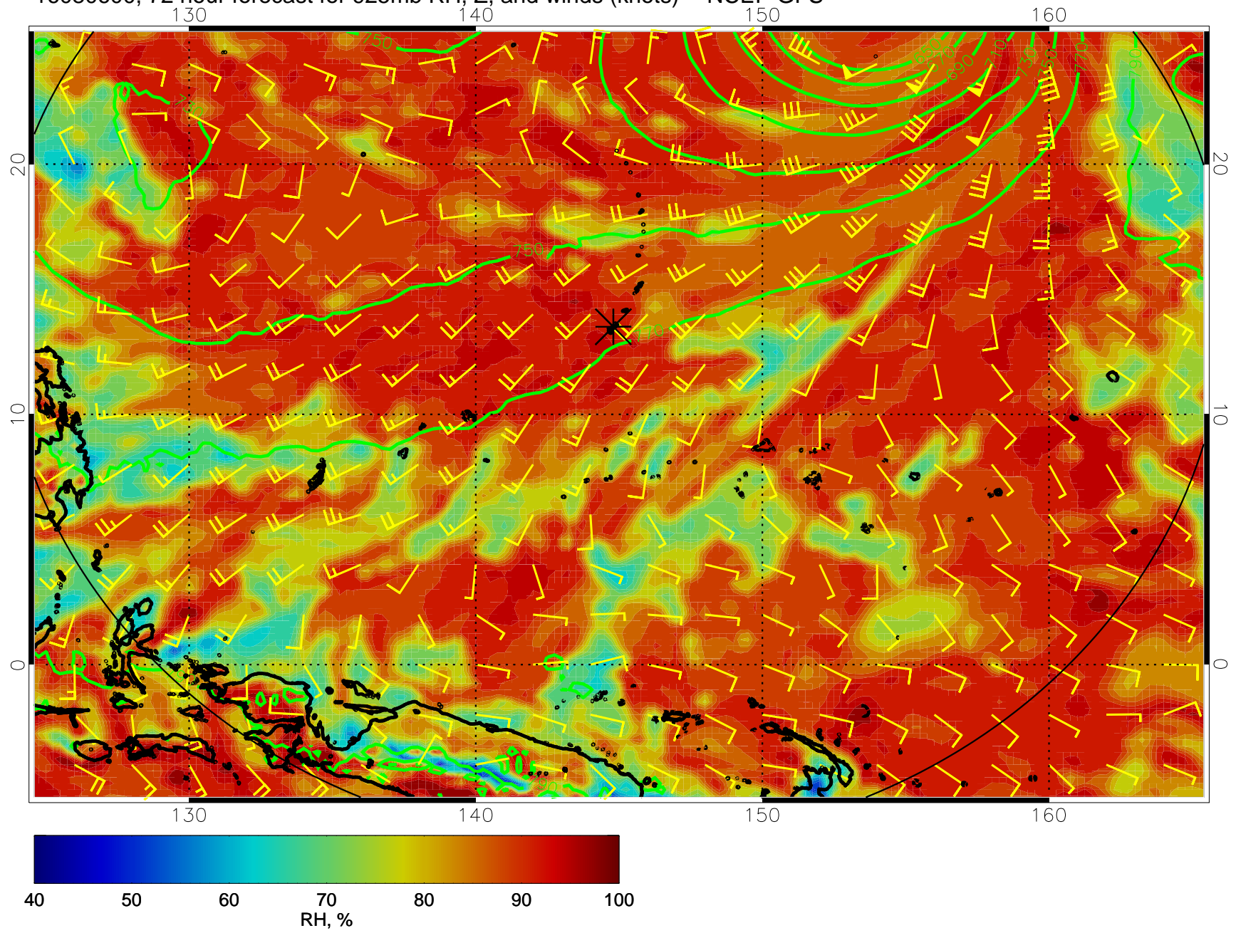
16080600, 72 hour forecast for 925mb RH, Z, and winds (knots) -- NCEP GFS
