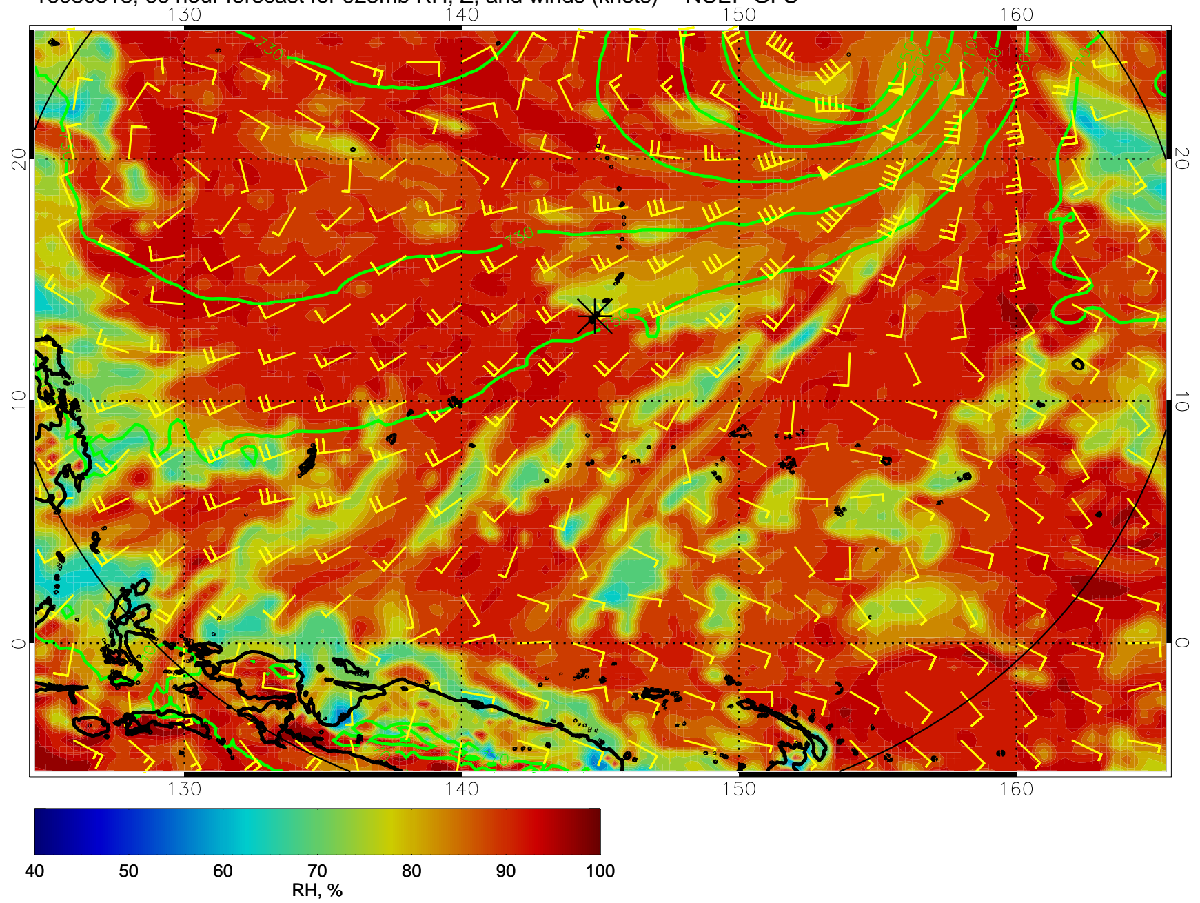
16080518, 66 hour forecast for 925mb RH, Z, and winds (knots) -- NCEP GFS
