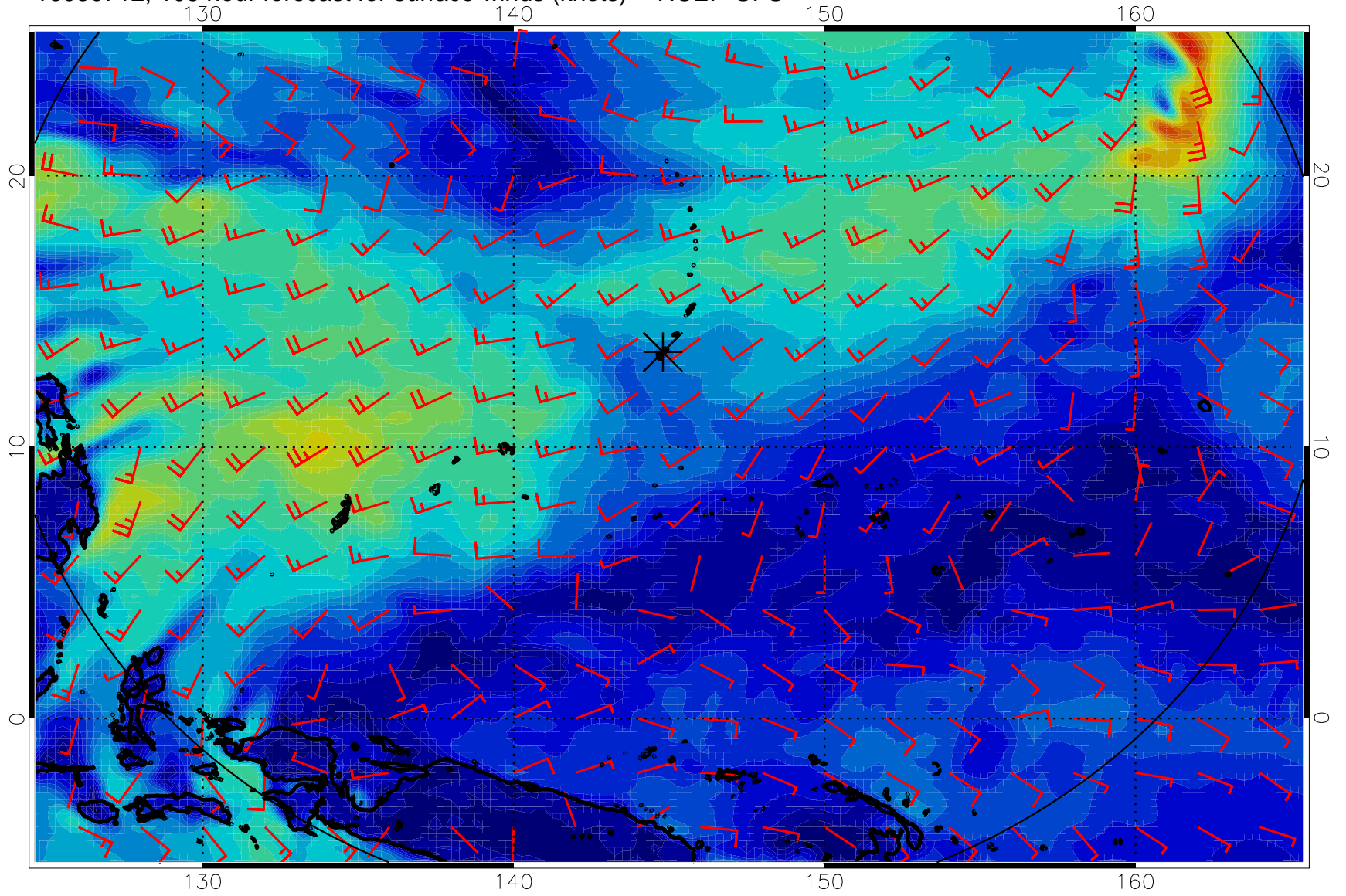
16080712, 108 hour forecast for surface winds (knots) -- NCEP GFS
