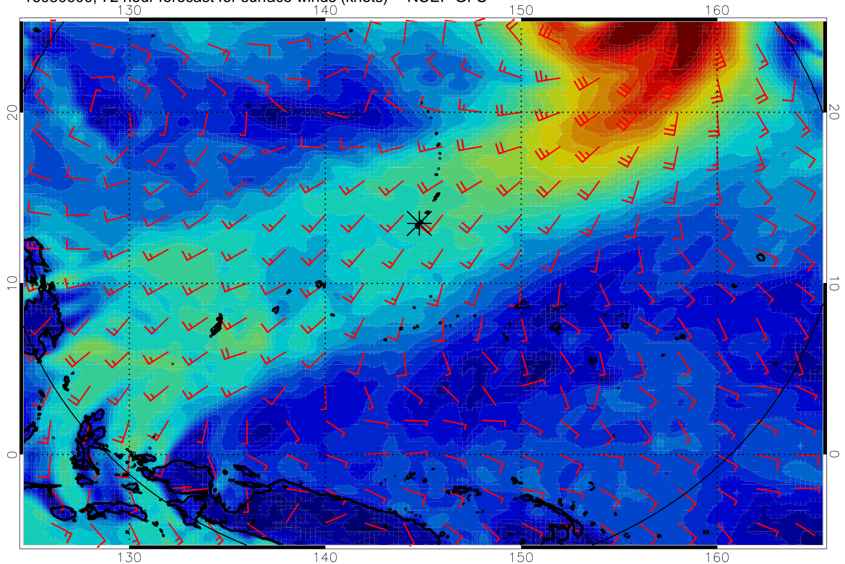
16080600, 72 hour forecast for surface winds (knots) -- NCEP GFS
