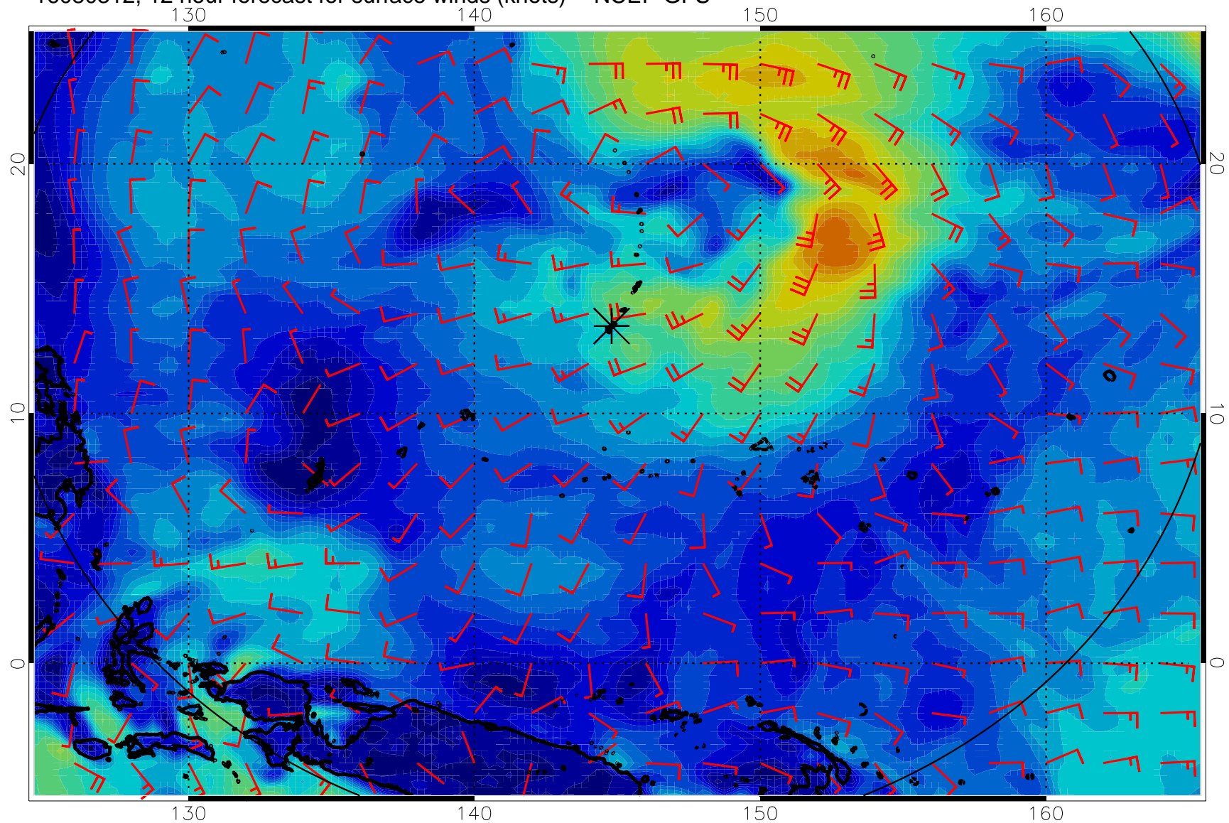
16080312, 12 hour forecast for surface winds (knots) -- NCEP GFS
