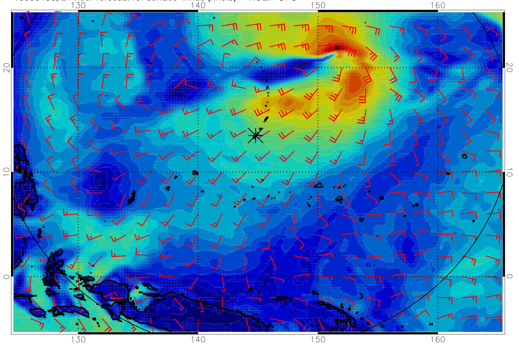
16080400, 24 hour forecast for surface winds (knots) -- NCEP GFS
