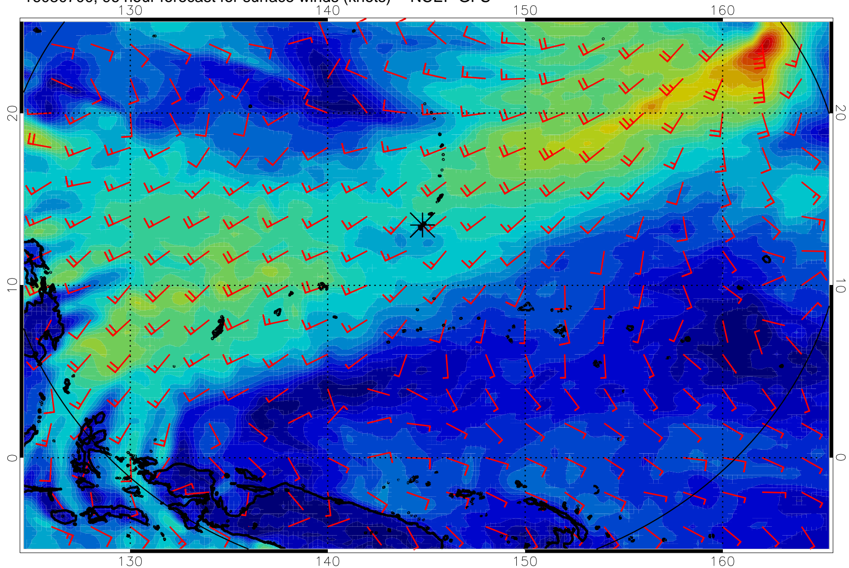
16080700, 96 hour forecast for surface winds (knots) -- NCEP GFS
