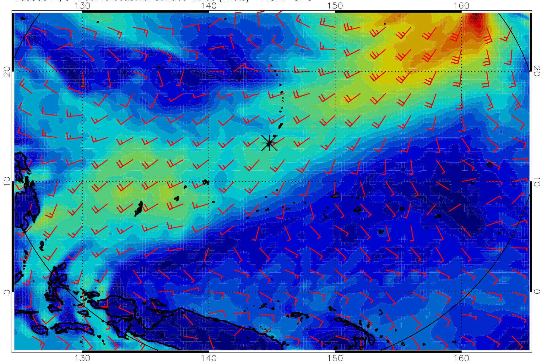
16080612, 84 hour forecast for surface winds (knots) -- NCEP GFS
