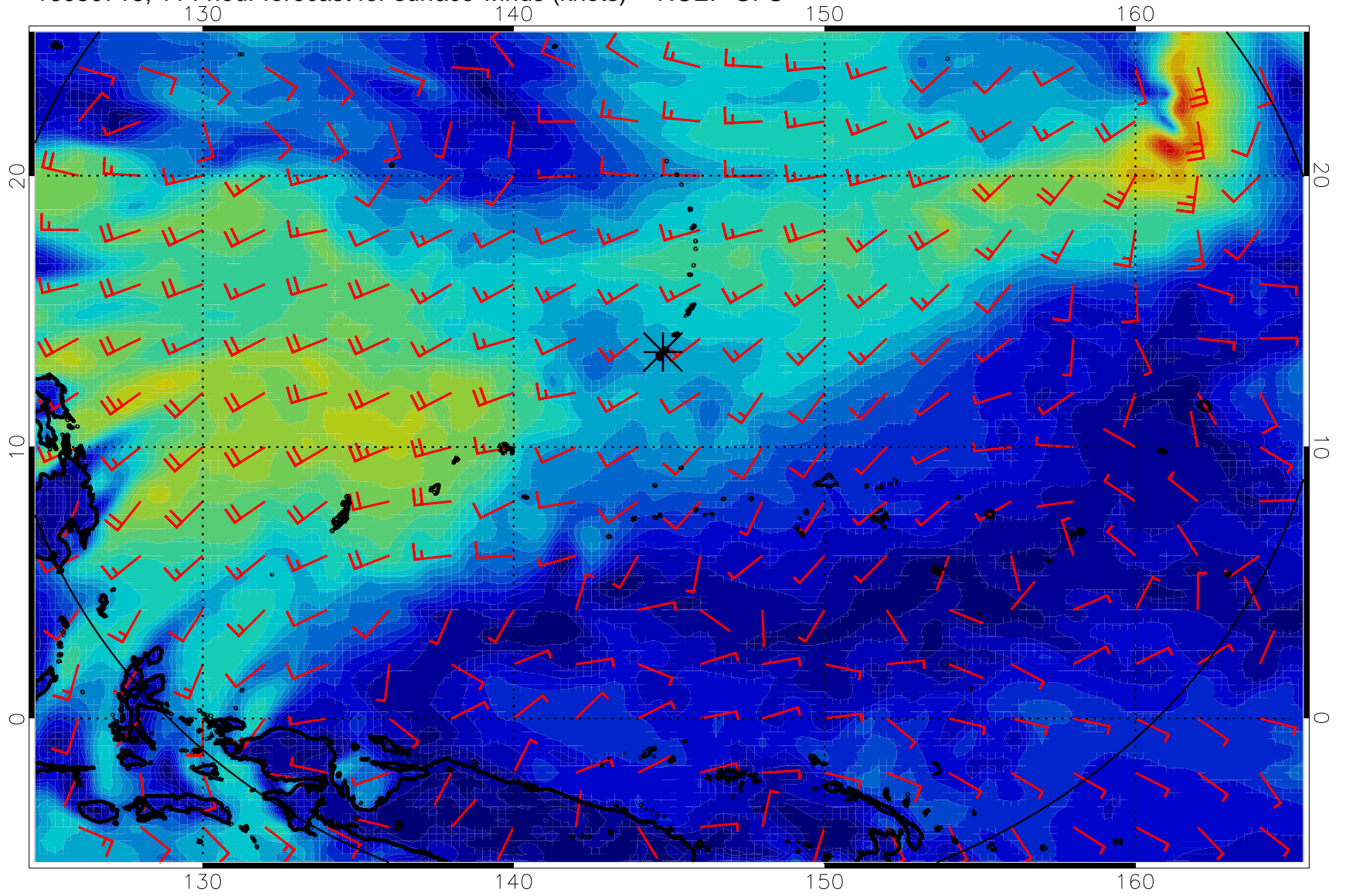
16080718, 114 hour forecast for surface winds (knots) -- NCEP GFS
