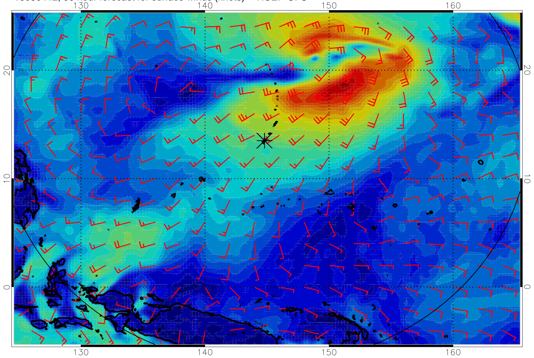
16080412, 36 hour forecast for surface winds (knots) -- NCEP GFS
