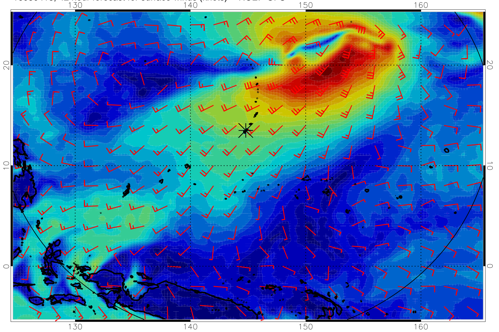
16080418, 42 hour forecast for surface winds (knots) -- NCEP GFS
