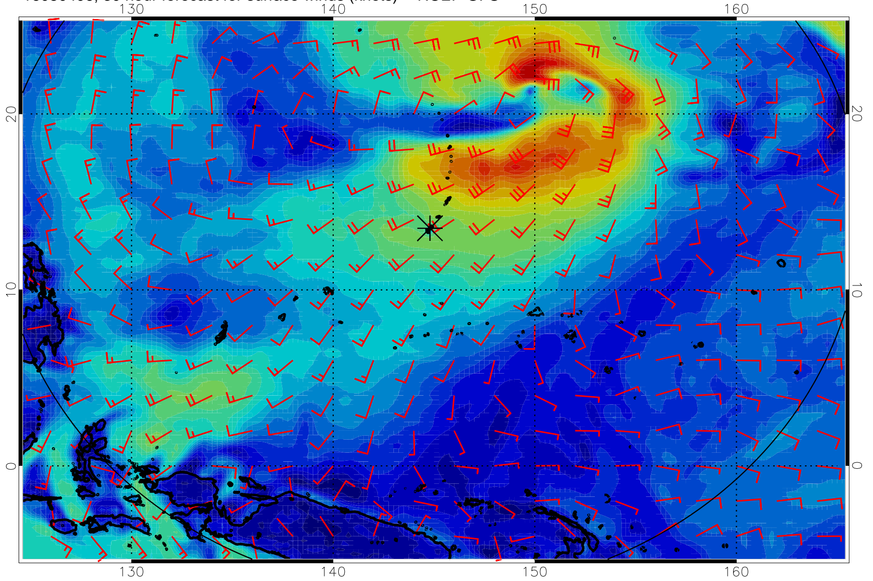
16080406, 30 hour forecast for surface winds (knots) -- NCEP GFS
