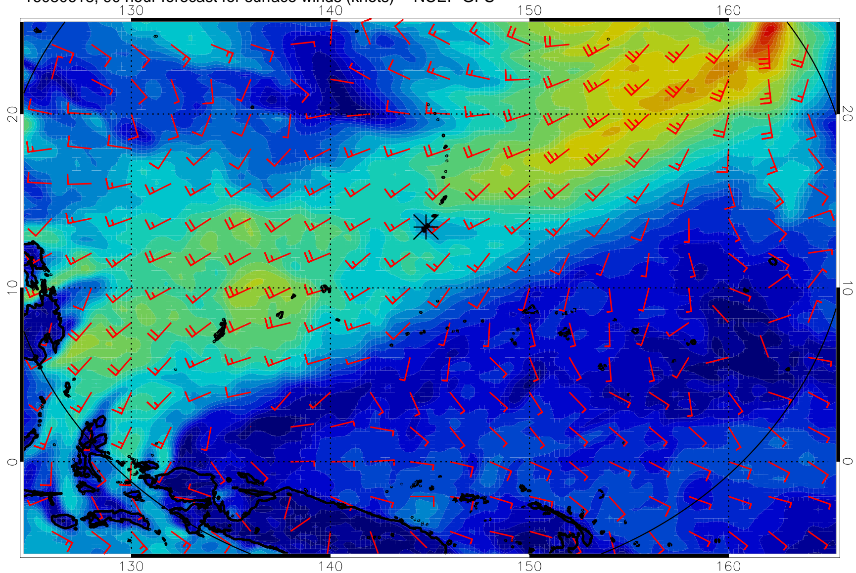
16080618, 90 hour forecast for surface winds (knots) -- NCEP GFS
