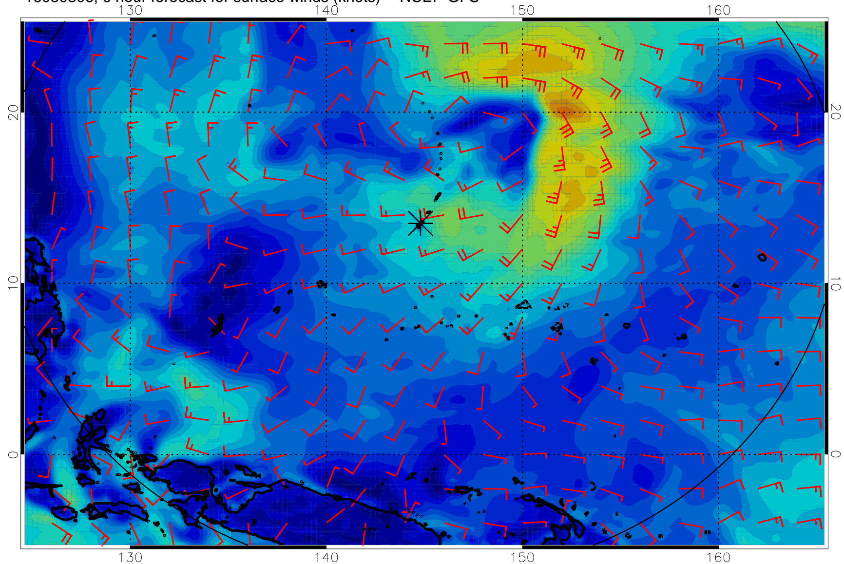
16080306, 6 hour forecast for surface winds (knots) -- NCEP GFS
