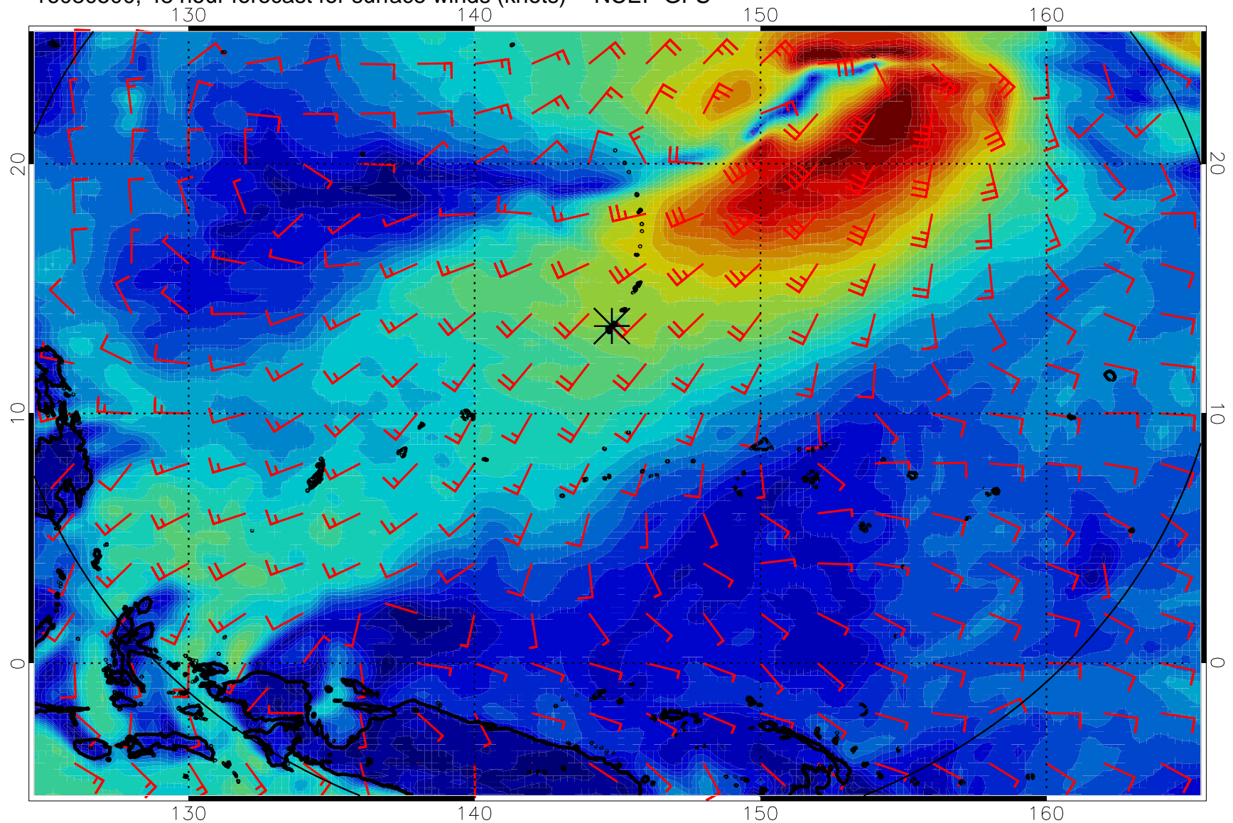
16080500, 48 hour forecast for surface winds (knots) -- NCEP GFS
