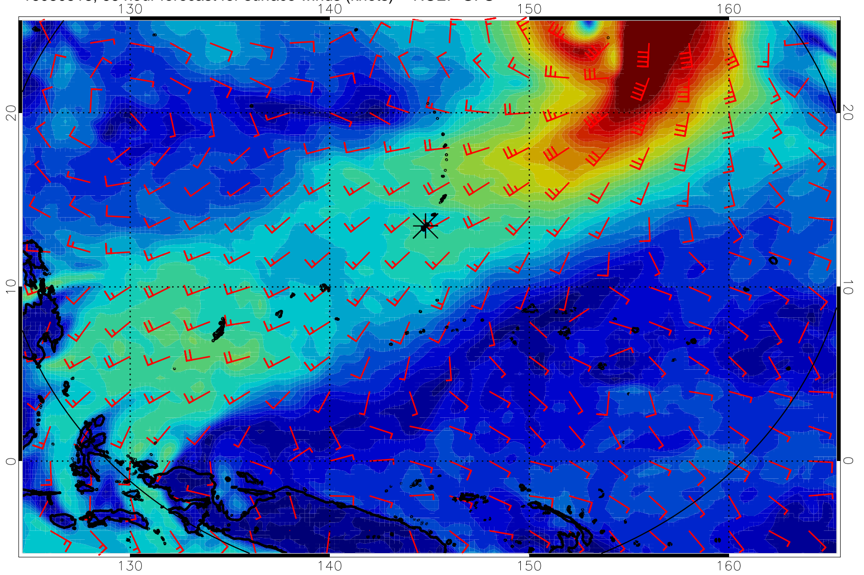
16080518, 66 hour forecast for surface winds (knots) -- NCEP GFS
