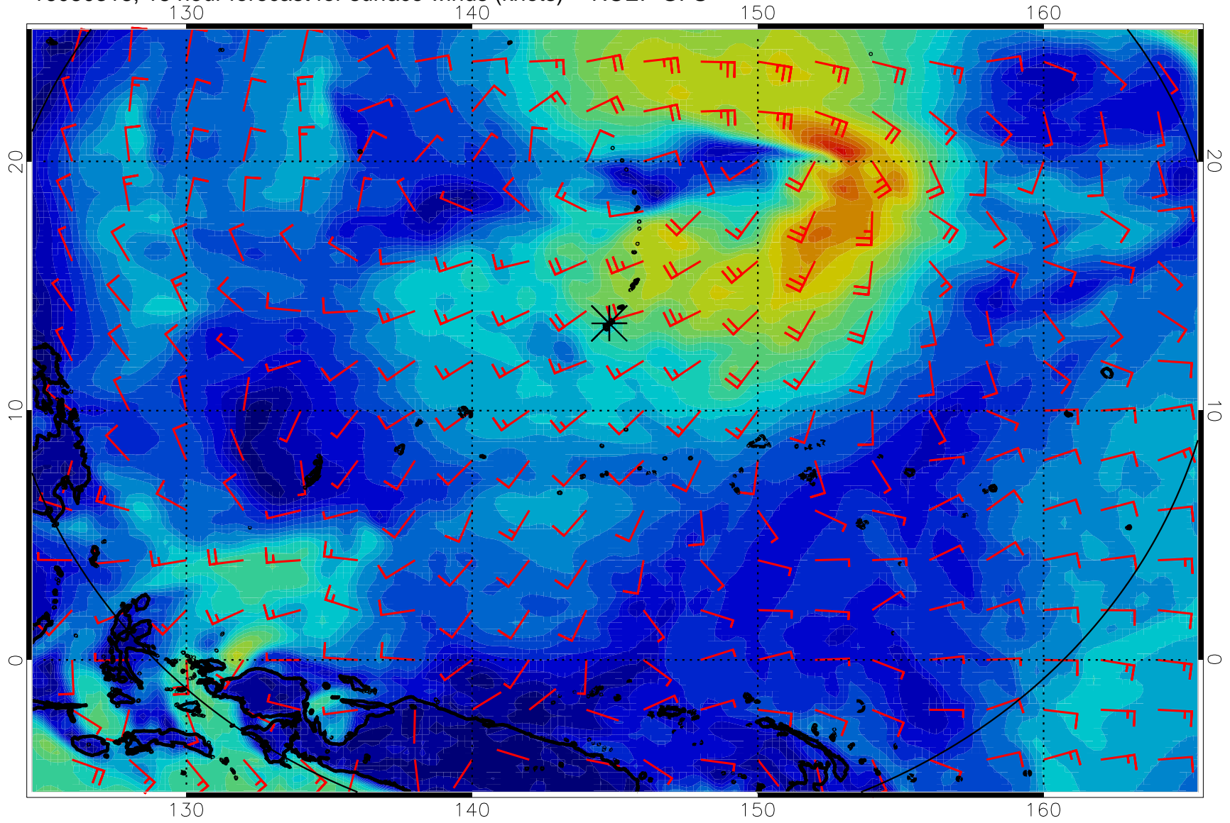
16080318, 18 hour forecast for surface winds (knots) -- NCEP GFS
