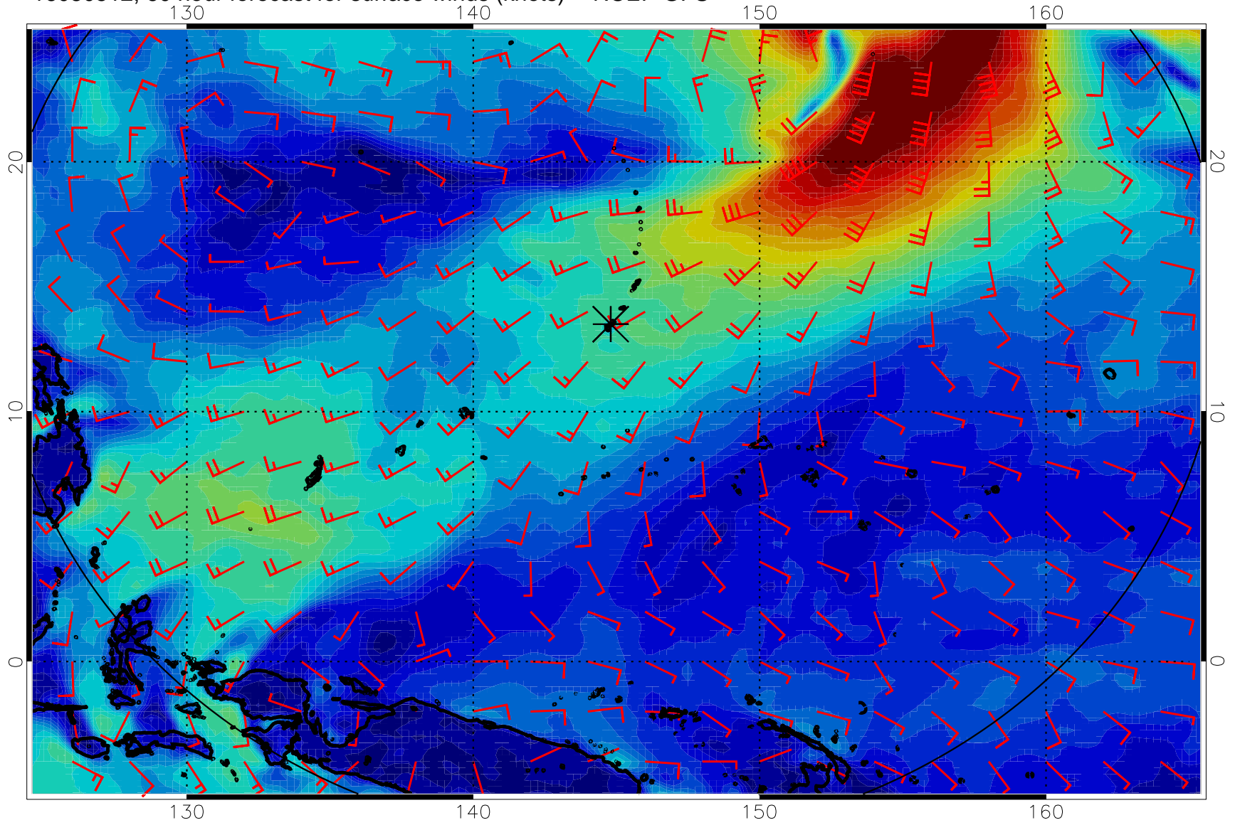
16080512, 60 hour forecast for surface winds (knots) -- NCEP GFS
