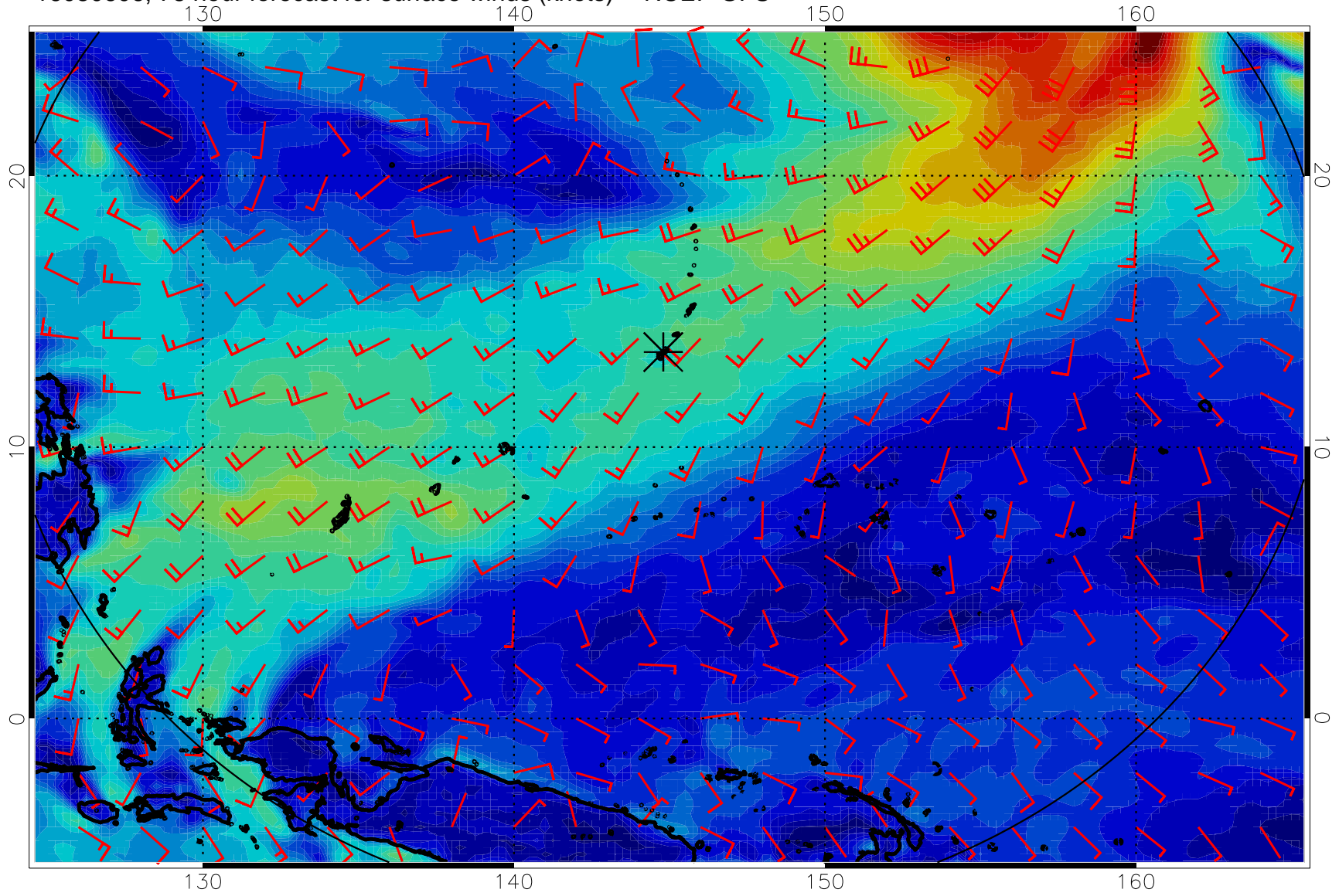
16080606, 78 hour forecast for surface winds (knots) -- NCEP GFS
