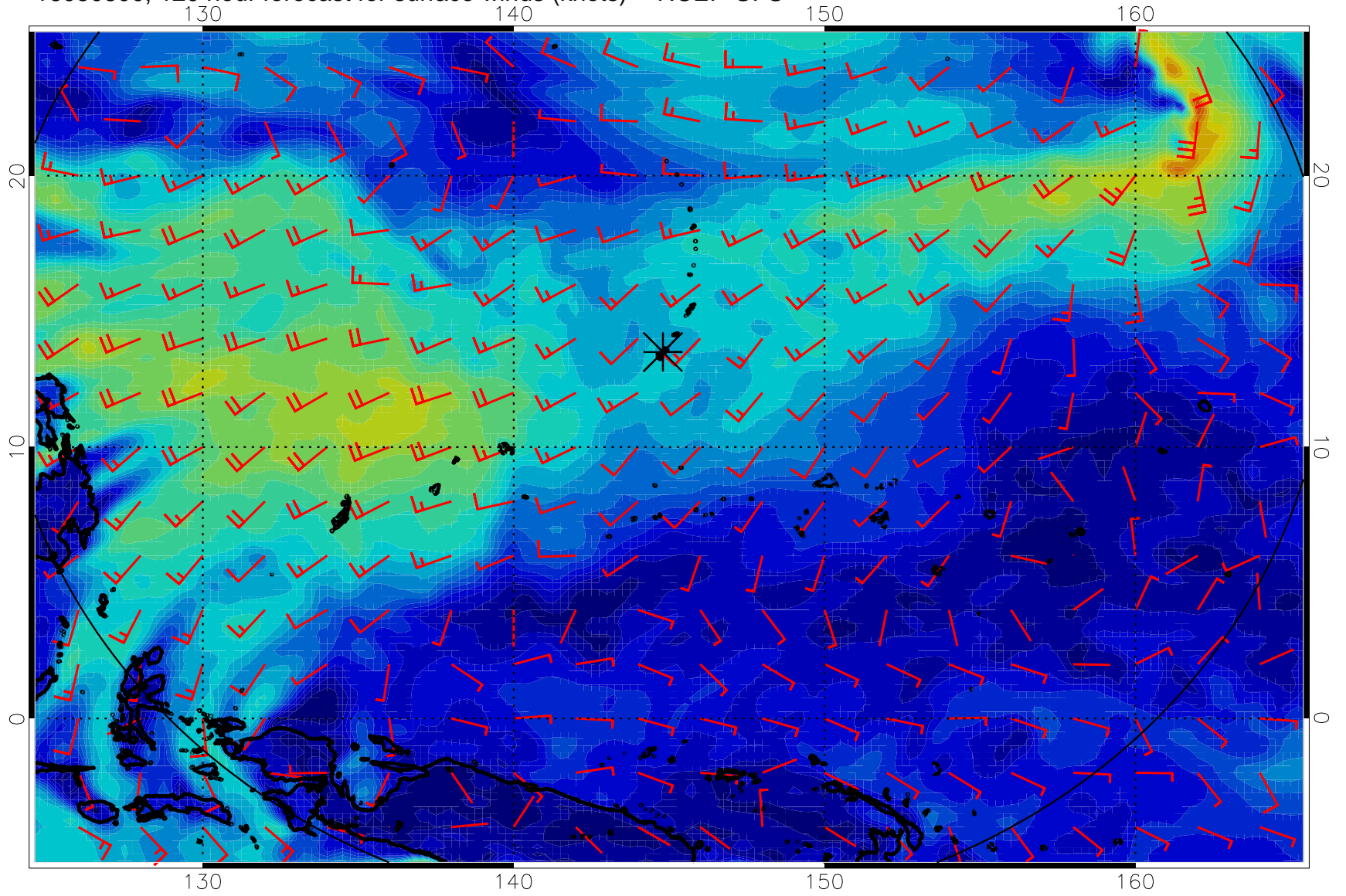
16080800, 120 hour forecast for surface winds (knots) -- NCEP GFS
