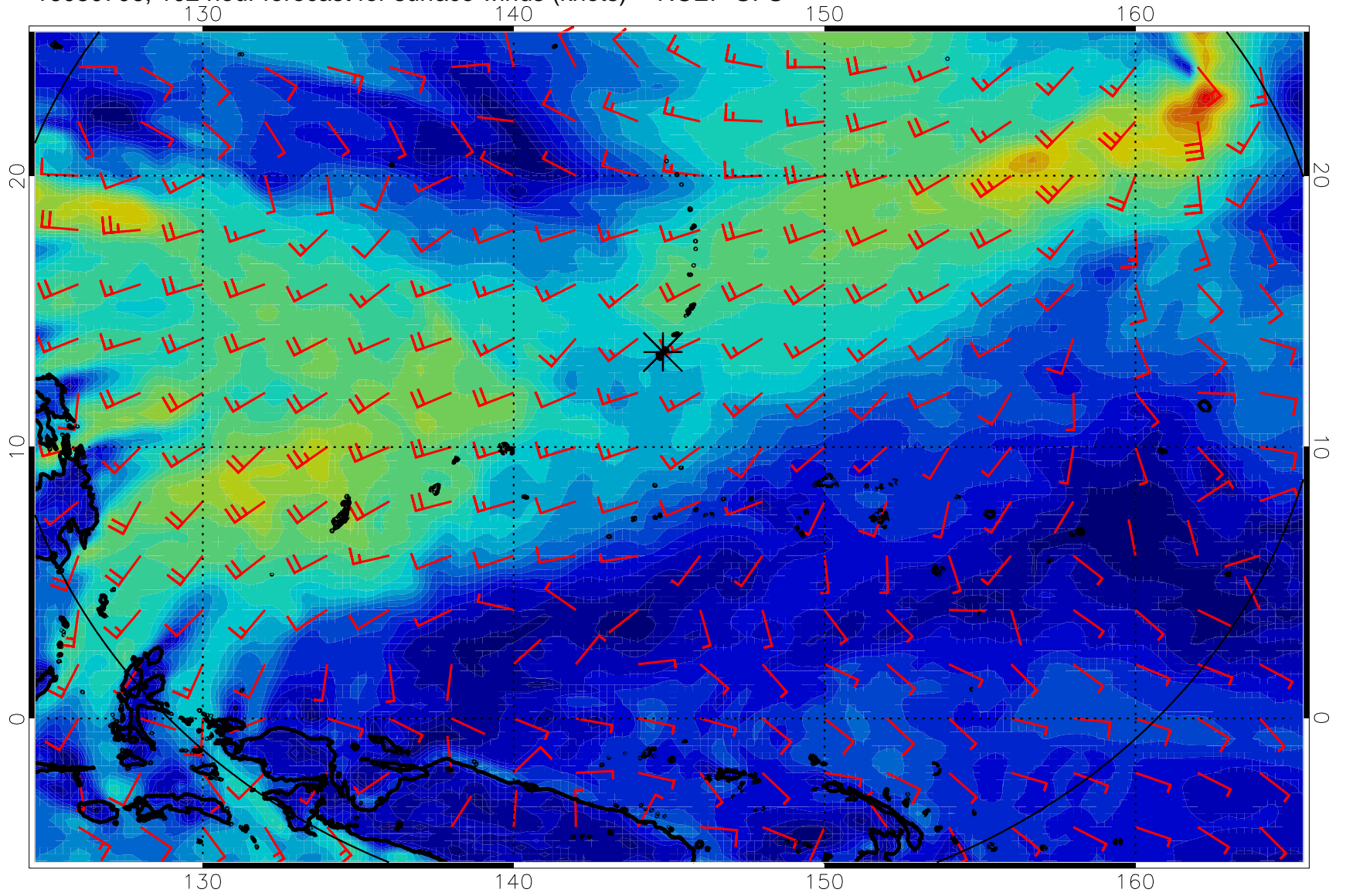
16080706, 102 hour forecast for surface winds (knots) -- NCEP GFS
