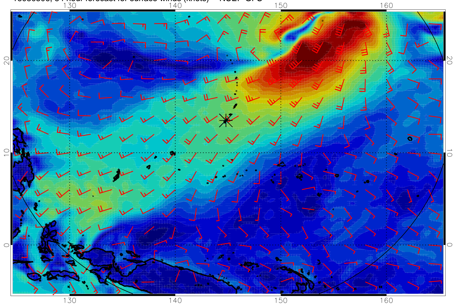
16080506, 54 hour forecast for surface winds (knots) -- NCEP GFS
