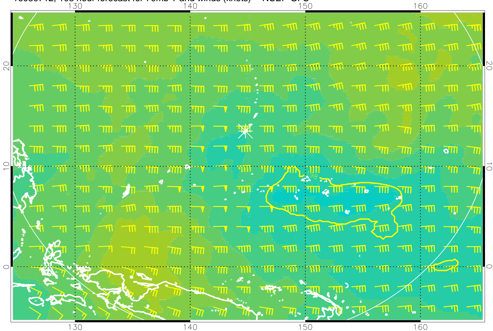
16080712, 108 hour forecast for 70mb T and winds (knots) -- NCEP GFS
