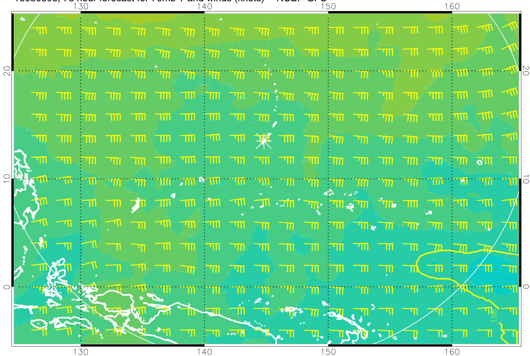
16080606, 78 hour forecast for 70mb T and winds (knots) -- NCEP GFS
