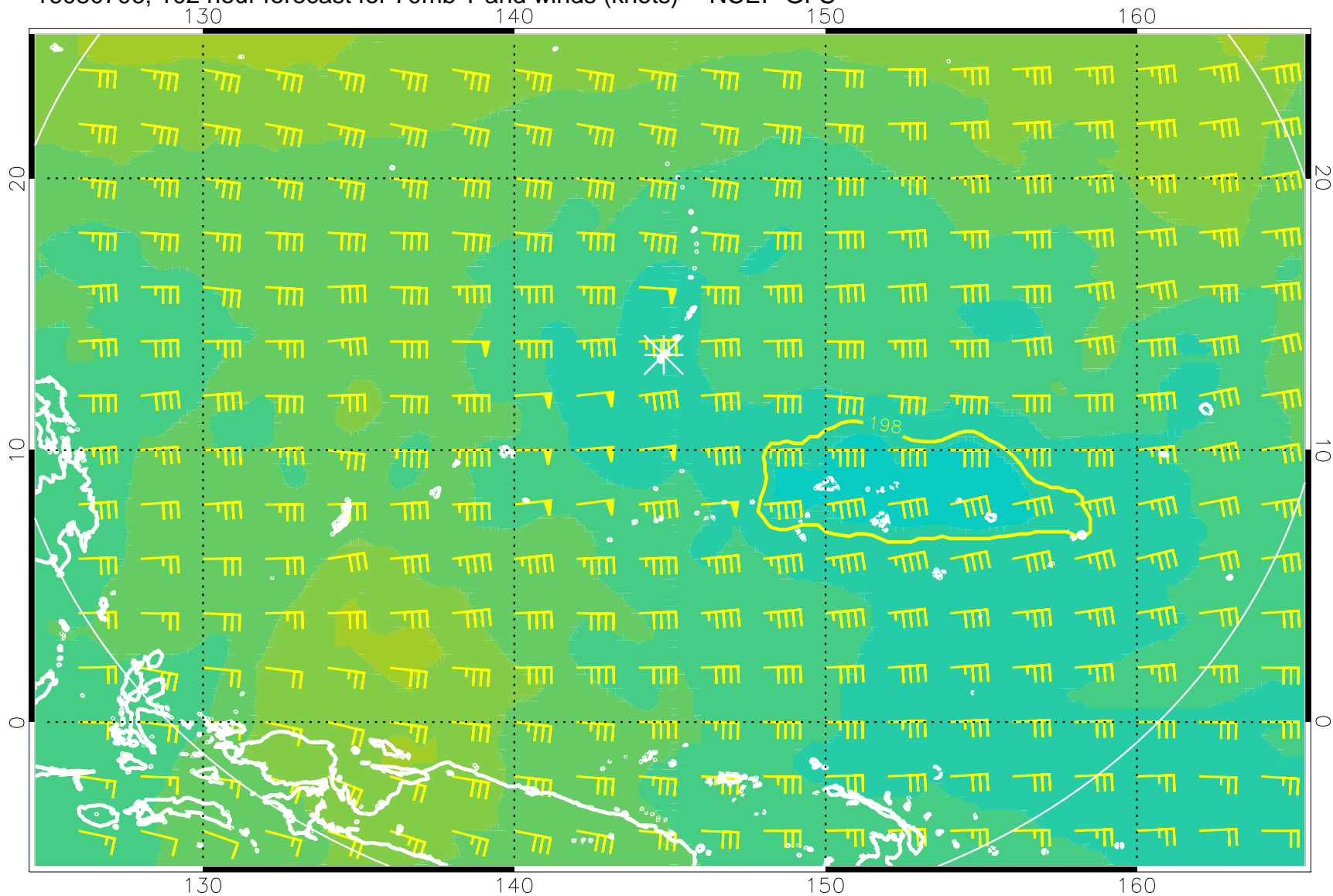
16080706, 102 hour forecast for 70mb T and winds (knots) -- NCEP GFS
