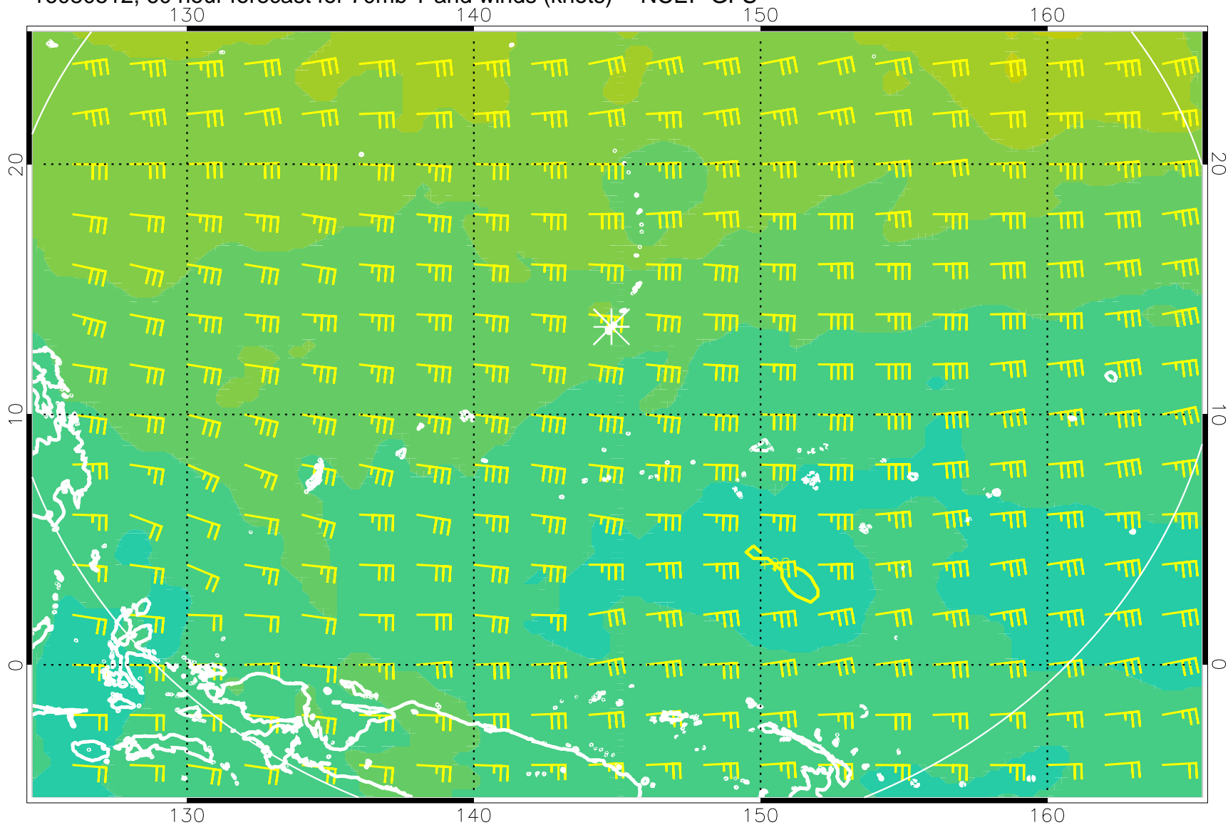
16080512, 60 hour forecast for 70mb T and winds (knots) -- NCEP GFS
