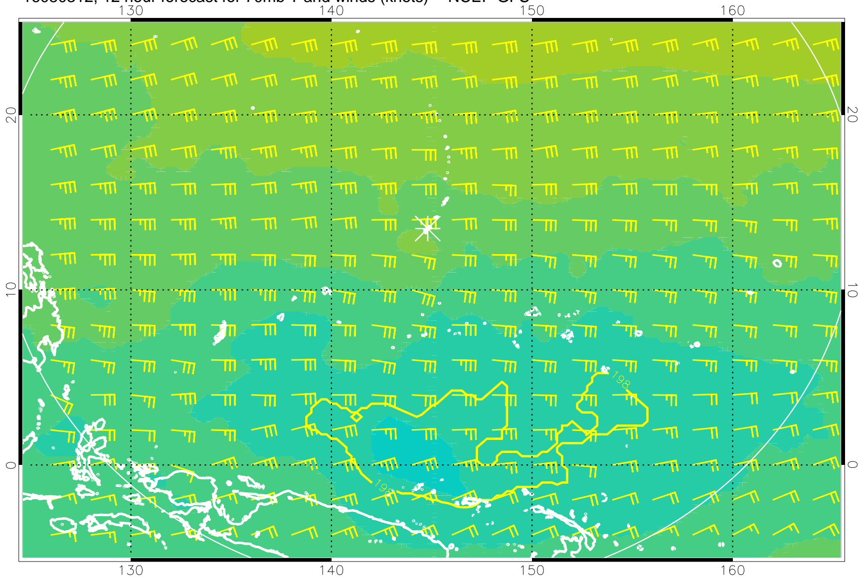
16080312, 12 hour forecast for 70mb T and winds (knots) -- NCEP GFS
