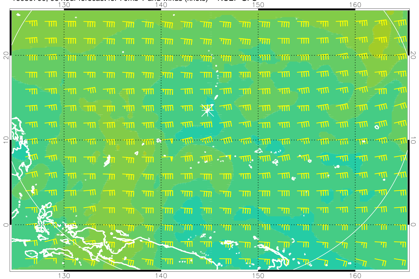
16080700, 96 hour forecast for 70mb T and winds (knots) -- NCEP GFS
