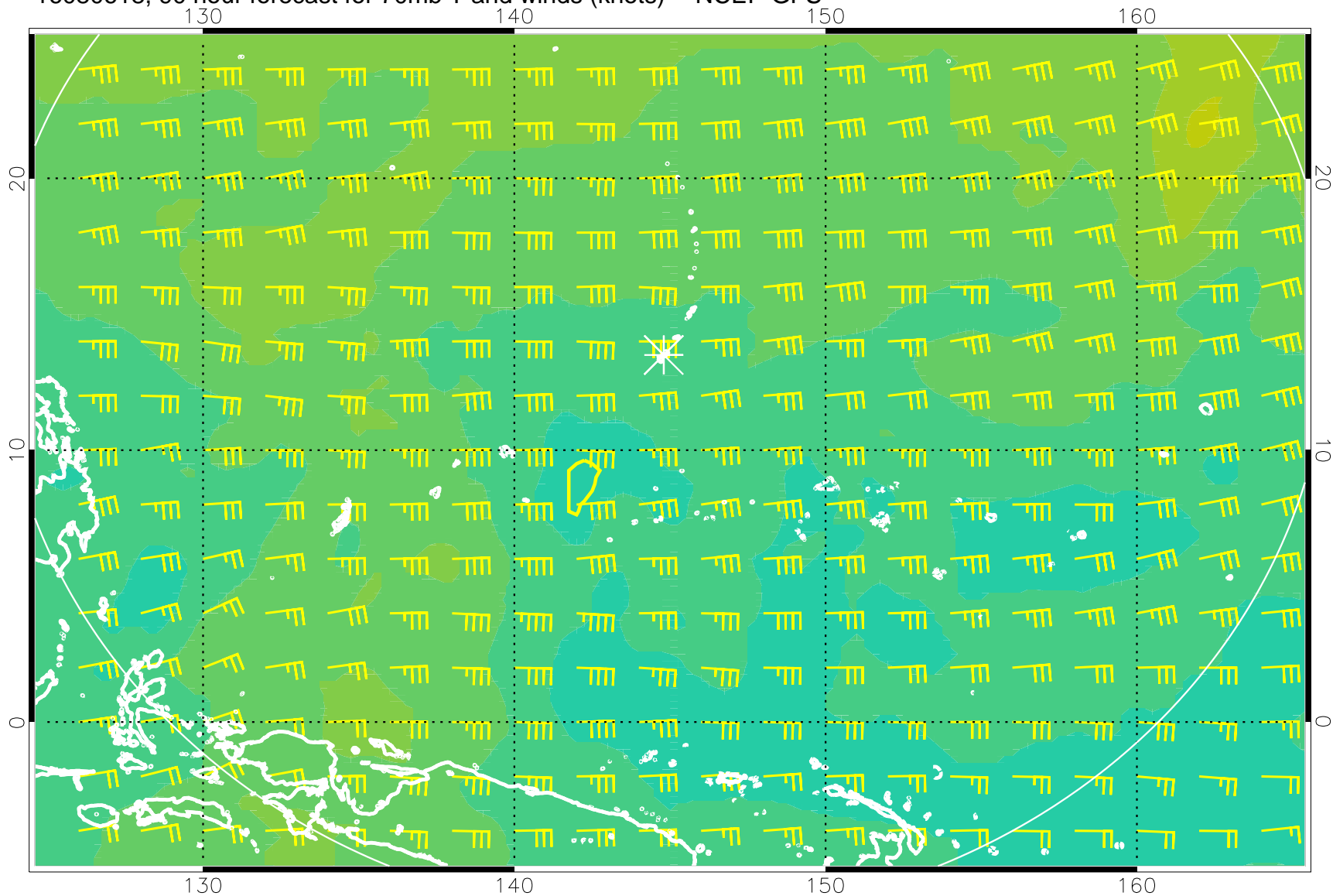
16080618, 90 hour forecast for 70mb T and winds (knots) -- NCEP GFS
