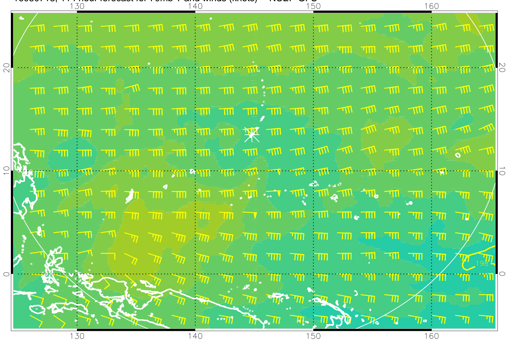
16080718, 114 hour forecast for 70mb T and winds (knots) -- NCEP GFS
