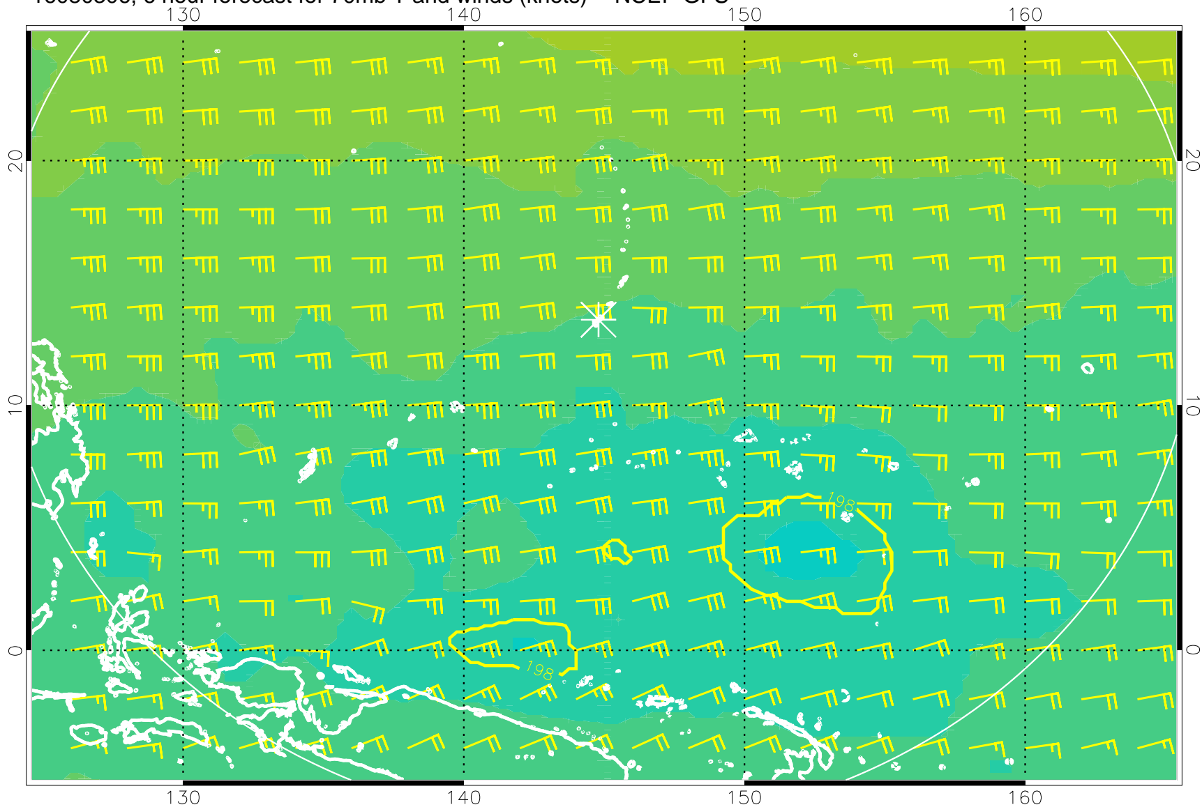
16080306, 6 hour forecast for 70mb T and winds (knots) -- NCEP GFS
