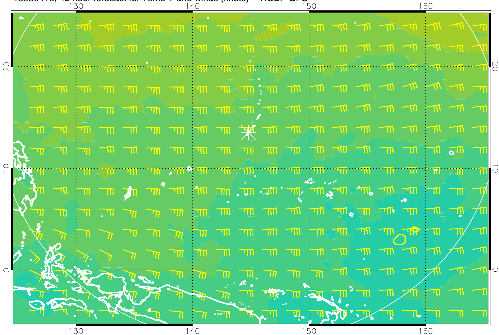
16080418, 42 hour forecast for 70mb T and winds (knots) -- NCEP GFS
