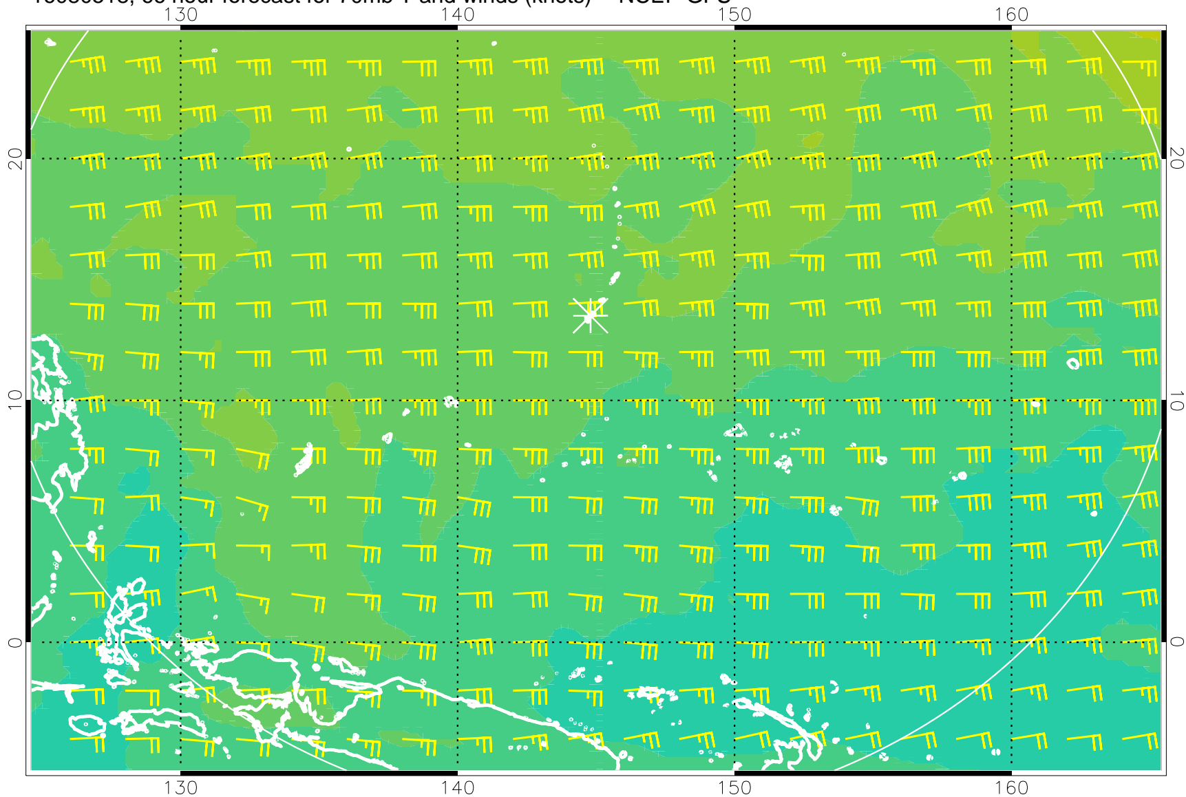
16080518, 66 hour forecast for 70mb T and winds (knots) -- NCEP GFS
