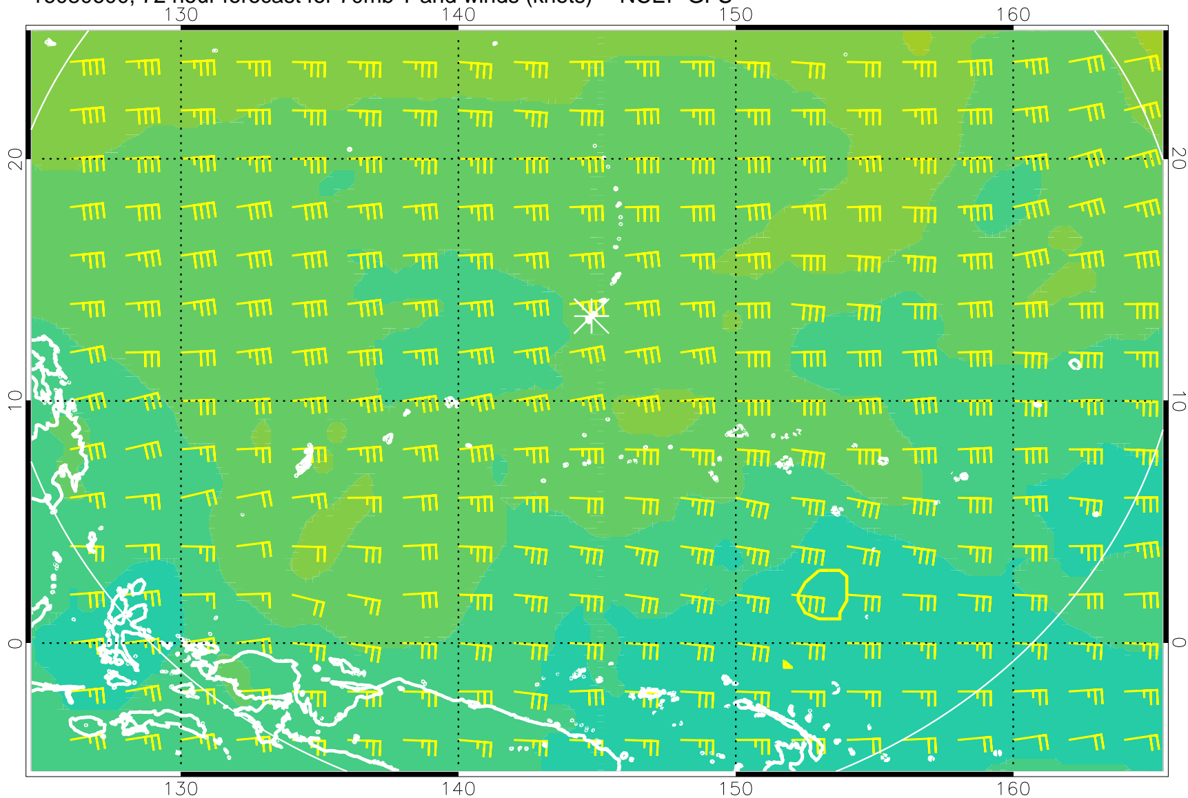
16080600, 72 hour forecast for 70mb T and winds (knots) -- NCEP GFS
