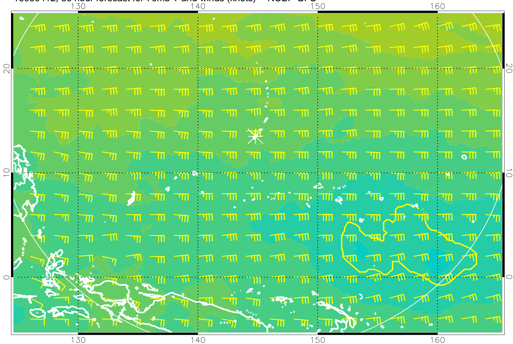
16080412, 36 hour forecast for 70mb T and winds (knots) -- NCEP GFS
