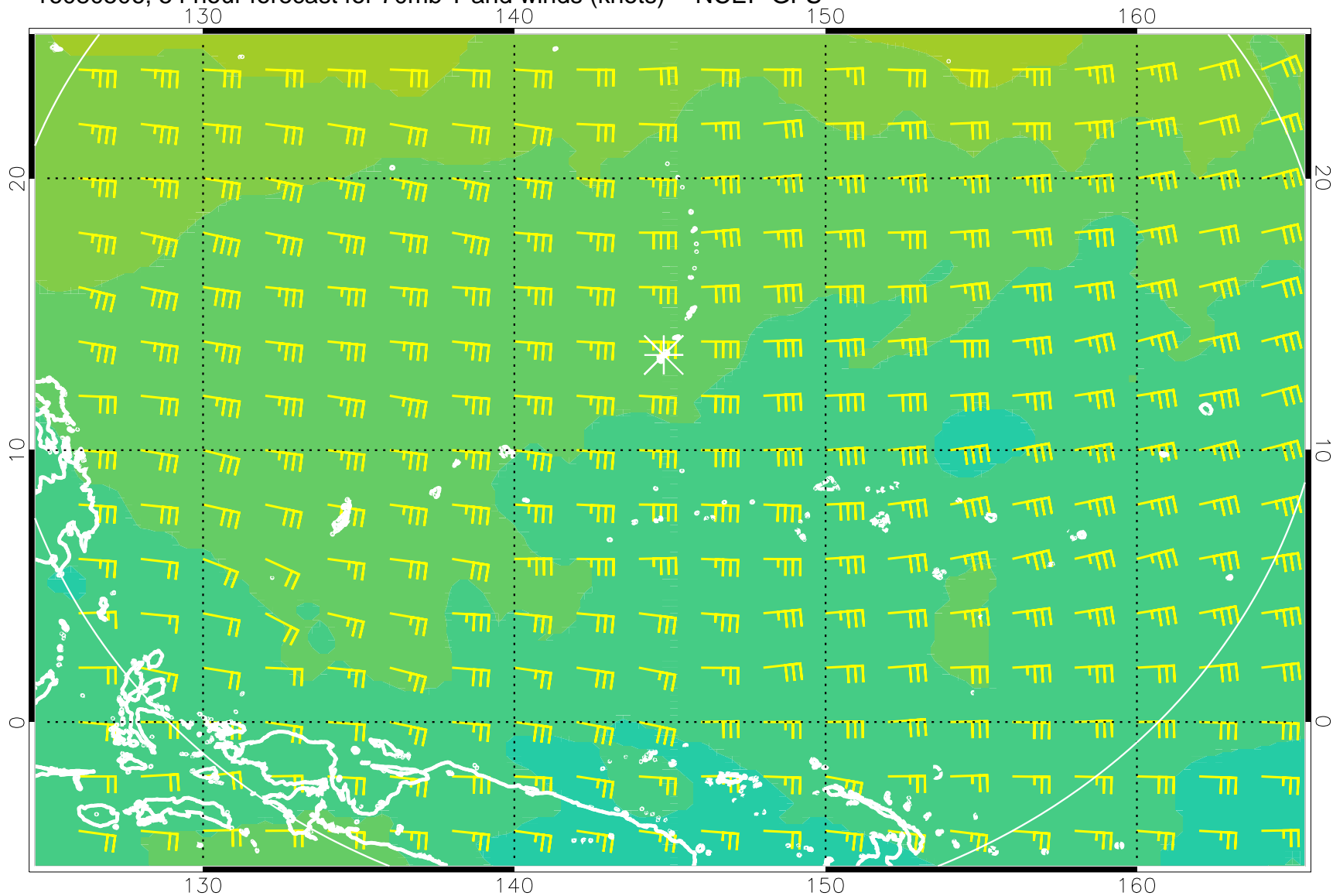
16080506, 54 hour forecast for 70mb T and winds (knots) -- NCEP GFS
