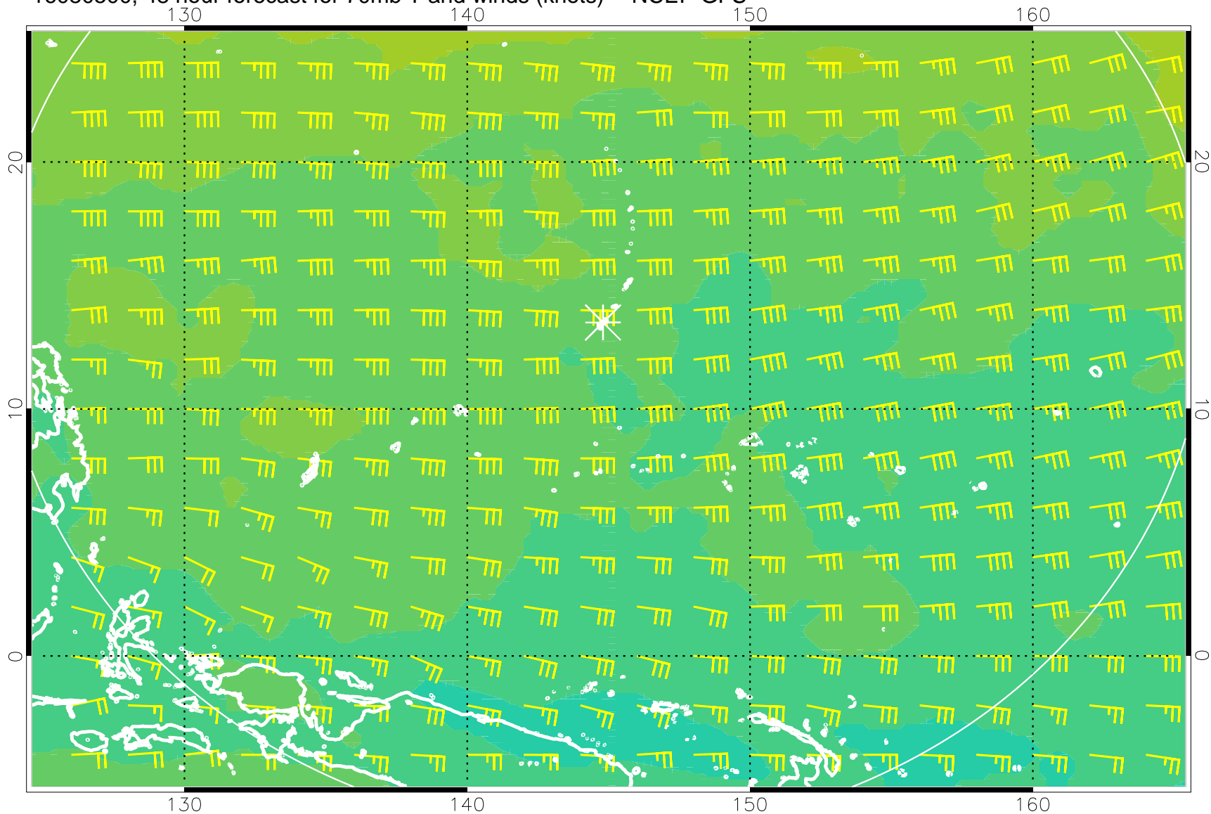
16080500, 48 hour forecast for 70mb T and winds (knots) -- NCEP GFS
