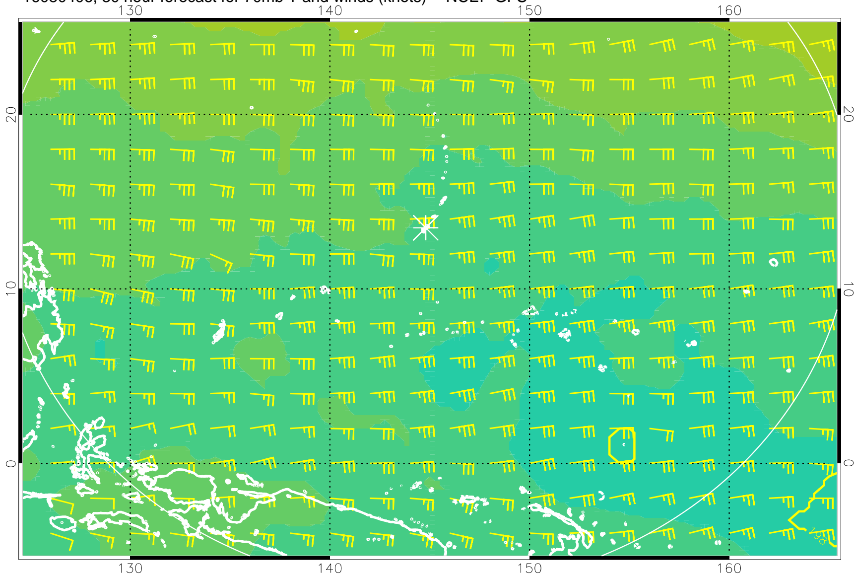
16080406, 30 hour forecast for 70mb T and winds (knots) -- NCEP GFS
