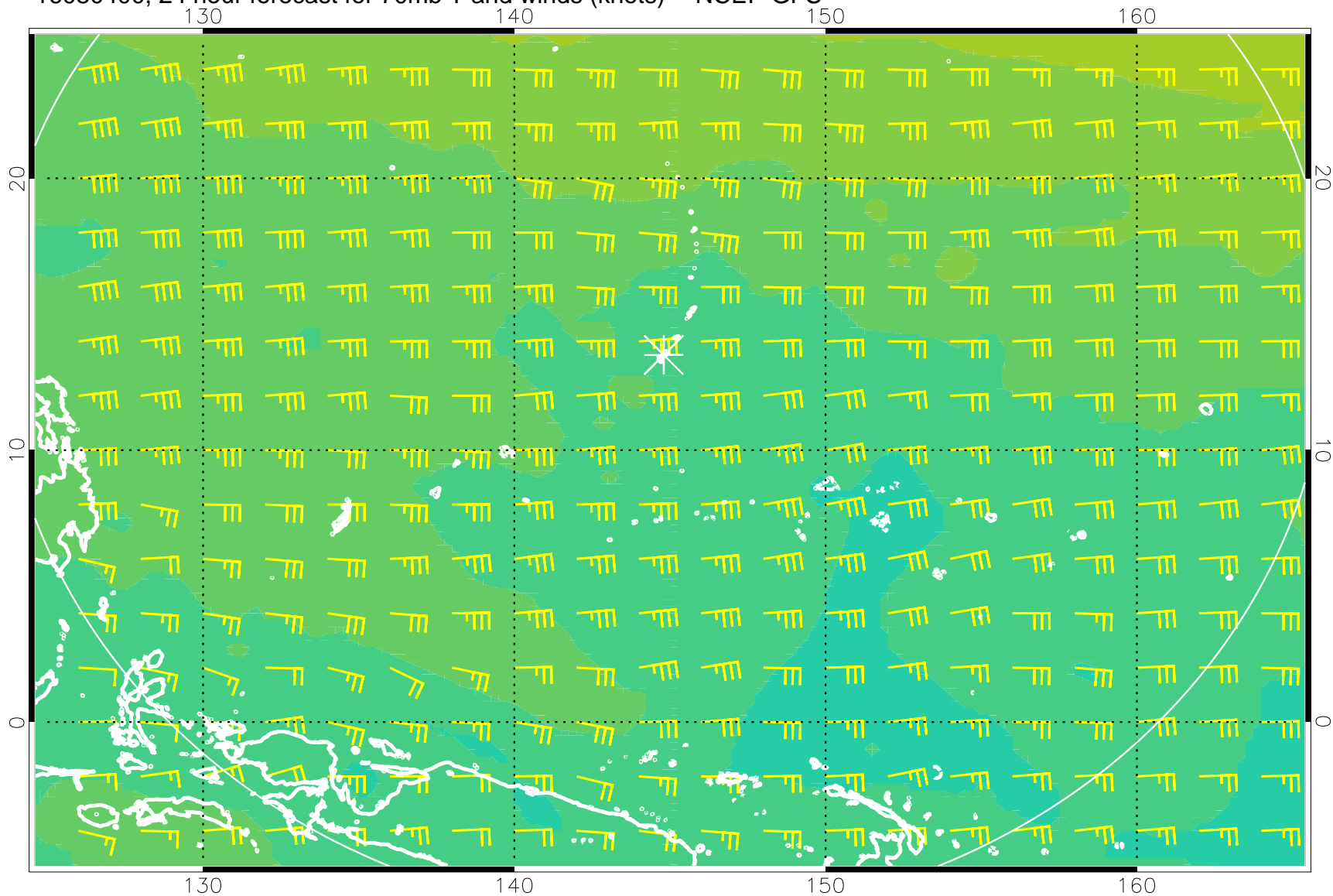
16080400, 24 hour forecast for 70mb T and winds (knots) -- NCEP GFS
