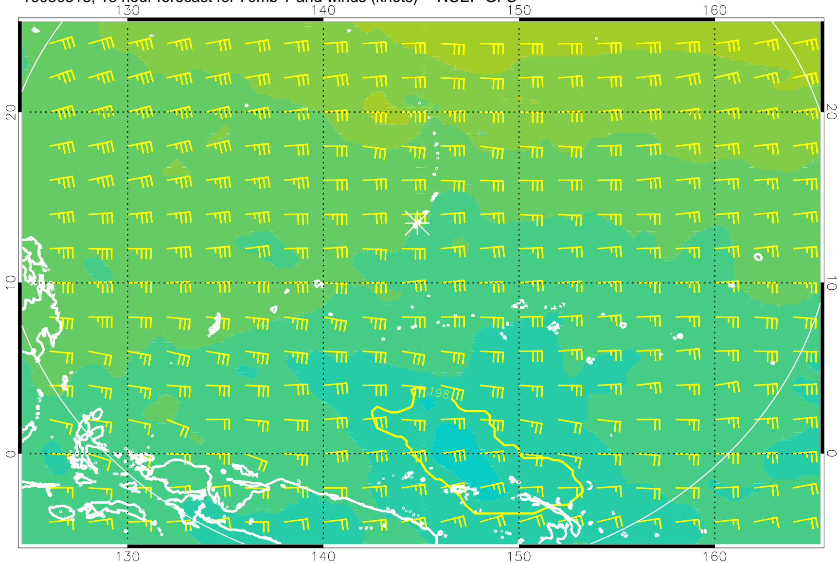
16080318, 18 hour forecast for 70mb T and winds (knots) -- NCEP GFS
