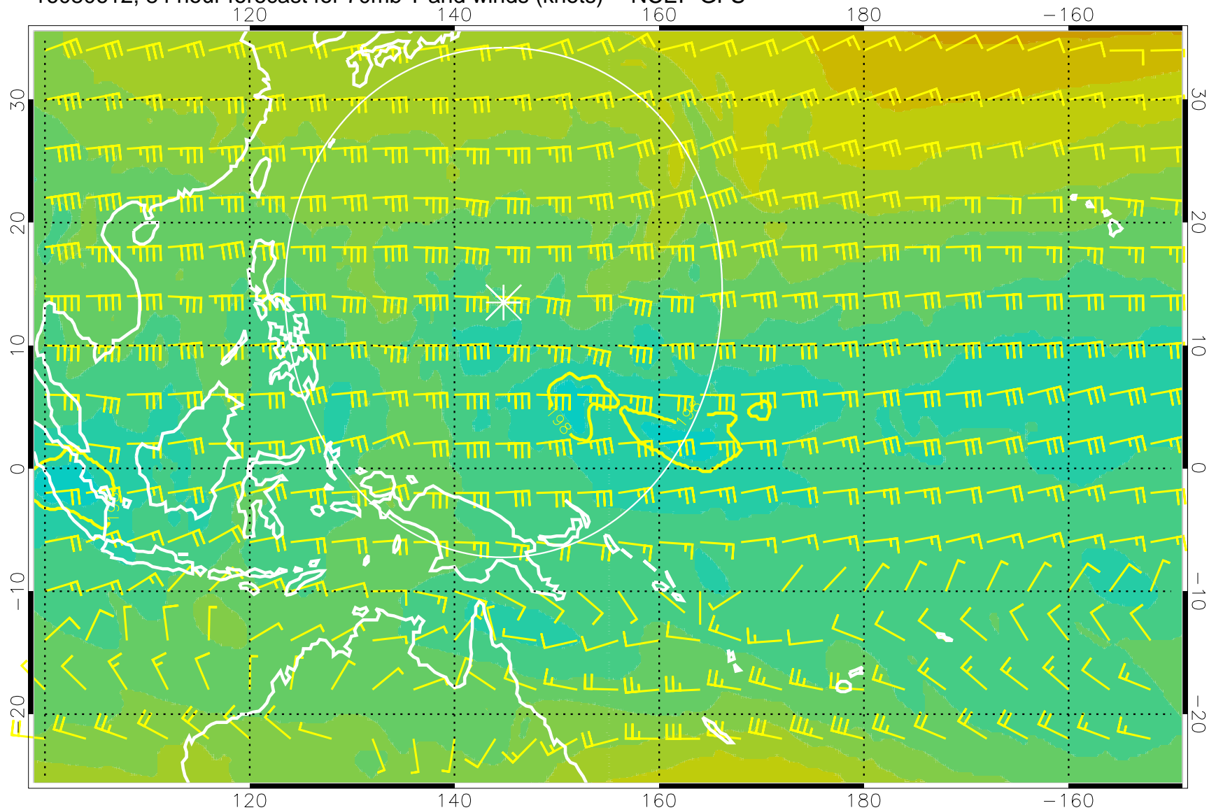
16080612, 84 hour forecast for 70mb T and winds (knots) -- NCEP GFS
