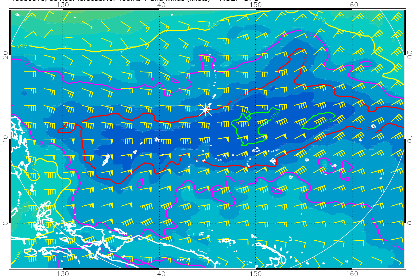
16080518, 66 hour forecast for 100mb T and winds (knots) -- NCEP GFS
