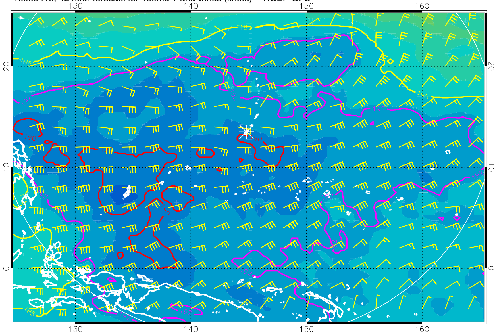
16080418, 42 hour forecast for 100mb T and winds (knots) -- NCEP GFS
