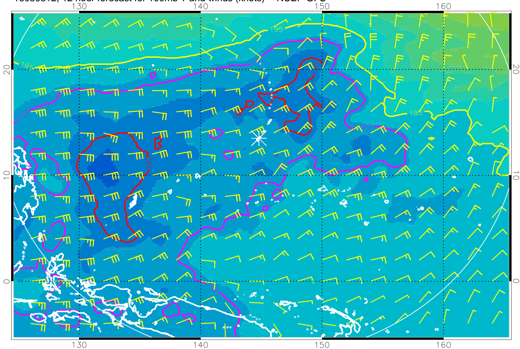
16080312, 12 hour forecast for 100mb T and winds (knots) -- NCEP GFS
