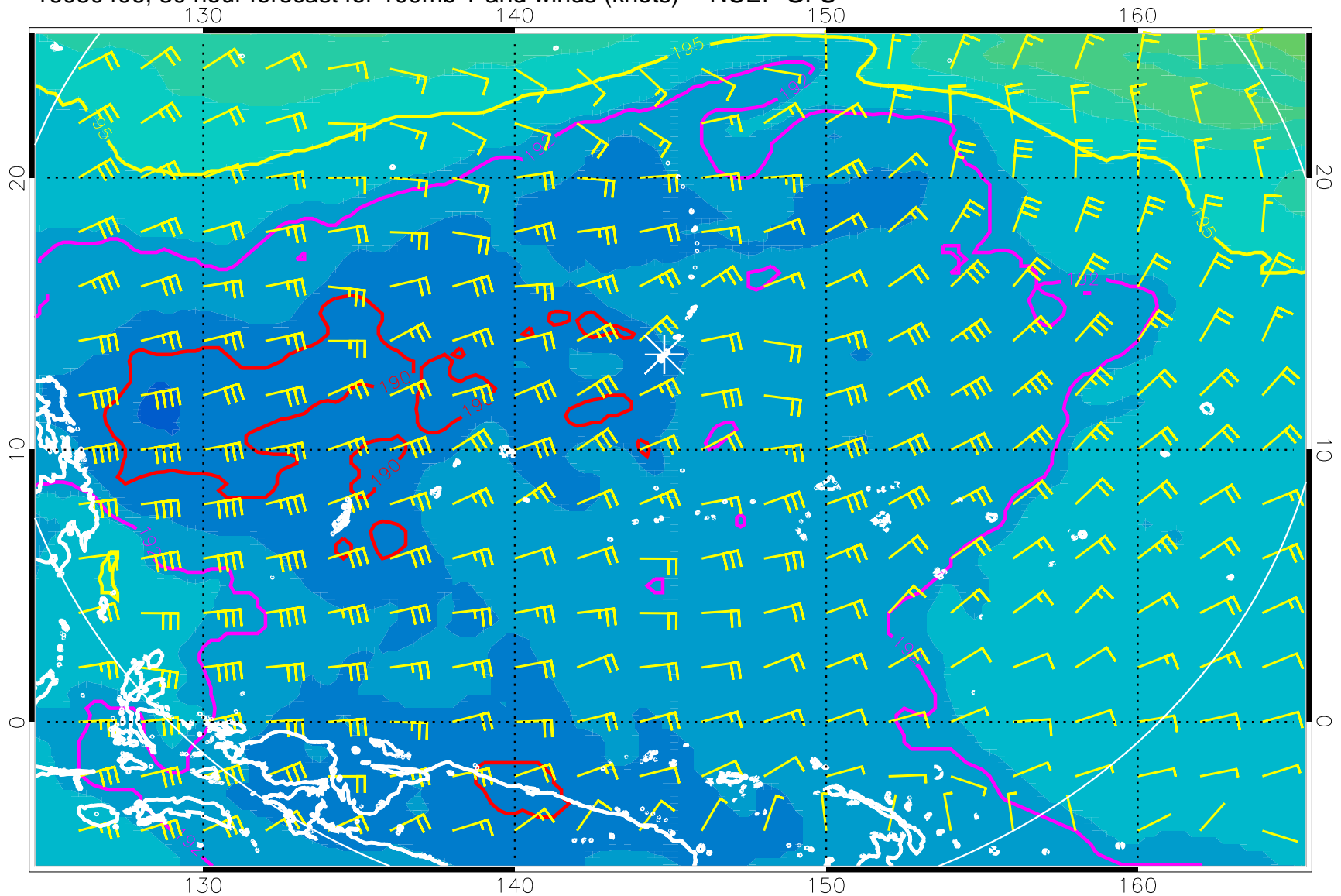
16080406, 30 hour forecast for 100mb T and winds (knots) -- NCEP GFS
