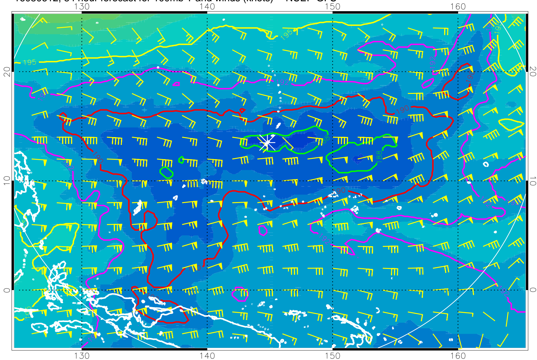
16080612, 84 hour forecast for 100mb T and winds (knots) -- NCEP GFS
