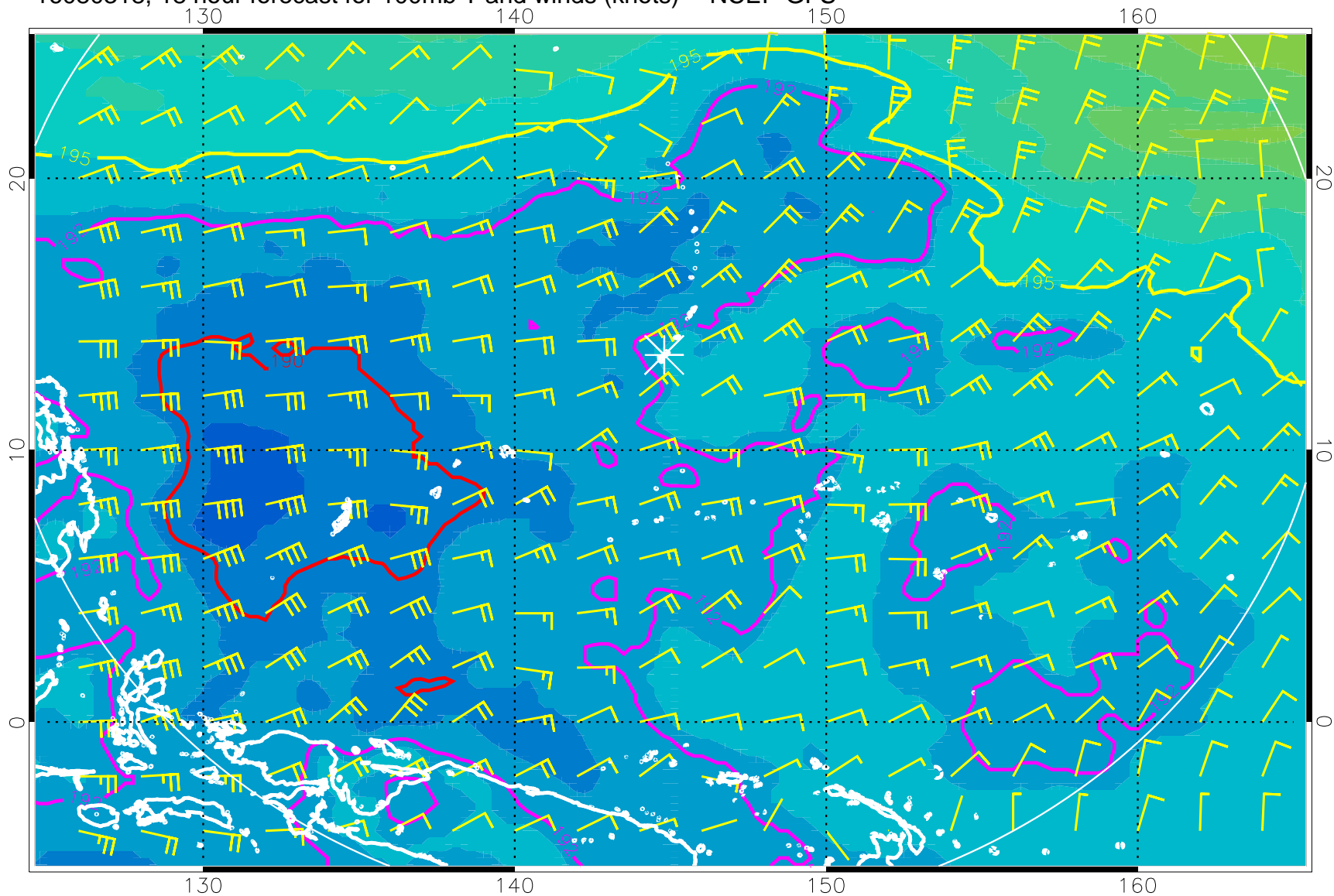
16080318, 18 hour forecast for 100mb T and winds (knots) -- NCEP GFS
