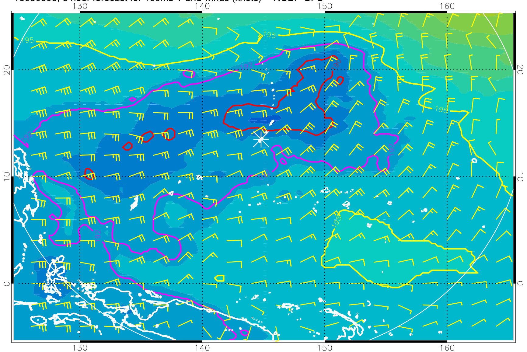
16080306, 6 hour forecast for 100mb T and winds (knots) -- NCEP GFS
