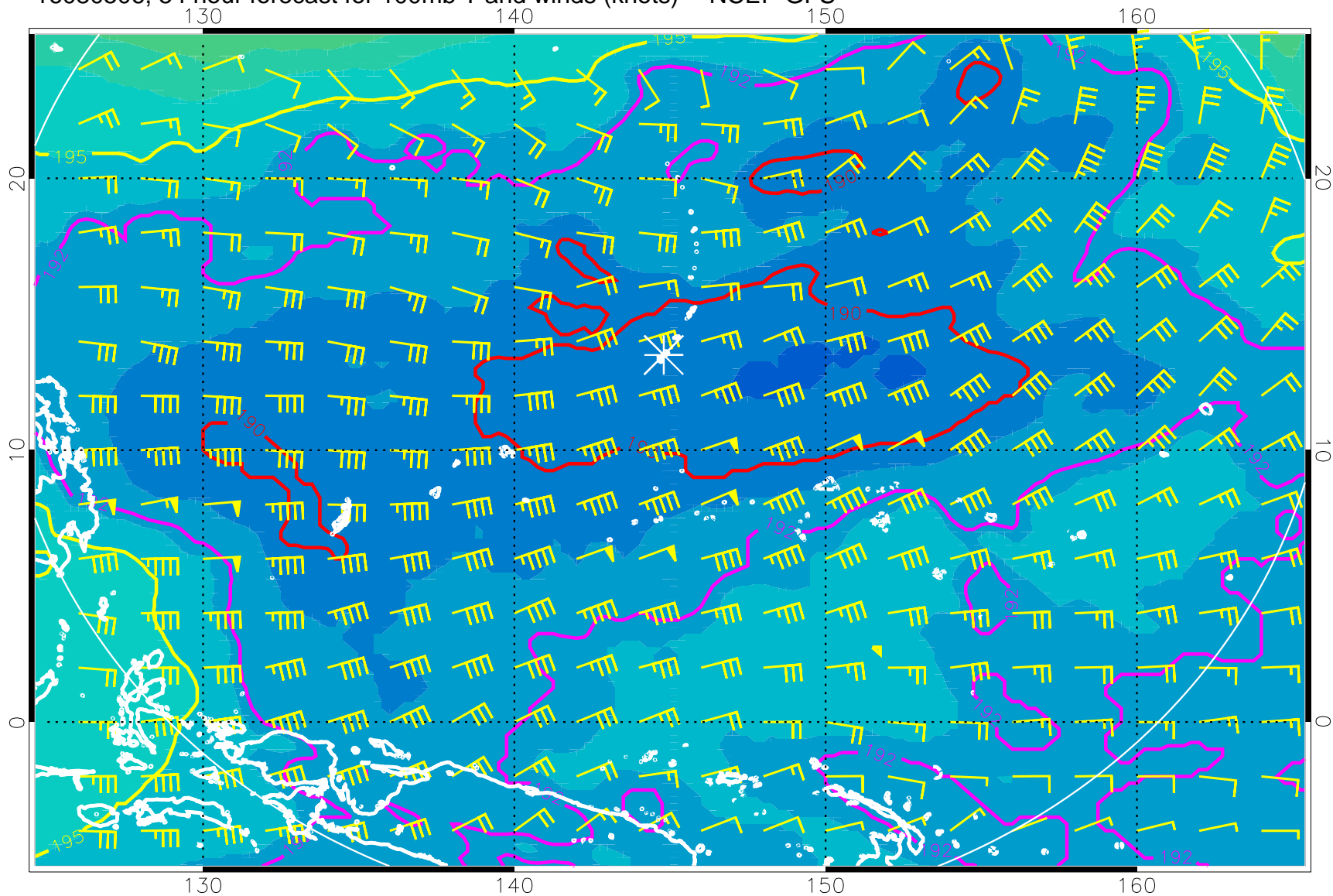
16080506, 54 hour forecast for 100mb T and winds (knots) -- NCEP GFS
