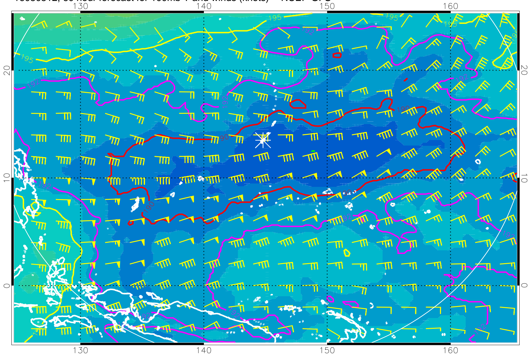
16080512, 60 hour forecast for 100mb T and winds (knots) -- NCEP GFS
