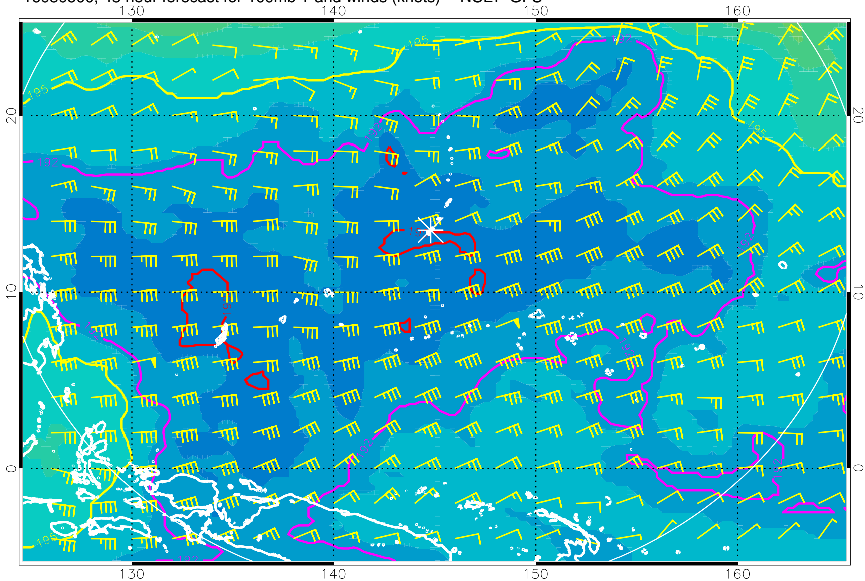
16080500, 48 hour forecast for 100mb T and winds (knots) -- NCEP GFS
