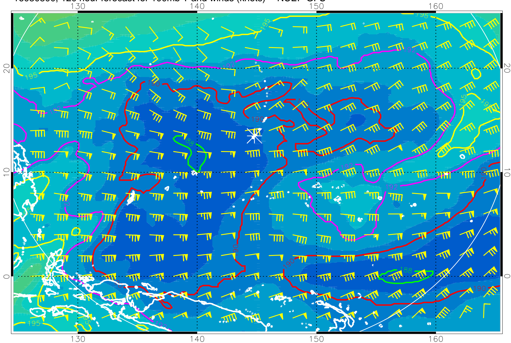
16080800, 120 hour forecast for 100mb T and winds (knots) -- NCEP GFS
