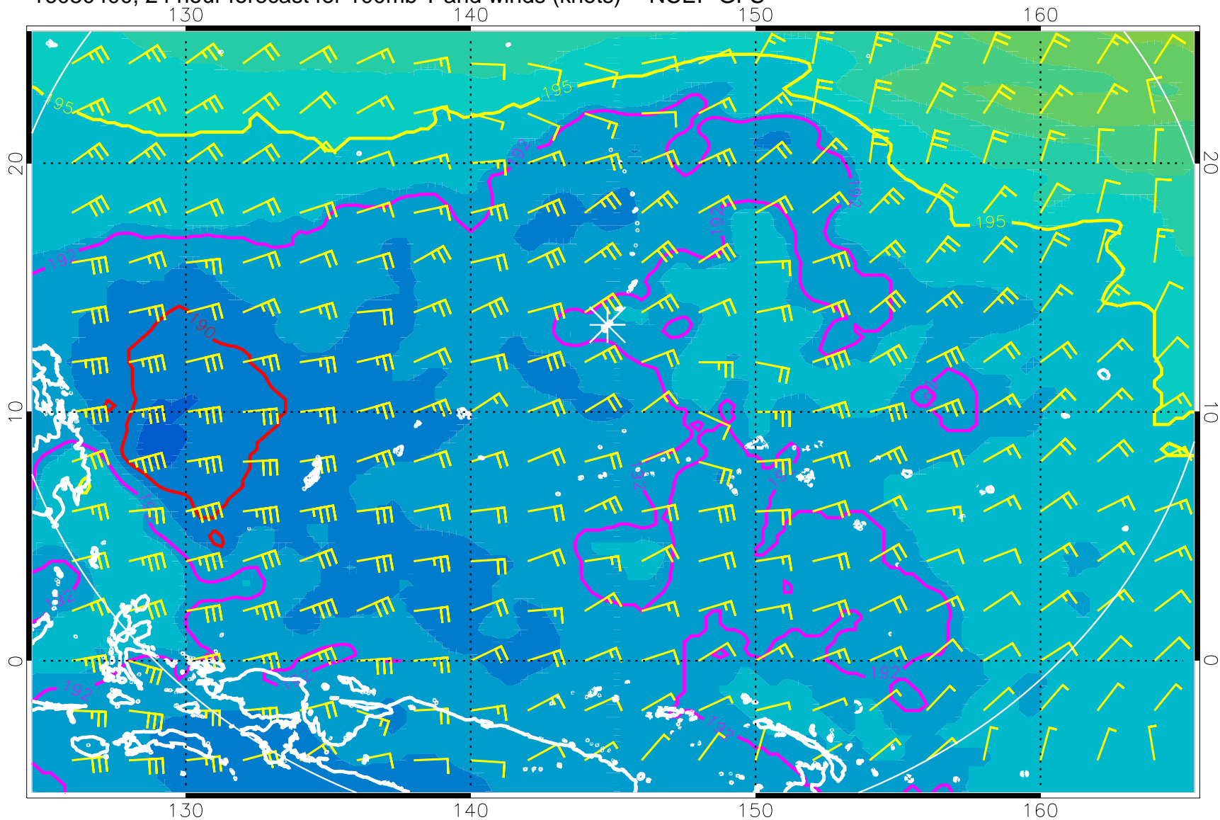
16080400, 24 hour forecast for 100mb T and winds (knots) -- NCEP GFS
