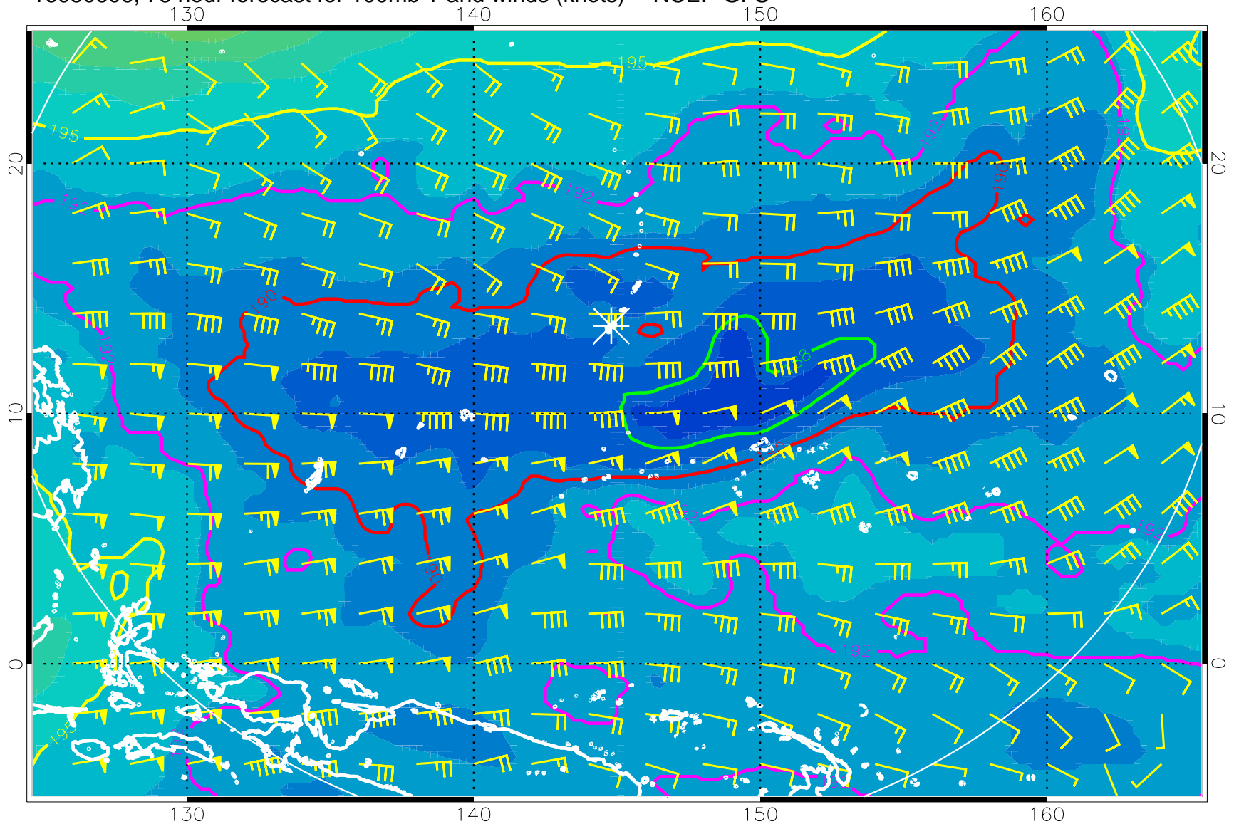
16080606, 78 hour forecast for 100mb T and winds (knots) -- NCEP GFS
