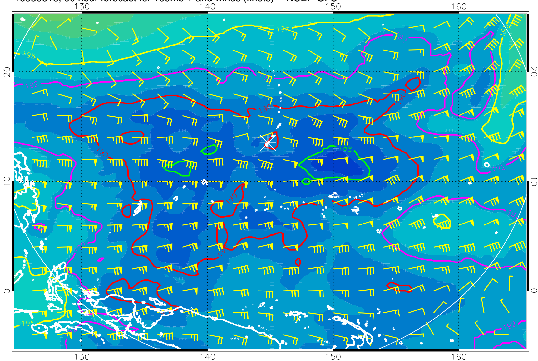
16080618, 90 hour forecast for 100mb T and winds (knots) -- NCEP GFS
