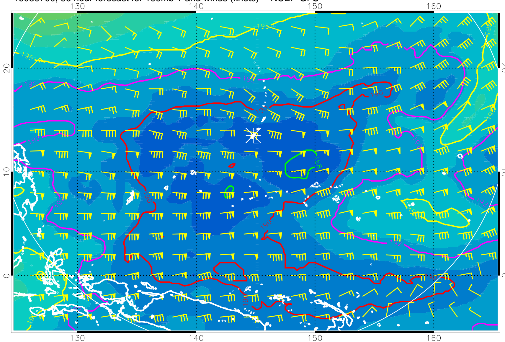
16080700, 96 hour forecast for 100mb T and winds (knots) -- NCEP GFS
