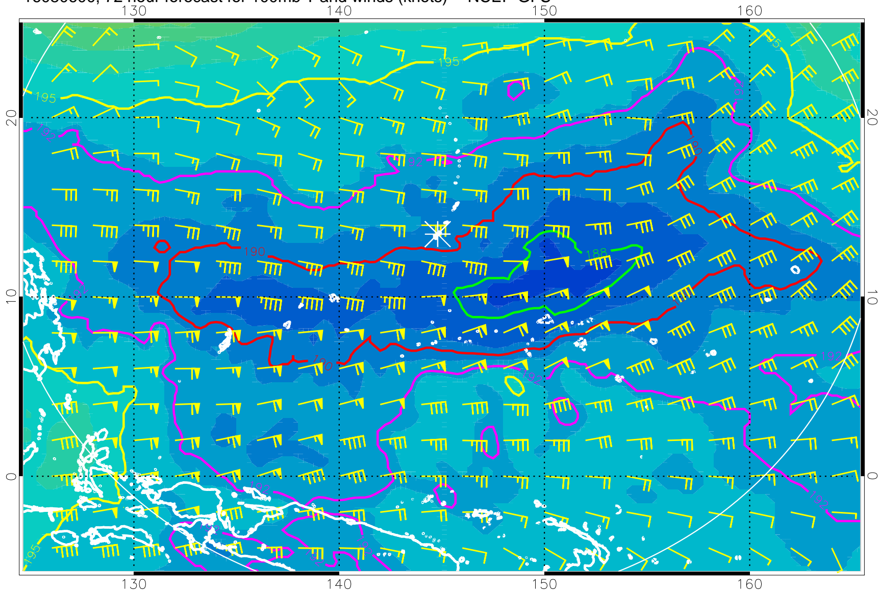
16080600, 72 hour forecast for 100mb T and winds (knots) -- NCEP GFS
