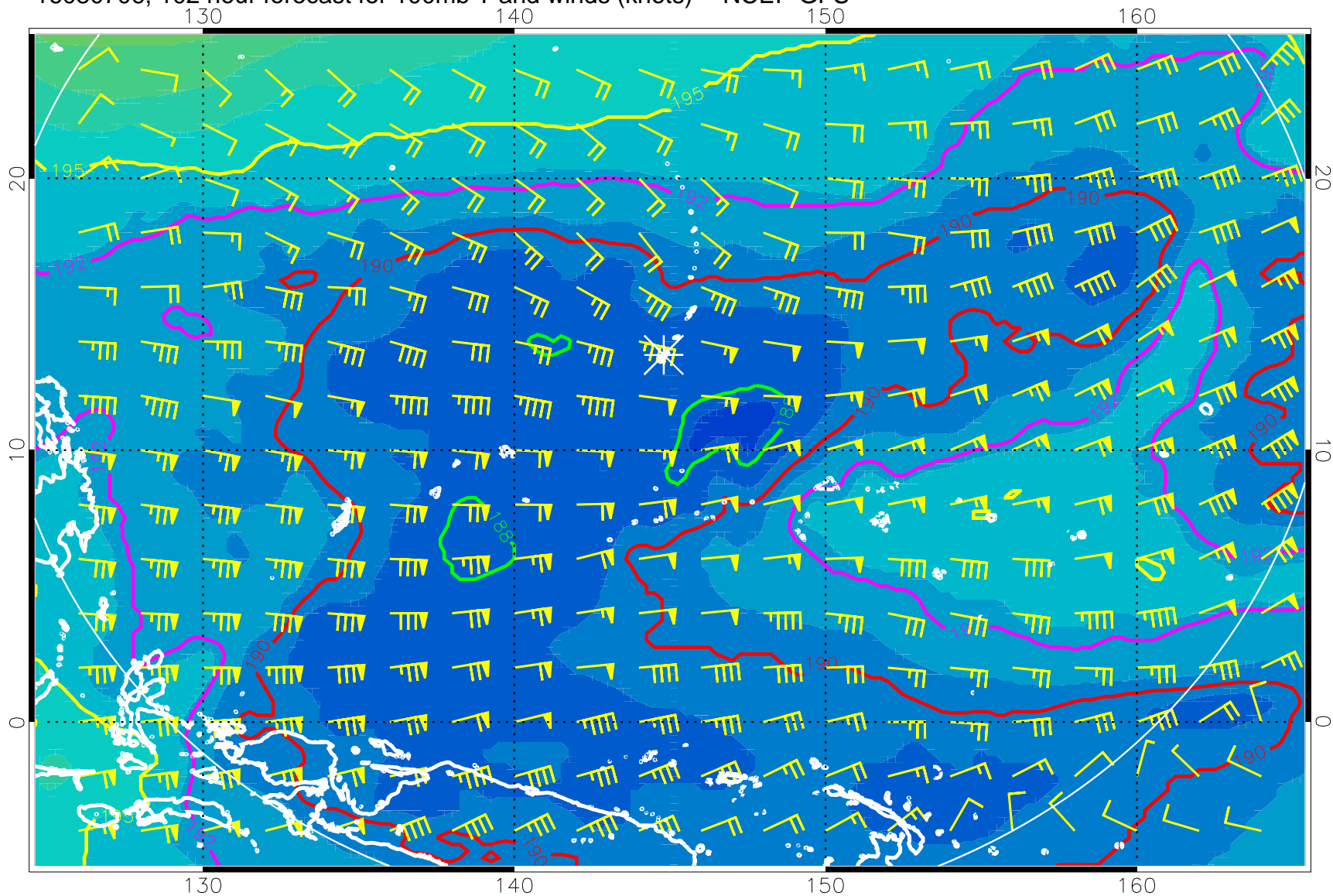
16080706, 102 hour forecast for 100mb T and winds (knots) -- NCEP GFS
