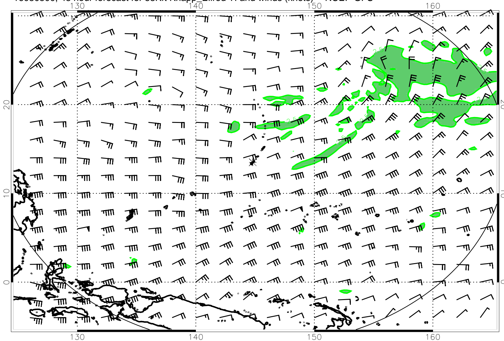
16080500, 48 hour forecast for 53Kft Knapp_Ellrod TI and winds (knots) -- NCEP GFS
