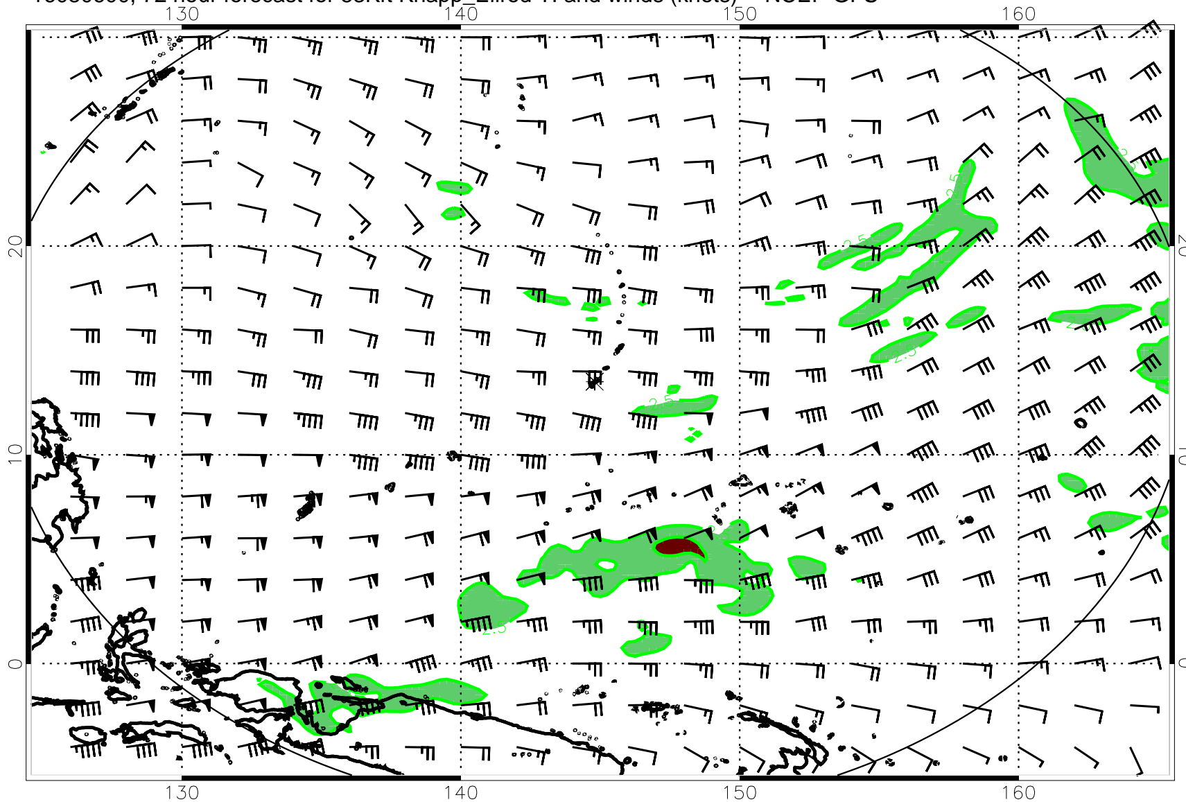
16080600, 72 hour forecast for 53Kft Knapp_Ellrod TI and winds (knots) -- NCEP GFS
