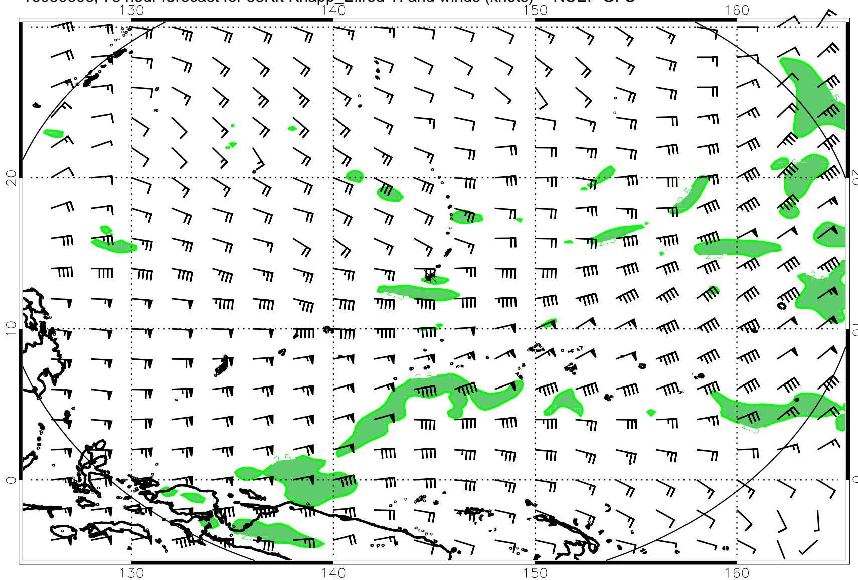
16080606, 78 hour forecast for 53Kft Knapp_Ellrod TI and winds (knots) -- NCEP GFS
