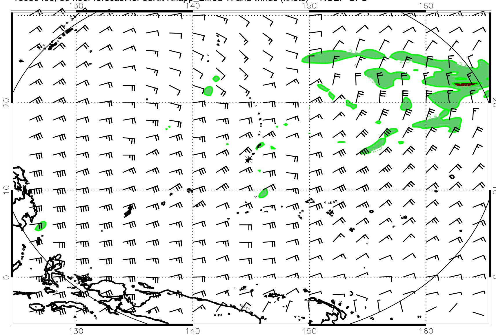
16080406, 30 hour forecast for 53Kft Knapp_Ellrod TI and winds (knots) -- NCEP GFS
